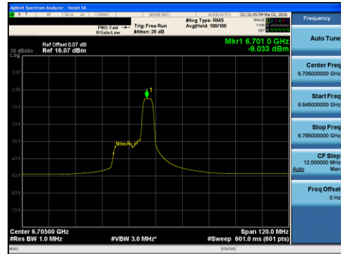
Plot 7-87 PSD Antenna 1 (80MHz BW 802.11ax(RU) RU52 Index44 - Ch.151)
