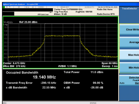
Plot 7-34 26dB BW & 99% OBW Antenna 1 (20MHz BW 802.11ax(RU) RU242 Index61 - Ch.105)
