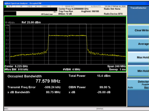
Plot 7-6 26dB BW & 99% OBW Antenna 0 (80MHz BW 802.11ax(RU) RU996 Index67 - Ch.55)
