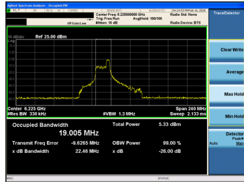
Plot 7-3 26dB BW & 99% OBW Antenna 0 (80MHz BW 802.11ax(RU) RU52 Index44 - Ch.55)
