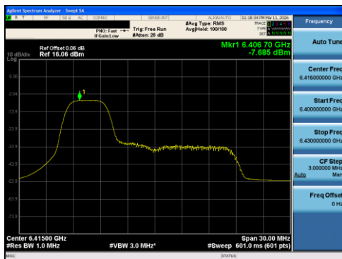
Plot 7-49 PSD Antenna 0 (20MHz BW 802.11ax(RU) RU52 Index37 - Ch.93)
