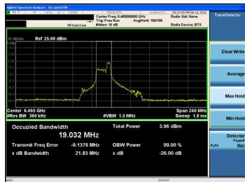
Plot 7-9 26dB BW & 99% OBW Antenna 0 (80MHz BW 802.11ax(RU) RU52 Index44 - Ch.103)
