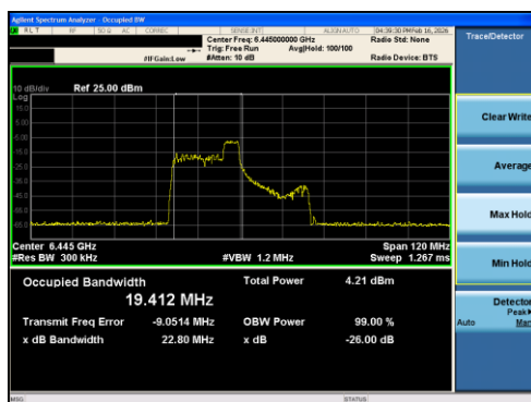
Plot 7-8 26dB BW & 99% OBW Antenna 0 (40MHz BW 802.11ax(RU) RU52 Index40 - Ch.99)
