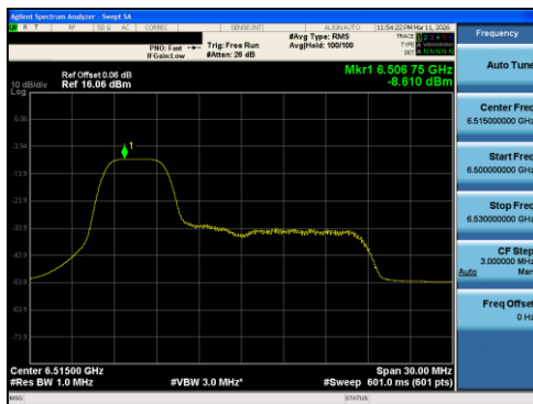
Plot 7-55 PSD Antenna 0 (20MHz BW 802.11ax(RU) RU52 Index37 - Ch.113)
