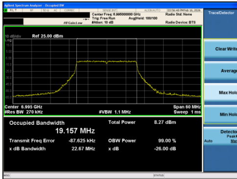
Plot 7-22 26dB BW & 99% OBW Antenna 0 (20MHz BW 802.11ax(RU) RU242 Index61 - Ch.209)
