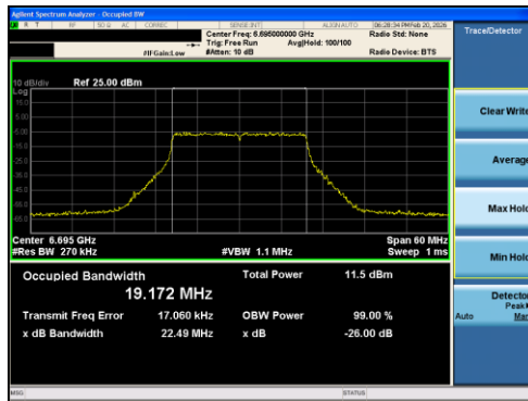
Plot 7-40 26dB BW & 99% OBW Antenna 1 (20MHz BW 802.11ax(RU) RU242 Index61 - Ch.149)
