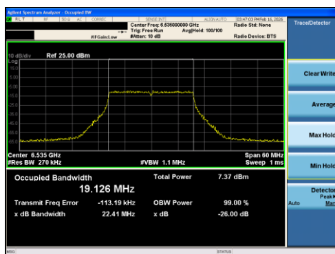
Plot 7-16 26dB BW & 99% OBW Antenna 0 (20MHz BW 802.11ax(RU) RU242 Index61 - Ch.117)
