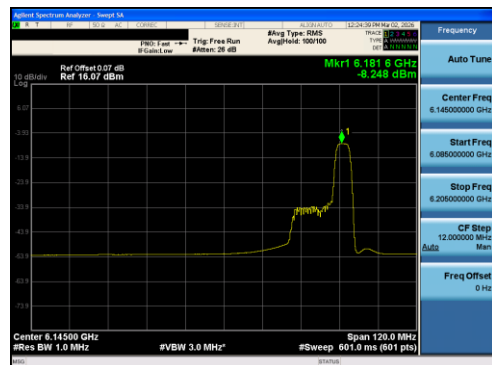
Plot 7-75 PSD Antenna 1 (80MHz BW 802.11ax(RU) RU52 Index52 - Ch.39)
