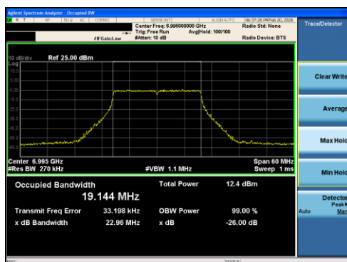
Plot 7-47 26dB BW & 99% OBW Antenna 1 (20MHz BW 802.11ax(RU) RU242 Index61 - Ch.209)
