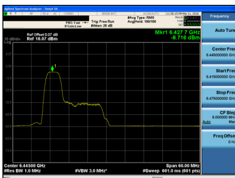
Plot 7-56 PSD Antenna 0 (40MHz BW 802.11ax(RU) RU52 Index37 - Ch.99)
