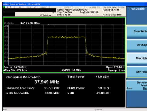
Plot 7-41 26dB BW & 99% OBW Antenna 1 (40MHz BW 802.11ax(RU) RU484 Index65 - Ch.155)
