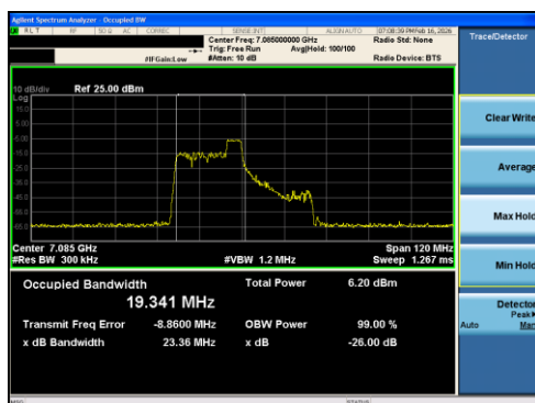
Plot 7-20 26dB BW & 99% OBW Antenna 0 (40MHz BW 802.11ax(RU) RU52 Index40 - Ch.227)
