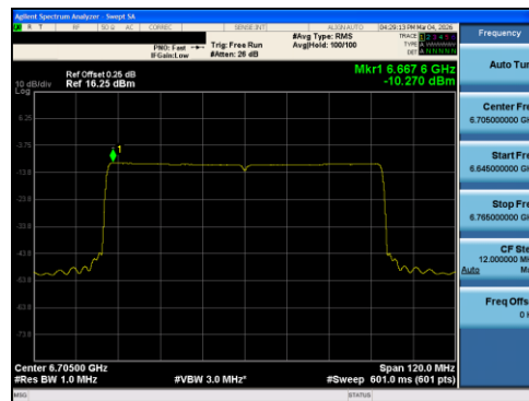
Plot 7-66 PSD Antenna 0 (80MHz BW 802.11ax(RU) RU996 Index67 - Ch.151)
