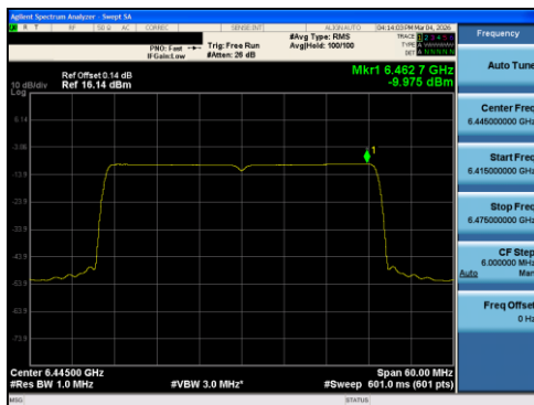
Plot 7-59 PSD Antenna 0 (40MHz BW 802.11ax(RU) RU484 Index65 - Ch.99)
