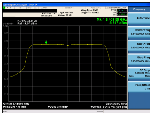
Plot 7-76 PSD Antenna 1 (20MHz BW 802.11ax(RU) RU242 Index61 - Ch.93)
