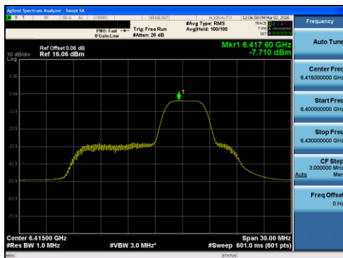
Plot 7-73 PSD Antenna 1 (20MHz BW 802.11ax(RU) RU52 Index39 - Ch.93)
