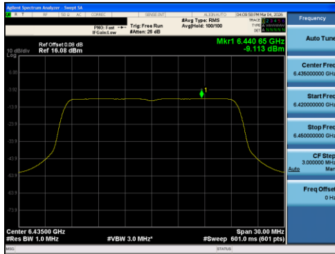
Plot 7-58 PSD Antenna 0 (20MHz BW 802.11ax(RU) RU242 Index61 - Ch.97)
