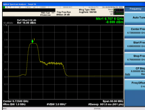
Plot 7-86 PSD Antenna 1 (40MHz BW 802.11ax(RU) RU52 Index37 - Ch.155)
