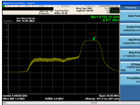
Plot 7-85 PSD Antenna 1 (20MHz BW 802.11ax(RU) RU52 Index40 - Ch.149)
