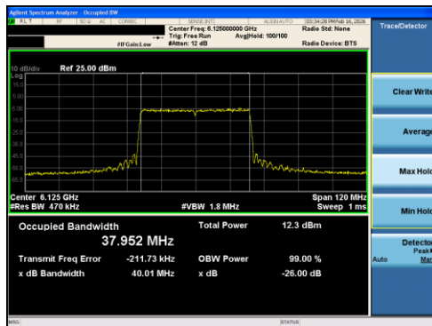
Plot 7-5 26dB BW & 99% OBW Antenna 0 (40MHz BW 802.11ax(RU) RU484 Index65 - Ch.35)
