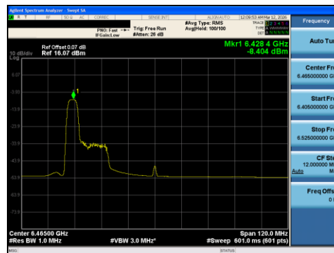
Plot 7-57 PSD Antenna 0 (80Mhz BW 802.11ax(RU) RU52 Index37 - Ch.103)
