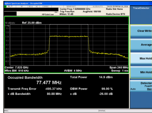
Plot 7-24 26dB BW & 99% OBW Antenna 0 (80MHz BW 802.11ax(RU) RU996 Index67 - Ch.215)
