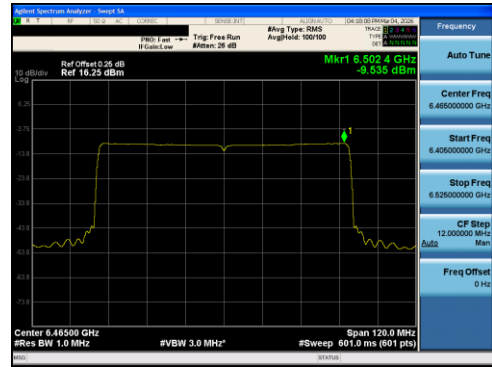
Plot 7-60 PSD Antenna 0 (80MHz BW 802.11ax(RU) RU996 Index67 - Ch.103)
