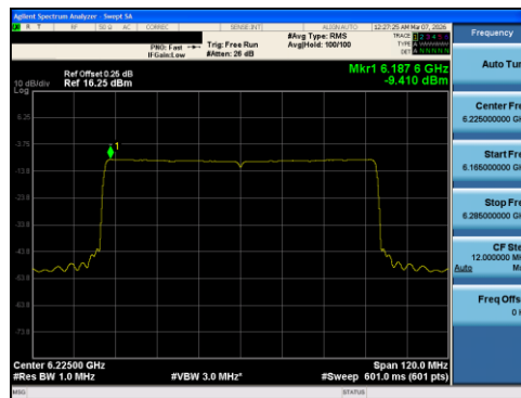
Plot 7-54 PSD Antenna 0 (80MHz BW 802.11ax(RU) RU996 Index67 - Ch.55)
