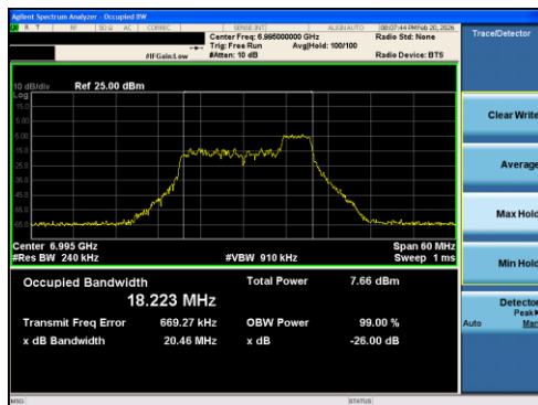
Plot 7-43 26dB BW & 99% OBW Antenna 1 (20MHz BW 802.11ax(RU) RU52 Index40 - Ch.209)
