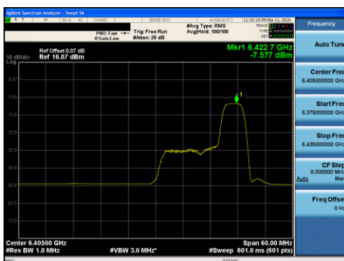
Plot 7-50 PSD Antenna 0 (40MHz BW 802.11ax(RU) RU52 Index44 - Ch.91)
