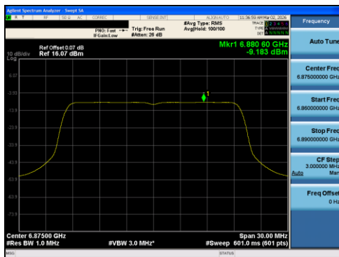
Plot 7-88 PSD Antenna 1 (20MHz BW 802.11ax(RU) RU242 Index61 - Ch.185)
