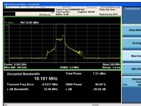
Plot 7-39 26dB BW & 99% OBW Antenna 1 (80MHz BW 802.11ax(RU) RU52 Index44 - Ch.119)
