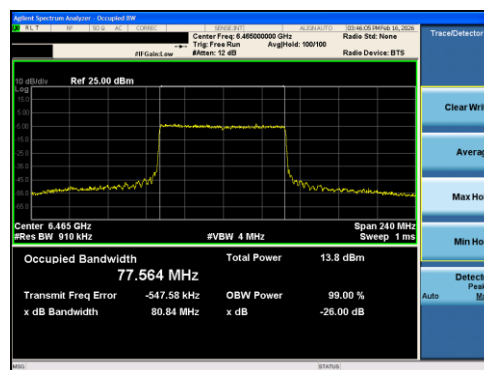
Plot 7-12 26dB BW & 99% OBW Antenna 0 (80MHz BW 802.11ax(RU) RU996 Index67 - Ch.103)
