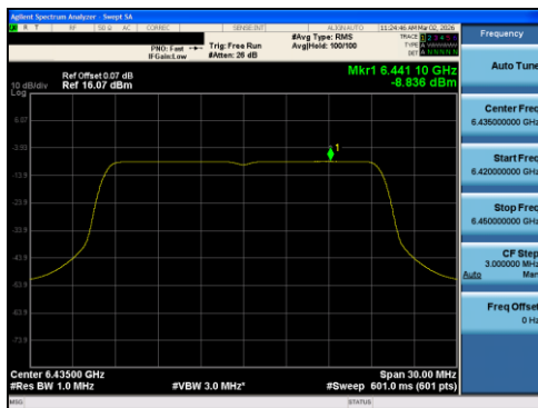
Plot 7-82 PSD Antenna 1 (20MHz BW 802.11ax(RU) RU242 Index61 - Ch.97)
