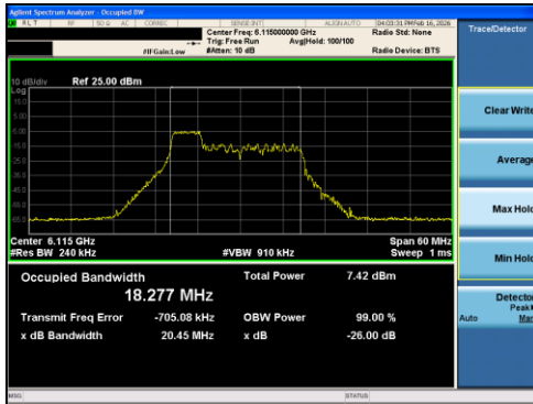
Plot 7-1 26dB BW & 99% OBW Antenna 0 (20MHz BW 802.11ax(RU) RU52 Index37 - Ch.33)
