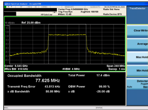
Plot 7-42 26dB BW & 99% OBW Antenna 1 (80MHz BW 802.11ax(RU) RU996 Index67 - Ch.119)
