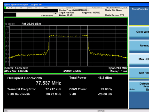
Plot 7-36 26dB BW & 99% OBW Antenna 1 (80Mhz BW 802.11ax(RU) RU996 Index67 - Ch.103)
