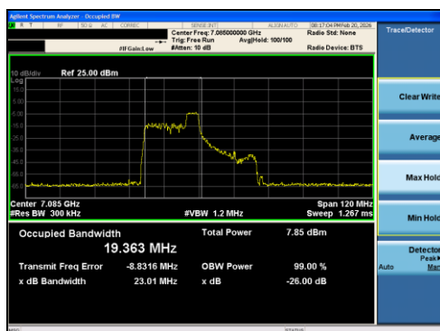
Plot 7-44 26dB BW & 99% OBW Antenna 1 (40MHz BW 802.11ax(RU) RU52 Index40 - Ch.227)
