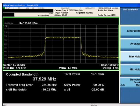
Plot 7-17 26dB BW & 99% OBW Antenna 0 (40MHz BW 802.11ax(RU) RU484 Index65 - Ch.155)
