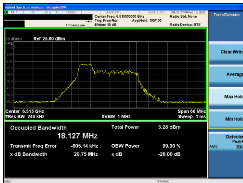
Plot 7-7 26dB BW & 99% OBW Antenna 0 (20MHz BW 802.11ax(RU) RU52 Index37 - Ch.113)
