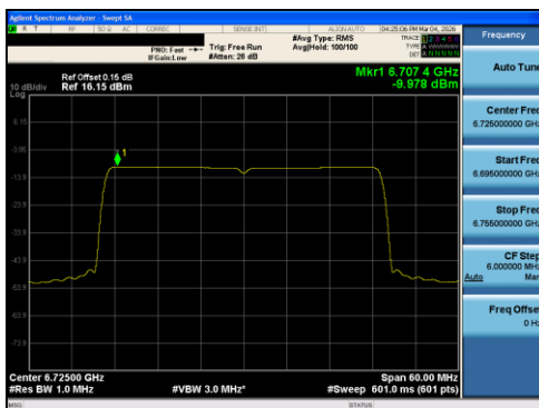
Plot 7-65 PSD Antenna 0 (40MHz BW 802.11ax(RU) RU484 Index65 - Ch.155)
