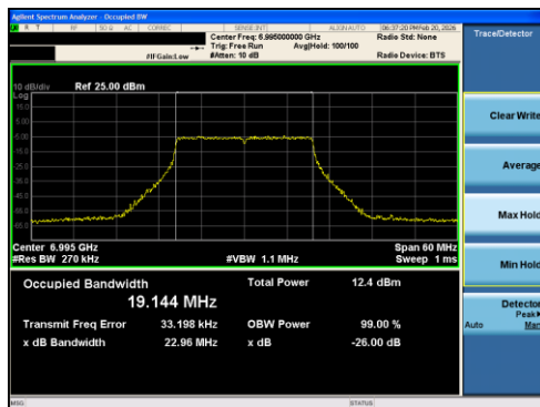
Plot 7-46 26dB BW & 99% OBW Antenna 1 (20MHz BW 802.11ax(RU) RU242 Index61 - Ch.209)
