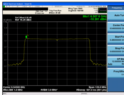
Plot 7-90 PSD Antenna 1 (80MHz BW 802.11ax(RU) RU996 Index67 - Ch.119)
