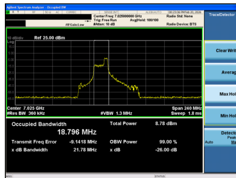
Plot 7-45 26dB BW & 99% OBW Antenna 1 (80MHz BW 802.11ax(RU) RU52 Index44 - Ch.215)
