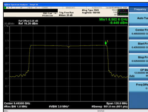
Plot 7-84 PSD Antenna 1 (80MHz BW 802.11ax(RU) RU996 Index67 - Ch.103)
