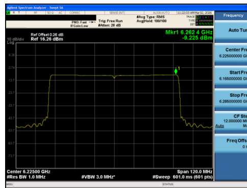
Plot 7-78 PSD Antenna 1 (80MHz BW 802.11ax(RU) RU996 Index67 - Ch.55)
