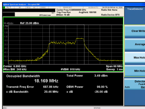
Plot 7-19 26dB BW & 99% OBW Antenna 0 (20MHz BW 802.11ax(RU) RU52 Index40 - Ch.189)
