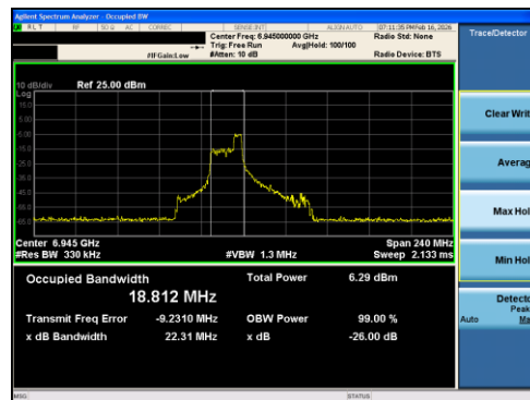
Plot 7-21 26dB BW & 99% OBW Antenna 0 (80MHz BW 802.11ax(RU) RU52 Index44 - Ch.199)
