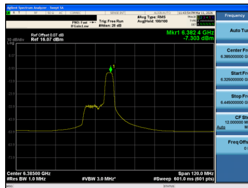
Plot 7-51 PSD Antenna 0 (80MHz BW 802.11ax(RU) RU52 Index44 - Ch.87)
