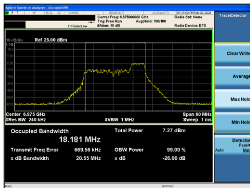
Plot 7-37 26dB BW & 99% OBW Antenna 1 (20MHz BW 802.11ax(RU) RU52 Index40 - Ch.185)
