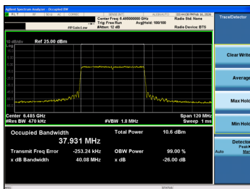
Plot 7-11 26dB BW & 99% OBW Antenna 0 (40MHz BW 802.11ax(RU) RU484 Index65 - Ch.107)
