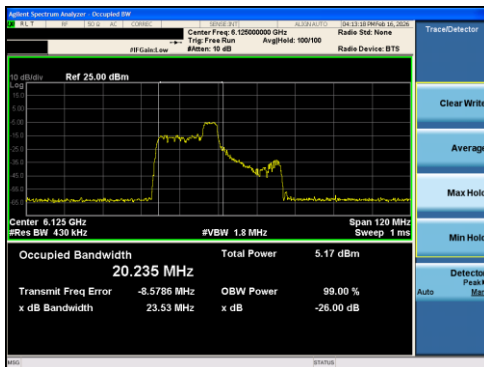
Plot 7-2 26dB BW & 99% OBW Antenna 0 (40MHz BW 802.11ax(RU) RU52 Index40 - Ch.35)
