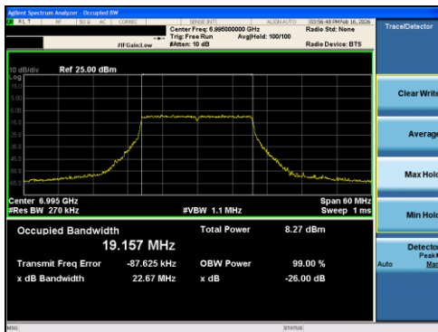
Plot 7-23 26dB BW & 99% OBW Antenna 0 (20MHz BW 802.11ax(RU) RU242 Index61 - Ch.209)
