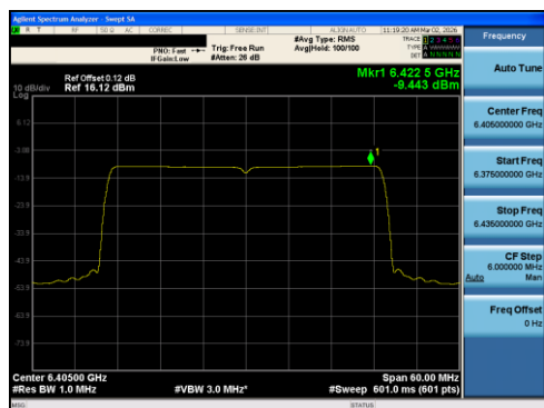
Plot 7-77 PSD Antenna 1 (40MHz BW 802.11ax(RU) RU484 Index65 - Ch.91)
