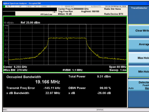
Plot 7-4 26dB BW & 99% OBW Antenna 0 (20MHz BW 802.11ax(RU) RU242 Index61 - Ch.61)
