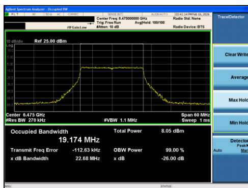
Plot 7-10 26dB BW & 99% OBW Antenna 0 (20MHz BW 802.11ax(RU) RU242 Index61 - Ch.105)
