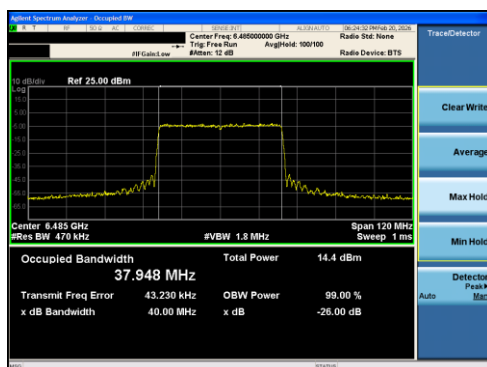
Plot 7-35 26dB BW & 99% OBW Antenna 1 (40MHz BW 802.11ax(RU) RU484 Index65 - Ch.107)
