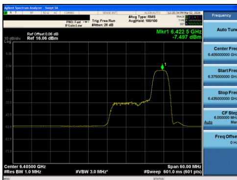
Plot 7-74 PSD Antenna 1 (40MHz BW 802.11ax(RU) RU52 Index44 - Ch.91)
