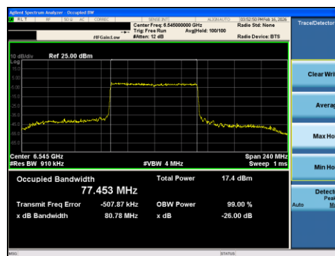
Plot 7-18 26dB BW & 99% OBW Antenna 0 (80MHz BW 802.11ax(RU) RU996 Index67 - Ch.119)
