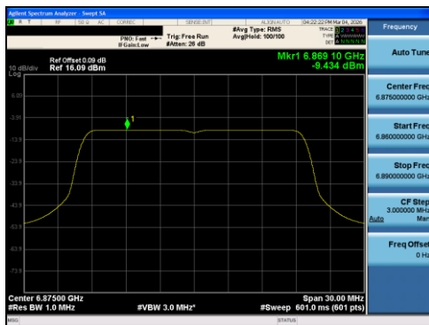
Plot 7-64 PSD Antenna 0 (20MHz BW 802.11ax(RU) RU242 Index61 - Ch.185)
