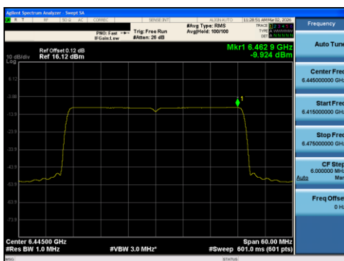
Plot 7-83 PSD Antenna 1 (40MHz BW 802.11ax(RU) RU484 Index65 - Ch.99)
