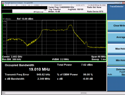
Plot 7-1. 99% OBW Antenna 1 Common (802.11ax OFDMA – RU26 Index 8 – Ch. 11)
