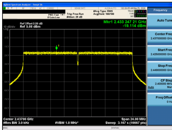
Plot 7-39. Power Spectral Density Plot Antenna 0 (802.11ax OFDMA – RU242 Index 61 – Ch. 6)
