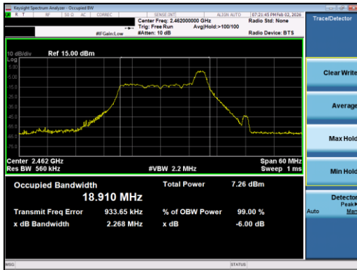
Plot 7-9. 99% OBW Plot Antenna 0 (802.11ax OFDMA – RU26 Index 8 – Ch. 11)
