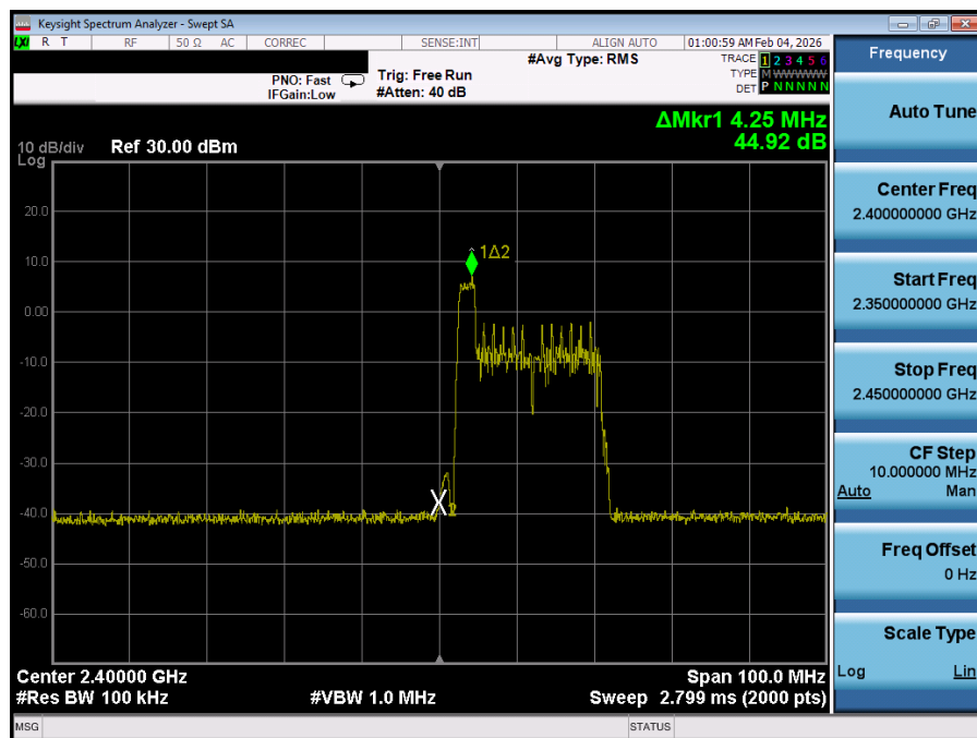
Plot 7-69. Band Edge Antenna 0 (802.11ax OFDMA – RU26 Index 0 – Ch. 1)
