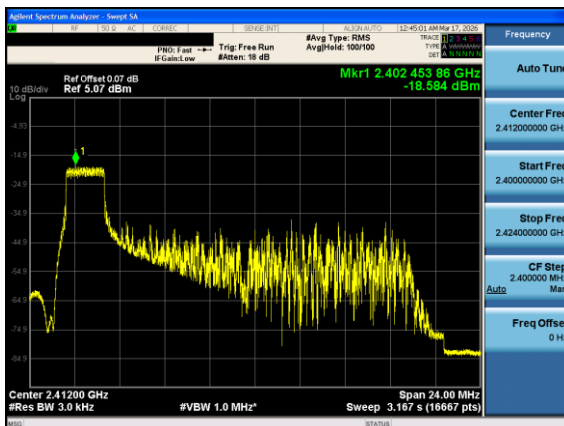
Plot 7-41. Power Spectral Density Plot Antenna 1 Common (802.11ax OFDMA – RU26 Index 0 – Ch. 1)
