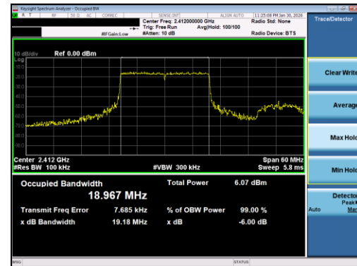
Plot 7-16. 99% OBW Plot Antenna 1 Common (802.11ax OFDMA – RU242 – Ch. 1)
