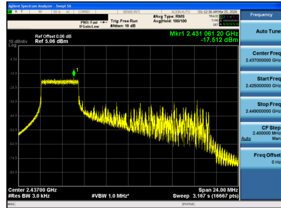
Plot 7-46. Power Spectral Density Plot Antenna 0 (802.11ax OFDMA – RU52 Index 37 – Ch. 6)
