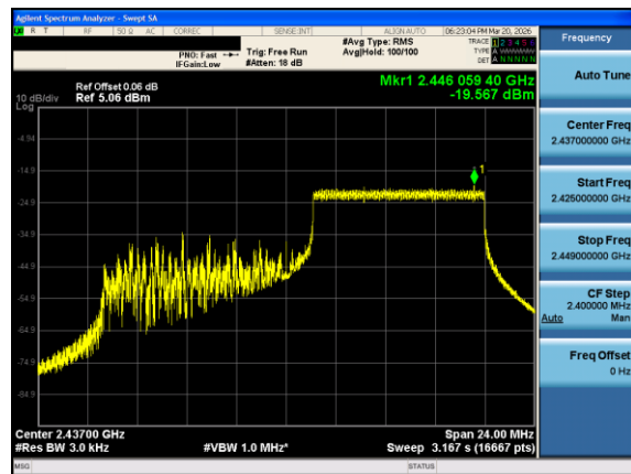
Plot 7-52. Power Spectral Density Plot Antenna 1 Dedicated (802.11ax OFDMA – RU106 Index 54 – Ch. 6)
