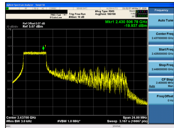
Plot 7-42. Power Spectral Density Plot Antenna 1 Common (802.11ax OFDMA – RU52 Index 37 – Ch. 6)
