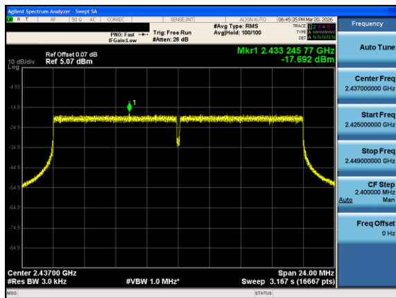
Plot 7-51. Power Spectral Density Plot Antenna 1 Dedicated (802.11ax OFDMA – RU242 Index 61 – Ch. 6)
