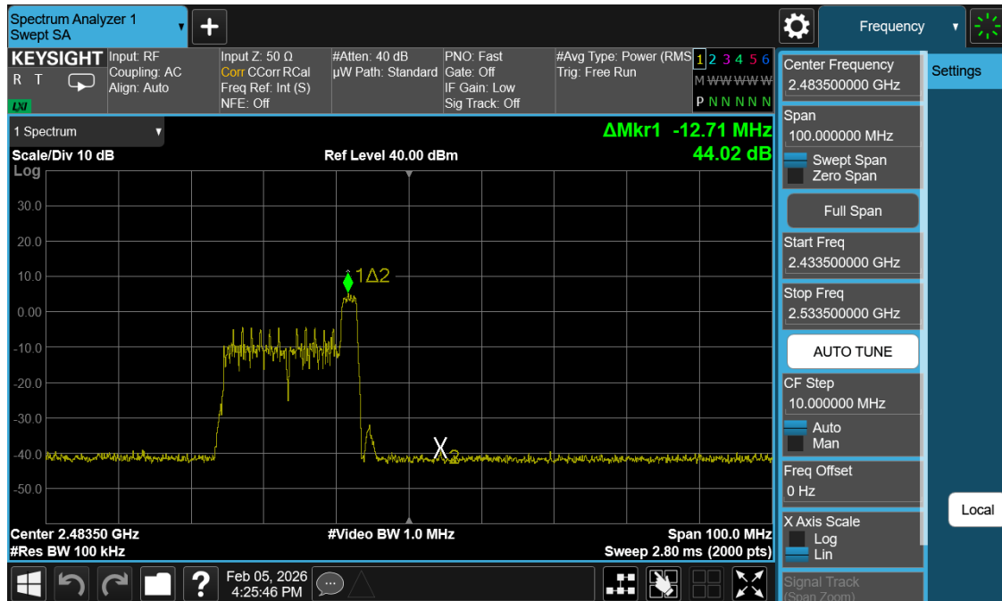
Plot 7-55. Band Edge Antenna 1 Common (802.11ax OFDMA – RU26 Index 8 – Ch. 12)
