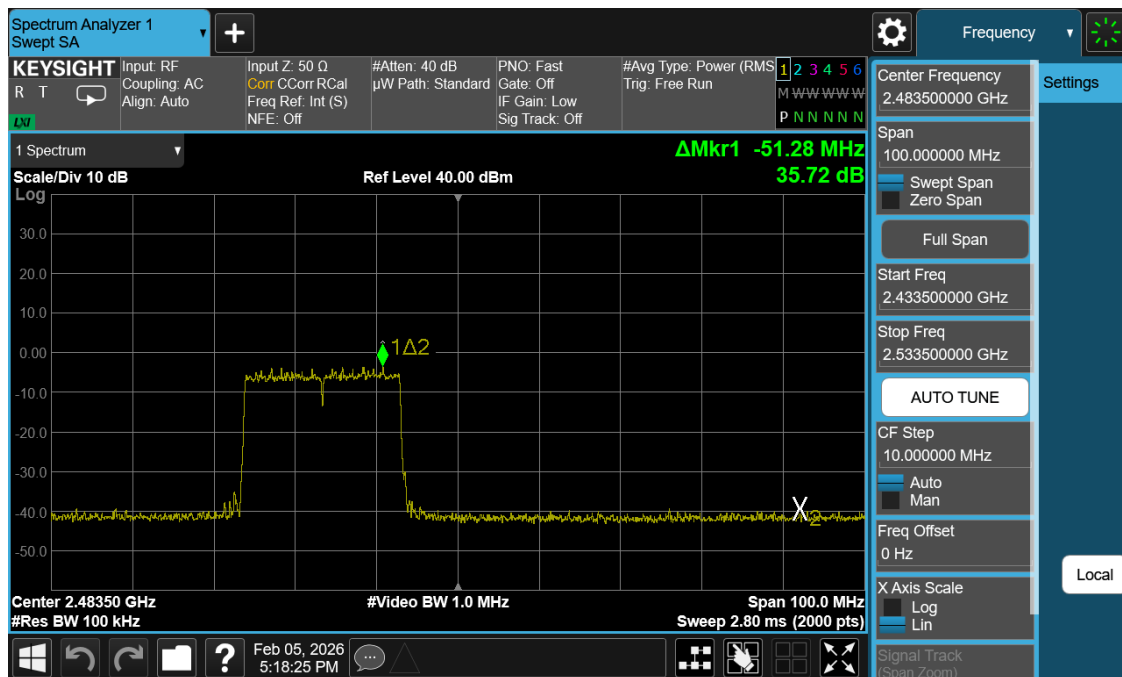
Plot 7-68. Band Edge Antenna 1 Common (802.11ax OFDMA – RU242 – Ch. 12)
