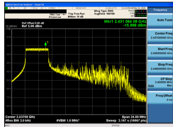
Plot 7-35. Power Spectral Density Plot Antenna 1 Dedicated (802.11ax OFDMA – RU52 Index 37 – Ch. 6)
