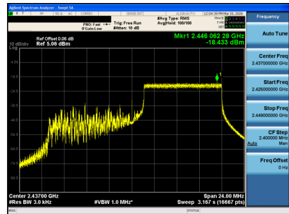
Plot 7-36. Power Spectral Density Plot Antenna 1 Dedicated (802.11ax OFDMA – RU106 Index 54 – Ch. 6)
