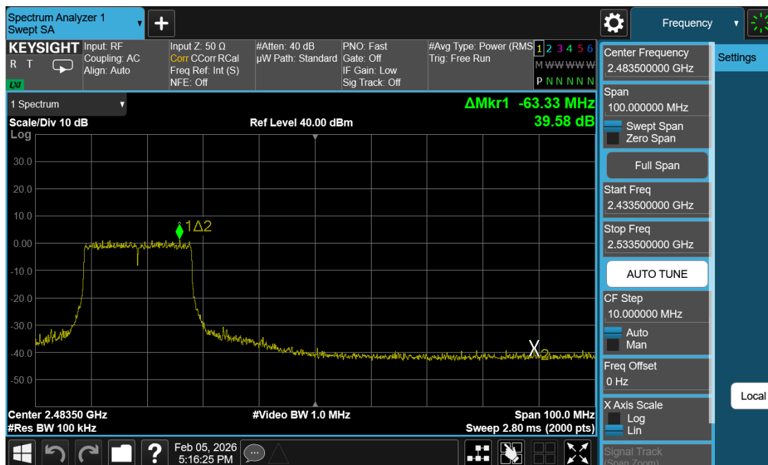
Plot 7-65. Band Edge Antenna 1 Common (802.11ax OFDMA – RU242 – Ch. 9)
