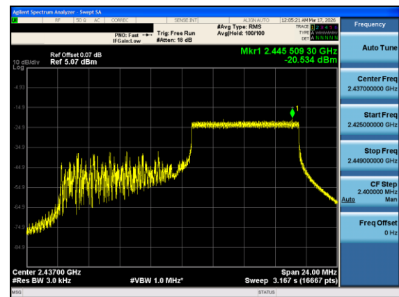
Plot 7-28. Power Spectral Density Plot Antenna 1 Common (802.11ax OFDMA – RU106 Index 54 – Ch. 6)
