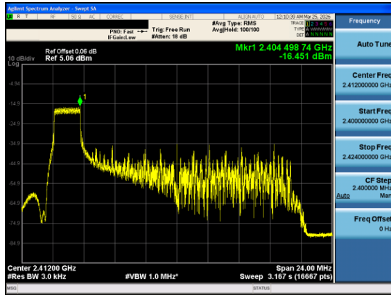
Plot 7-37. Power Spectral Density Plot Antenna 0 (802.11ax OFDMA – RU26 Index 0 – Ch. 1)
