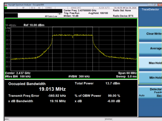
Plot 7-20. 6dB BW OBW Plot Antenna 0 (802.11ax OFDMA – RU242 – Ch. 6)
