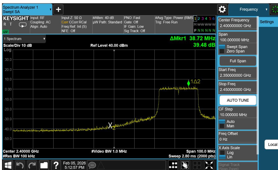
Plot 7-60. Band Edge Antenna 1 Common (802.11ax OFDMA – RU242 – Ch. 5)
