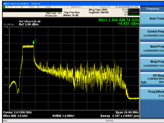
Plot 7-45. Power Spectral Density Plot Antenna 0 (802.11ax OFDMA – RU26 Index 0 – Ch. 1)
