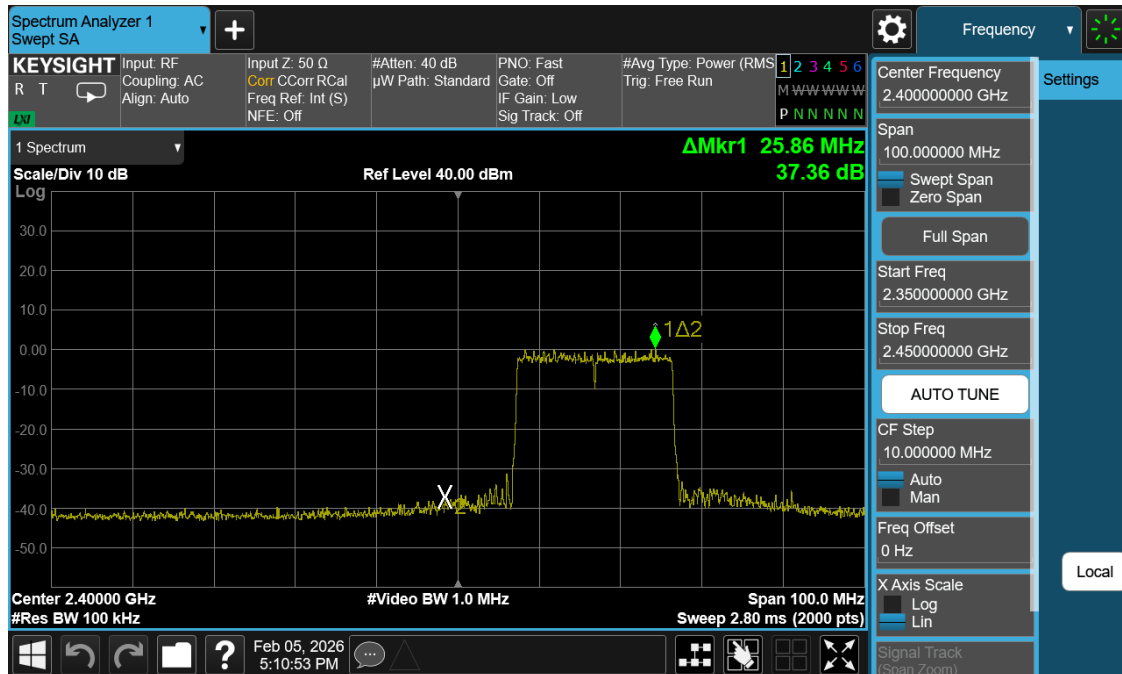
Plot 7-57. Band Edge Antenna 1 Common (802.11ax OFDMA – RU242 – Ch. 2)
