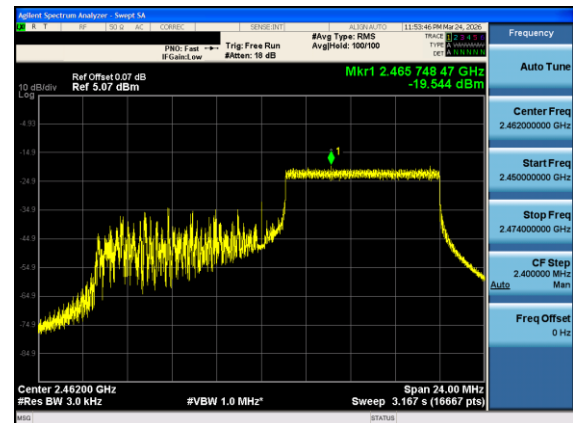
Plot 7-32. Power Spectral Density Plot Antenna 0 (802.11ax OFDMA - RU106 Index 54 - Ch. 11)
