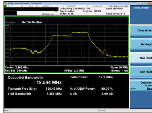
Plot 7-3. 99% OBW Antenna 1 Common (802.11ax OFDMA – RU106 Index 53 – Ch. 11)
