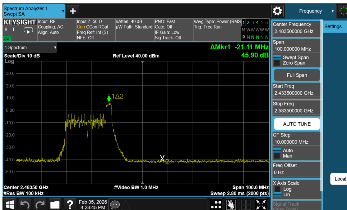
Plot 7-54. Band Edge Antenna 1 Common (802.11ax OFDMA – RU26 Index 8 – Ch. 11)
