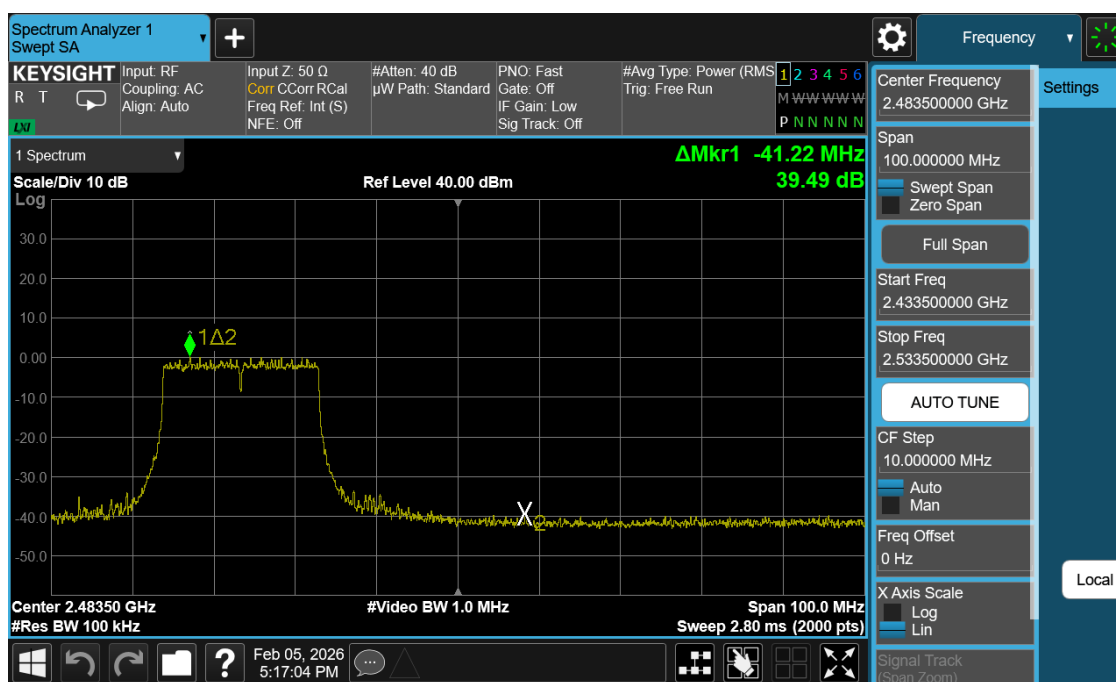
Plot 7-66. Band Edge Antenna 1 Common (802.11ax OFDMA – RU242 – Ch. 10)
