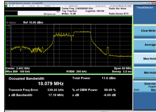
Plot 7-14. 99% OBW Plot Antenna 1 Common (802.11ax OFDMA – RU106 Index 54 – Ch. 11)
