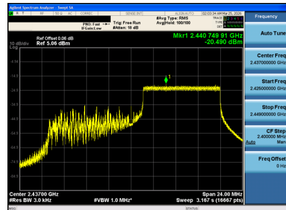
Plot 7-40. Power Spectral Density Plot Antenna 0 (802.11ax OFDMA – RU106 Index 54 – Ch. 6)
