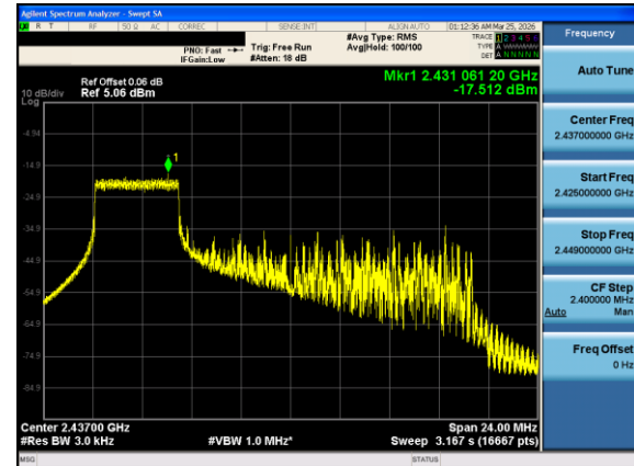
Plot 7-38. Power Spectral Density Plot Antenna 0 (802.11ax OFDMA – RU52 Index 37 – Ch. 6)
