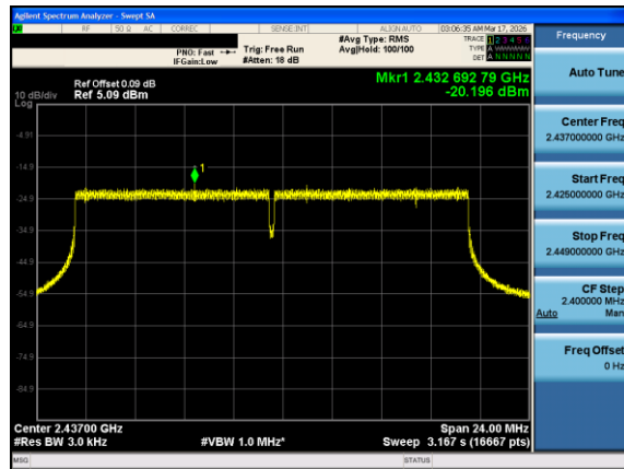
Plot 7-43. Power Spectral Density Plot Antenna 1 Common (802.11ax OFDMA – RU242 Index 61 – Ch. 6)
