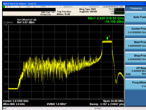
Plot 7-29. Power Spectral Density Plot Antenna 0 (802.11ax OFDMA - RU26 Index 8 - Ch. 1)
