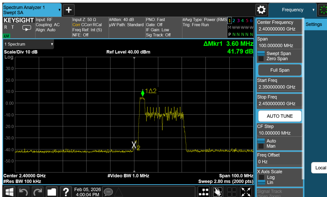
Plot 7-53. Band Edge Antenna 1 Common (802.11ax OFDMA – RU26 Index 0 – Ch. 1)
