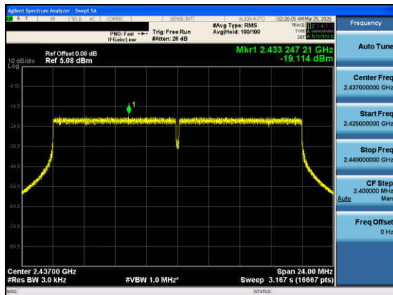
Plot 7-47. Power Spectral Density Plot Antenna 0 (802.11ax OFDMA – RU242 Index 61 – Ch. 6)
