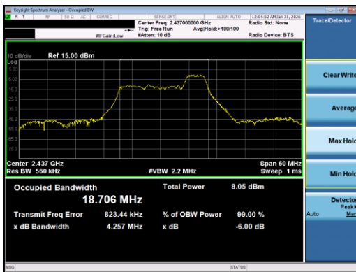
Plot 7-2. 99% OBW Antenna 1 Common (802.11ax OFDMA – RU52 Index 40 – Ch. 6)
