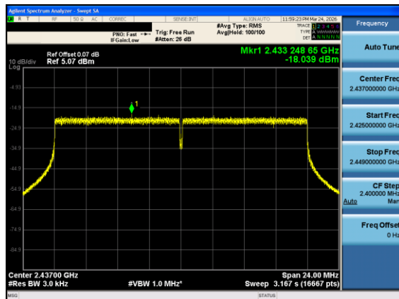
Plot 7-31. Power Spectral Density Plot Antenna 0 (802.11ax OFDMA - RU242 Index 61 - Ch. 6)
