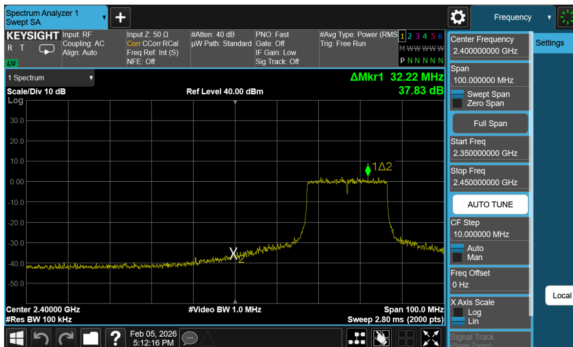
Plot 7-59. Band Edge Antenna 1 Common (802.11ax OFDMA – RU242 – Ch. 4)
