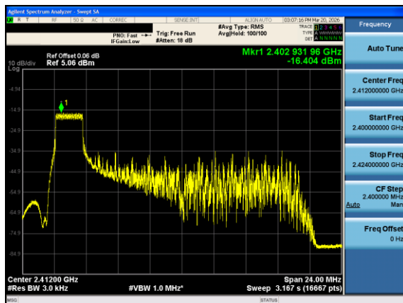
Plot 7-49. Power Spectral Density Plot Antenna 1 Dedicated (802.11ax OFDMA – RU26 Index 0 – Ch. 1)
