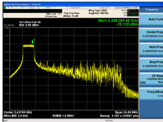
Plot 7-33. Power Spectral Density Plot Antenna 1 Dedicated (802.11ax OFDMA – RU26 Index 0 – Ch. 6)
