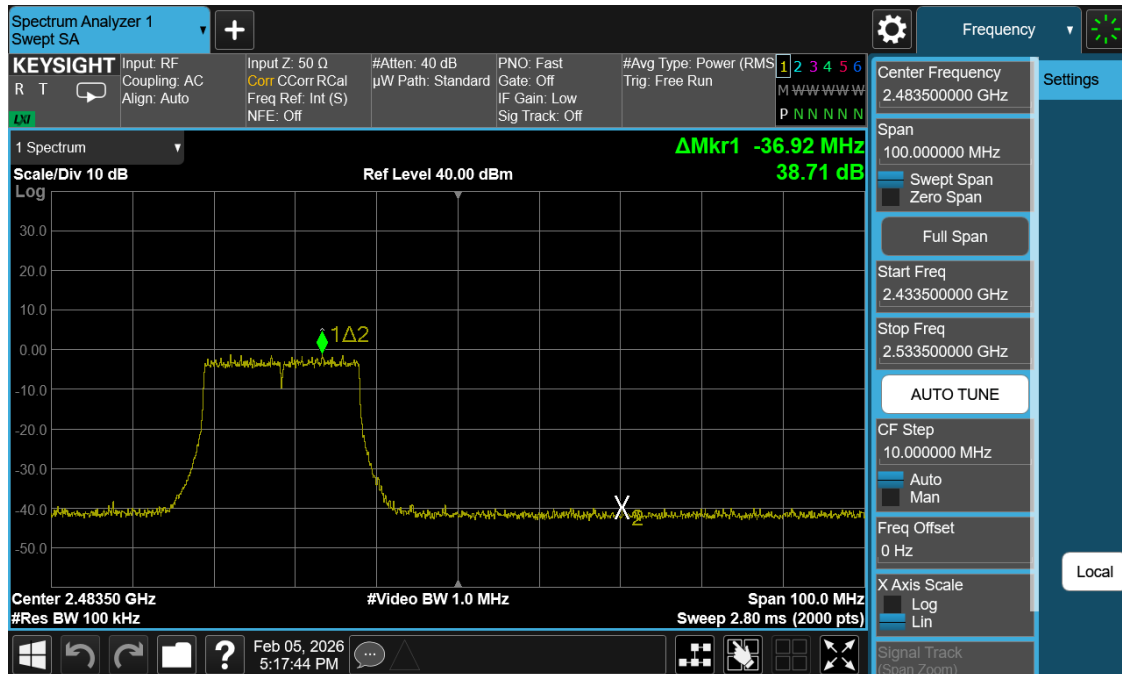
Plot 7-67. Band Edge Antenna 1 Common (802.11ax OFDMA – RU242 – Ch. 11)
