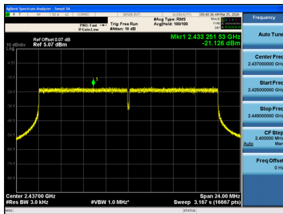
Plot 7-27. Power Spectral Density Plot Antenna 1 Common (802.11ax OFDMA – RU242 Index 61 – Ch. 6)
