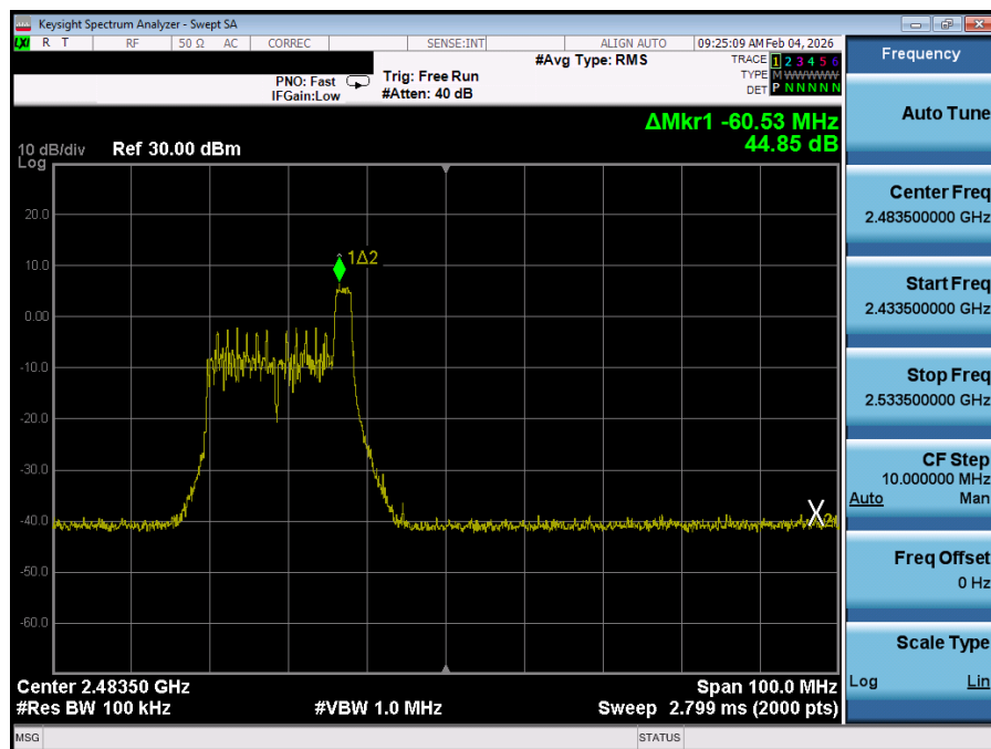
Plot 7-70. Band Edge Antenna 0 (802.11ax OFDMA – RU26 Index 8 – Ch. 11)
