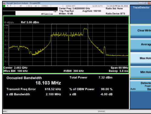
Plot 7-13. 99% OBW Antenna 1 Common (802.11ax OFDMA – RU26 Index 8 – Ch. 11)
