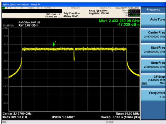
Plot 7-34. Power Spectral Density Plot Antenna 1 Dedicated (802.11ax OFDMA – RU242 Index 61 – Ch. 6)
