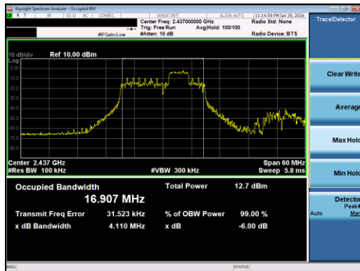
Plot 7-15. 99% OBW Antenna 1 Common (802.11ax OFDMA – RU52 Index 39 – Ch. 6)
