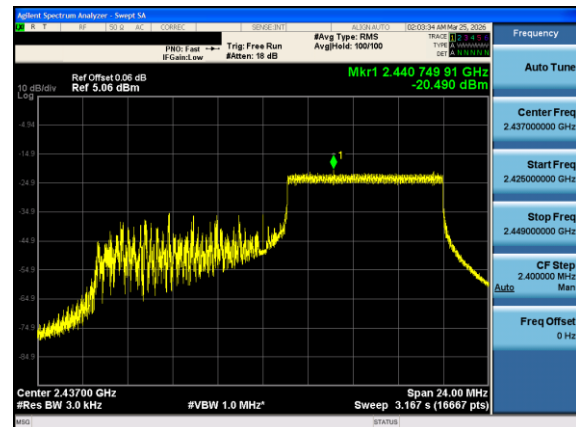
Plot 7-48. Power Spectral Density Plot Antenna 0 (802.11ax OFDMA – RU106 Index 54 – Ch. 6)
