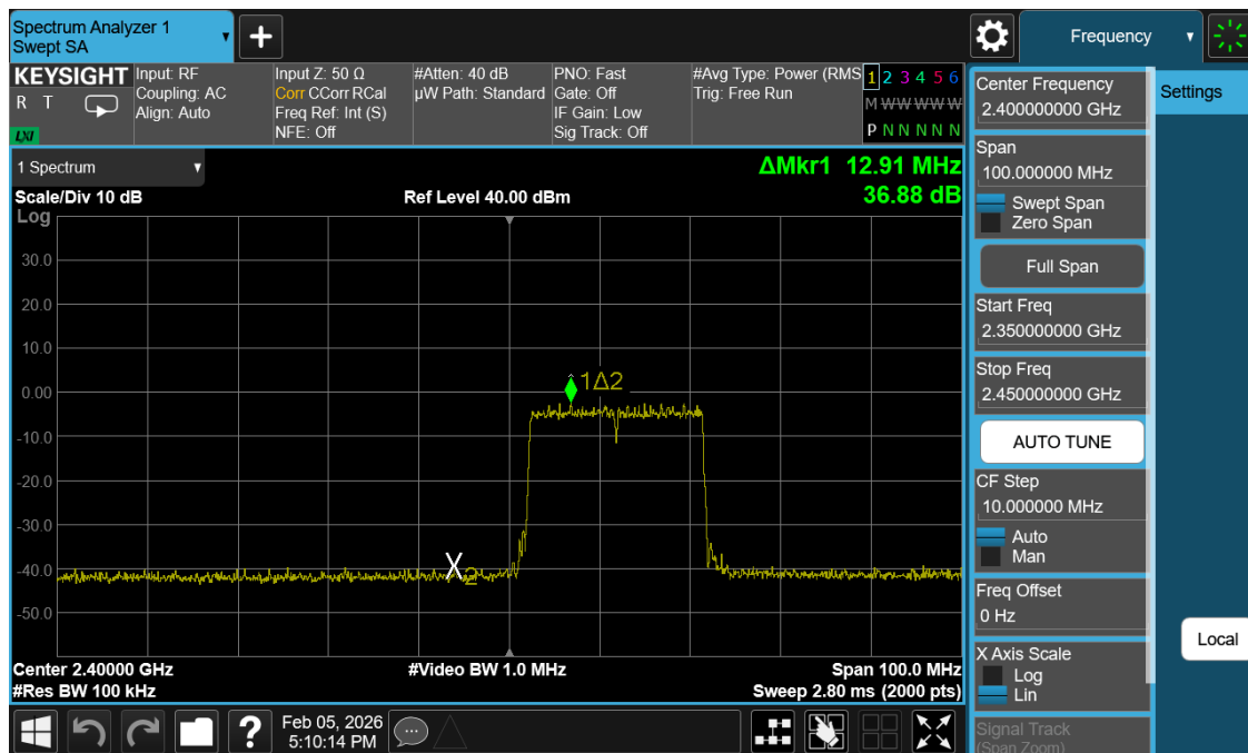
Plot 7-56. Band Edge Antenna 1 Common (802.11ax OFDMA – RU242 – Ch. 1)
