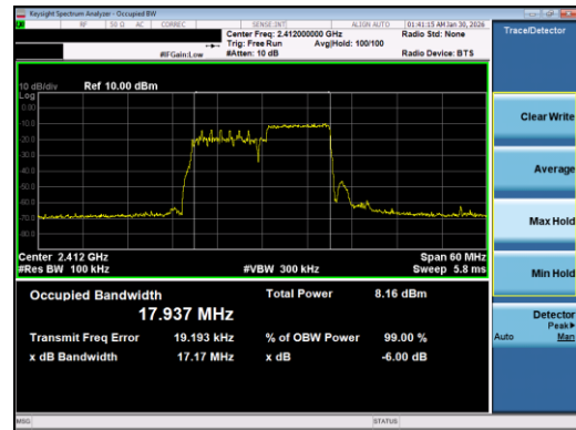
Plot 7-18. 6dB BW OBW Plot Antenna 0 (802.11ax OFDMA – RU106 Index 54 – Ch. 1)
