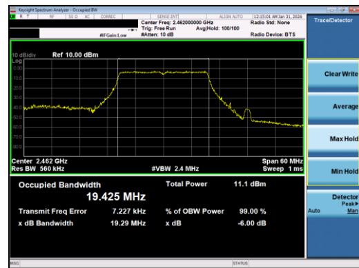
Plot 7-4. 99% OBW Plot Antenna 1 Common (802.11ax OFDMA – RU242 – Ch. 11)
