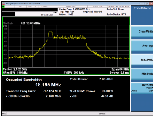
Plot 7-17. 6dB BW OBW Plot Antenna 0 (802.11ax OFDMA – RU26 Index 0 – Ch. 11)
