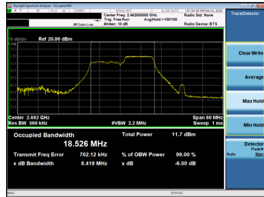
Plot 7-10. 99% OBW Plot Antenna 0 (802.11ax OFDMA – RU106 Index 54 – Ch. 11)
