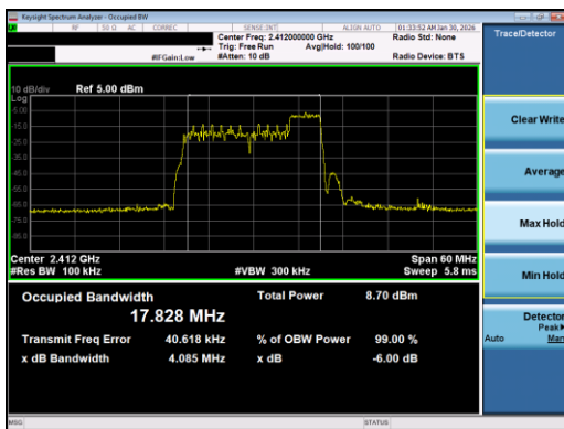
Plot 7-19. 6dB BW OBW Plot Antenna 0 (802.11ax OFDMA – RU52 Index 40 – Ch. 1)
