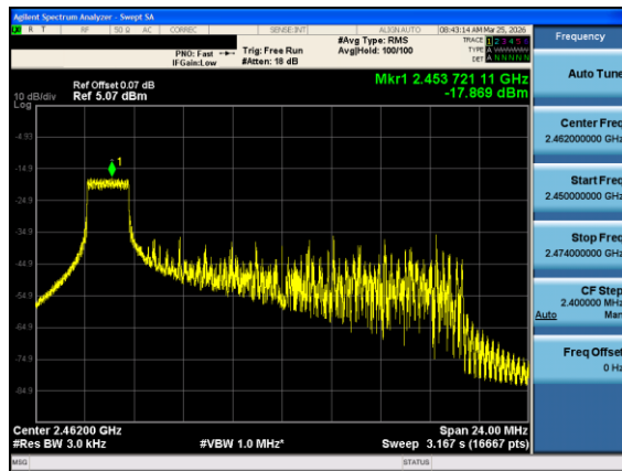
Plot 7-25. Power Spectral Density Plot Antenna 1 Common (802.11ax OFDMA – RU26 Index 0 – Ch. 11)
