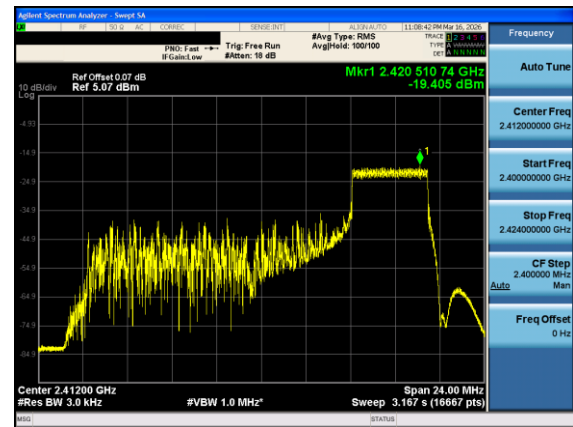
Plot 7-26. Power Spectral Density Plot Antenna 1 Common (802.11ax OFDMA – RU52 Index 40 – Ch. 1)
