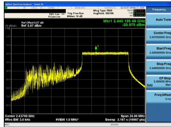
Plot 7-44. Power Spectral Density Plot Antenna 1 Common (802.11ax OFDMA – RU106 Index 54 – Ch. 6)
