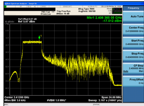
Plot 7-30. Power Spectral Density Plot Antenna 0 (802.11ax OFDMA - RU52 Index 37 - Ch. 1)
