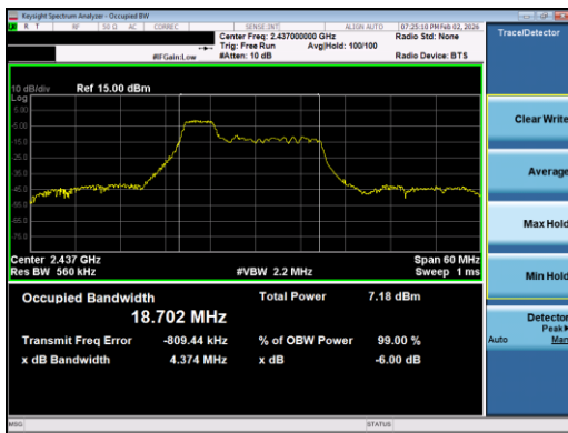
Plot 7-11. 99% OBW Plot Antenna 0 (802.11ax OFDMA – RU52 Index 37 – Ch. 6)
