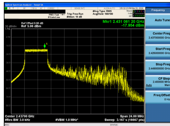
Plot 7-50. Power Spectral Density Plot Antenna 1 Dedicated (802.11ax OFDMA – RU52 Index 37 – Ch. 6)
