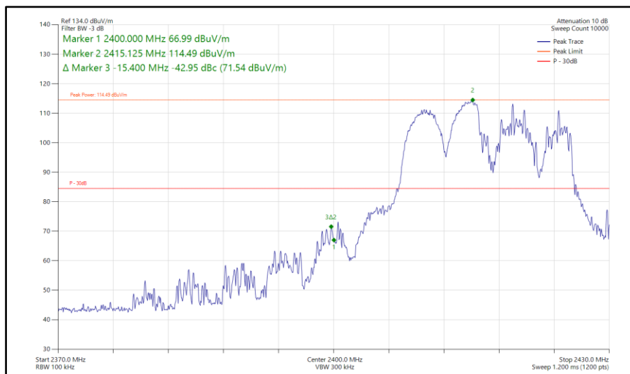
Figure 347 - 802.11ax HE20, RU106-53, CDD, Core 0-1 - 2417 MHz Band Edge Frequency 2400 MHz
