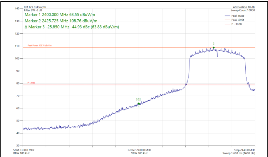
Figure 307 - 802.11ax HE20, SU, SISO, Core 0 - 2427 MHz Band Edge Frequency 2400 MHz
