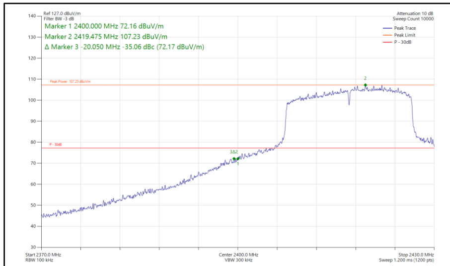
Figure 327 - 802.11ax HE20, SU, SISO, Core 1 - 2417 MHz Band Edge Frequency 2400 MHz
