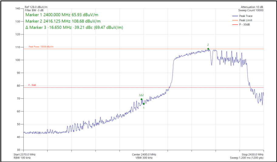
Figure 310 - 802.11be EHT20, RU106+26-82, SISO, Core 0 - 2417 MHz Band Edge Frequency 2400 MHz
