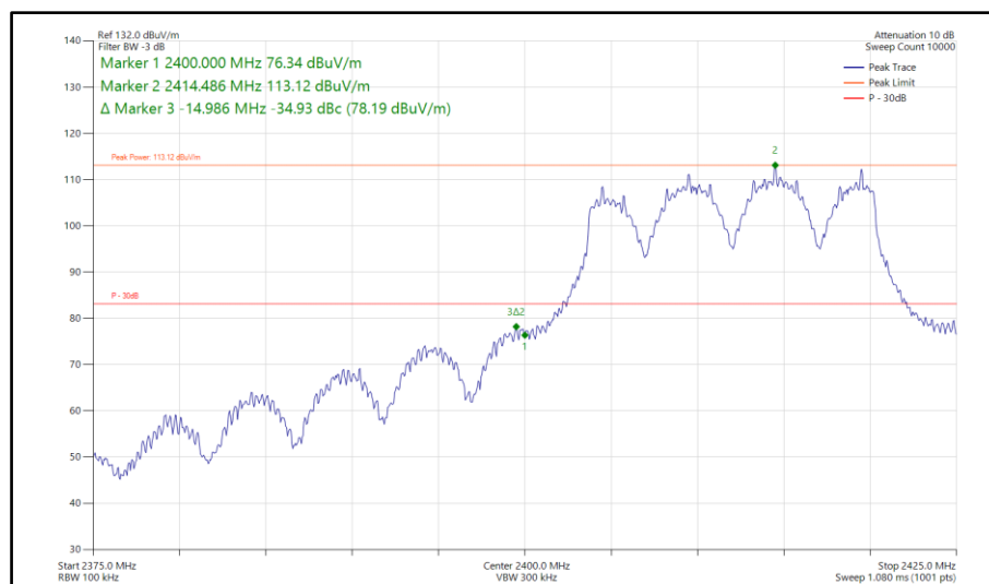
Figure 334 - 802.11g, CDD, Core 0-1 - 2412 MHz Band Edge Frequency 2400 MHz
