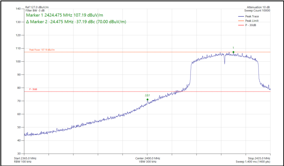
Figure 306 - 802.11ax HE20, SU, SISO, Core 0 - 2422 MHz Band Edge Frequency 2400 MHz
