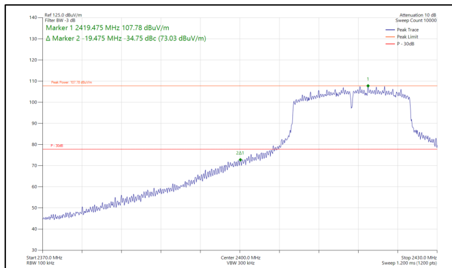
Figure 298 - 802.11n HT20, SISO, Core 0 - 2417 MHz Band Edge Frequency 2400 MHz
