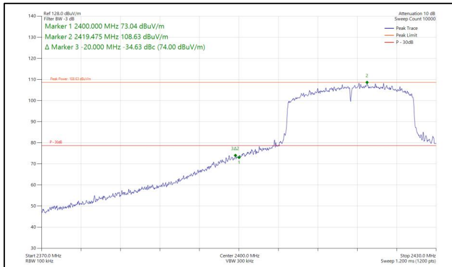
Figure 304 - 802.11ax HE20, SU, SISO, Core 0 - 2417 MHz Band Edge Frequency 2400 MHz
