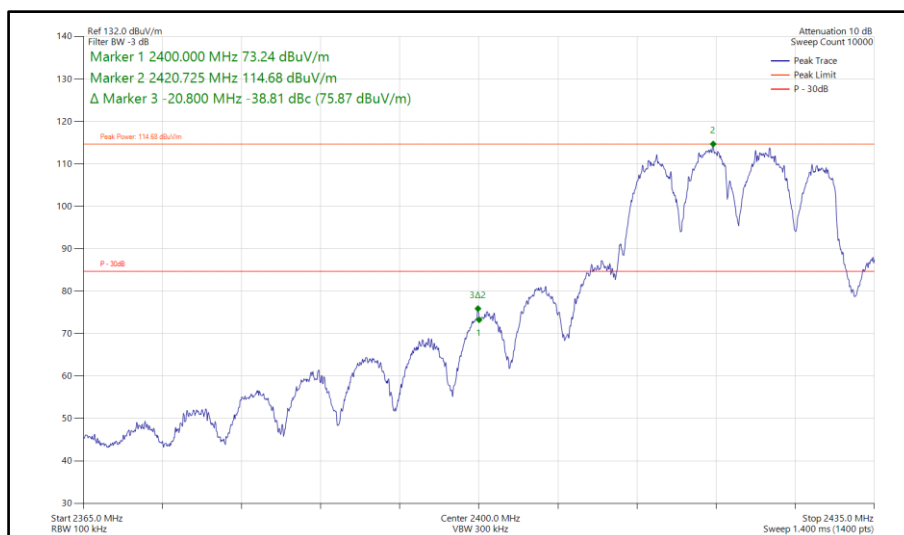
Figure 348 - 802.11ax HE20, SU, CDD, Core 0-1 - 2422 MHz Band Edge Frequency 2400 MHz
