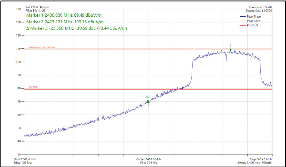
Figure 329 - 802.11ax HE20, SU, SISO, Core 1 - 2422 MHz Band Edge Frequency 2400 MHz
