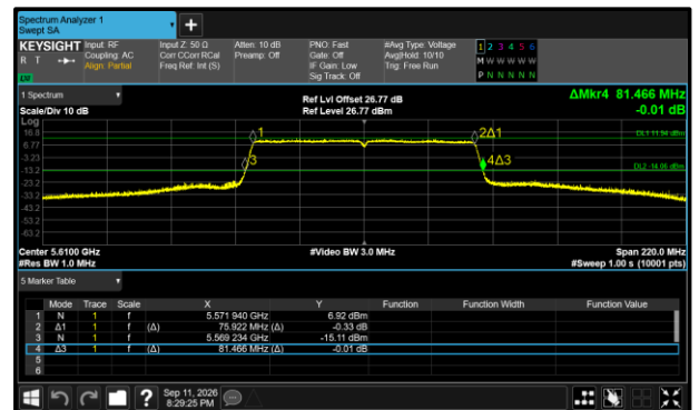
Figure 397 - 802.11ac VHT80 Maximum 99% OBW
