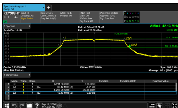
Figure 394 - 802.11n HT40 Minimum 99% OBW
