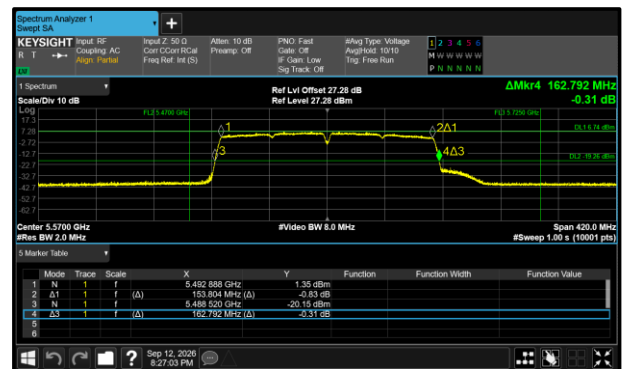
Figure 399 - 802.11ac VHT160 Maximum 99% OBW
