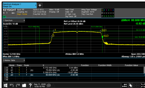
Figure 396 - 802.11ac VHT80 Minimum 99% OBW
