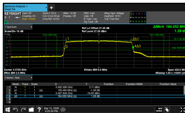
Figure 407 - 802.11ax HE160 SU Maximum 99% OBW
