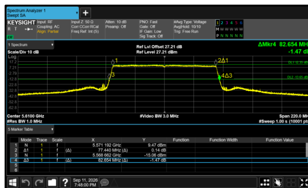
Figure 405 - 802.11ax HE80 SU Maximum 99% OBW
