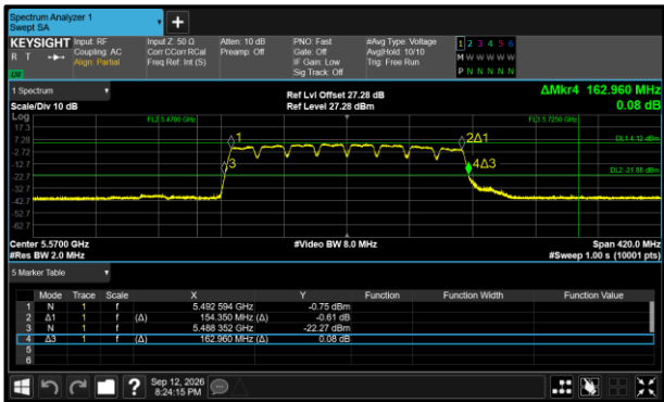
Figure 415 - 802.11a160 Maximum 99% OBW
