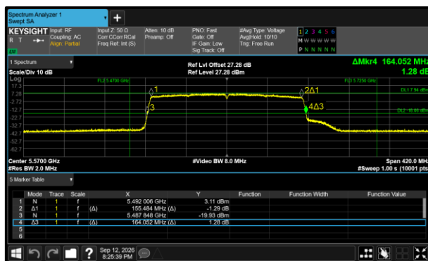
Figure 406 - 802.11ax HE160 SU Minimum 99% OBW
