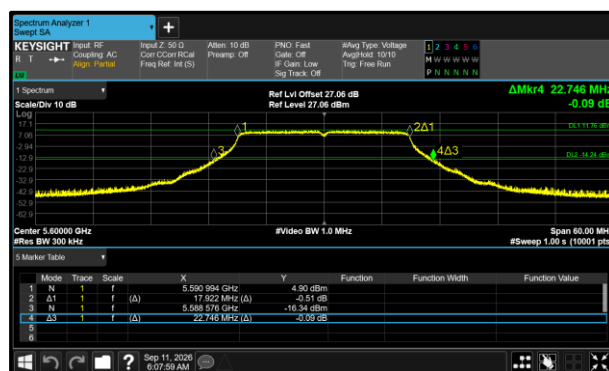
Figure 393 - 802.11n HT20 Maximum 99% OBW
