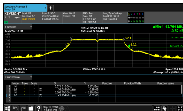
Figure 395 - 802.11n HT40 Maximum 99% OBW
