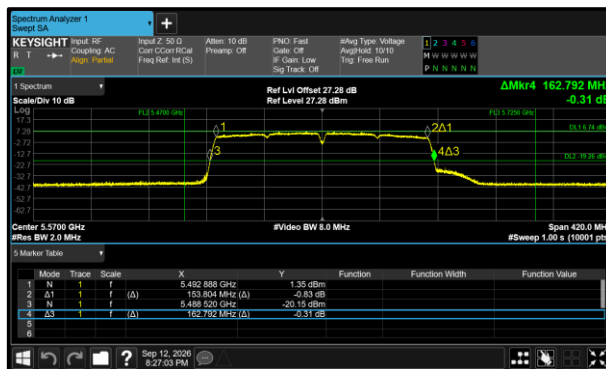
Figure 398 - 802.11ac VHT160 Minimum 99% OBW
