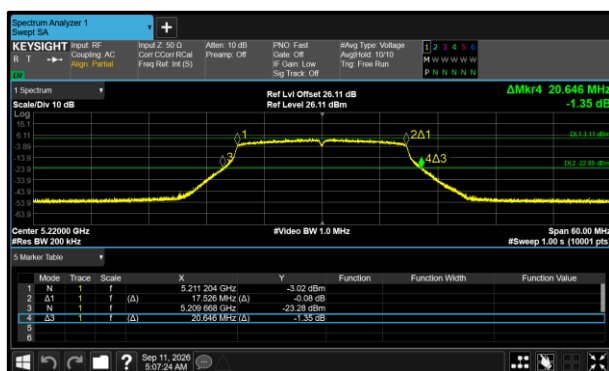
Figure 392 - 802.11n HT20 Minimum 99% OBW
