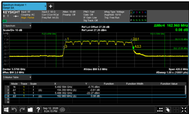
Figure 414 - 802.11a160 Minimum 99% OBW
