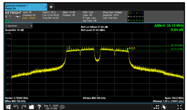
Figure 567 - 802.11a40 Maximum 6 dB EBW
