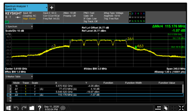
Figure 517 - 802.11a80 Maximum 26 dB EBW
