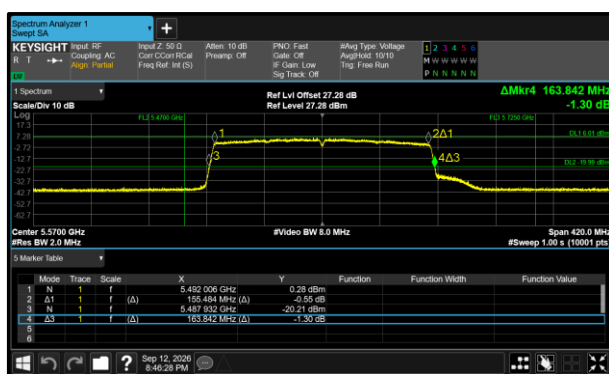
Figure 510 - 802.11ax HE160 SU Minimum 26 dB EBW
