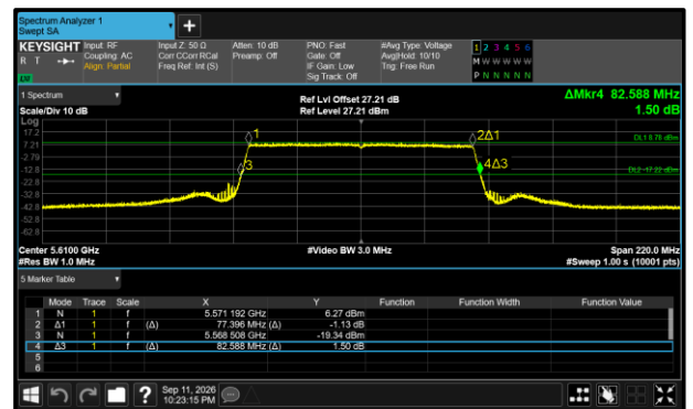
Figure 549 - 802.11ax HE80 SU Maximum 26 dB EBW
