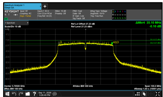
Figure 573 - 802.11n HT40 Maximum 6 dB EBW
