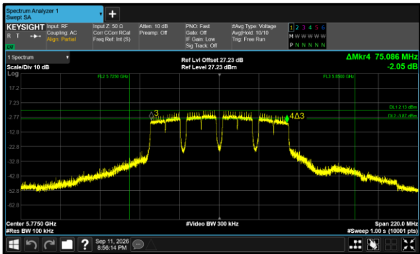
Figure 586 - 802.11a80 Minimum 6 dB EBW
