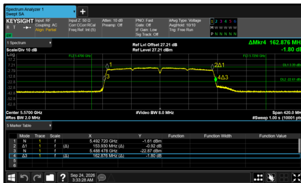
Figure 526 - 802.11ac VHT160 Minimum 26 dB EBW
