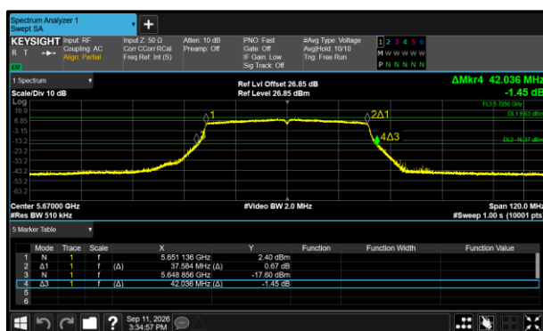
Figure 506 - 802.11ax HE40 SU Minimum 26 dB EBW
