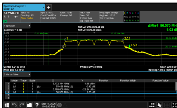
Figure 516 - 802.11a80 Minimum 26 dB EBW
