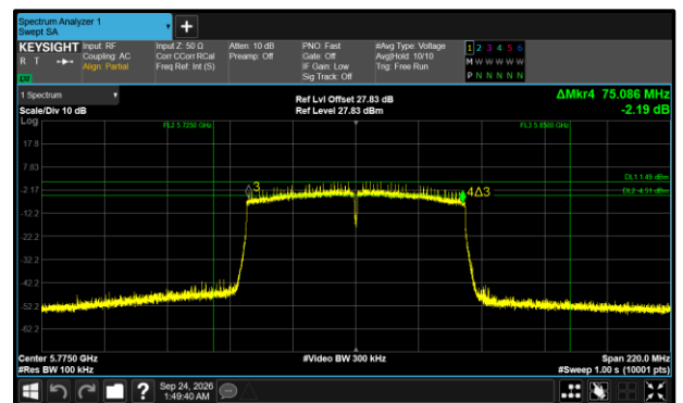
Figure 593 - 802.11ac VHT80 Maximum 6 dB EBW
