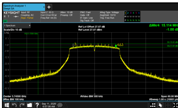
Figure 552 - 802.11n HT20 Minimum 6 dB EBW
