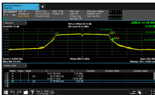
Figure 538 - 802.11ac VHT40 Minimum 26 dB EBW
