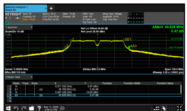
Figure 515 - 802.11a40 Maximum 26 dB EBW
