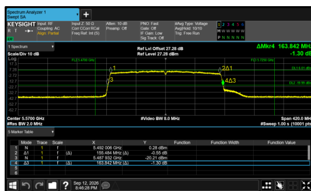
Figure 511 - 802.11ax HE160 SU Maximum 26 dB EBW
