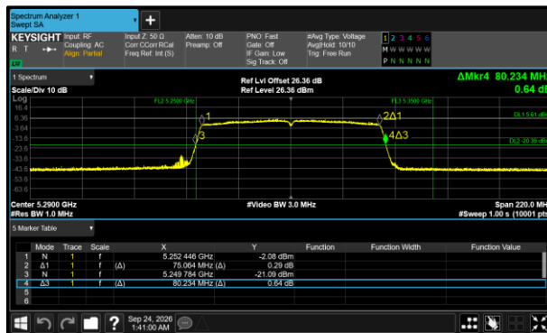
Figure 524 - 802.11ac VHT80 Minimum 26 dB EBW
