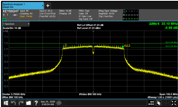
Figure 591 - 802.11n HT40 Maximum 6 dB EBW
