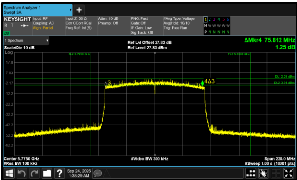
Figure 599 - 802.11ax HE80 SU Maximum 6 dB EBW
