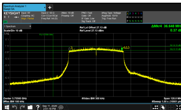
Figure 560 - 802.11ax HE40 SU Minimum 6 dB EBW
