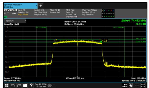
Figure 563 - 802.11ax HE80 SU Maximum 6 dB EBW
