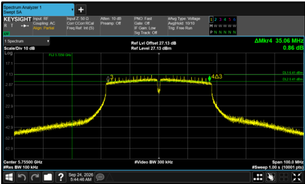
Figure 590 - 802.11n HT40 Minimum 6 dB EBW
