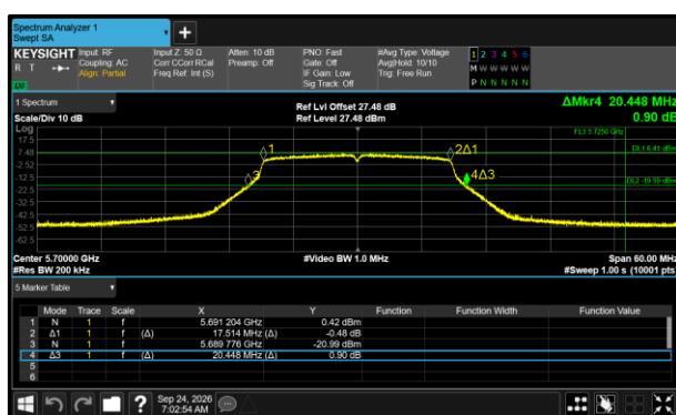
Figure 520 - 802.11n HT20 Minimum 26 dB EBW
