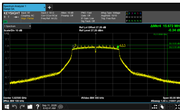
Figure 564 - 802.11a20 Minimum 6 dB EBW
