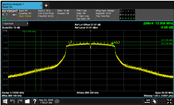
Figure 588 - 802.11n HT20 Minimum 6 dB EBW
