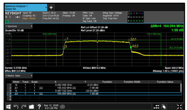
Figure 551 - 802.11ax HE160 SU Maximum 26 dB EBW
