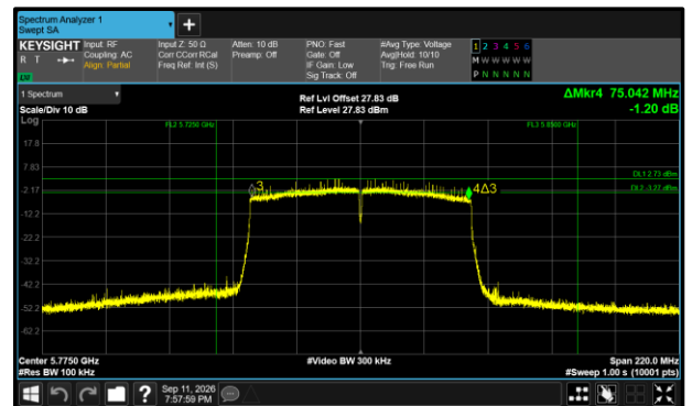
Figure 557 - 802.11ac VHT80 Maximum 6 dB EBW
