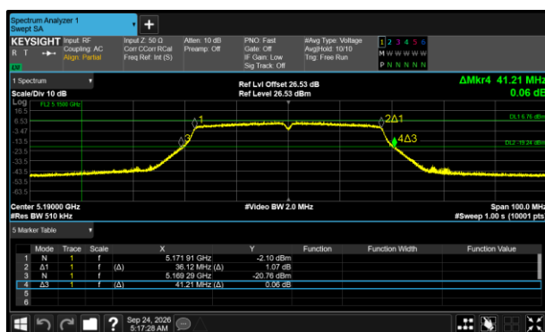
Figure 522 - 802.11n HT40 Minimum 26 dB EBW
