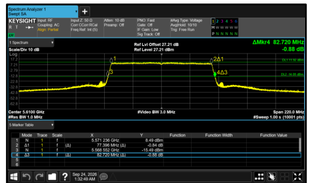
Figure 533 - 802.11ax HE80 SU Maximum 26 dB EBW
