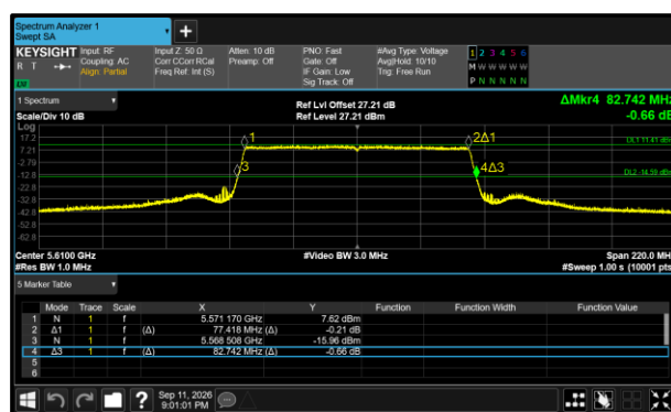
Figure 509 - 802.11ax HE80 SU Maximum 26 dB EBW
