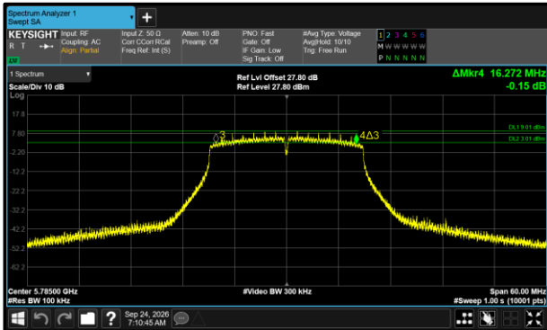
Figure 589 - 802.11n HT20 Maximum 6 dB EBW
