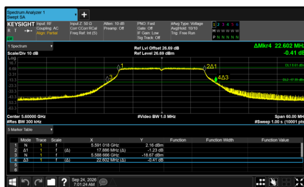
Figure 521 - 802.11n HT20 Maximum 26 dB EBW
