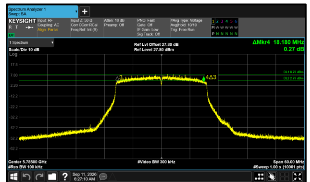
Figure 559 - 802.11ax HE20 SU Maximum 6 dB EBW
