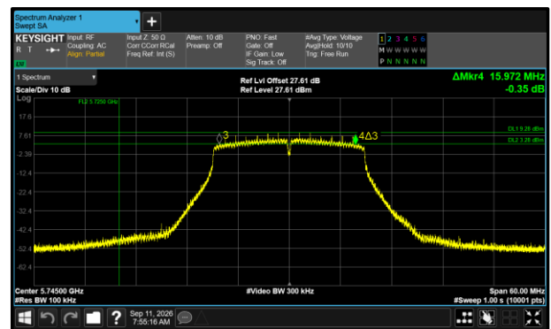
Figure 571 - 802.11n HT20 Maximum 6 dB EBW
