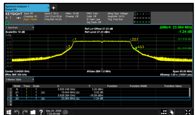
Figure 529 - 802.11ax HE20 SU Maximum 26 dB EBW
