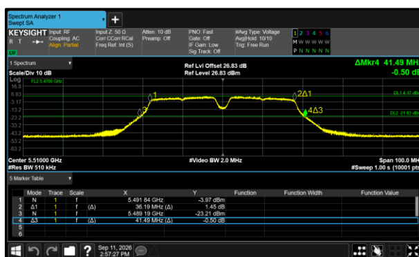
Figure 514 - 802.11a40 Minimum 26 dB EBW
