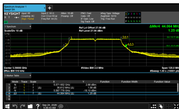
Figure 523 - 802.11n HT40 Maximum 26 dB EBW
