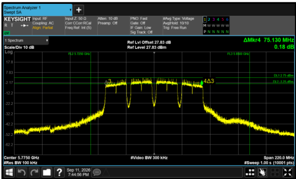
Figure 569 - 802.11a80 Maximum 6 dB EBW
