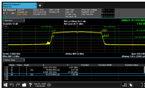
Figure 532 - 802.11ax HE80 SU Minimum 26 dB EBW
