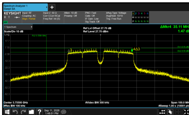
Figure 566 - 802.11a40 Minimum 6 dB EBW
