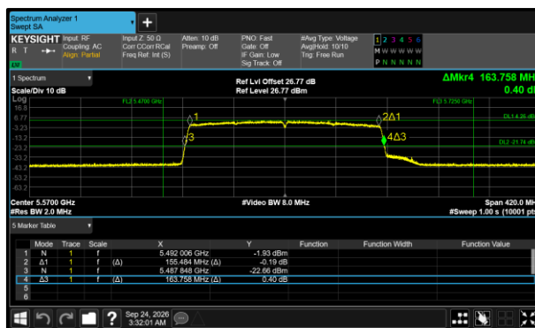
Figure 534 - 802.11ax HE160 SU Minimum 26 dB EBW
