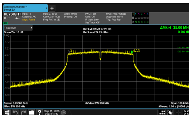
Figure 554 - 802.11n HT40 Minimum 6 dB EBW
