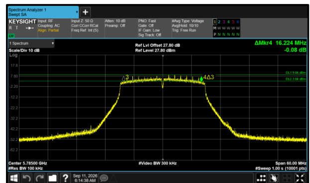
Figure 553 - 802.11n HT20 Maximum 6 dB EBW
