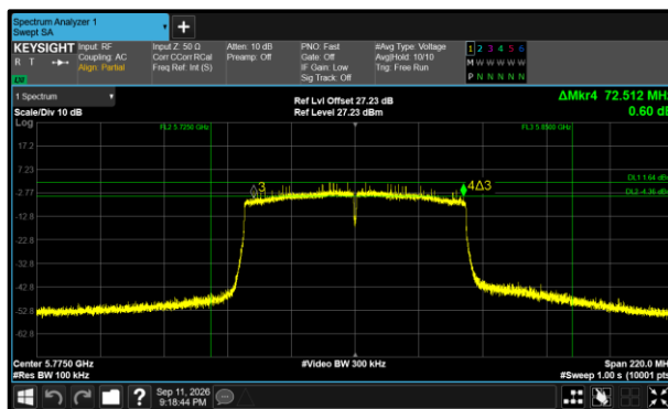
Figure 574 - 802.11ac VHT80 Minimum 6 dB EBW
