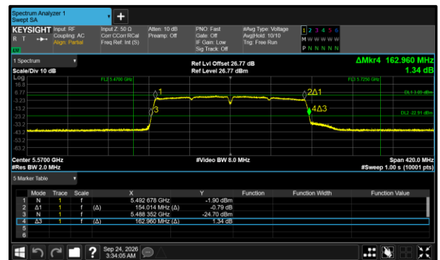
Figure 527 - 802.11ac VHT160 Maximum 26 dB EBW
