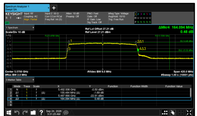
Figure 535 - 802.11ax HE160 SU Maximum 26 dB EBW
