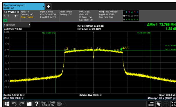
Figure 556 - 802.11ac VHT80 Minimum 6 dB EBW
