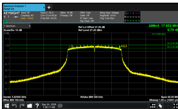
Figure 594 - 802.11ax HE20 SU Minimum 6 dB EBW
