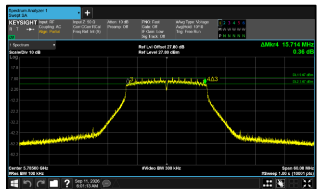
Figure 565 - 802.11a20 Maximum 6 dB EBW
