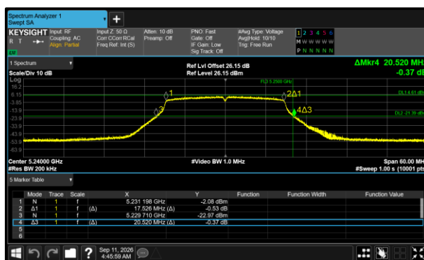
Figure 536 - 802.11ac VHT20 Minimum 26 dB EBW
