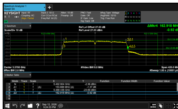
Figure 543 - 802.11ac VHT160 Maximum 26 dB EBW
