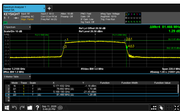
Figure 508 - 802.11ax HE80 SU Minimum 26 dB EBW
