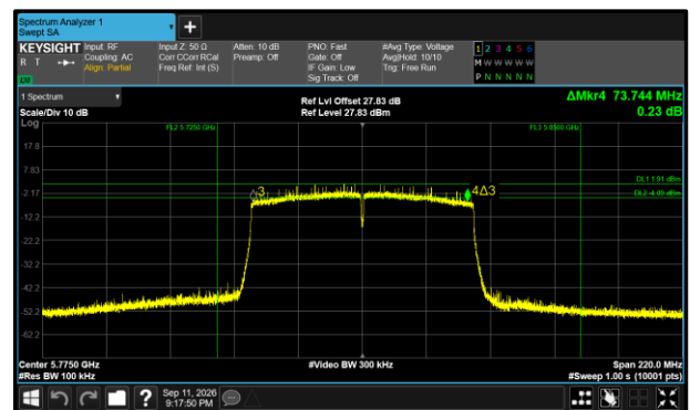
Figure 575 - 802.11ac VHT80 Maximum 6 dB EBW
