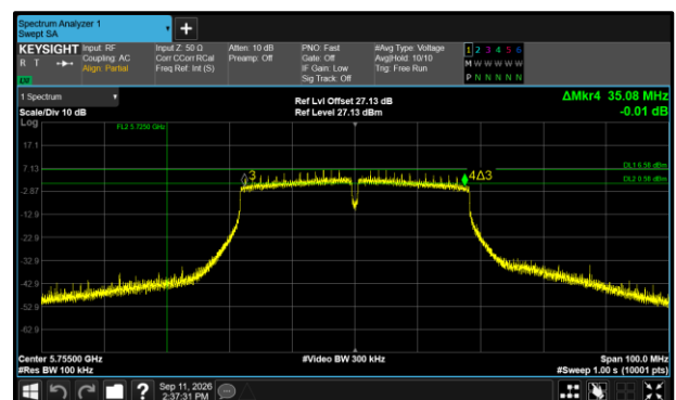
Figure 555 - 802.11n HT40 Maximum 6 dB EBW
