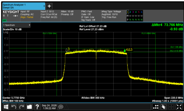
Figure 598 - 802.11ax HE80 SU Minimum 6 dB EBW
