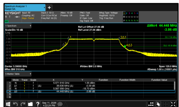
Figure 539 - 802.11ac VHT40 Maximum 26 dB EBW
