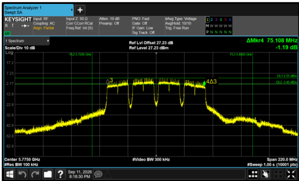
Figure 568 - 802.11a80 Minimum 6 dB EBW
