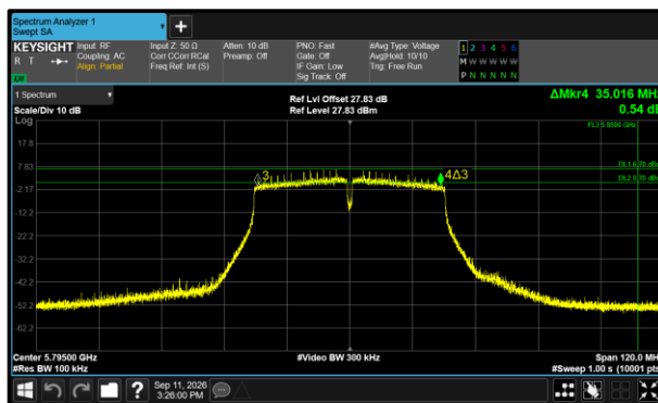
Figure 572 - 802.11n HT40 Minimum 6 dB EBW
