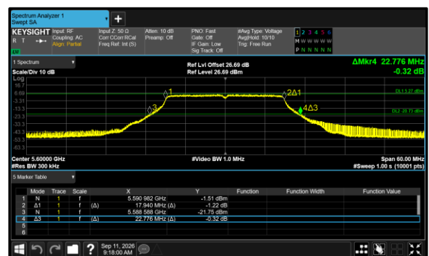
Figure 537 - 802.11ac VHT20 Maximum 26 dB EBW
