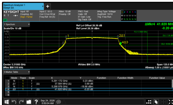
Figure 530 - 802.11ax HE40 SU Minimum 26 dB EBW
