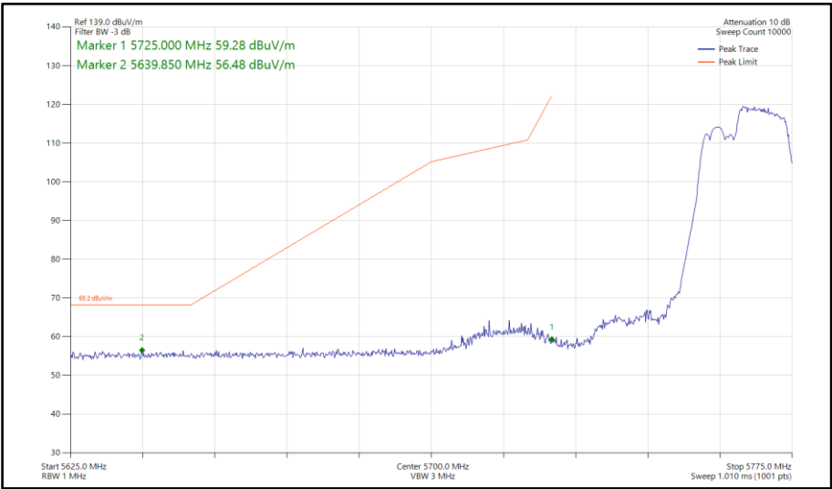
Figure 830 - 802.11be EHT40, RU106+26-85, SISO, Core 1 - 5755 MHz Band Edge Frequency 5725 MHz
