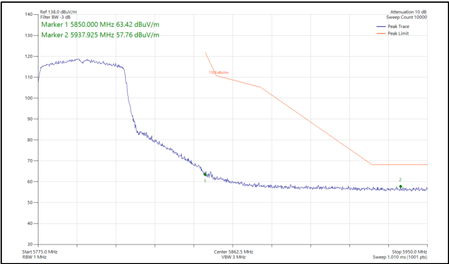
Figure 846 - 802.11ax HE40, SU, SISO, Core 1 - 5795 MHz Band Edge Frequency 5850 MHz
