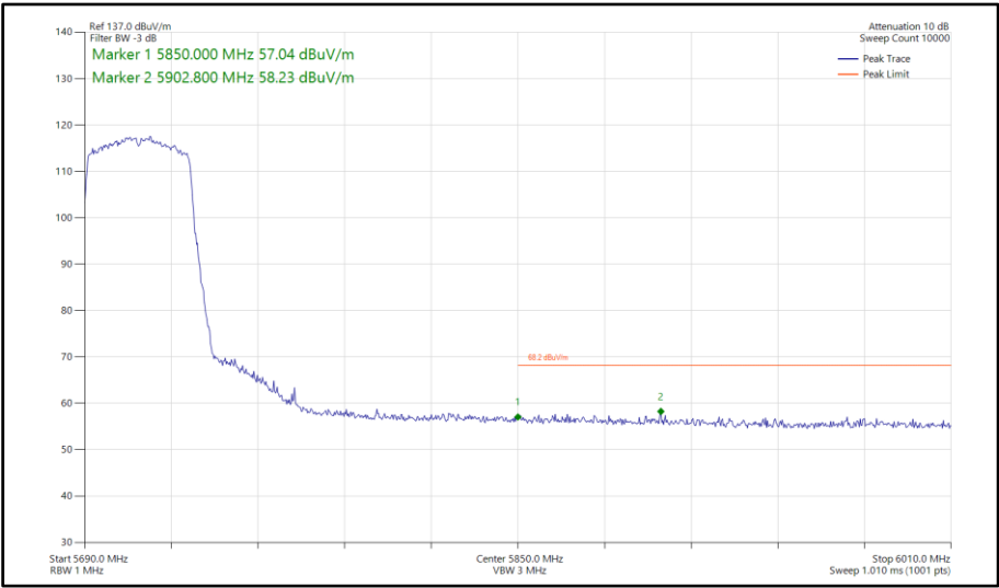
Figure 806 - 802.11ax HE40, SU, SISO, Core 0 - 5710 MHz Band Edge Frequency 5850 MHz
