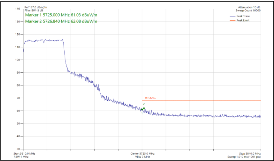
Figure 834 - 802.11ax HE40, SU, SISO, Core 1 - 5630 MHz Band Edge Frequency 5725 MHz
