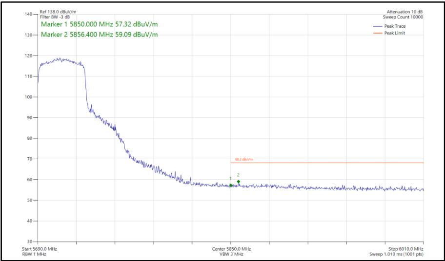
Figure 844 - 802.11ax HE40, SU, SISO, Core 1 - 5710 MHz Band Edge Frequency 5850 MHz
