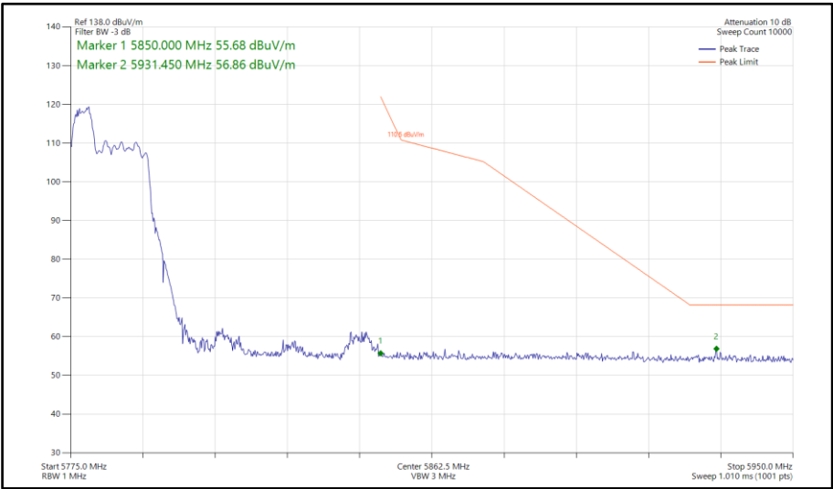
Figure 809 - 802.11ax HE40, RU52-37, SISO, Core 0 - 5795 MHz Band Edge Frequency 5850 MHz
