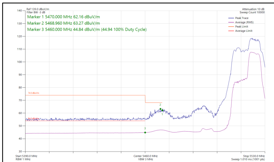
Figure 823 - 802.11be EHT40, RU52+26-75, SISO, Core 1 - 5510 MHz Band Edge Frequency 5470 MHz
