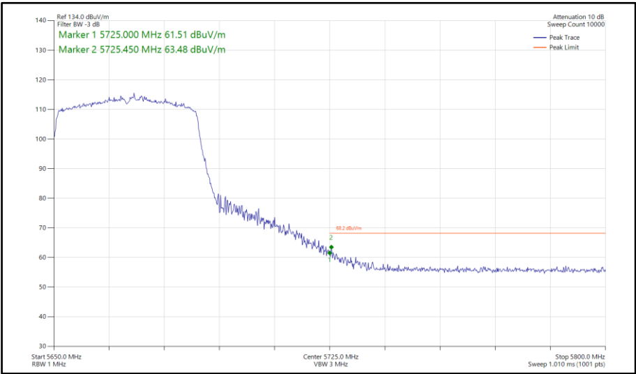
Figure 836 - 802.11ax HE40, SU, SISO, Core 1 - 5670 MHz Band Edge Frequency 5725 MHz
