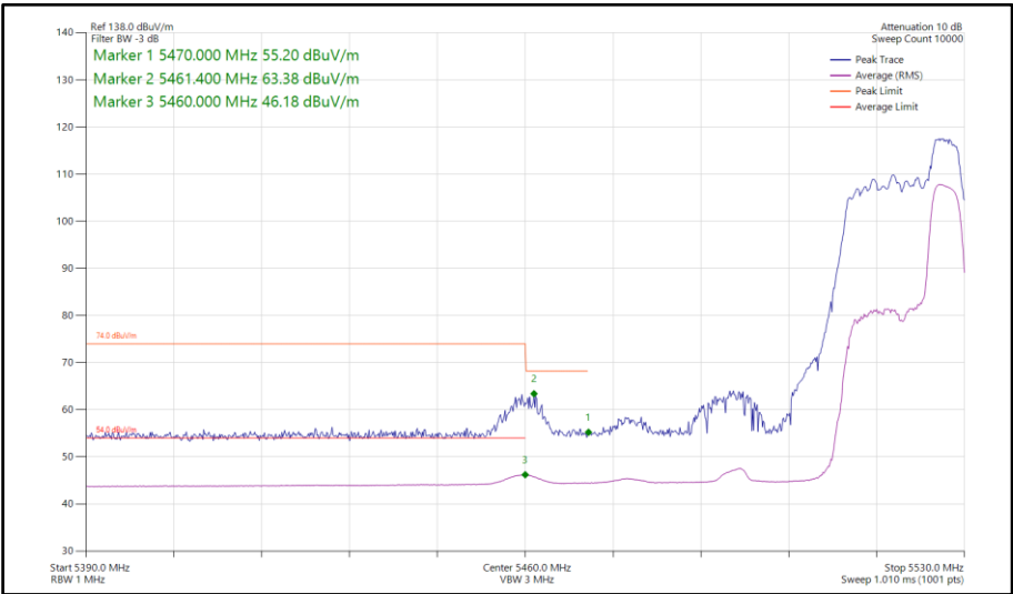
Figure 780 - 802.11ax HE40, RU52-44, SISO, Core 0 - 5510 MHz Band Edge Frequency 5470 MHz
