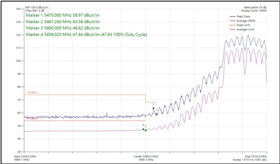
Figure 850 - 802.11a a40, CDD, Core 0-1 - 5550 MHz Band Edge Frequency 5470 MHz
