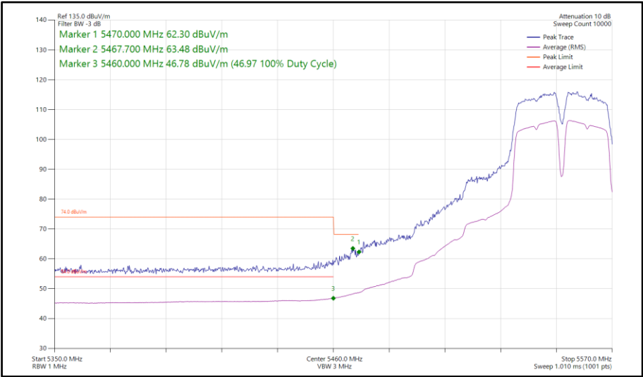
Figure 812 - 802.11a a40, SISO, Core 1 - 5550 MHz Band Edge Frequency 5470 MHz
