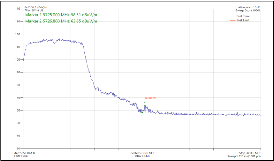
Figure 833 - 802.11n HT40, SISO, Core 1 - 5670 MHz Band Edge Frequency 5725 MHz
