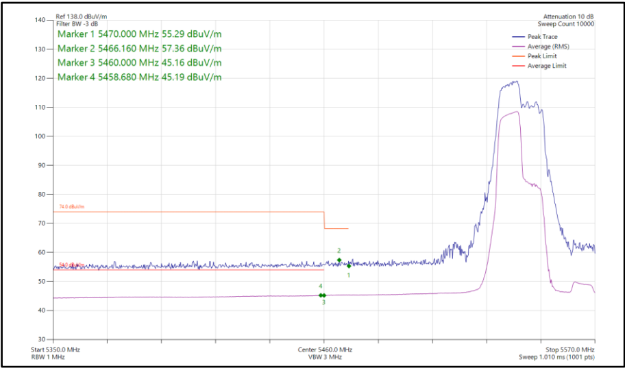
Figure 782 - 802.11ax HE40, RU106-53, SISO, Core 0 - 5550 MHz Band Edge Frequency 5470 MHz
