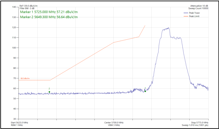
Figure 792 - 802.11be EHT40, RU52+26-70, SISO, Core 0 - 5755 MHz Band Edge Frequency 5725 MHz
