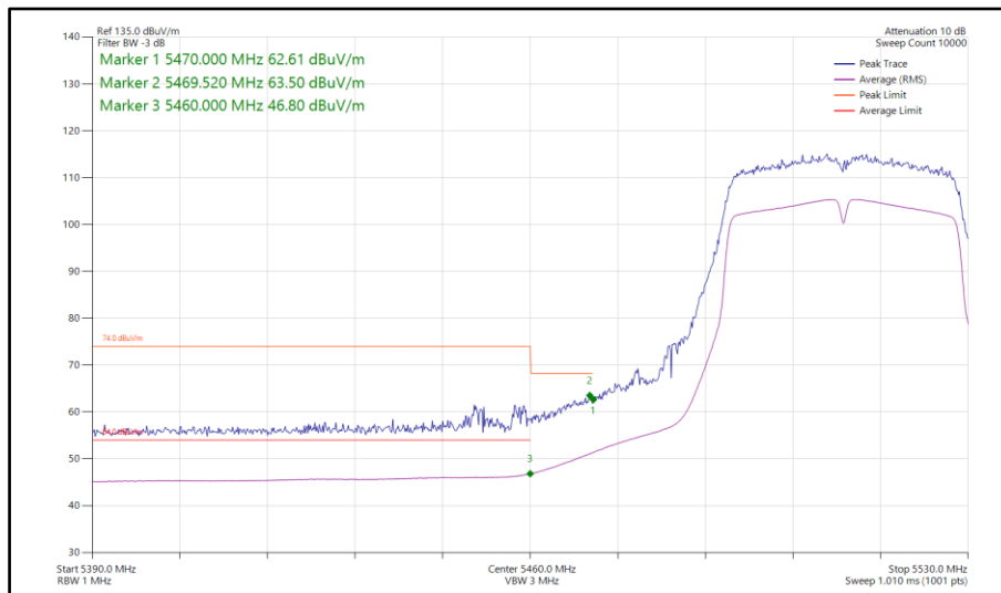
Figure 776 - 802.11n HT40, SISO, Core 0 - 5510 MHz Band Edge Frequency 5470 MHz
