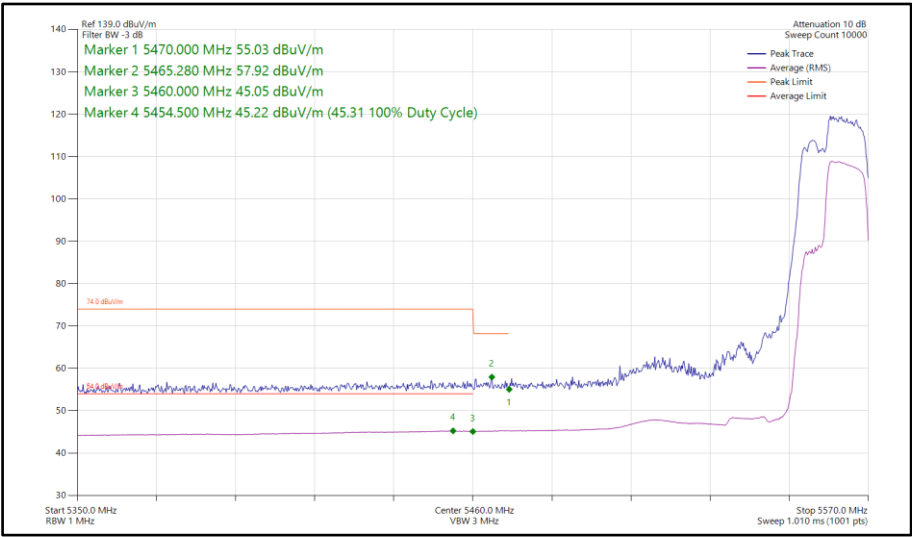
Figure 786 - 802.11be EHT40, RU106+26-85, SISO, Core 0 - 5550 MHz Band Edge Frequency 5470 MHz
