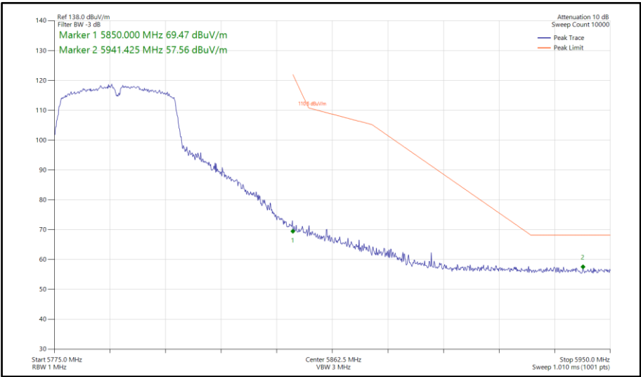
Figure 805 - 802.11n HT40, SISO, Core 0 - 5795 MHz Band Edge Frequency 5850 MHz
