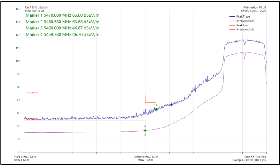
Figure 815 - 802.11n HT40, SISO, Core 1 - 5550 MHz Band Edge Frequency 5470 MHz
