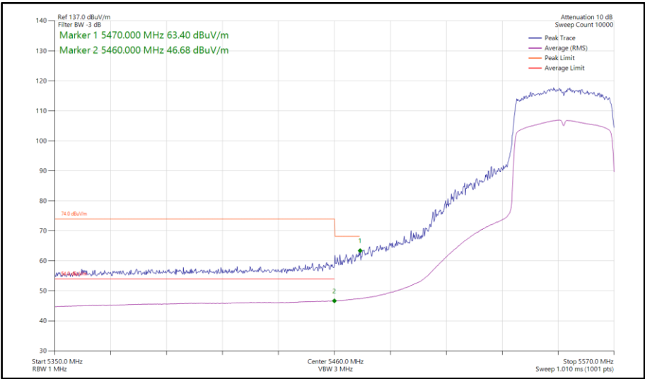
Figure 781 - 802.11ax HE40, SU, SISO, Core 0 - 5550 MHz Band Edge Frequency 5470 MHz
