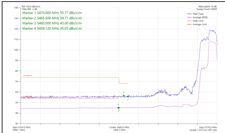
Figure 820 - 802.11ax HE40, RU106-56, SISO, Core 1 - 5550 MHz Band Edge Frequency 5470 MHz
