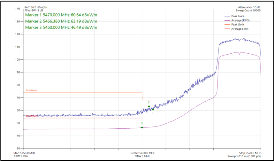
Figure 819 - 802.11ax HE40, SU, SISO, Core 1 - 5550 MHz Band Edge Frequency 5470 MHz
