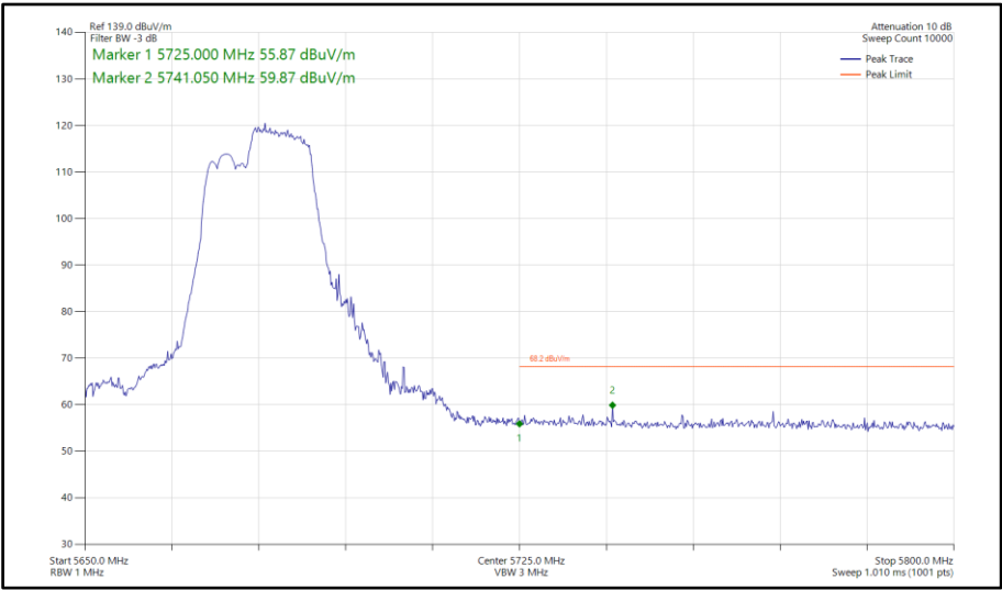
Figure 839 - 802.11be EHT40, RU106+26-85, SISO, Core 1 - 5670 MHz Band Edge Frequency 5725 MHz
