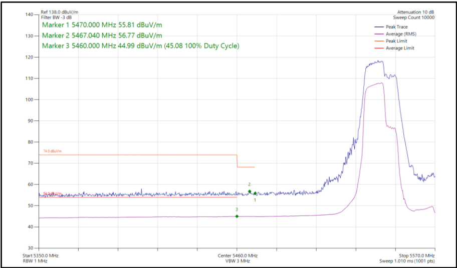
Figure 824 - 802.11be EHT40, RU106+26-82, SISO, Core 1 - 5550 MHz Band Edge Frequency 5470 MHz
