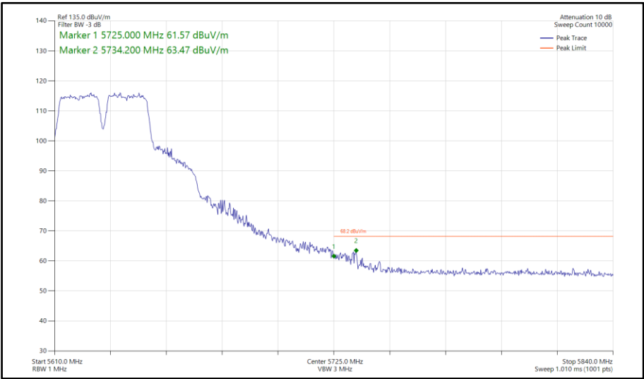
Figure 793 - 802.11a a40, SISO, Core 0 - 5630 MHz Band Edge Frequency 5725 MHz
