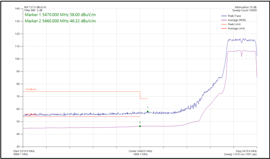
Figure 778 - 802.11n HT40, SISO, Core 0 - 5590 MHz Band Edge Frequency 5470 MHz
