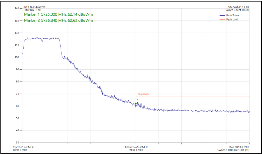
Figure 832 - 802.11n HT40, SISO, Core 1 - 5630 MHz Band Edge Frequency 5725 MHz
