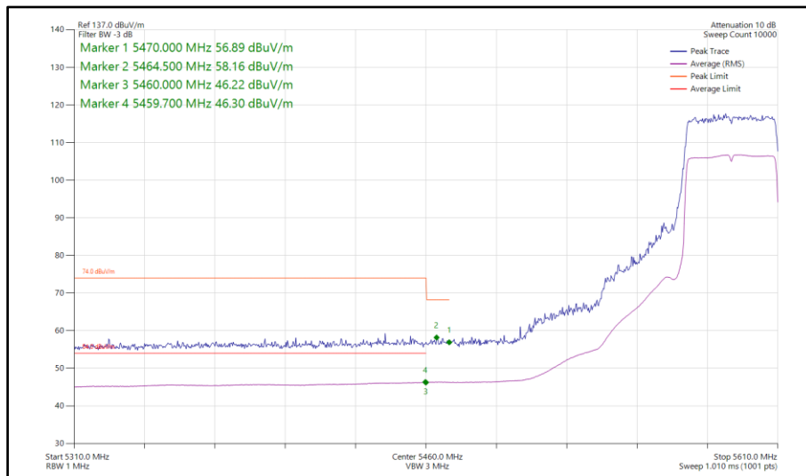
Figure 821 - 802.11ax HE40, SU, SISO, Core 1 - 5590 MHz Band Edge Frequency 5470 MHz
