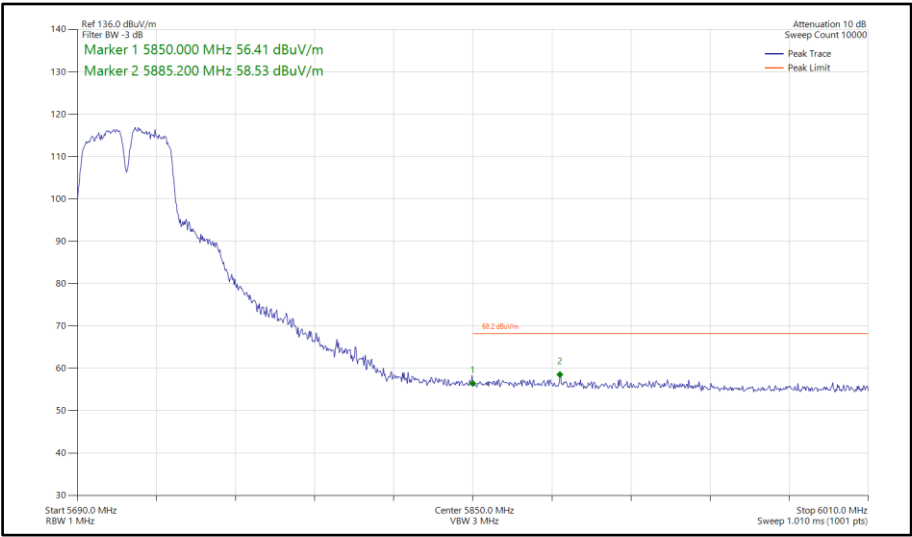
Figure 802 - 802.11a a40, SISO, Core 0 - 5710 MHz Band Edge Frequency 5850 MHz
