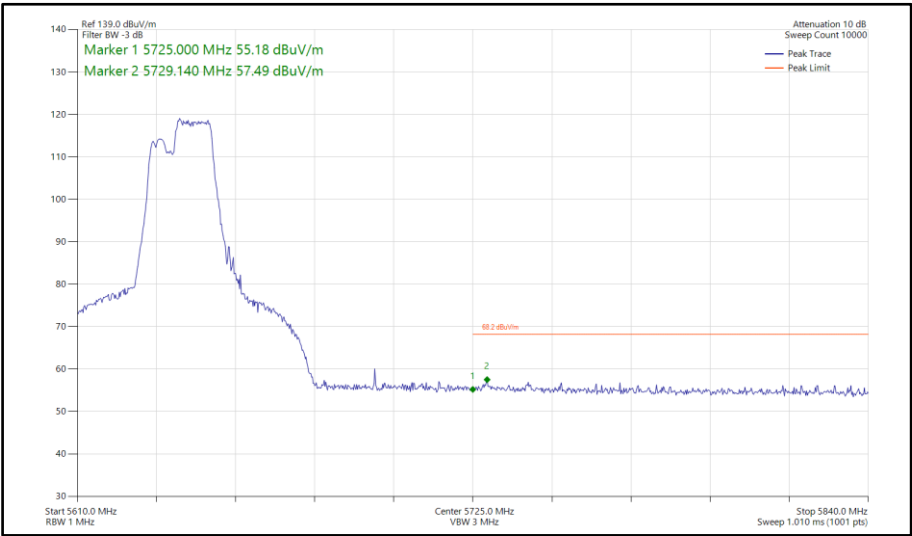
Figure 838 - 802.11be EHT40, RU106+26-85, SISO, Core 1 - 5630 MHz Band Edge Frequency 5725 MHz
