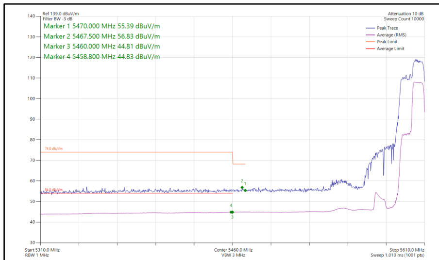
Figure 822 - 802.11ax HE40, RU106-56, SISO, Core 1 - 5590 MHz Band Edge Frequency 5470 MHz
