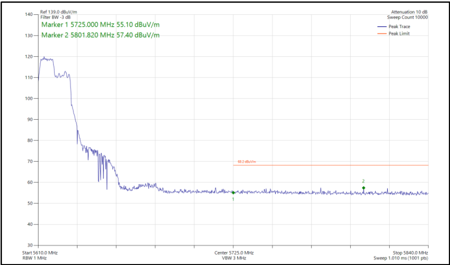
Figure 797 - 802.11ax HE40, RU106-53, SISO, Core 0 - 5630 MHz Band Edge Frequency 5725 MHz
