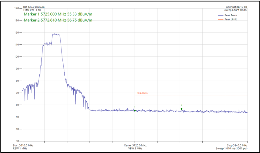
Figure 835 - 802.11ax HE40, RU106-56, SISO, Core 1 - 5630 MHz Band Edge Frequency 5725 MHz
