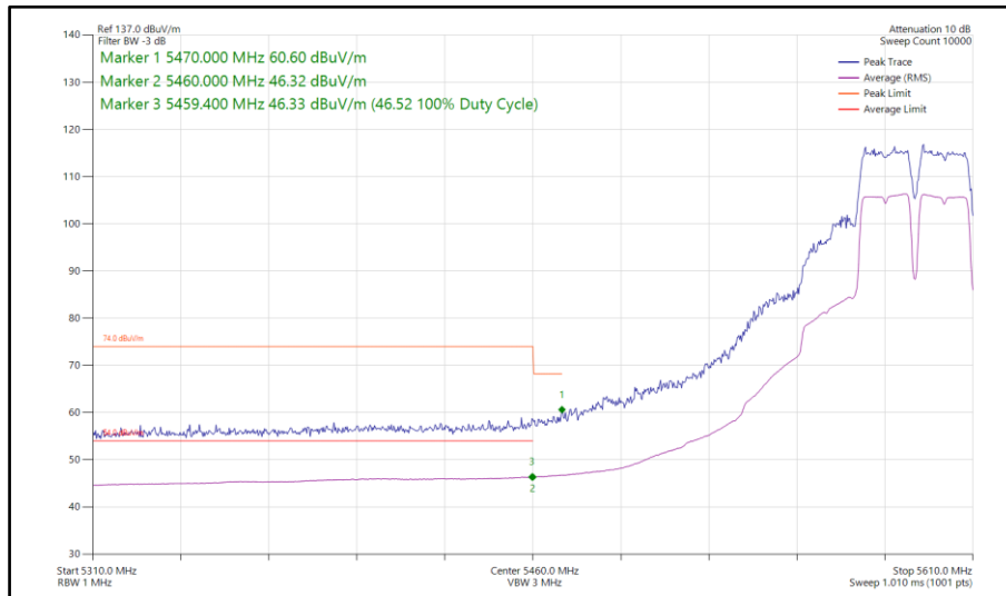
Figure 775 - 802.11a a40, SISO, Core 0 - 5590 MHz Band Edge Frequency 5470 MHz
