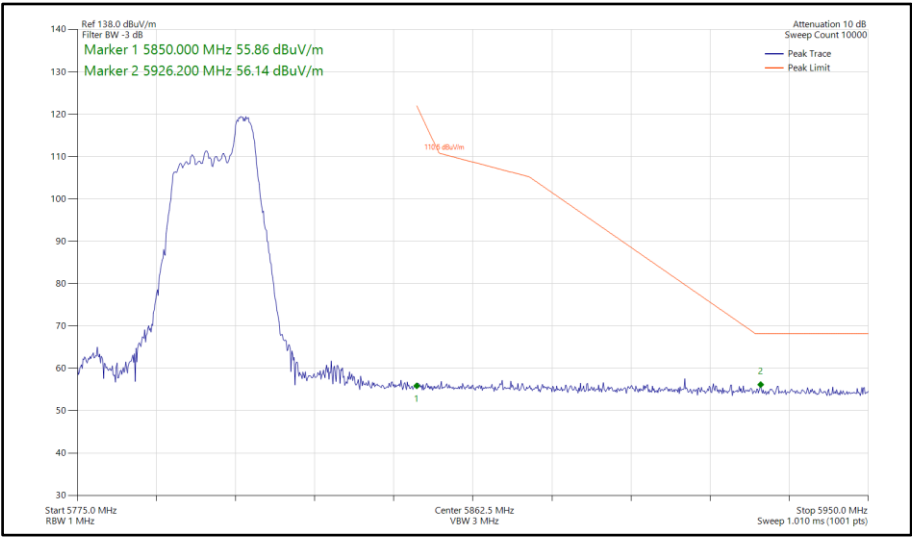
Figure 847 - 802.11ax HE40, RU52-44, SISO, Core 1 - 5795 MHz Band Edge Frequency 5850 MHz
