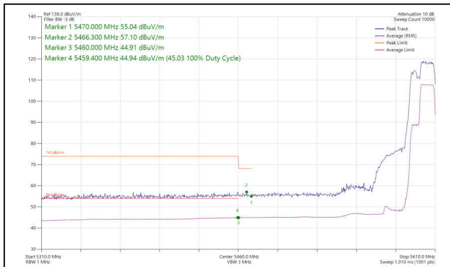
Figure 787 - 802.11be EHT40, RU106+26-85, SISO, Core 0 - 5590 MHz Band Edge Frequency 5470 MHz
