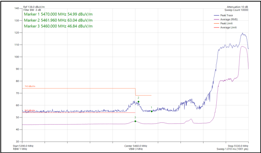
Figure 818 - 802.11ax HE40, RU52-44, SISO, Core 1 - 5510 MHz Band Edge Frequency 5470 MHz
