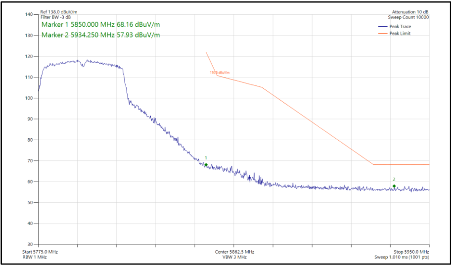
Figure 843 - 802.11n HT40, SISO, Core 1 - 5795 MHz Band Edge Frequency 5850 MHz
