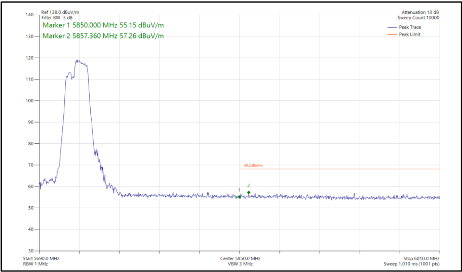
Figure 810 - 802.11be EHT40, RU106+26-85, SISO, Core 0 - 5710 MHz Band Edge Frequency 5850 MHz
