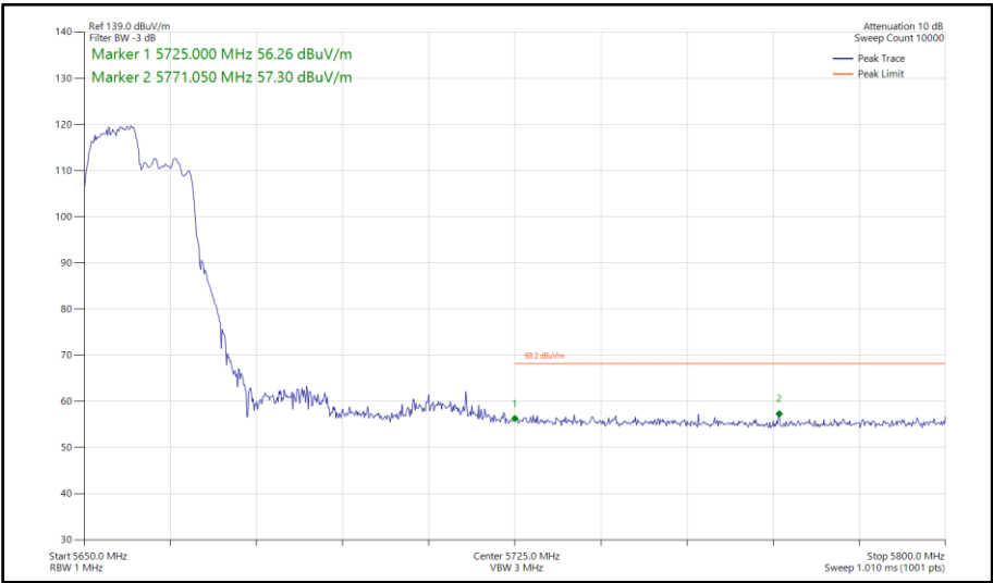
Figure 799 - 802.11ax HE40, RU106-53, SISO, Core 0 - 5670 MHz Band Edge Frequency 5725 MHz
