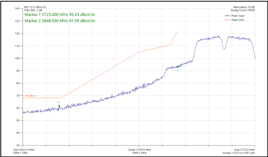
Figure 826 - 802.11a a40, SISO, Core 1 - 5755 MHz Band Edge Frequency 5725 MHz
