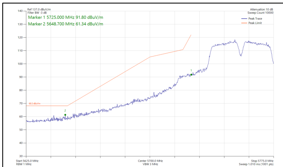
Figure 788 - 802.11a a40, SISO, Core 0 - 5755 MHz Band Edge Frequency 5725 MHz
