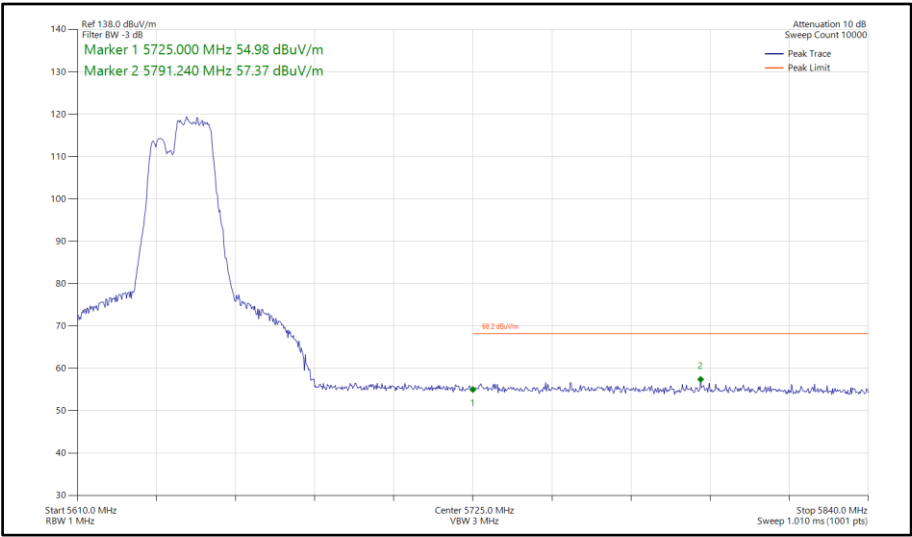
Figure 800 - 802.11be EHT40, RU106+26-85, SISO, Core 0 - 5630 MHz Band Edge Frequency 5725 MHz
