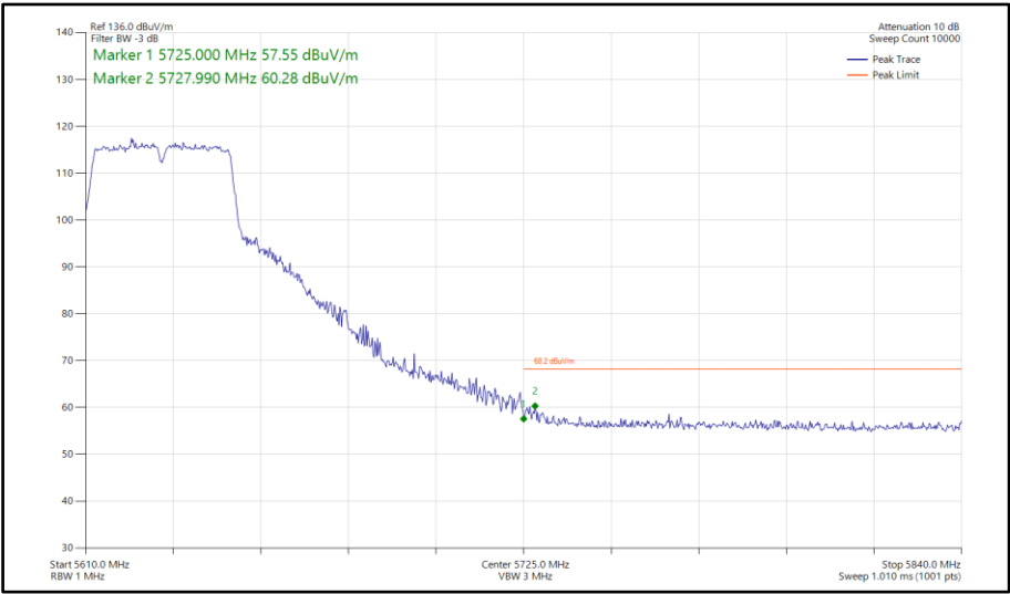
Figure 794 - 802.11n HT40, SISO, Core 0 - 5630 MHz Band Edge Frequency 5725 MHz
