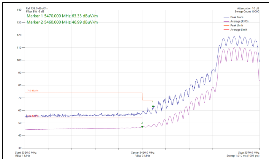
Figure 853 - 802.11n HT40, CDD, Core 0-1 - 5550 MHz Band Edge Frequency 5470 MHz
