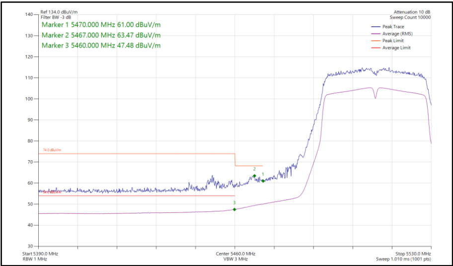
Figure 814 - 802.11n HT40, SISO, Core 1 - 5510 MHz Band Edge Frequency 5470 MHz
