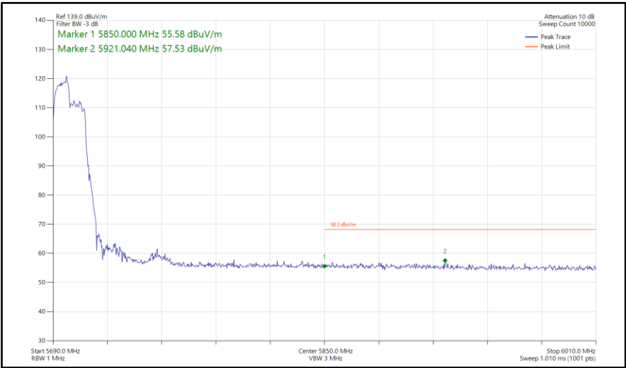
Figure 807 - 802.11ax HE40, RU106-53, SISO, Core 0 - 5710 MHz Band Edge Frequency 5850 MHz
