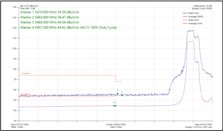
Figure 825 - 802.11be EHT40, RU106+26-82, SISO, Core 1 - 5590 MHz Band Edge Frequency 5470 MHz
