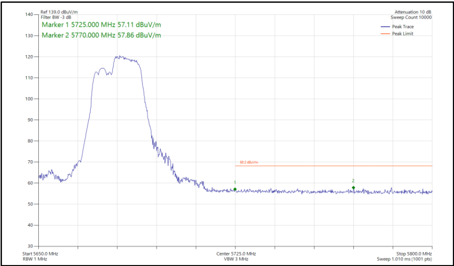
Figure 801 - 802.11be EHT40, RU106+26-85, SISO, Core 0 - 5670 MHz Band Edge Frequency 5725 MHz
