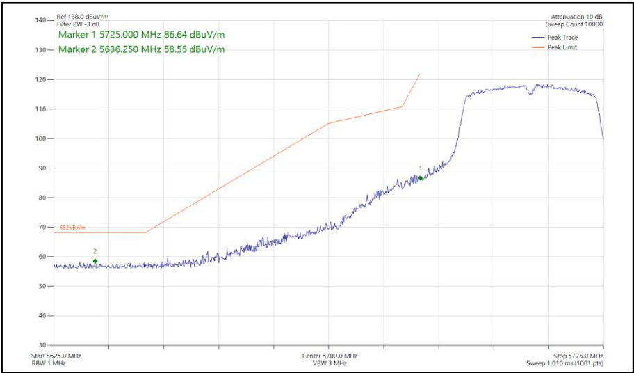
Figure 789 - 802.11n HT40, SISO, Core 0 - 5755 MHz Band Edge Frequency 5725 MHz
