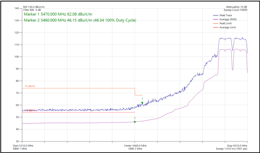
Figure 813 - 802.11a a40, SISO, Core 1 - 5590 MHz Band Edge Frequency 5470 MHz
