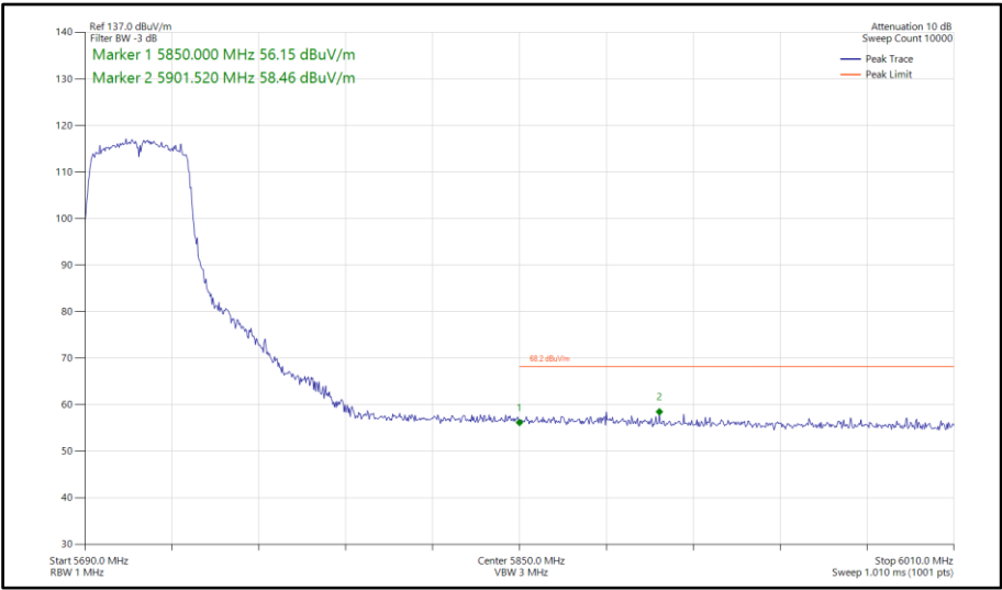
Figure 804 - 802.11n HT40, SISO, Core 0 - 5710 MHz Band Edge Frequency 5850 MHz
