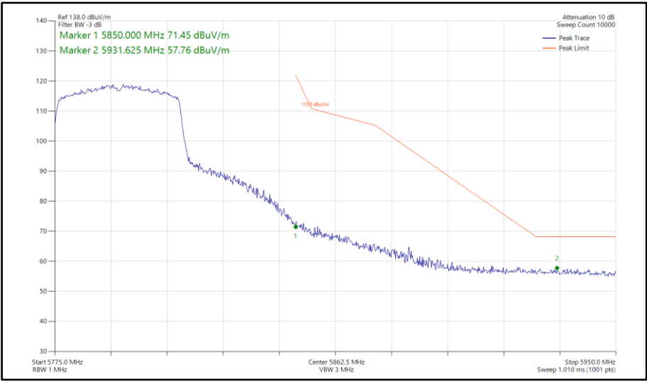
Figure 808 - 802.11ax HE40, SU, SISO, Core 0 - 5795 MHz Band Edge Frequency 5850 MHz
