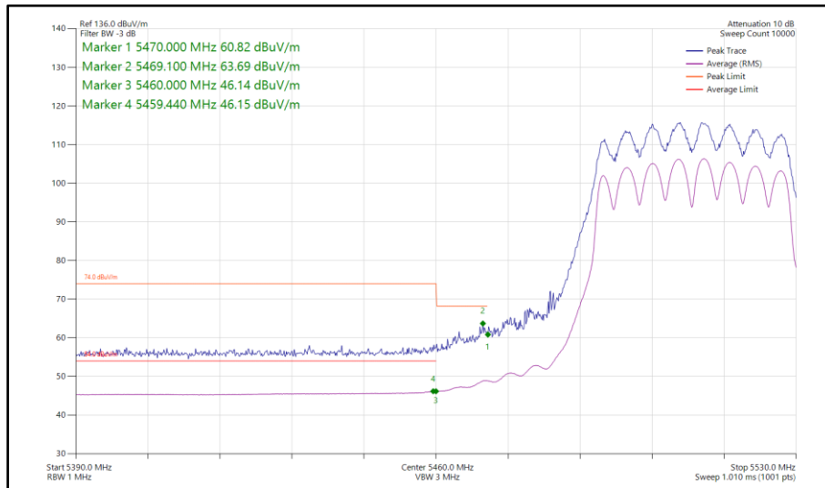
Figure 852 - 802.11n HT40, CDD, Core 0-1 - 5510 MHz Band Edge Frequency 5470 MHz
