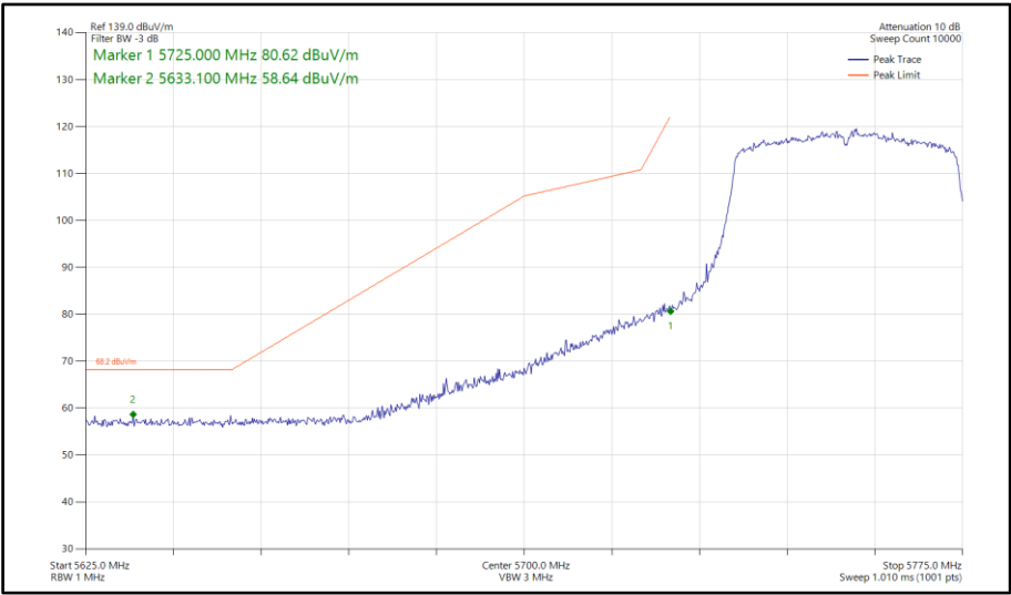
Figure 790 - 802.11ax HE40, SU, SISO, Core 0 - 5755 MHz Band Edge Frequency 5725 MHz
