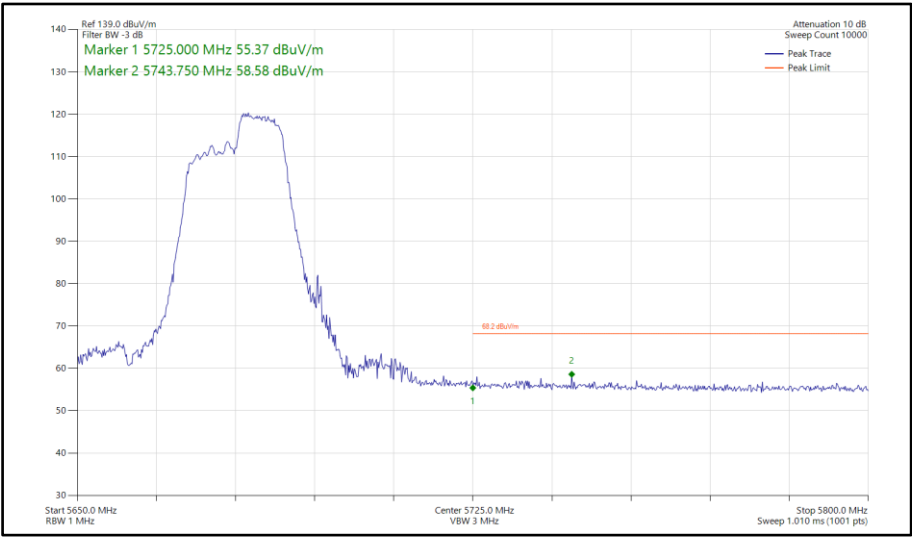
Figure 837 - 802.11ax HE40, RU106-56, SISO, Core 1 - 5670 MHz Band Edge Frequency 5725 MHz
