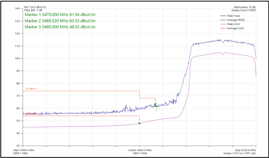
Figure 817 - 802.11ax HE40, SU, SISO, Core 1 - 5510 MHz Band Edge Frequency 5470 MHz
