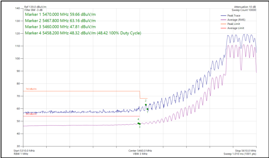
Figure 851 - 802.11a a40, CDD, Core 0-1 - 5590 MHz Band Edge Frequency 5470 MHz
