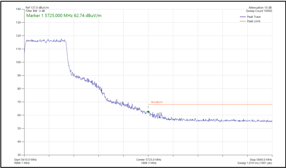
Figure 796 - 802.11ax HE40, SU, SISO, Core 0 - 5630 MHz Band Edge Frequency 5725 MHz
