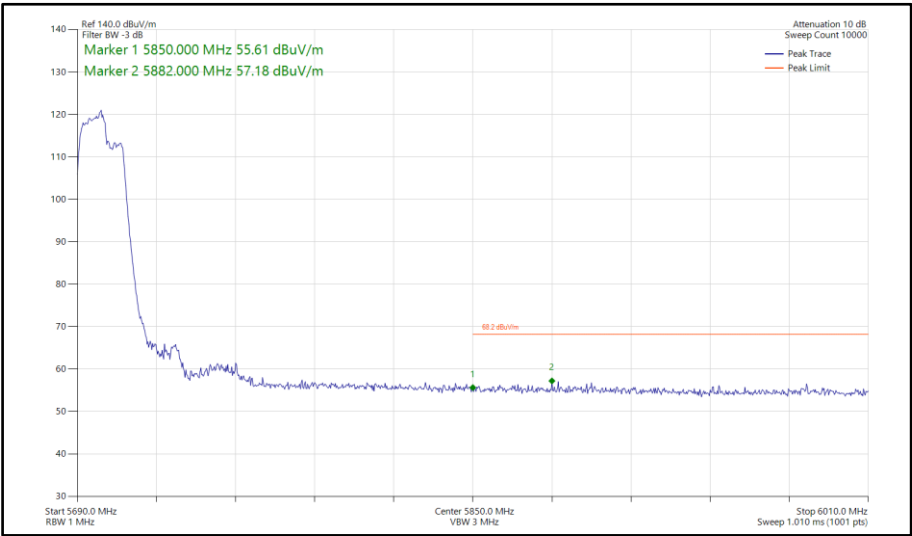
Figure 848 - 802.11be EHT40, RU106+26-82, SISO, Core 1 - 5710 MHz Band Edge Frequency 5850 MHz
