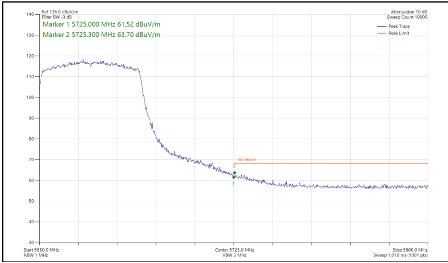
Figure 798 - 802.11ax HE40, SU, SISO, Core 0 - 5670 MHz Band Edge Frequency 5725 MHz
