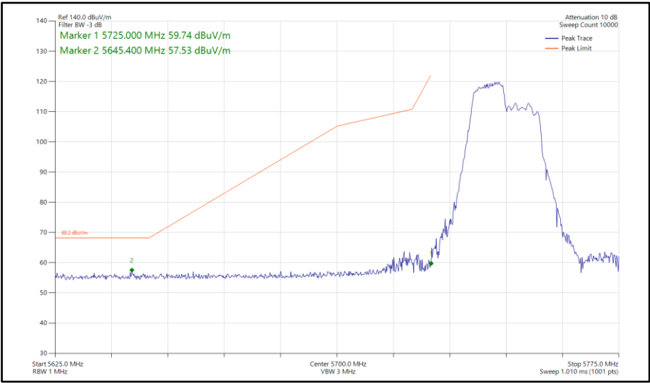
Figure 829 - 802.11ax HE40, RU106-53, SISO, Core 1 - 5755 MHz Band Edge Frequency 5725 MHz
