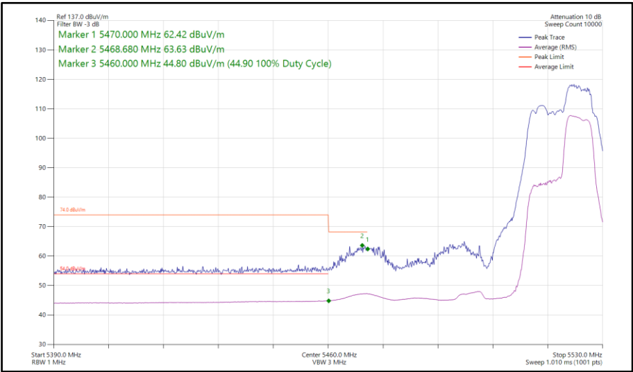
Figure 785 - 802.11be EHT40, RU52+26-75, SISO, Core 0 - 5510 MHz Band Edge Frequency 5470 MHz
