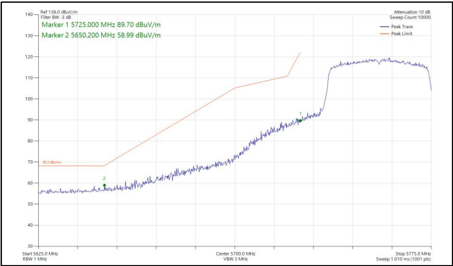
Figure 828 - 802.11ax HE40, SU, SISO, Core 1 - 5755 MHz Band Edge Frequency 5725 MHz
