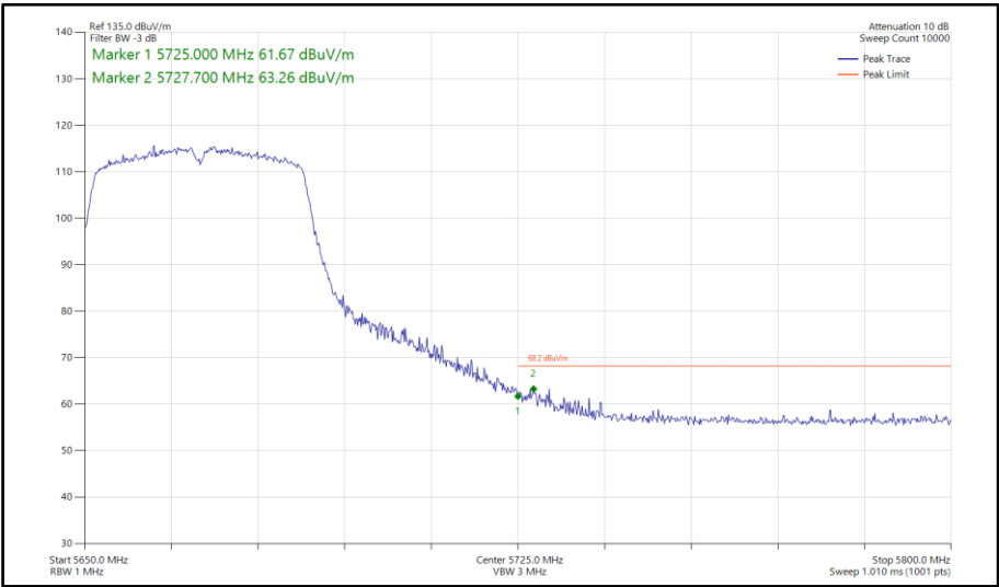
Figure 795 - 802.11n HT40, SISO, Core 0 - 5670 MHz Band Edge Frequency 5725 MHz
