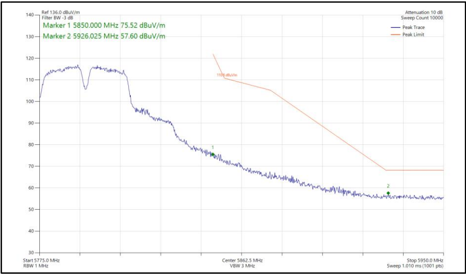
Figure 841 - 802.11a a40, SISO, Core 1 - 5795 MHz Band Edge Frequency 5850 MHz
