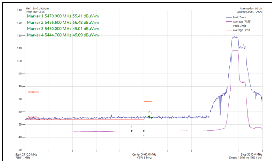
Figure 784 - 802.11ax HE40, RU106-53, SISO, Core 0 - 5590 MHz Band Edge Frequency 5470 MHz
