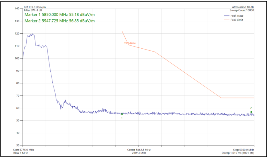
Figure 811 - 802.11be EHT40, RU52+26-70, SISO, Core 0 - 5795 MHz Band Edge Frequency 5850 MHz
