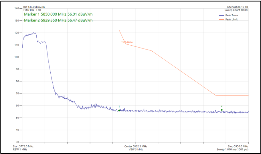
Figure 849 - 802.11be EHT40, RU106+26-82, SISO, Core 1 - 5795 MHz Band Edge Frequency 5850 MHz
