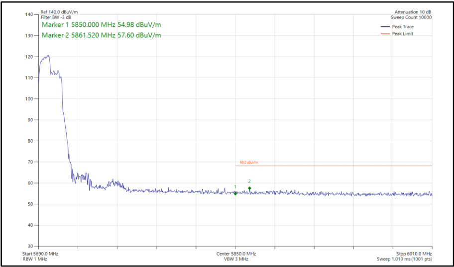
Figure 845 - 802.11ax HE40, RU106-53, SISO, Core 1 - 5710 MHz Band Edge Frequency 5850 MHz
