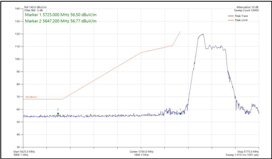
Figure 791 - 802.11ax HE40, RU52-37, SISO, Core 0 - 5755 MHz Band Edge Frequency 5725 MHz
