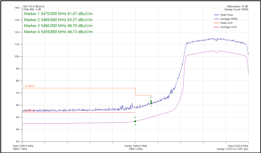
Figure 779 - 802.11ax HE40, SU, SISO, Core 0 - 5510 MHz Band Edge Frequency 5470 MHz
