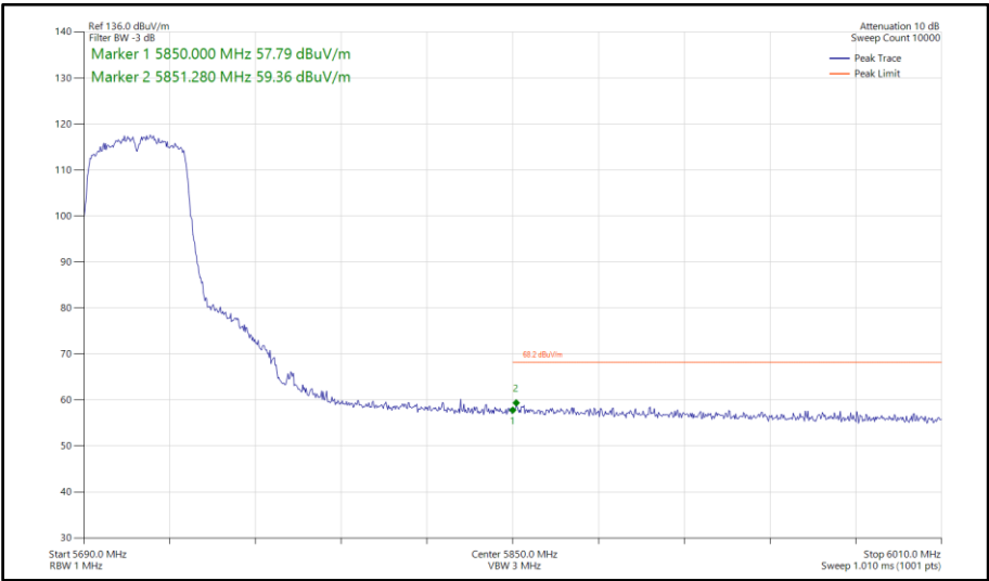
Figure 842 - 802.11n HT40, SISO, Core 1 - 5710 MHz Band Edge Frequency 5850 MHz
