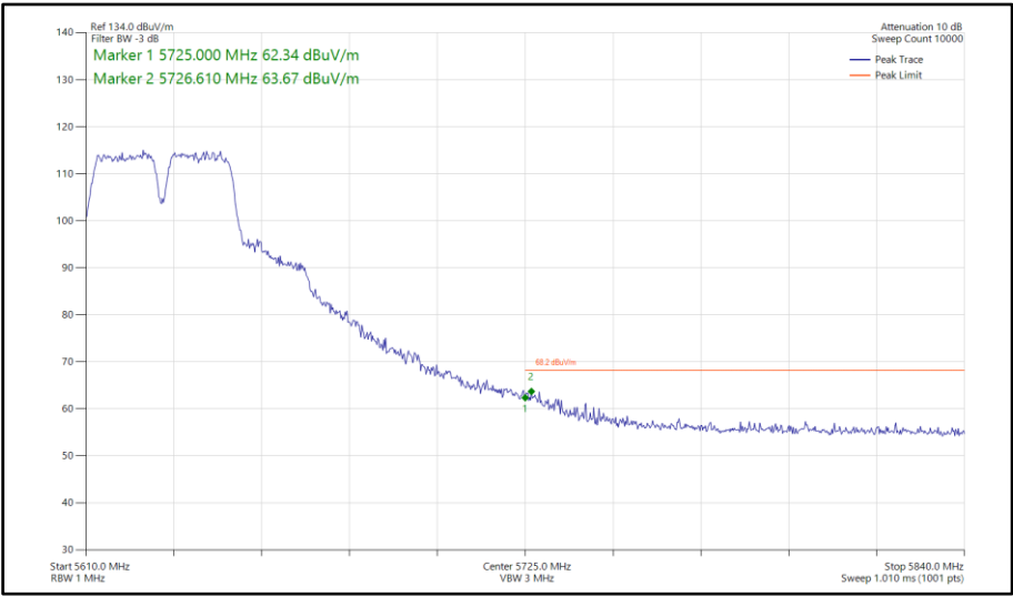
Figure 831 - 802.11a a40, SISO, Core 1 - 5630 MHz Band Edge Frequency 5725 MHz
