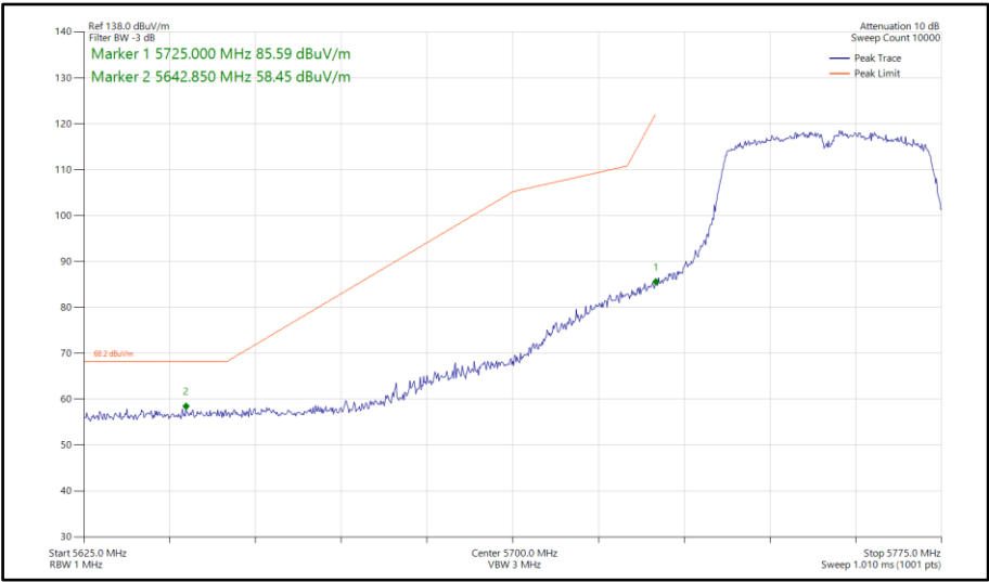
Figure 827 - 802.11n HT40, SISO, Core 1 - 5755 MHz Band Edge Frequency 5725 MHz
