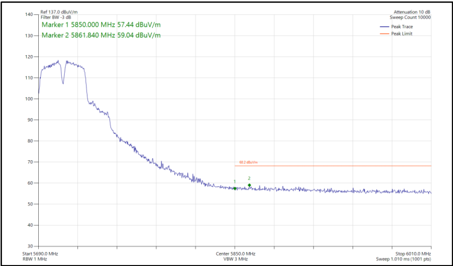
Figure 840 - 802.11a a40, SISO, Core 1 - 5710 MHz Band Edge Frequency 5850 MHz
