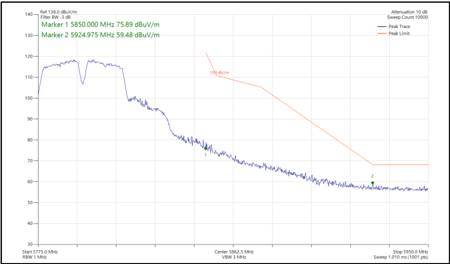
Figure 803 - 802.11a a40, SISO, Core 0 - 5795 MHz Band Edge Frequency 5850 MHz
