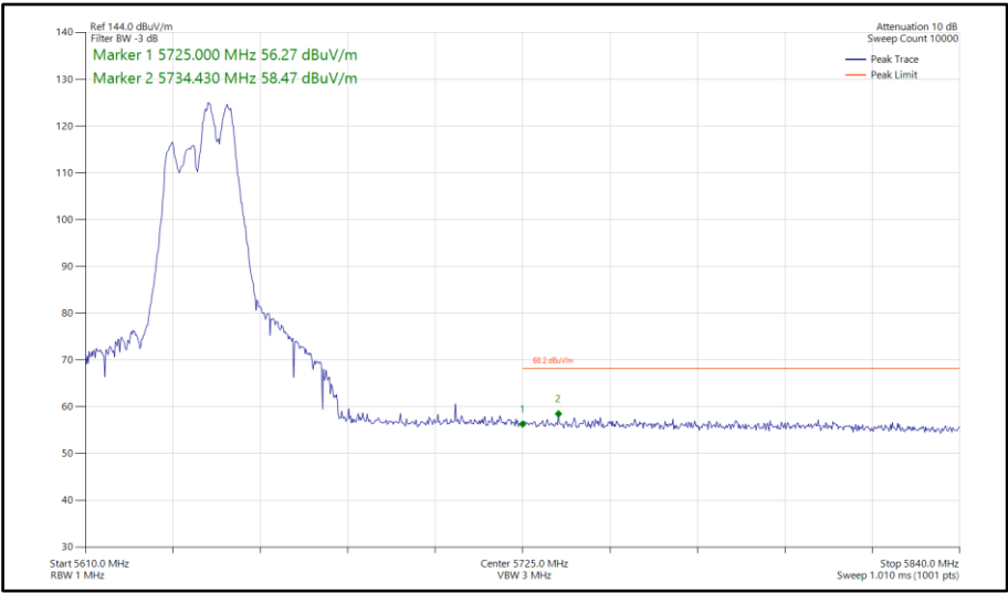
Figure 908 - 802.11ax HE40, RU106-56, SDM, Core 0-1 - 5630 MHz Band Edge Frequency 5725 MHz
