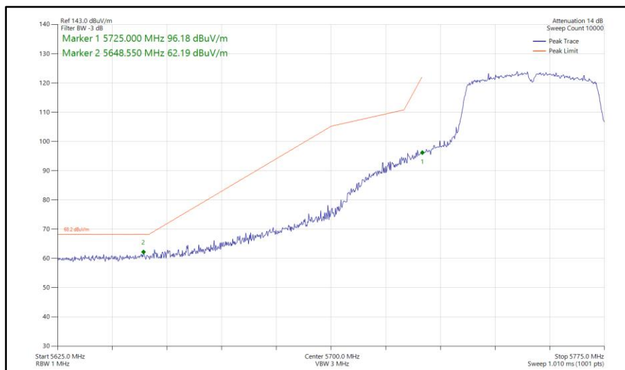
Figure 927 - 802.11ac VHT40, TxBF, Core 0-1 - 5755 MHz Band Edge Frequency 5725 MHz
