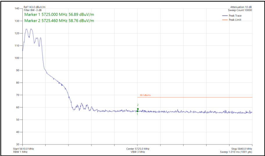
Figure 911 - 802.11be EHT40, RU106+26-82, SDM, Core 0-1 - 5630 MHz Band Edge Frequency 5725 MHz
