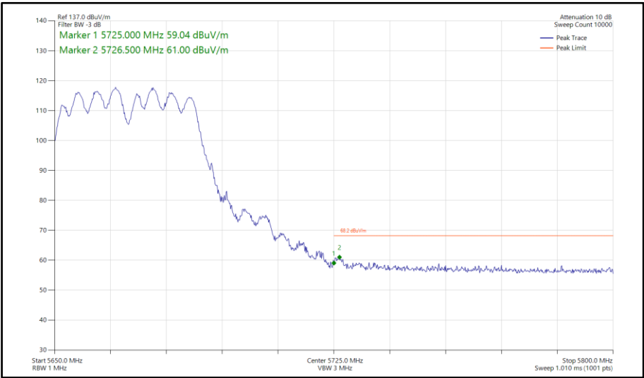
Figure 870 - 802.11a a40, CDD, Core 0-1 - 5670 MHz Band Edge Frequency 5725 MHz
