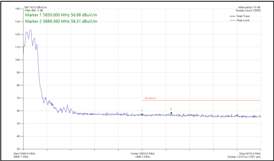
Figure 919 - 802.11be EHT40, RU106+26-82, SDM, Core 0-1 - 5710 MHz Band Edge Frequency 5850 MHz
