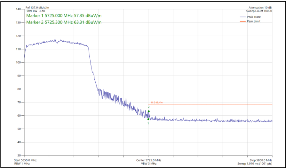
Figure 932 - 802.11ax HE40, SU, TxBF, Core 0-1 - 5670 MHz Band Edge Frequency 5725 MHz
