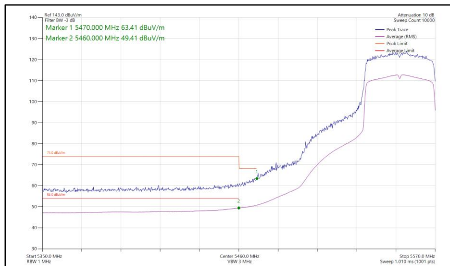
Figure 925 - 802.11ax HE40, SU, TxBF, Core 0-1 - 5550 MHz Band Edge Frequency 5470 MHz
