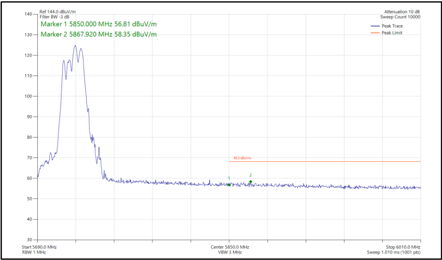
Figure 887 - 802.11be EHT40, RU106+26-85, CDD, Core 0-1 - 5710 MHz Band Edge Frequency 5850 MHz
