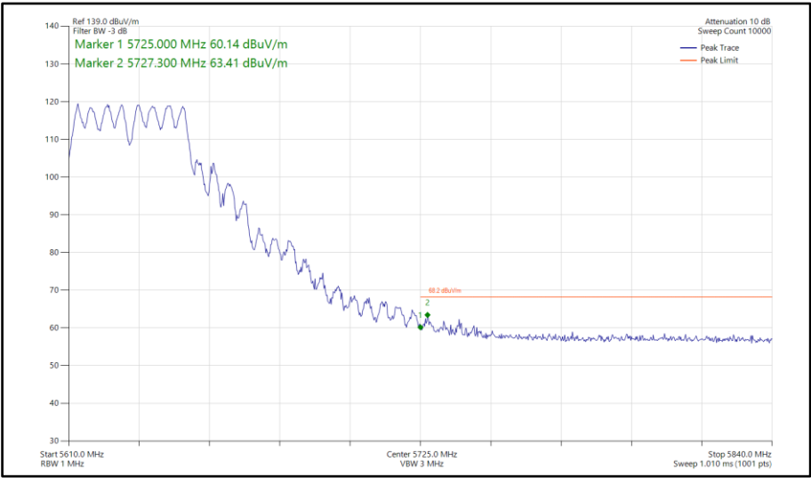
Figure 869 - 802.11a a40, CDD, Core 0-1 - 5630 MHz Band Edge Frequency 5725 MHz
