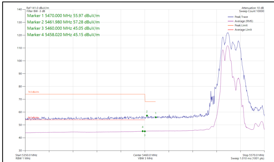
Figure 858 - 802.11ax HE40, RU106-53, CDD, Core 0-1 - 5550 MHz Band Edge Frequency 5470 MHz
