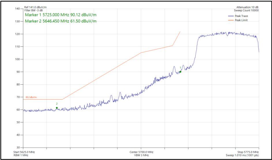
Figure 902 - 802.11ax HE40, SU, SDM, Core 0-1 - 5755 MHz Band Edge Frequency 5725 MHz
