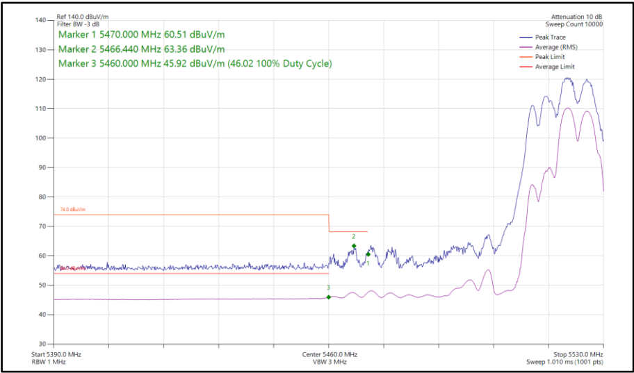
Figure 898 - 802.11be EHT40, RU106+26-85, SDM, Core 0-1 - 5510 MHz Band Edge Frequency 5470 MHz
