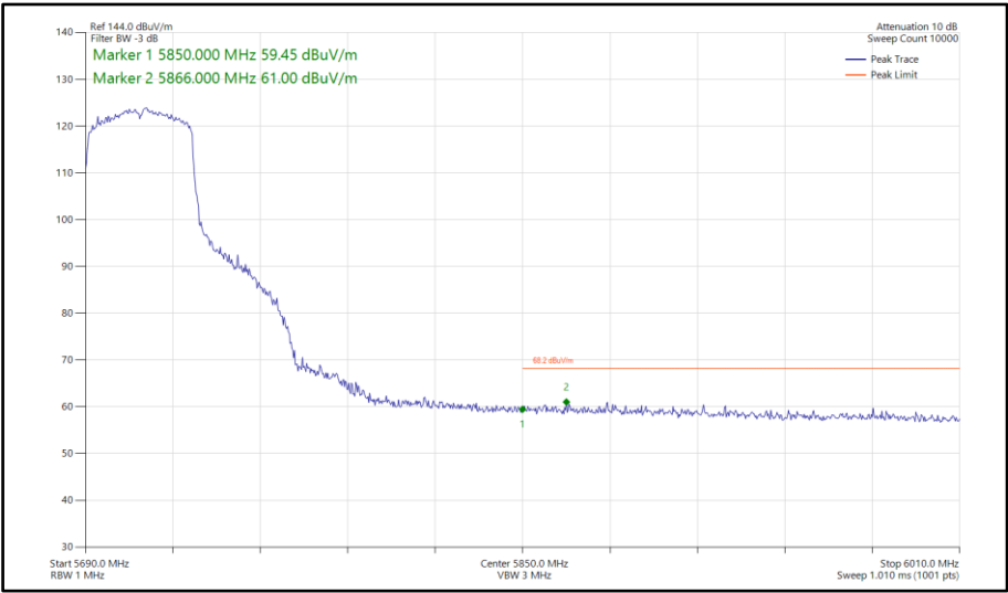
Figure 935 - 802.11ax HE40, SU, TxBF, Core 0-1 - 5710 MHz Band Edge Frequency 5850 MHz
