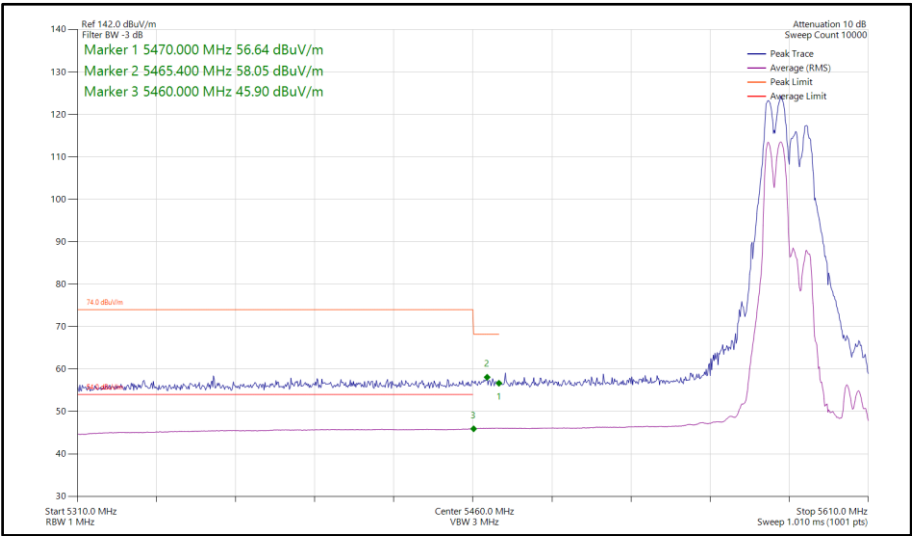
Figure 897 - 802.11ax HE40, RU106-53, SDM, Core 0-1 - 5590 MHz Band Edge Frequency 5470 MHz
