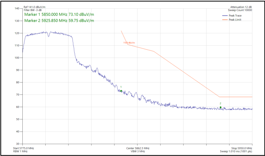
Figure 914 - 802.11n HT40, SDM, Core 0-1 - 5795 MHz Band Edge Frequency 5850 MHz
