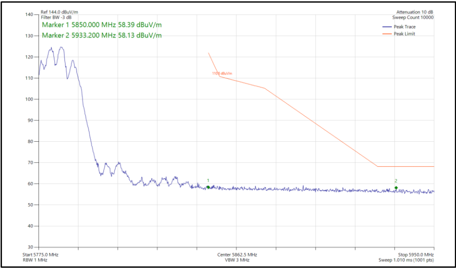
Figure 920 - 802.11be EHT40, RU106+26-82, SDM, Core 0-1 - 5795 MHz Band Edge Frequency 5850 MHz
