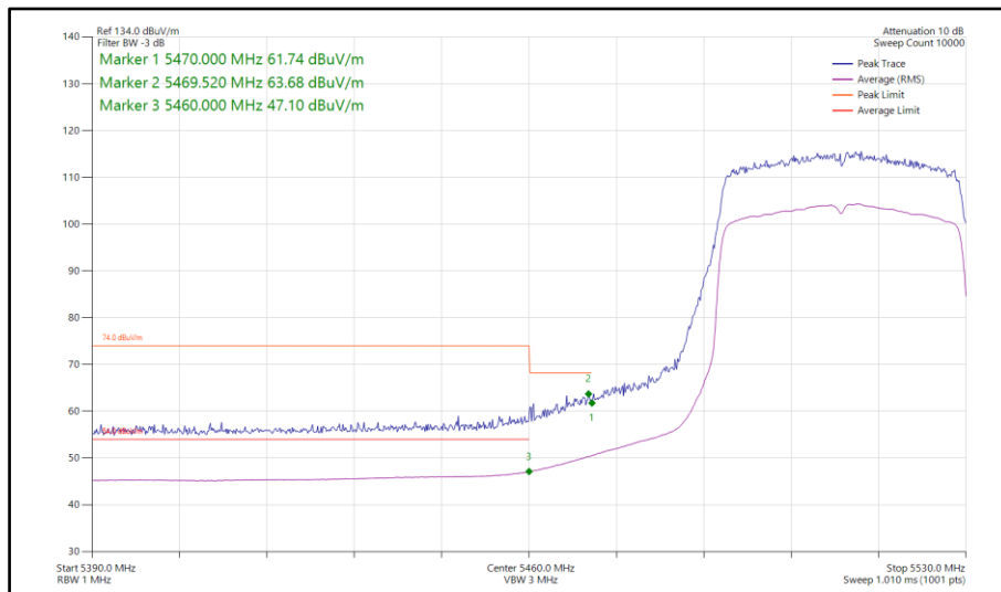
Figure 892 - 802.11ax HE40, SU, SDM, Core 0-1 - 5510 MHz Band Edge Frequency 5470 MHz
