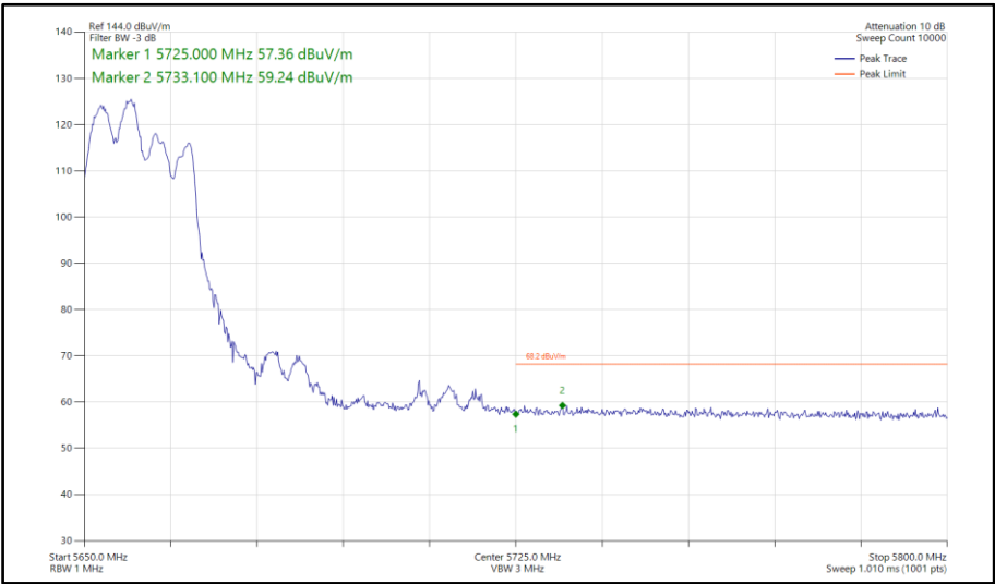
Figure 876 - 802.11ax HE40, RU106-53, CDD, Core 0-1 - 5670 MHz Band Edge Frequency 5725 MHz
