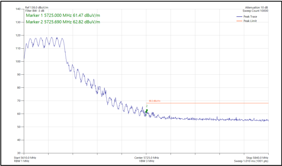
Figure 871 - 802.11n HT40, CDD, Core 0-1 - 5630 MHz Band Edge Frequency 5725 MHz
