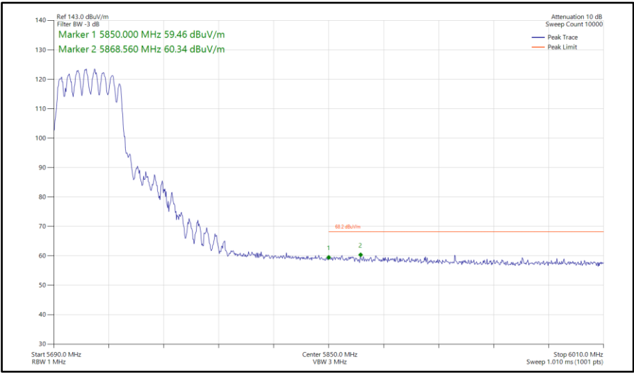
Figure 883 - 802.11ax HE40, SU, CDD, Core 0-1 - 5710 MHz Band Edge Frequency 5850 MHz
