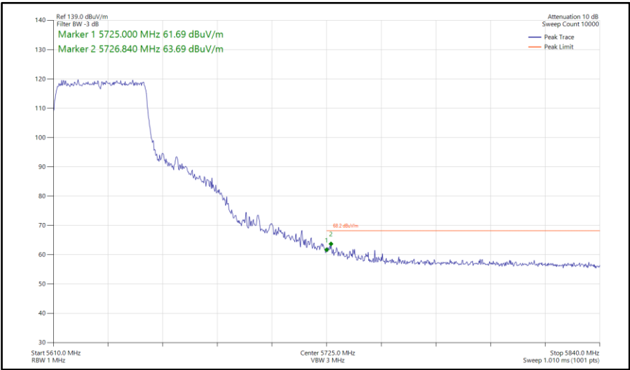
Figure 907 - 802.11ax HE40, SU, SDM, Core 0-1 - 5630 MHz Band Edge Frequency 5725 MHz
