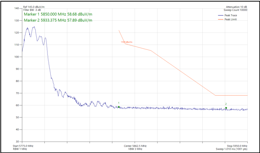
Figure 888 - 802.11be EHT40, RU106+26-82, CDD, Core 0-1 - 5795 MHz Band Edge Frequency 5850 MHz
