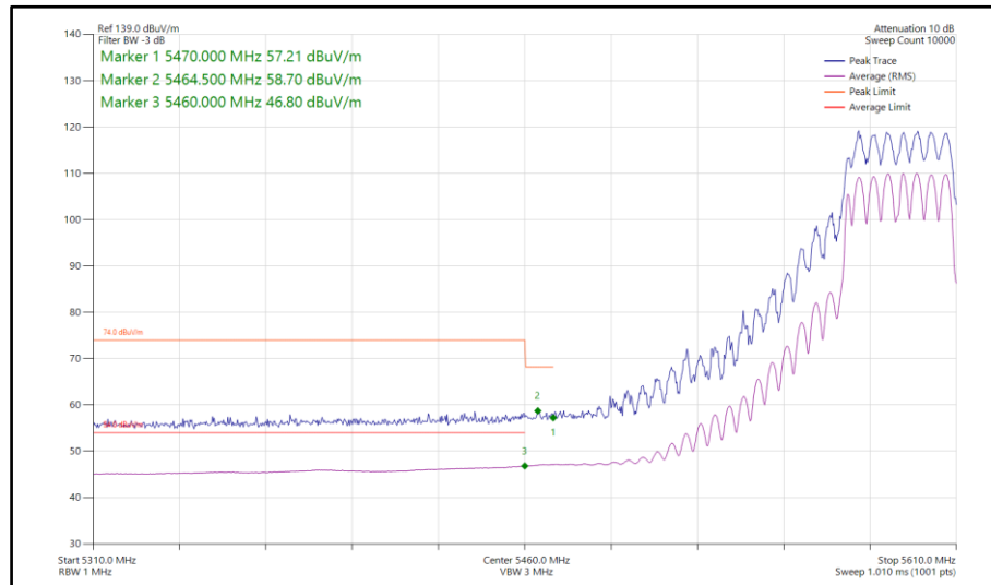
Figure 854 - 802.11n HT40, CDD, Core 0-1 - 5590 MHz Band Edge Frequency 5470 MHz
