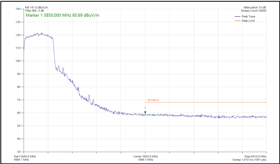
Figure 915 - 802.11ax HE40, SU, SDM, Core 0-1 - 5710 MHz Band Edge Frequency 5850 MHz
