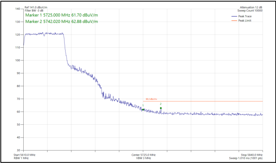
Figure 931 - 802.11ax HE40, SU, TxBF, Core 0-1 - 5630 MHz Band Edge Frequency 5725 MHz
