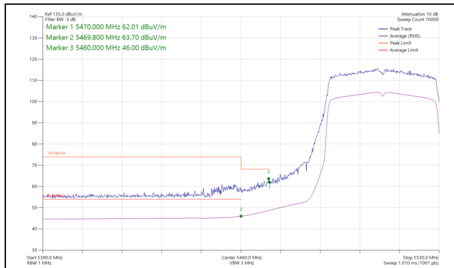
Figure 924 - 802.11ax HE40, SU, TxBF, Core 0-1 - 5510 MHz Band Edge Frequency 5470 MHz
