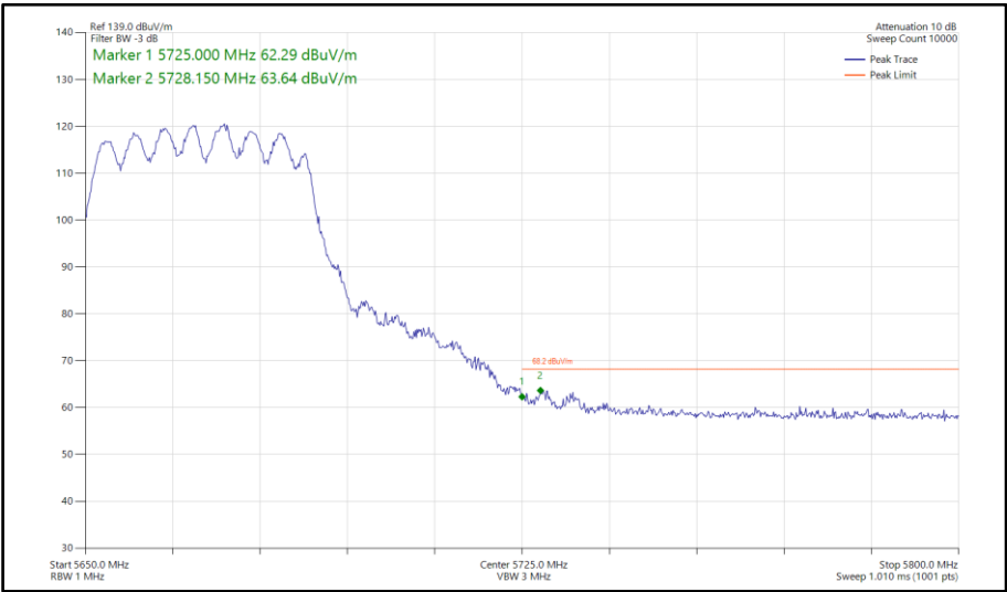
Figure 872 - 802.11n HT40, CDD, Core 0-1 - 5670 MHz Band Edge Frequency 5725 MHz
