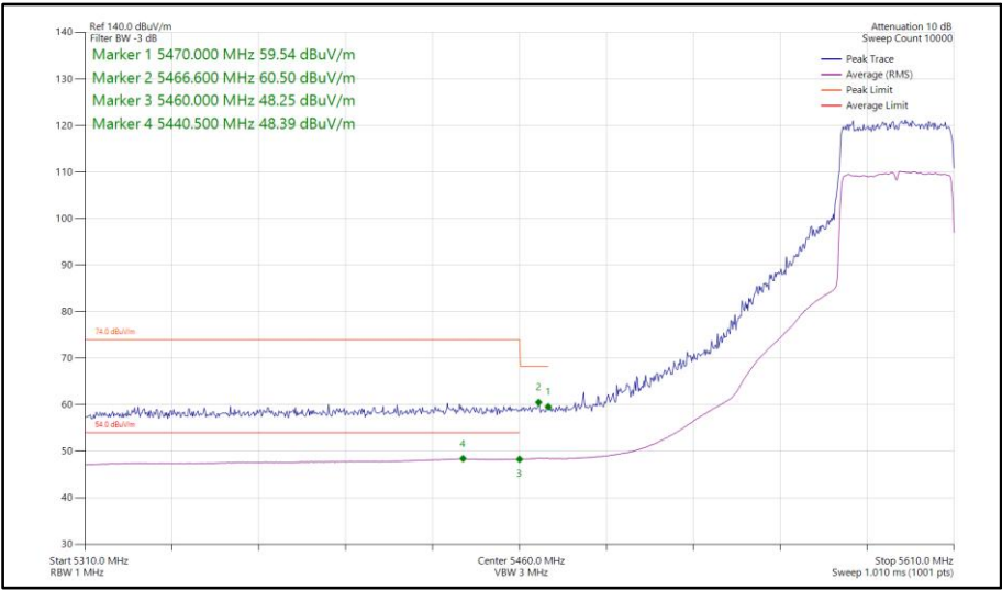
Figure 896 - 802.11ax HE40, SU, SDM, Core 0-1 - 5590 MHz Band Edge Frequency 5470 MHz
