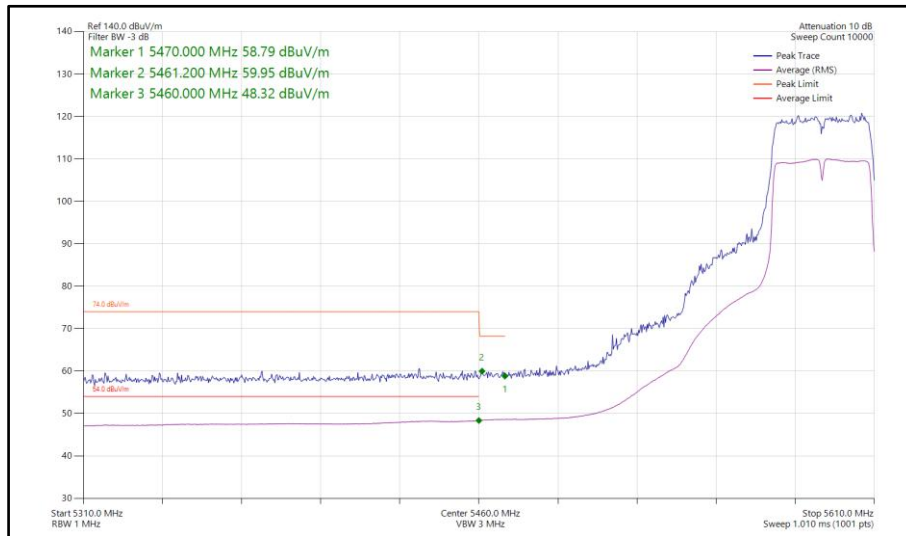
Figure 891 - 802.11n HT40, SDM, Core 0-1 - 5590 MHz Band Edge Frequency 5470 MHz
