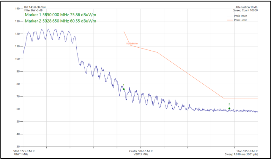
Figure 885 - 802.11ax HE40, SU, CDD, Core 0-1 - 5795 MHz Band Edge Frequency 5850 MHz
