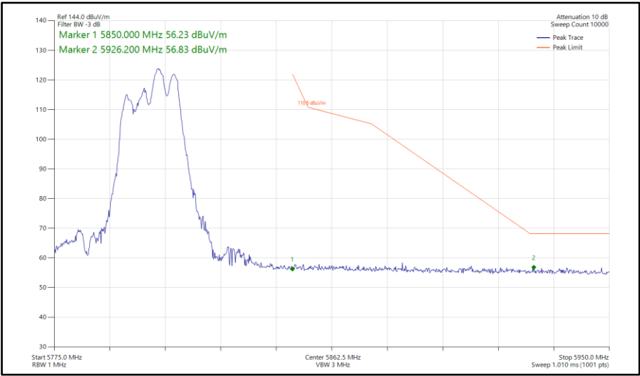
Figure 918 - 802.11ax HE40, RU106-56, SDM, Core 0-1 - 5795 MHz Band Edge Frequency 5850 MHz
