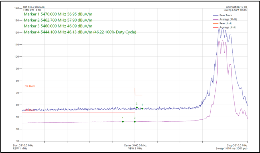
Figure 900 - 802.11be EHT40, RU106+26-82, SDM, Core 0-1 - 5590 MHz Band Edge Frequency 5470 MHz
