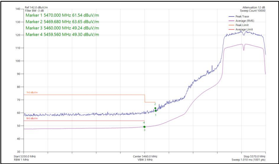
Figure 922 - 802.11ac VHT40, TxBF, Core 0-1 - 5550 MHz Band Edge Frequency 5470 MHz
