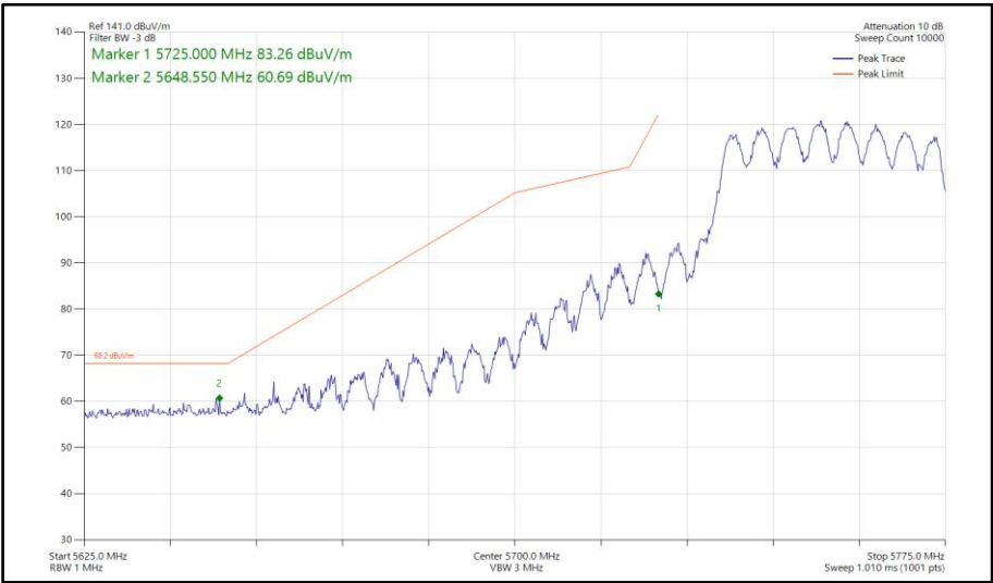
Figure 866 - 802.11ax HE40, SU, CDD, Core 0-1 - 5755 MHz Band Edge Frequency 5725 MHz
