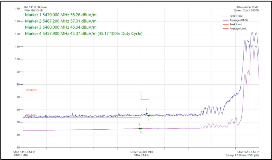
Figure 863 - 802.11be EHT40, RU106+26-85, CDD, Core 0-1 - 5590 MHz Band Edge Frequency 5470 MHz
