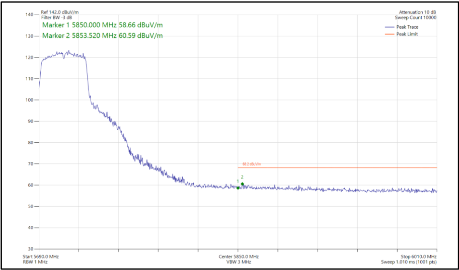
Figure 933 - 802.11ac VHT40, TxBF, Core 0-1 - 5710 MHz Band Edge Frequency 5850 MHz
