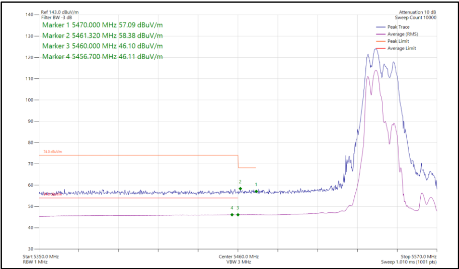
Figure 895 - 802.11ax HE40, RU106-53, SDM, Core 0-1 - 5550 MHz Band Edge Frequency 5470 MHz
