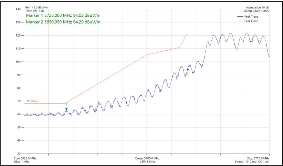
Figure 864 - 802.11a a40, CDD, Core 0-1 - 5755 MHz Band Edge Frequency 5725 MHz
