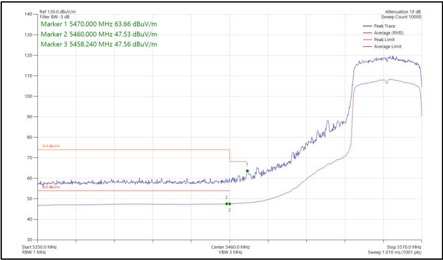
Figure 894 - 802.11ax HE40, SU, SDM, Core 0-1 - 5550 MHz Band Edge Frequency 5470 MHz
