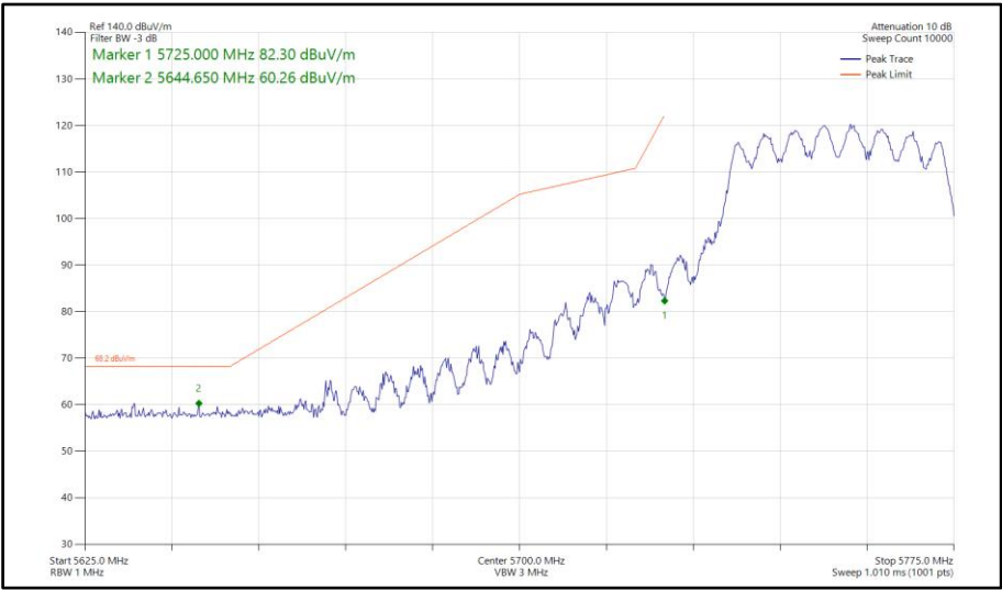
Figure 865 - 802.11n HT40, CDD, Core 0-1 - 5755 MHz Band Edge Frequency 5725 MHz
