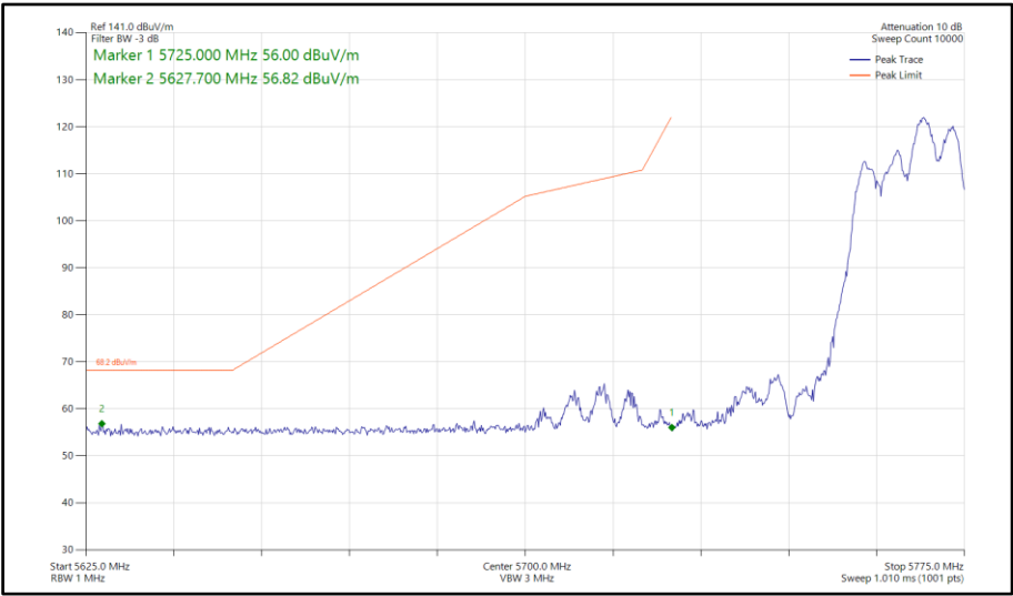
Figure 867 - 802.11ax HE40, RU106-56, CDD, Core 0-1 - 5755 MHz Band Edge Frequency 5725 MHz
