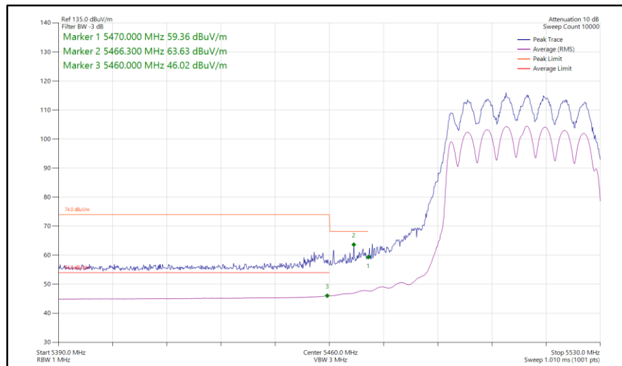
Figure 855 - 802.11ax HE40, SU, CDD, Core 0-1 - 5510 MHz Band Edge Frequency 5470 MHz
