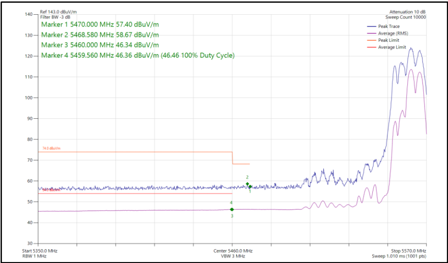
Figure 899 - 802.11be EHT40, RU106+26-85, SDM, Core 0-1 - 5550 MHz Band Edge Frequency 5470 MHz
