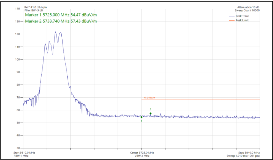
Figure 874 - 802.11ax HE40, RU106-56, CDD, Core 0-1 - 5630 MHz Band Edge Frequency 5725 MHz
