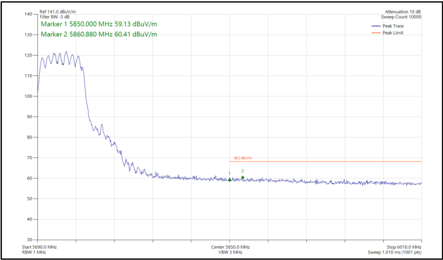
Figure 881 - 802.11n HT40, CDD, Core 0-1 - 5710 MHz Band Edge Frequency 5850 MHz
