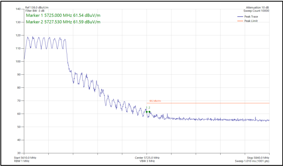
Figure 873 - 802.11ax HE40, SU, CDD, Core 0-1 - 5630 MHz Band Edge Frequency 5725 MHz
