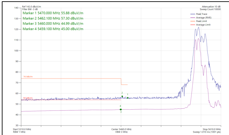
Figure 860 - 802.11ax HE40, RU106-53, CDD, Core 0-1 - 5590 MHz Band Edge Frequency 5470 MHz
