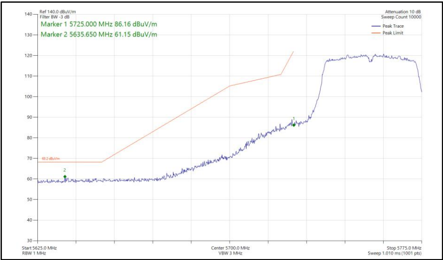
Figure 901 - 802.11n HT40, SDM, Core 0-1 - 5755 MHz Band Edge Frequency 5725 MHz
