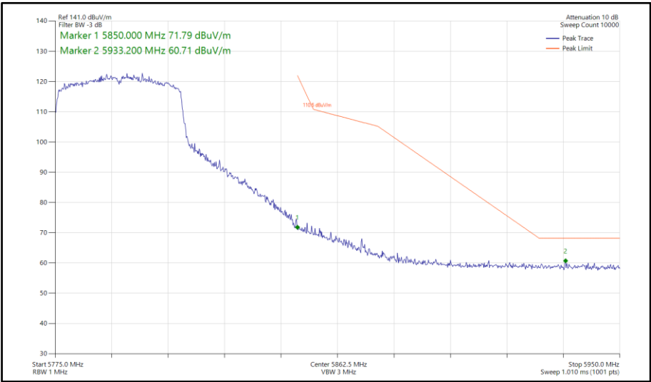
Figure 917 - 802.11ax HE40, SU, SDM, Core 0-1 - 5795 MHz Band Edge Frequency 5850 MHz
