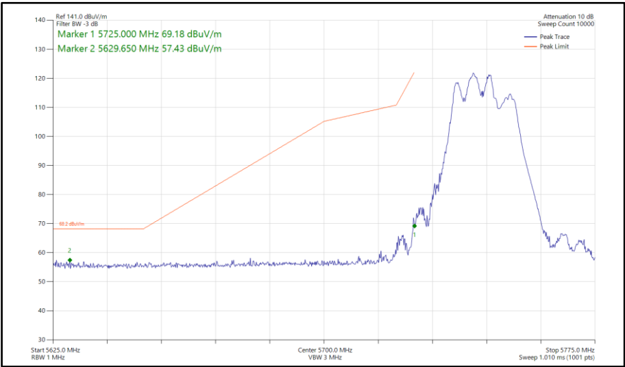
Figure 868 - 802.11be EHT40, RU106+26-82, CDD, Core 0-1 - 5755 MHz Band Edge Frequency 5725 MHz
