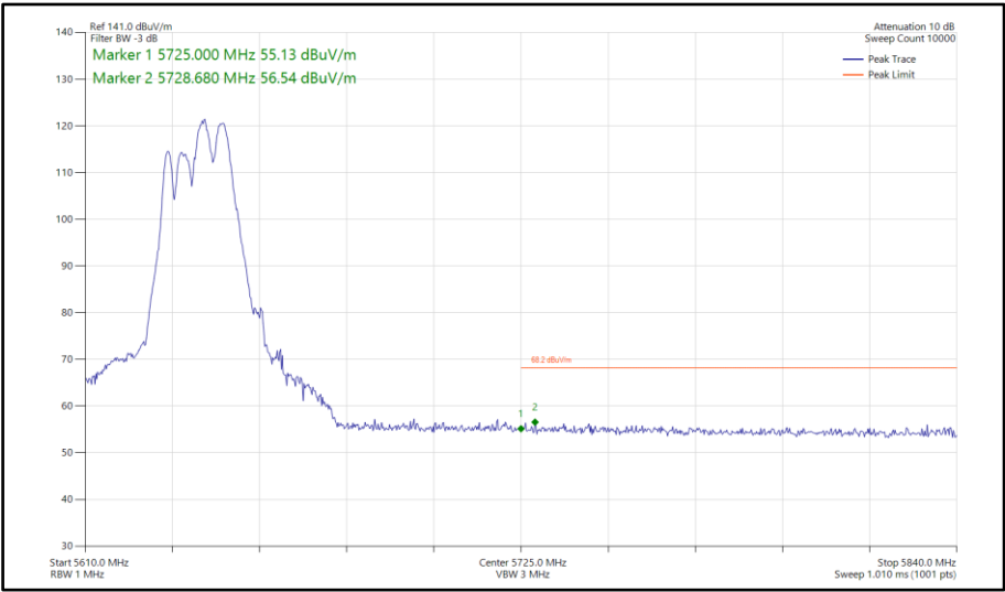
Figure 877 - 802.11be EHT40, RU106+26-85, CDD, Core 0-1 - 5630 MHz Band Edge Frequency 5725 MHz
