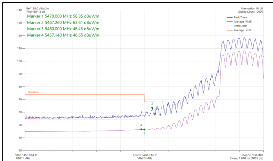
Figure 857 - 802.11ax HE40, SU, CDD, Core 0-1 - 5550 MHz Band Edge Frequency 5470 MHz
