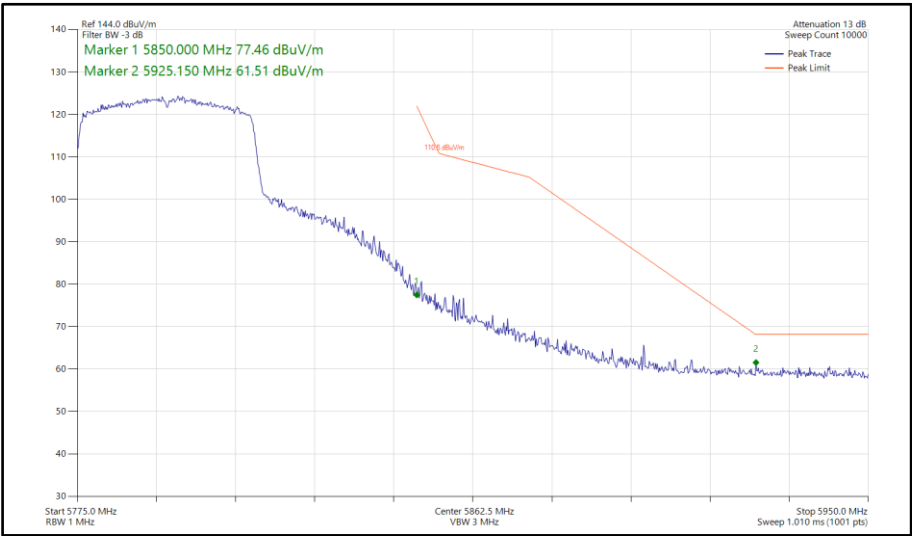
Figure 936 - 802.11ax HE40, SU, TxBF, Core 0-1 - 5795 MHz Band Edge Frequency 5850 MHz
