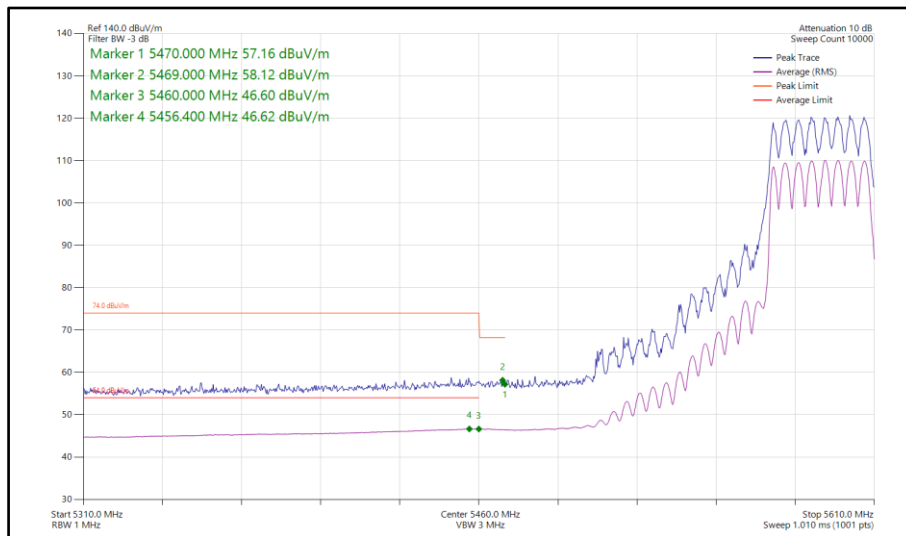
Figure 859 - 802.11ax HE40, SU, CDD, Core 0-1 - 5590 MHz Band Edge Frequency 5470 MHz
