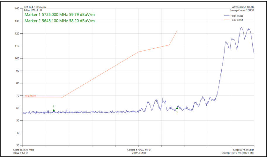
Figure 903 - 802.11ax HE40, RU106-56, SDM, Core 0-1 - 5755 MHz Band Edge Frequency 5725 MHz
