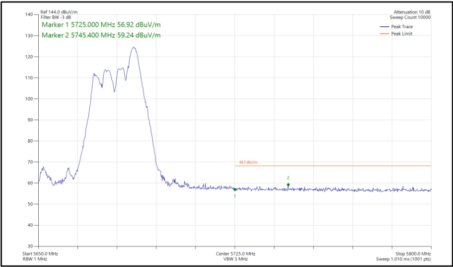
Figure 910 - 802.11ax HE40, RU52-44, SDM, Core 0-1 - 5670 MHz Band Edge Frequency 5725 MHz
