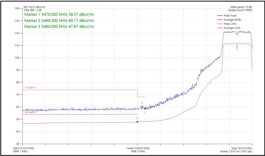
Figure 923 - 802.11ac VHT40, TxBF, Core 0-1 - 5590 MHz Band Edge Frequency 5470 MHz
