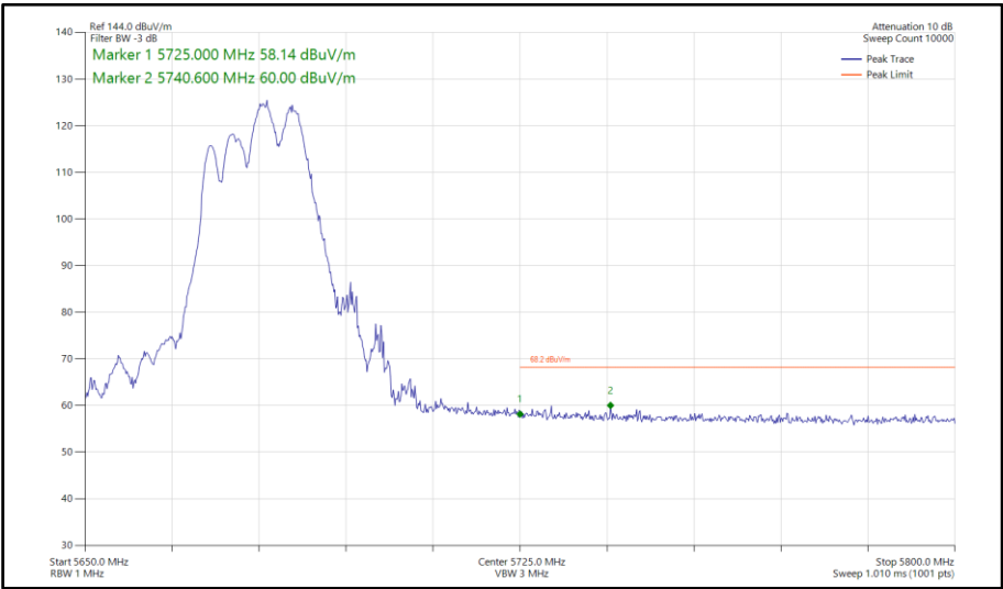
Figure 878 - 802.11be EHT40, RU106+26-85, CDD, Core 0-1 - 5670 MHz Band Edge Frequency 5725 MHz
