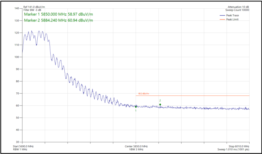
Figure 879 - 802.11a a40, CDD, Core 0-1 - 5710 MHz Band Edge Frequency 5850 MHz
