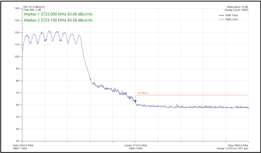
Figure 875 - 802.11ax HE40, SU, CDD, Core 0-1 - 5670 MHz Band Edge Frequency 5725 MHz
