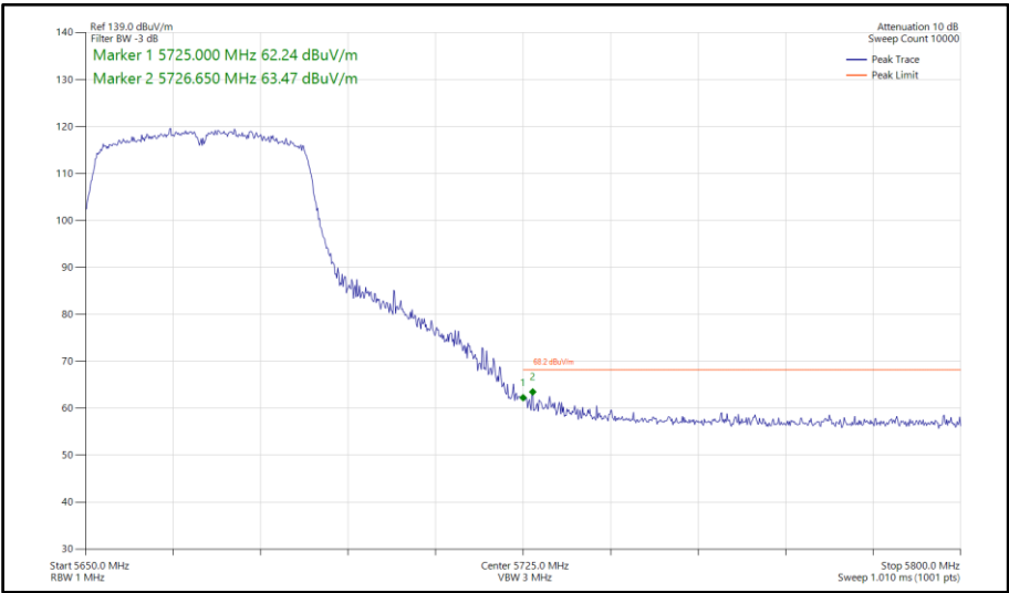
Figure 930 - 802.11ac VHT40, TxBF, Core 0-1 - 5670 MHz Band Edge Frequency 5725 MHz
