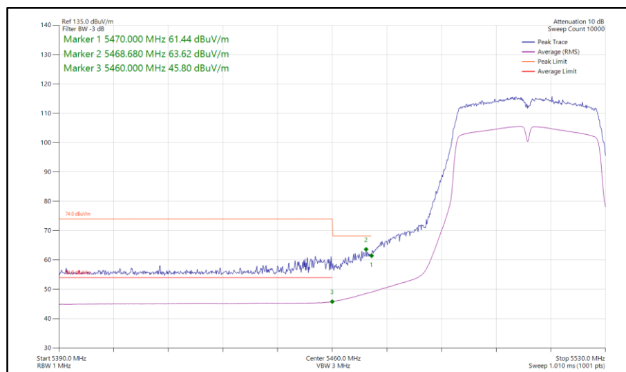
Figure 921 - 802.11ac VHT40, TxBF, Core 0-1 - 5510 MHz Band Edge Frequency 5470 MHz
