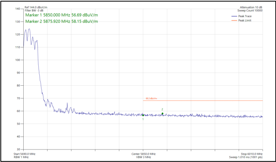
Figure 916 - 802.11ax HE40, RU106-53, SDM, Core 0-1 - 5710 MHz Band Edge Frequency 5850 MHz
