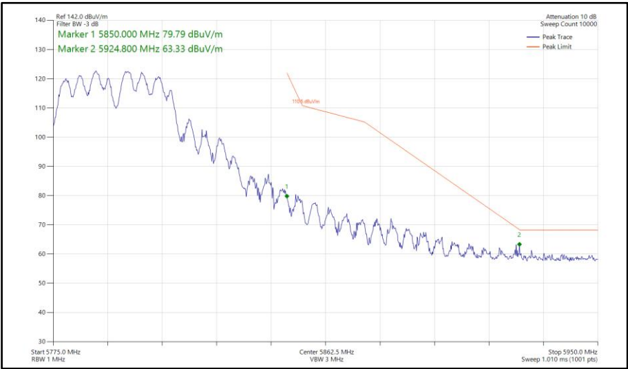
Figure 880 - 802.11a a40, CDD, Core 0-1 - 5795 MHz Band Edge Frequency 5850 MHz
