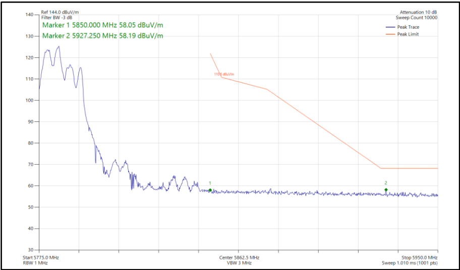
Figure 886 - 802.11ax HE40, RU106-53, CDD, Core 0-1 - 5795 MHz Band Edge Frequency 5850 MHz
