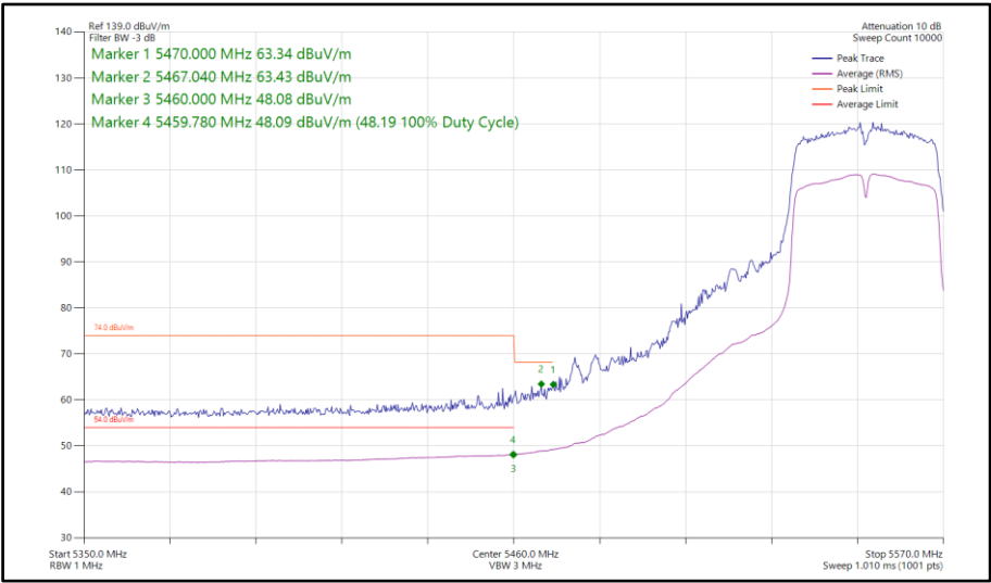
Figure 890 - 802.11n HT40, SDM, Core 0-1 - 5550 MHz Band Edge Frequency 5470 MHz
