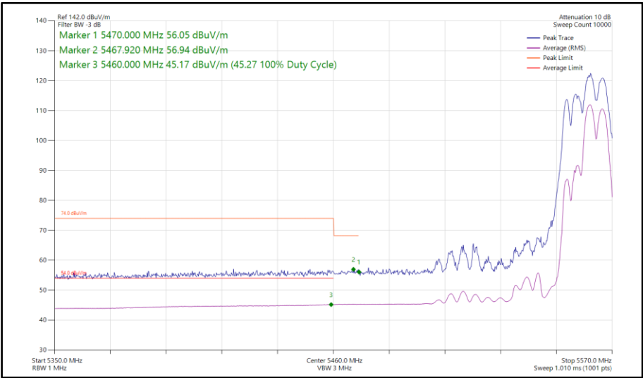
Figure 862 - 802.11be EHT40, RU106+26-85, CDD, Core 0-1 - 5550 MHz Band Edge Frequency 5470 MHz
