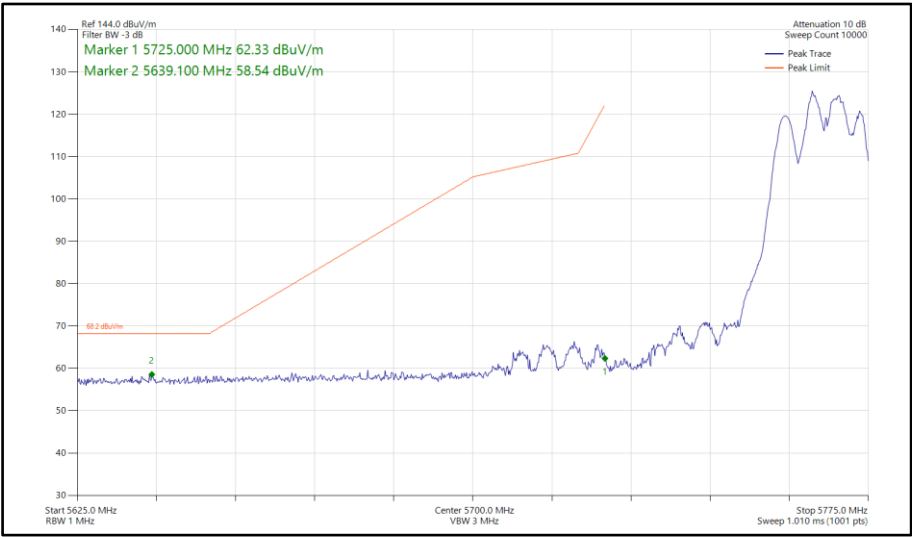
Figure 904 - 802.11be EHT40, RU106+26-85, SDM, Core 0-1 - 5755 MHz Band Edge Frequency 5725 MHz
