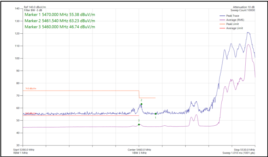
Figure 893 - 802.11ax HE40, RU52-44, SDM, Core 0-1 - 5510 MHz Band Edge Frequency 5470 MHz
