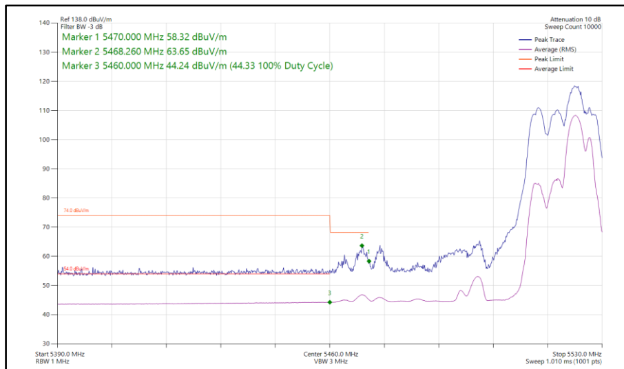
Figure 861 - 802.11be EHT40, RU52+26-75, CDD, Core 0-1 - 5510 MHz Band Edge Frequency 5470 MHz
