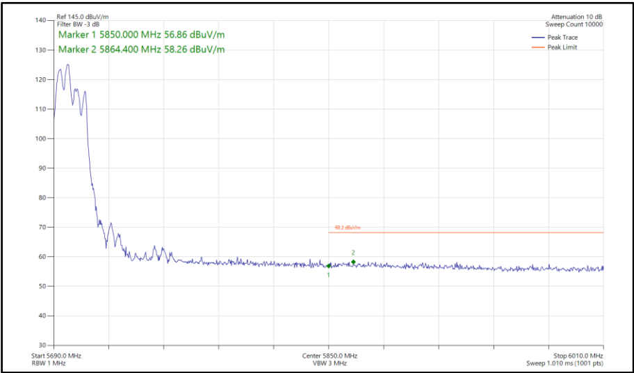
Figure 884 - 802.11ax HE40, RU106-53, CDD, Core 0-1 - 5710 MHz Band Edge Frequency 5850 MHz
