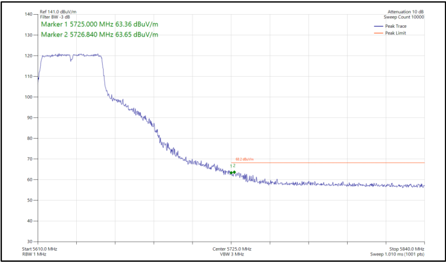
Figure 929 - 802.11ac VHT40, TxBF, Core 0-1 - 5630 MHz Band Edge Frequency 5725 MHz
