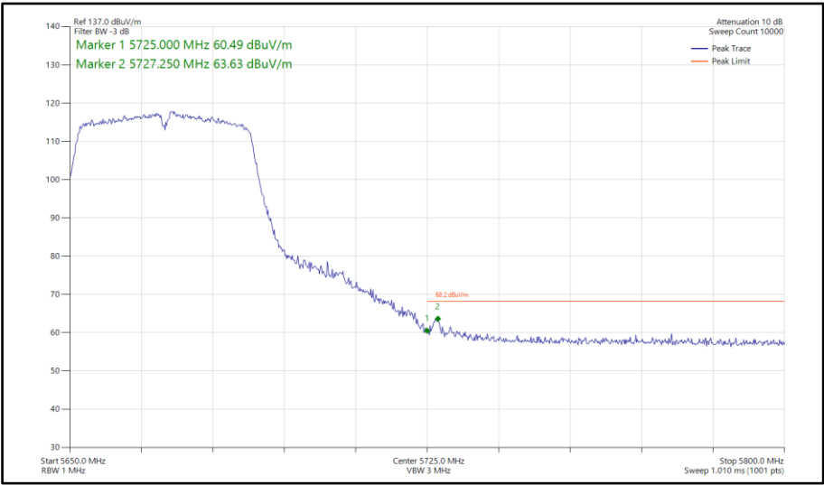
Figure 906 - 802.11n HT40, SDM, Core 0-1 - 5670 MHz Band Edge Frequency 5725 MHz
