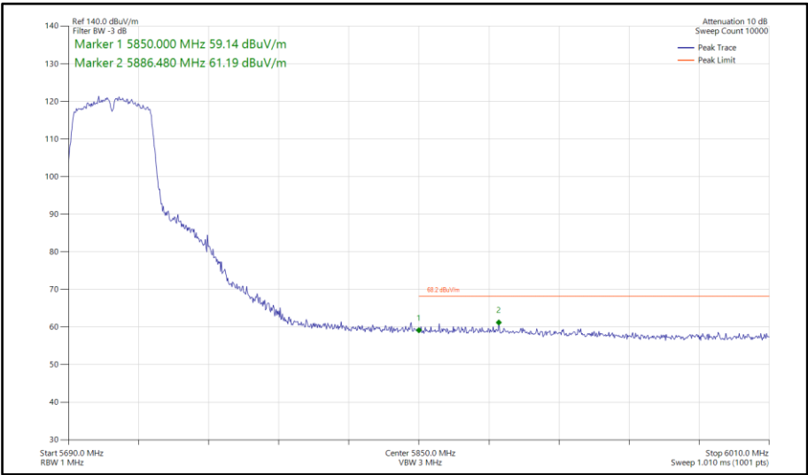
Figure 913 - 802.11n HT40, SDM, Core 0-1 - 5710 MHz Band Edge Frequency 5850 MHz
