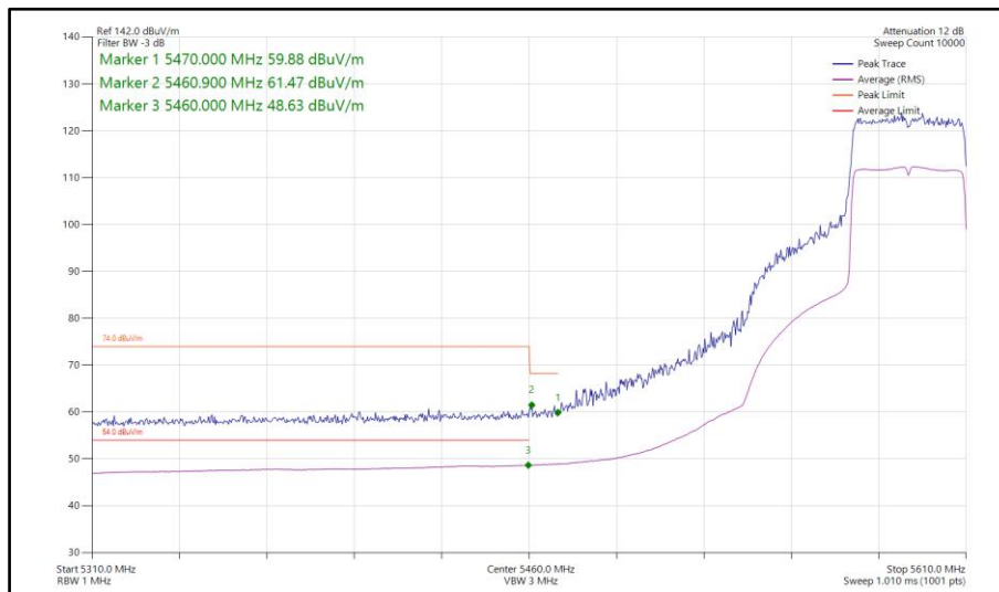
Figure 926 - 802.11ax HE40, SU, TxBF, Core 0-1 - 5590 MHz Band Edge Frequency 5470 MHz
