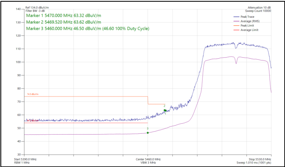
Figure 889 - 802.11n HT40, SDM, Core 0-1 - 5510 MHz Band Edge Frequency 5470 MHz
