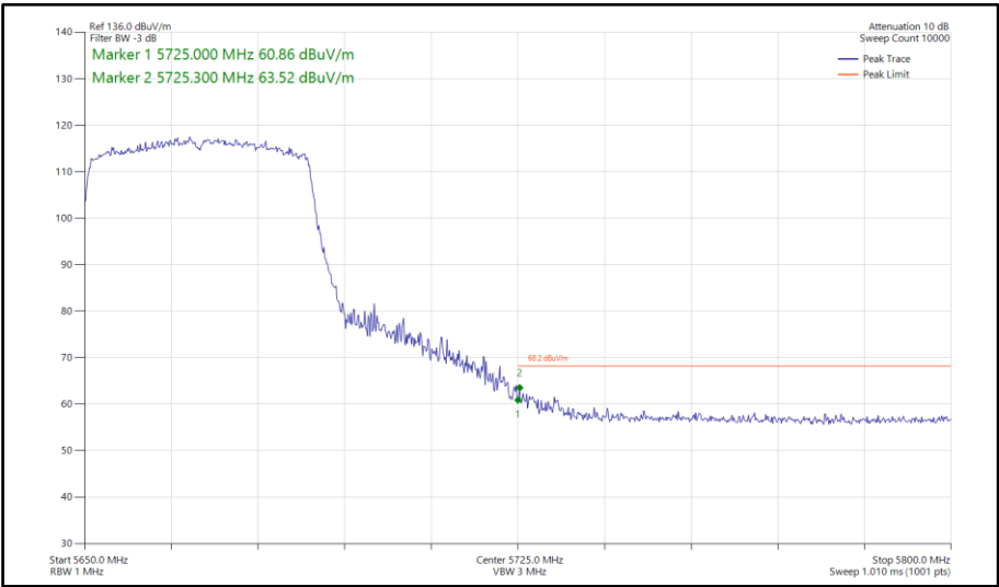
Figure 909 - 802.11ax HE40, SU, SDM, Core 0-1 - 5670 MHz Band Edge Frequency 5725 MHz
