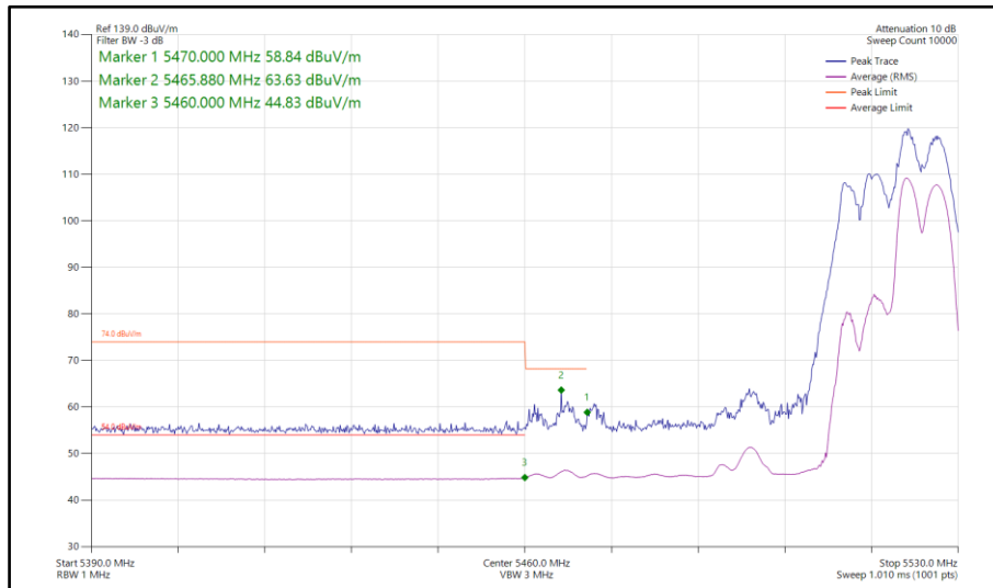
Figure 856 - 802.11ax HE40, RU106-56, CDD, Core 0-1 - 5510 MHz Band Edge Frequency 5470 MHz
