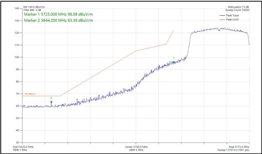
Figure 928 - 802.11ax HE40, SU, TxBF, Core 0-1 - 5755 MHz Band Edge Frequency 5725 MHz
