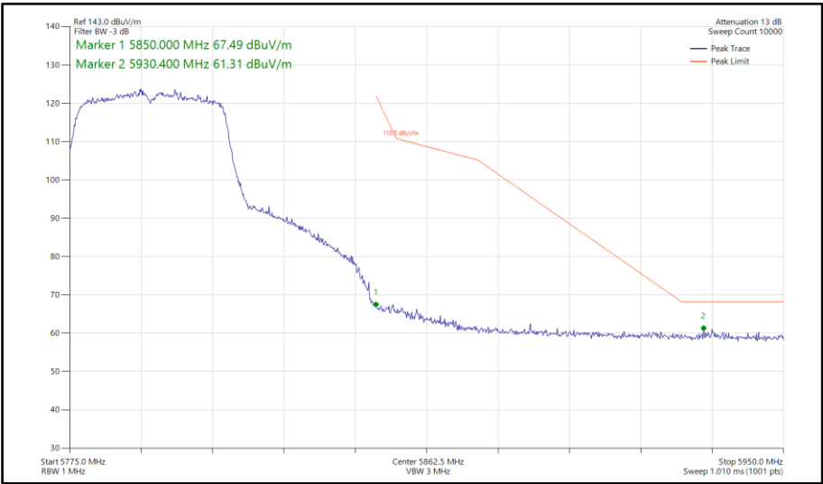
Figure 934 - 802.11ac VHT40, TxBF, Core 0-1 - 5795 MHz Band Edge Frequency 5850 MHz
