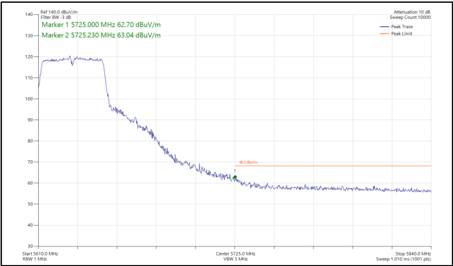
Figure 905 - 802.11n HT40, SDM, Core 0-1 - 5630 MHz Band Edge Frequency 5725 MHz
