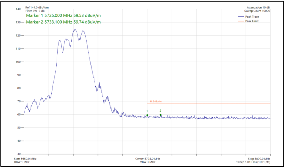
Figure 912 - 802.11be EHT40, RU106+26-85, SDM, Core 0-1 - 5670 MHz Band Edge Frequency 5725 MHz
