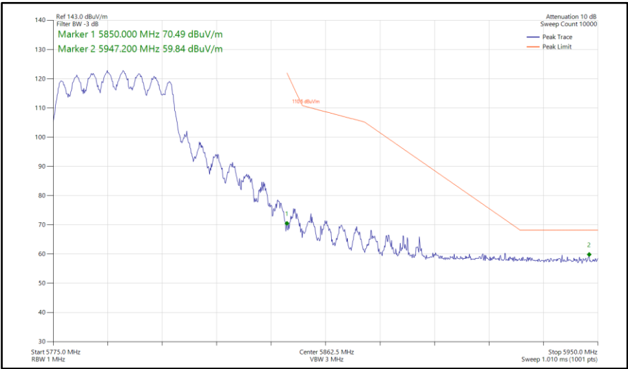
Figure 882 - 802.11n HT40, CDD, Core 0-1 - 5795 MHz Band Edge Frequency 5850 MHz
