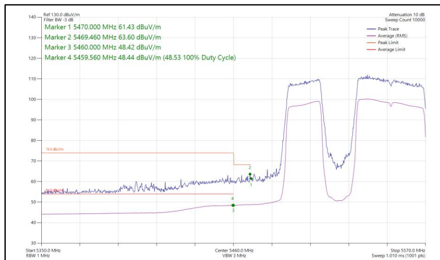
Figure 964 - 802.11be EHT80, RU484+242-91, SISO, Core 1 - 5530 MHz Band Edge Frequency 5470 MHz
