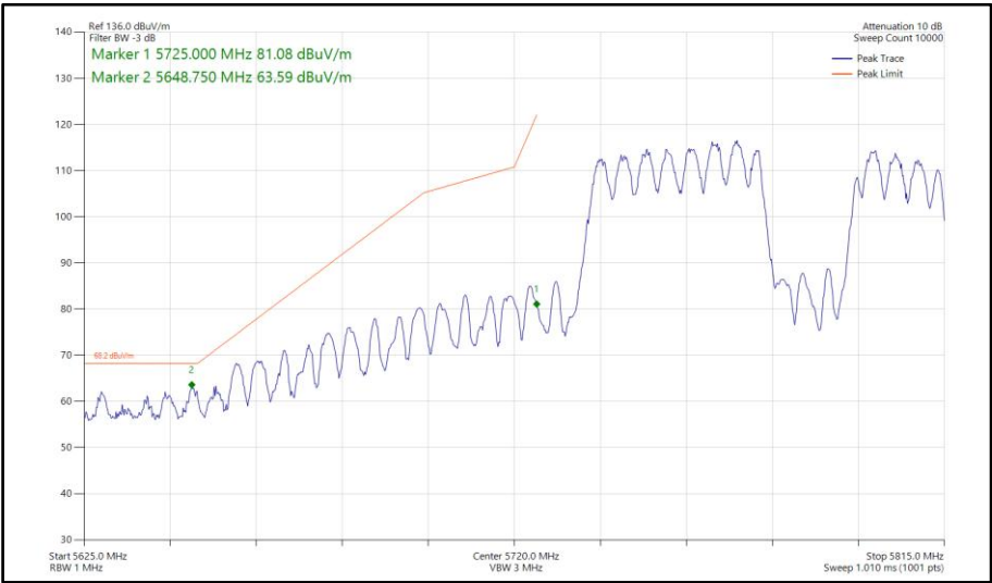
Figure 993 - 802.11be EHT80, RU484+242-92, CDD, Core 0-1 - 5775 MHz Band Edge Frequency 5725 MHz
