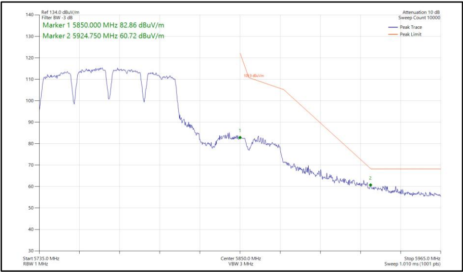
Figure 952 - 802.11a a80, SISO, Core 0 - 5775 MHz Band Edge Frequency 5850 MHz
