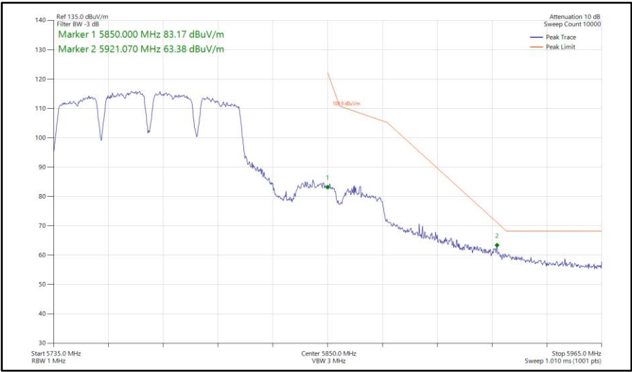
Figure 976 - 802.11a a80, SISO, Core 1 - 5775 MHz Band Edge Frequency 5850 MHz
