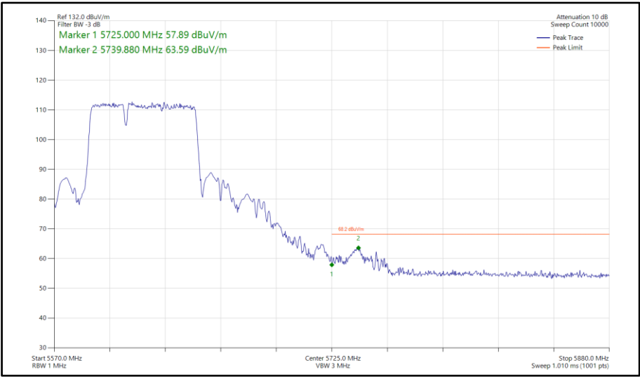
Figure 974 - 802.11be EHT80, RU484+242-90, SISO, Core 1 - 5610 MHz Band Edge Frequency 5725 MHz
