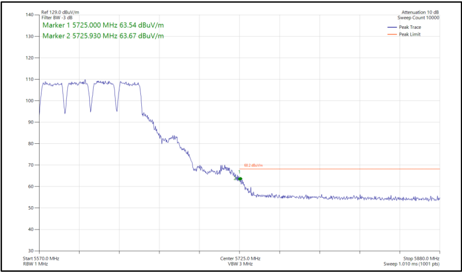
Figure 970 - 802.11a a80, SISO, Core 1 - 5610 MHz Band Edge Frequency 5725 MHz
