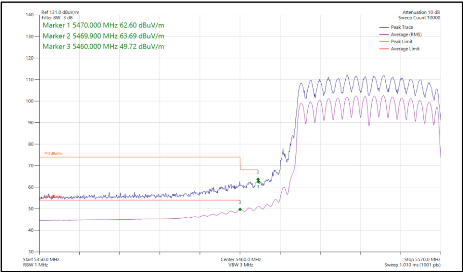
Figure 985 - 802.11ac VHT80, CDD, Core 0-1 - 5530 MHz Band Edge Frequency 5470 MHz
