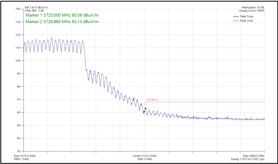
Figure 996 - 802.11ax HE80, SU, CDD, Core 0-1 - 5610 MHz Band Edge Frequency 5725 MHz
