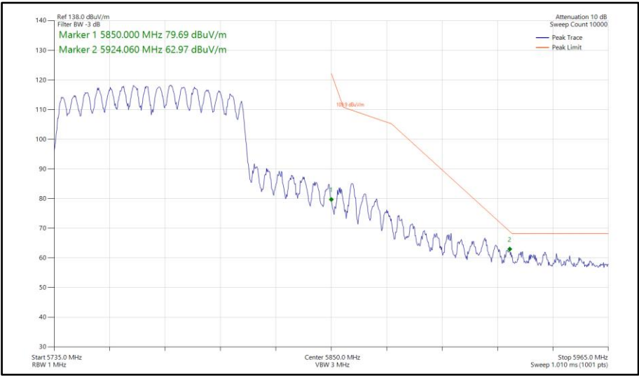
Figure 1002 - 802.11ac VHT80, CDD, Core 0-1 - 5775 MHz Band Edge Frequency 5850 MHz
