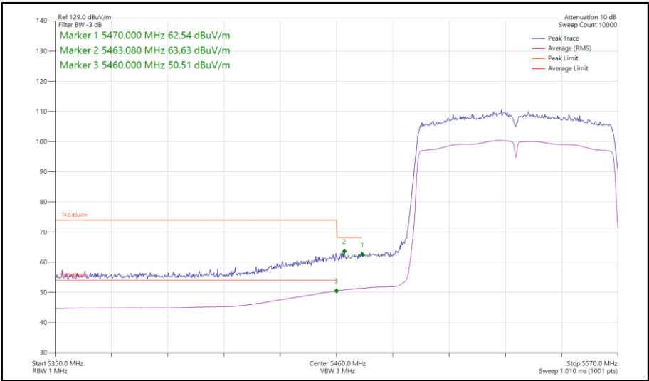
Figure 961 - 802.11ac VHT80, SISO, Core 1 - 5530 MHz Band Edge Frequency 5470 MHz
