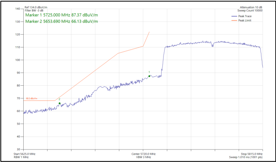
Figure 966 - 802.11ac VHT80, SISO, Core 1 - 5775 MHz Band Edge Frequency 5725 MHz
