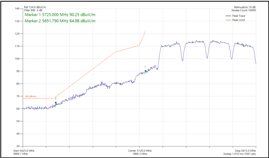
Figure 941 - 802.11a a80, SISO, Core 0 - 5775 MHz Band Edge Frequency 5725 MHz
