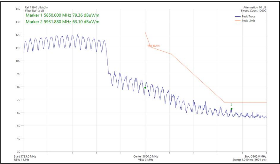
Figure 1005 - 802.11ax HE80, SU, CDD, Core 0-1 - 5775 MHz Band Edge Frequency 5850 MHz
