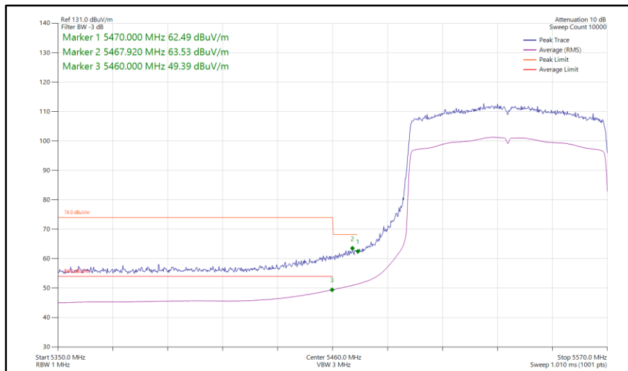
Figure 938 - 802.11ax HE80, SU, SISO, Core 0 - 5530 MHz Band Edge Frequency 5470 MHz
