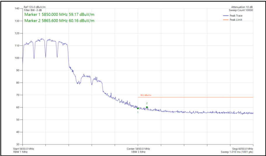
Figure 975 - 802.11a a80, SISO, Core 1 - 5690 MHz Band Edge Frequency 5850 MHz
