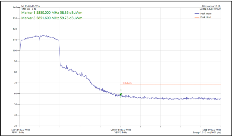
Figure 953 - 802.11ac VHT80, SISO, Core 0 - 5690 MHz Band Edge Frequency 5850 MHz
