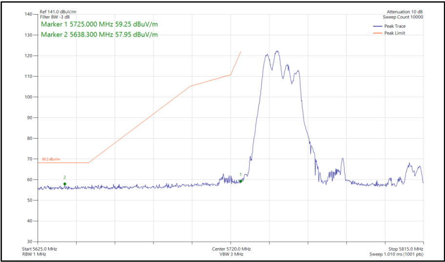
Figure 992 - 802.11ax HE80, RU106-53, CDD, Core 0-1 - 5775 MHz Band Edge Frequency 5725 MHz
