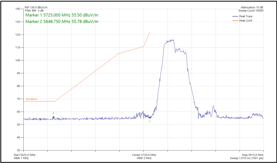
Figure 944 - 802.11ax HE80, RU106-53, SISO, Core 0 - 5775 MHz Band Edge Frequency 5725 MHz
