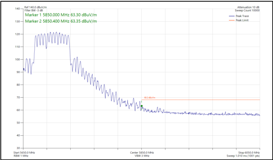
Figure 1007 - 802.11be EHT80, RU484+242-90, CDD, Core 0-1 - 5690 MHz Band Edge Frequency 5850 MHz
