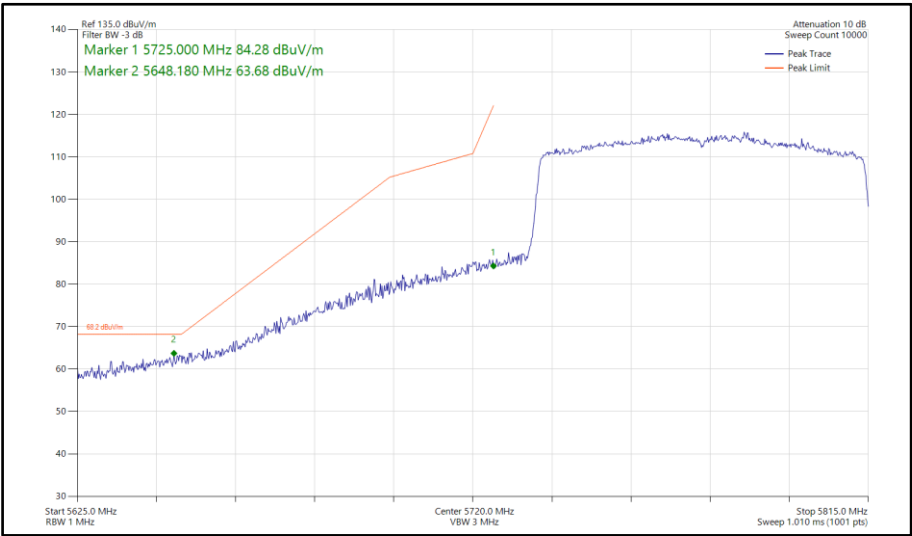
Figure 967 - 802.11ax HE80, SU, SISO, Core 1 - 5775 MHz Band Edge Frequency 5725 MHz
