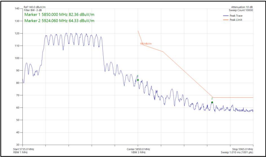
Figure 1008 - 802.11be EHT80, RU484+242-90, CDD, Core 0-1 - 5775 MHz Band Edge Frequency 5850 MHz
