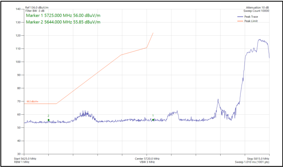
Figure 968 - 802.11ax HE80, RU106-60, SISO, Core 1 - 5775 MHz Band Edge Frequency 5725 MHz
