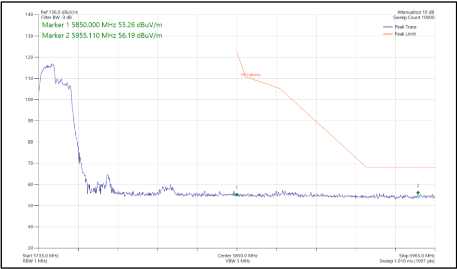
Figure 958 - 802.11ax HE80, RU106-53, SISO, Core 0 - 5775 MHz Band Edge Frequency 5850 MHz
