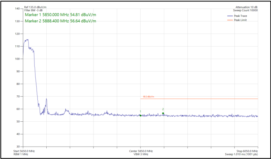
Figure 956 - 802.11ax HE80, RU106-53, SISO, Core 0 - 5690 MHz Band Edge Frequency 5850 MHz
