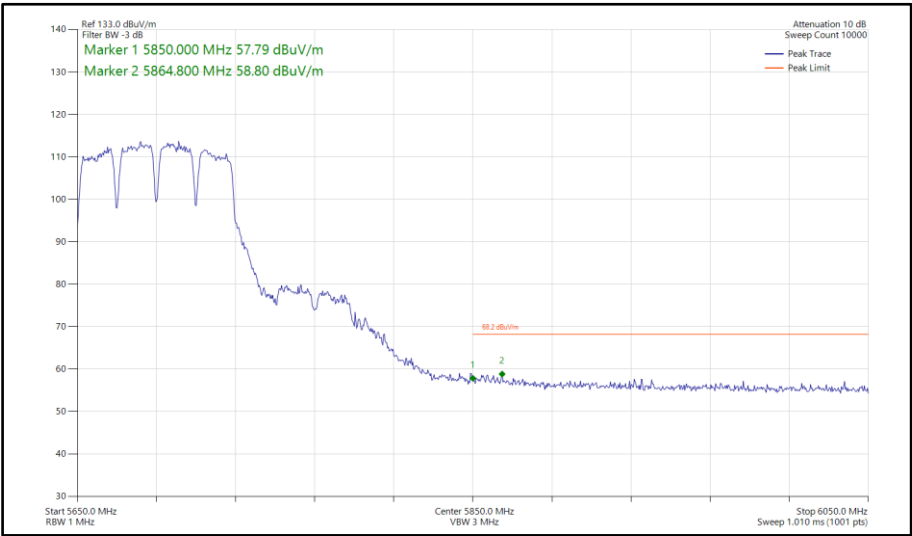
Figure 951 - 802.11a a80, SISO, Core 0 - 5690 MHz Band Edge Frequency 5850 MHz
