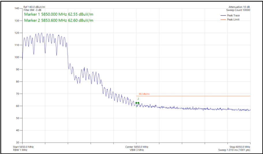
Figure 999 - 802.11a a80, CDD, Core 0-1 - 5690 MHz Band Edge Frequency 5850 MHz
