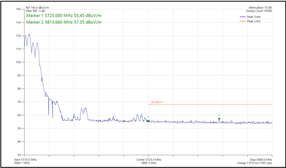
Figure 1019 - 802.11ax HE80, RU106-53, SDM, Core 0-1 - 5610 MHz Band Edge Frequency 5725 MHz
