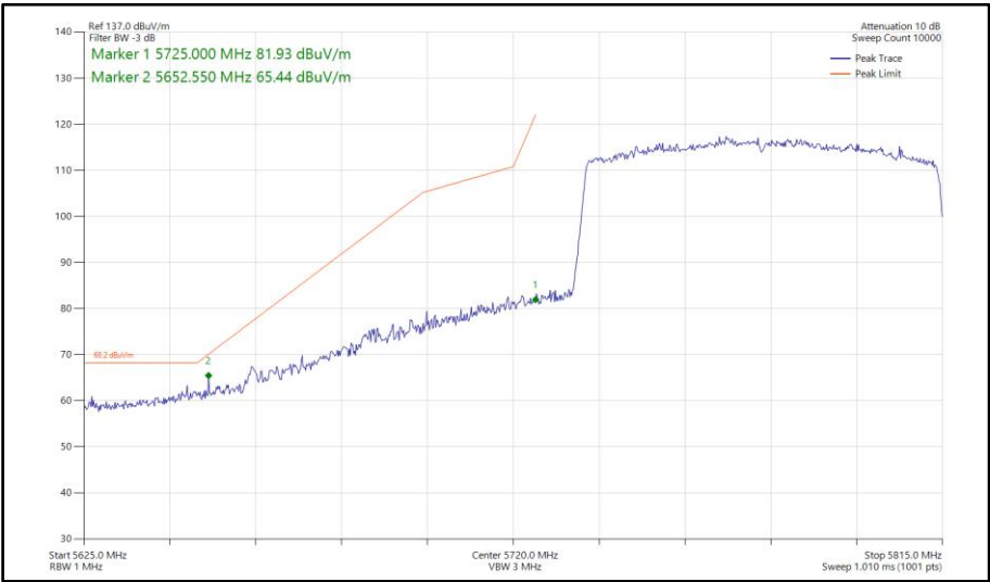
Figure 1014 - 802.11ax HE80, SU, SDM, Core 0-1 - 5775 MHz Band Edge Frequency 5725 MHz
