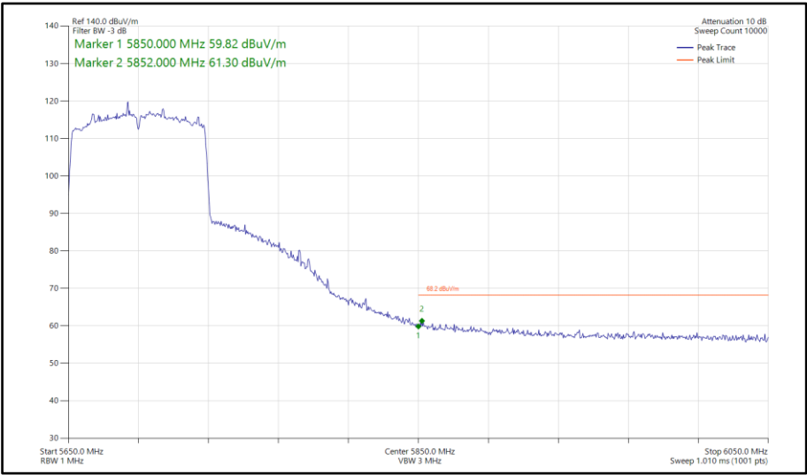
Figure 1021 - 802.11ac VHT80, SDM, Core 0-1 - 5690 MHz Band Edge Frequency 5850 MHz
