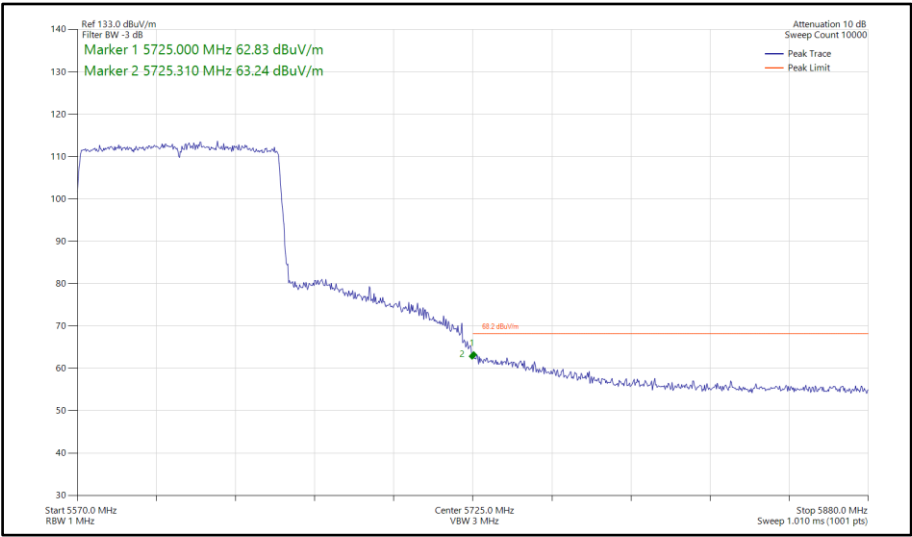
Figure 972 - 802.11ax HE80, SU, SISO, Core 1 - 5610 MHz Band Edge Frequency 5725 MHz
