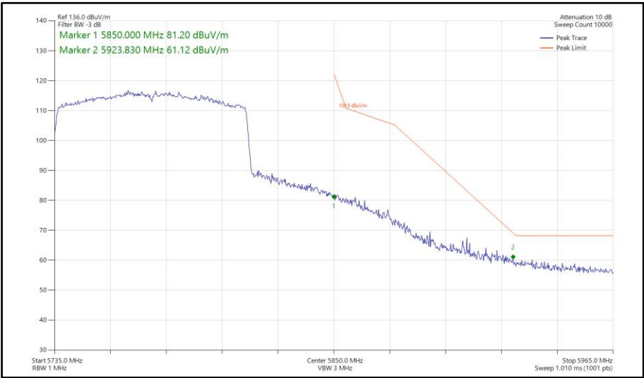
Figure 981 - 802.11ax HE80, SU, SISO, Core 1 - 5775 MHz Band Edge Frequency 5850 MHz
