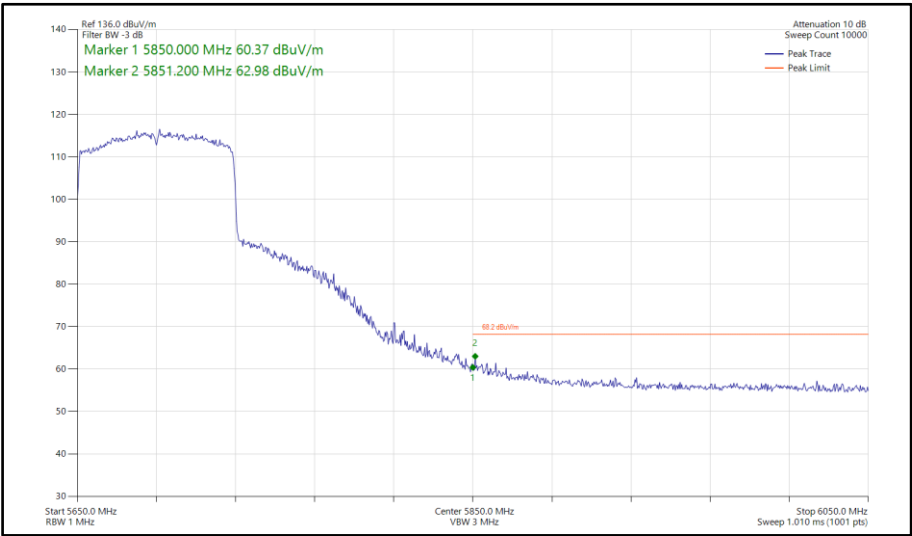
Figure 979 - 802.11ax HE80, SU, SISO, Core 1 - 5690 MHz Band Edge Frequency 5850 MHz
