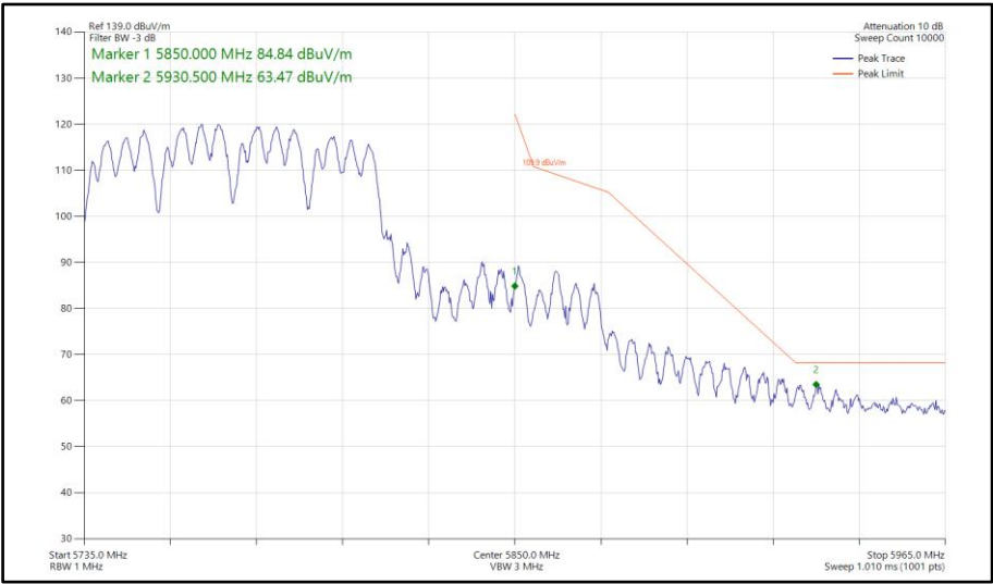
Figure 1000 - 802.11a a80, CDD, Core 0-1 - 5775 MHz Band Edge Frequency 5850 MHz
