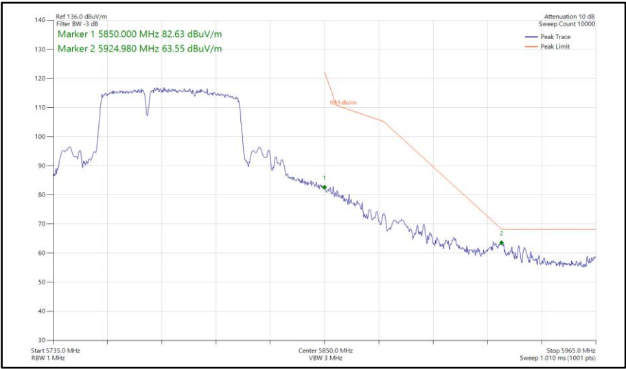
Figure 984 - 802.11be EHT80, RU484+242-90, SISO, Core 1 - 5775 MHz Band Edge Frequency 5850 MHz
