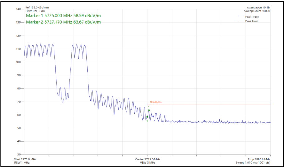
Figure 1020 - 802.11be EHT80, RU484+242-92, SDM, Core 0-1 - 5610 MHz Band Edge Frequency 5725 MHz
