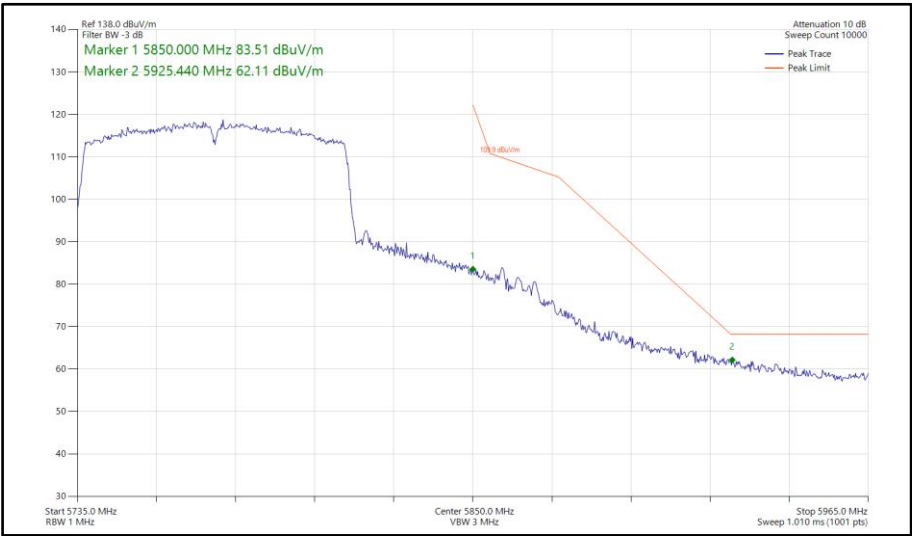
Figure 1022 - 802.11ac VHT80, SDM, Core 0-1 - 5775 MHz Band Edge Frequency 5850 MHz
