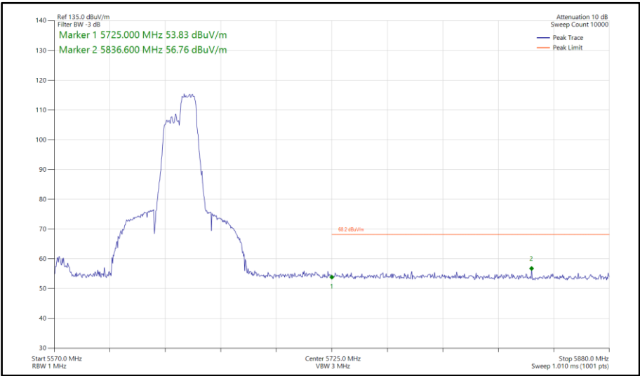
Figure 949 - 802.11ax HE80, RU106-60, SISO, Core 0 - 5610 MHz Band Edge Frequency 5725 MHz
