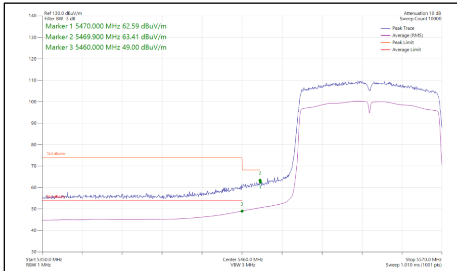
Figure 937 - 802.11ac VHT80, SISO, Core 0 - 5530 MHz Band Edge Frequency 5470 MHz
