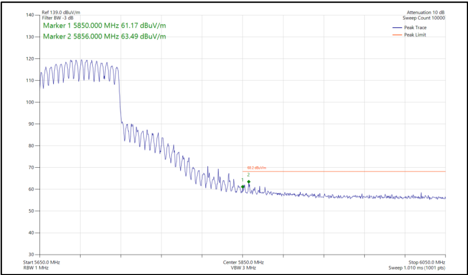
Figure 1003 - 802.11ax HE80, SU, CDD, Core 0-1 - 5690 MHz Band Edge Frequency 5850 MHz
