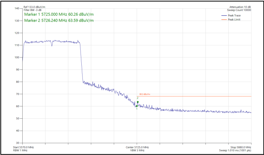
Figure 1017 - 802.11ac VHT80, SDM, Core 0-1 - 5610 MHz Band Edge Frequency 5725 MHz
