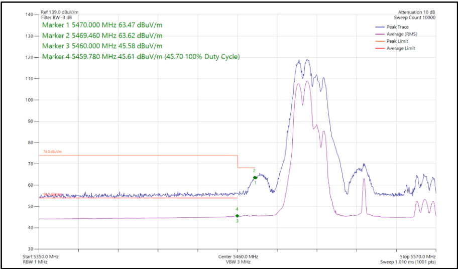
Figure 1012 - 802.11be EHT80, RU106+26-82, SDM, Core 0-1 - 5530 MHz Band Edge Frequency 5470 MHz
