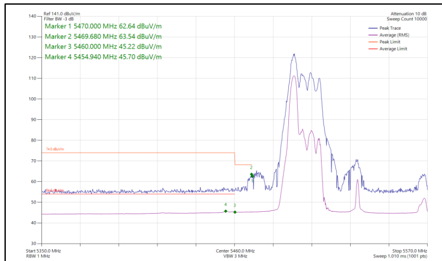
Figure 987 - 802.11ax HE80, RU52-37, CDD, Core 0-1 - 5530 MHz Band Edge Frequency 5470 MHz
