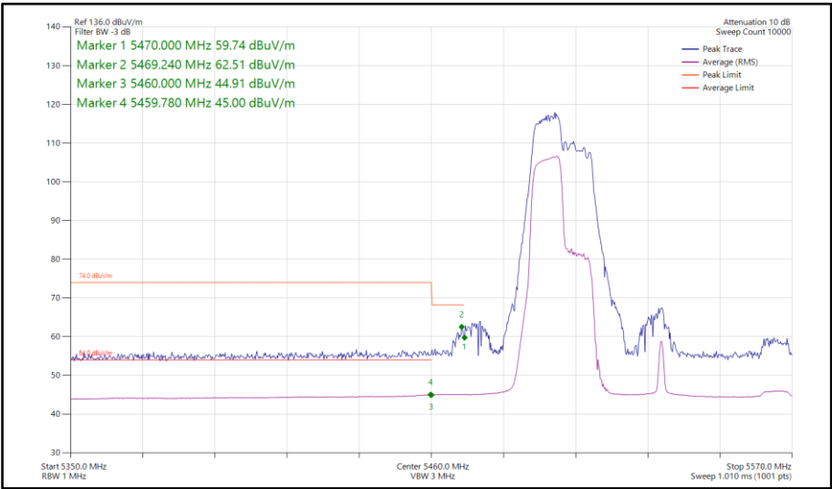
Figure 939 - 802.11ax HE80, RU106-53, SISO, Core 0 - 5530 MHz Band Edge Frequency 5470 MHz
