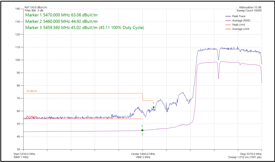
Figure 940 - 802.11be EHT80, RU484+242-90, SISO, Core 0 - 5530 MHz Band Edge Frequency 5470 MHz
