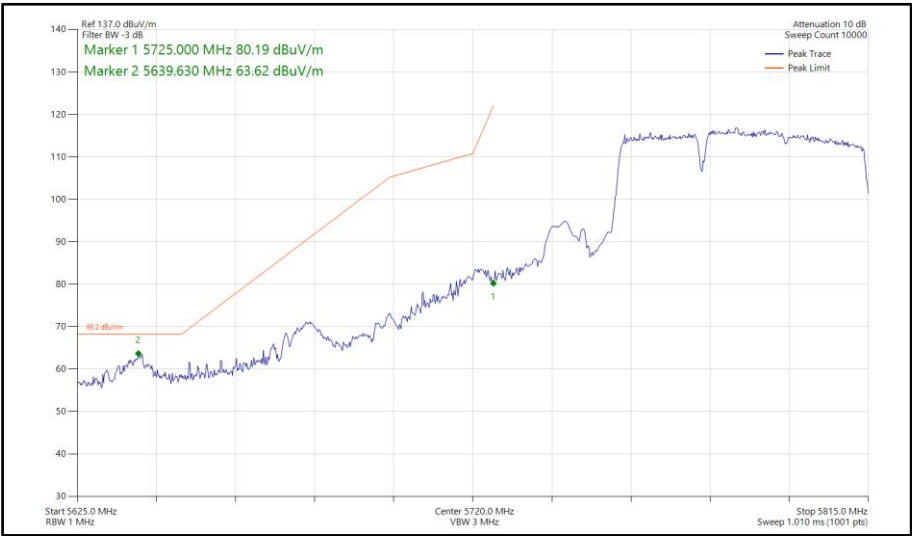
Figure 969 - 802.11be EHT80, RU484+242-90, SISO, Core 1 - 5775 MHz Band Edge Frequency 5725 MHz
