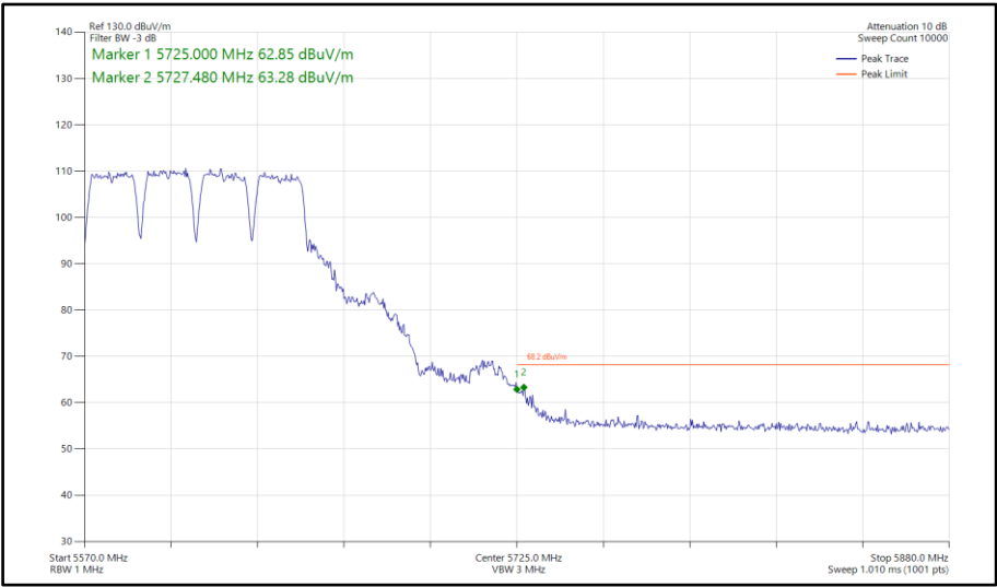
Figure 946 - 802.11a a80, SISO, Core 0 - 5610 MHz Band Edge Frequency 5725 MHz
