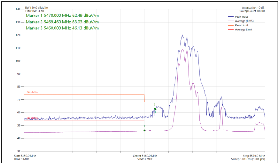
Figure 1011 - 802.11ax HE80, RU106-53, SDM, Core 0-1 - 5530 MHz Band Edge Frequency 5470 MHz
