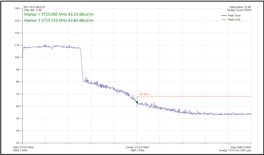
Figure 948 - 802.11ax HE80, SU, SISO, Core 0 - 5610 MHz Band Edge Frequency 5725 MHz
