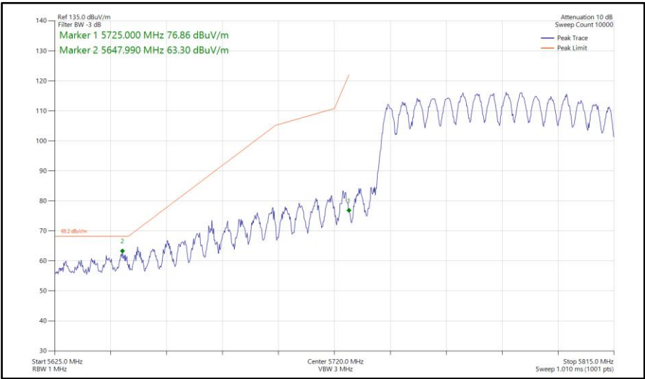
Figure 991 - 802.11ax HE80, SU, CDD, Core 0-1 - 5775 MHz Band Edge Frequency 5725 MHz
