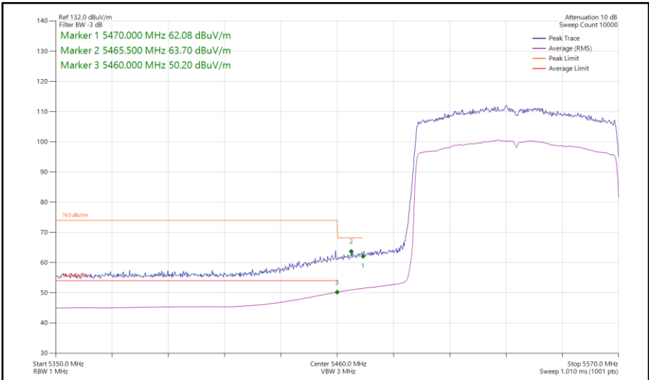
Figure 1010 - 802.11ax HE80, SU, SDM, Core 0-1 - 5530 MHz Band Edge Frequency 5470 MHz
