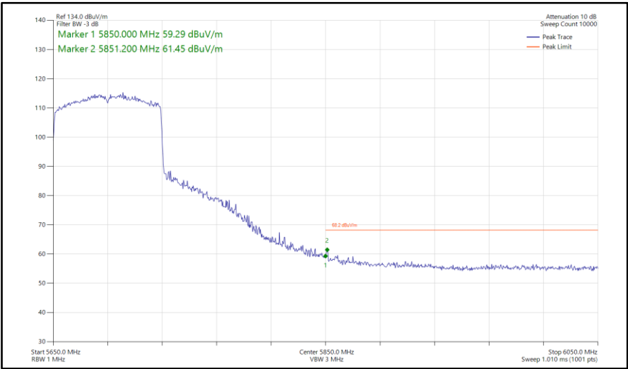
Figure 955 - 802.11ax HE80, SU, SISO, Core 0 - 5690 MHz Band Edge Frequency 5850 MHz
