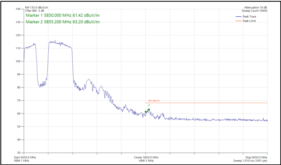
Figure 959 - 802.11be EHT80, RU484+242-91, SISO, Core 0 - 5690 MHz Band Edge Frequency 5850 MHz
