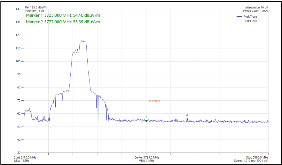
Figure 973 - 802.11ax HE80, RU106-60, SISO, Core 1 - 5610 MHz Band Edge Frequency 5725 MHz
