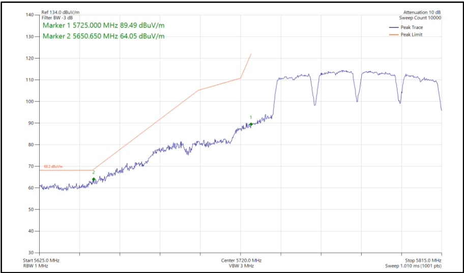
Figure 965 - 802.11a a80, SISO, Core 1 - 5775 MHz Band Edge Frequency 5725 MHz
