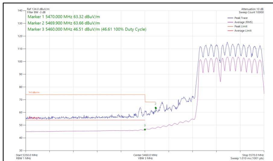
Figure 988 - 802.11be EHT80, RU484+242-90, CDD, Core 0-1 - 5530 MHz Band Edge Frequency 5470 MHz
