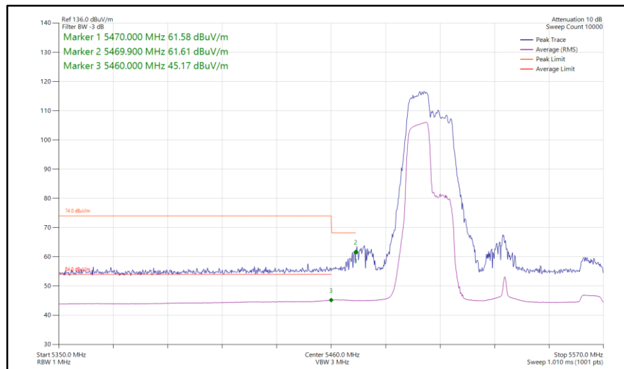
Figure 963 - 802.11ax HE80, RU106-53, SISO, Core 1 - 5530 MHz Band Edge Frequency 5470 MHz
