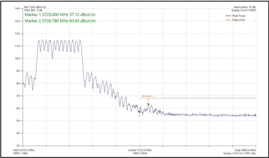
Figure 998 - 802.11be EHT80, RU484+242-90, CDD, Core 0-1 - 5610 MHz Band Edge Frequency 5725 MHz
