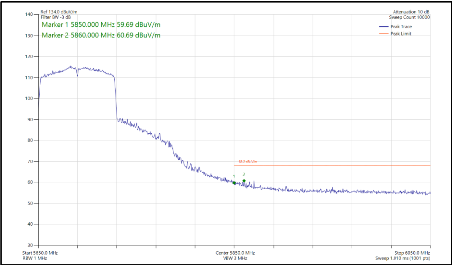
Figure 977 - 802.11ac VHT80, SISO, Core 1 - 5690 MHz Band Edge Frequency 5850 MHz
