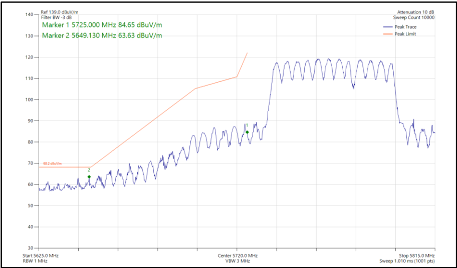
Figure 1016 - 802.11be EHT80, RU484+242-93, SDM, Core 0-1 - 5775 MHz Band Edge Frequency 5725 MHz
