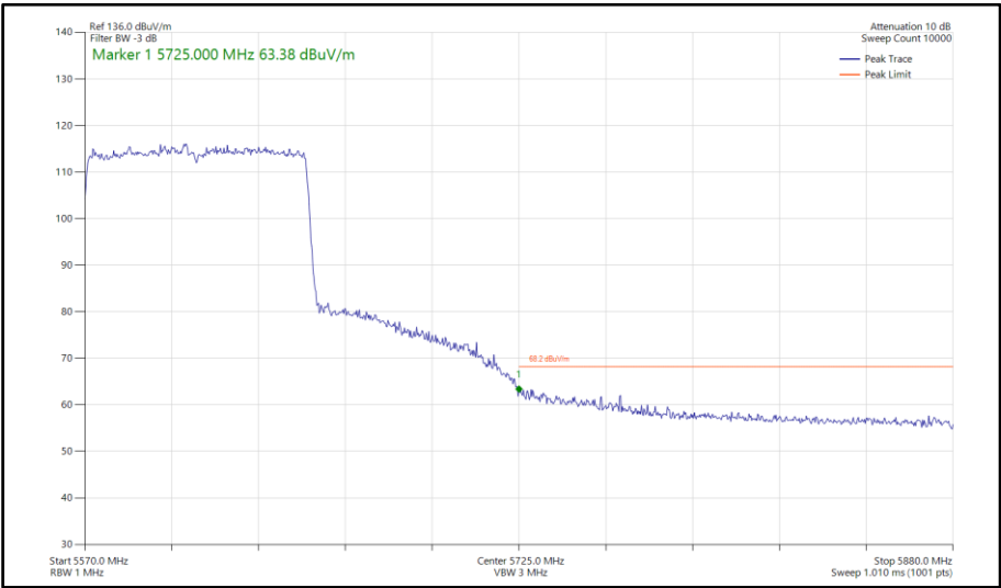
Figure 1018 - 802.11ax HE80, SU, SDM, Core 0-1 - 5610 MHz Band Edge Frequency 5725 MHz
