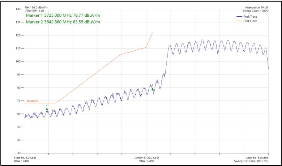
Figure 990 - 802.11ac VHT80, CDD, Core 0-1 - 5775 MHz Band Edge Frequency 5725 MHz
