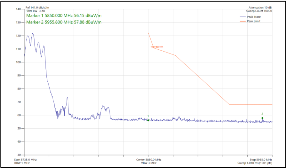
Figure 1006 - 802.11ax HE80, RU106-53, CDD, Core 0-1 - 5775 MHz Band Edge Frequency 5850 MHz
