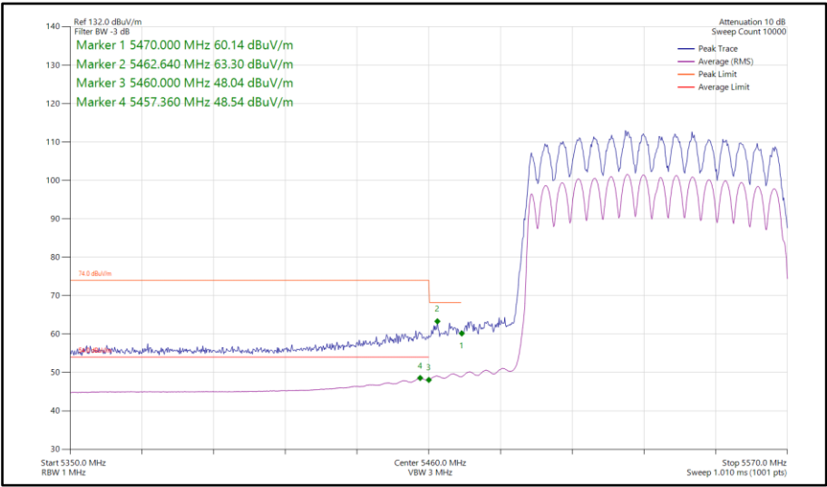
Figure 986 - 802.11ax HE80, SU, CDD, Core 0-1 - 5530 MHz Band Edge Frequency 5470 MHz
