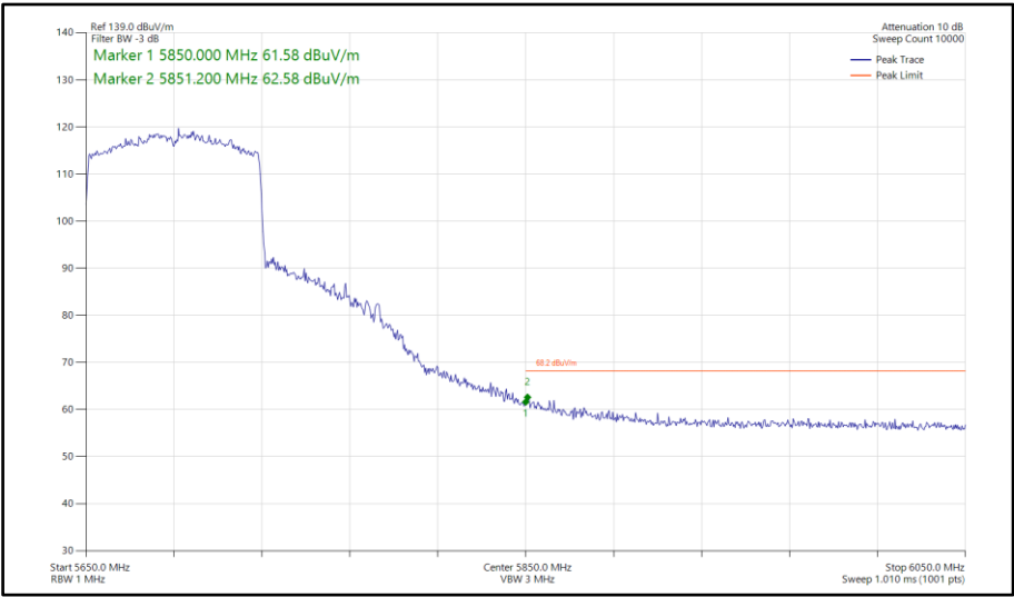
Figure 1023 - 802.11ax HE80, SU, SDM, Core 0-1 - 5690 MHz Band Edge Frequency 5850 MHz
