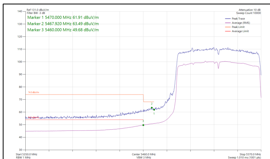
Figure 1009 - 802.11ac VHT80, SDM, Core 0-1 - 5530 MHz Band Edge Frequency 5470 MHz
