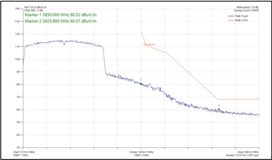
Figure 978 - 802.11ac VHT80, SISO, Core 1 - 5775 MHz Band Edge Frequency 5850 MHz
