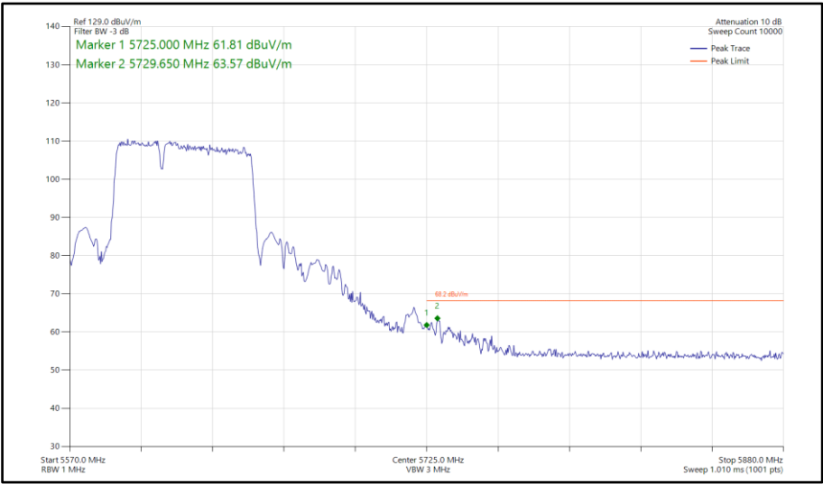
Figure 950 - 802.11be EHT80, RU484+242-90, SISO, Core 0 - 5610 MHz Band Edge Frequency 5725 MHz
