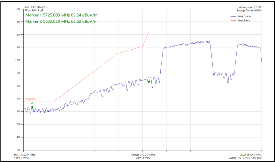
Figure 945 - 802.11be EHT80, RU484+242-92, SISO, Core 0 - 5775 MHz Band Edge Frequency 5725 MHz
