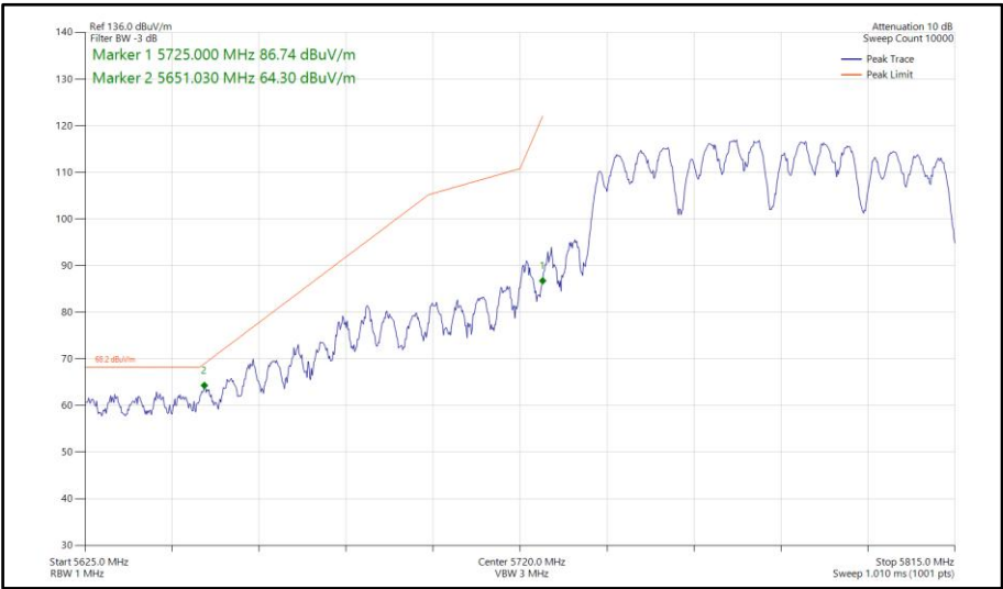
Figure 989 - 802.11a a80, CDD, Core 0-1 - 5775 MHz Band Edge Frequency 5725 MHz
