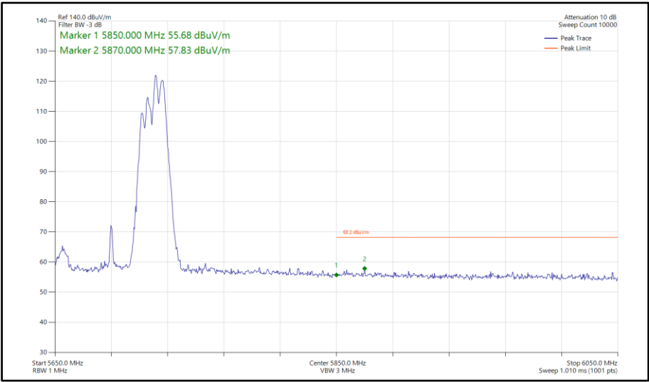
Figure 1004 - 802.11ax HE80, RU106-60, CDD, Core 0-1 - 5690 MHz Band Edge Frequency 5850 MHz
