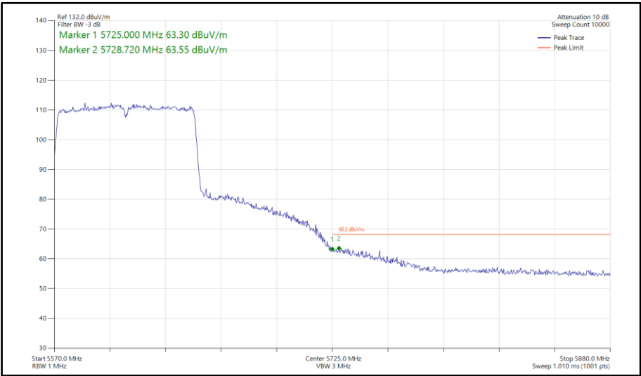
Figure 971 - 802.11ac VHT80, SISO, Core 1 - 5610 MHz Band Edge Frequency 5725 MHz
