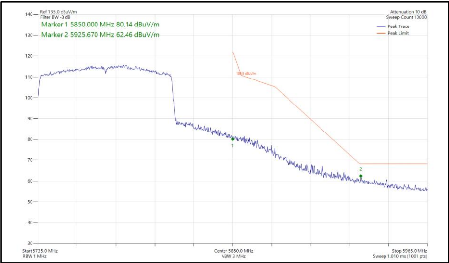
Figure 957 - 802.11ax HE80, SU, SISO, Core 0 - 5775 MHz Band Edge Frequency 5850 MHz
