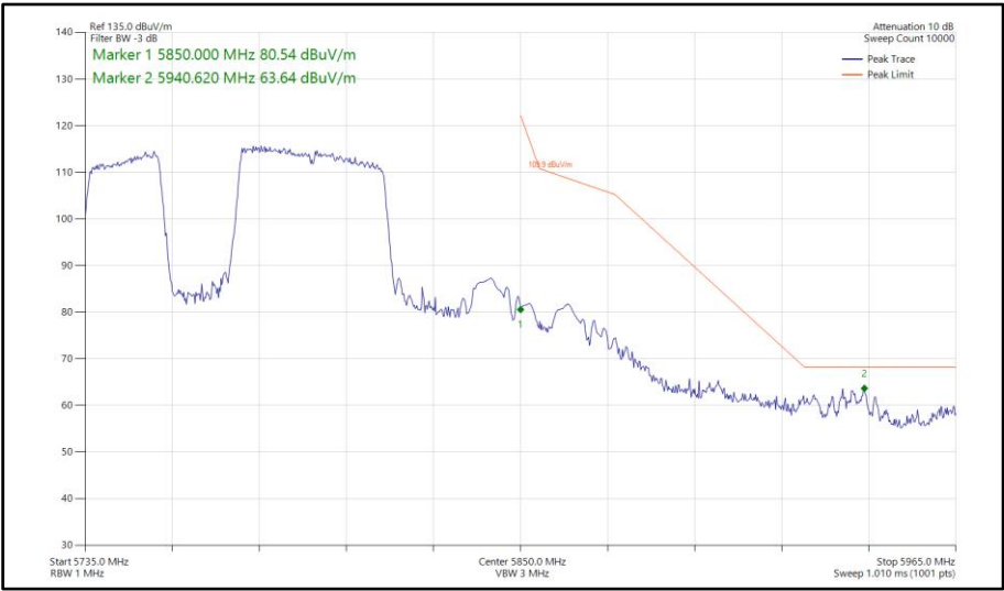
Figure 960 - 802.11be EHT80, RU484+242-91, SISO, Core 0 - 5775 MHz Band Edge Frequency 5850 MHz
