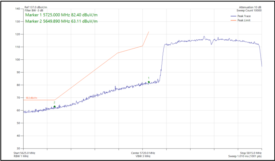
Figure 1013 - 802.11ac VHT80, SDM, Core 0-1 - 5775 MHz Band Edge Frequency 5725 MHz
