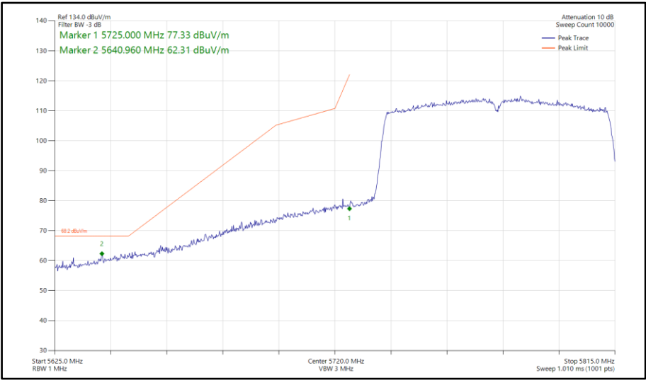
Figure 942 - 802.11ac VHT80, SISO, Core 0 - 5775 MHz Band Edge Frequency 5725 MHz
