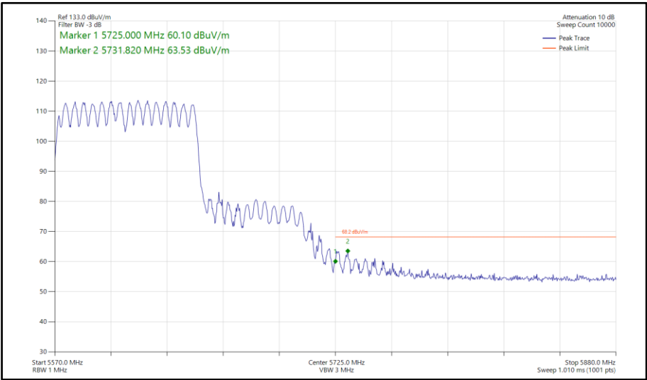
Figure 995 - 802.11ac VHT80, CDD, Core 0-1 - 5610 MHz Band Edge Frequency 5725 MHz
