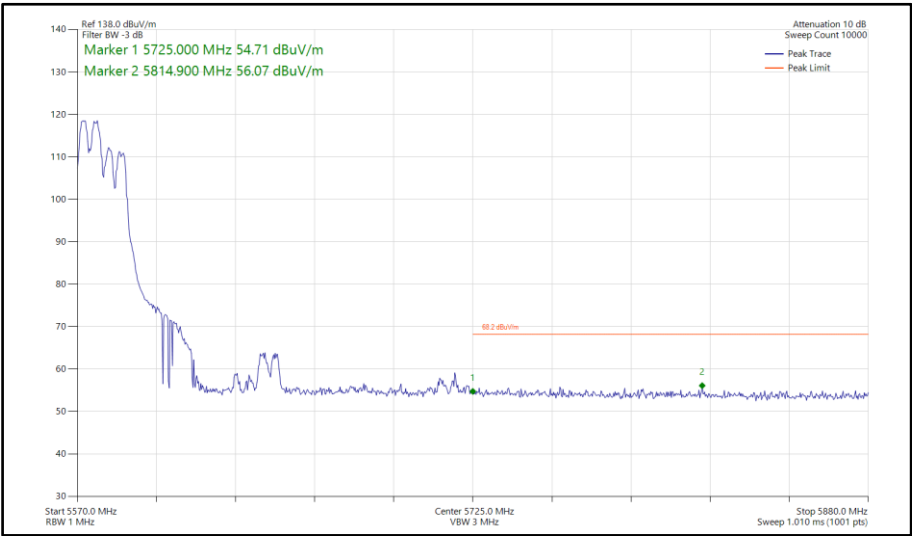
Figure 997 - 802.11ax HE80, RU106-53, CDD, Core 0-1 - 5610 MHz Band Edge Frequency 5725 MHz
