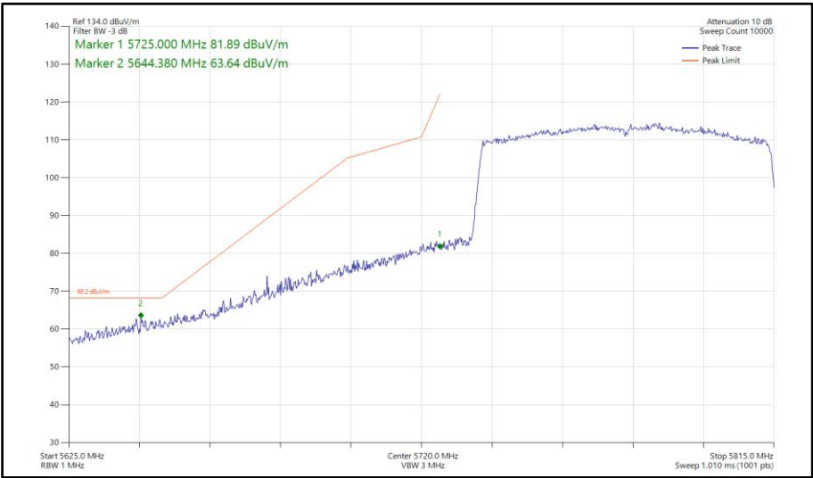
Figure 943 - 802.11ax HE80, SU, SISO, Core 0 - 5775 MHz Band Edge Frequency 5725 MHz
