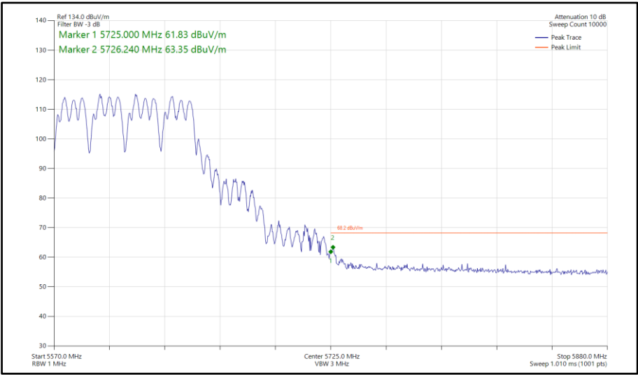
Figure 994 - 802.11a a80, CDD, Core 0-1 - 5610 MHz Band Edge Frequency 5725 MHz
