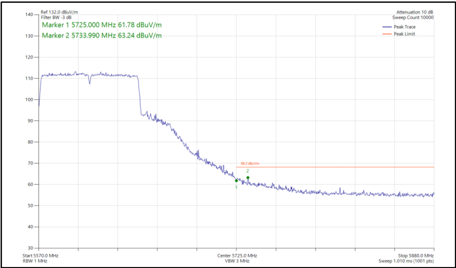
Figure 947 - 802.11ac VHT80, SISO, Core 0 - 5610 MHz Band Edge Frequency 5725 MHz
