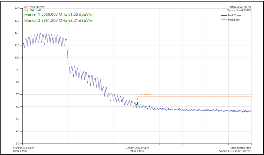
Figure 1001 - 802.11ac VHT80, CDD, Core 0-1 - 5690 MHz Band Edge Frequency 5850 MHz
