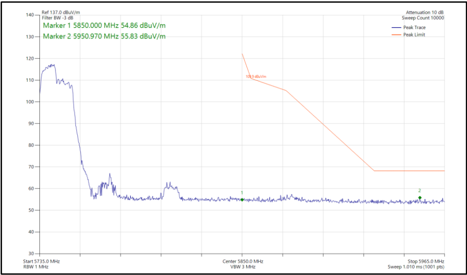
Figure 982 - 802.11ax HE80, RU106-53, SISO, Core 1 - 5775 MHz Band Edge Frequency 5850 MHz
