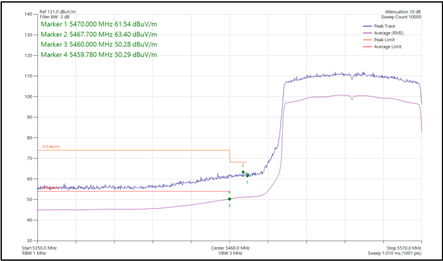
Figure 962 - 802.11ax HE80, SU, SISO, Core 1 - 5530 MHz Band Edge Frequency 5470 MHz
