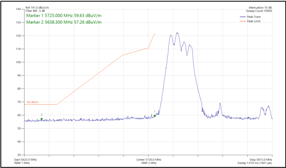
Figure 1015 - 802.11ax HE80, RU106-53, SDM, Core 0-1 - 5775 MHz Band Edge Frequency 5725 MHz
