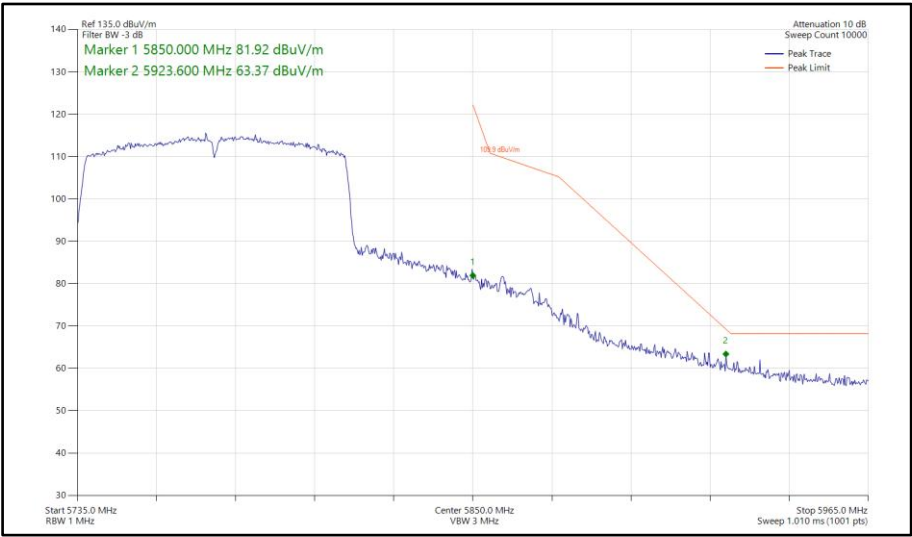
Figure 954 - 802.11ac VHT80, SISO, Core 0 - 5775 MHz Band Edge Frequency 5850 MHz
