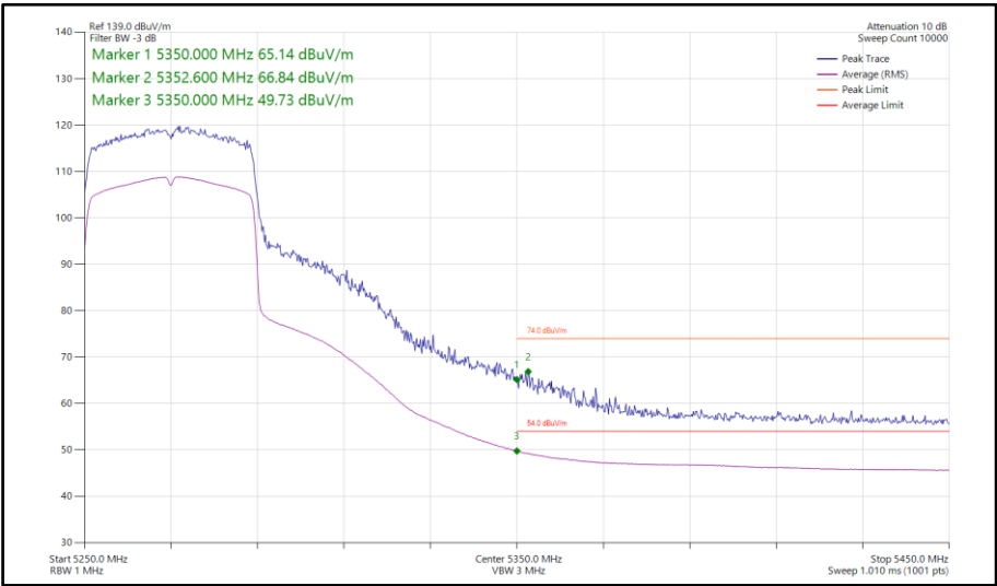
Figure 138 - 802.11ax HE40, SU, SISO, Core 0 - 5270 MHz Band Edge Frequency 5350 MHz
