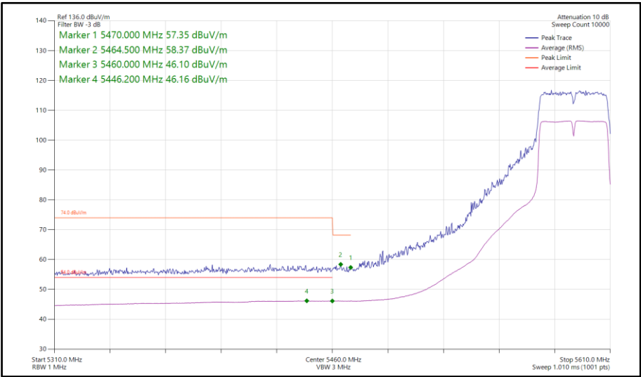
Figure 183 - 802.11n HT40, SISO, Core 1 - 5590 MHz Band Edge Frequency 5460 MHz
