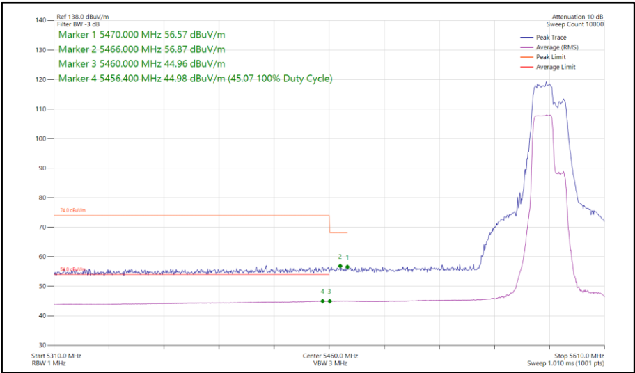
Figure 158 - 802.11be EHT40, RU106+26-82, SISO, Core 0 - 5590 MHz Band Edge Frequency 5460 MHz
