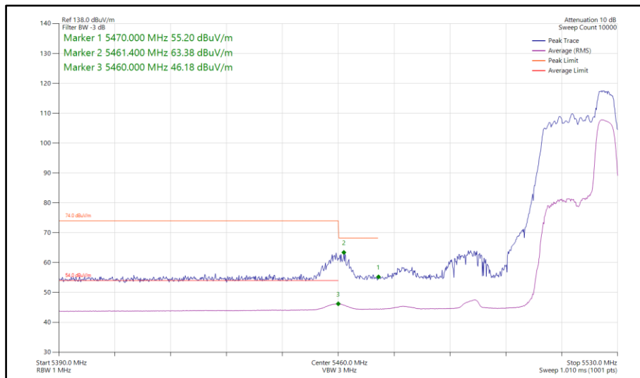
Figure 151 - 802.11ax HE40, RU52-44, SISO, Core 0 - 5510 MHz Band Edge Frequency 5460 MHz
