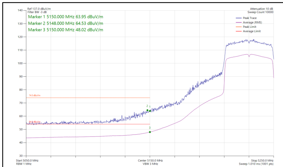
Figure 165 - 802.11ax HE40, SU, SISO, Core 1 - 5230 MHz Band Edge Frequency 5150 MHz
