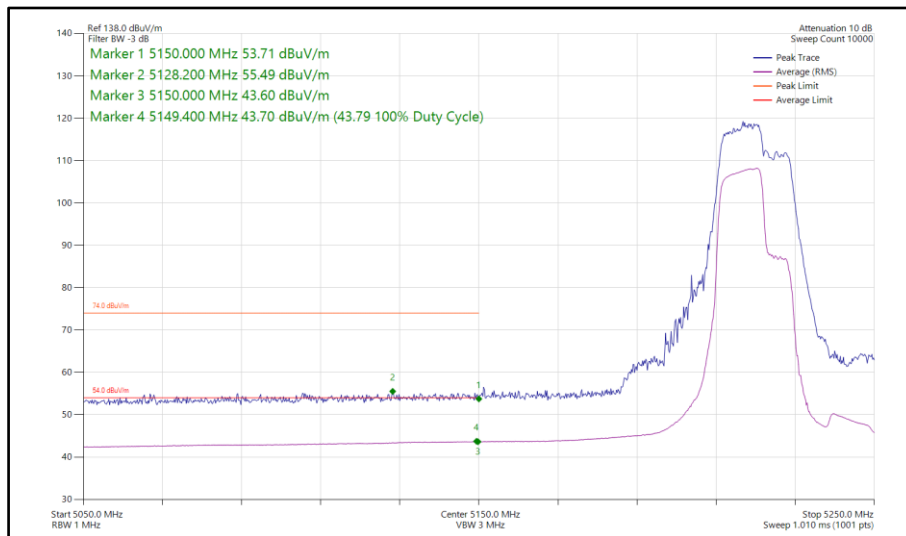
Figure 168 - 802.11be EHT40, RU106+26-82, SISO, Core 1 - 5230 MHz Band Edge Frequency 5150 MHz
