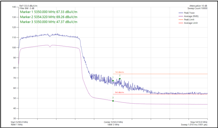
Figure 140 - 802.11ax HE40, SU, SISO, Core 0 - 5310 MHz Band Edge Frequency 5350 MHz
