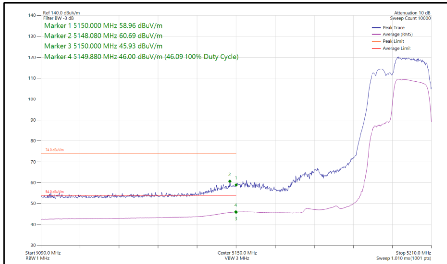
Figure 167 - 802.11be EHT40, RU106+26-85, SISO, Core 1 - 5190 MHz Band Edge Frequency 5150 MHz
