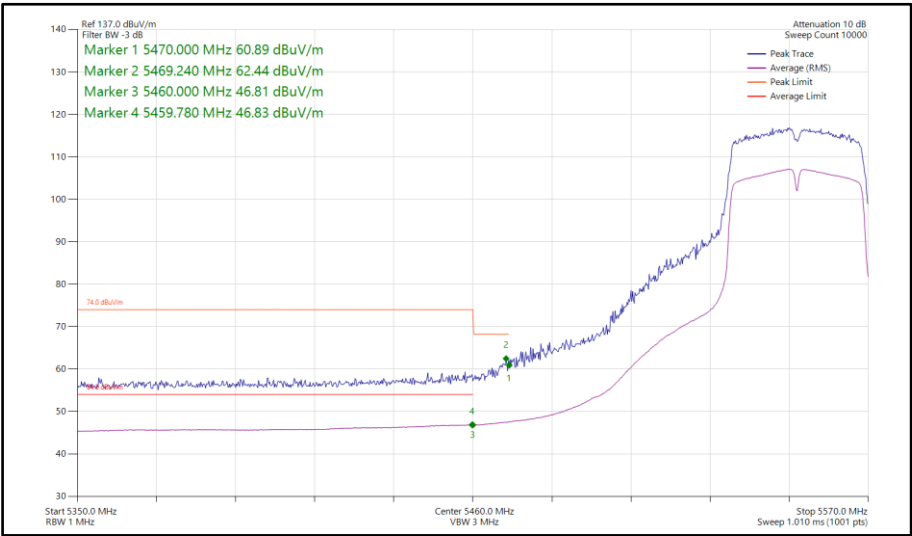
Figure 148 - 802.11n HT40, SISO, Core 0 - 5550 MHz Band Edge Frequency 5460 MHz
