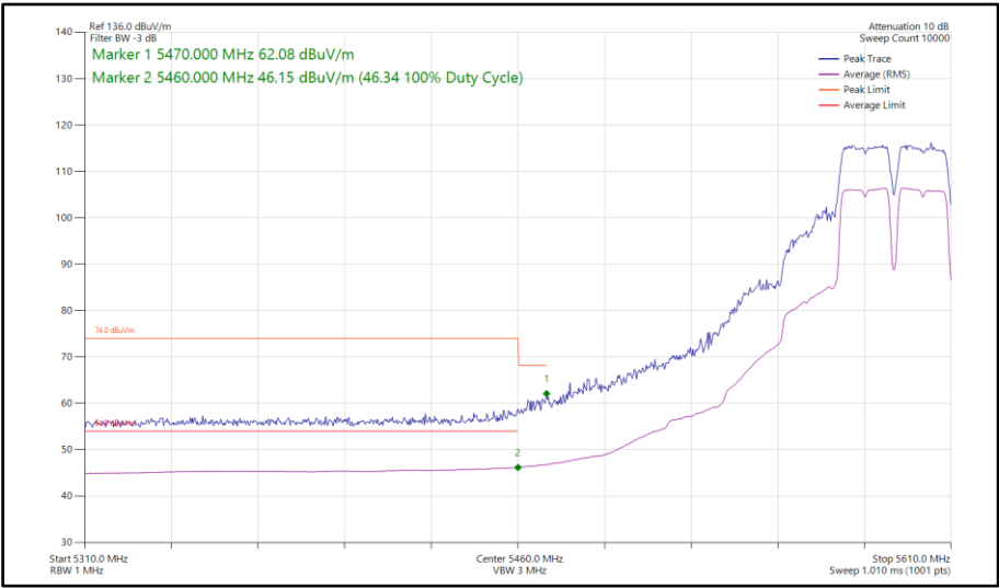
Figure 180 - 802.11a a40, SISO, Core 1 - 5590 MHz Band Edge Frequency 5460 MHz
