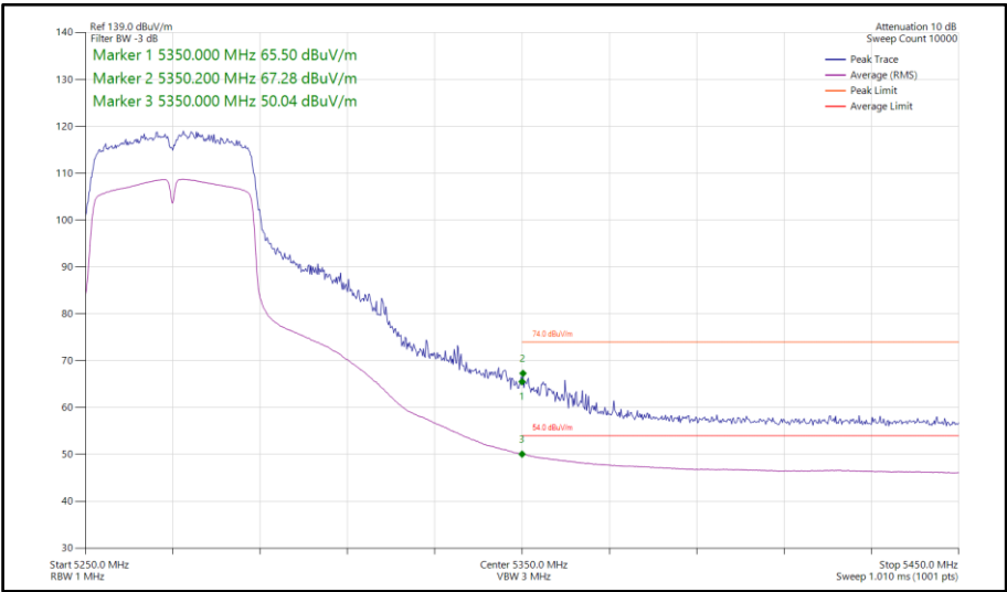
Figure 136 - 802.11n HT40, SISO, Core 0 - 5270 MHz Band Edge Frequency 5350 MHz
