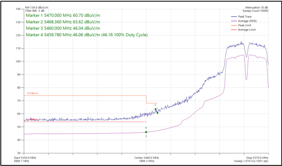
Figure 145 - 802.11a a40, SISO, Core 0 - 5550 MHz Band Edge Frequency 5460 MHz
