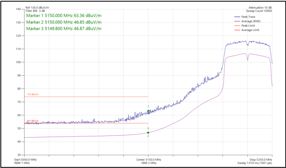
Figure 162 - 802.11n HT40, SISO, Core 1 - 5230 MHz Band Edge Frequency 5150 MHz
