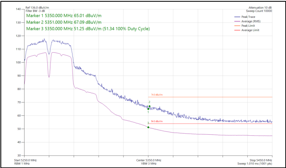
Figure 169 - 802.11a a40, SISO, Core 1 - 5270 MHz Band Edge Frequency 5350 MHz
