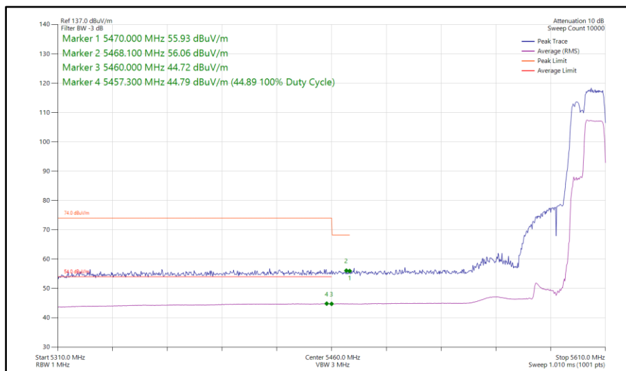
Figure 192 - 802.11be EHT40, RU106+26-85, SISO, Core 1 - 5590 MHz Band Edge Frequency 5460 MHz
