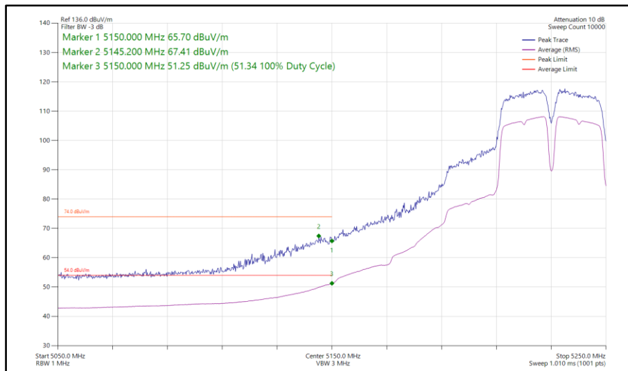
Figure 160 - 802.11a a40, SISO, Core 1 - 5230 MHz Band Edge Frequency 5150 MHz
