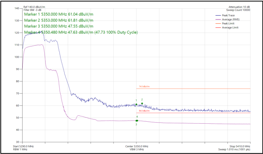
Figure 143 - 802.11be EHT40, RU106+26-82, SISO, Core 0 - 5310 MHz Band Edge Frequency 5350 MHz
