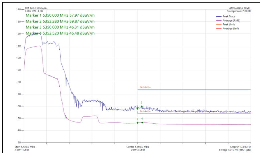
Figure 176 - 802.11ax HE40, RU106-53, SISO, Core 1 - 5310 MHz Band Edge Frequency 5350 MHz
