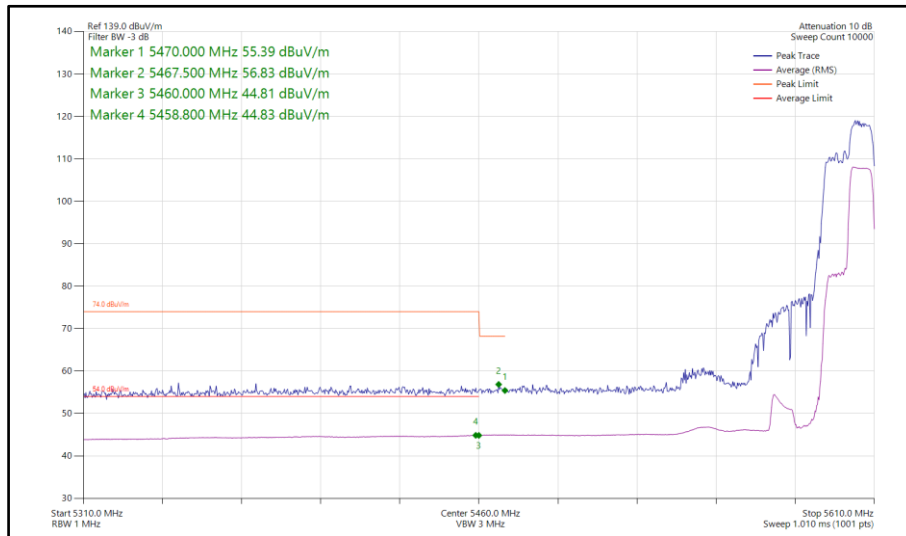
Figure 189 - 802.11ax HE40, RU106-56, SISO, Core 1 - 5590 MHz Band Edge Frequency 5460 MHz
