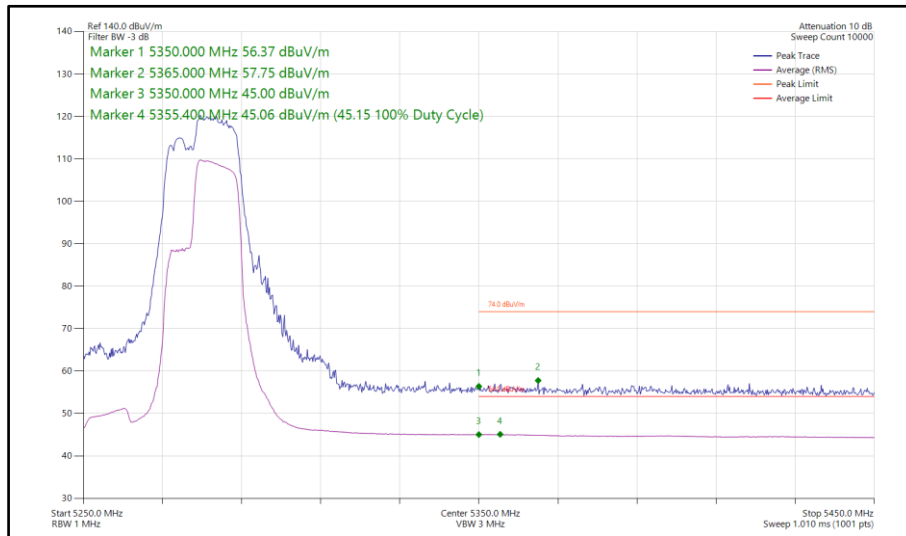
Figure 177 - 802.11be EHT40, RU106+26-85, SISO, Core 1 - 5270 MHz Band Edge Frequency 5350 MHz
