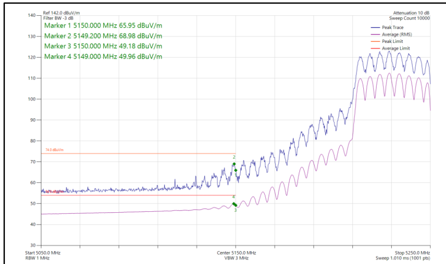
Figure 199 - 802.11ax HE40, SU, CDD, Core 0-1 - 5230 MHz Band Edge Frequency 5150 MHz
