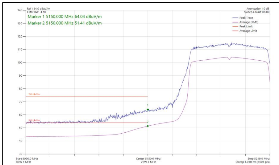
Figure 163 - 802.11ax HE40, SU, SISO, Core 1 - 5190 MHz Band Edge Frequency 5150 MHz
