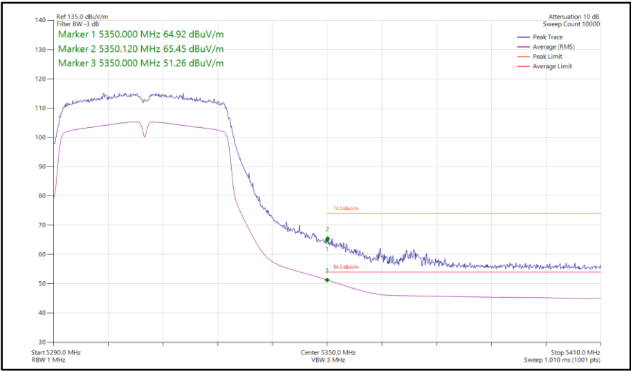
Figure 172 - 802.11n HT40, SISO, Core 1 - 5310 MHz Band Edge Frequency 5350 MHz
