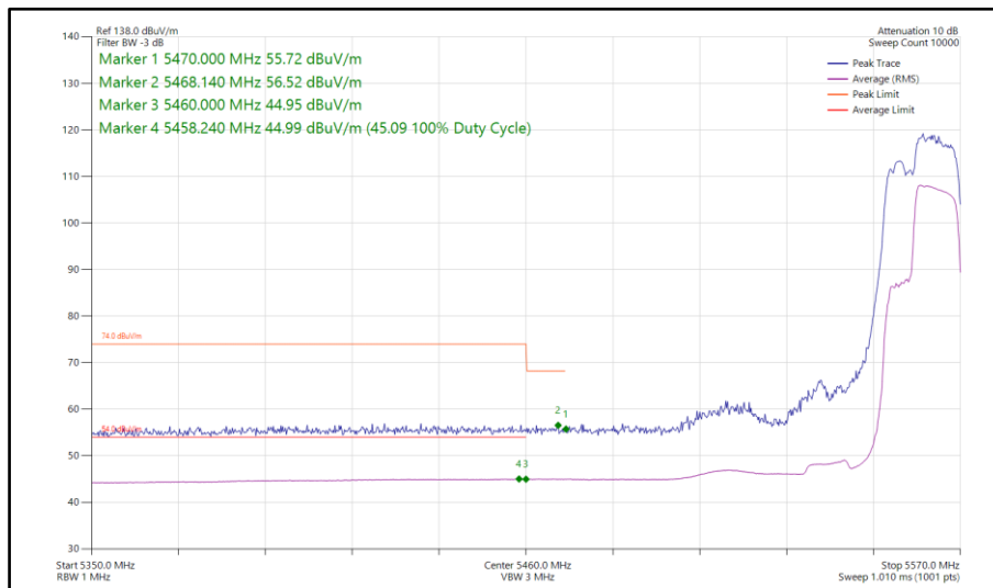
Figure 191 - 802.11be EHT40, RU106+26-85, SISO, Core 1 - 5550 MHz Band Edge Frequency 5460 MHz
