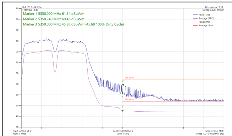
Figure 135 - 802.11a a40, SISO, Core 0 - 5310 MHz Band Edge Frequency 5350 MHz
