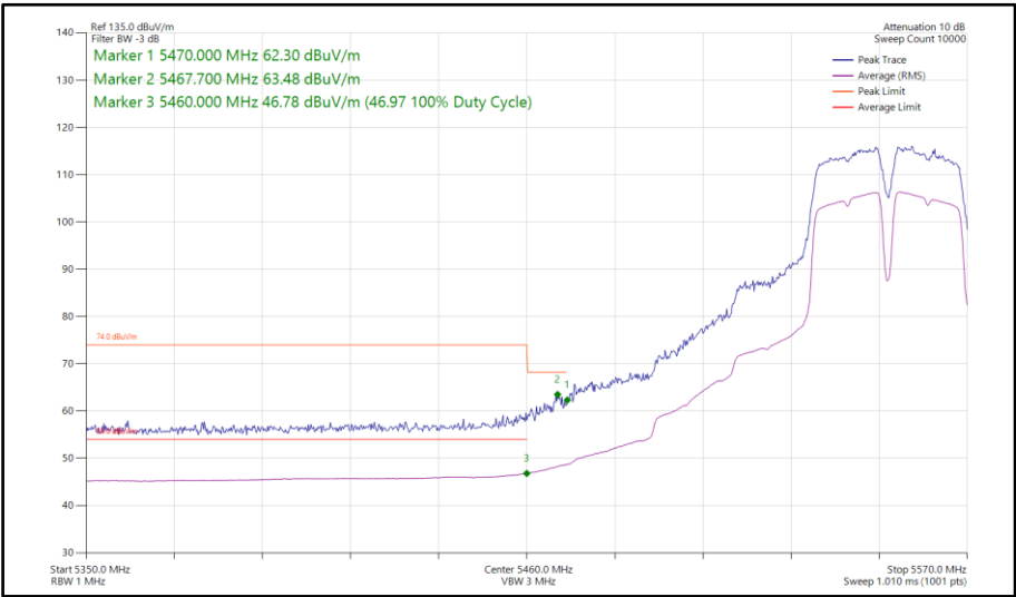
Figure 179 - 802.11a a40, SISO, Core 1 - 5550 MHz Band Edge Frequency 5460 MHz
