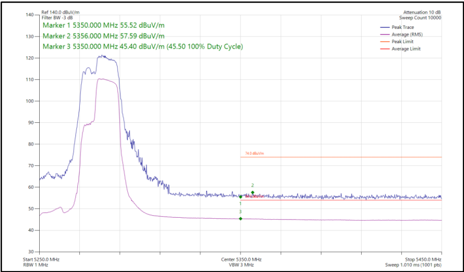
Figure 142 - 802.11be EHT40, RU106+26-85, SISO, Core 0 - 5270 MHz Band Edge Frequency 5350 MHz
