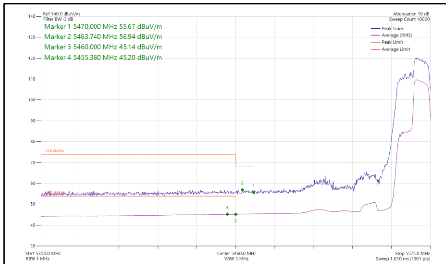
Figure 153 - 802.11ax HE40, RU106-56, SISO, Core 0 - 5550 MHz Band Edge Frequency 5460 MHz
