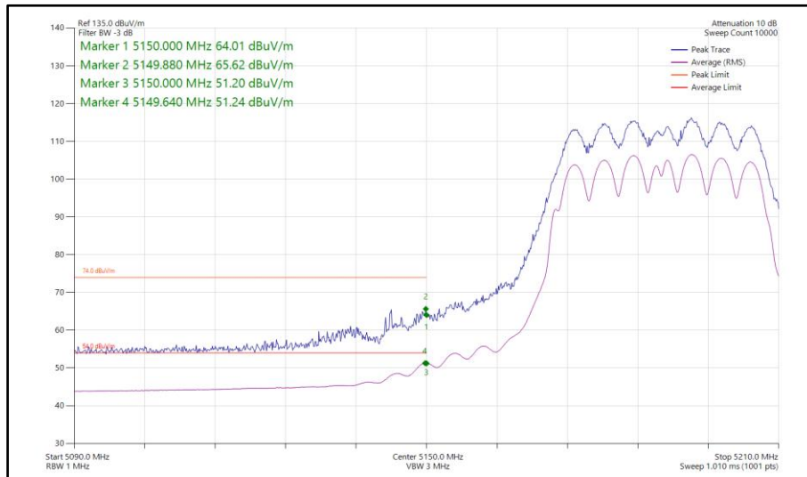
Figure 195 - 802.11n HT40, CDD, Core 0-1 - 5190 MHz Band Edge Frequency 5150 MHz
