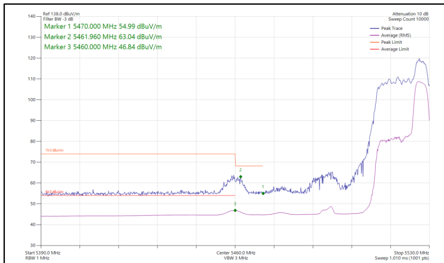
Figure 185 - 802.11ax HE40, RU52-44, SISO, Core 1 - 5510 MHz Band Edge Frequency 5460 MHz
