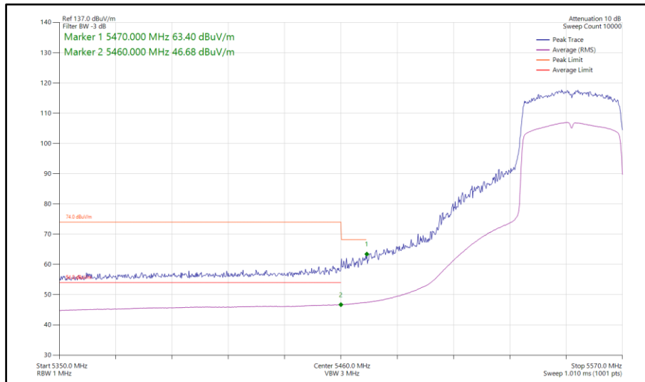
Figure 152 - 802.11ax HE40, SU, SISO, Core 0 - 5550 MHz Band Edge Frequency 5460 MHz
