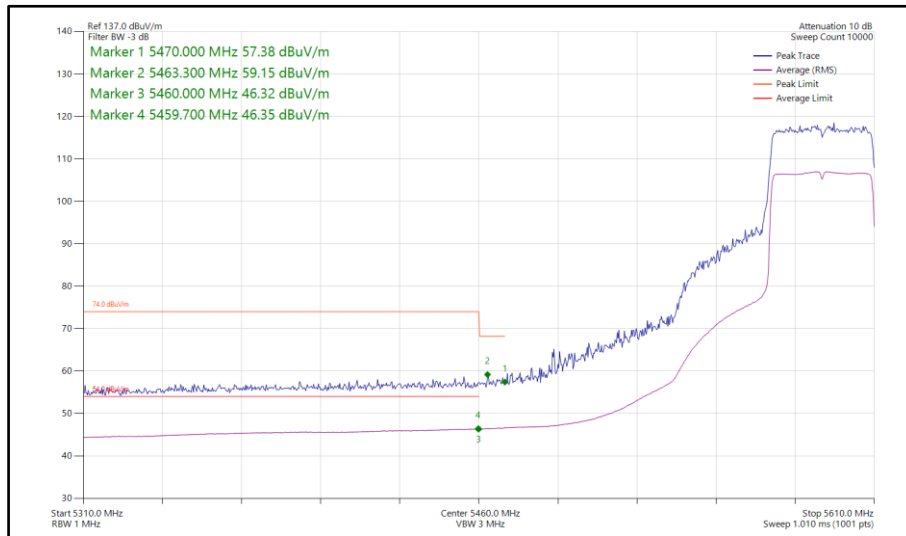
Figure 154 - 802.11ax HE40, SU, SISO, Core 0 - 5590 MHz Band Edge Frequency 5460 MHz
