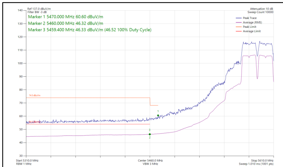
Figure 146 - 802.11a a40, SISO, Core 0 - 5590 MHz Band Edge Frequency 5460 MHz
