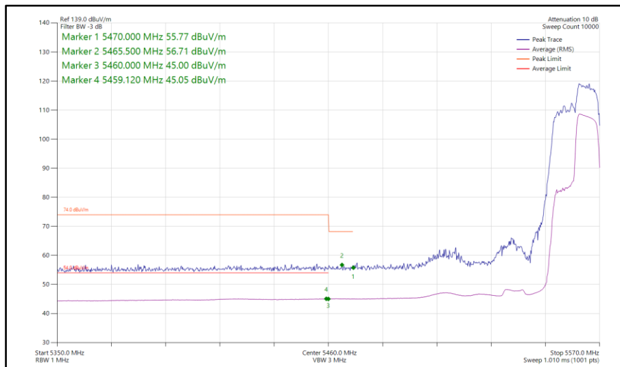
Figure 187 - 802.11ax HE40, RU106-56, SISO, Core 1 - 5550 MHz Band Edge Frequency 5460 MHz
