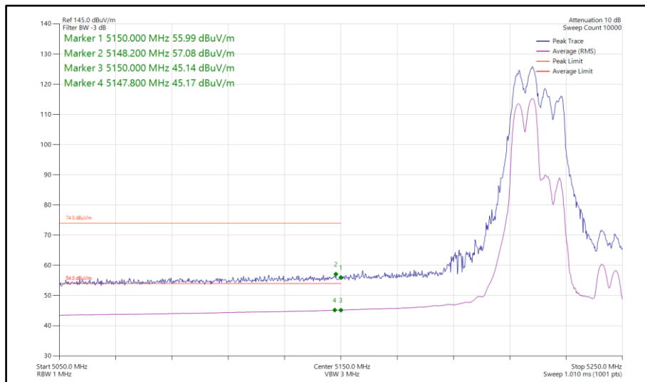
Figure 200 - 802.11ax HE40, RU106-53, CDD, Core 0-1 - 5230 MHz Band Edge Frequency 5150 MHz
