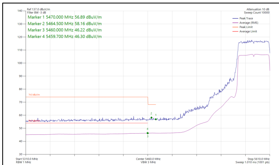
Figure 188 - 802.11ax HE40, SU, SISO, Core 1 - 5590 MHz Band Edge Frequency 5460 MHz
