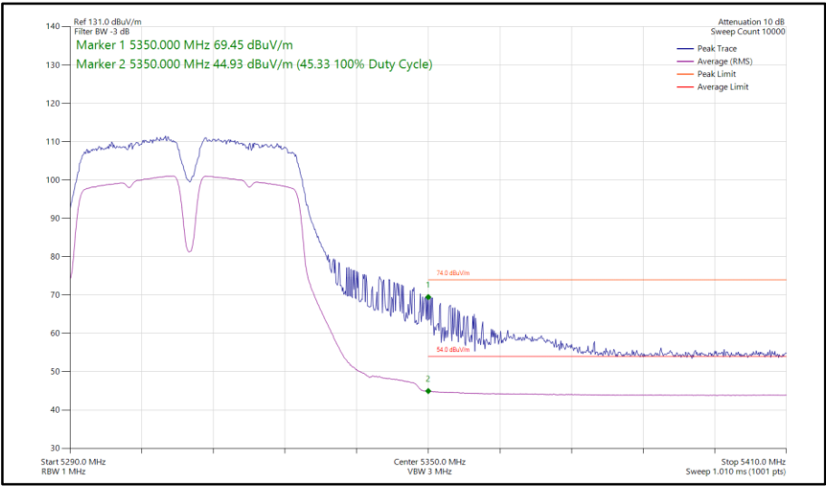
Figure 170 - 802.11a a40, SISO, Core 1 - 5310 MHz Band Edge Frequency 5350 MHz
