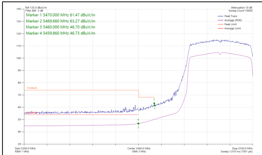
Figure 150 - 802.11ax HE40, SU, SISO, Core 0 - 5510 MHz Band Edge Frequency 5460 MHz
