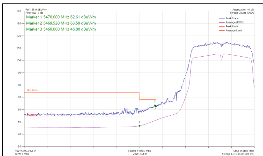
Figure 147 - 802.11n HT40, SISO, Core 0 - 5510 MHz Band Edge Frequency 5460 MHz
