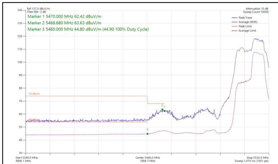
Figure 156 - 802.11be EHT40, RU52+26-75, SISO, Core 0 - 5510 MHz Band Edge Frequency 5460 MHz
