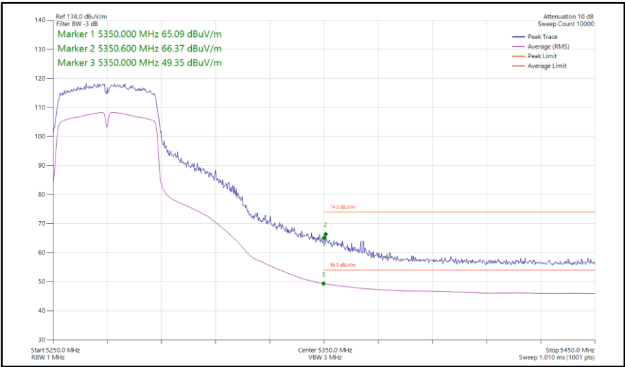
Figure 171 - 802.11n HT40, SISO, Core 1 - 5270 MHz Band Edge Frequency 5350 MHz
