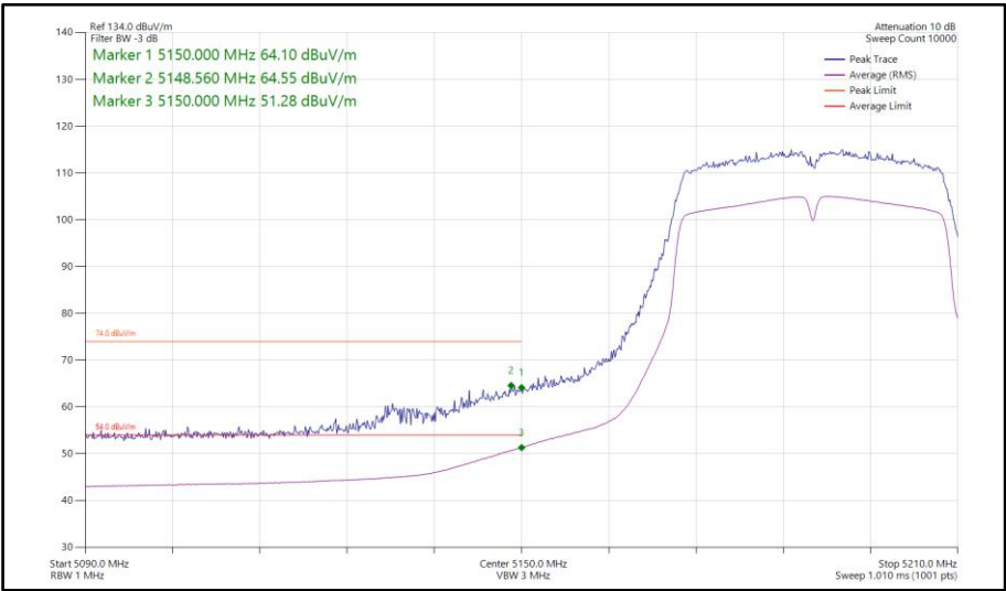
Figure 161 - 802.11n HT40, SISO, Core 1 - 5190 MHz Band Edge Frequency 5150 MHz
