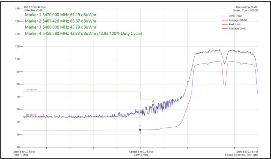
Figure 144 - 802.11a a40, SISO, Core 0 - 5510 MHz Band Edge Frequency 5460 MHz
