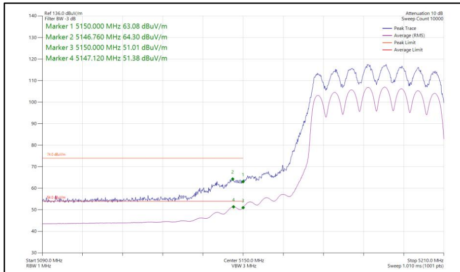
Figure 197 - 802.11ax HE40, SU, CDD, Core 0-1 - 5190 MHz Band Edge Frequency 5150 MHz
