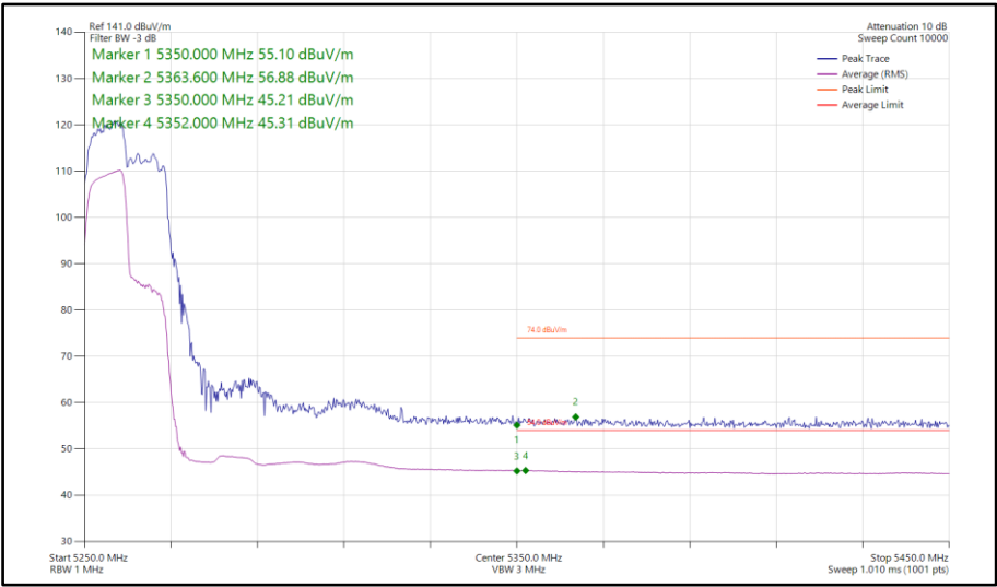
Figure 139 - 802.11ax HE40, RU106-53, SISO, Core 0 - 5270 MHz Band Edge Frequency 5350 MHz
