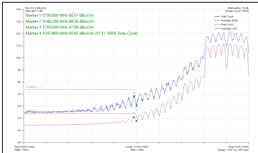
Figure 194 - 802.11a a40, CDD, Core 0-1 - 5230 MHz Band Edge Frequency 5150 MHz
