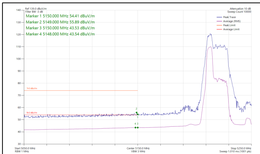
Figure 166 - 802.11ax HE40, RU52-37, SISO, Core 1 - 5230 MHz Band Edge Frequency 5150 MHz
