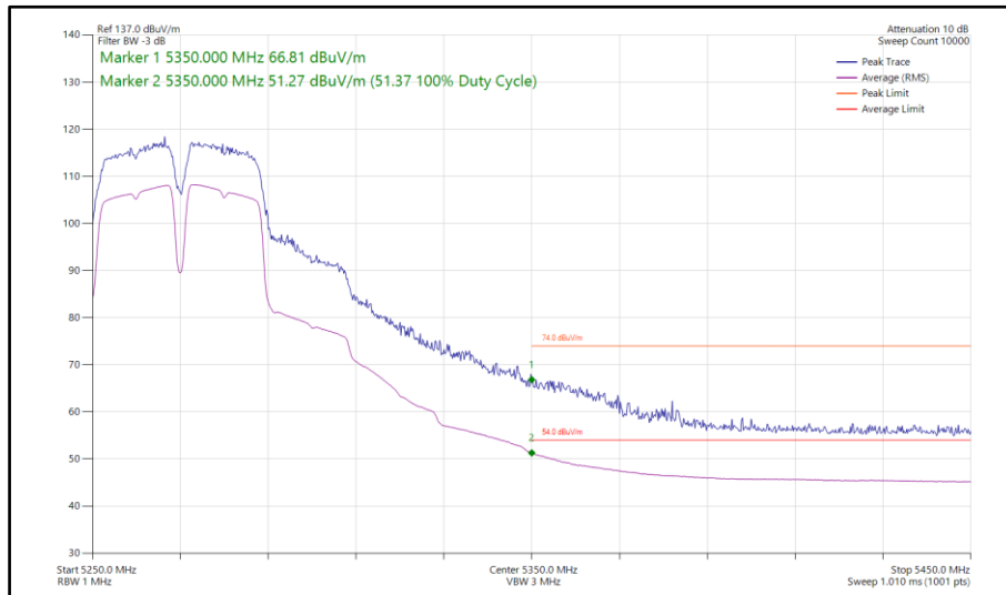
Figure 134 - 802.11a a40, SISO, Core 0 - 5270 MHz Band Edge Frequency 5350 MHz
