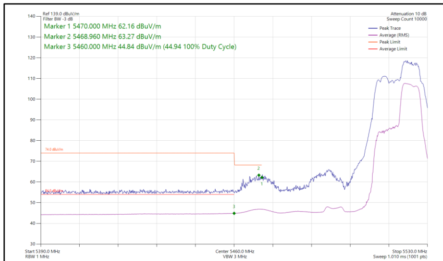
Figure 190 - 802.11be EHT40, RU52+26-75, SISO, Core 1 - 5510 MHz Band Edge Frequency 5460 MHz
