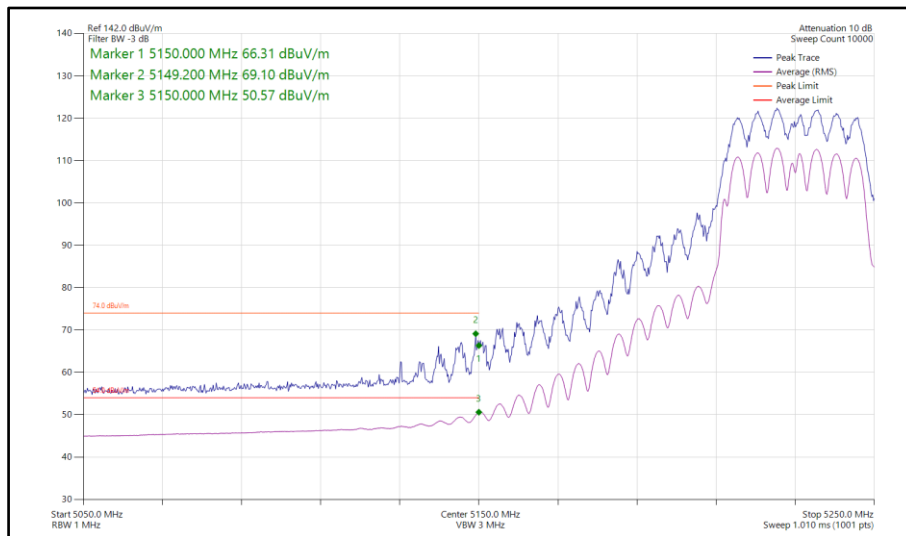
Figure 196 - 802.11n HT40, CDD, Core 0-1 - 5230 MHz Band Edge Frequency 5150 MHz
