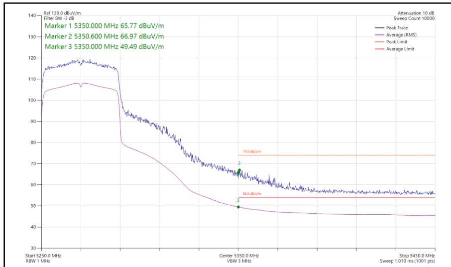
Figure 173 - 802.11ax HE40, SU, SISO, Core 1 - 5270 MHz Band Edge Frequency 5350 MHz
