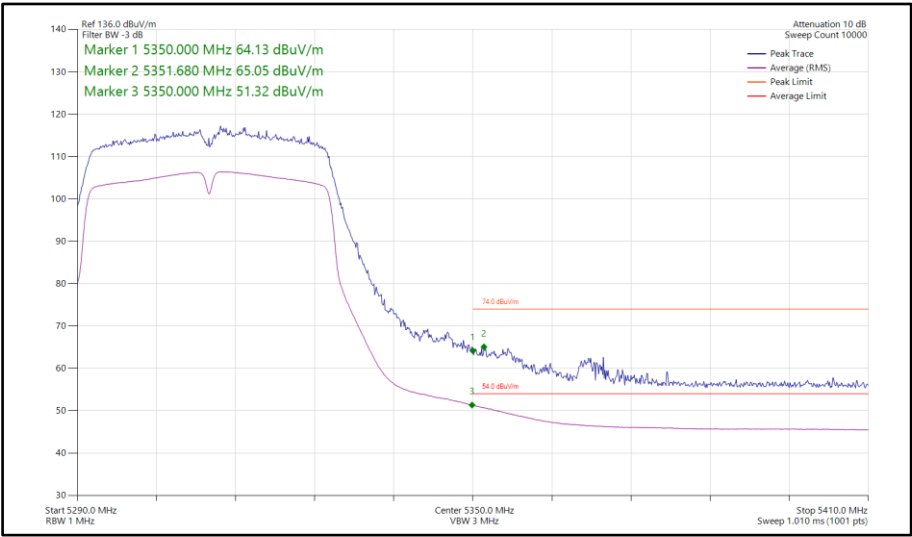
Figure 137 - 802.11n HT40, SISO, Core 0 - 5310 MHz Band Edge Frequency 5350 MHz
