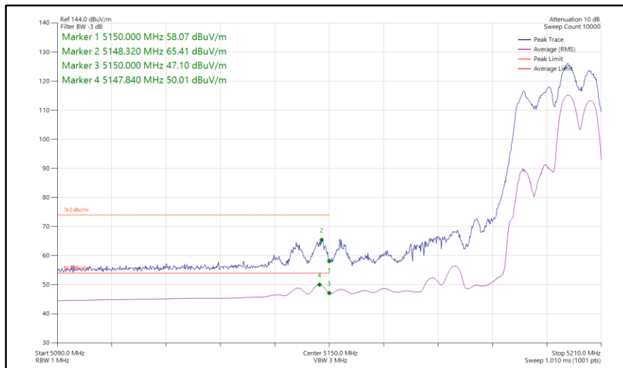
Figure 198 - 802.11ax HE40, RU106-56, CDD, Core 0-1 - 5190 MHz Band Edge Frequency 5150 MHz
