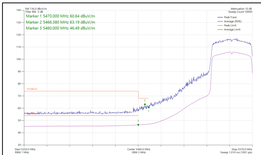
Figure 186 - 802.11ax HE40, SU, SISO, Core 1 - 5550 MHz Band Edge Frequency 5460 MHz
