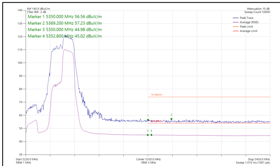
Figure 174 - 802.11ax HE40, RU106-56, SISO, Core 1 - 5270 MHz Band Edge Frequency 5350 MHz
