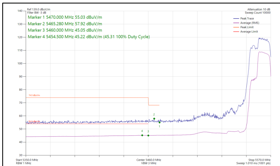
Figure 157 - 802.11be EHT40, RU106+26-85, SISO, Core 0 - 5550 MHz Band Edge Frequency 5460 MHz
