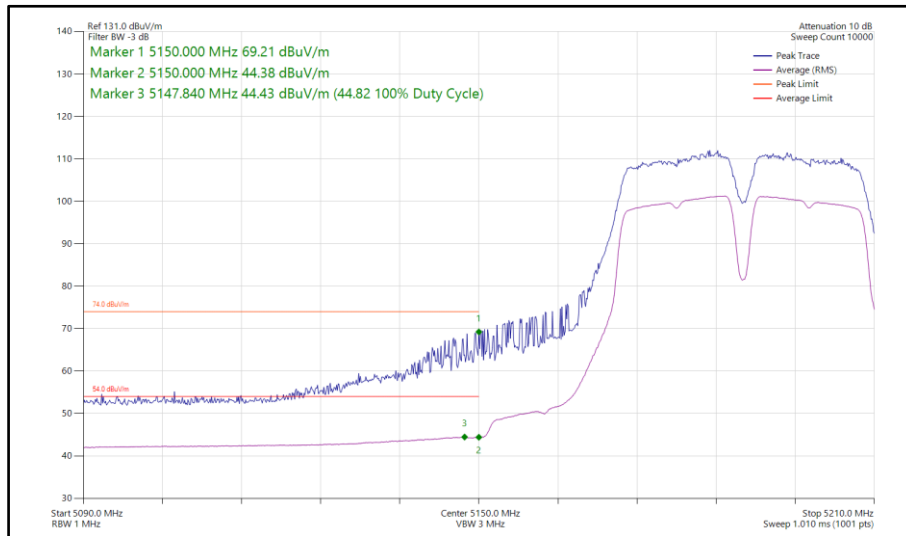
Figure 159 - 802.11a a40, SISO, Core 1 - 5190 MHz Band Edge Frequency 5150 MHz
