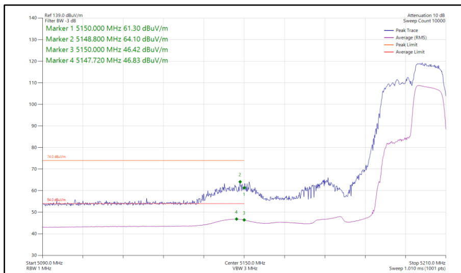
Figure 164 - 802.11ax HE40, RU106-56, SISO, Core 1 - 5190 MHz Band Edge Frequency 5150 MHz
