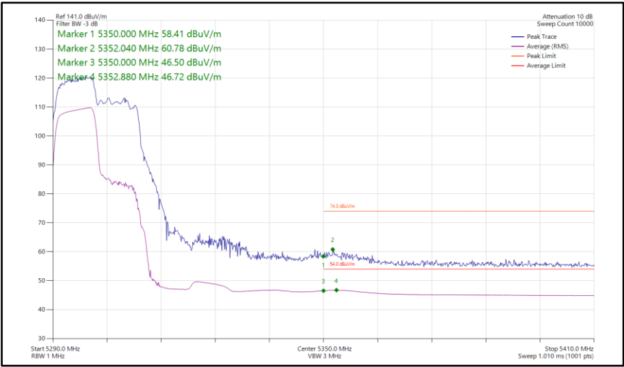
Figure 141 - 802.11ax HE40, RU106-53, SISO, Core 0 - 5310 MHz Band Edge Frequency 5350 MHz
