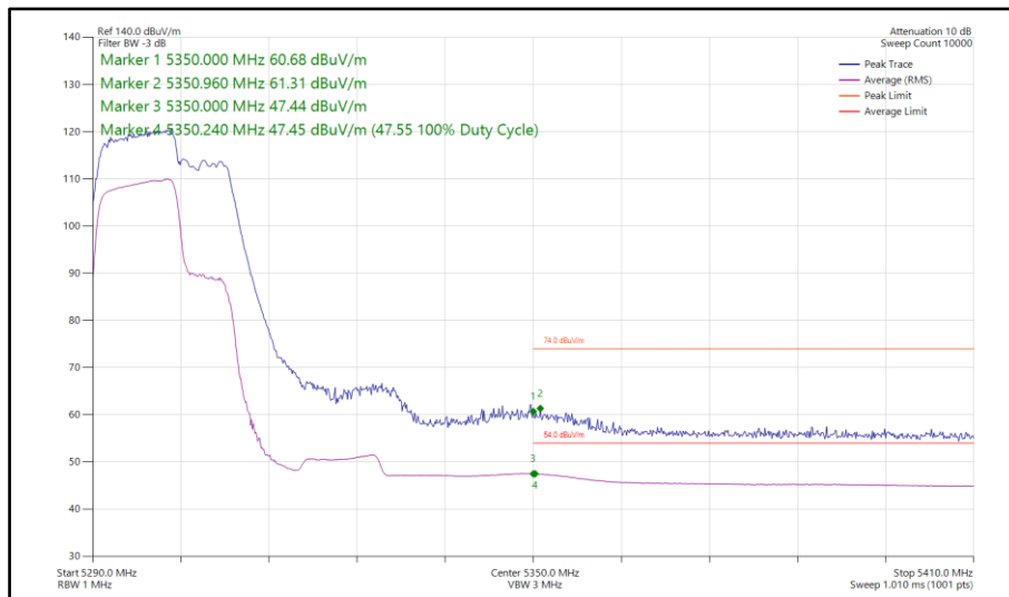
Figure 178 - 802.11be EHT40, RU106+26-82, SISO, Core 1 - 5310 MHz Band Edge Frequency 5350 MHz
