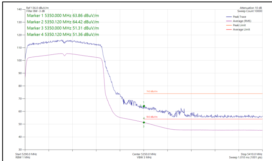
Figure 175 - 802.11ax HE40, SU, SISO, Core 1 - 5310 MHz Band Edge Frequency 5350 MHz
