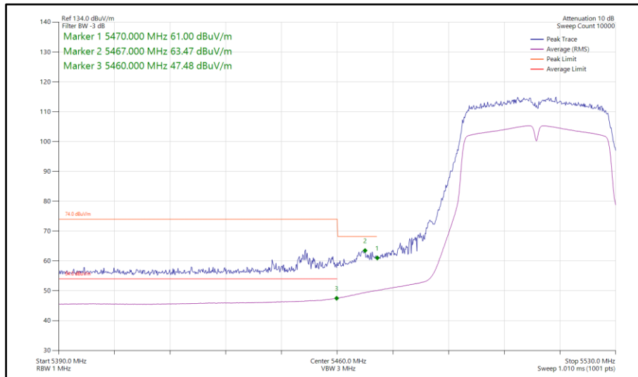
Figure 181 - 802.11n HT40, SISO, Core 1 - 5510 MHz Band Edge Frequency 5460 MHz
