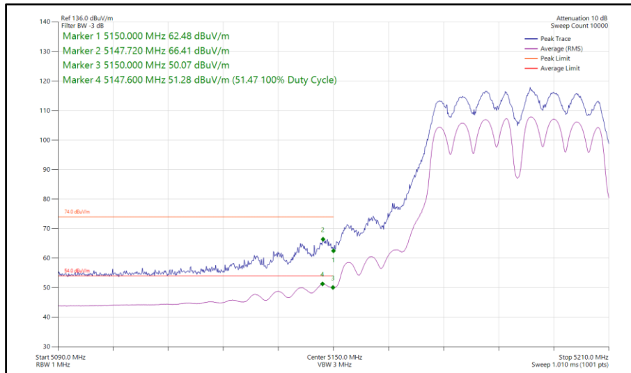
Figure 193 - 802.11a a40, CDD, Core 0-1 - 5190 MHz Band Edge Frequency 5150 MHz
