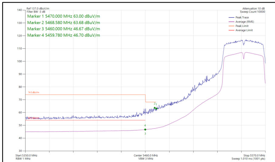
Figure 182 - 802.11n HT40, SISO, Core 1 - 5550 MHz Band Edge Frequency 5460 MHz
