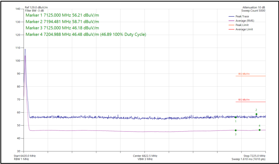
Figure 218 - Narrowband HDT6, SISO, Core 1 - 6425 MHz Band Edge Frequency 7125 MHz
