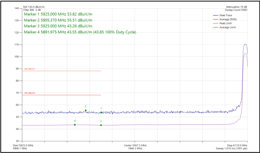
Figure 236 - Narrowband HDRPM12, MIMO, Core 0-1 - 6107 MHz Band Edge Frequency 5925 MHz
