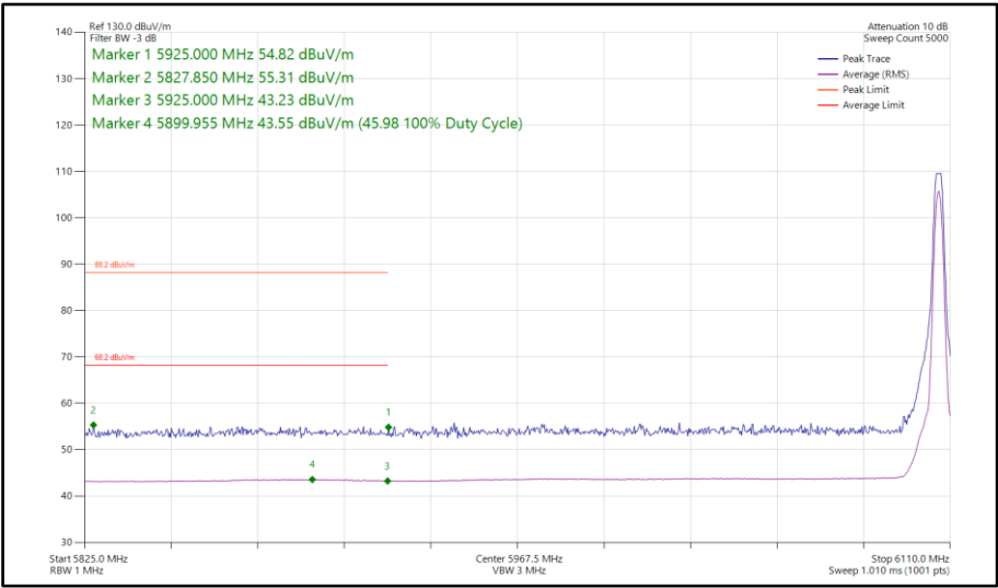
Figure 210 - Narrowband CS1LE2M, SISO, Core 1 - 6106 MHz Band Edge Frequency 5925 MHz
