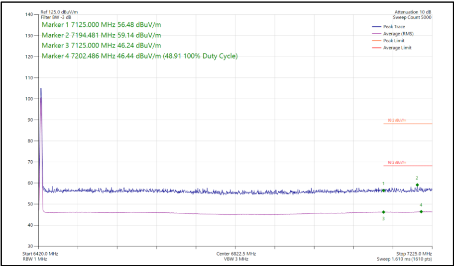
Figure 247 - Narrowband LE2M, MIMO, Core 0-1 - 6425 MHz Band Edge Frequency 7125 MHz
