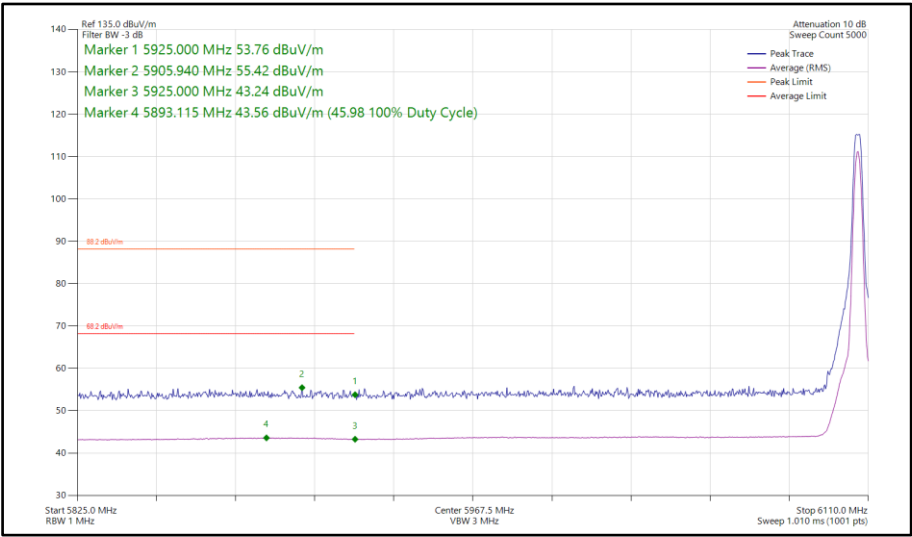
Figure 242 - Narrowband CS1LE2M, MIMO, Core 0-1 - 6106 MHz Band Edge Frequency 5925 MHz
