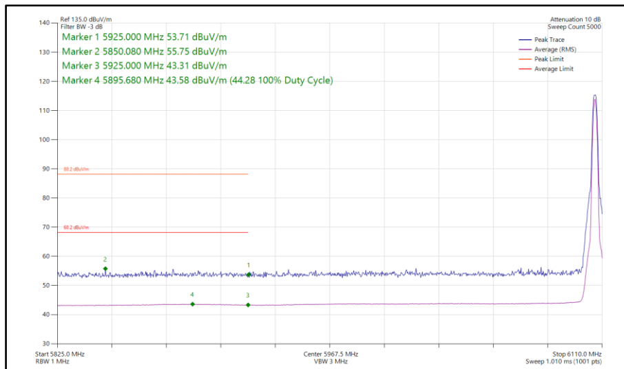
Figure 230 - Narrowband LE1M, MIMO, Core 0-1 - 6106 MHz Band Edge Frequency 5925 MHz
