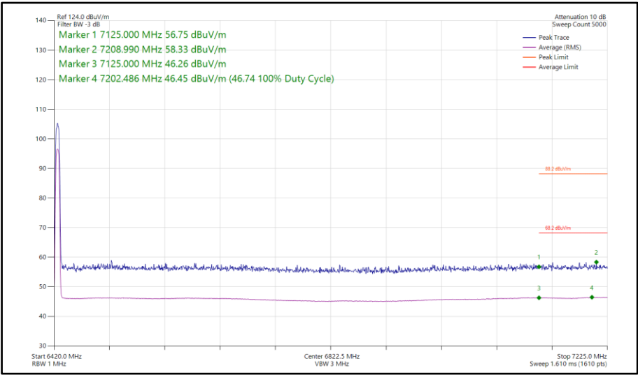
Figure 220 - Narrowband HDRPM12, SISO, Core 1 - 6425 MHz Band Edge Frequency 7125 MHz
