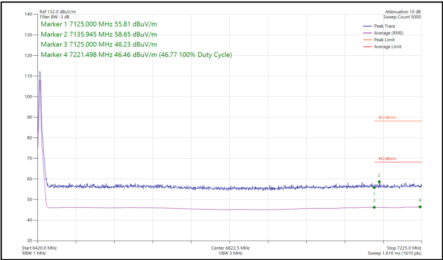
Figure 249 - Narrowband HDT4, MIMO, Core 0-1 - 6425 MHz Band Edge Frequency 7125 MHz
