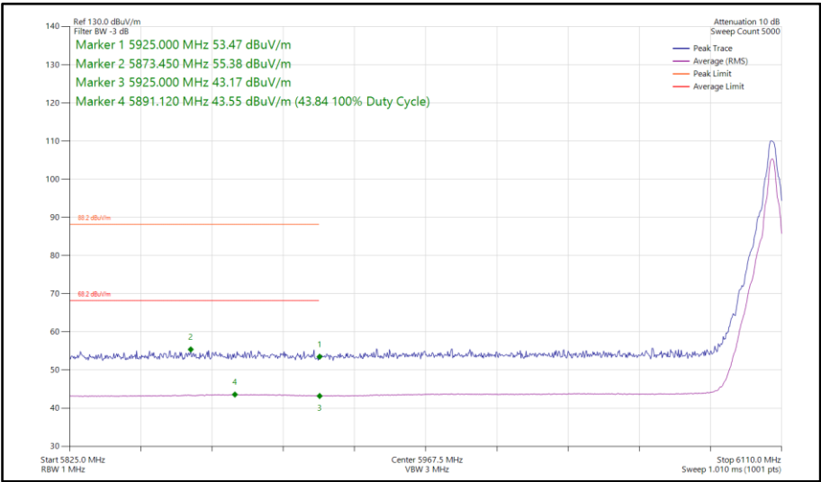
Figure 201 - Narrowband HDT4, SISO, Core 1 - 6106 MHz Band Edge Frequency 5925 MHz
