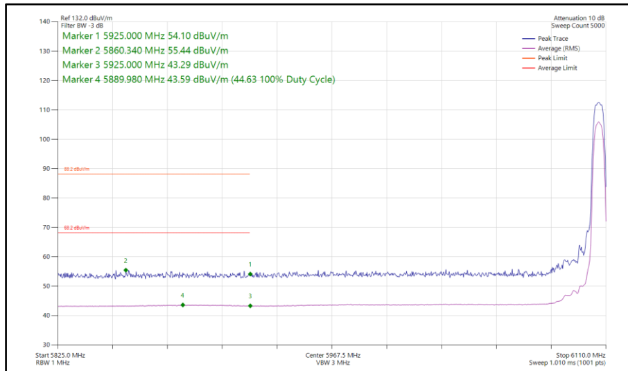
Figure 229 - Narrowband HDR8, MIMO, Core 0-1 - 6106 MHz Band Edge Frequency 5925 MHz
