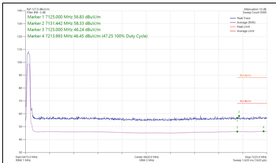
Figure 256 - Narrowband XHDRPL24, MIMO, Core 0-1 - 6425 MHz Band Edge Frequency 7125 MHz
