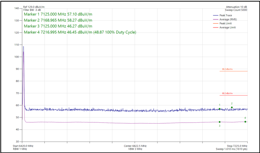
Figure 215 - Narrowband LE2M, SISO, Core 1 - 6425 MHz Band Edge Frequency 7125 MHz
