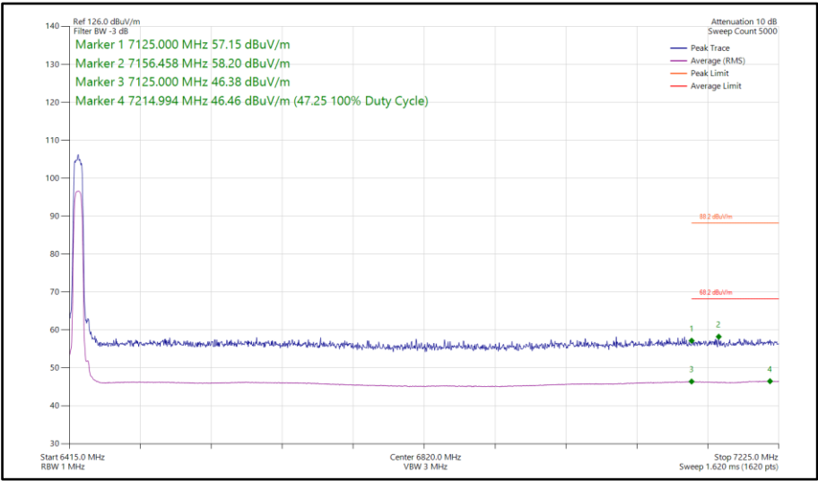
Figure 192 - Narrowband XHDRPL24, SISO, Core 0 - 6425 MHz Band Edge Frequency 7125 MHz
