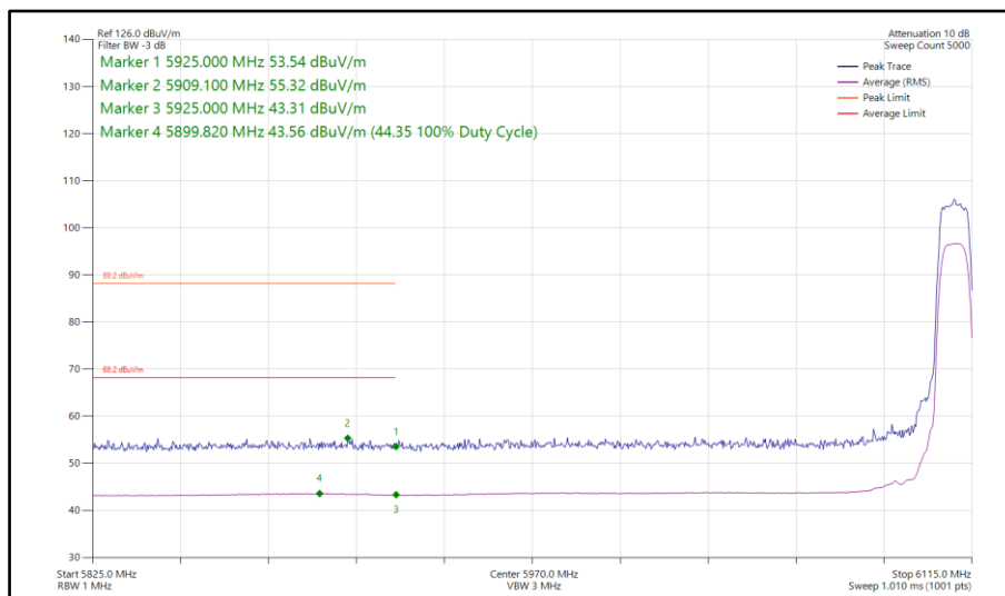
Figure 208 - Narrowband XHDRPL24, SISO, Core 1 - 6109 MHz Band Edge Frequency 5925 MHz
