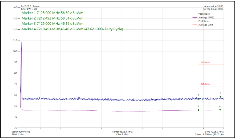
Figure 211 - Narrowband DH5, SISO, Core 1 - 6425 MHz Band Edge Frequency 7125 MHz
