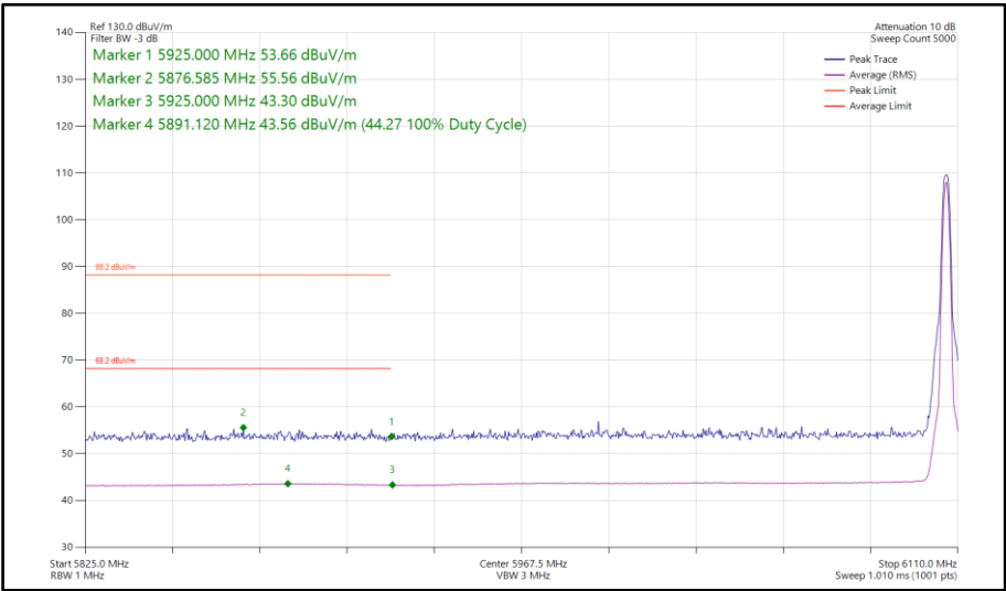
Figure 209 - Narrowband CS1LE1M, SISO, Core 1 - 6106 MHz Band Edge Frequency 5925 MHz
