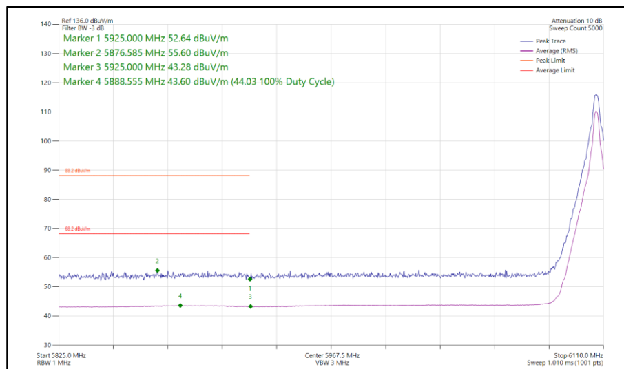
Figure 234 - Narrowband HDT6, MIMO, Core 0-1 - 6106 MHz Band Edge Frequency 5925 MHz
