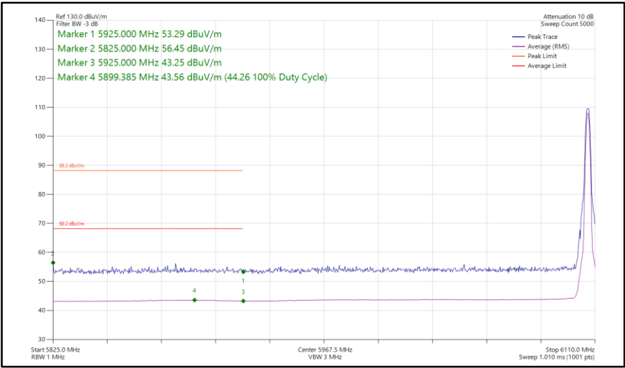
Figure 198 - Narrowband LE1M, SISO, Core 1 - 6106 MHz Band Edge Frequency 5925 MHz
