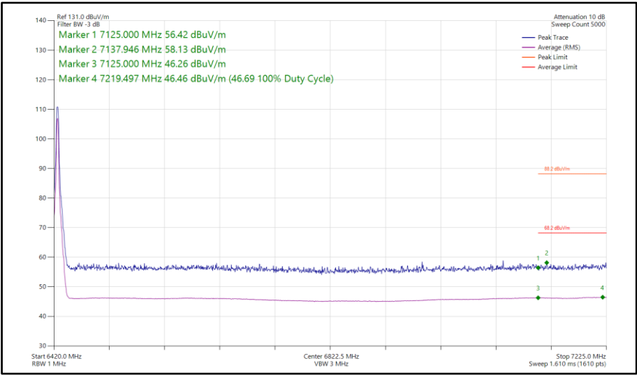
Figure 248 - Narrowband HDT3, MIMO, Core 0-1 - 6425 MHz Band Edge Frequency 7125 MHz
