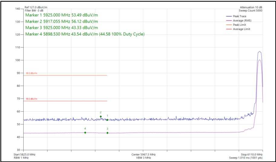
Figure 197 - Narrowband HDR8, SISO, Core 1 - 6106 MHz Band Edge Frequency 5925 MHz
