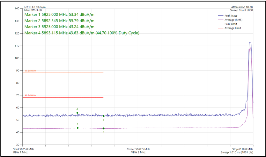
Figure 228 - Narrowband HDR4, MIMO, Core 0-1 - 6106 MHz Band Edge Frequency 5925 MHz
