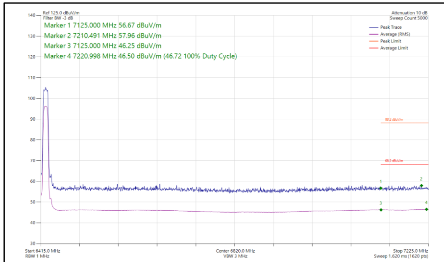
Figure 189 - Narrowband HDRPL8, SISO, Core 0 - 6425 MHz Band Edge Frequency 7125 MHz
