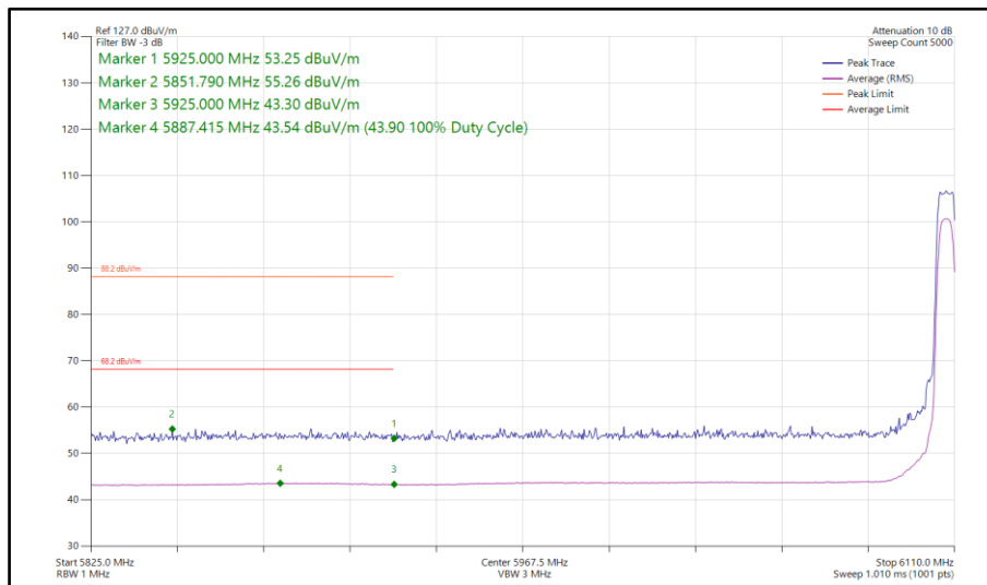
Figure 207 - Narrowband XHDRPM8, SISO, Core 1 - 6107 MHz Band Edge Frequency 5925 MHz
