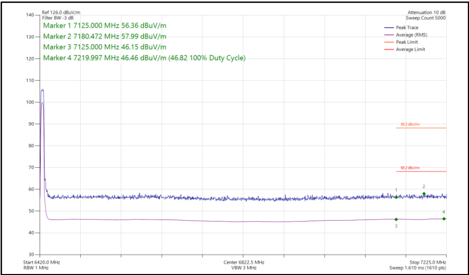
Figure 191 - Narrowband XHDRPM8, SISO, Core 0 - 6425 MHz Band Edge Frequency 7125 MHz
