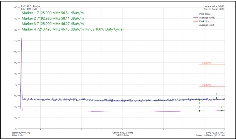
Figure 243 - Narrowband DH5, MIMO, Core 0-1 - 6425 MHz Band Edge Frequency 7125 MHz
