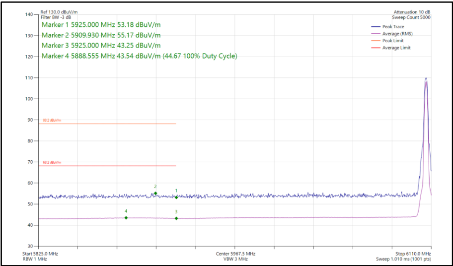
Figure 195 - Narrowband DH5, SISO, Core 1 - 6106 MHz Band Edge Frequency 5925 MHz
