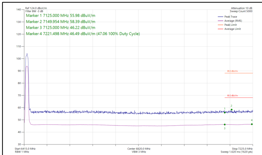
Figure 190 - Narrowband HDRPL24, SISO, Core 0 - 6425 MHz Band Edge Frequency 7125 MHz
