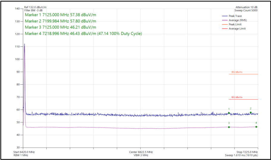
Figure 246 - Narrowband LE1M, MIMO, Core 0-1 - 6425 MHz Band Edge Frequency 7125 MHz
