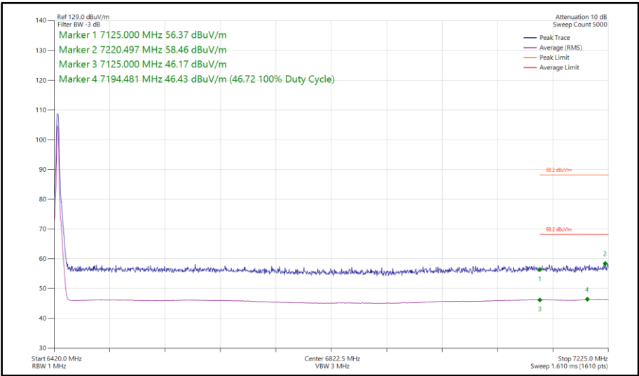
Figure 217 - Narrowband HDT4, SISO, Core 1 - 6425 MHz Band Edge Frequency 7125 MHz
