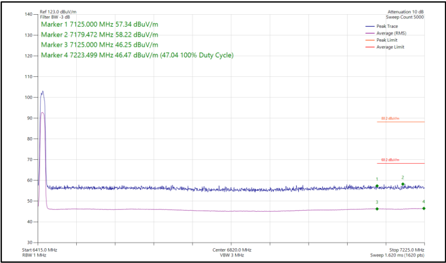
Figure 222 - Narrowband HDRPL24, SISO, Core 1 - 6425 MHz Band Edge Frequency 7125 MHz
