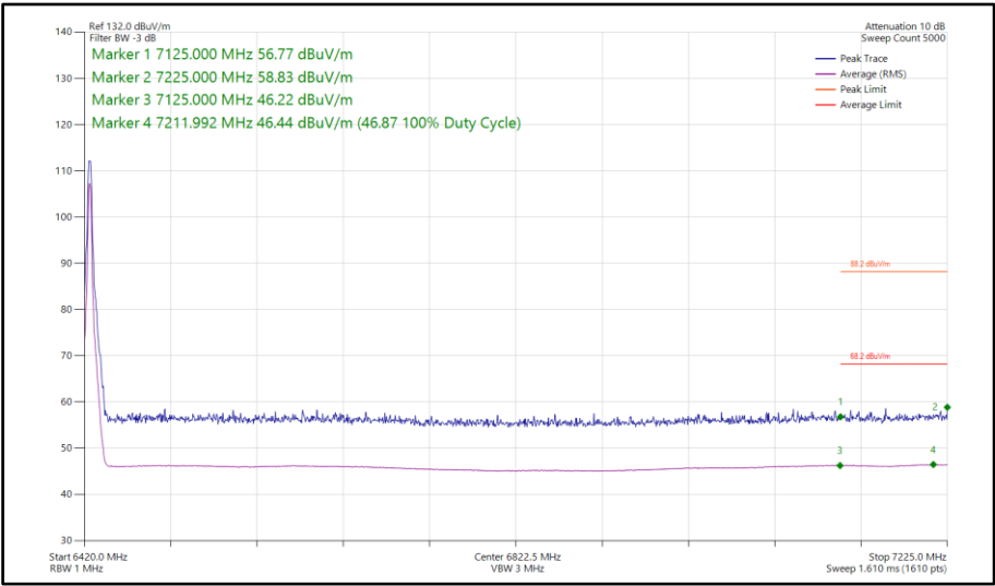
Figure 250 - Narrowband HDT6, MIMO, Core 0-1 - 6425 MHz Band Edge Frequency 7125 MHz
