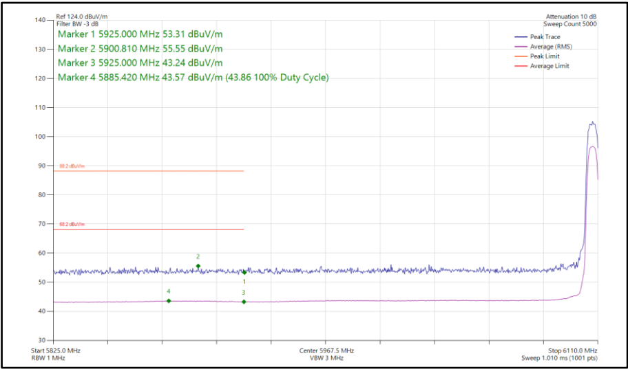
Figure 204 - Narrowband HDRPM12, SISO, Core 1 - 6107 MHz Band Edge Frequency 5925 MHz
