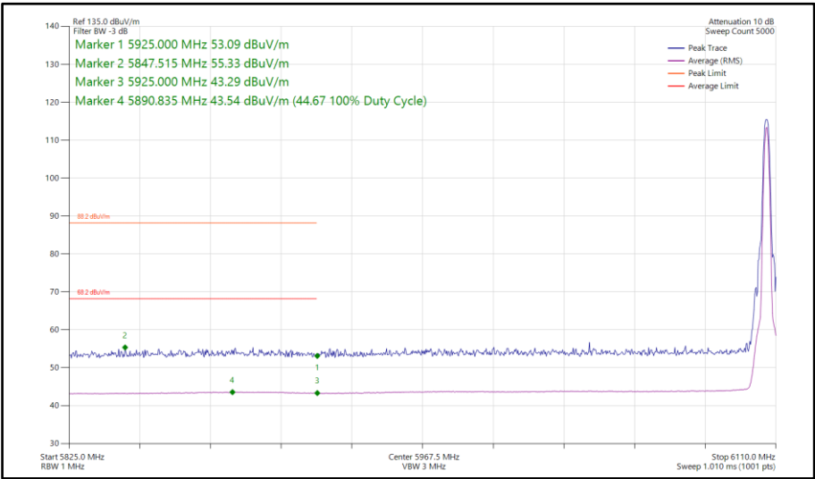
Figure 227 - Narrowband DH5, MIMO, Core 0-1 - 6106 MHz Band Edge Frequency 5925 MHz
