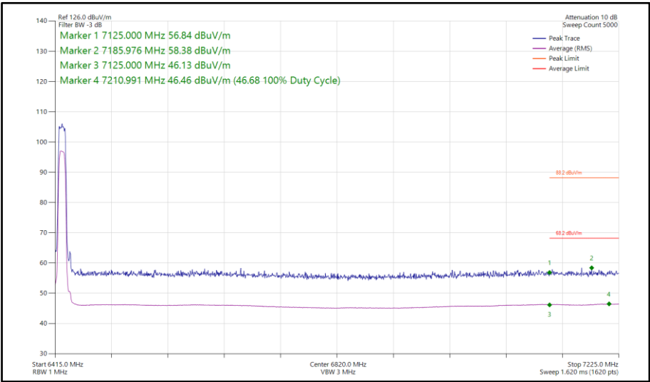
Figure 253 - Narrowband HDRPL8, MIMO, Core 0-1 - 6425 MHz Band Edge Frequency 7125 MHz
