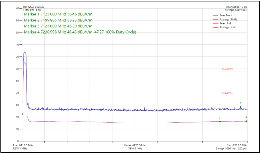
Figure 224 - Narrowband XHDRPL24, SISO, Core 1 - 6425 MHz Band Edge Frequency 7125 MHz
