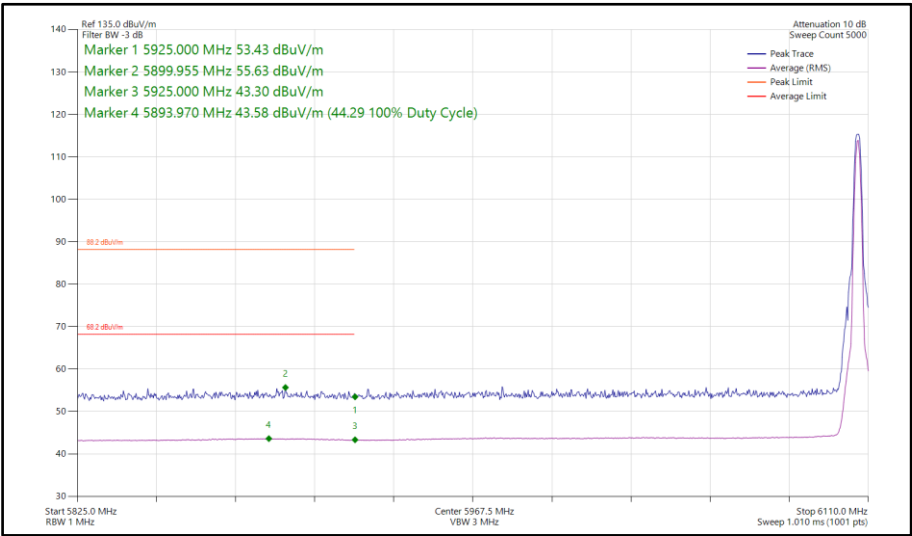
Figure 241 - Narrowband CS1LE1M, MIMO, Core 0-1 - 6106 MHz Band Edge Frequency 5925 MHz
