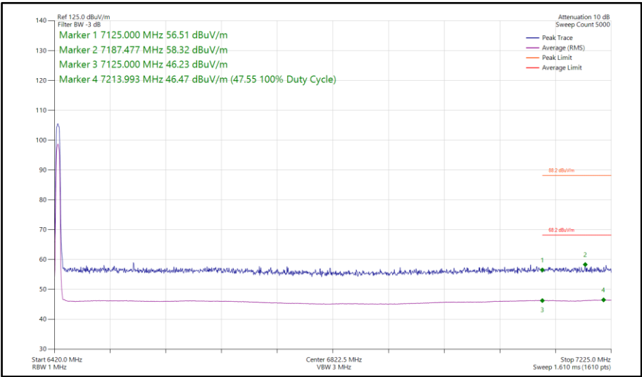
Figure 213 - Narrowband HDR8, SISO, Core 1 - 6425 MHz Band Edge Frequency 7125 MHz
