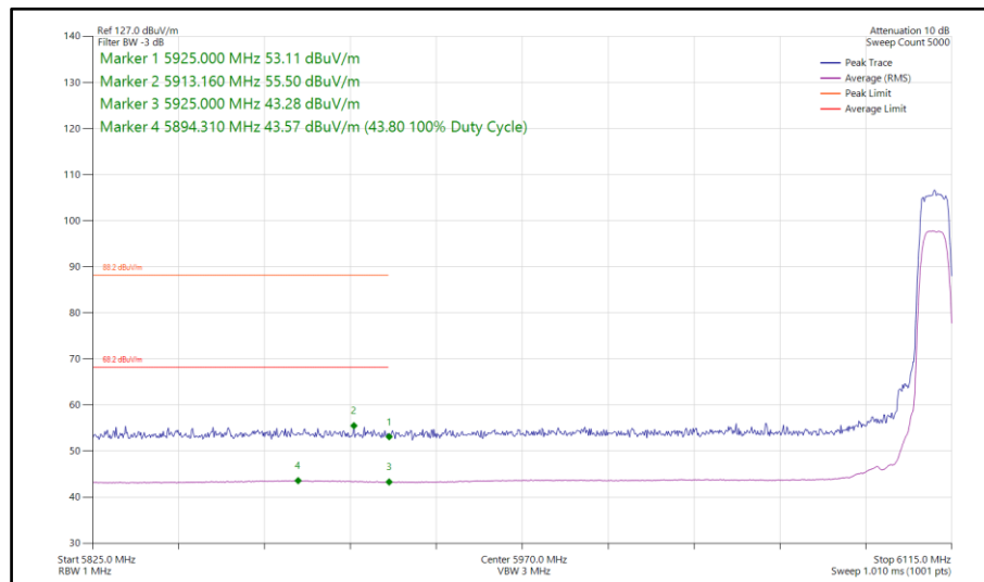
Figure 205 - Narrowband HDRPL8, SISO, Core 1 - 6109 MHz Band Edge Frequency 5925 MHz
