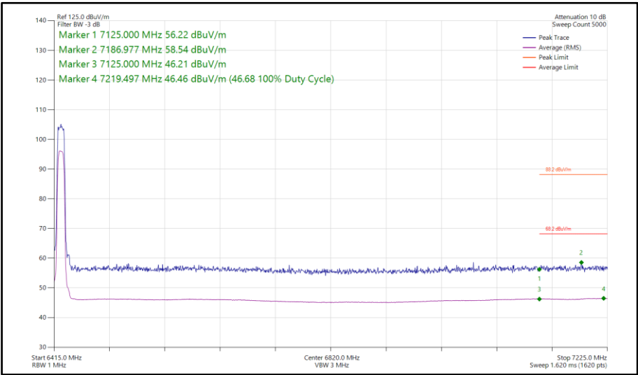
Figure 221 - Narrowband HDRPL8, SISO, Core 1 - 6425 MHz Band Edge Frequency 7125 MHz
