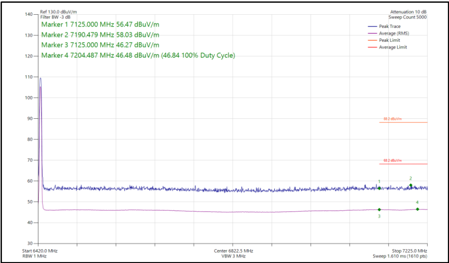
Figure 251 - Narrowband HDRPS2, MIMO, Core 0-1 - 6425 MHz Band Edge Frequency 7125 MHz
