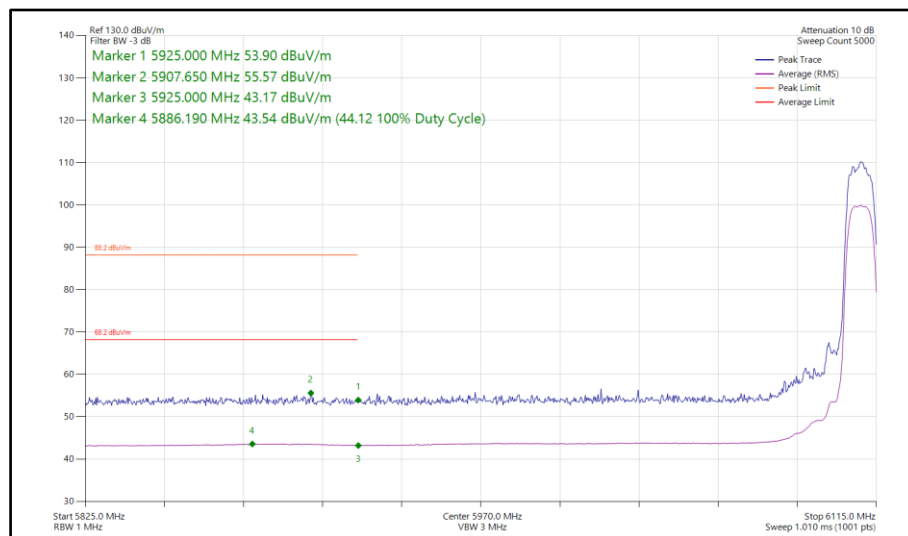
Figure 238 - Narrowband HDRPL24, MIMO, Core 0-1 - 6109 MHz Band Edge Frequency 5925 MHz
