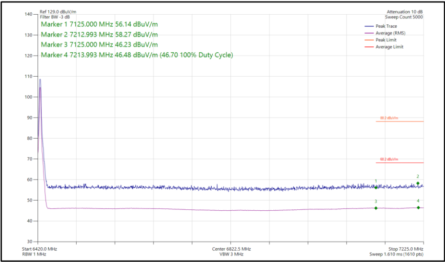
Figure 216 - Narrowband HDT3, SISO, Core 1 - 6425 MHz Band Edge Frequency 7125 MHz
