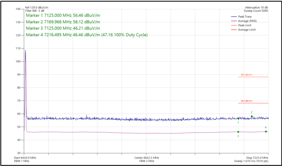
Figure 214 - Narrowband LE1M, SISO, Core 1 - 6425 MHz Band Edge Frequency 7125 MHz
