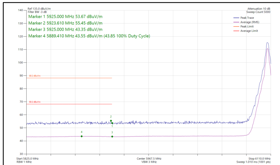
Figure 233 - Narrowband HDT4, MIMO, Core 0-1 - 6106 MHz Band Edge Frequency 5925 MHz
