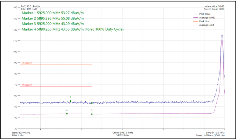
Figure 231 - Narrowband LE2M, MIMO, Core 0-1 - 6106 MHz Band Edge Frequency 5925 MHz
