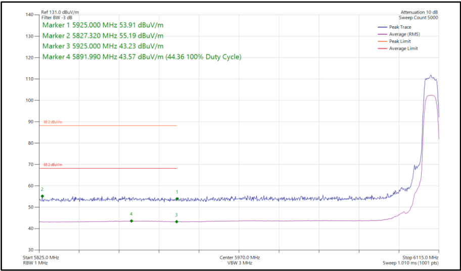
Figure 240 - Narrowband XHDRPL24, MIMO, Core 0-1 - 6109 MHz Band Edge Frequency 5925 MHz
