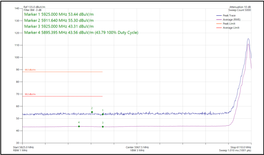
Figure 232 - Narrowband HDT3, MIMO, Core 0-1 - 6106 MHz Band Edge Frequency 5925 MHz
