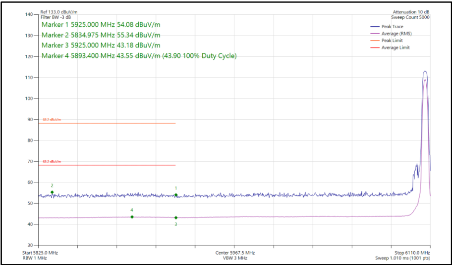
Figure 235 - Narrowband HDRPS2, MIMO, Core 0-1 - 6106 MHz Band Edge Frequency 5925 MHz
