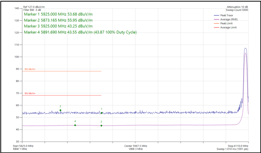
Figure 203 - Narrowband HDRPS2, SISO, Core 1 - 6106 MHz Band Edge Frequency 5925 MHz
