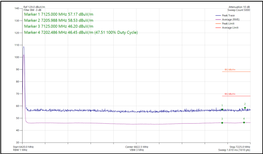
Figure 245 - Narrowband HDR8, MIMO, Core 0-1 - 6425 MHz Band Edge Frequency 7125 MHz
