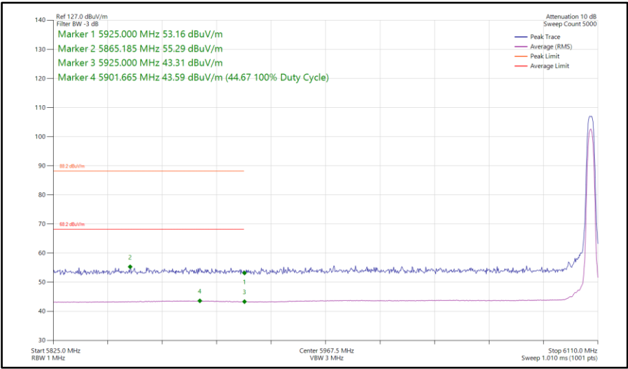
Figure 196 - Narrowband HDR4, SISO, Core 1 - 6106 MHz Band Edge Frequency 5925 MHz
