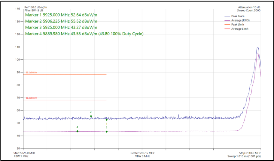
Figure 200 - Narrowband HDT3, SISO, Core 1 - 6106 MHz Band Edge Frequency 5925 MHz
