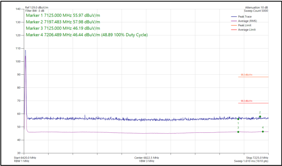
Figure 226 - Narrowband CS1LE2M, SISO, Core 1 - 6425 MHz Band Edge Frequency 7125 MHz
