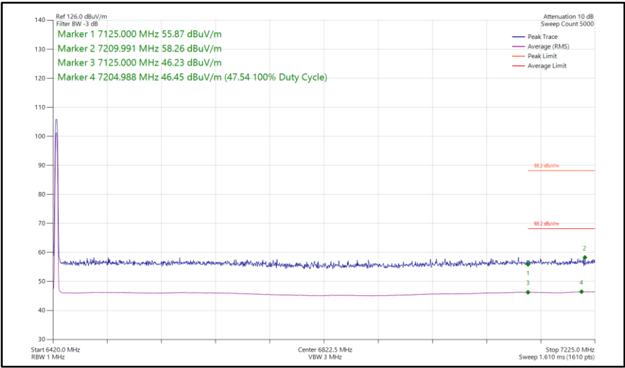
Figure 212 - Narrowband HDR4, SISO, Core 1 - 6425 MHz Band Edge Frequency 7125 MHz
