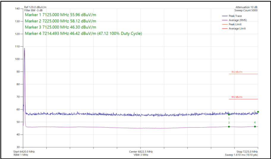
Figure 225 - Narrowband CS1LE1M, SISO, Core 1 - 6425 MHz Band Edge Frequency 7125 MHz
