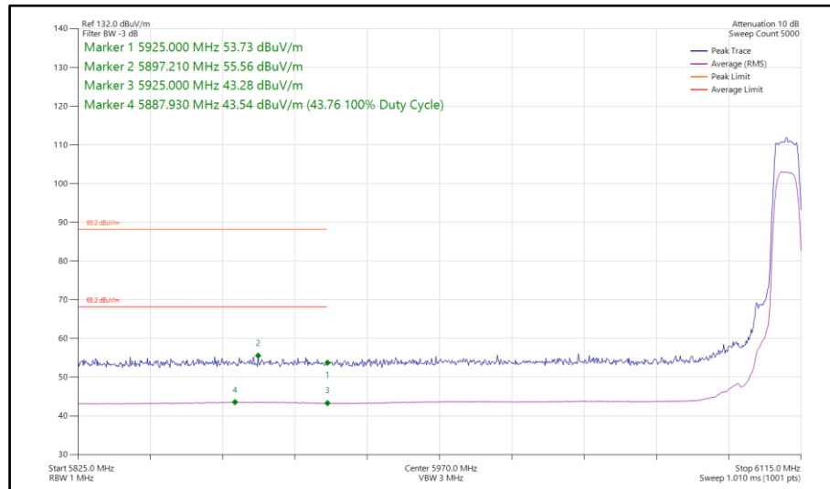
Figure 237 - Narrowband HDRPL8, MIMO, Core 0-1 - 6109 MHz Band Edge Frequency 5925 MHz
