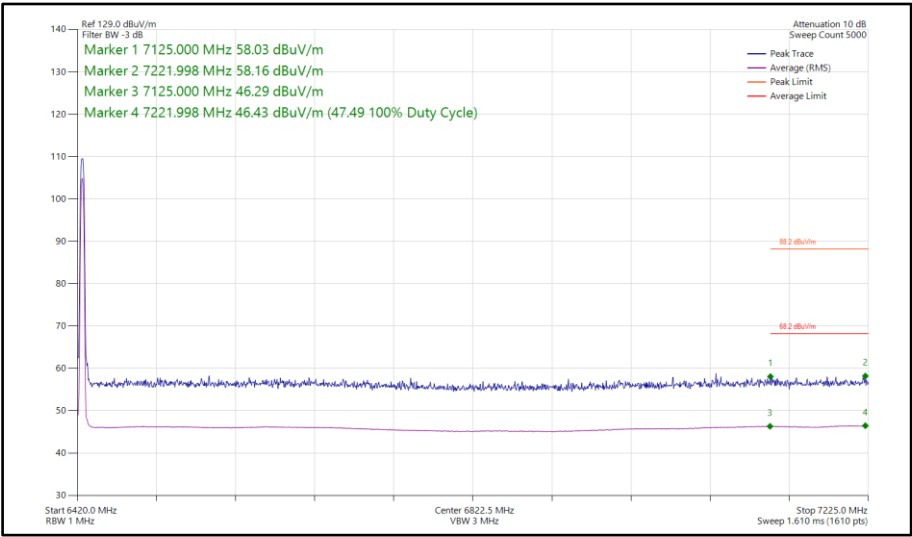
Figure 244 - Narrowband HDR4, MIMO, Core 0-1 - 6425 MHz Band Edge Frequency 7125 MHz
