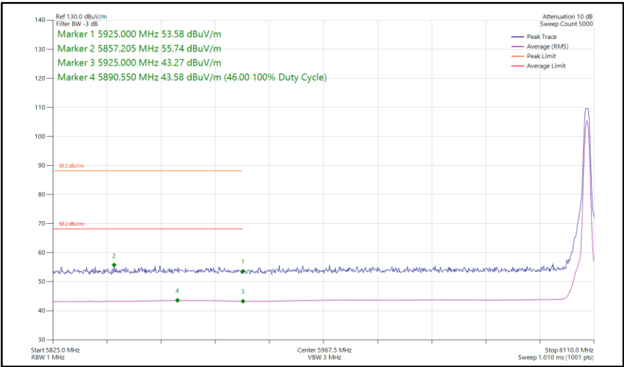
Figure 199 - Narrowband LE2M, SISO, Core 1 - 6106 MHz Band Edge Frequency 5925 MHz
