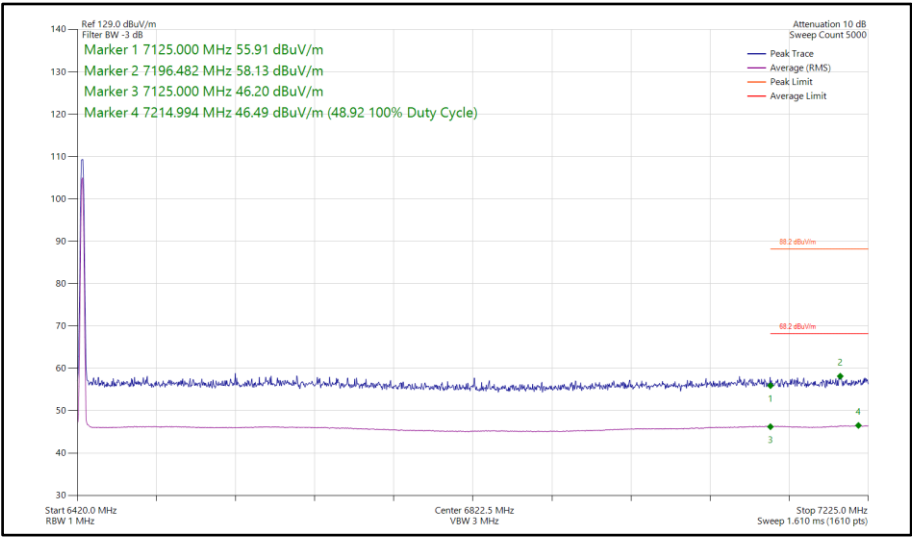
Figure 194 - Narrowband CS1LE2M, SISO, Core 0 - 6425 MHz Band Edge Frequency 7125 MHz
