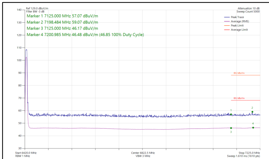
Figure 255 - Narrowband XHDRPM8, MIMO, Core 0-1 - 6425 MHz Band Edge Frequency 7125 MHz
