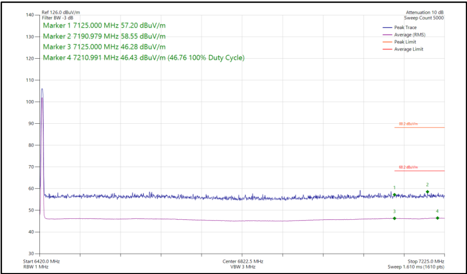
Figure 219 - Narrowband HDRPS2, SISO, Core 1 - 6425 MHz Band Edge Frequency 7125 MHz
