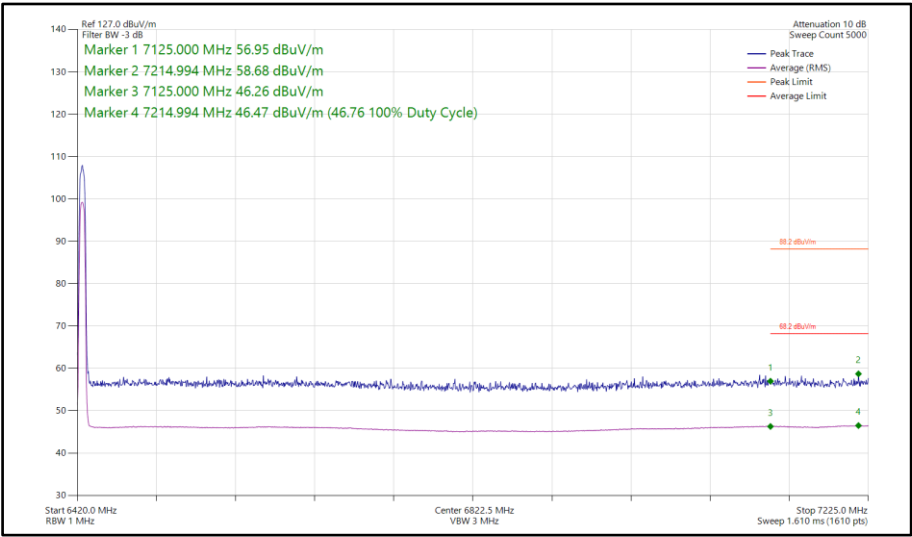
Figure 252 - Narrowband HDRPM12, MIMO, Core 0-1 - 6425 MHz Band Edge Frequency 7125 MHz
