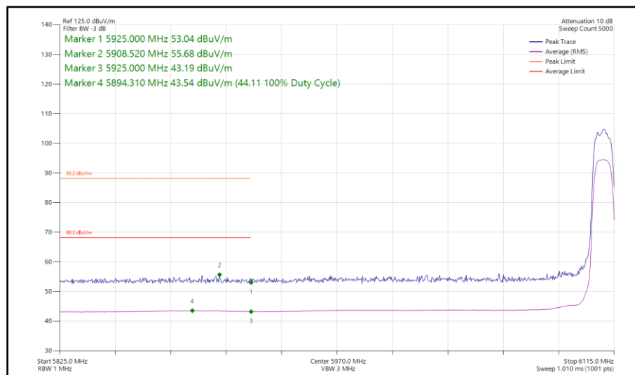
Figure 206 - Narrowband HDRPL24, SISO, Core 1 - 6109 MHz Band Edge Frequency 5925 MHz
