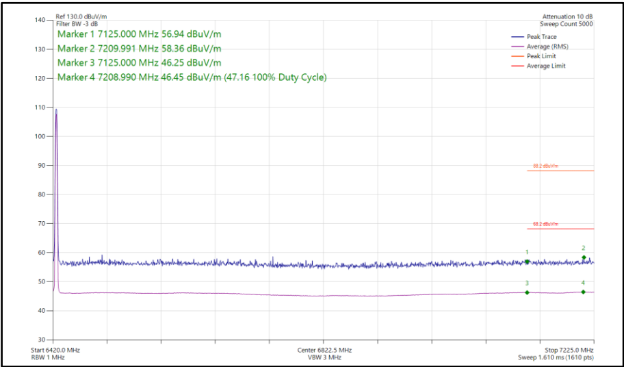
Figure 193 - Narrowband CS1LE1M, SISO, Core 0 - 6425 MHz Band Edge Frequency 7125 MHz
