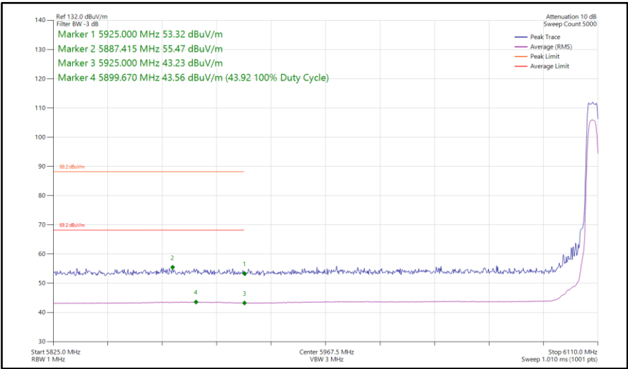
Figure 239 - Narrowband XHDRPM8, MIMO, Core 0-1 - 6107 MHz Band Edge Frequency 5925 MHz
