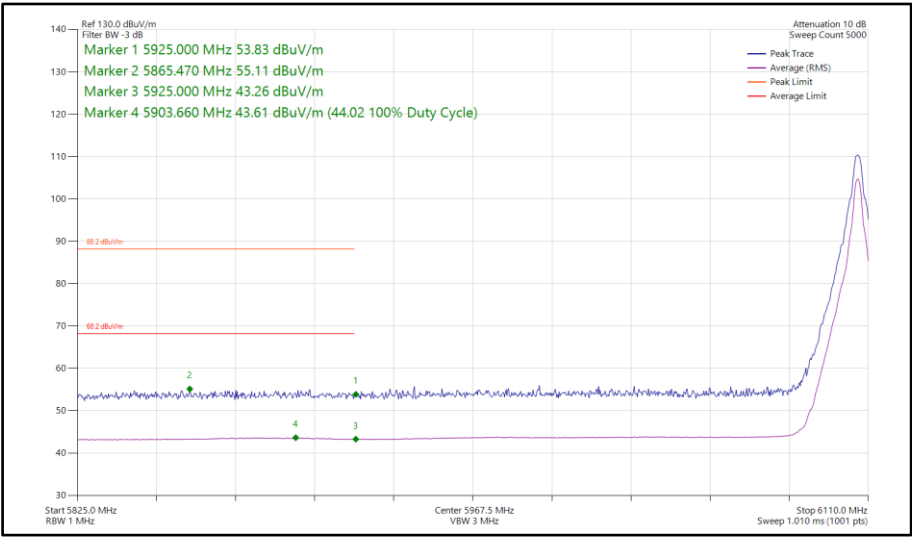
Figure 202 - Narrowband HDT6, SISO, Core 1 - 6106 MHz Band Edge Frequency 5925 MHz
