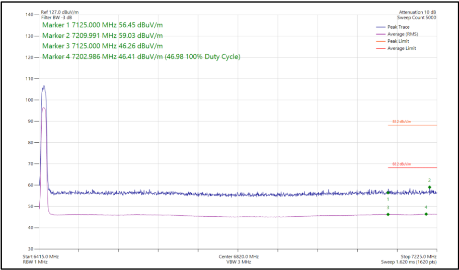
Figure 254 - Narrowband HDRPL24, MIMO, Core 0-1 - 6425 MHz Band Edge Frequency 7125 MHz
