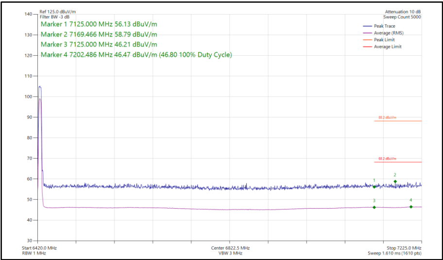
Figure 223 - Narrowband XHDRPM8, SISO, Core 1 - 6425 MHz Band Edge Frequency 7125 MHz
