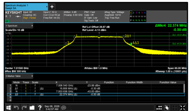
Figure 172 - 802.11a20 VLP Maximum 99% OBW
