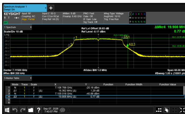
Figure 173 - 802.11a20 LPI Minimum 99% OBW
