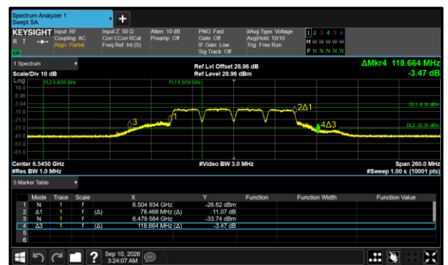
Figure 186 - 802.11a80 LPI Maximum 99% OBW
