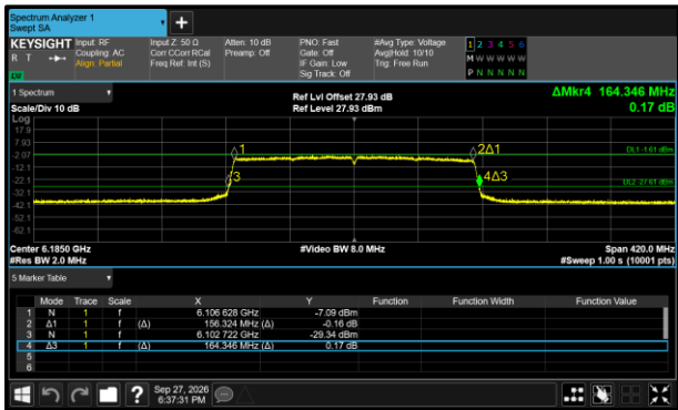
Figure 215 - 802.11ax HE160 SU VLP Minimum 26 dB EBW
