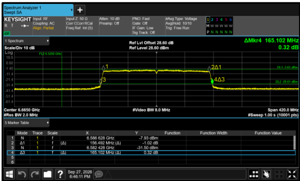
Figure 216 - 802.11ax HE160 SU VLP Maximum 26 dB EBW
