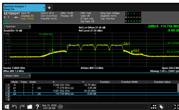
Figure 185 - 802.11a80 LPI Minimum 99% OBW
