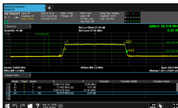
Figure 246 - 802.11ax HE80 SU LPI Maximum 26 dB EBW
