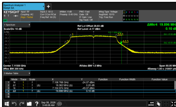
Figure 171 - 802.11a20 VLP Minimum 99% OBW
