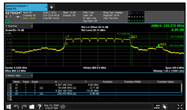
Figure 190 - 802.11a160 SP Maximum 99% OBW
