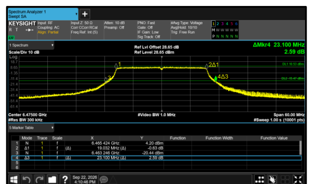
Figure 202 - 802.11ax HE20 SU SP Maximum 26 dB EBW
