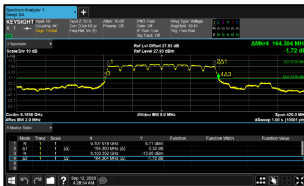
Figure 189 - 802.11a160 SP Minimum 99% OBW
