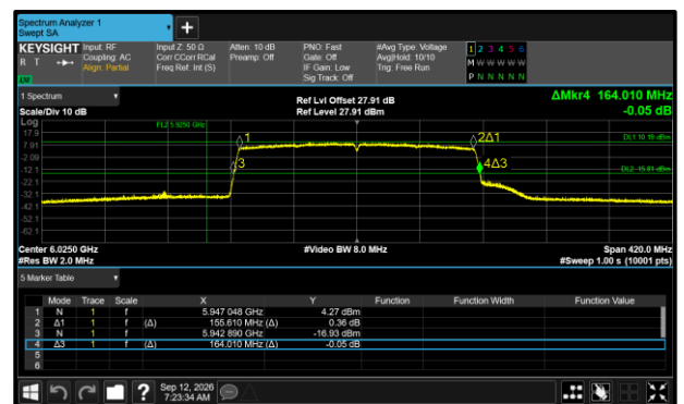
Figure 280 - 802.11ax HE160 SU SP Maximum 99% OBW
