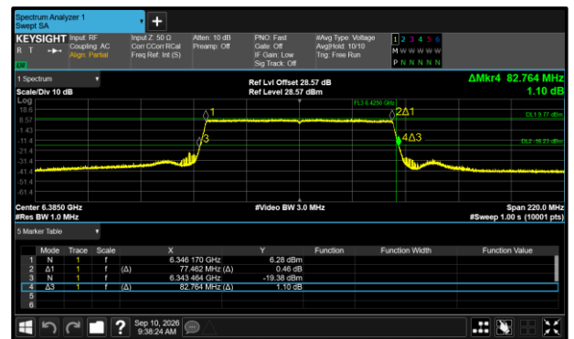
Figure 278 - 802.11ax HE80 SU SP Maximum 99% OBW
