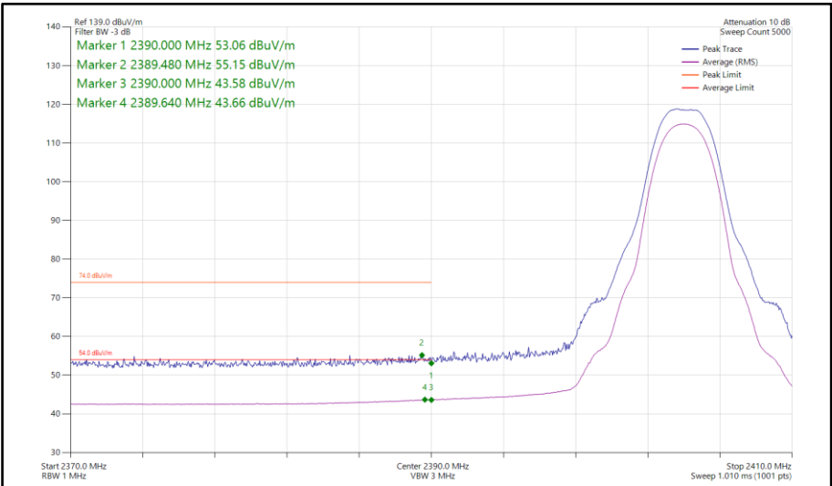
Figure 152 - Bluetooth HDT4, SISO, Core 1 - 2404 MHz Band Edge Frequency 2390 MHz
