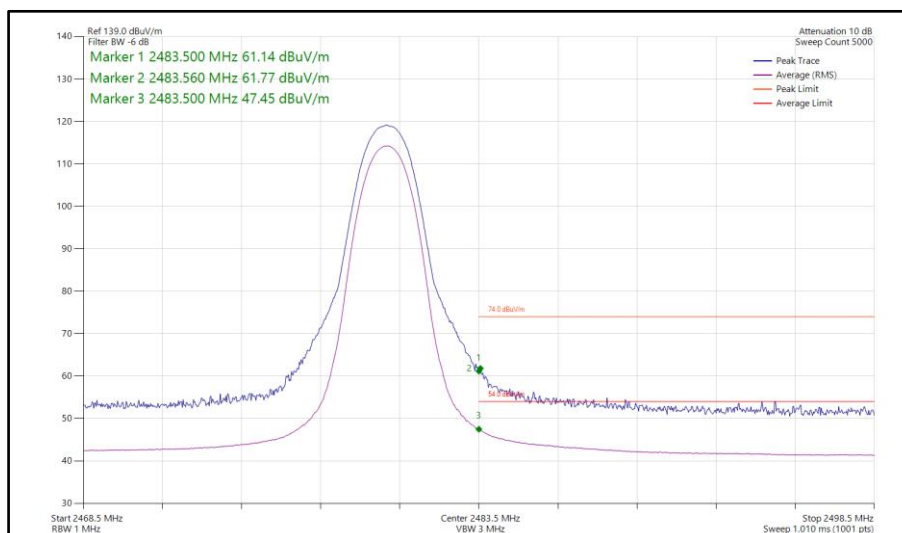
Figure 130 - Bluetooth 3DH5, SISO, Core 0 - 2480 MHz Band Edge Frequency 2483.5 MHz
