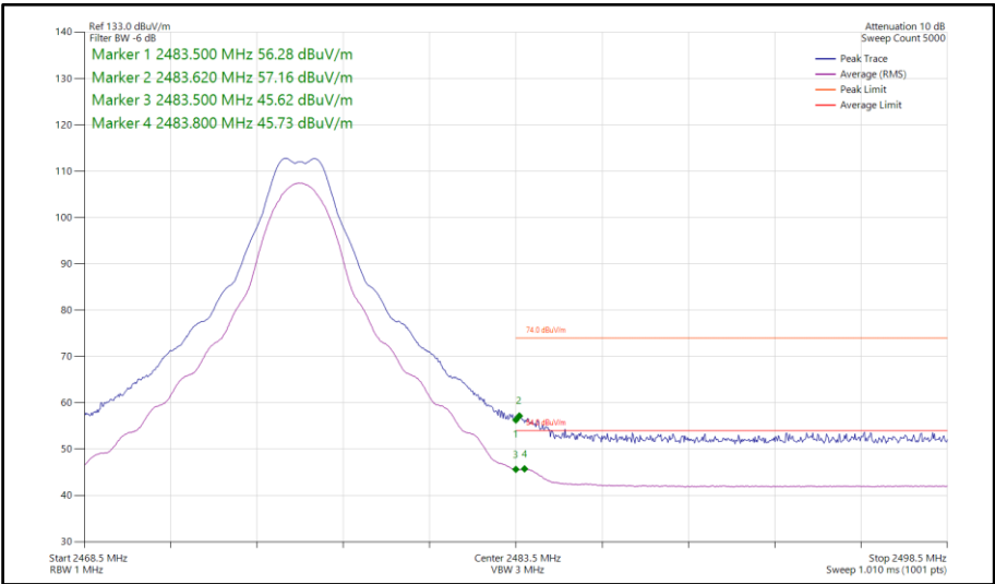
Figure 113 - Bluetooth CS1LE2M, MIMO, Core 0-1 - 2476 MHz Band Edge Frequency 2483.5 MHz
