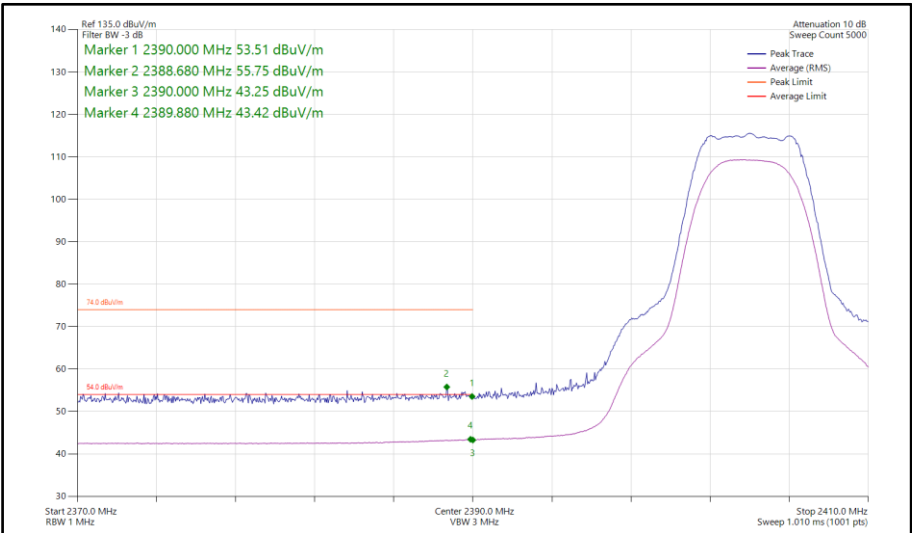
Figure 126 - Bluetooth XHDRPM8, SISO, Core 0 - 2404 MHz Band Edge Frequency 2390 MHz
