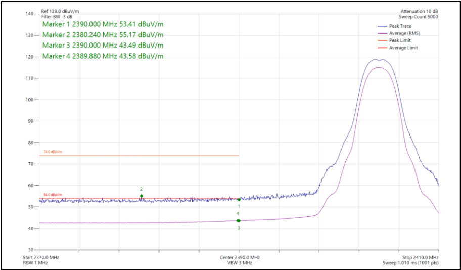
Figure 151 - Bluetooth HDT3, SISO, Core 1 - 2404 MHz Band Edge Frequency 2390 MHz
