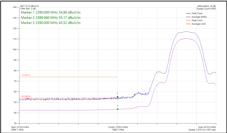
Figure 118 - Bluetooth HDR8, SISO, Core 0 - 2404 MHz Band Edge Frequency 2390 MHz
