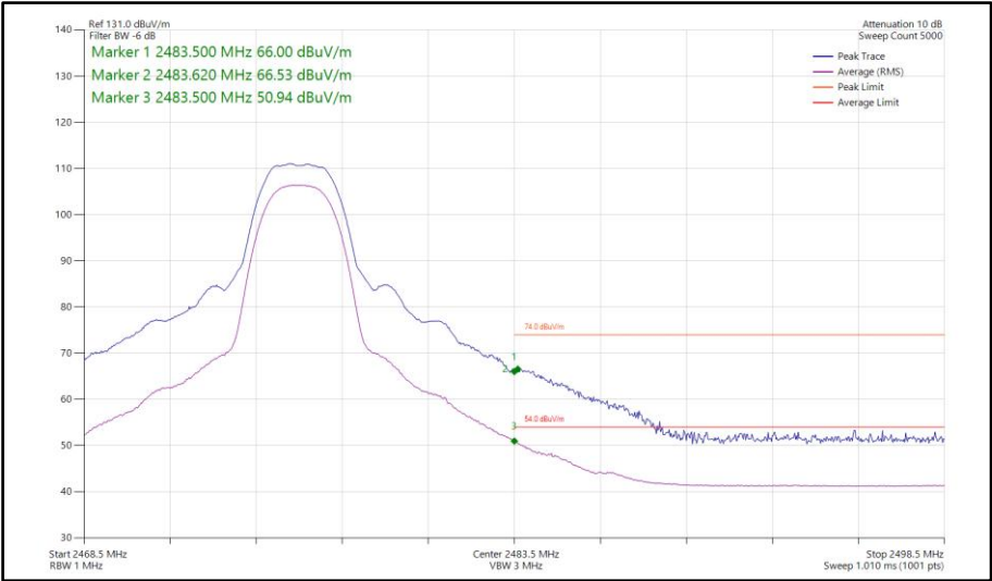
Figure 106 - Bluetooth HDT3, MIMO, Core 0-1 - 2476 MHz Band Edge Frequency 2483.5 MHz
