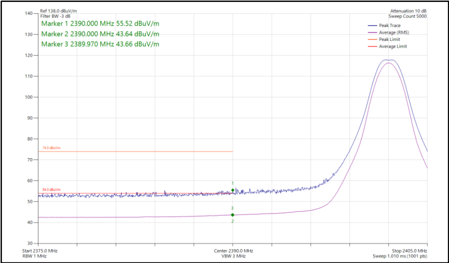
Figure 157 - Bluetooth CS1LE1M, SISO, Core 1 - 2402 MHz Band Edge Frequency 2390 MHz
