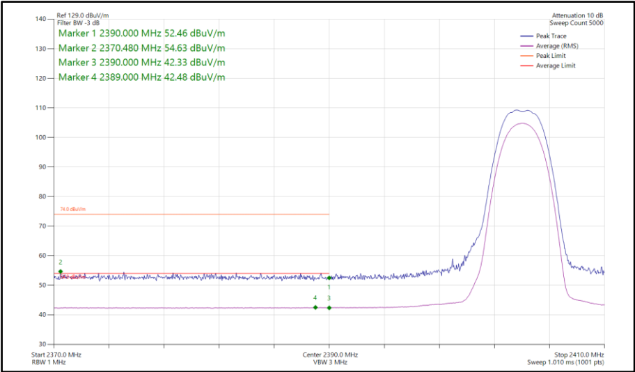
Figure 88 - Bluetooth HDR4, MIMO, Core 0-1 - 2404 MHz Band Edge Frequency 2390 MHz
