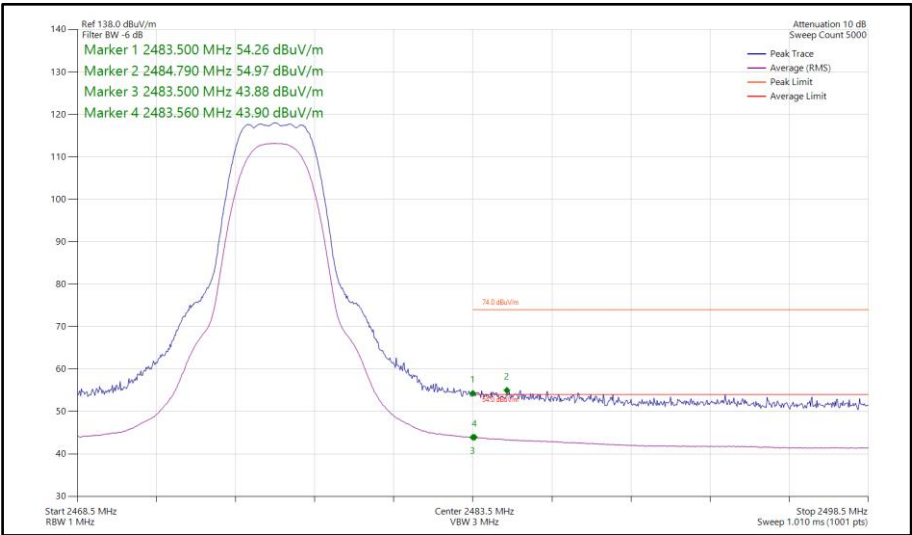
Figure 138 - Bluetooth HDRPS2, SISO, Core 0 - 2476 MHz Band Edge Frequency 2483.5 MHz
