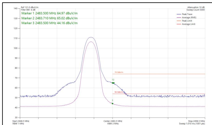
Figure 101 - Bluetooth 3DH5, MIMO, Core 0-1 - 2480 MHz Band Edge Frequency 2483.5 MHz
