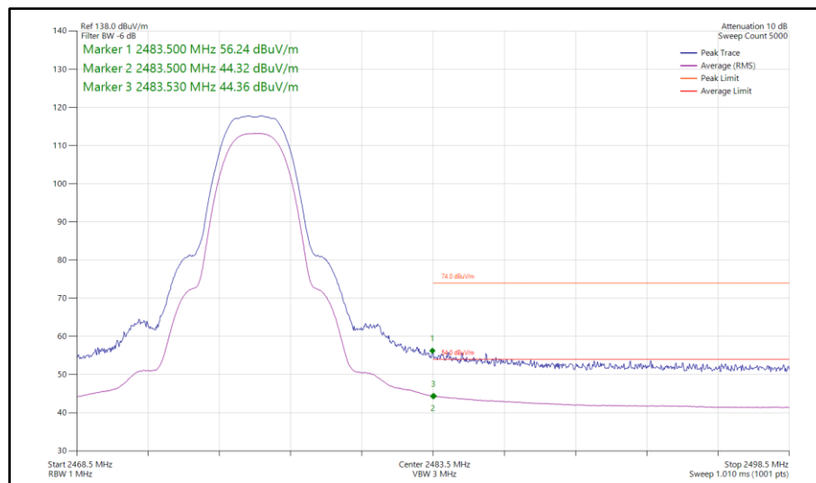
Figure 135 - Bluetooth HDT3, SISO, Core 0 - 2476 MHz Band Edge Frequency 2483.5 MHz
