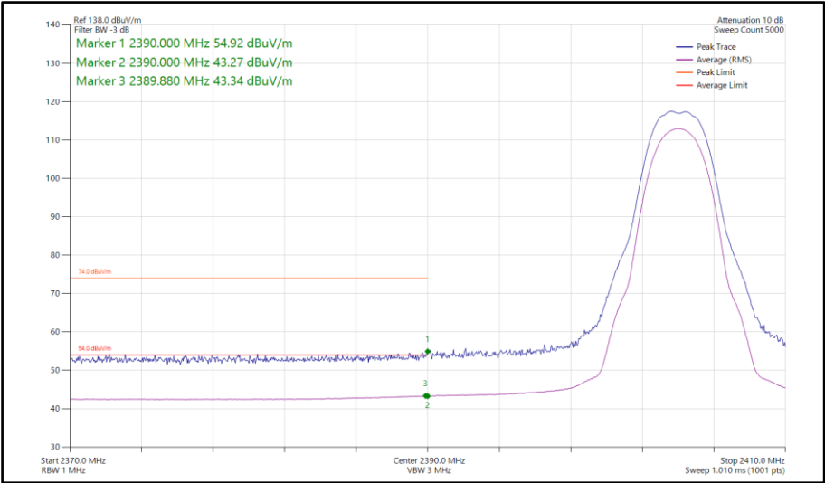
Figure 117 - Bluetooth HDR4, SISO, Core 0 - 2404 MHz Band Edge Frequency 2390 MHz
