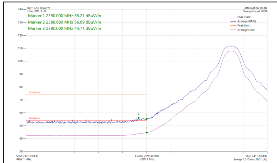
Figure 92 - Bluetooth HDT3, MIMO, Core 0-1 - 2404 MHz Band Edge Frequency 2390 MHz
