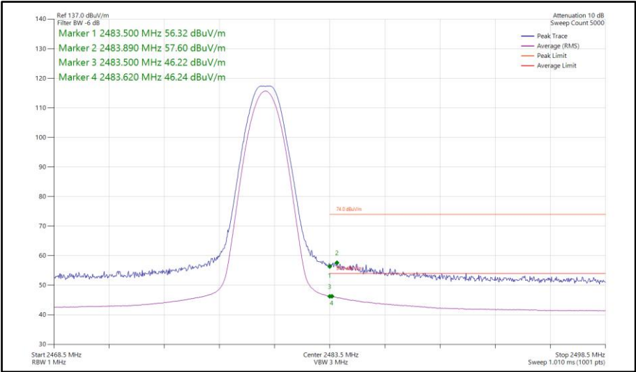
Figure 133 - Bluetooth LE1M, SISO, Core 0 - 2480 MHz Band Edge Frequency 2483.5 MHz
