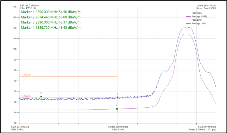
Figure 153 - Bluetooth HDT6, SISO, Core 1 - 2404 MHz Band Edge Frequency 2390 MHz
