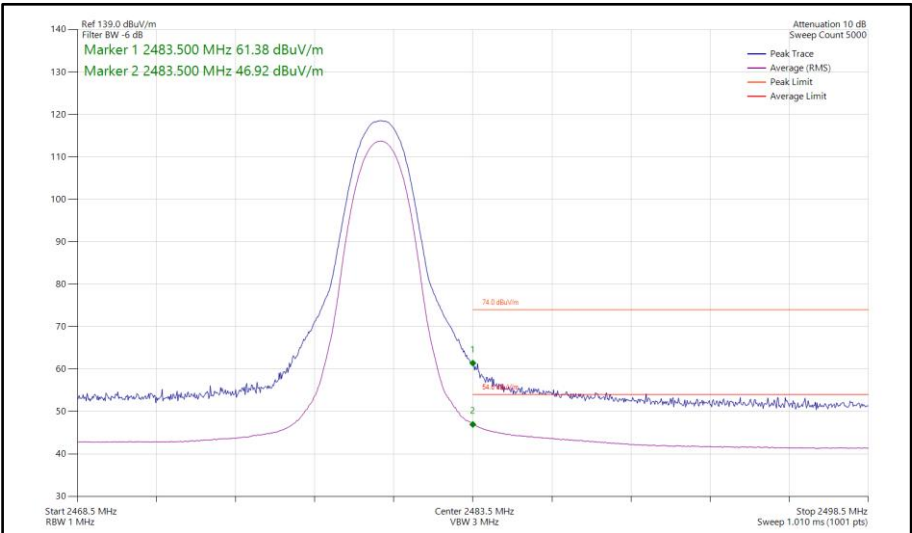
Figure 160 - Bluetooth 3DH5, SISO, Core 1 - 2480 MHz Band Edge Frequency 2483.5 MHz
