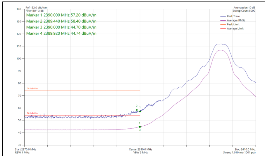
Figure 94 - Bluetooth HDT6, MIMO, Core 0-1 - 2404 MHz Band Edge Frequency 2390 MHz
