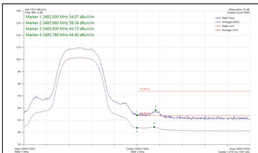
Figure 103 - Bluetooth HDR8, MIMO, Core 0-1 - 2476 MHz Band Edge Frequency 2483.5 MHz
