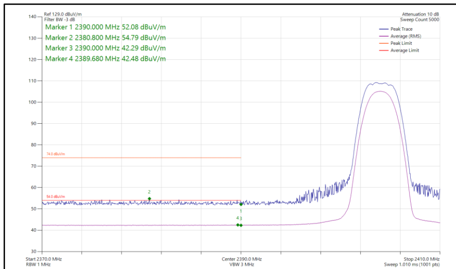
Figure 95 - Bluetooth HDRPS2, MIMO, Core 0-1 - 2404 MHz Band Edge Frequency 2390 MHz
