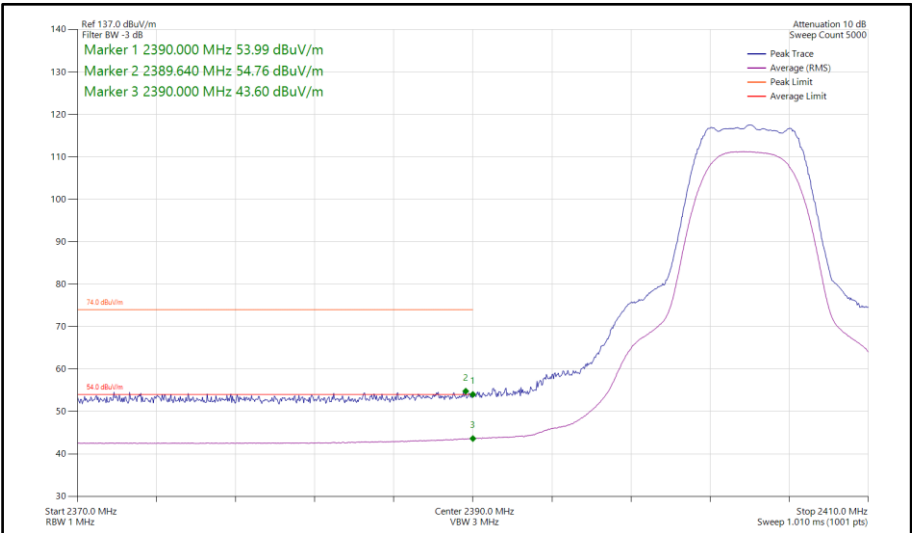
Figure 156 - Bluetooth XHDRPM8, SISO, Core 1 - 2404 MHz Band Edge Frequency 2390 MHz
