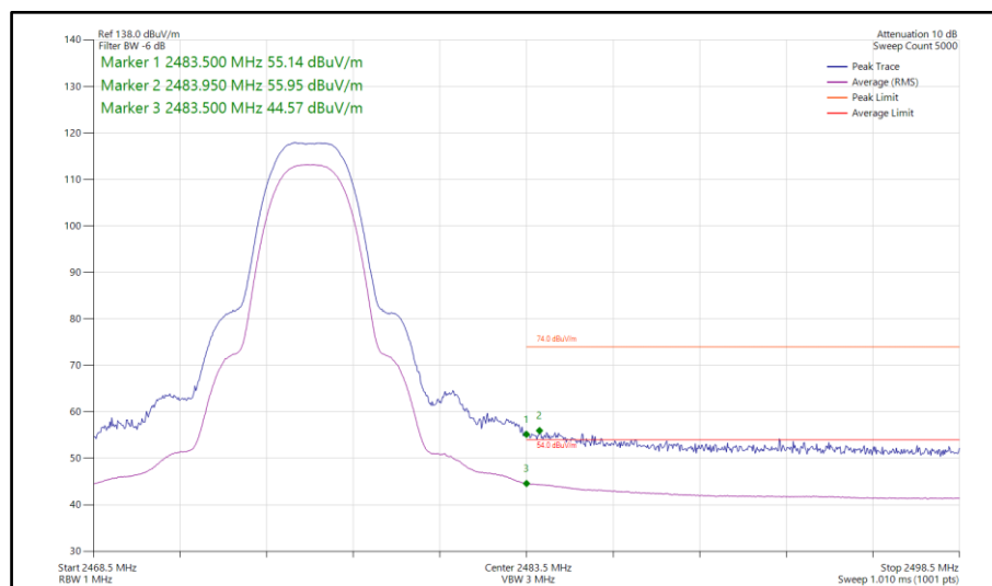
Figure 136 - Bluetooth HDT4, SISO, Core 0 - 2476 MHz Band Edge Frequency 2483.5 MHz
