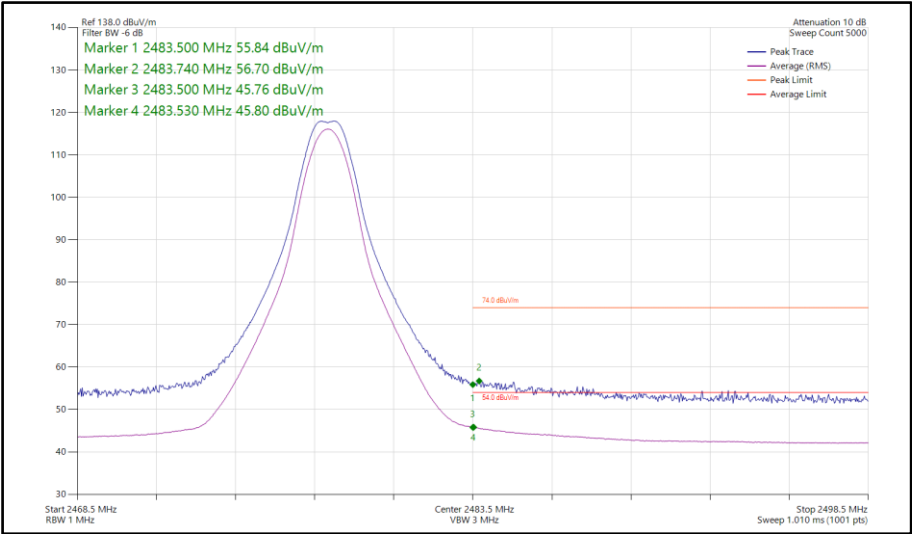
Figure 141 - Bluetooth CS1LE1M, SISO, Core 0 - 2478 MHz Band Edge Frequency 2483.5 MHz
