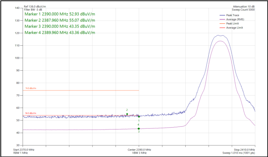
Figure 147 - Bluetooth HDR4, SISO, Core 1 - 2404 MHz Band Edge Frequency 2390 MHz
