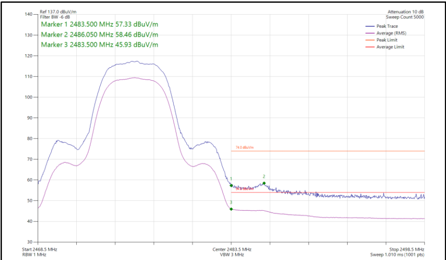
Figure 132 - Bluetooth HDR8, SISO, Core 0 - 2476 MHz Band Edge Frequency 2483.5 MHz
