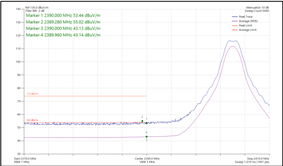
Figure 128 - Bluetooth CS1LE2M, SISO, Core 0 - 2404 MHz Band Edge Frequency 2390 MHz
