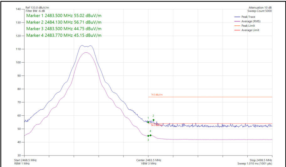
Figure 84 - Bluetooth CS1LE2M, SISO, Core 2 - 2476 MHz Band Edge Frequency 2483.5 MHz
