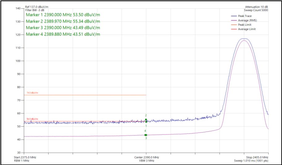
Figure 119 - Bluetooth LE1M, SISO, Core 0 - 2402 MHz Band Edge Frequency 2390 MHz
