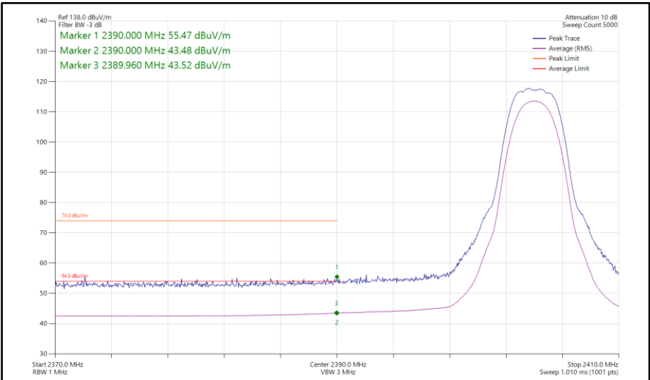
Figure 154 - Bluetooth HDRPS2, SISO, Core 1 - 2404 MHz Band Edge Frequency 2390 MHz
