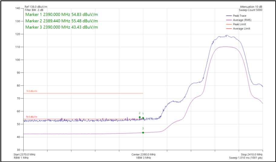
Figure 155 - Bluetooth HDRPM12, SISO, Core 1 - 2404 MHz Band Edge Frequency 2390 MHz
