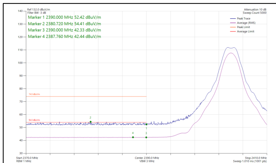
Figure 99 - Bluetooth CS1LE2M, MIMO, Core 0-1 - 2404 MHz Band Edge Frequency 2390 MHz
