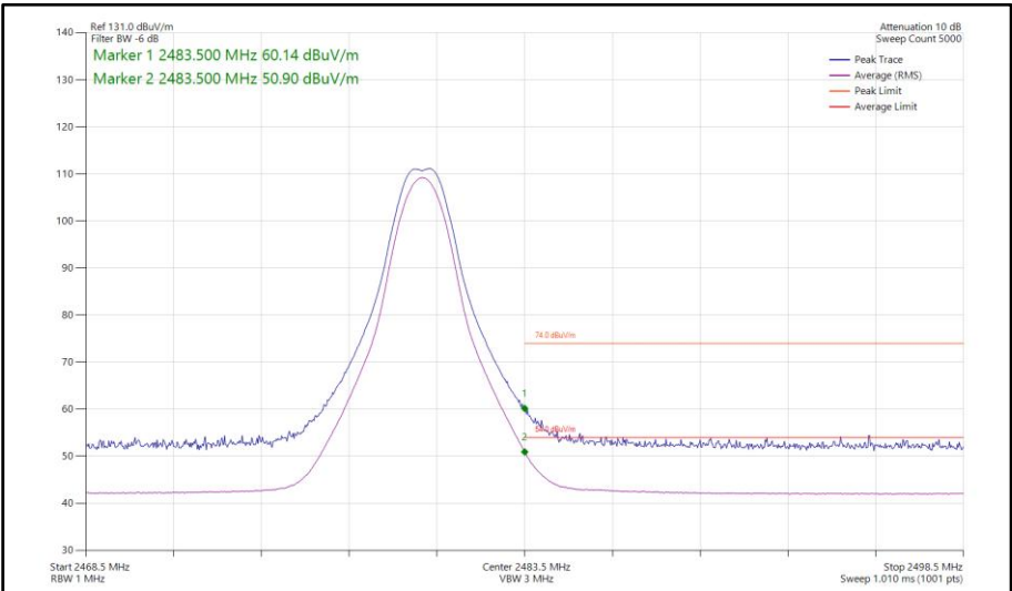
Figure 142 - Bluetooth CS1LE1M, SISO, Core 0 - 2480 MHz Band Edge Frequency 2483.5 MHz
