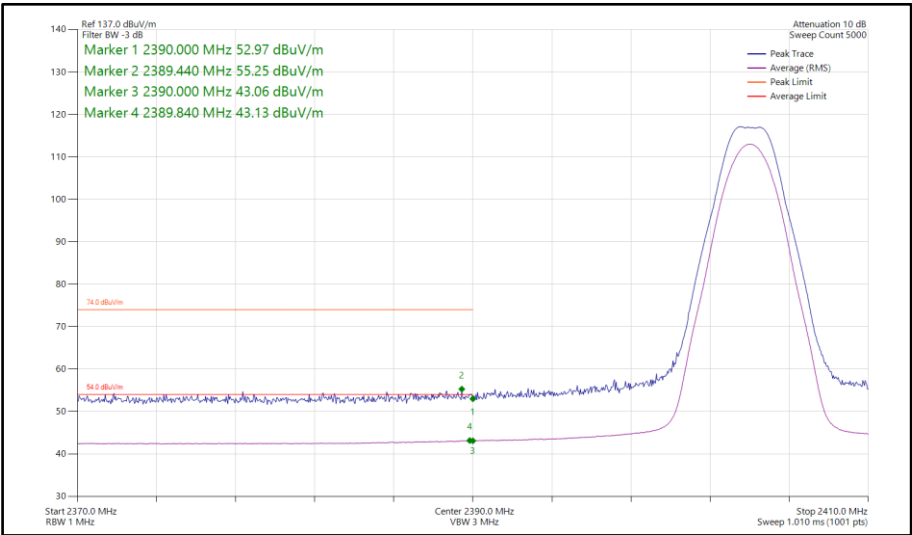
Figure 120 - Bluetooth LE2M, SISO, Core 0 - 2404 MHz Band Edge Frequency 2390 MHz
