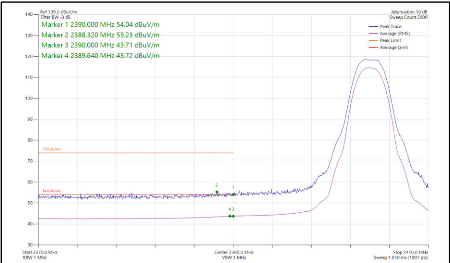
Figure 122 - Bluetooth HDT4, SISO, Core 0 - 2404 MHz Band Edge Frequency 2390 MHz
