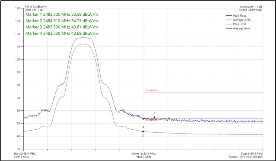
Figure 131 - Bluetooth HDR4, SISO, Core 0 - 2476 MHz Band Edge Frequency 2483.5 MHz
