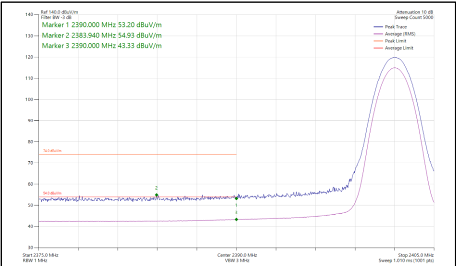
Figure 146 - Bluetooth 3DH5, SISO, Core 1 - 2402 MHz Band Edge Frequency 2390 MHz
