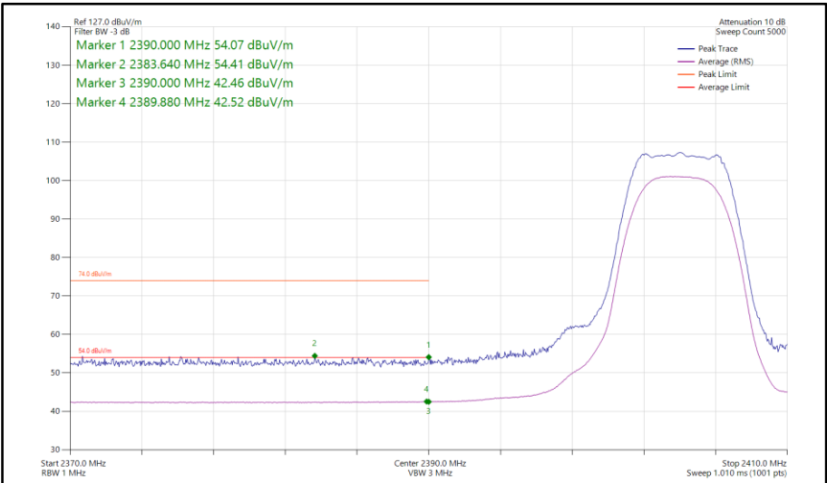
Figure 97 - Bluetooth XHDRPM8, MIMO, Core 0-1 - 2404 MHz Band Edge Frequency 2390 MHz
