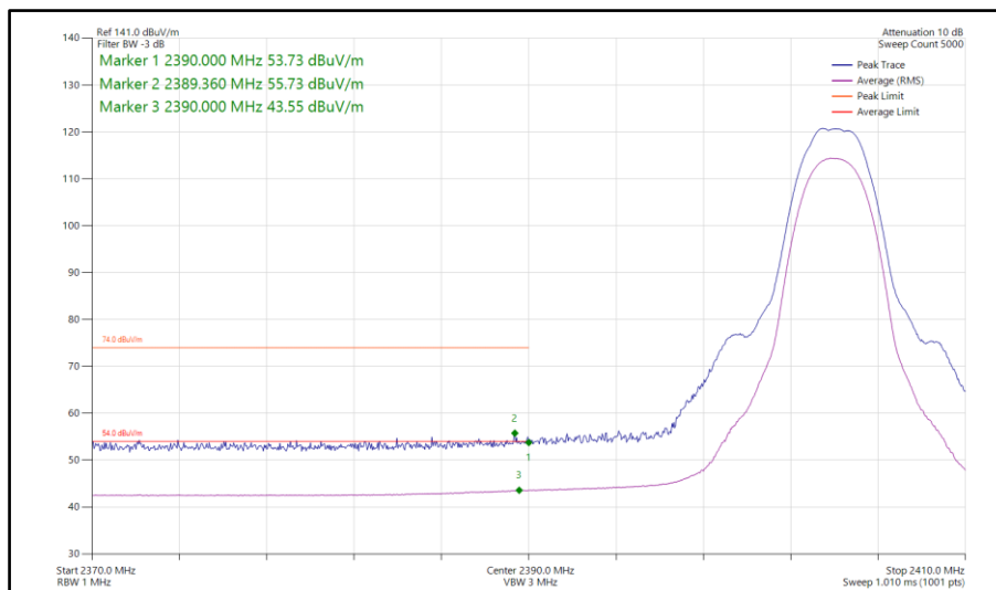
Figure 123 - Bluetooth HDT6, SISO, Core 0 - 2404 MHz Band Edge Frequency 2390 MHz
