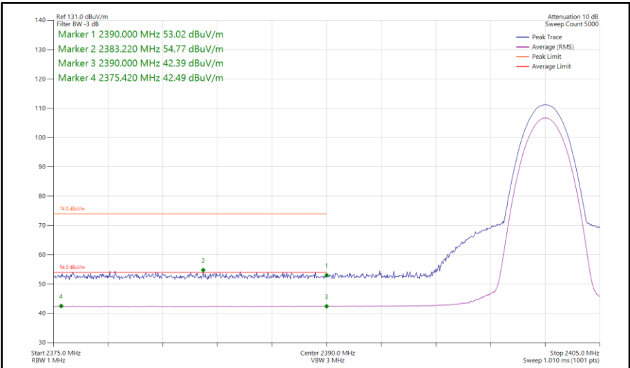
Figure 87 - Bluetooth 3DH5, MIMO, Core 0-1 - 2402 MHz Band Edge Frequency 2390 MHz
