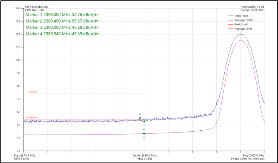
Figure 145 - Bluetooth 2DH5, SISO, Core 1 - 2402 MHz Band Edge Frequency 2390 MHz
