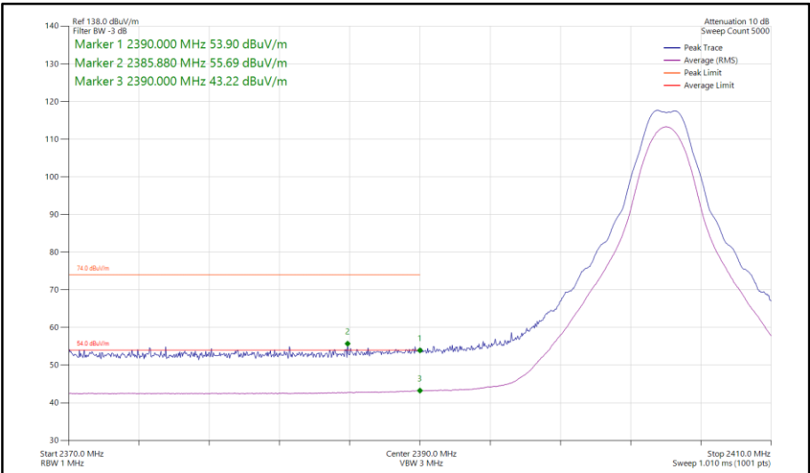
Figure 158 - Bluetooth CS1LE2M, SISO, Core 1 - 2404 MHz Band Edge Frequency 2390 MHz
