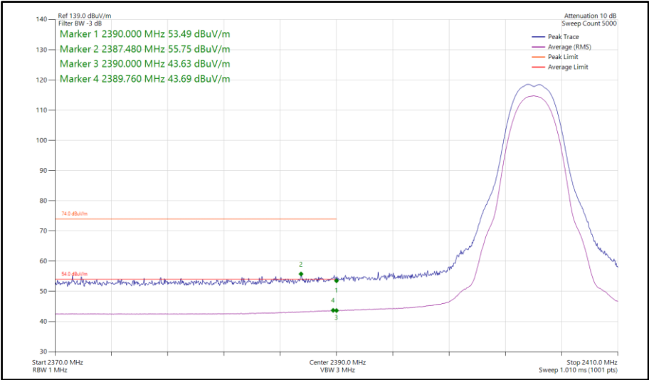
Figure 121 - Bluetooth HDT3, SISO, Core 0 - 2404 MHz Band Edge Frequency 2390 MHz
