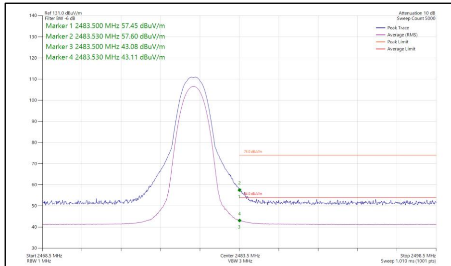
Figure 100 - Bluetooth 2DH5, MIMO, Core 0-1 - 2480 MHz Band Edge Frequency 2483.5 MHz
