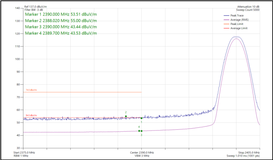
Figure 149 - Bluetooth LE1M, SISO, Core 1 - 2402 MHz Band Edge Frequency 2390 MHz
