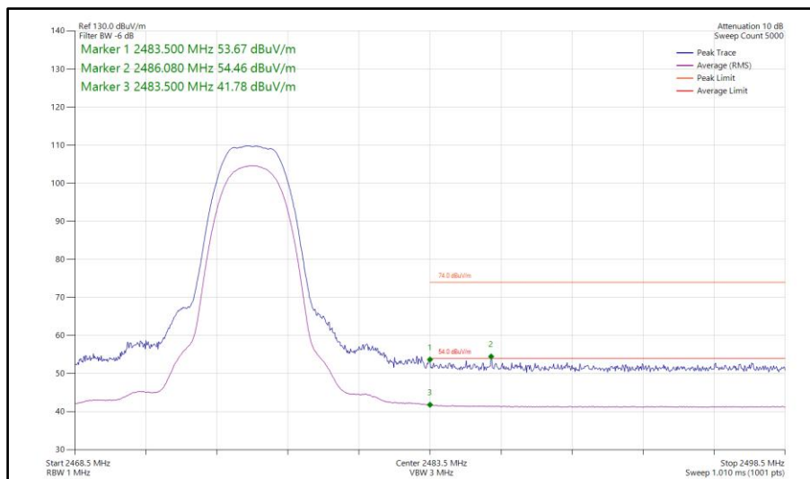
Figure 102 - Bluetooth HDR4, MIMO, Core 0-1 - 2476 MHz Band Edge Frequency 2483.5 MHz
