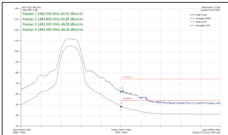
Figure 108 - Bluetooth HDT6, MIMO, Core 0-1 - 2476 MHz Band Edge Frequency 2483.5 MHz
