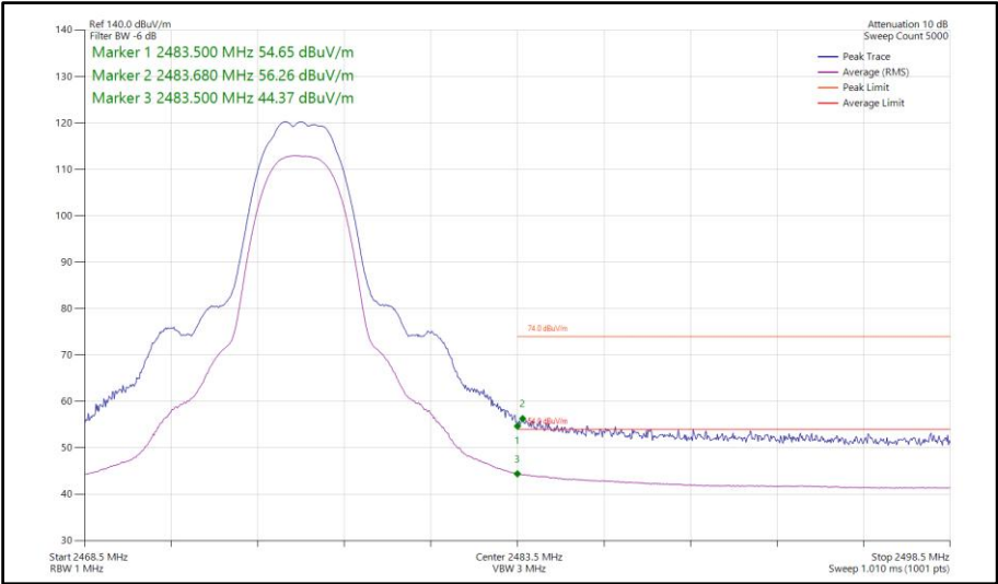
Figure 137 - Bluetooth HDT6, SISO, Core 0 - 2476 MHz Band Edge Frequency 2483.5 MHz
