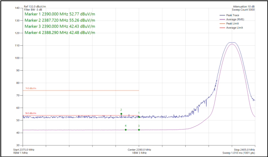
Figure 90 - Bluetooth LE1M, MIMO, Core 0-1 - 2402 MHz Band Edge Frequency 2390 MHz
