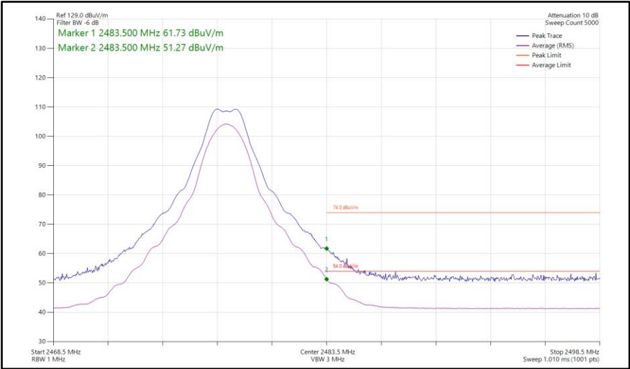
Figure 85 - Bluetooth CS1LE2M, SISO, Core 2 - 2478 MHz Band Edge Frequency 2483.5 MHz
