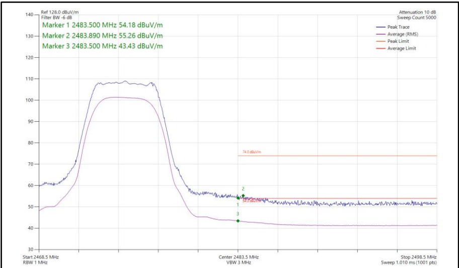
Figure 111 - Bluetooth XHDRPM8, MIMO, Core 0-1 - 2475 MHz Band Edge Frequency 2483.5 MHz
