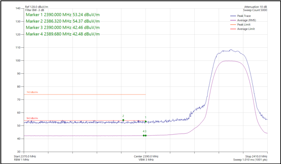
Figure 96 - Bluetooth HDRPM12, MIMO, Core 0-1 - 2404 MHz Band Edge Frequency 2390 MHz
