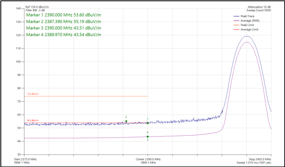
Figure 115 - Bluetooth 2DH5, SISO, Core 0 - 2402 MHz Band Edge Frequency 2390 MHz
