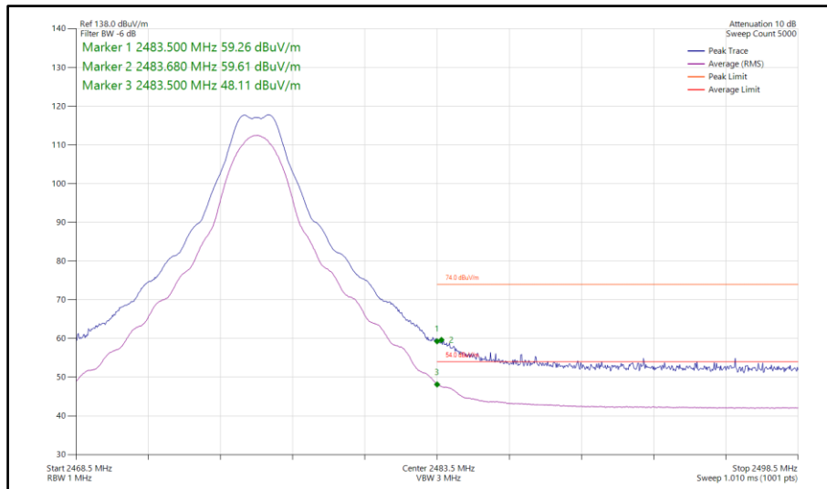
Figure 143 - Bluetooth CS1LE2M, SISO, Core 0 - 2476 MHz Band Edge Frequency 2483.5 MHz
