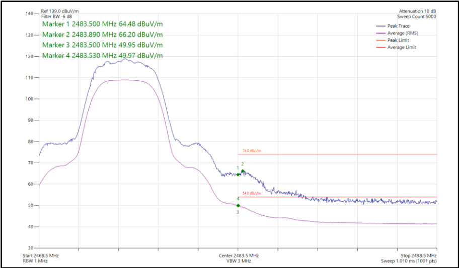
Figure 139 - Bluetooth HDRPM12, SISO, Core 0 - 2475 MHz Band Edge Frequency 2483.5 MHz
