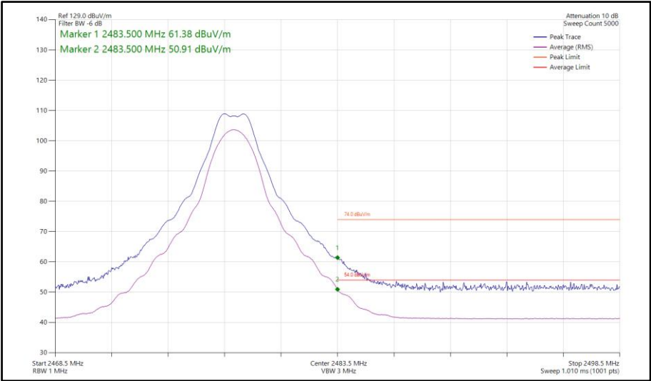
Figure 114 - Bluetooth CS1LE2M, MIMO, Core 0-1 - 2478 MHz Band Edge Frequency 2483.5 MHz
