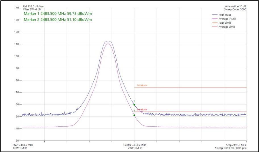
Figure 112 - Bluetooth CS1LE1M, MIMO, Core 0-1 - 2480 MHz Band Edge Frequency 2483.5 MHz
