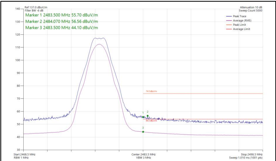
Figure 134 - Bluetooth LE2M, SISO, Core 0 - 2478 MHz Band Edge Frequency 2483.5 MHz
