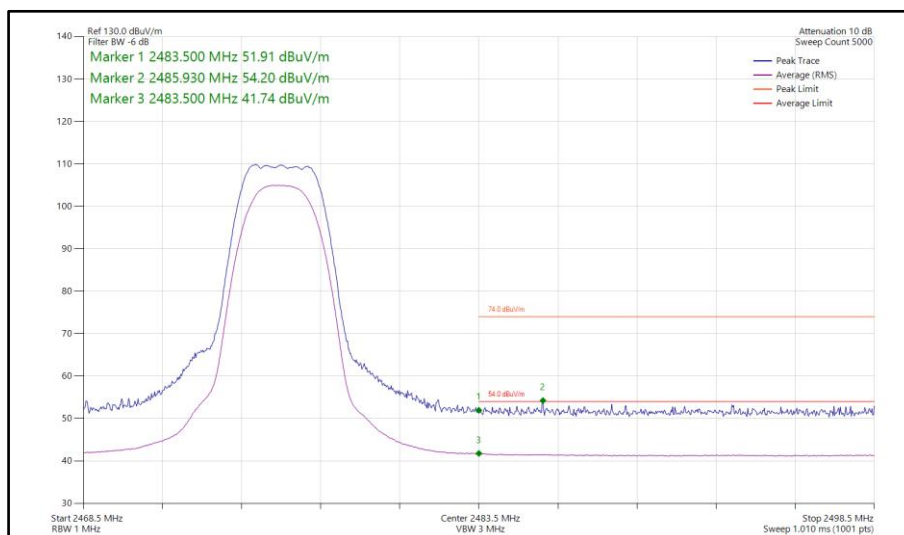
Figure 109 - Bluetooth HDRPS2, MIMO, Core 0-1 - 2476 MHz Band Edge Frequency 2483.5 MHz
