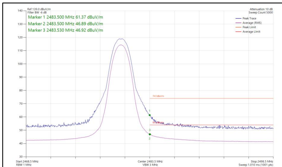
Figure 129 - Bluetooth 2DH5, SISO, Core 0 - 2480 MHz Band Edge Frequency 2483.5 MHz
