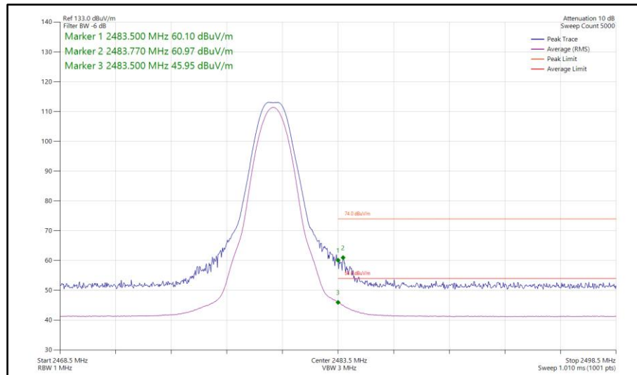
Figure 104 - Bluetooth LE1M, MIMO, Core 0-1 - 2480 MHz Band Edge Frequency 2483.5 MHz
