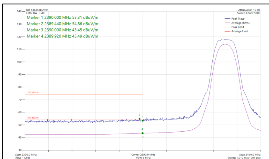
Figure 124 - Bluetooth HDRPS2, SISO, Core 0 - 2404 MHz Band Edge Frequency 2390 MHz
