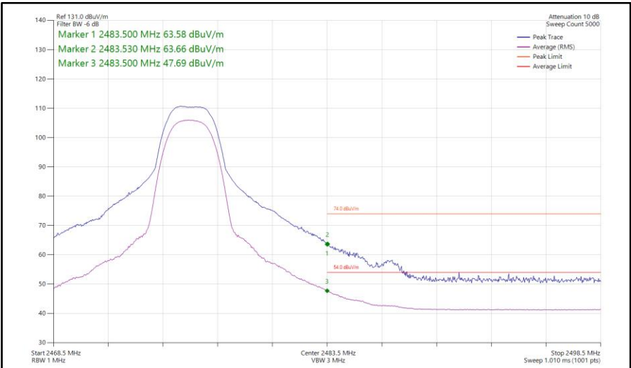
Figure 107 - Bluetooth HDT4, MIMO, Core 0-1 - 2476 MHz Band Edge Frequency 2483.5 MHz
