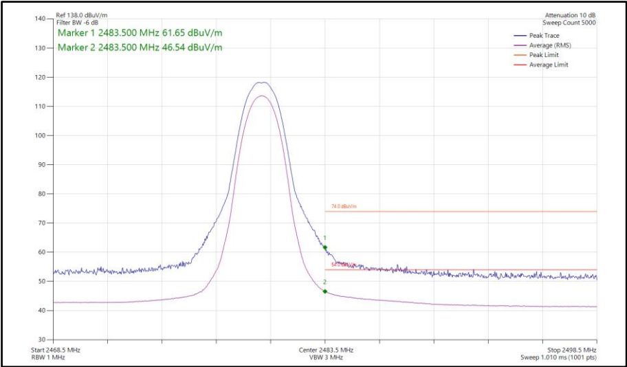
Figure 159 - Bluetooth 2DH5, SISO, Core 1 - 2480 MHz Band Edge Frequency 2483.5 MHz
