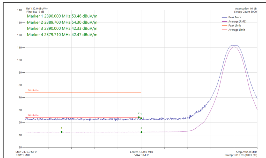
Figure 98 - Bluetooth CS1LE1M, MIMO, Core 0-1 - 2402 MHz Band Edge Frequency 2390 MHz
