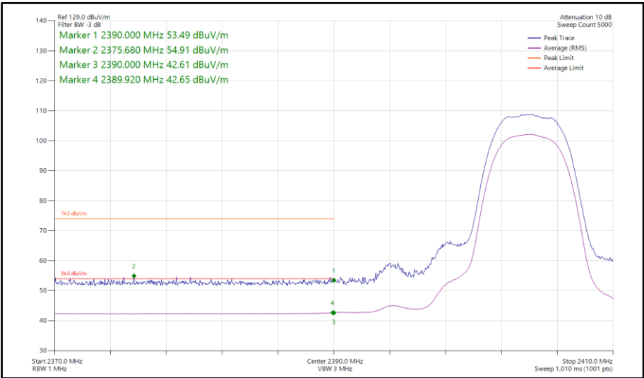
Figure 89 - Bluetooth HDR8, MIMO, Core 0-1 - 2404 MHz Band Edge Frequency 2390 MHz
