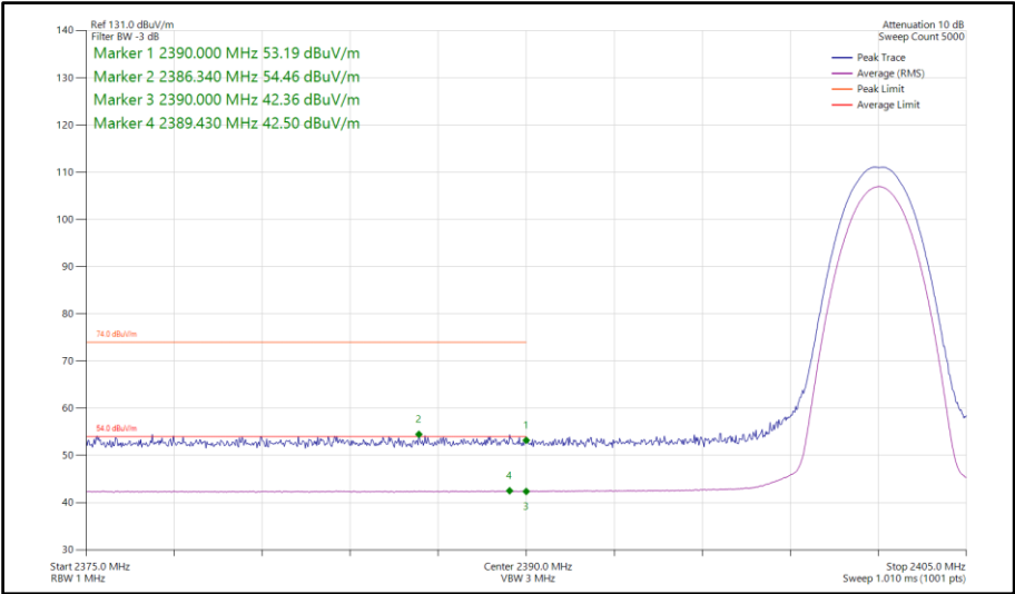
Figure 86 - Bluetooth 2DH5, MIMO, Core 0-1 - 2402 MHz Band Edge Frequency 2390 MHz
