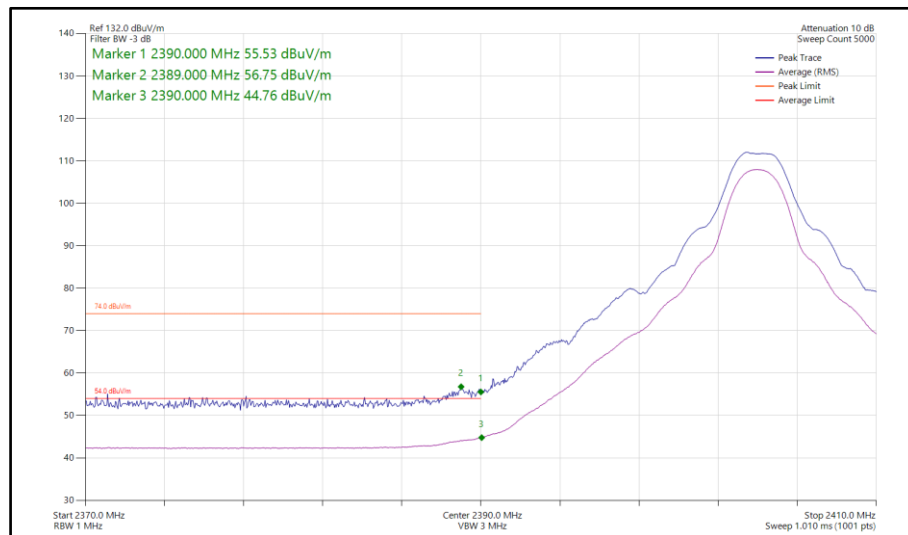
Figure 93 - Bluetooth HDT4, MIMO, Core 0-1 - 2404 MHz Band Edge Frequency 2390 MHz
