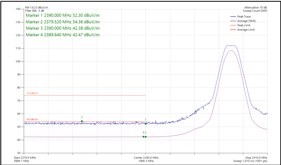
Figure 91 - Bluetooth LE2M, MIMO, Core 0-1 - 2404 MHz Band Edge Frequency 2390 MHz
