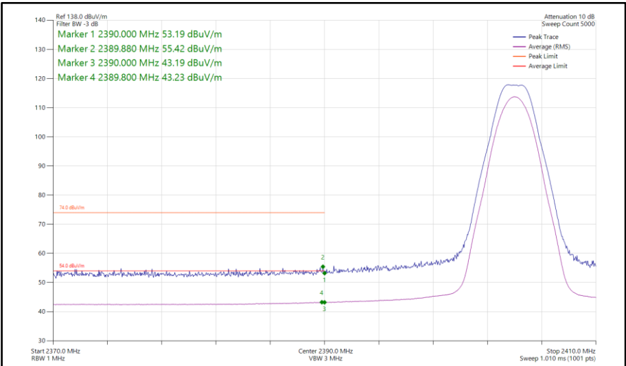
Figure 150 - Bluetooth LE2M, SISO, Core 1 - 2404 MHz Band Edge Frequency 2390 MHz
