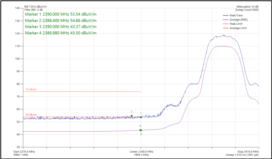
Figure 125 - Bluetooth HDRPM12, SISO, Core 0 - 2404 MHz Band Edge Frequency 2390 MHz
