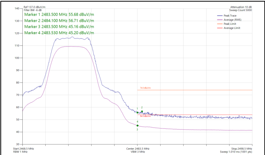
Figure 140 - Bluetooth XHDRPM8, SISO, Core 0 - 2475 MHz Band Edge Frequency 2483.5 MHz
