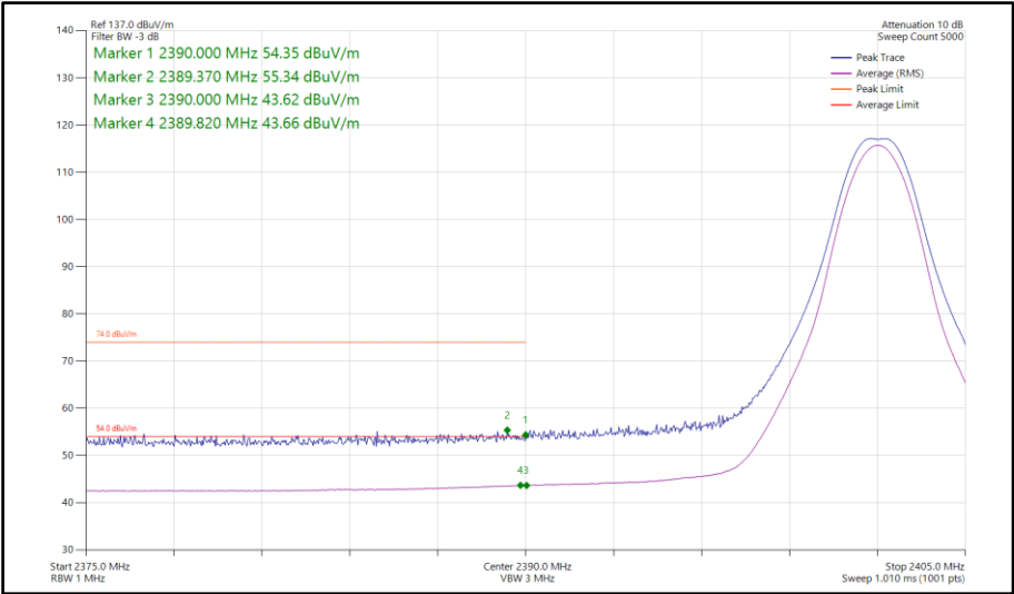
Figure 127 - Bluetooth CS1LE1M, SISO, Core 0 - 2402 MHz Band Edge Frequency 2390 MHz
