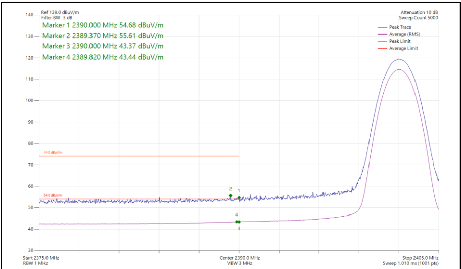
Figure 116 - Bluetooth 3DH5, SISO, Core 0 - 2402 MHz Band Edge Frequency 2390 MHz
