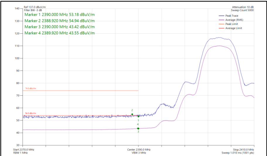
Figure 148 - Bluetooth HDR8, SISO, Core 1 - 2404 MHz Band Edge Frequency 2390 MHz
