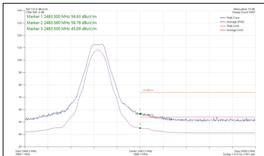
Figure 105 - Bluetooth LE2M, MIMO, Core 0-1 - 2478 MHz Band Edge Frequency 2483.5 MHz
