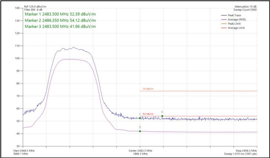
Figure 110 - Bluetooth HDRPM12, MIMO, Core 0-1 - 2475 MHz Band Edge Frequency 2483.5 MHz
