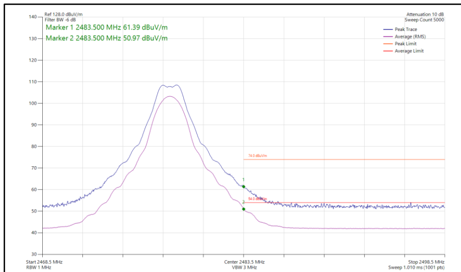
Figure 144 - Bluetooth CS1LE2M, SISO, Core 0 - 2478 MHz Band Edge Frequency 2483.5 MHz
