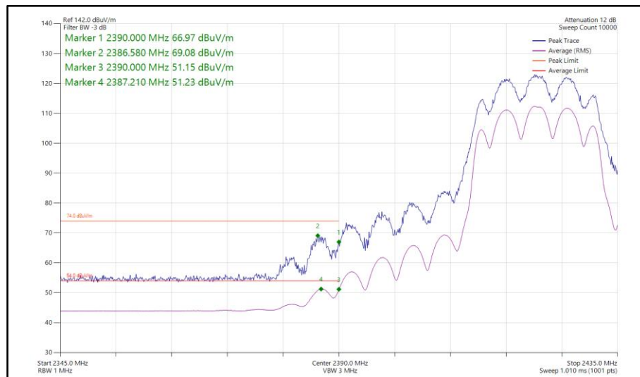
Figure 139 - 802.11ax HE20, SU, CDD, Core 0-1 - 2422 MHz Band Edge Frequency 2390 MHz
