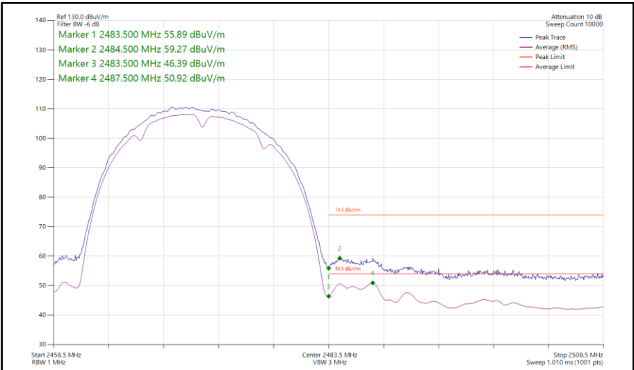
Figure 90 - 802.11b, SISO, Core 1 - 2472 MHz Band Edge Frequency 2483.5 MHz
