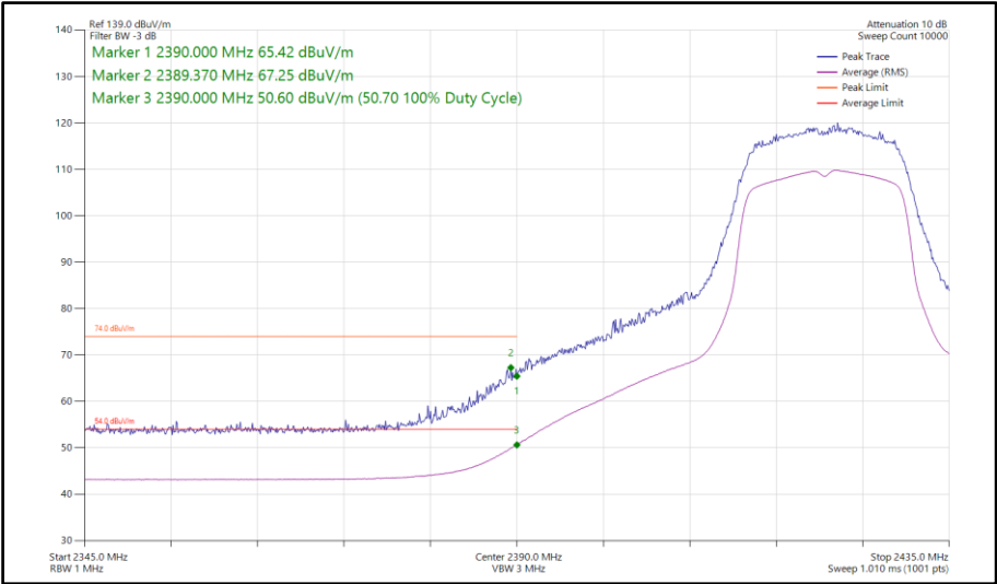
Figure 69 - 802.11g, SISO, Core 1 - 2422 MHz Band Edge Frequency 2390 MHz
