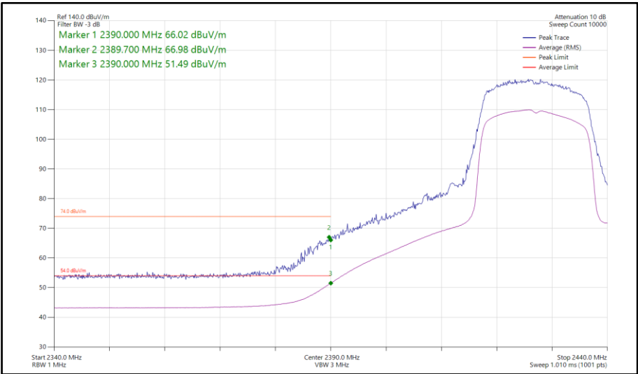
Figure 82 - 802.11ax HE20, SU, SISO, Core 1 - 2427 MHz Band Edge Frequency 2390 MHz
