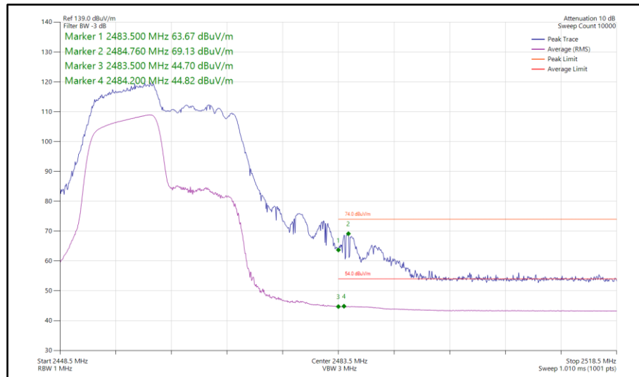
Figure 115 - 802.11ax HE20, RU106-53, SISO, Core 1 - 2462 MHz Band Edge Frequency 2483.5 MHz
