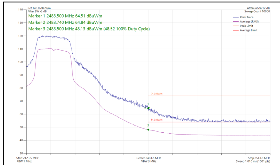
Figure 91 - 802.11g, SISO, Core 1 - 2437 MHz Band Edge Frequency 2483.5 MHz
