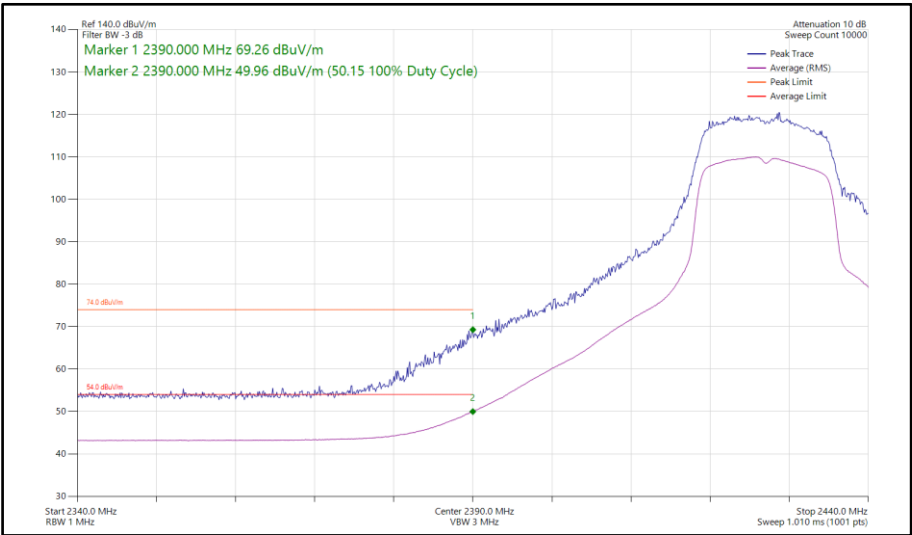
Figure 70 - 802.11g, SISO, Core 1 - 2427 MHz Band Edge Frequency 2390 MHz
