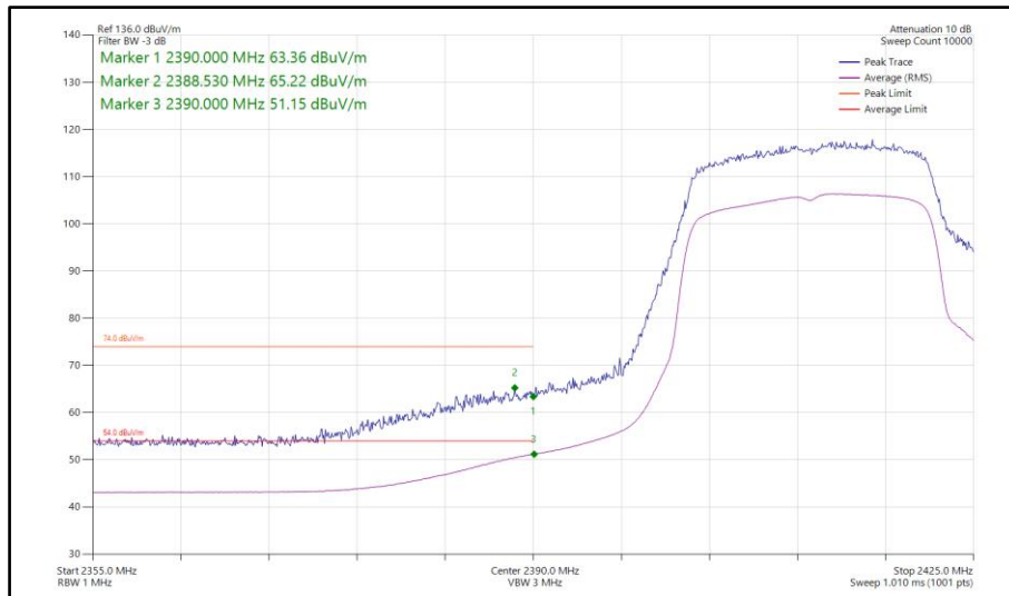
Figure 77 - 802.11ax HE20, SU, SISO, Core 1 - 2412 MHz Band Edge Frequency 2390 MHz
