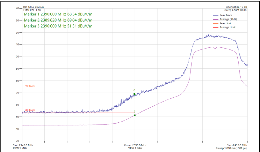
Figure 74 - 802.11n HT20, SISO, Core 1 - 2422 MHz Band Edge Frequency 2390 MHz
