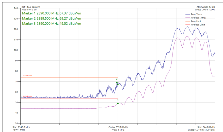
Figure 133 - 802.11n HT20, CDD, Core 0-1 - 2427 MHz Band Edge Frequency 2390 MHz
