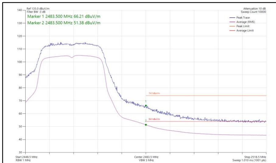
Figure 104 - 802.11n HT20, SISO, Core 1 - 2462 MHz Band Edge Frequency 2483.5 MHz
