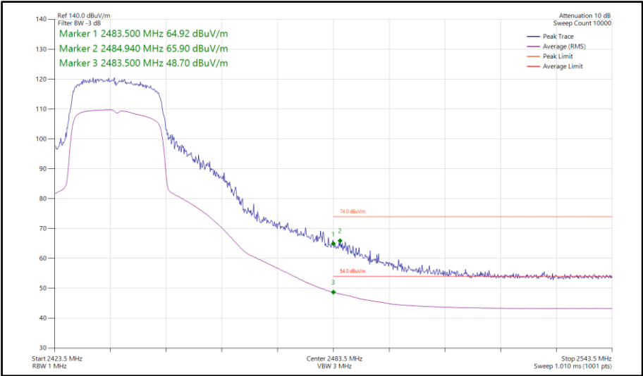
Figure 107 - 802.11ax HE20, SU, SISO, Core 1 - 2437 MHz Band Edge Frequency 2483.5 MHz
