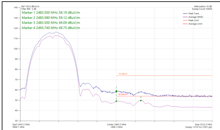
Figure 87 - 802.11b, SISO, Core 1 - 2457 MHz Band Edge Frequency 2483.5 MHz
