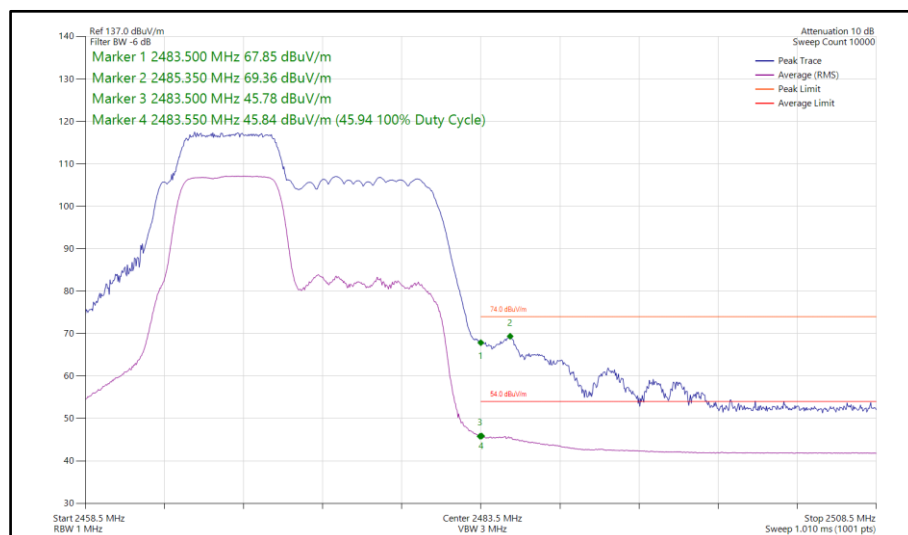
Figure 124 - 802.11be EHT20, RU52+26-70, SISO, Core 1 - 2472 MHz Band Edge Frequency 2483.5 MHz
