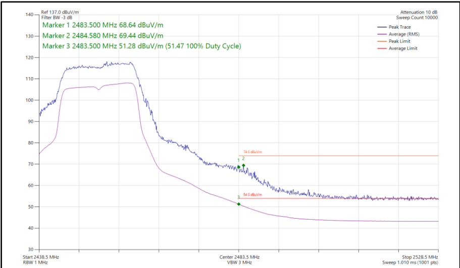
Figure 94 - 802.11g, SISO, Core 1 - 2452 MHz Band Edge Frequency 2483.5 MHz
