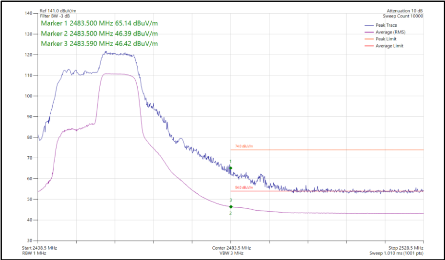
Figure 111 - 802.11ax HE20, RU106-54, SISO, Core 1 - 2452 MHz Band Edge Frequency 2483.5 MHz
