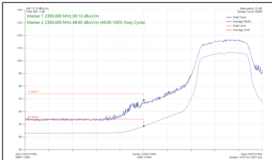
Figure 68 - 802.11g, SISO, Core 1 - 2417 MHz Band Edge Frequency 2390 MHz
