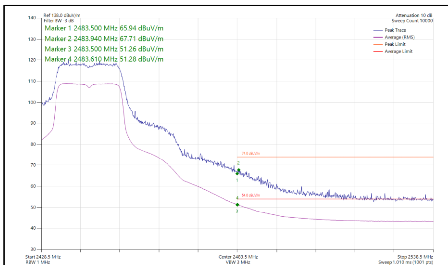
Figure 100 - 802.11n HT20, SISO, Core 1 - 2442 MHz Band Edge Frequency 2483.5 MHz
