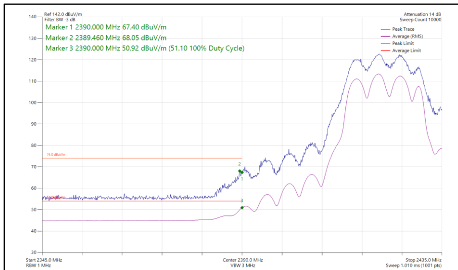
Figure 127 - 802.11g, CDD, Core 0-1 - 2422 MHz Band Edge Frequency 2390 MHz
