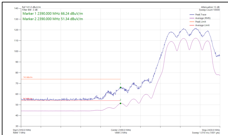
Figure 131 - 802.11n HT20, CDD, Core 0-1 - 2417 MHz Band Edge Frequency 2390 MHz
