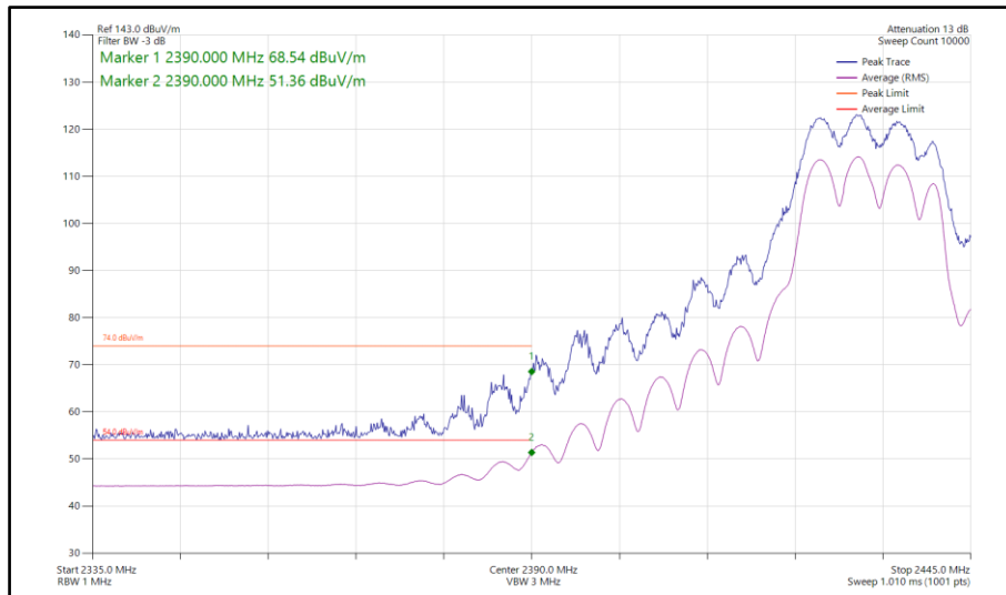
Figure 134 - 802.11n HT20, CDD, Core 0-1 - 2432 MHz Band Edge Frequency 2390 MHz
