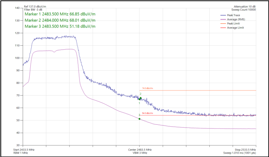
Figure 109 - 802.11ax HE20, SU, SISO, Core 1 - 2447 MHz Band Edge Frequency 2483.5 MHz
