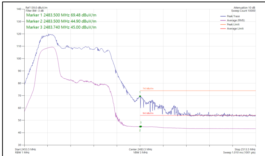
Figure 117 - 802.11ax HE20, RU52-37, SISO, Core 1 - 2467 MHz Band Edge Frequency 2483.5 MHz
