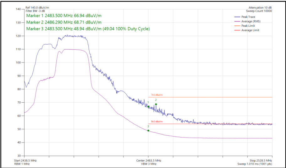
Figure 120 - 802.11be EHT20, RU106+26-83, SISO, Core 1 - 2452 MHz Band Edge Frequency 2483.5 MHz
