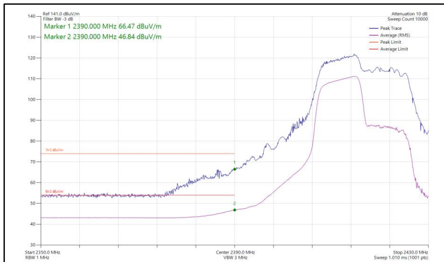
Figure 80 - 802.11ax HE20, RU106-53, SISO, Core 1 - 2417 MHz Band Edge Frequency 2390 MHz
