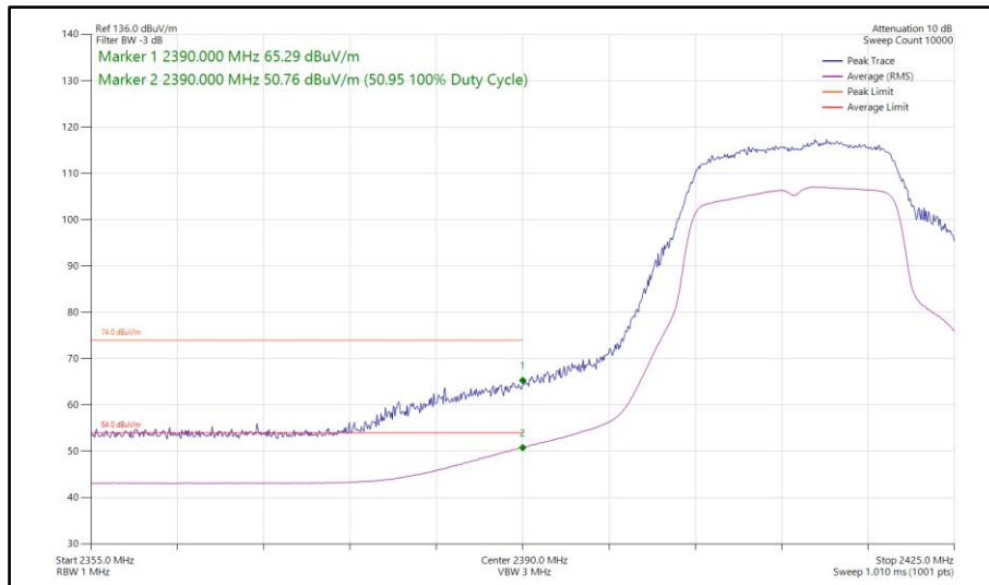
Figure 67 - 802.11g, SISO, Core 1 - 2412 MHz Band Edge Frequency 2390 MHz
