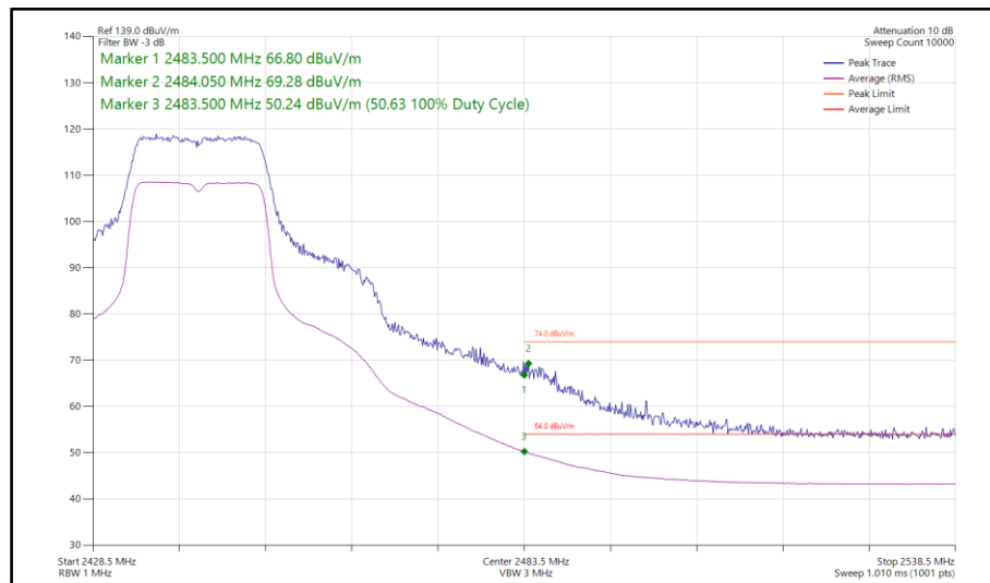
Figure 92 - 802.11g, SISO, Core 1 - 2442 MHz Band Edge Frequency 2483.5 MHz
