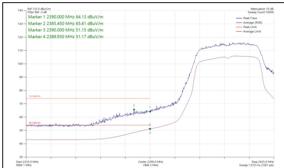
Figure 72 - 802.11n HT20, SISO, Core 1 - 2412 MHz Band Edge Frequency 2390 MHz
