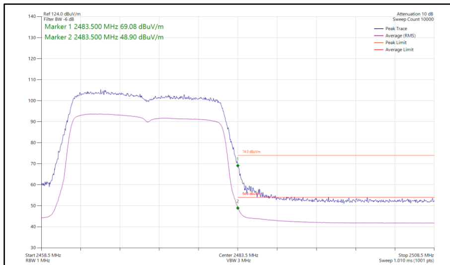
Figure 118 - 802.11ax HE20, SU, SISO, Core 1 - 2472 MHz Band Edge Frequency 2483.5 MHz
