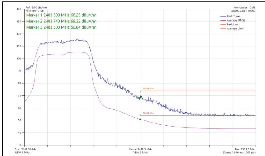
Figure 103 - 802.11n HT20, SISO, Core 1 - 2457 MHz Band Edge Frequency 2483.5 MHz
