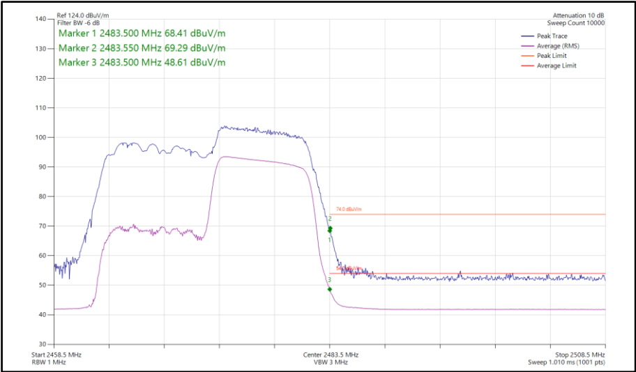
Figure 119 - 802.11ax HE20, RU106-54, SISO, Core 1 - 2472 MHz Band Edge Frequency 2483.5 MHz
