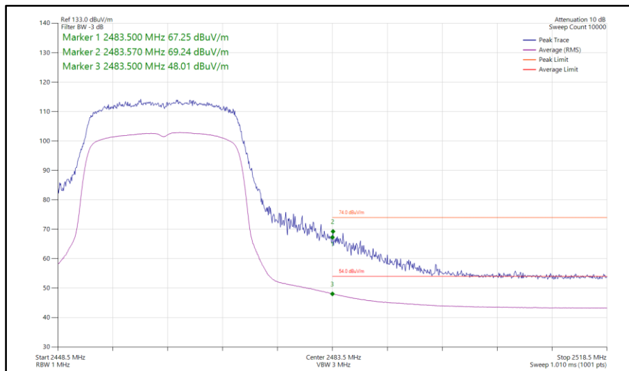
Figure 114 - 802.11ax HE20, SU, SISO, Core 1 - 2462 MHz Band Edge Frequency 2483.5 MHz
