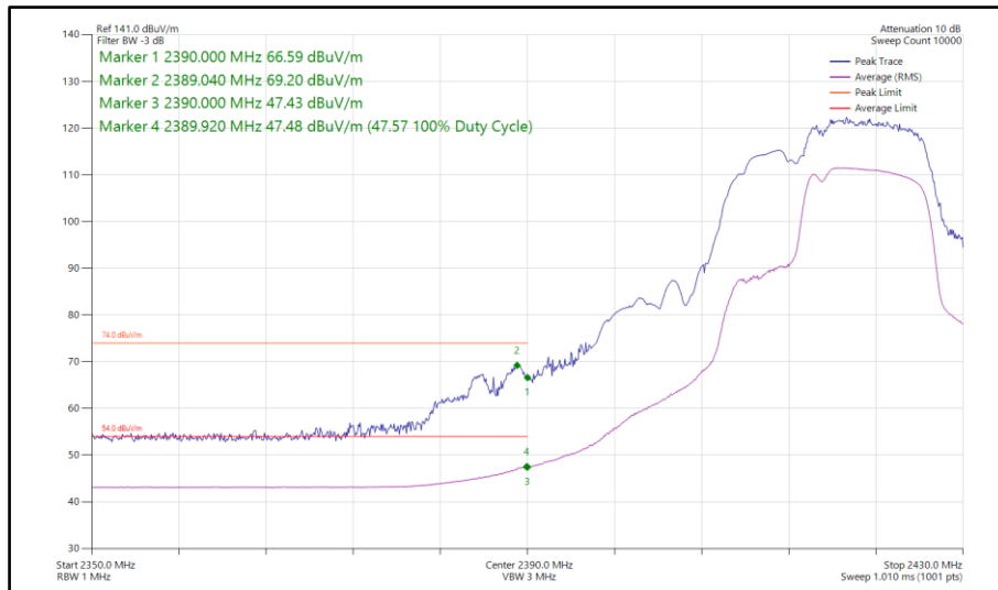
Figure 85 - 802.11be EHT20, RU106+26-83, SISO, Core 1 - 2417 MHz Band Edge Frequency 2390 MHz
