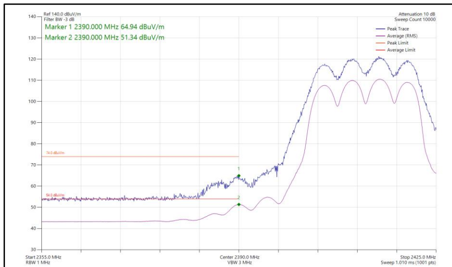
Figure 135 - 802.11ax HE20, SU, CDD, Core 0-1 - 2412 MHz Band Edge Frequency 2390 MHz
