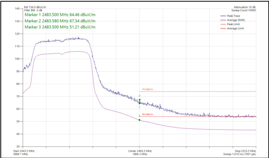
Figure 112 - 802.11ax HE20, SU, SISO, Core 1 - 2457 MHz Band Edge Frequency 2483.5 MHz
