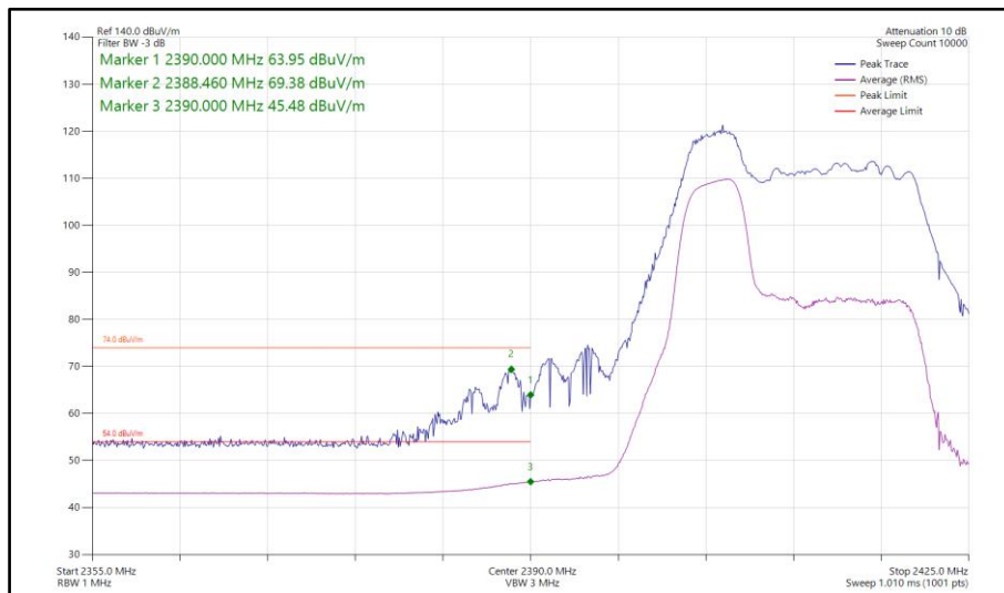
Figure 78 - 802.11ax HE20, RU52-37, SISO, Core 1 - 2412 MHz Band Edge Frequency 2390 MHz
