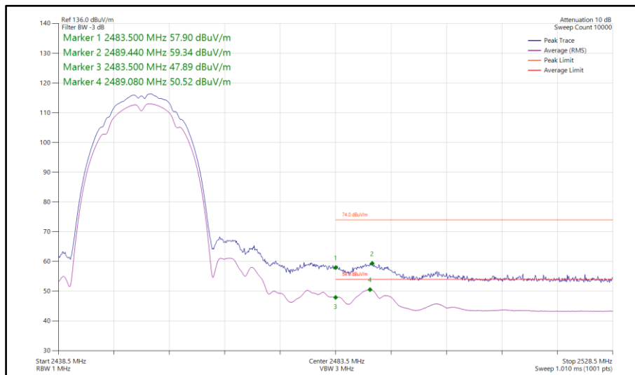
Figure 86 - 802.11b, SISO, Core 1 - 2452 MHz Band Edge Frequency 2483.5 MHz
