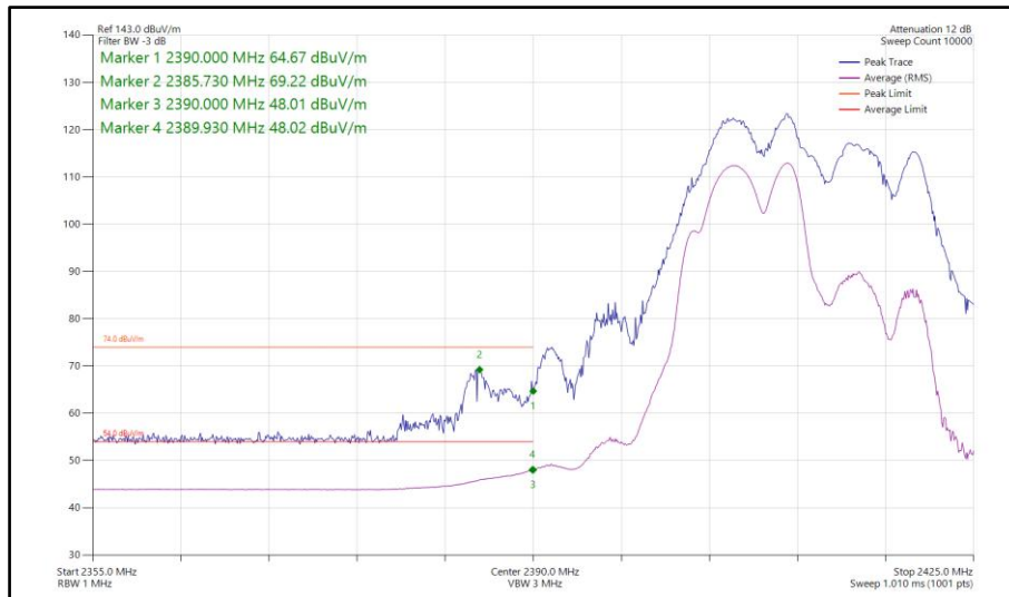
Figure 136 - 802.11ax HE20, RU106-53, CDD, Core 0-1 - 2412 MHz Band Edge Frequency 2390 MHz
