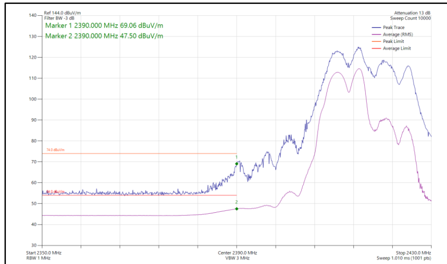
Figure 138 - 802.11ax HE20, RU106-53, CDD, Core 0-1 - 2417 MHz Band Edge Frequency 2390 MHz
