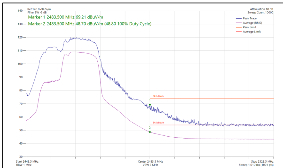
Figure 121 - 802.11be EHT20, RU106+26-83, SISO, Core 1 - 2457 MHz Band Edge Frequency 2483.5 MHz
