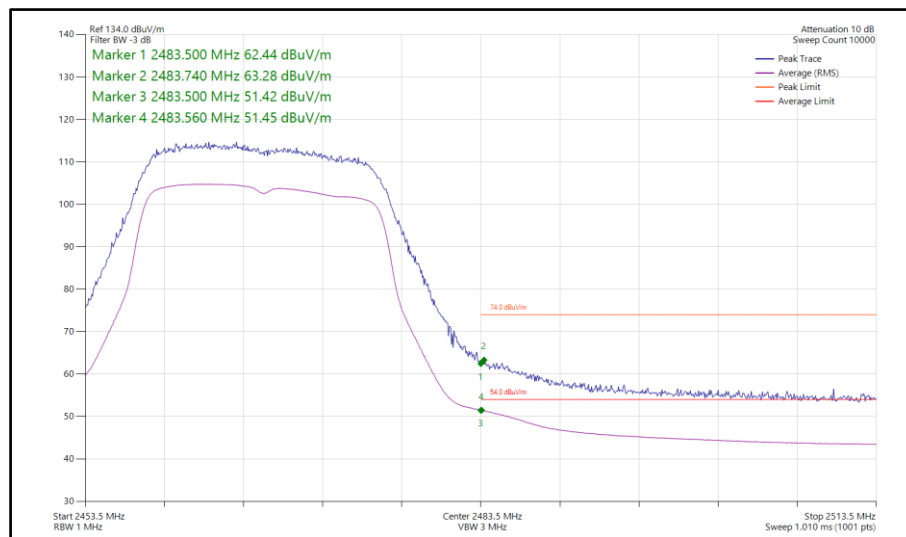
Figure 105 - 802.11n HT20, SISO, Core 1 - 2467 MHz Band Edge Frequency 2483.5 MHz
