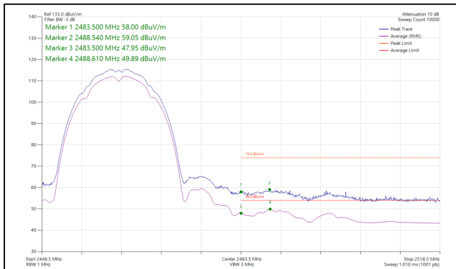
Figure 88 - 802.11b, SISO, Core 1 - 2462 MHz Band Edge Frequency 2483.5 MHz
