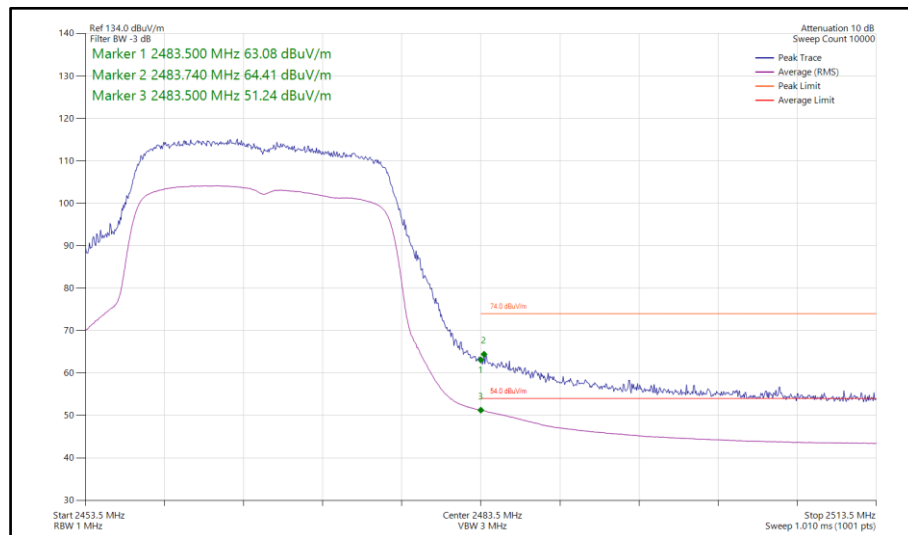
Figure 116 - 802.11ax HE20, SU, SISO, Core 1 - 2467 MHz Band Edge Frequency 2483.5 MHz
