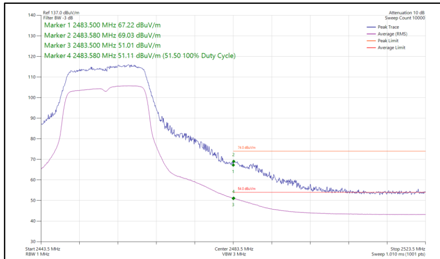
Figure 95 - 802.11g, SISO, Core 1 - 2457 MHz Band Edge Frequency 2483.5 MHz
