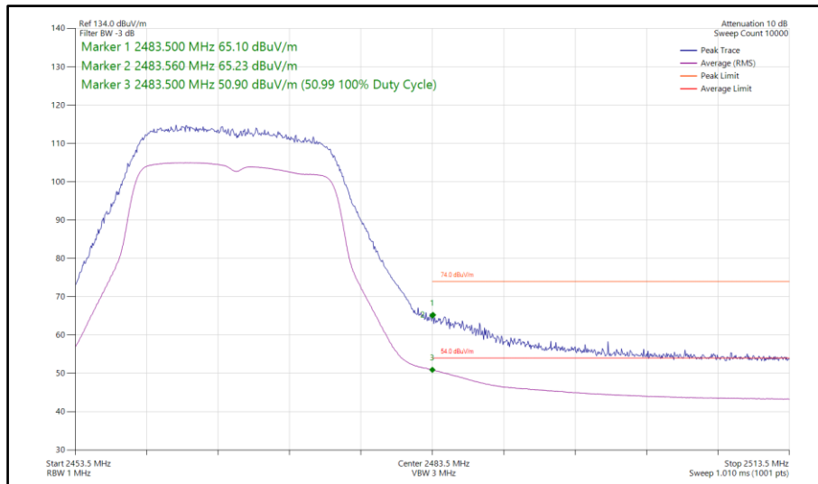
Figure 97 - 802.11g, SISO, Core 1 - 2467 MHz Band Edge Frequency 2483.5 MHz
