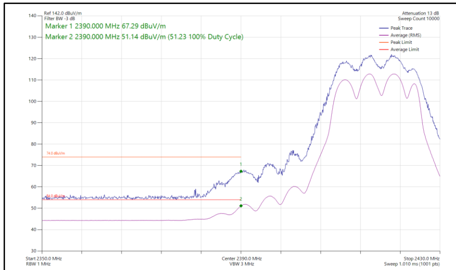
Figure 126 - 802.11g, CDD, Core 0-1 - 2417 MHz Band Edge Frequency 2390 MHz
