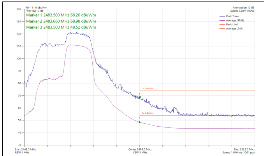
Figure 113 - 802.11ax HE20, RU106-54, SISO, Core 1 - 2457 MHz Band Edge Frequency 2483.5 MHz
