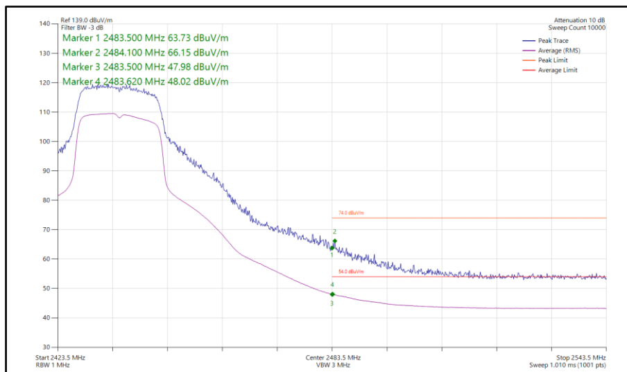
Figure 99 - 802.11n HT20, SISO, Core 1 - 2437 MHz Band Edge Frequency 2483.5 MHz
