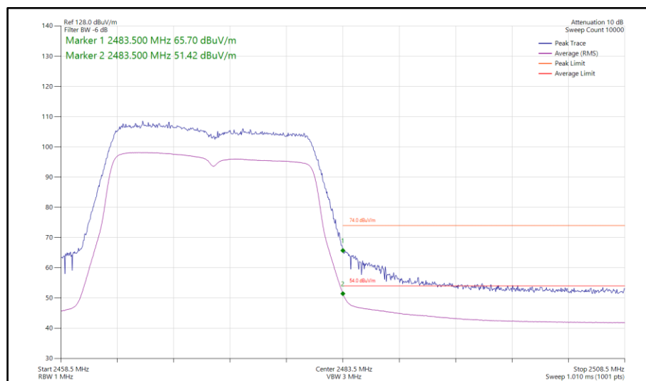
Figure 106 - 802.11n HT20, SISO, Core 1 - 2472 MHz Band Edge Frequency 2483.5 MHz
