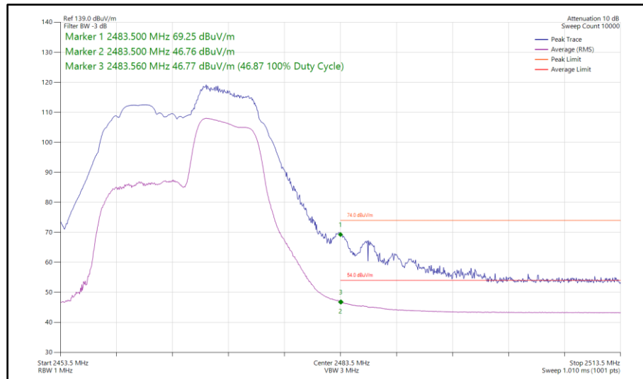
Figure 123 - 802.11be EHT20, RU52+26-72, SISO, Core 1 - 2467 MHz Band Edge Frequency 2483.5 MHz
