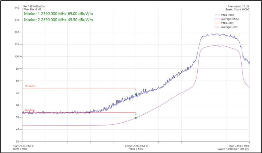
Figure 75 - 802.11n HT20, SISO, Core 1 - 2427 MHz Band Edge Frequency 2390 MHz
