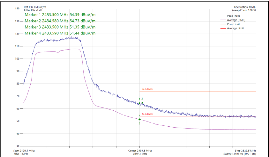
Figure 102 - 802.11n HT20, SISO, Core 1 - 2452 MHz Band Edge Frequency 2483.5 MHz
