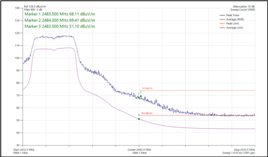
Figure 101 - 802.11n HT20, SISO, Core 1 - 2447 MHz Band Edge Frequency 2483.5 MHz
