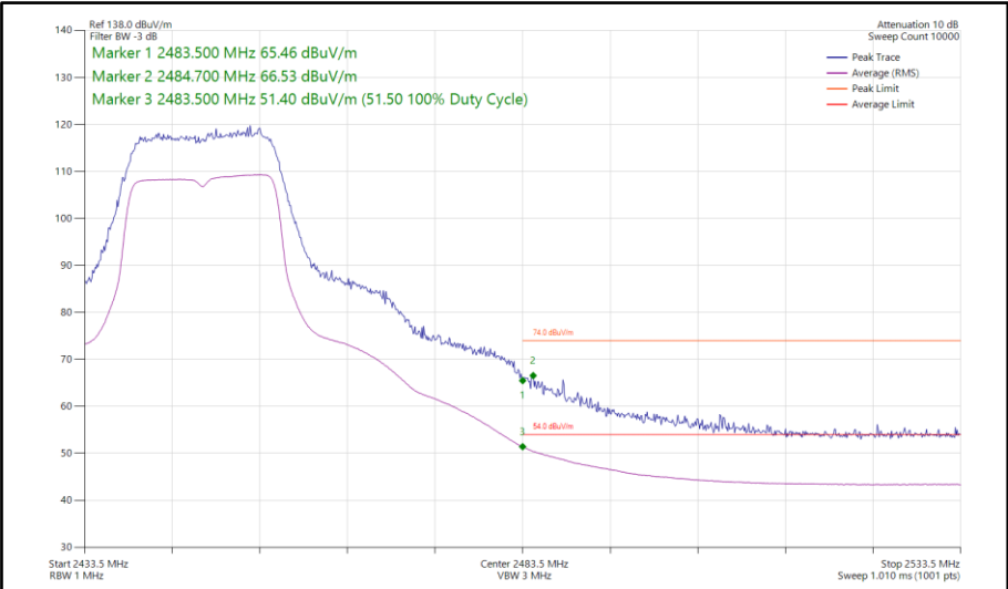
Figure 93 - 802.11g, SISO, Core 1 - 2447 MHz Band Edge Frequency 2483.5 MHz
