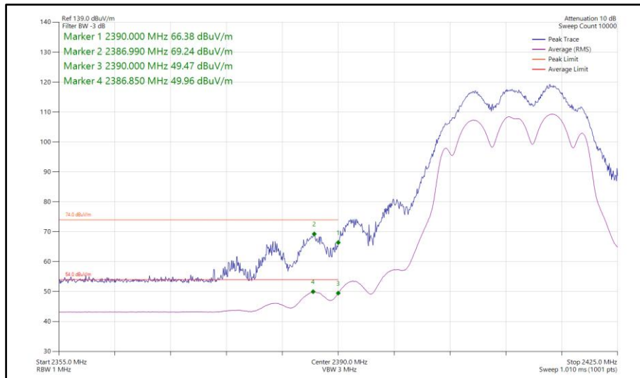
Figure 130 - 802.11n HT20, CDD, Core 0-1 - 2412 MHz Band Edge Frequency 2390 MHz
