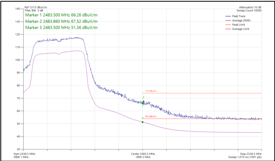
Figure 110 - 802.11ax HE20, SU, SISO, Core 1 - 2452 MHz Band Edge Frequency 2483.5 MHz
