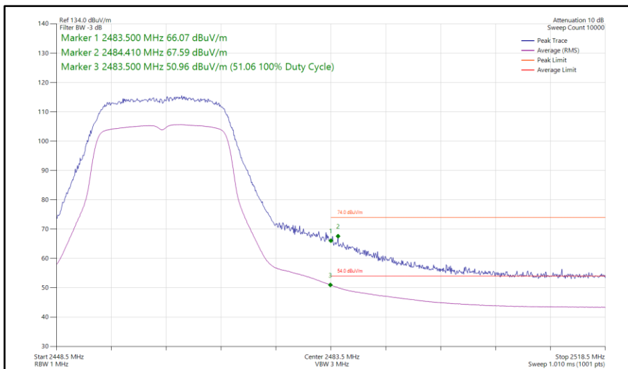
Figure 96 - 802.11g, SISO, Core 1 - 2462 MHz Band Edge Frequency 2483.5 MHz
