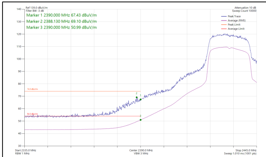
Figure 83 - 802.11ax HE20, SU, SISO, Core 1 - 2432 MHz Band Edge Frequency 2390 MHz
