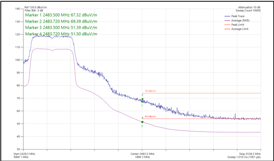
Figure 108 - 802.11ax HE20, SU, SISO, Core 1 - 2442 MHz Band Edge Frequency 2483.5 MHz
