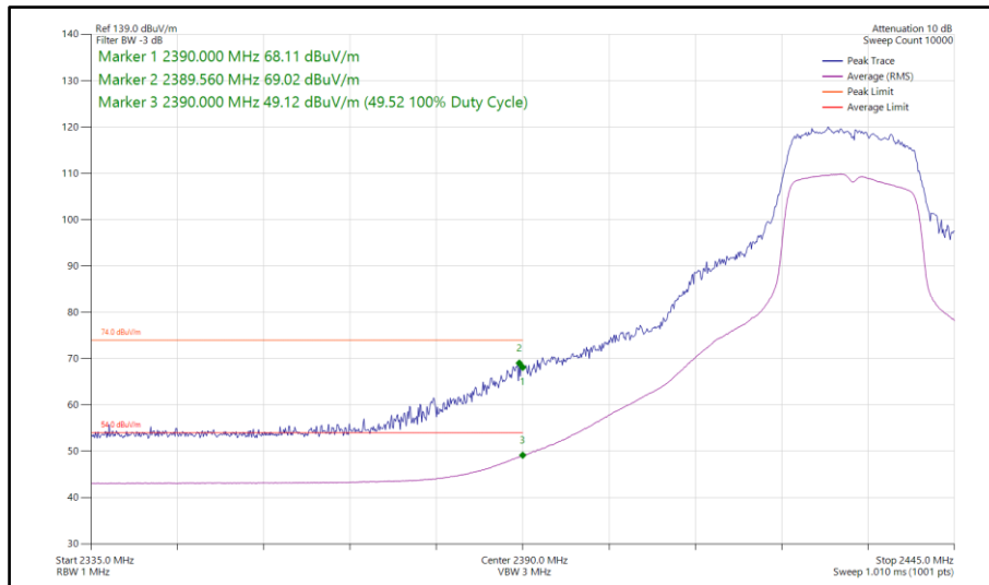
Figure 71 - 802.11g, SISO, Core 1 - 2432 MHz Band Edge Frequency 2390 MHz
