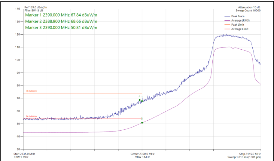
Figure 76 - 802.11n HT20, SISO, Core 1 - 2432 MHz Band Edge Frequency 2390 MHz
