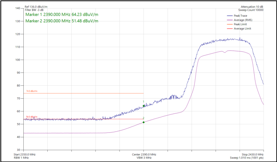
Figure 73 - 802.11n HT20, SISO, Core 1 - 2417 MHz Band Edge Frequency 2390 MHz
