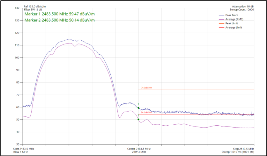
Figure 89 - 802.11b, SISO, Core 1 - 2467 MHz Band Edge Frequency 2483.5 MHz
