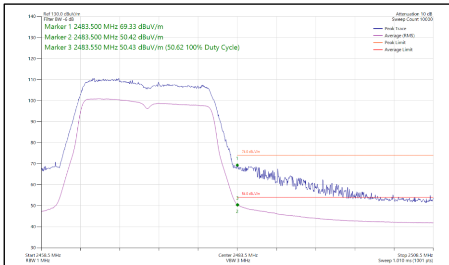
Figure 98 - 802.11g, SISO, Core 1 - 2472 MHz Band Edge Frequency 2483.5 MHz
