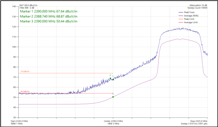
Figure 81 - 802.11ax HE20, SU, SISO, Core 1 - 2422 MHz Band Edge Frequency 2390 MHz
