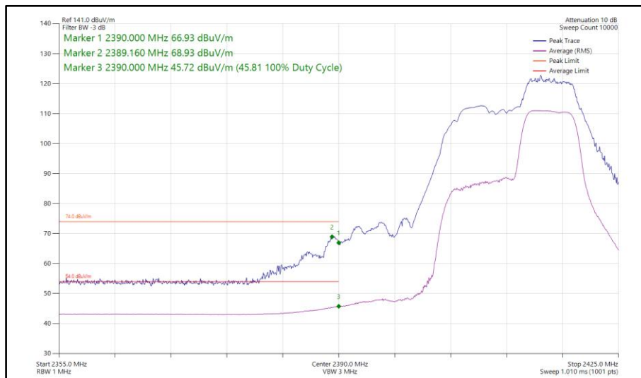
Figure 84 - 802.11be EHT20, RU52+26-72, SISO, Core 1 - 2412 MHz Band Edge Frequency 2390 MHz
