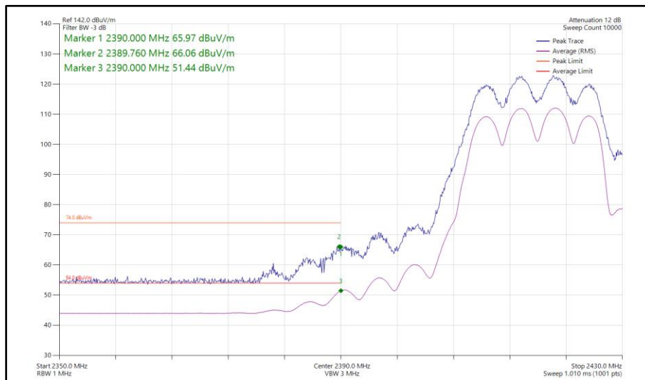
Figure 137 - 802.11ax HE20, SU, CDD, Core 0-1 - 2417 MHz Band Edge Frequency 2390 MHz
