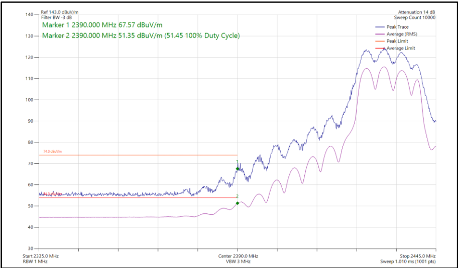
Figure 129 - 802.11g, CDD, Core 0-1 - 2432 MHz Band Edge Frequency 2390 MHz
