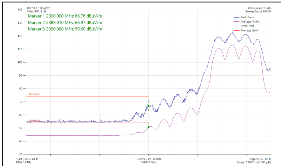
Figure 132 - 802.11n HT20, CDD, Core 0-1 - 2422 MHz Band Edge Frequency 2390 MHz
