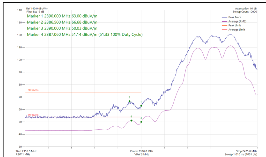
Figure 125 - 802.11g, CDD, Core 0-1 - 2412 MHz Band Edge Frequency 2390 MHz
