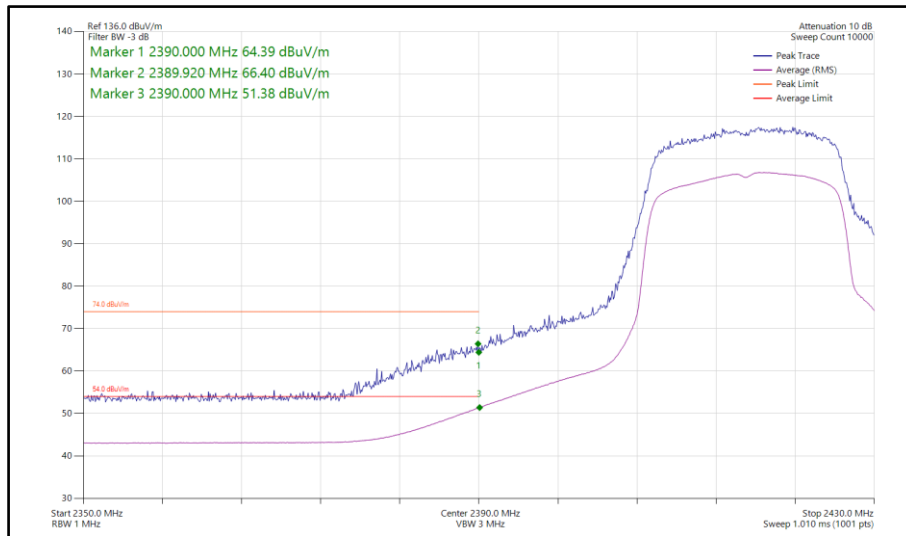
Figure 79 - 802.11ax HE20, SU, SISO, Core 1 - 2417 MHz Band Edge Frequency 2390 MHz
