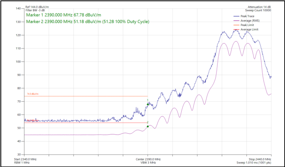
Figure 128 - 802.11g, CDD, Core 0-1 - 2427 MHz Band Edge Frequency 2390 MHz
