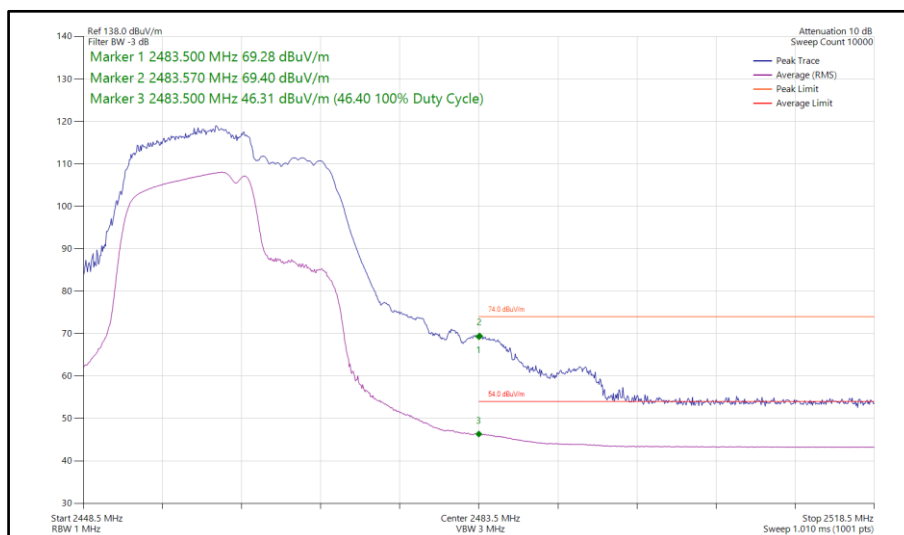
Figure 122 - 802.11be EHT20, RU106+26-82, SISO, Core 1 - 2462 MHz Band Edge Frequency 2483.5 MHz
