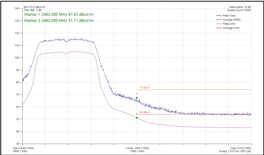
Figure 197 - 802.11n HT20, SDM, Core 0-1 - 2462 MHz Band Edge Frequency 2483.5 MHz
