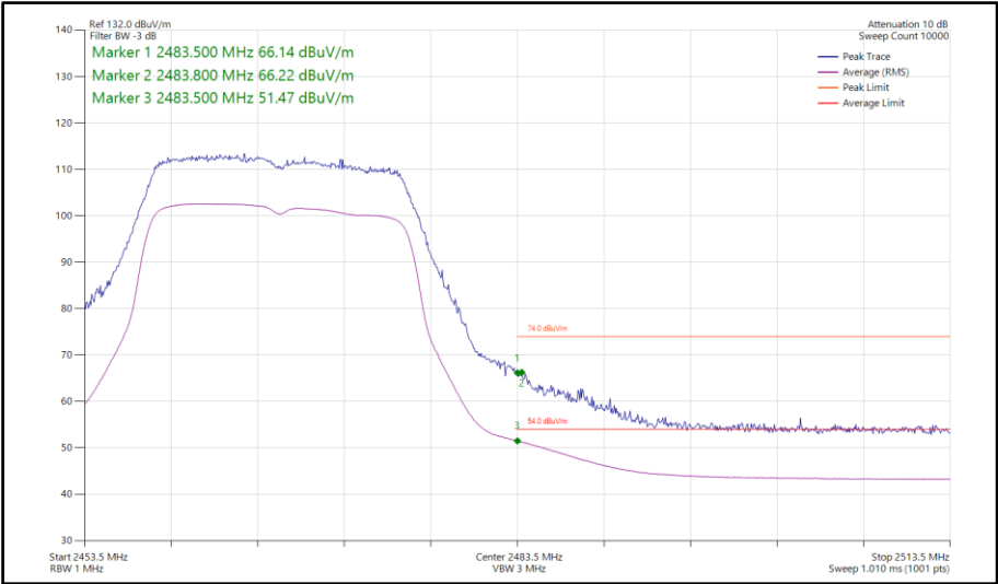
Figure 198 - 802.11n HT20, SDM, Core 0-1 - 2467 MHz Band Edge Frequency 2483.5 MHz
