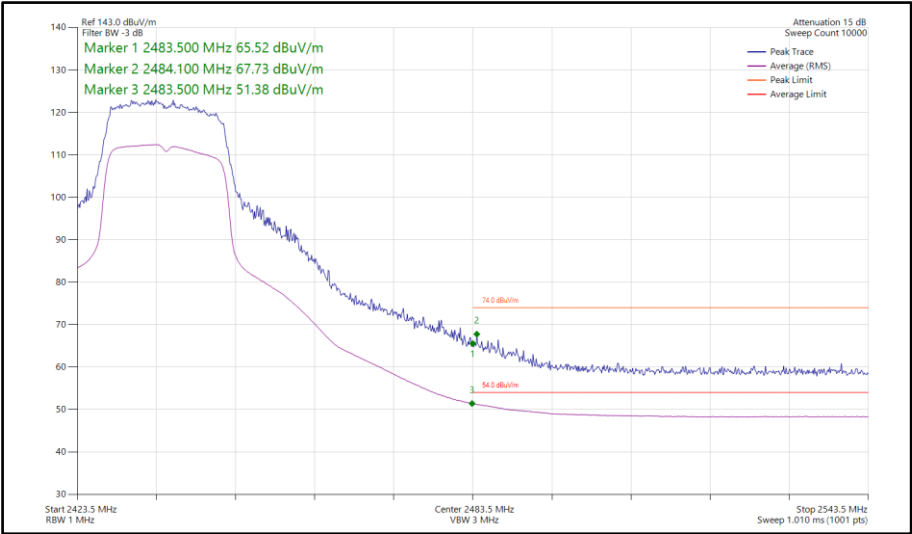
Figure 192 - 802.11n HT20, SDM, Core 0-1 - 2437 MHz Band Edge Frequency 2483.5 MHz
