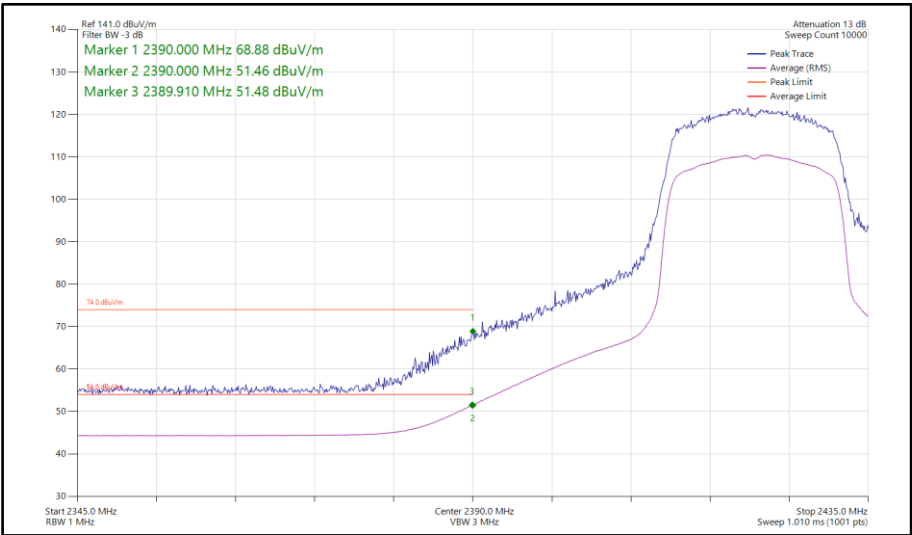
Figure 187 - 802.11ax HE20, SU, SDM, Core 0-1 - 2422 MHz Band Edge Frequency 2390 MHz
