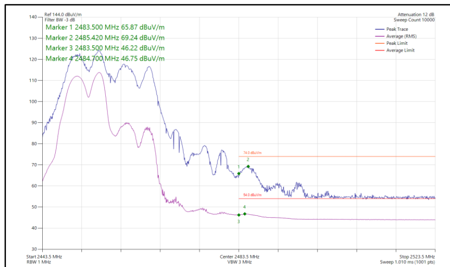
Figure 166 - 802.11ax HE20, RU106-53, CDD, Core 0-1 - 2457 MHz Band Edge Frequency 2483.5 MHz
