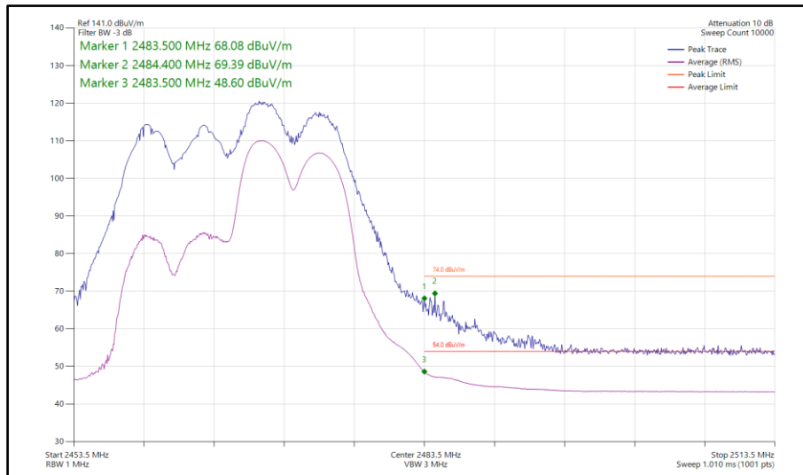
Figure 170 - 802.11ax HE20, RU106-54, CDD, Core 0-1 - 2467 MHz Band Edge Frequency 2483.5 MHz
