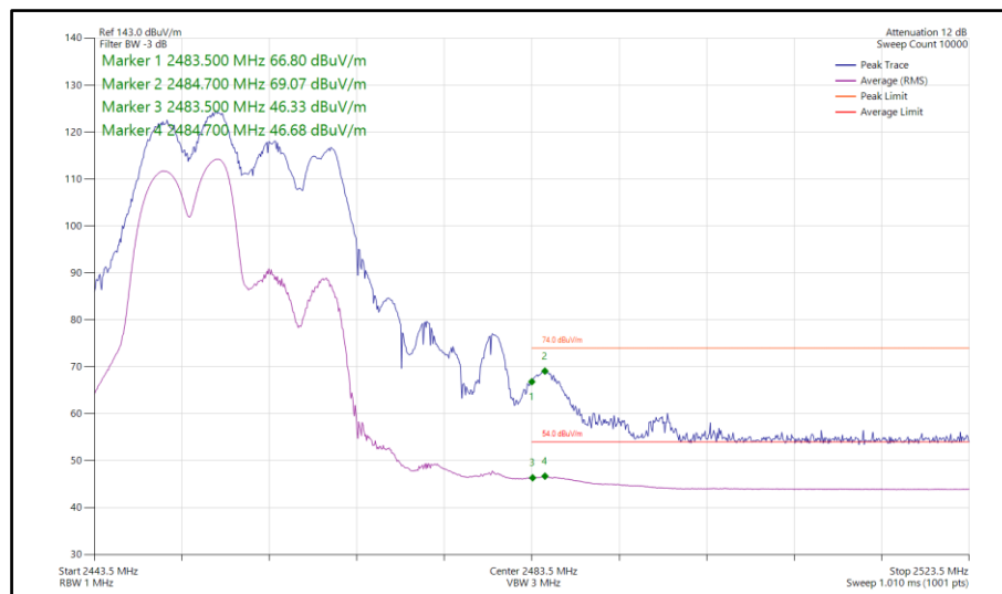
Figure 206 - 802.11ax HE20, RU106-53, SDM, Core 0-1 - 2457 MHz Band Edge Frequency 2483.5 MHz
