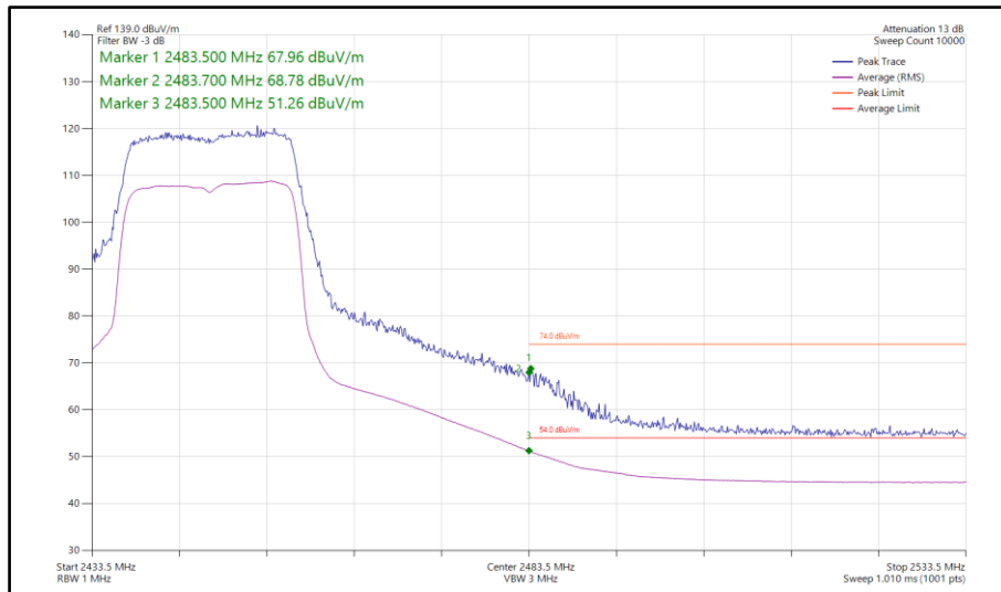
Figure 202 - 802.11ax HE20, SU, SDM, Core 0-1 - 2447 MHz Band Edge Frequency 2483.5 MHz
