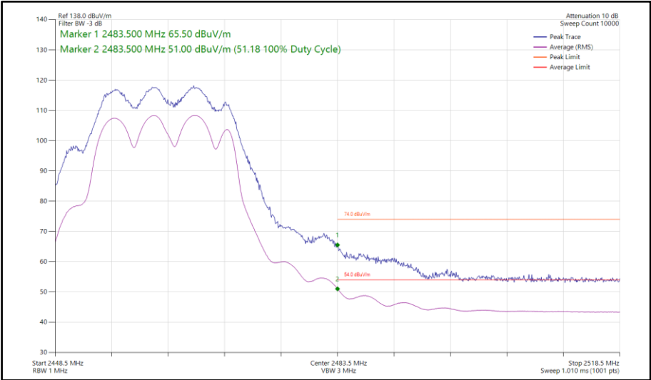
Figure 149 - 802.11g, CDD, Core 0-1 - 2462 MHz Band Edge Frequency 2483.5 MHz
