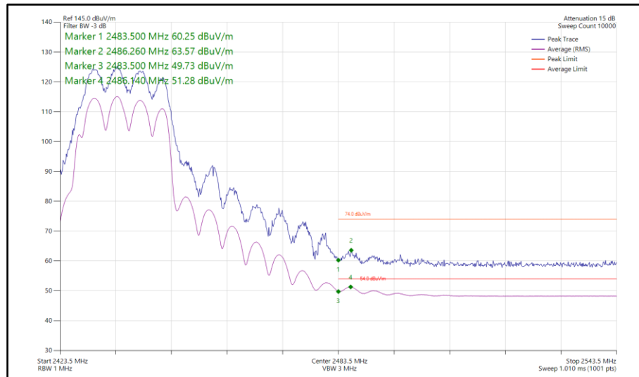
Figure 160 - 802.11ax HE20, SU, CDD, Core 0-1 - 2437 MHz Band Edge Frequency 2483.5 MHz
