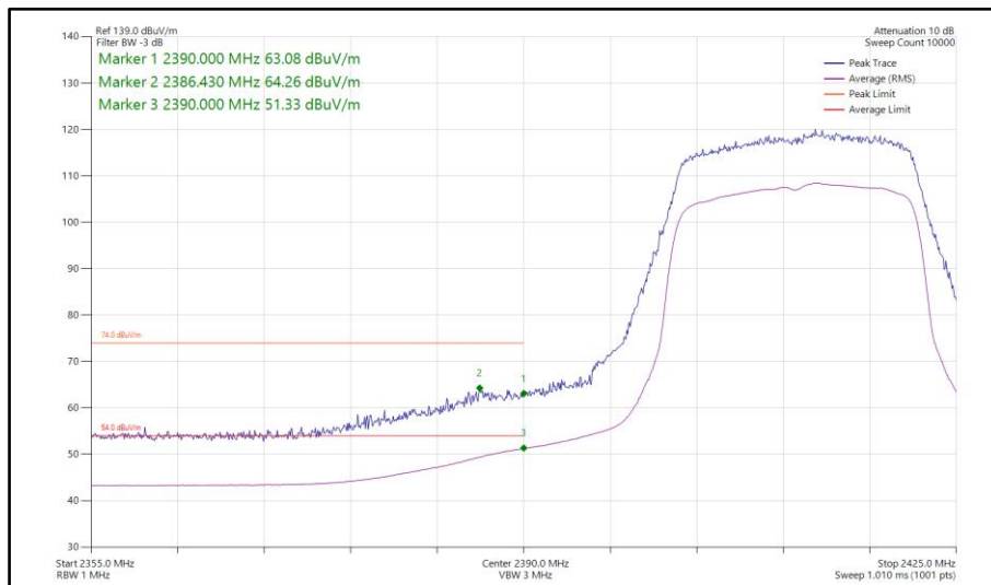
Figure 183 - 802.11ax HE20, SU, SDM, Core 0-1 - 2412 MHz Band Edge Frequency 2390 MHz
