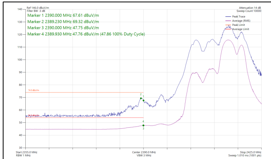
Figure 190 - 802.11be EHT20, RU52+26-72, SDM, Core 0-1 - 2412 MHz Band Edge Frequency 2390 MHz
