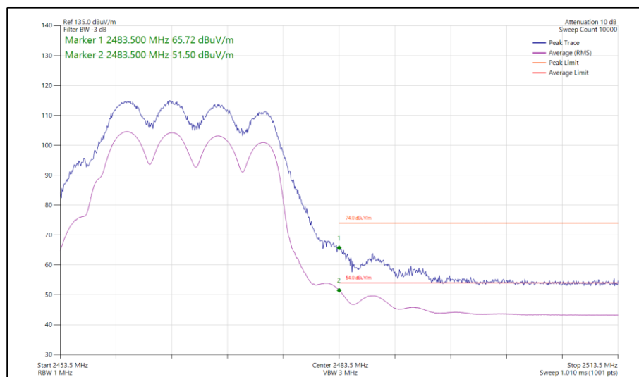
Figure 169 - 802.11ax HE20, SU, CDD, Core 0-1 - 2467 MHz Band Edge Frequency 2483.5 MHz
