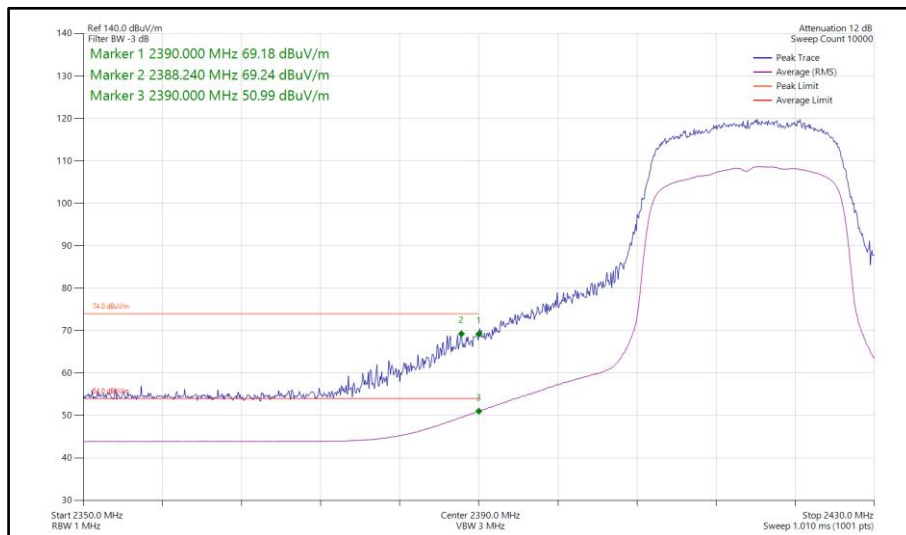
Figure 185 - 802.11ax HE20, SU, SDM, Core 0-1 - 2417 MHz Band Edge Frequency 2390 MHz
