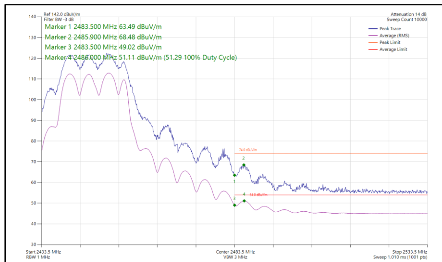
Figure 146 - 802.11g, CDD, Core 0-1 - 2447 MHz Band Edge Frequency 2483.5 MHz
