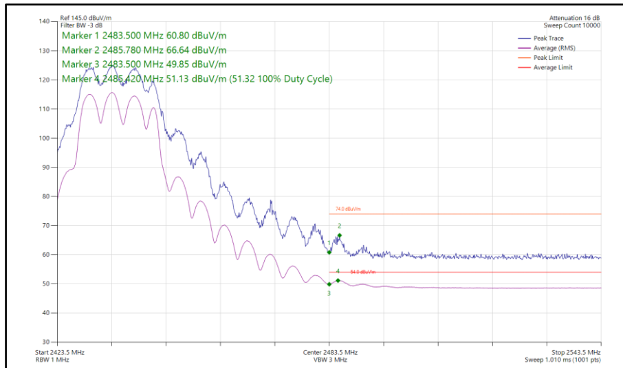
Figure 144 - 802.11g, CDD, Core 0-1 - 2437 MHz Band Edge Frequency 2483.5 MHz
