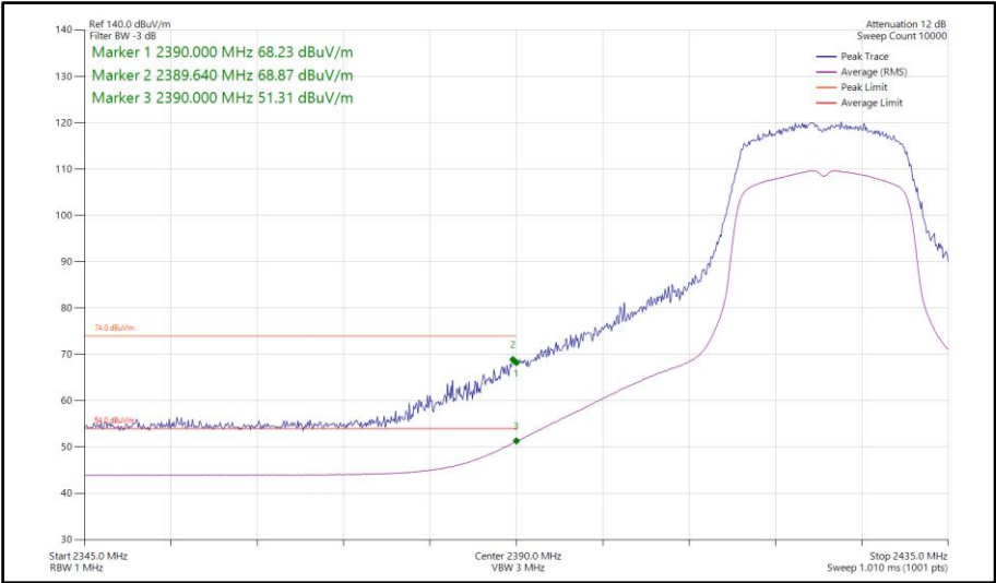
Figure 180 - 802.11n HT20, SDM, Core 0-1 - 2422 MHz Band Edge Frequency 2390 MHz
