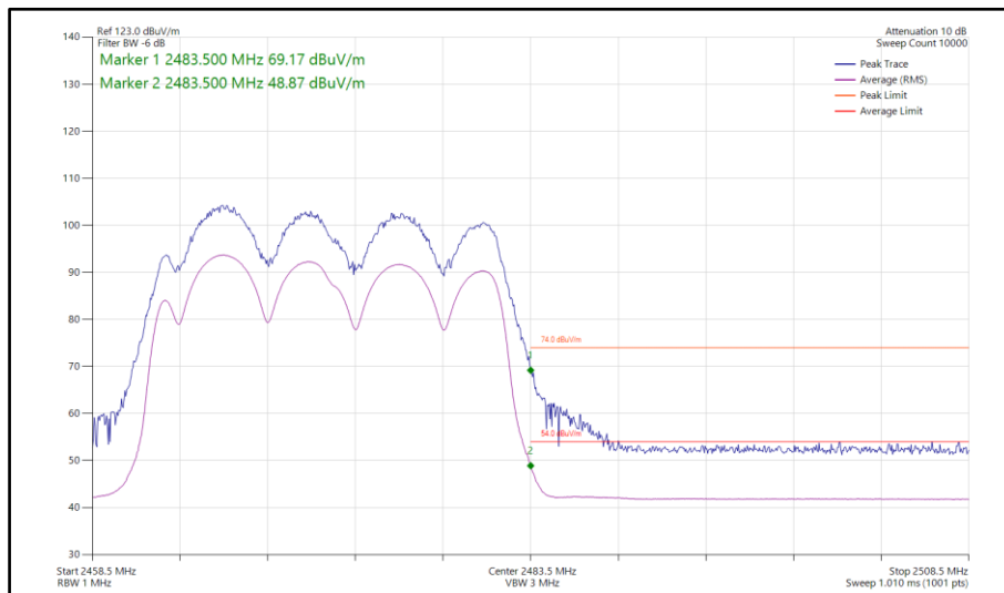
Figure 171 - 802.11ax HE20, SU, CDD, Core 0-1 - 2472 MHz Band Edge Frequency 2483.5 MHz
