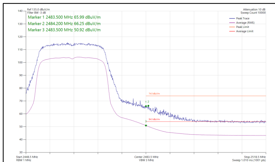
Figure 207 - 802.11ax HE20, SU, SDM, Core 0-1 - 2462 MHz Band Edge Frequency 2483.5 MHz
