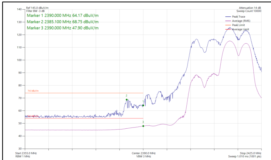
Figure 184 - 802.11ax HE20, RU106-54, SDM, Core 0-1 - 2412 MHz Band Edge Frequency 2390 MHz
