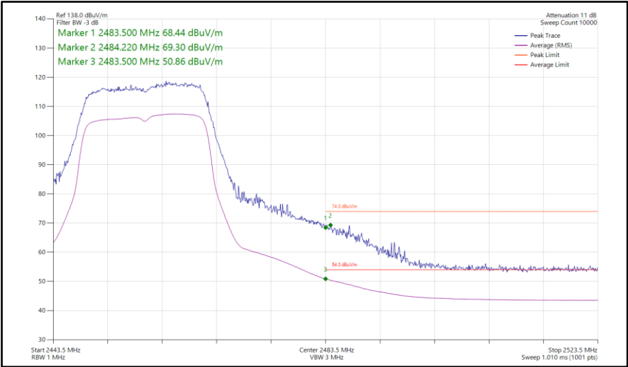
Figure 196 - 802.11n HT20, SDM, Core 0-1 - 2457 MHz Band Edge Frequency 2483.5 MHz
