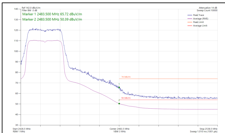
Figure 201 - 802.11ax HE20, SU, SDM, Core 0-1 - 2442 MHz Band Edge Frequency 2483.5 MHz
