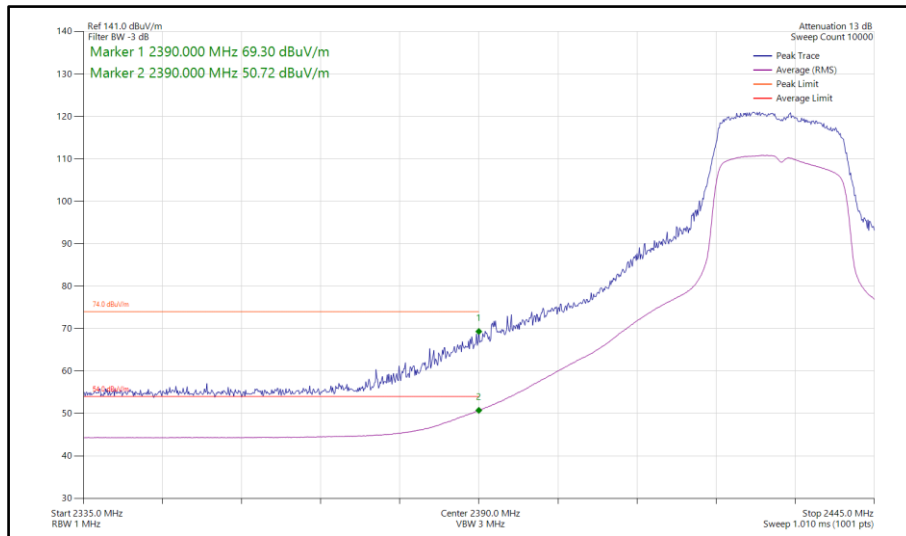
Figure 182 - 802.11n HT20, SDM, Core 0-1 - 2432 MHz Band Edge Frequency 2390 MHz
