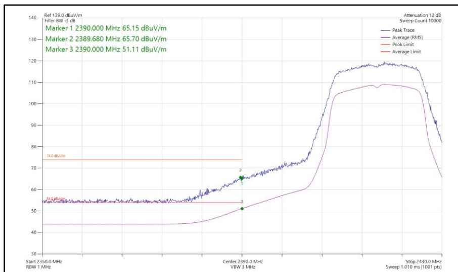
Figure 179 - 802.11n HT20, SDM, Core 0-1 - 2417 MHz Band Edge Frequency 2390 MHz
