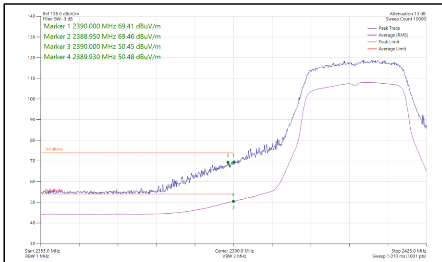
Figure 178 - 802.11n HT20, SDM, Core 0-1 - 2412 MHz Band Edge Frequency 2390 MHz
