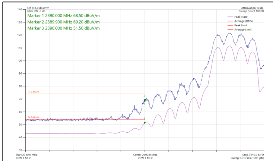
Figure 140 - 802.11ax HE20, SU, CDD, Core 0-1 - 2427 MHz Band Edge Frequency 2390 MHz
