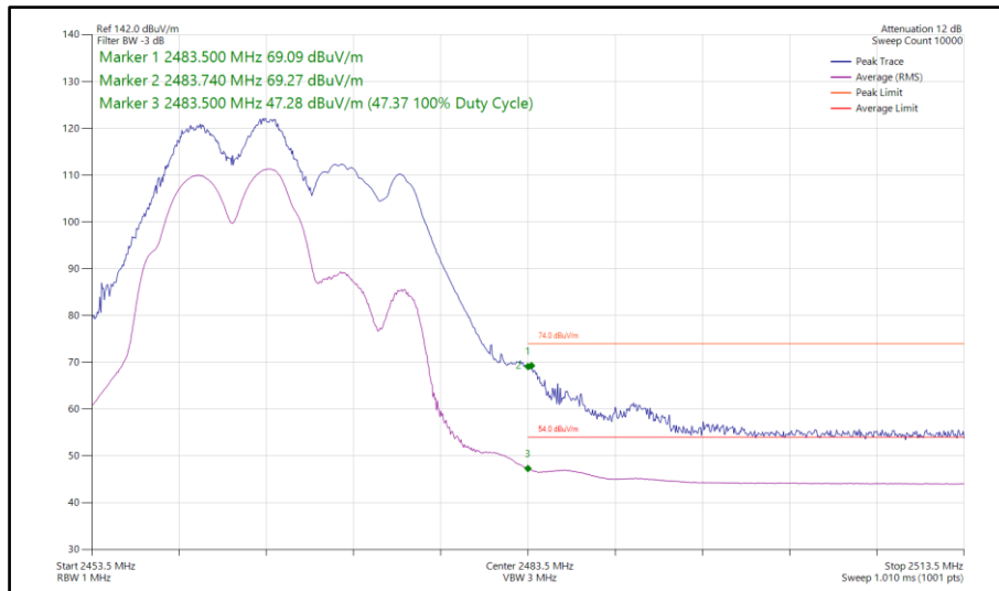
Figure 176 - 802.11be EHT20, RU106+26-82, CDD, Core 0-1 - 2467 MHz Band Edge Frequency 2483.5 MHz
