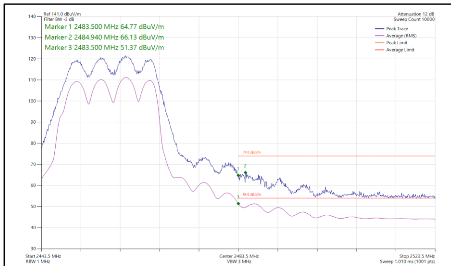
Figure 165 - 802.11ax HE20, SU, CDD, Core 0-1 - 2457 MHz Band Edge Frequency 2483.5 MHz
