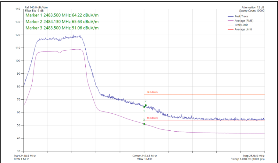
Figure 195 - 802.11n HT20, SDM, Core 0-1 - 2452 MHz Band Edge Frequency 2483.5 MHz
