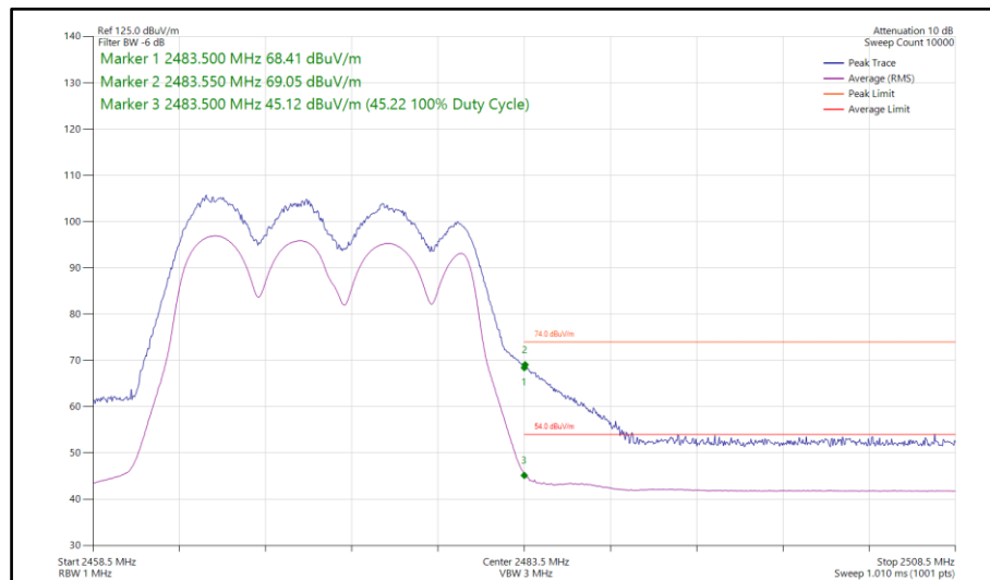
Figure 151 - 802.11g, CDD, Core 0-1 - 2472 MHz Band Edge Frequency 2483.5 MHz
