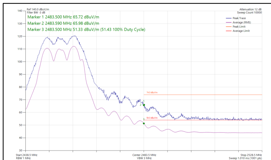
Figure 147 - 802.11g, CDD, Core 0-1 - 2452 MHz Band Edge Frequency 2483.5 MHz
