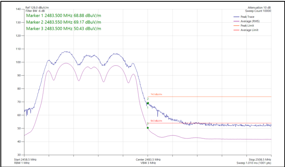
Figure 159 - 802.11n HT20, CDD, Core 0-1 - 2472 MHz Band Edge Frequency 2483.5 MHz
