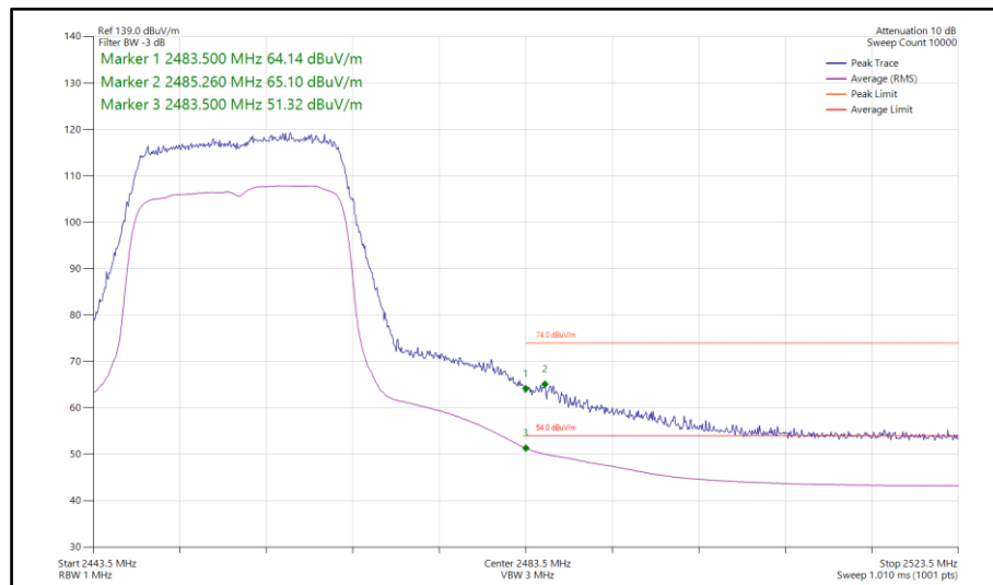
Figure 205 - 802.11ax HE20, SU, SDM, Core 0-1 - 2457 MHz Band Edge Frequency 2483.5 MHz
