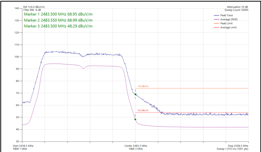
Figure 199 - 802.11n HT20, SDM, Core 0-1 - 2472 MHz Band Edge Frequency 2483.5 MHz
