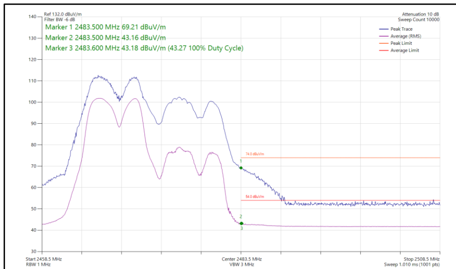
Figure 177 - 802.11be EHT20, RU52+26-70, CDD, Core 0-1 - 2472 MHz Band Edge Frequency 2483.5 MHz
