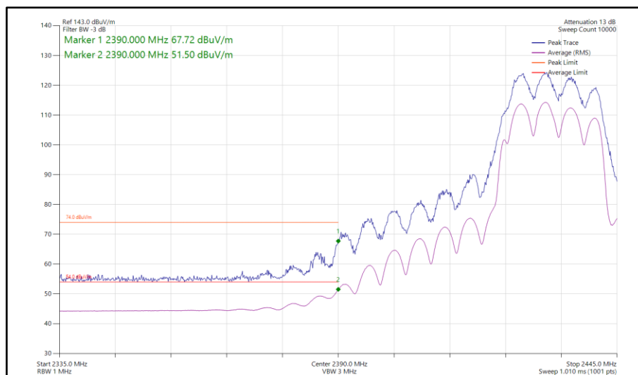
Figure 141 - 802.11ax HE20, SU, CDD, Core 0-1 - 2432 MHz Band Edge Frequency 2390 MHz
