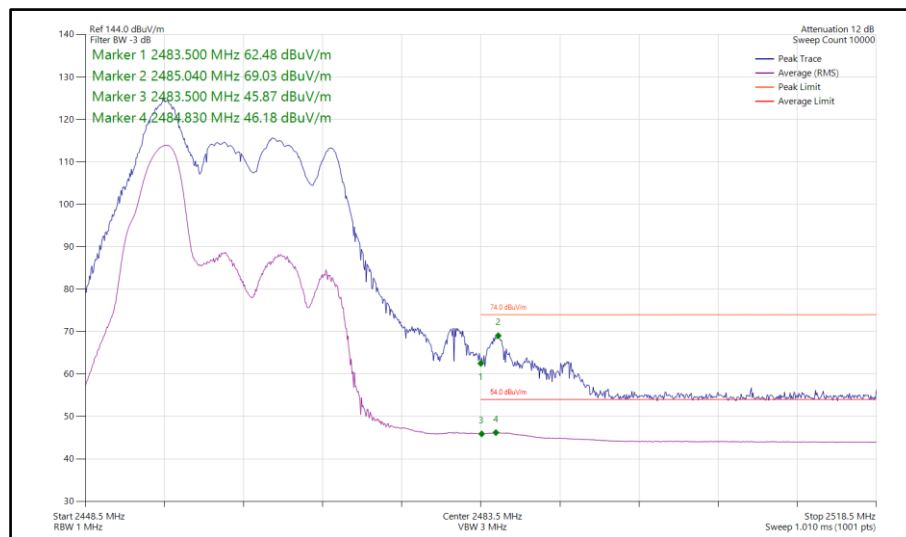
Figure 168 - 802.11ax HE20, RU52-37, CDD, Core 0-1 - 2462 MHz Band Edge Frequency 2483.5 MHz
