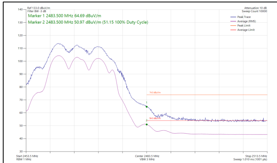
Figure 150 - 802.11g, CDD, Core 0-1 - 2467 MHz Band Edge Frequency 2483.5 MHz
