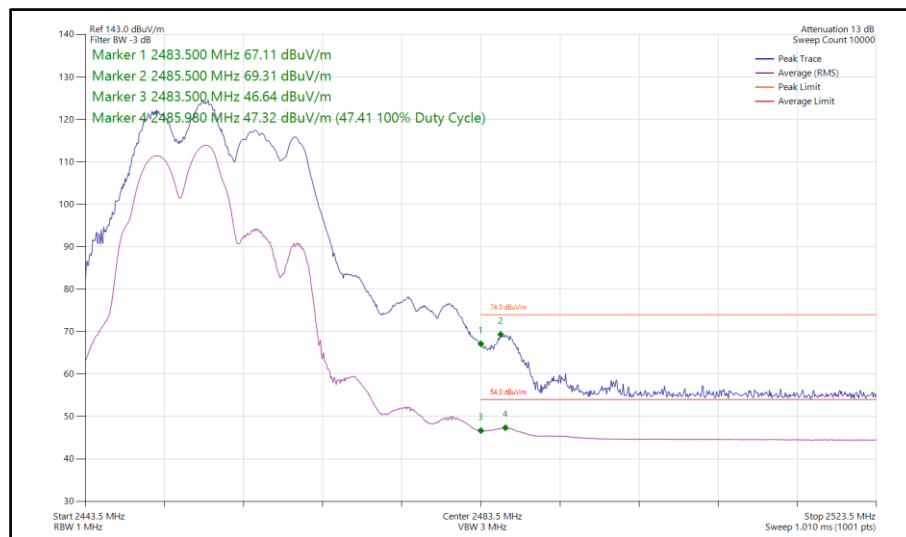
Figure 174 - 802.11be EHT20, RU106+26-82, CDD, Core 0-1 - 2457 MHz Band Edge Frequency 2483.5 MHz
