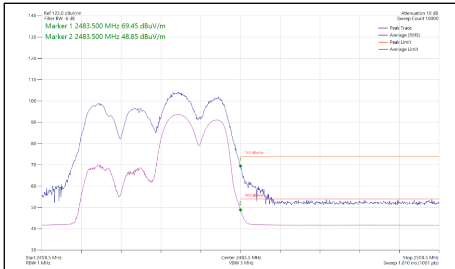
Figure 172 - 802.11ax HE20, RU106-54, CDD, Core 0-1 - 2472 MHz Band Edge Frequency 2483.5 MHz
