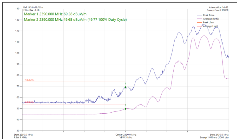
Figure 143 - 802.11be EHT20, RU106+26-83, CDD, Core 0-1 - 2417 MHz Band Edge Frequency 2390 MHz
