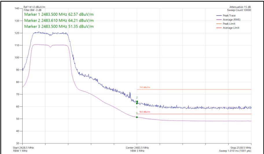
Figure 193 - 802.11n HT20, SDM, Core 0-1 - 2442 MHz Band Edge Frequency 2483.5 MHz
