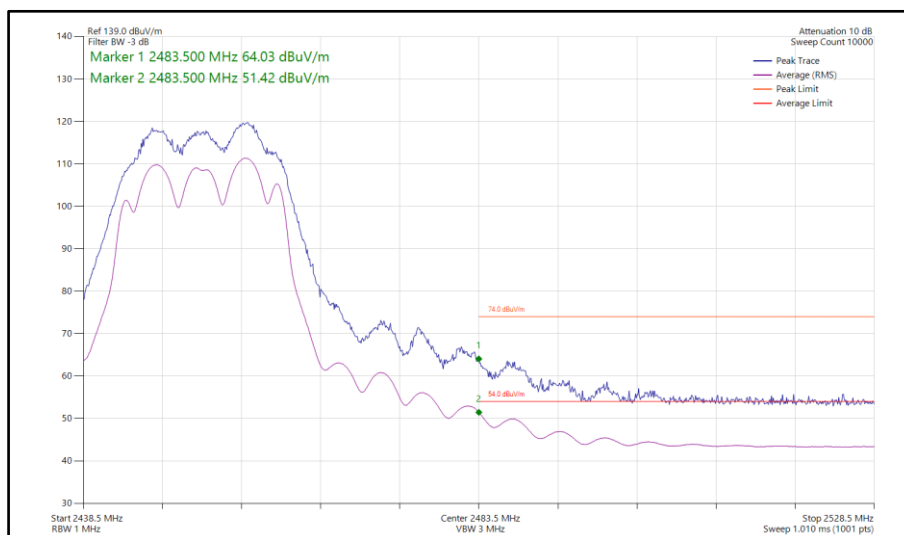
Figure 155 - 802.11n HT20, CDD, Core 0-1 - 2452 MHz Band Edge Frequency 2483.5 MHz
