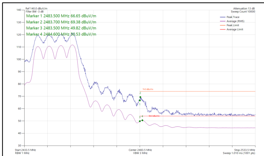
Figure 154 - 802.11n HT20, CDD, Core 0-1 - 2447 MHz Band Edge Frequency 2483.5 MHz
