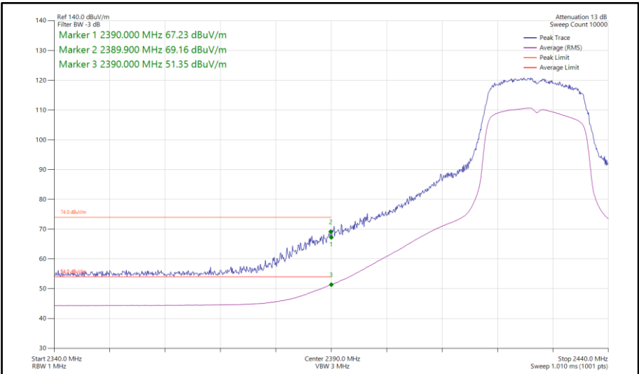
Figure 181 - 802.11n HT20, SDM, Core 0-1 - 2427 MHz Band Edge Frequency 2390 MHz
