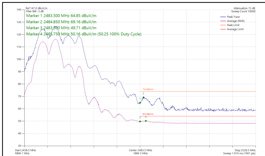
Figure 173 - 802.11be EHT20, RU106+26-82, CDD, Core 0-1 - 2452 MHz Band Edge Frequency 2483.5 MHz
