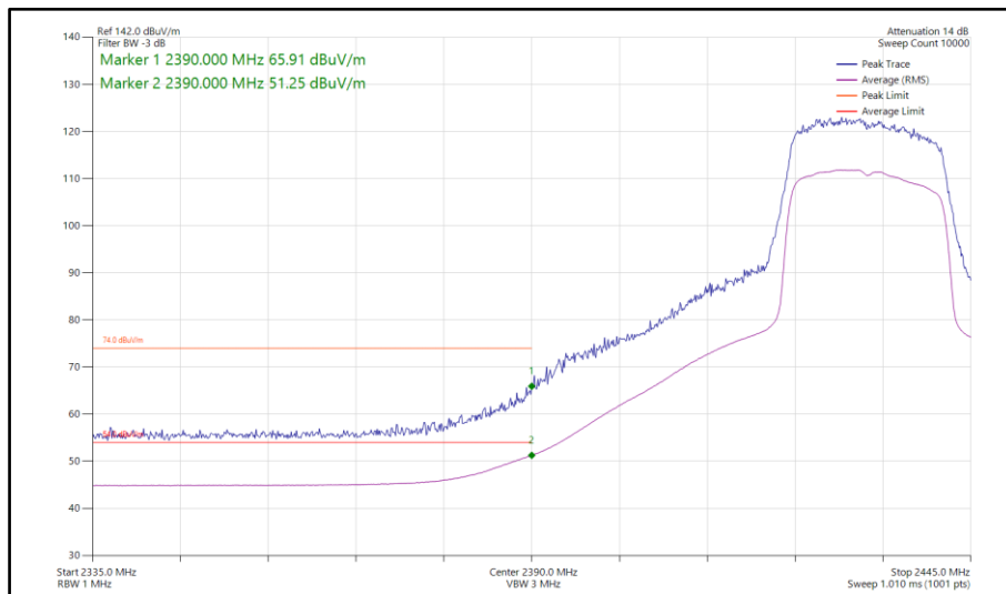
Figure 189 - 802.11ax HE20, SU, SDM, Core 0-1 - 2432 MHz Band Edge Frequency 2390 MHz
