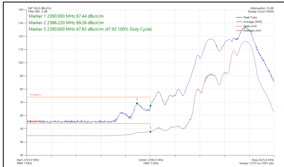
Figure 142 - 802.11be EHT20, RU52+26-72, CDD, Core 0-1 - 2412 MHz Band Edge Frequency 2390 MHz
