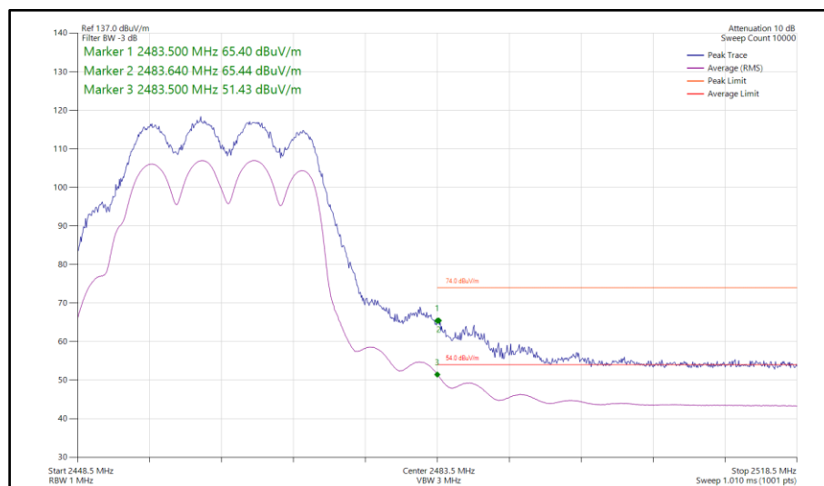
Figure 167 - 802.11ax HE20, SU, CDD, Core 0-1 - 2462 MHz Band Edge Frequency 2483.5 MHz
