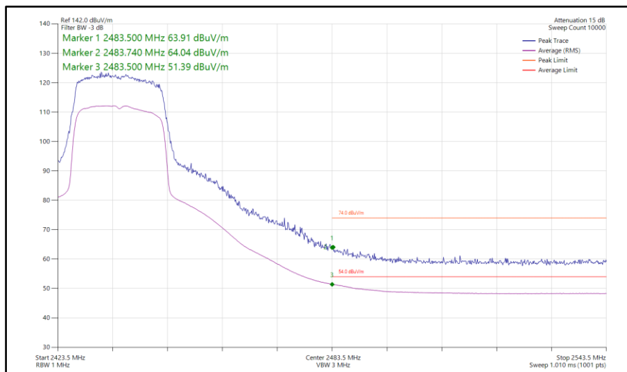
Figure 200 - 802.11ax HE20, SU, SDM, Core 0-1 - 2437 MHz Band Edge Frequency 2483.5 MHz
