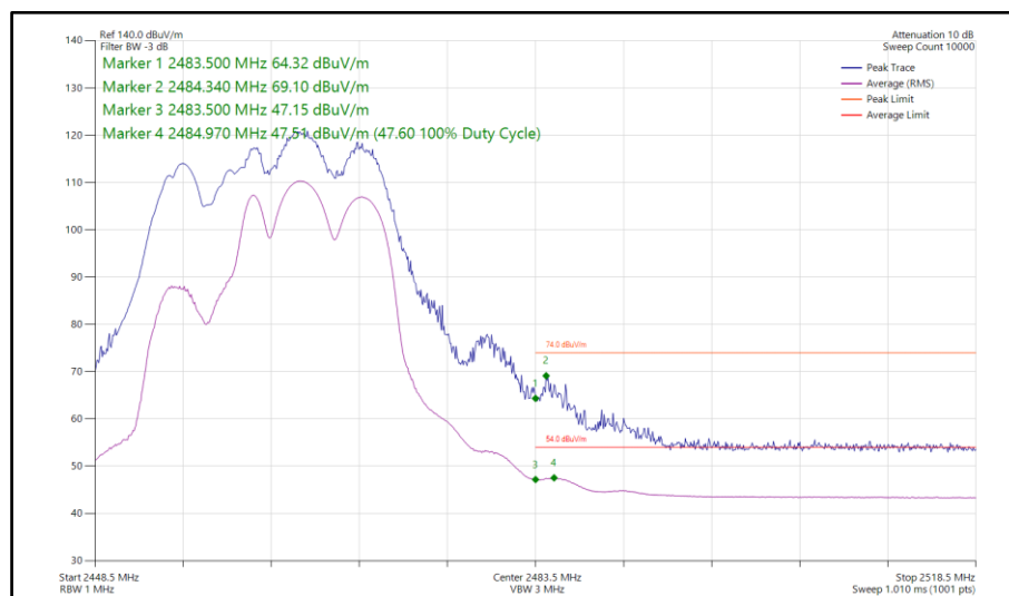
Figure 175 - 802.11be EHT20, RU106+26-83, CDD, Core 0-1 - 2462 MHz Band Edge Frequency 2483.5 MHz
