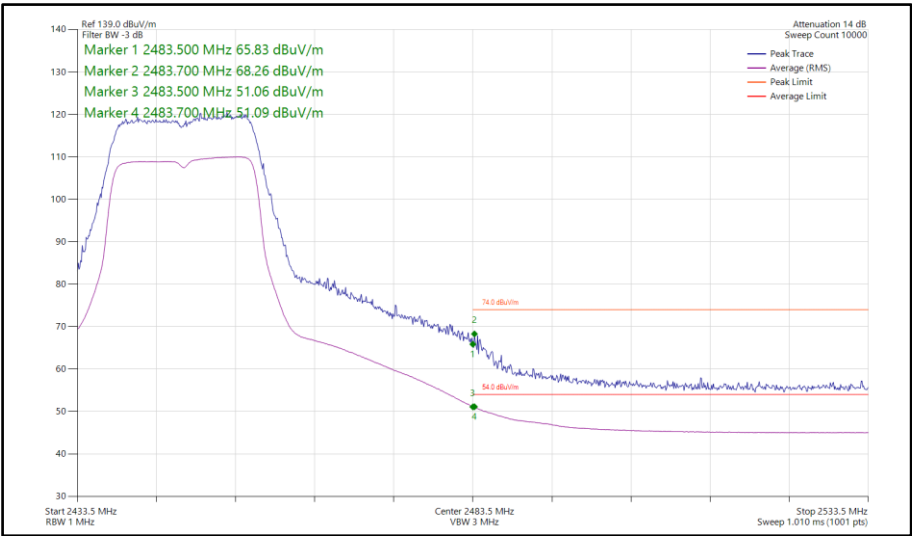
Figure 194 - 802.11n HT20, SDM, Core 0-1 - 2447 MHz Band Edge Frequency 2483.5 MHz
