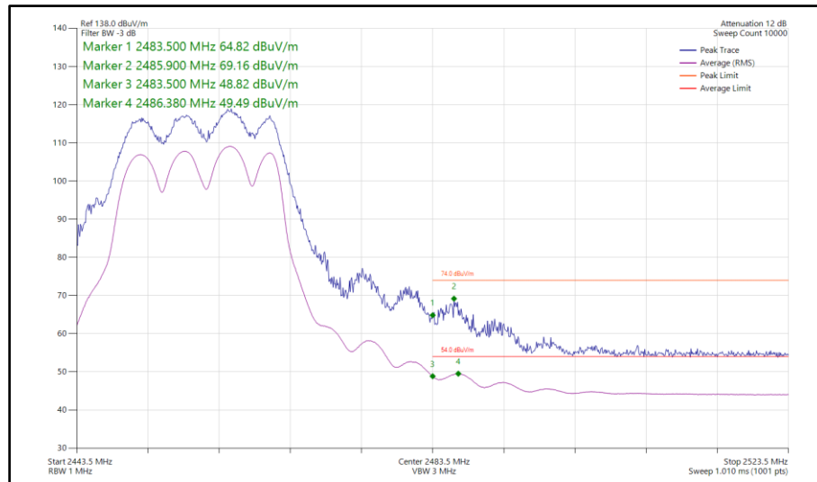
Figure 156 - 802.11n HT20, CDD, Core 0-1 - 2457 MHz Band Edge Frequency 2483.5 MHz
