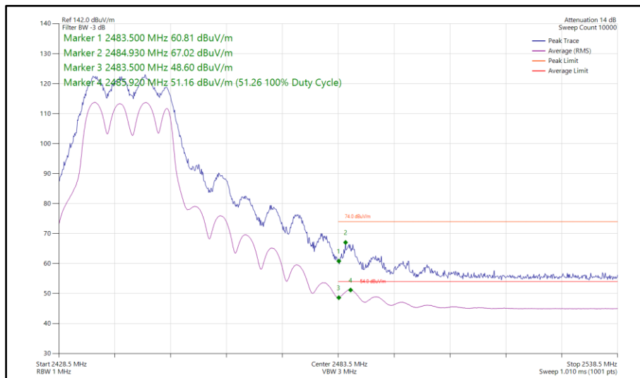
Figure 145 - 802.11g, CDD, Core 0-1 - 2442 MHz Band Edge Frequency 2483.5 MHz
