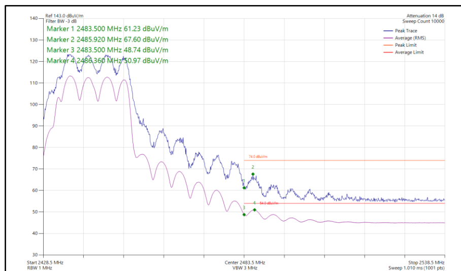
Figure 161 - 802.11ax HE20, SU, CDD, Core 0-1 - 2442 MHz Band Edge Frequency 2483.5 MHz
