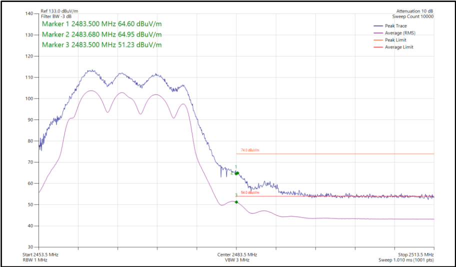
Figure 158 - 802.11n HT20, CDD, Core 0-1 - 2467 MHz Band Edge Frequency 2483.5 MHz
