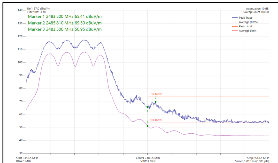
Figure 157 - 802.11n HT20, CDD, Core 0-1 - 2462 MHz Band Edge Frequency 2483.5 MHz
