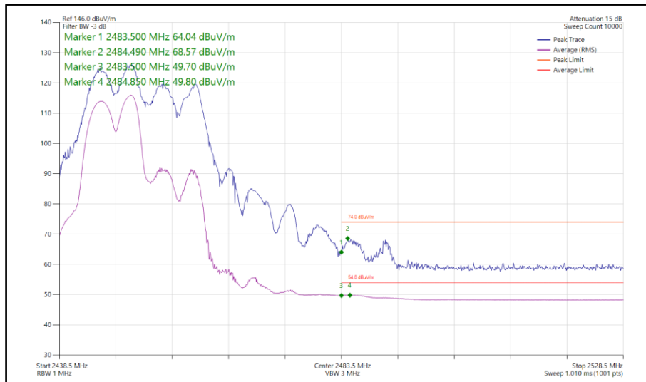
Figure 164 - 802.11ax HE20, RU106-53, CDD, Core 0-1 - 2452 MHz Band Edge Frequency 2483.5 MHz
