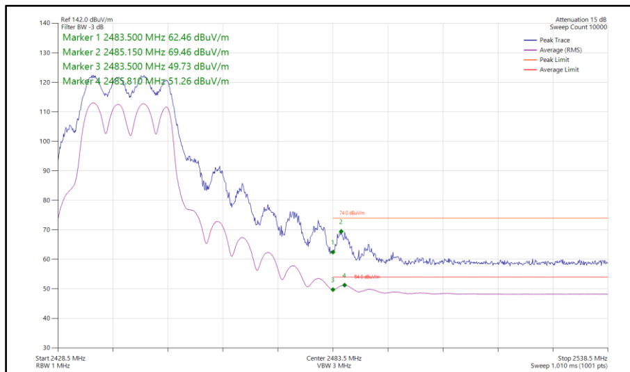
Figure 153 - 802.11n HT20, CDD, Core 0-1 - 2442 MHz Band Edge Frequency 2483.5 MHz
