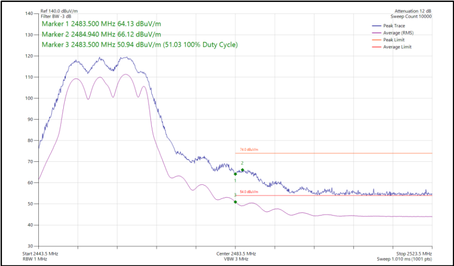
Figure 148 - 802.11g, CDD, Core 0-1 - 2457 MHz Band Edge Frequency 2483.5 MHz
