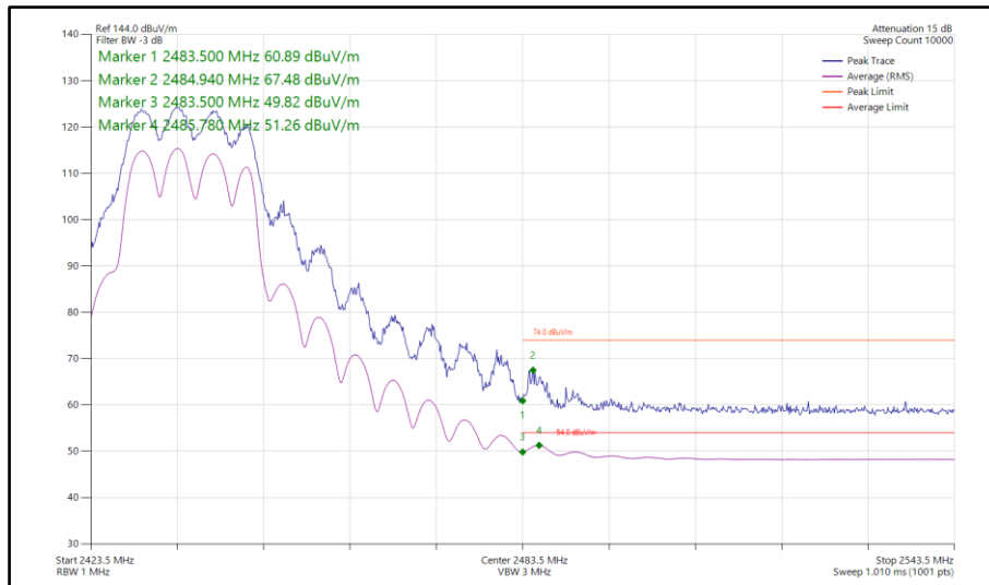
Figure 152 - 802.11n HT20, CDD, Core 0-1 - 2437 MHz Band Edge Frequency 2483.5 MHz
