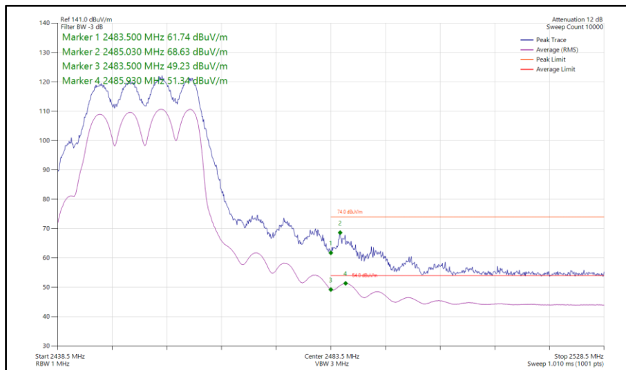
Figure 163 - 802.11ax HE20, SU, CDD, Core 0-1 - 2452 MHz Band Edge Frequency 2483.5 MHz
