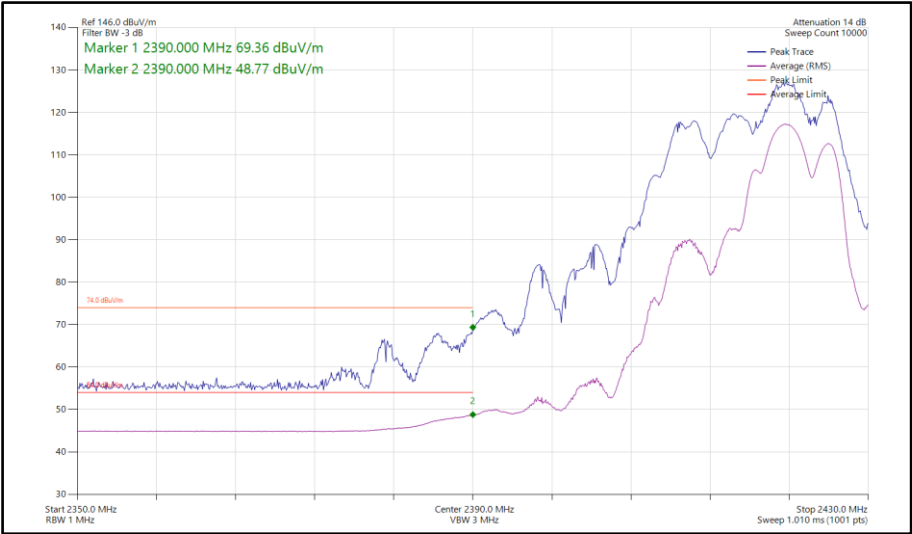
Figure 186 - 802.11ax HE20, RU106-54, SDM, Core 0-1 - 2417 MHz Band Edge Frequency 2390 MHz
