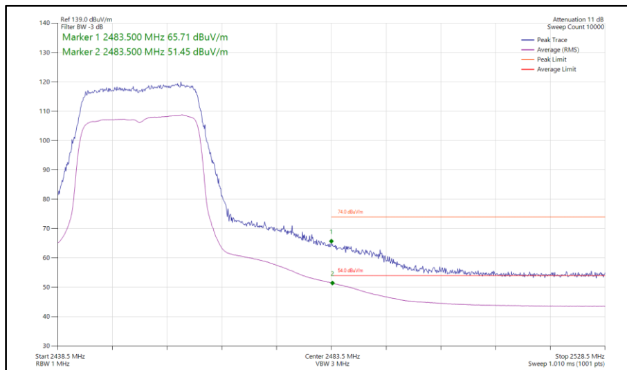
Figure 203 - 802.11ax HE20, SU, SDM, Core 0-1 - 2452 MHz Band Edge Frequency 2483.5 MHz
