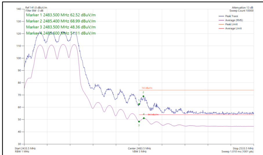
Figure 162 - 802.11ax HE20, SU, CDD, Core 0-1 - 2447 MHz Band Edge Frequency 2483.5 MHz
