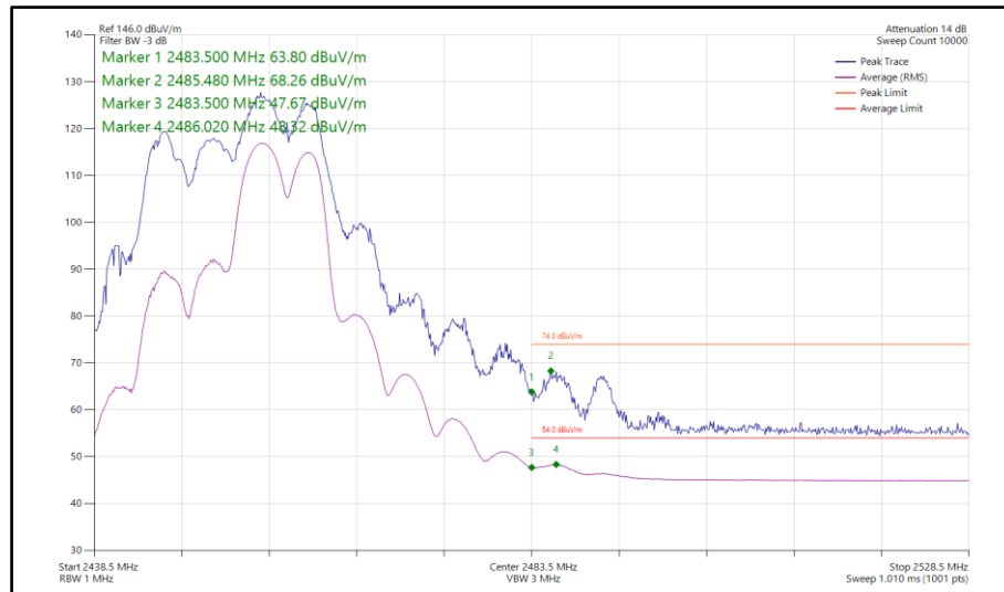
Figure 204 - 802.11ax HE20, RU106-54, SDM, Core 0-1 - 2452 MHz Band Edge Frequency 2483.5 MHz
