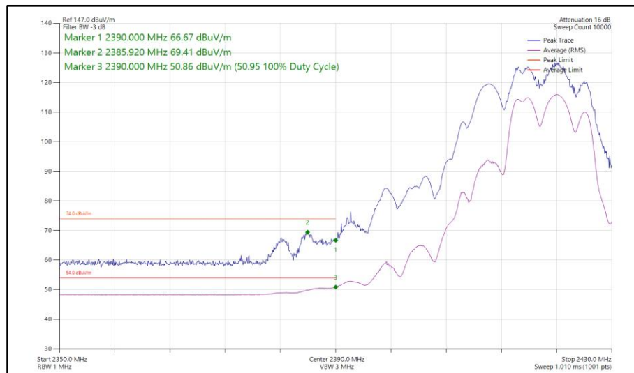
Figure 191 - 802.11be EHT20, RU106+26-83, SDM, Core 0-1 - 2417 MHz Band Edge Frequency 2390 MHz
