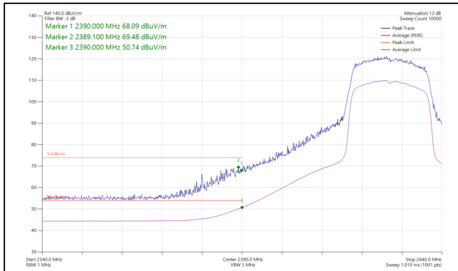
Figure 188 - 802.11ax HE20, SU, SDM, Core 0-1 - 2427 MHz Band Edge Frequency 2390 MHz
