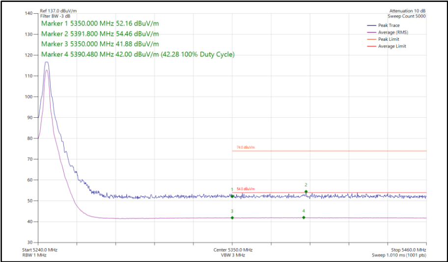
Figure 87 - Narrowband HDT4, MIMO, Core 0-1 - 5245 MHz Band Edge Frequency 5350 MHz
