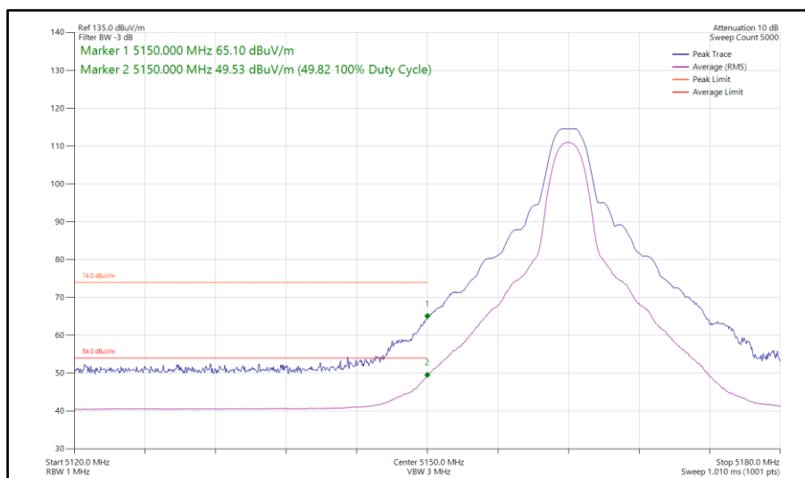
Figure 71 - Narrowband HDT4, MIMO, Core 0-1 - 5162 MHz Band Edge Frequency 5150 MHz
