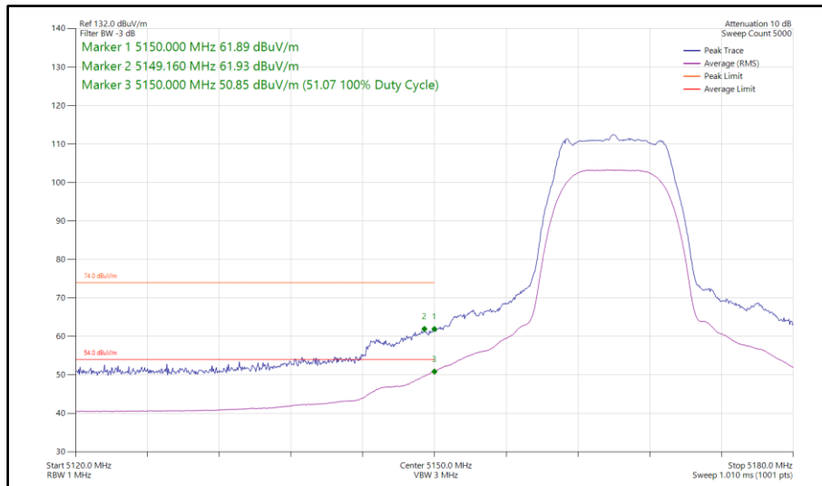
Figure 75 - Narrowband HDRPL8, MIMO, Core 0-1 - 5165 MHz Band Edge Frequency 5150 MHz
