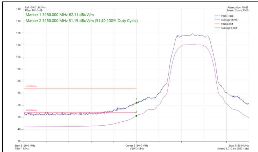
Figure 107 - Narrowband HDRPL8, SISO, Core 0 - 5165 MHz Band Edge Frequency 5150 MHz
