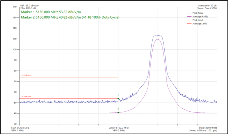
Figure 73 - Narrowband HDRPS2, MIMO, Core 0-1 - 5162 MHz Band Edge Frequency 5150 MHz
