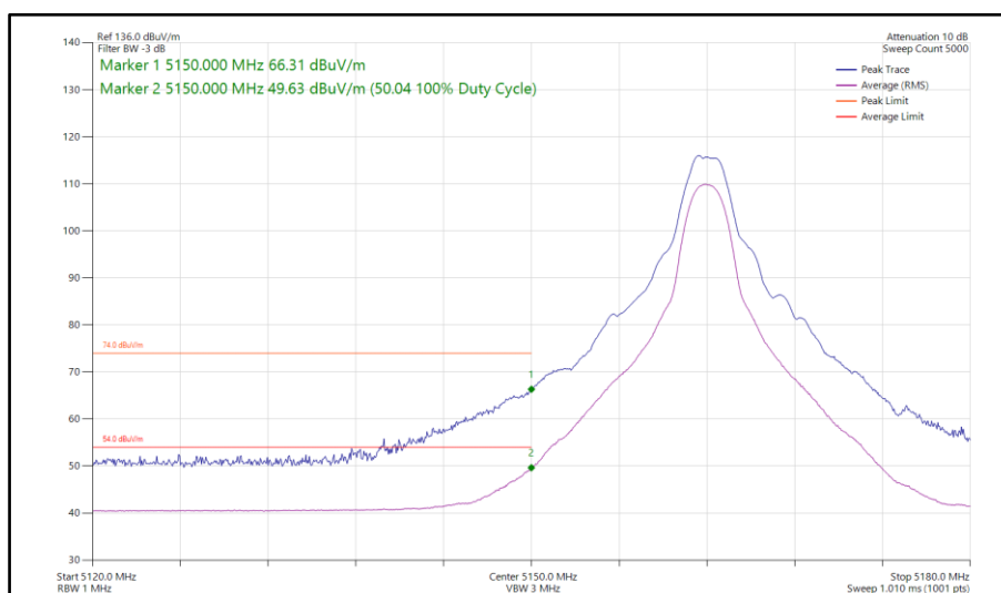
Figure 72 - Narrowband HDT6, MIMO, Core 0-1 - 5162 MHz Band Edge Frequency 5150 MHz
