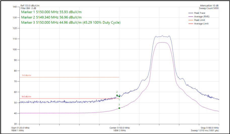
Figure 77 - Narrowband XHDRPM8, MIMO, Core 0-1 - 5163 MHz Band Edge Frequency 5150 MHz
