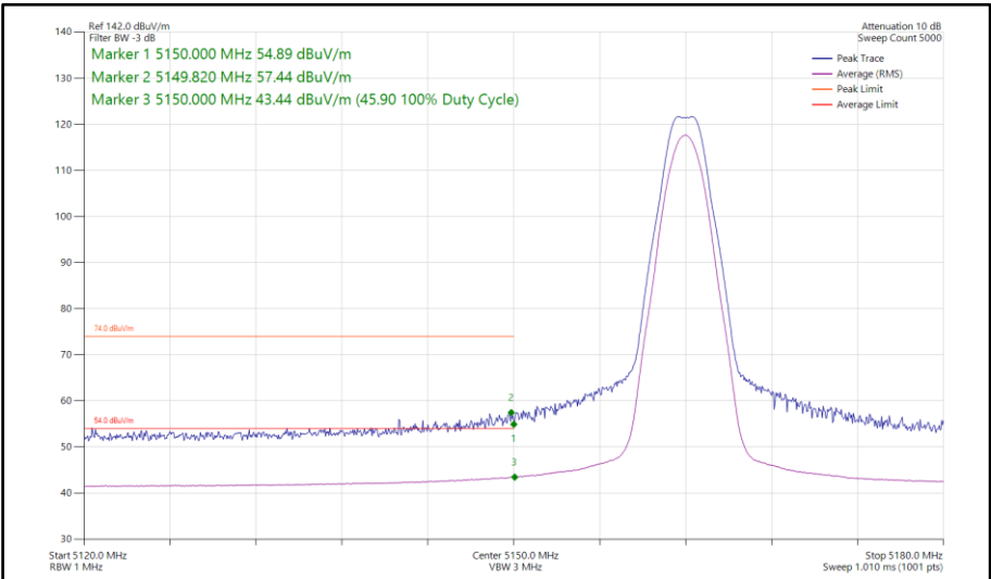
Figure 112 - Narrowband CS1LE2M, SISO, Core 0 - 5162 MHz Band Edge Frequency 5150 MHz
