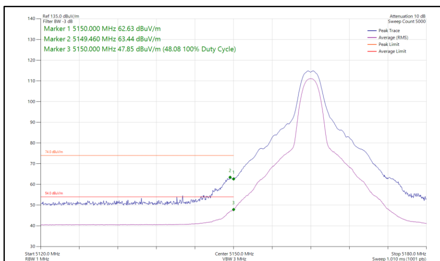
Figure 70 - Narrowband HDT3, MIMO, Core 0-1 - 5162 MHz Band Edge Frequency 5150 MHz
