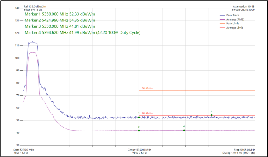
Figure 91 - Narrowband HDRPL8, MIMO, Core 0-1 - 5245 MHz Band Edge Frequency 5350 MHz
