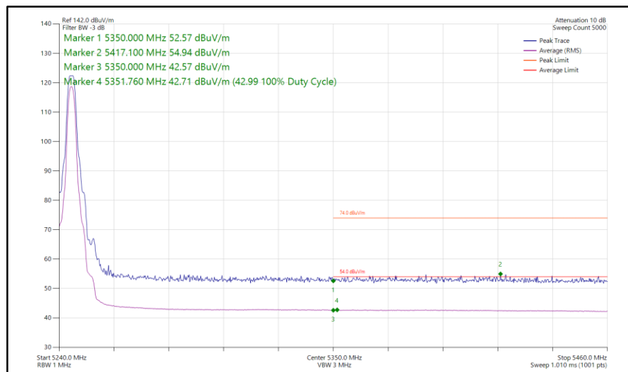
Figure 119 - Narrowband HDT4, SISO, Core 0 - 5245 MHz Band Edge Frequency 5350 MHz
