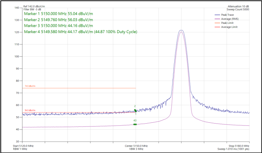
Figure 111 - Narrowband CS1LE1M, SISO, Core 0 - 5162 MHz Band Edge Frequency 5150 MHz
