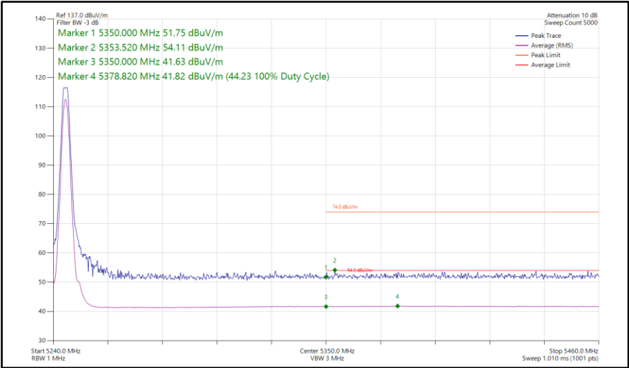
Figure 85 - Narrowband LE2M, MIMO, Core 0-1 - 5245 MHz Band Edge Frequency 5350 MHz
