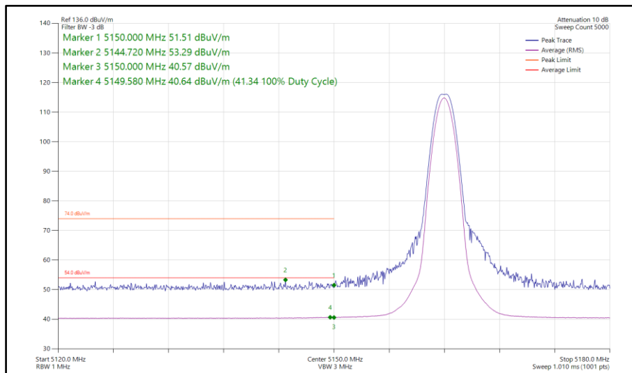
Figure 68 - Narrowband LE1M, MIMO, Core 0-1 - 5162 MHz Band Edge Frequency 5150 MHz
