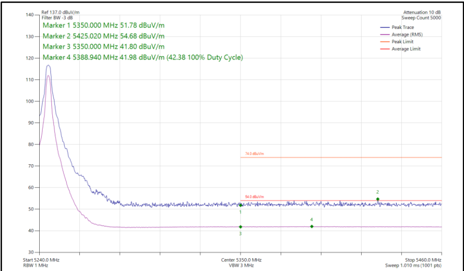
Figure 88 - Narrowband HDT6, MIMO, Core 0-1 - 5245 MHz Band Edge Frequency 5350 MHz
