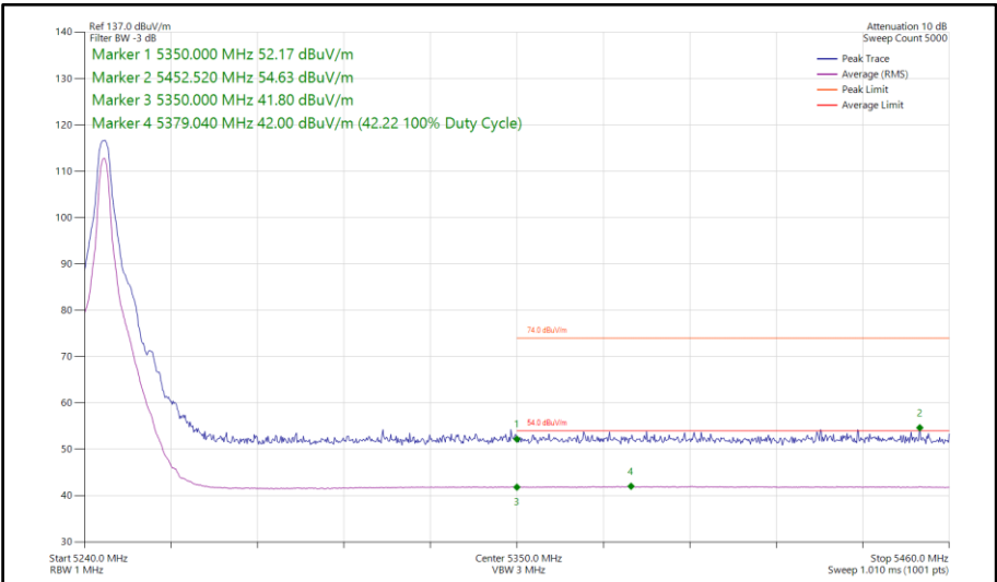
Figure 86 - Narrowband HDT3, MIMO, Core 0-1 - 5245 MHz Band Edge Frequency 5350 MHz
