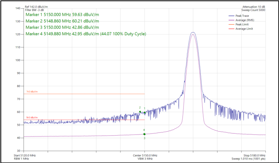
Figure 129 - Narrowband DH5, SISO, Core 1 - 5162 MHz Band Edge Frequency 5150 MHz
