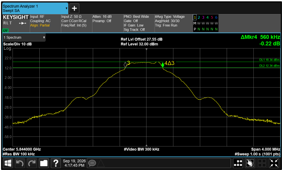
Figure 624 - Core 1 5844 MHz (CH119) 6 dB Bandwidth
