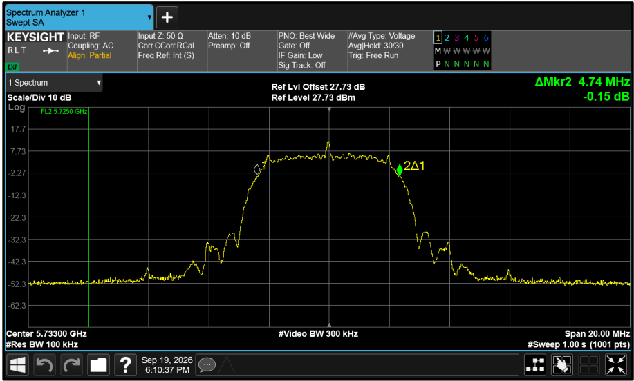
Figure 649 - Core 0 5733 MHz (CH8) 99% Bandwidth
