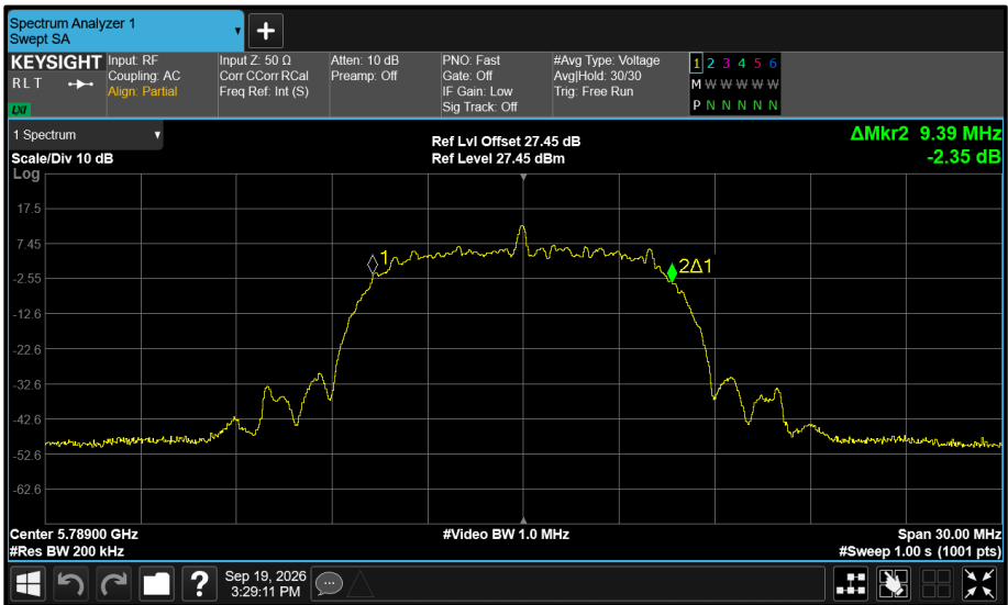
Figure 603 - Core 1 5789 MHz (CH64) 99% Bandwidth
