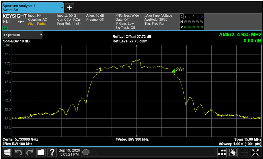
Figure 637 - Core 0 5733 MHz (CH8) 99% Bandwidth
