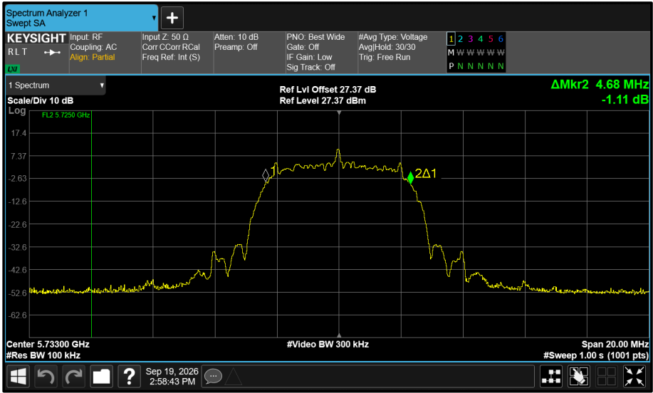
Figure 595 - Core 1 5733 MHz (CH8) 99% Bandwidth
