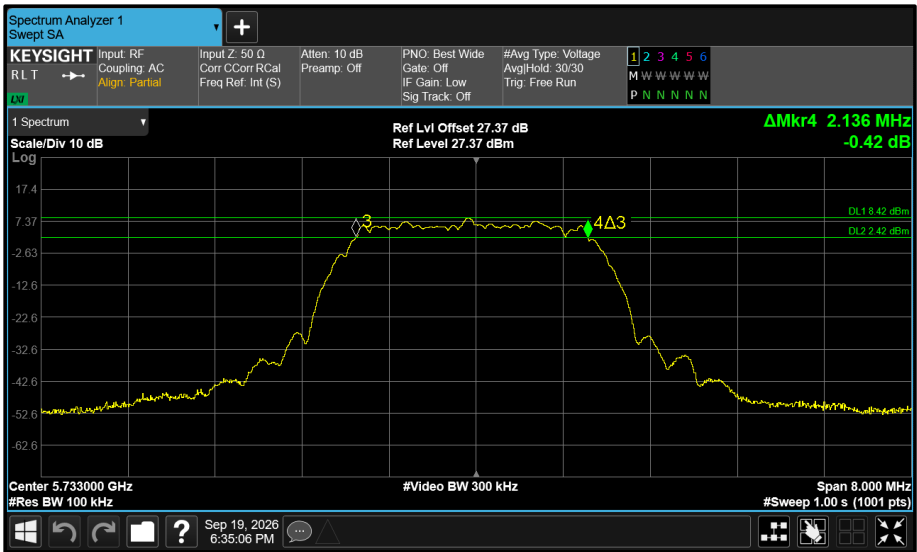
Figure 628 - Core 1 5733 MHz (CH8) 6 dB Bandwidth
