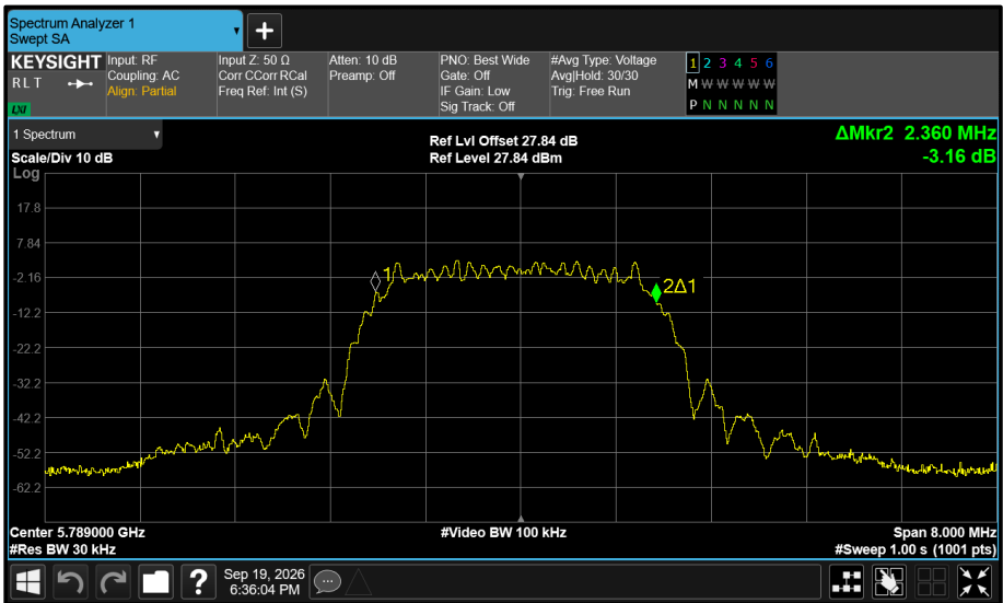
Figure 629 - Core 0 5789 MHz (CH64) 99% Bandwidth
