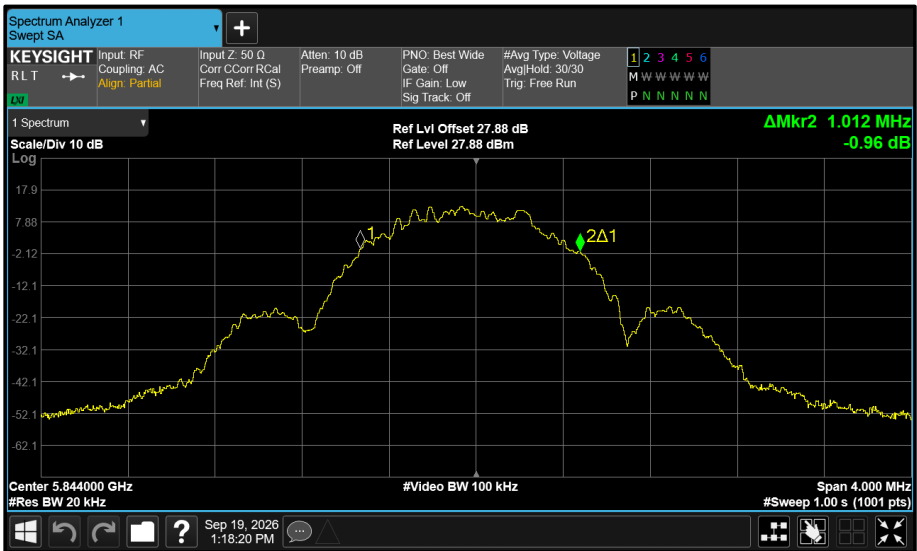
Figure 569 - Core 0 5844 MHz (CH119) 99% Bandwidth
