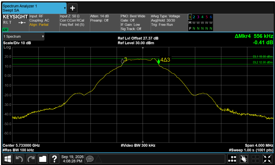
Figure 616 - Core 1 5733 MHz (CH8) 6 dB Bandwidth
