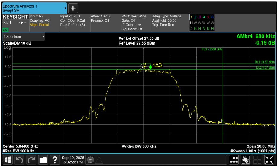
Figure 600 - Core 1 5844 MHz (CH119) 6 dB Bandwidth
