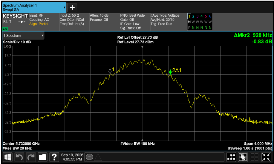
Figure 613 - Core 0 5733 MHz (CH8) 99% Bandwidth
