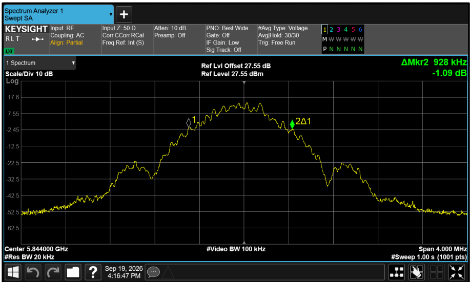
Figure 623 - Core 1 5844 MHz (CH119) 99% Bandwidth
