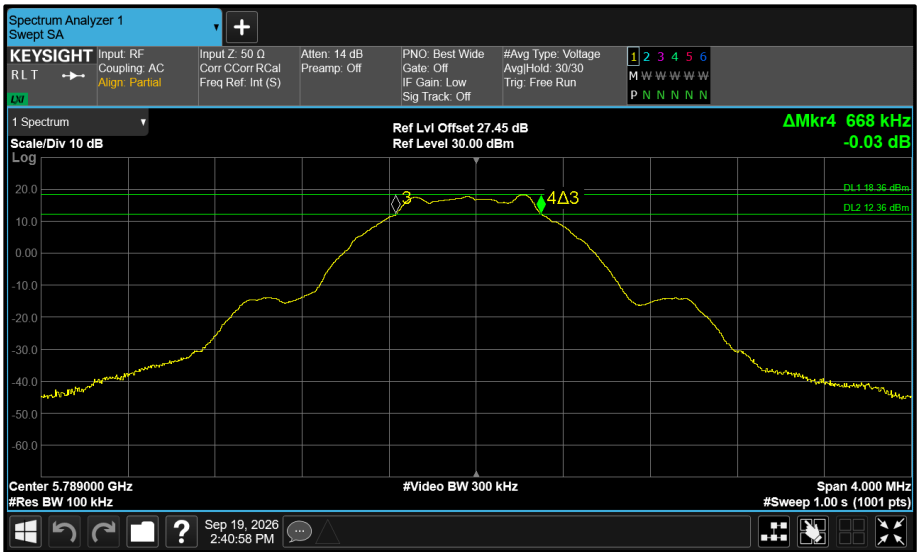
Figure 610 - Core 1 5789 MHz (CH64) 6 dB Bandwidth
