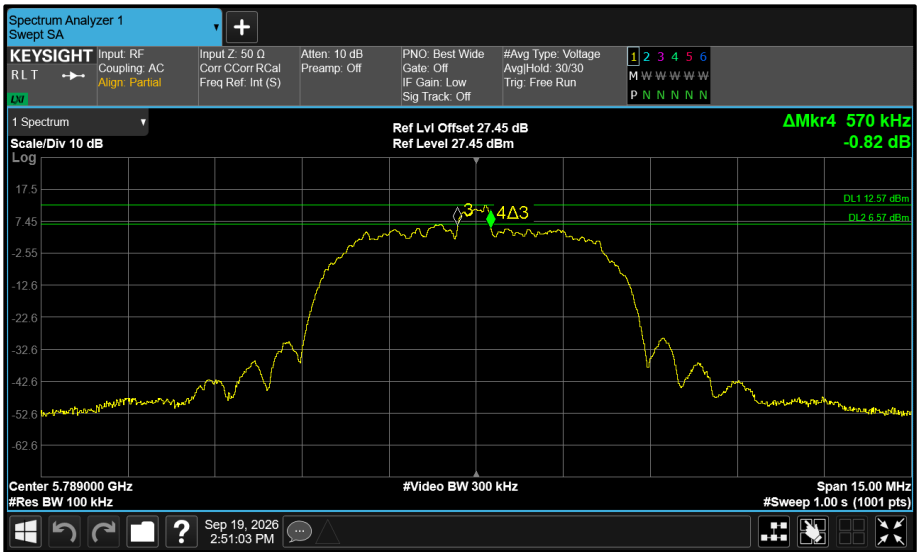
Figure 586 - Core 1 5789 MHz (CH64) 6 dB Bandwidth
