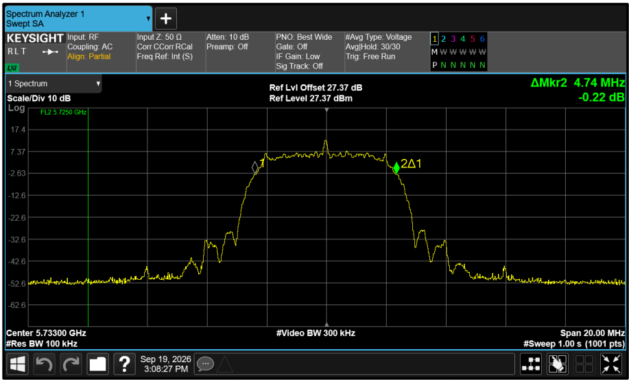
Figure 589 - Core 1 5733 MHz (CH8) 99% Bandwidth
