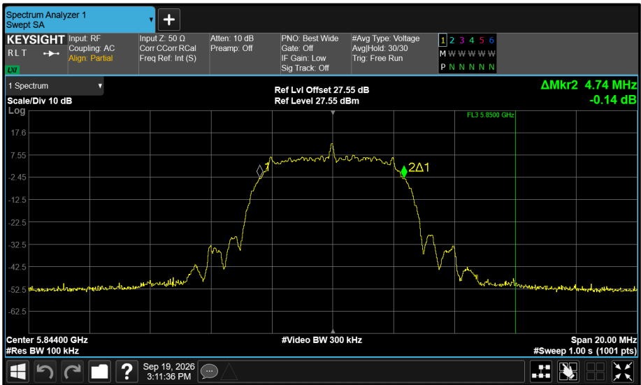
Figure 593 - Core 1 5844 MHz (CH119) 99% Bandwidth
