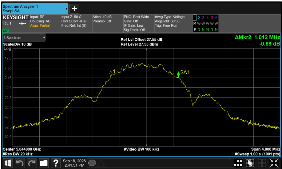
Figure 611 - Core 1 5844 MHz (CH119) 99% Bandwidth
