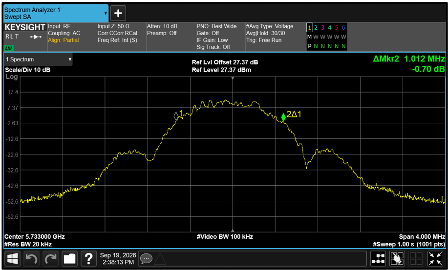
Figure 607 - Core 1 5733 MHz (CH8) 99% Bandwidth
