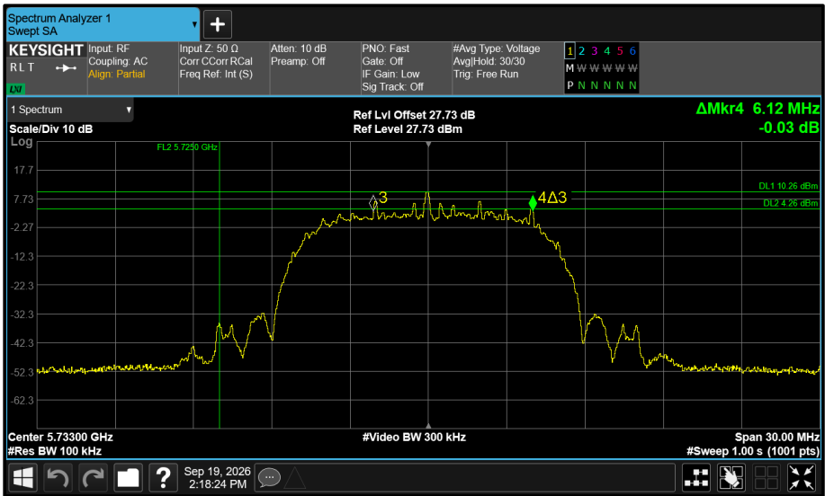
Figure 560 - Core 0 5733 MHz (CH8) 6 dB Bandwidth
