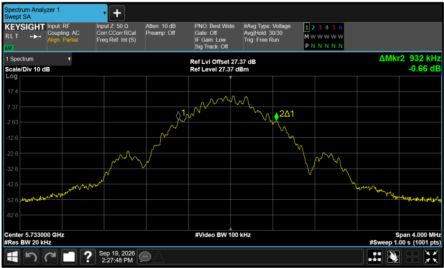
Figure 571 - Core 1 5733 MHz (CH8) 99% Bandwidth
