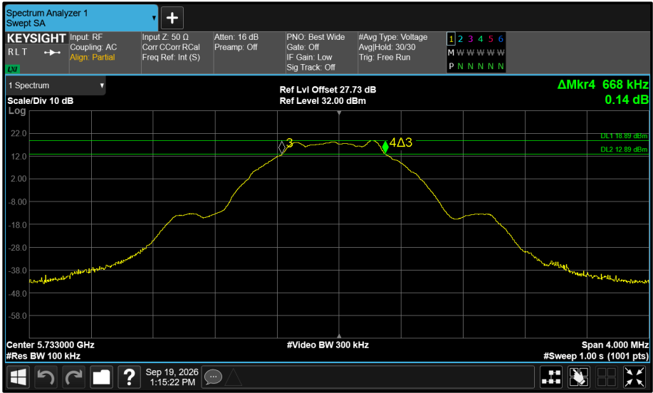
Figure 566 - Core 0 5733 MHz (CH8) 6 dB Bandwidth
