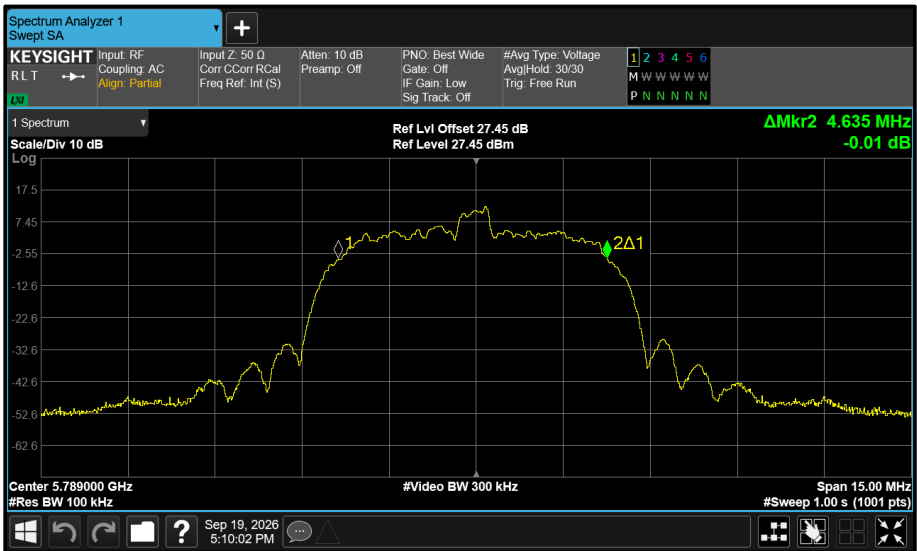
Figure 643 - Core 1 5789 MHz (CH64) 99% Bandwidth
