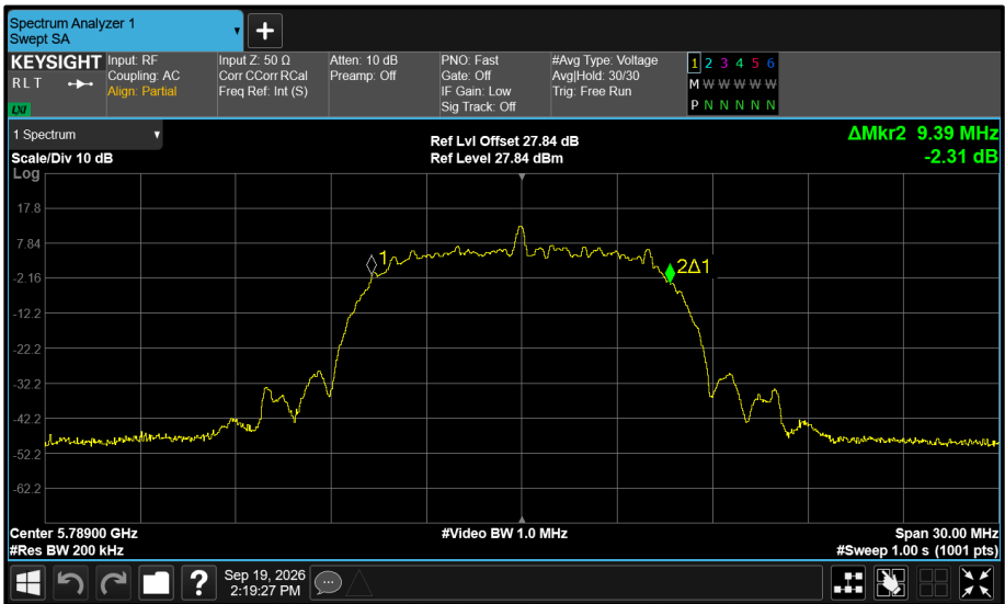
Figure 561 - Core 0 5789 MHz (CH64) 99% Bandwidth
