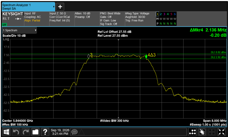
Figure 582 - Core 1 5844 MHz (CH119) 6 dB Bandwidth
