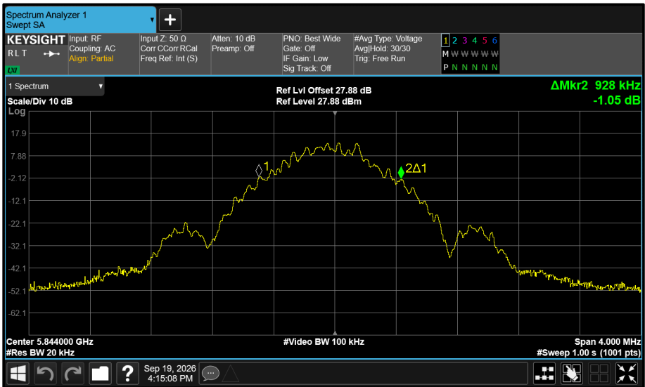
Figure 621 - Core 0 5844 MHz (CH119) 99% Bandwidth
