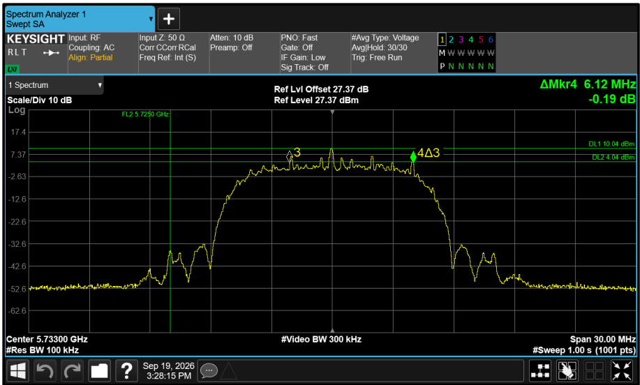
Figure 602 - Core 1 5733 MHz (CH8) 6 dB Bandwidth
