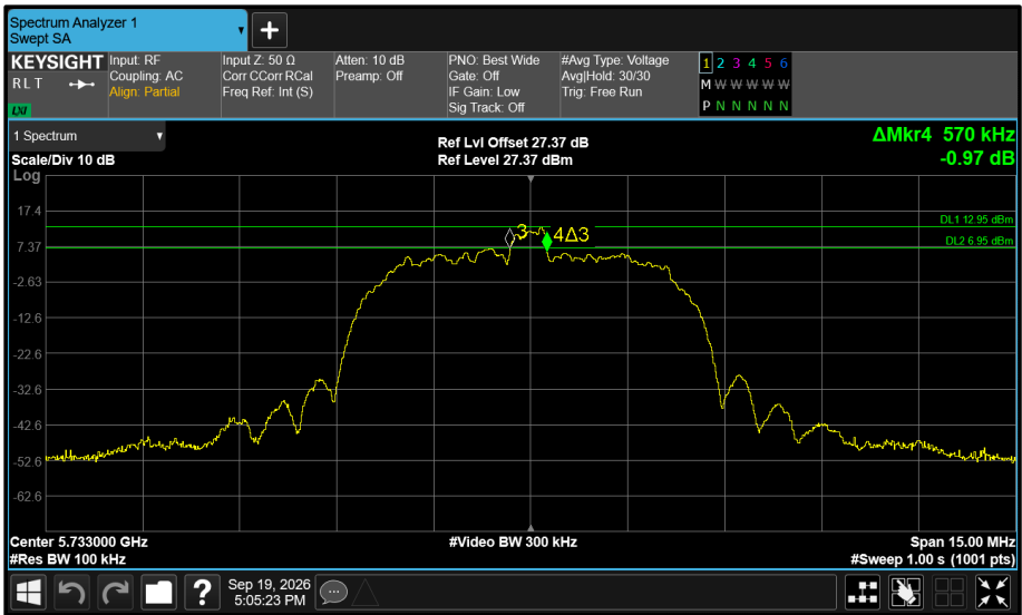
Figure 640 - Core 1 5733 MHz (CH8) 6 dB Bandwidth
