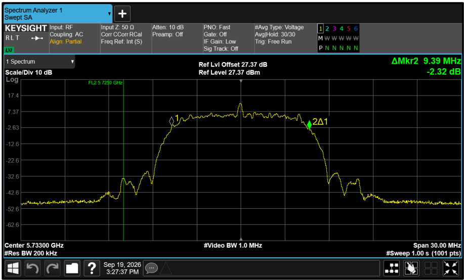
Figure 601 - Core 1 5733 MHz (CH8) 99% Bandwidth
