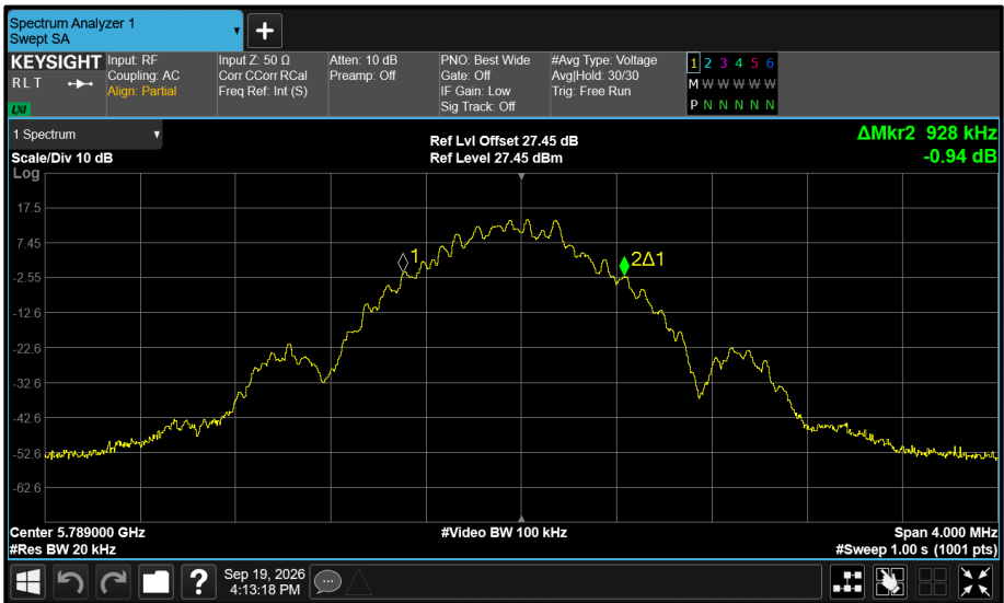
Figure 619 - Core 1 5789 MHz (CH64) 99% Bandwidth
