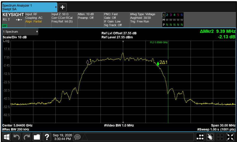
Figure 605 - Core 1 5844 MHz (CH119) 99% Bandwidth
