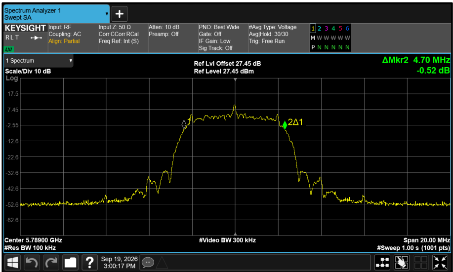
Figure 597 - Core 1 5789 MHz (CH64) 99% Bandwidth
