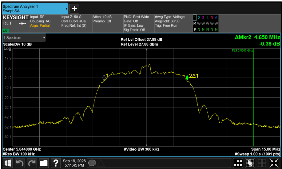
Figure 645 - Core 0 5844 MHz (CH119) 99% Bandwidth
