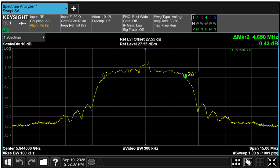
Figure 587 - Core 1 5844 MHz (CH119) 99% Bandwidth
