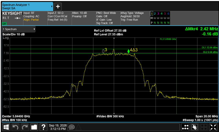
Figure 594 - Core 1 5844 MHz (CH119) 6 dB Bandwidth
