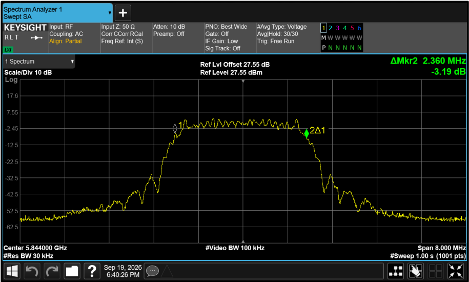
Figure 635 - Core 1 5844 MHz (CH119) 99% Bandwidth
