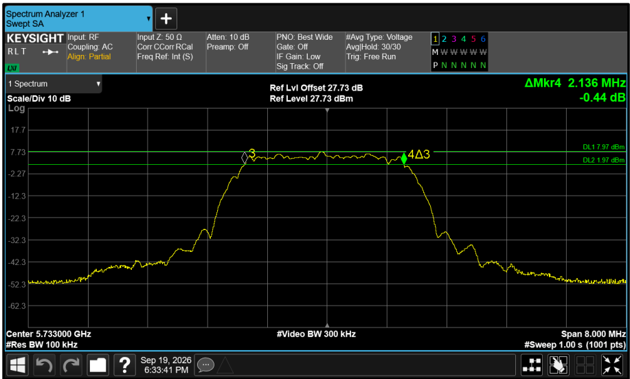
Figure 626 - Core 0 5733 MHz (CH8) 6 dB Bandwidth
