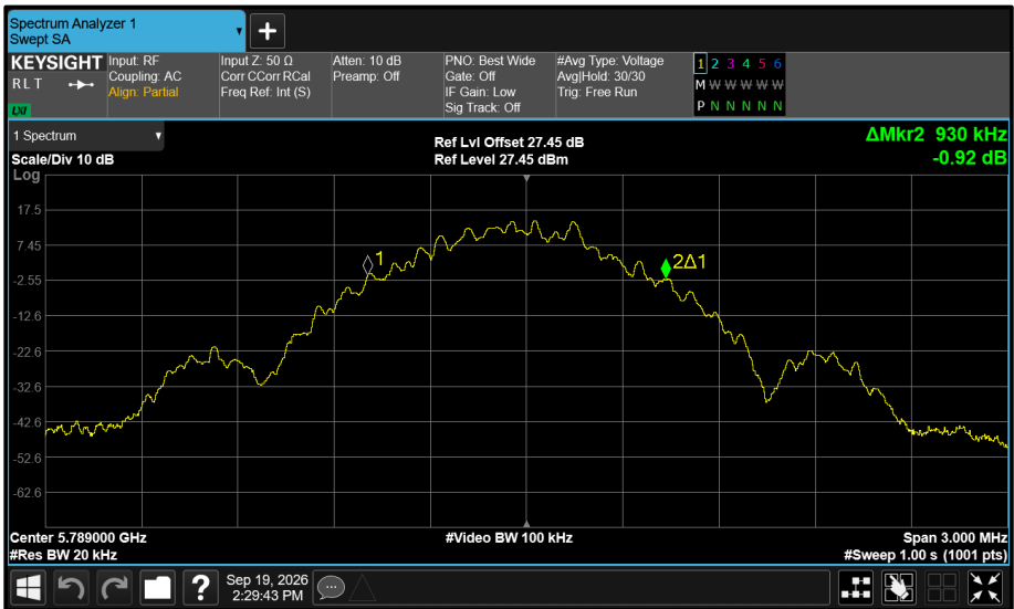
Figure 573 - Core 1 5789 MHz (CH64) 99% Bandwidth
