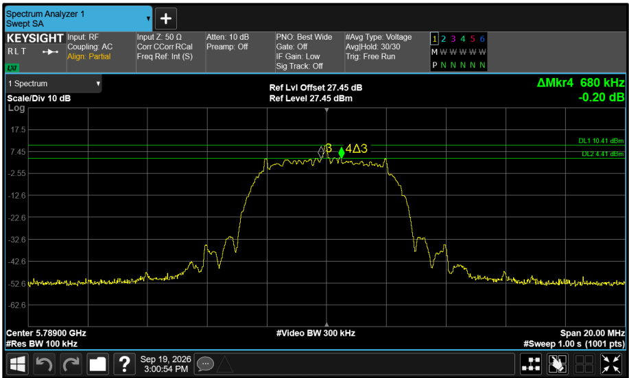
Figure 598 - Core 1 5789 MHz (CH64) 6 dB Bandwidth
