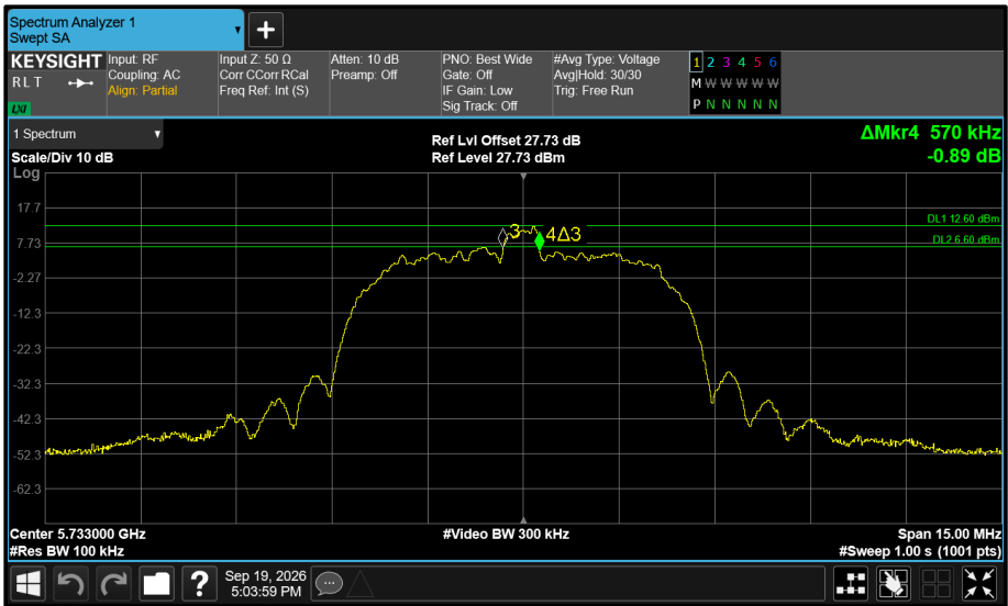
Figure 638 - Core 0 5733 MHz (CH8) 6 dB Bandwidth
