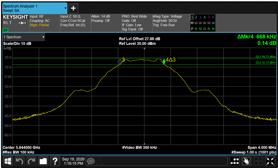
Figure 570 - Core 0 5844 MHz (CH119) 6 dB Bandwidth
