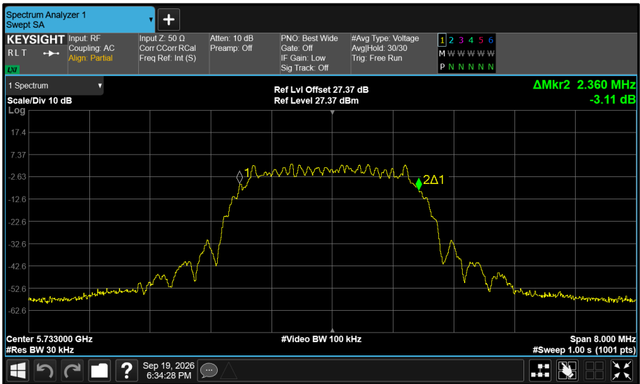
Figure 627 - Core 1 5733 MHz (CH8) 99% Bandwidth
