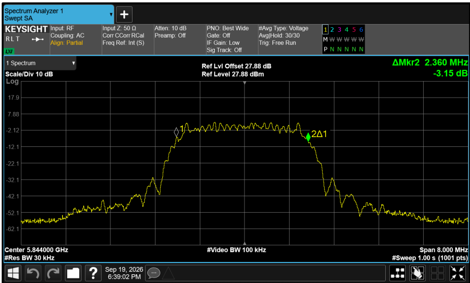
Figure 633 - Core 0 5844 MHz (CH119) 99% Bandwidth
