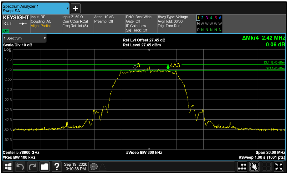
Figure 592 - Core 1 5789 MHz (CH64) 6 dB Bandwidth
