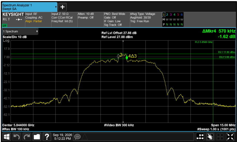
Figure 646 - Core 0 5844 MHz (CH119) 6 dB Bandwidth
