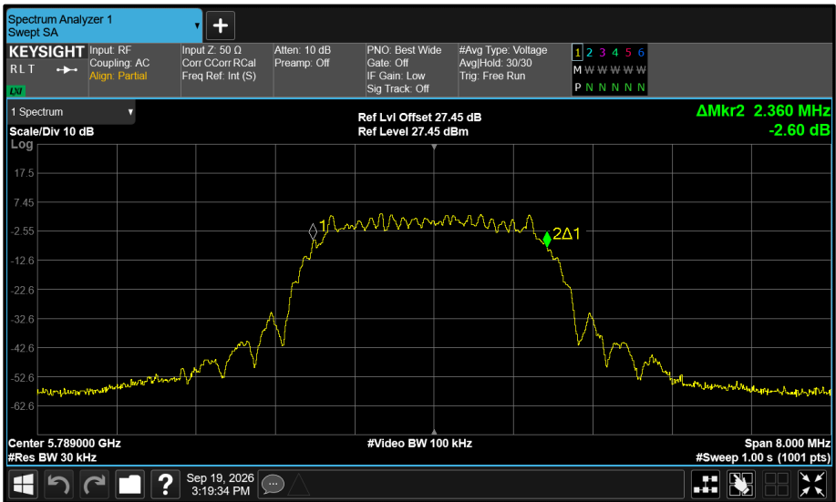
Figure 579 - Core 1 5789 MHz (CH64) 99% Bandwidth
