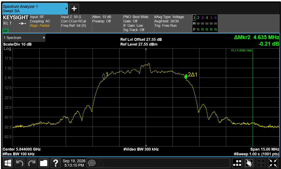
Figure 647 - Core 1 5844 MHz (CH119) 99% Bandwidth
