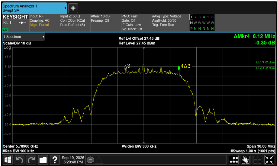
Figure 604 - Core 1 5789 MHz (CH64) 6 dB Bandwidth
