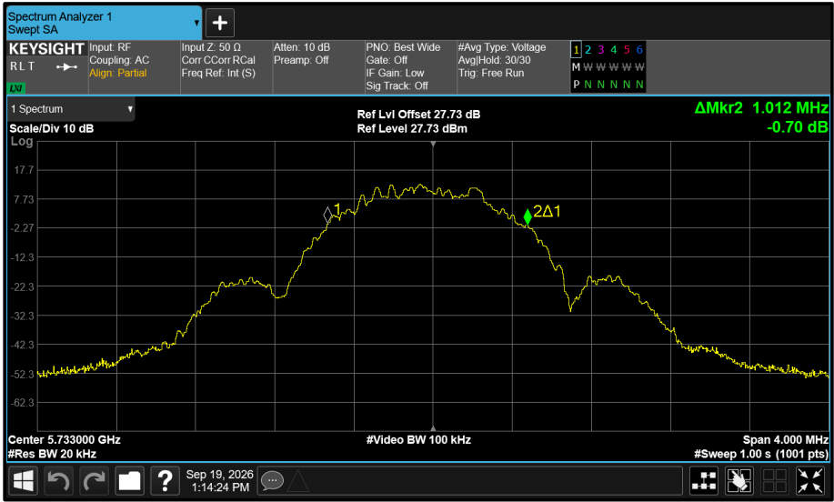
Figure 565 - Core 0 5733 MHz (CH8) 99% Bandwidth
