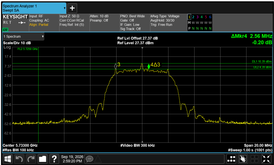
Figure 596 - Core 1 5733 MHz (CH8) 6 dB Bandwidth
