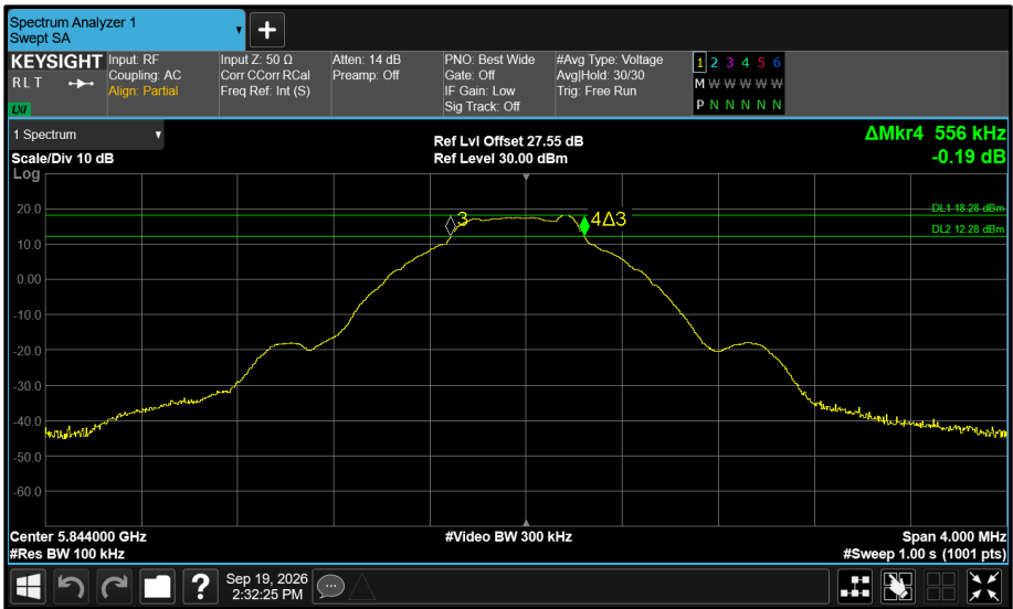
Figure 576 - Core 1 5844 MHz (CH119) 6 dB Bandwidth
