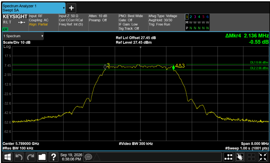
Figure 632 - Core 1 5789 MHz (CH64) 6 dB Bandwidth
