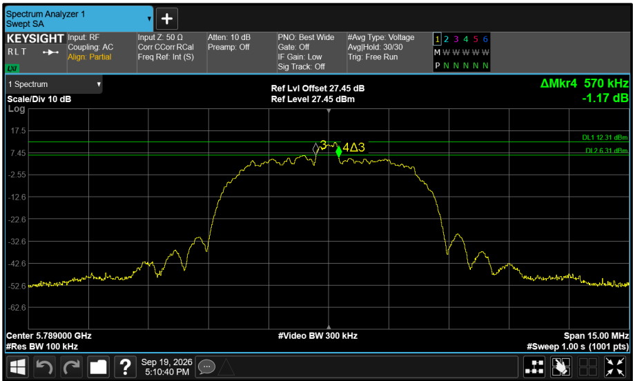
Figure 644 - Core 1 5789 MHz (CH64) 6 dB Bandwidth
