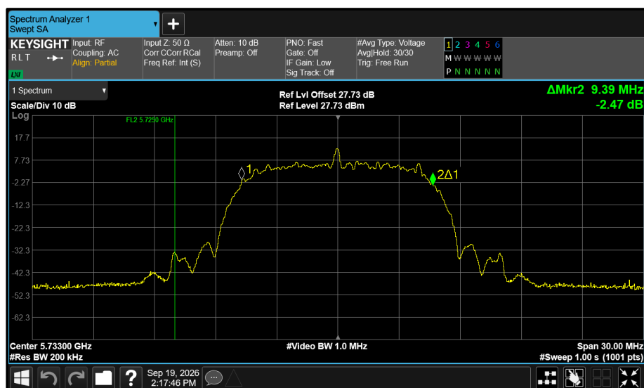
Figure 559 - Core 0 5733 MHz (CH8) 99% Bandwidth
