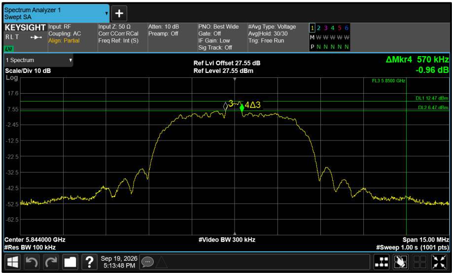
Figure 648 - Core 1 5844 MHz (CH119) 6 dB Bandwidth
