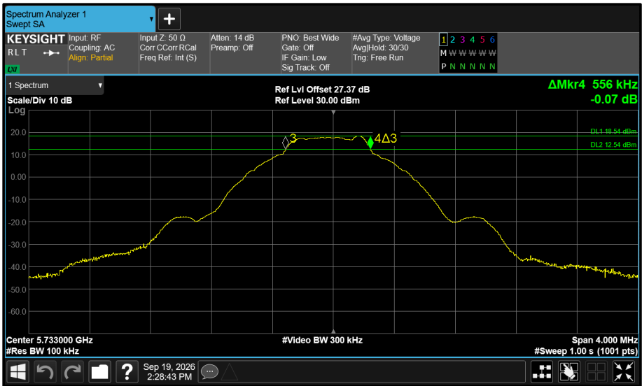
Figure 572 - Core 1 5733 MHz (CH8) 6 dB Bandwidth
