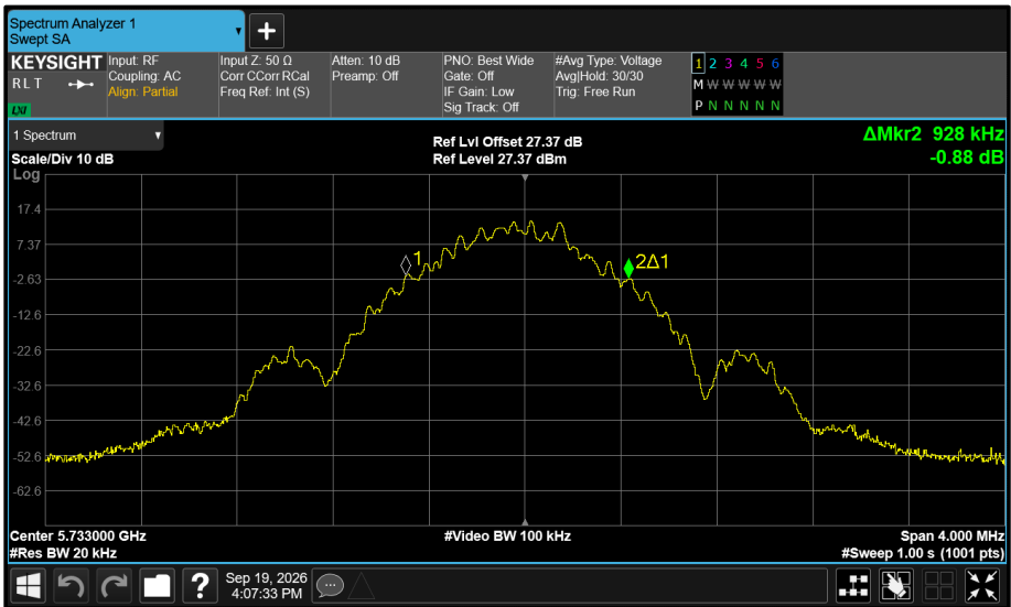
Figure 615 - Core 1 5733 MHz (CH8) 99% Bandwidth
