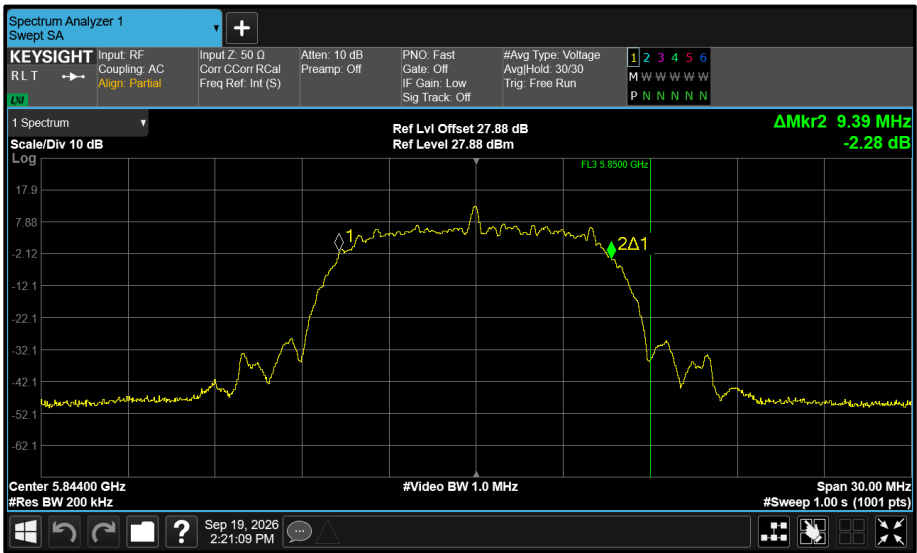
Figure 563 - Core 0 5844 MHz (CH119) 99% Bandwidth
