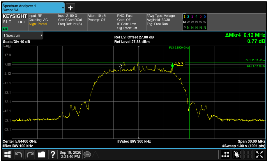
Figure 564 - Core 0 5844 MHz (CH119) 6 dB Bandwidth
