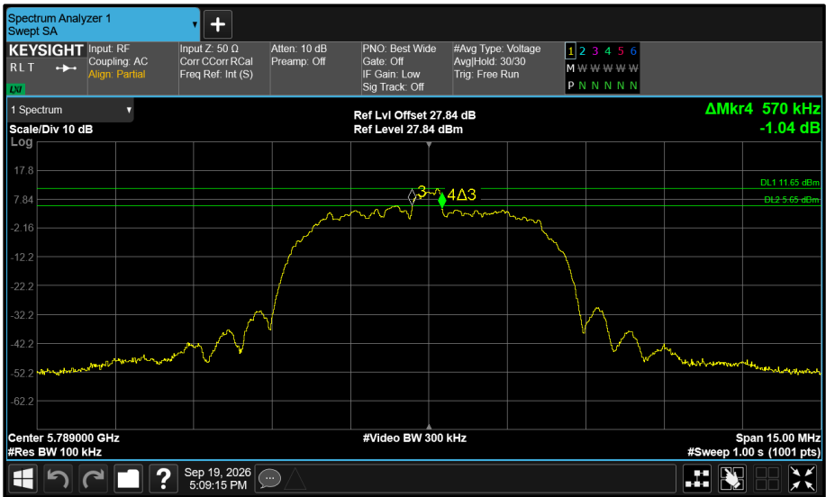
Figure 642 - Core 0 5789 MHz (CH64) 6 dB Bandwidth
