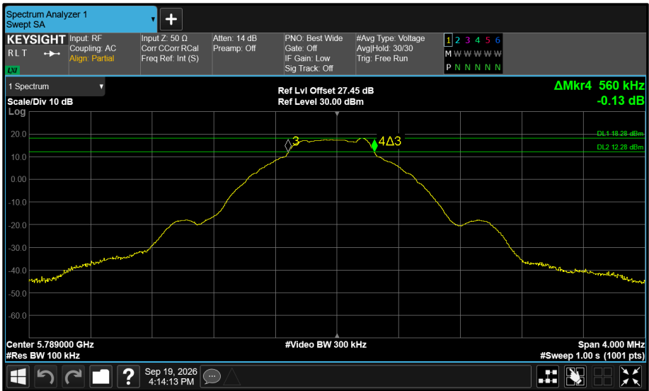
Figure 620 - Core 1 5789 MHz (CH64) 6 dB Bandwidth
