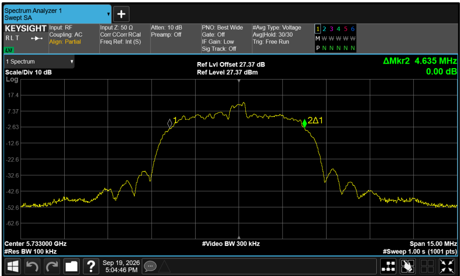
Figure 639 - Core 1 5733 MHz (CH8) 99% Bandwidth
