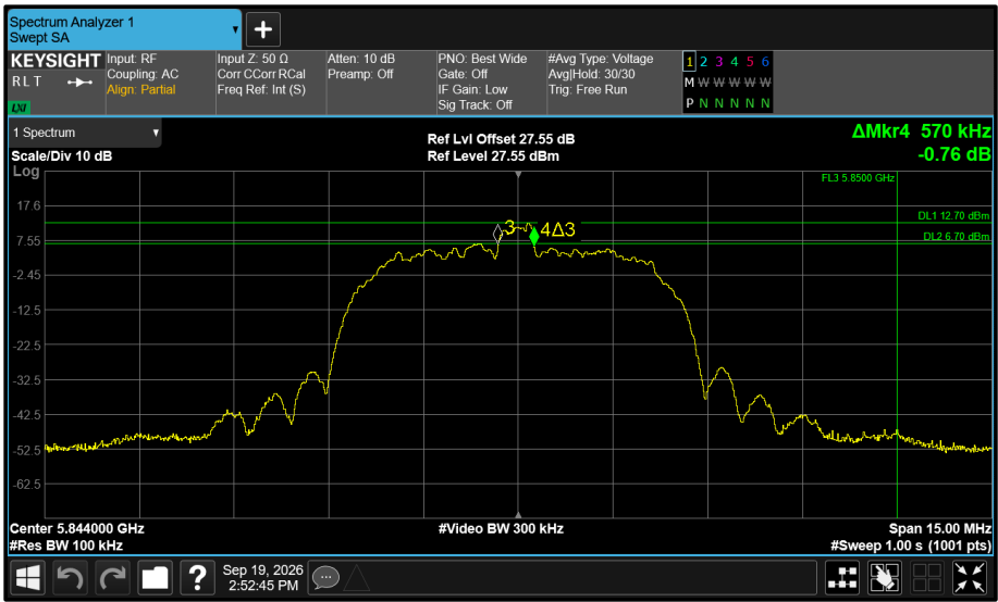
Figure 588 - Core 1 5844 MHz (CH119) 6 dB Bandwidth
