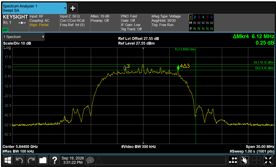
Figure 606 - Core 1 5844 MHz (CH119) 6 dB Bandwidth
