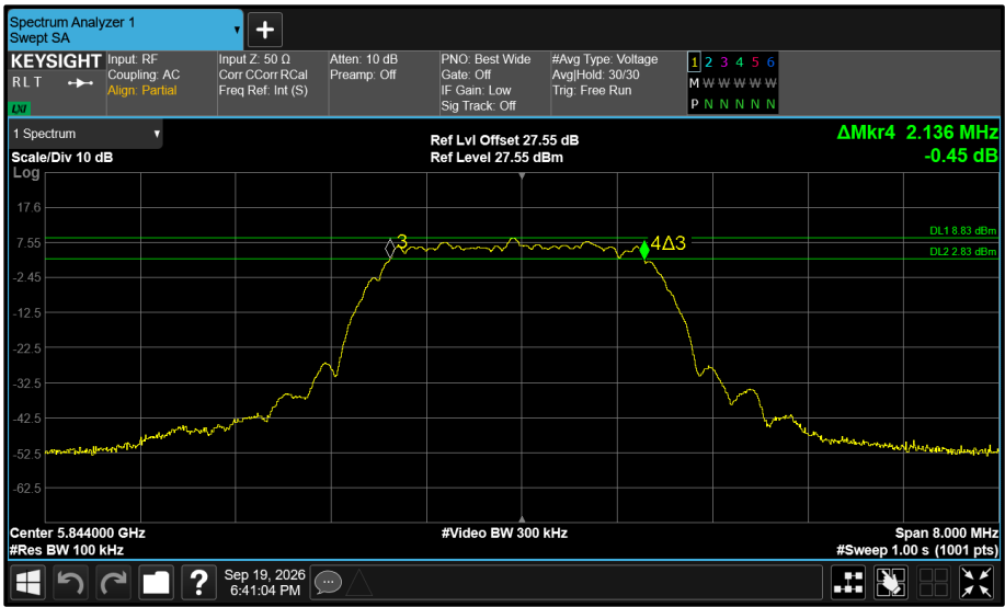
Figure 636 - Core 1 5844 MHz (CH119) 6 dB Bandwidth
