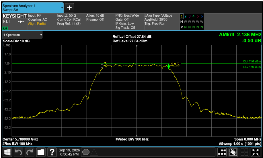
Figure 630 - Core 0 5789 MHz (CH64) 6 dB Bandwidth
