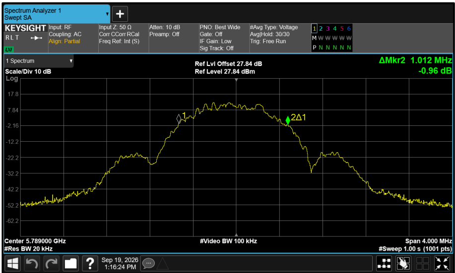
Figure 567 - Core 0 5789 MHz (CH64) 99% Bandwidth
