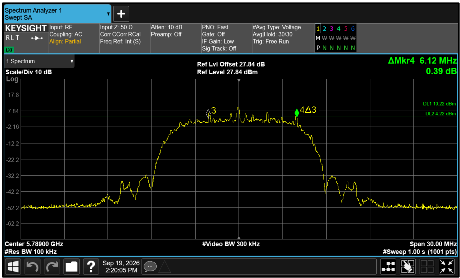
Figure 562 - Core 0 5789 MHz (CH64) 6 dB Bandwidth
