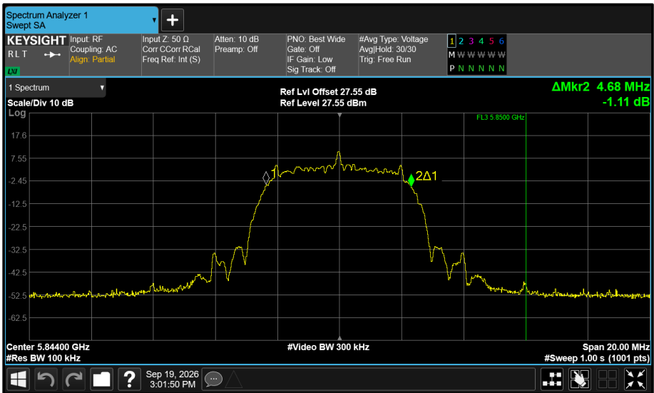
Figure 599 - Core 1 5844 MHz (CH119) 99% Bandwidth
