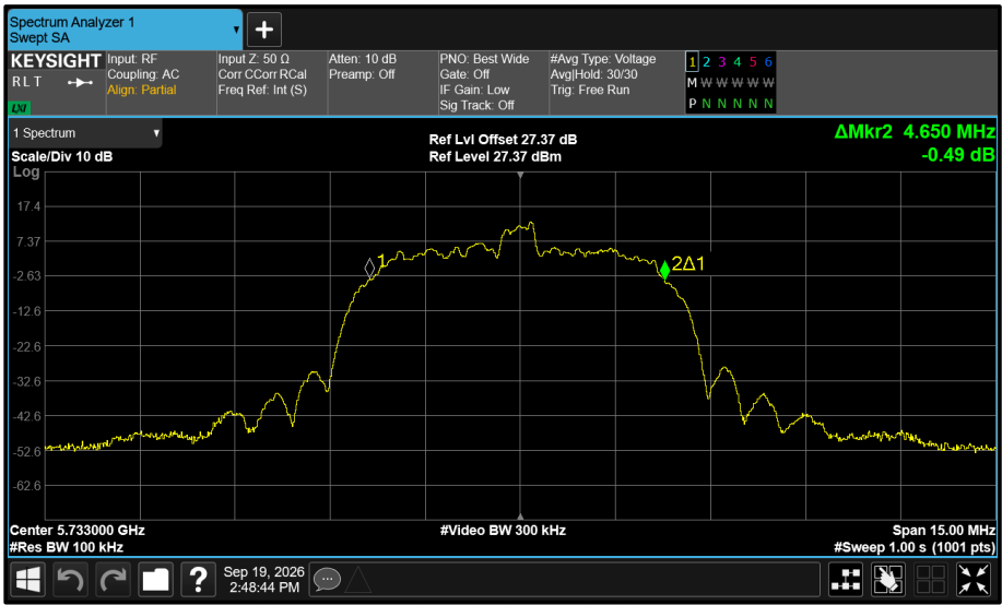
Figure 583 - Core 1 5733 MHz (CH8) 99% Bandwidth
