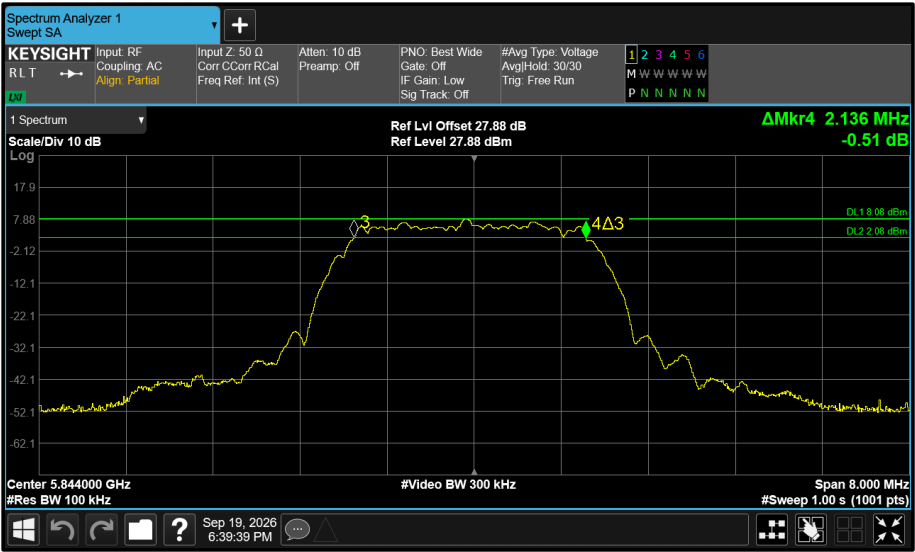
Figure 634 - Core 0 5844 MHz (CH119) 6 dB Bandwidth
