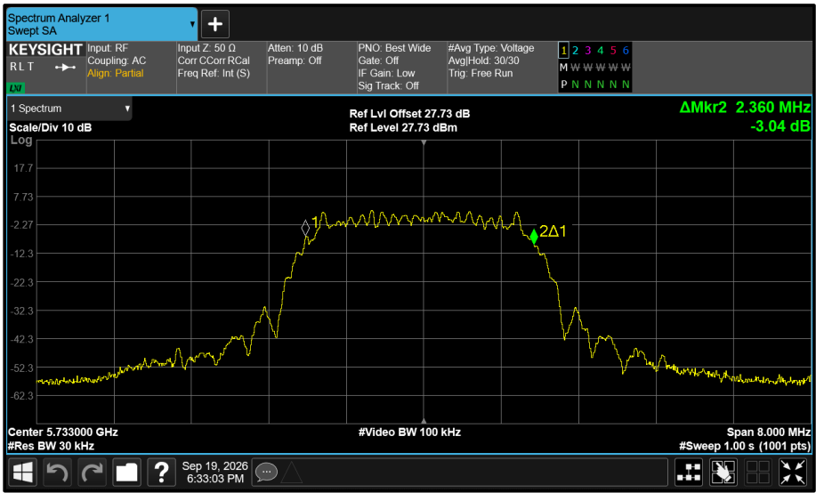
Figure 625 - Core 0 5733 MHz (CH8) 99% Bandwidth
