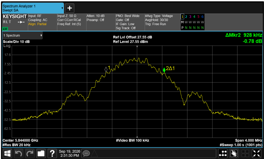
Figure 575 - Core 1 5844 MHz (CH119) 99% Bandwidth
