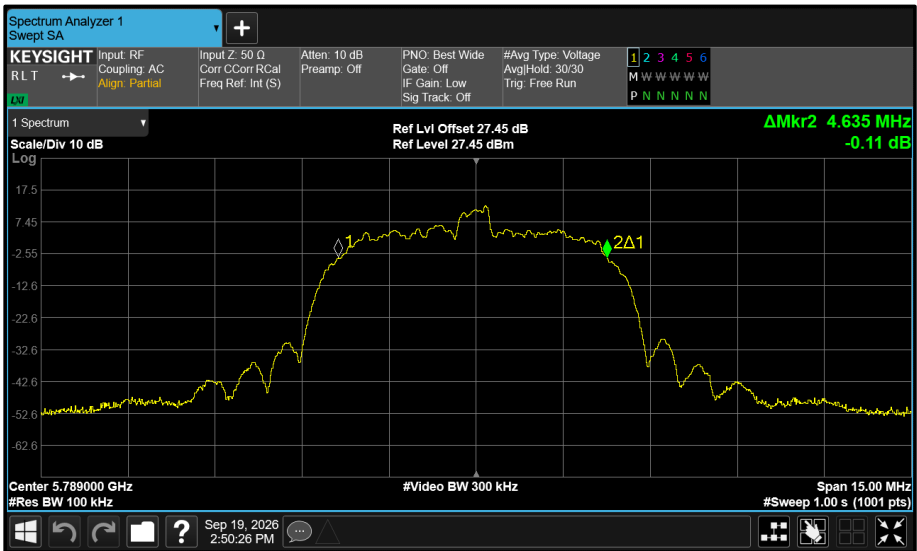
Figure 585 - Core 1 5789 MHz (CH64) 99% Bandwidth
