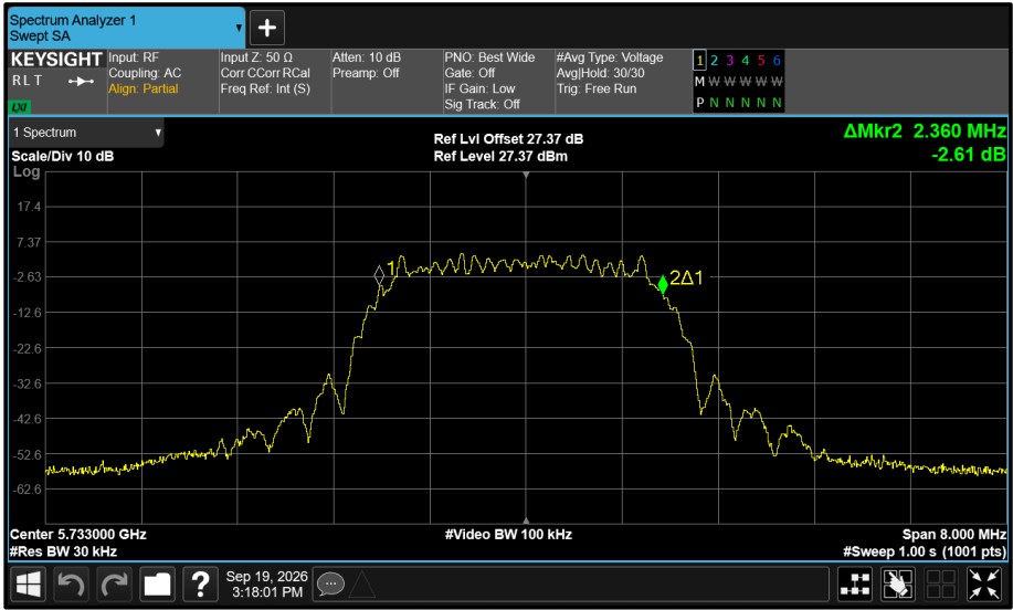
Figure 577 - Core 1 5733 MHz (CH8) 99% Bandwidth
