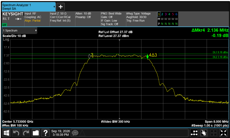
Figure 578 - Core 1 5733 MHz (CH8) 6 dB Bandwidth
