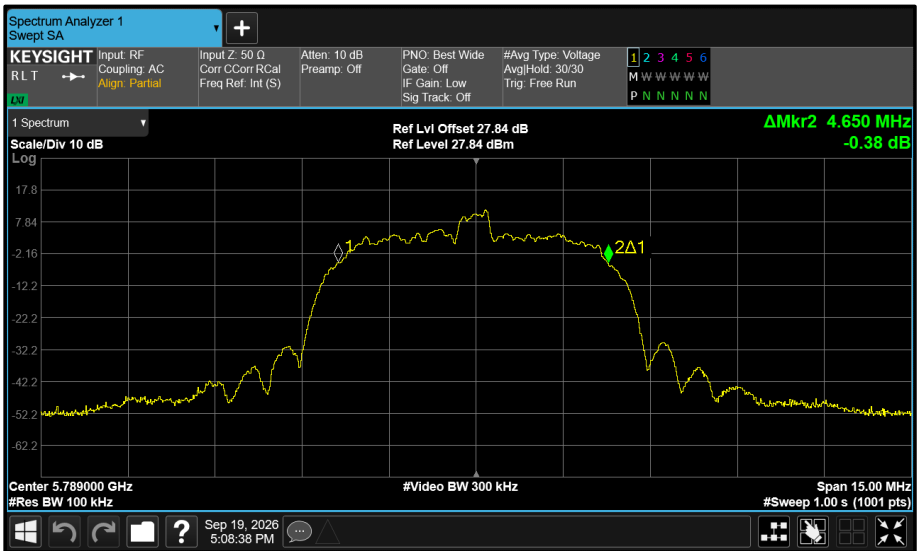
Figure 641 - Core 0 5789 MHz (CH64) 99% Bandwidth
