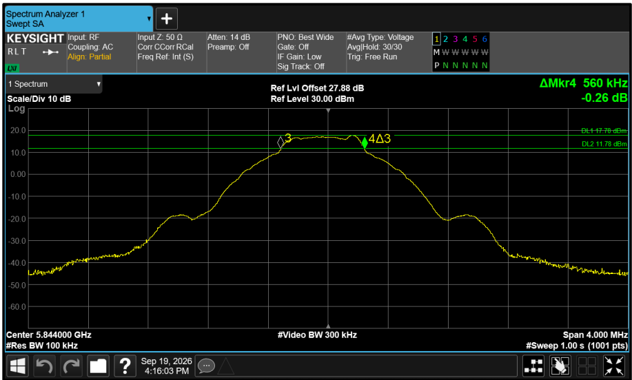
Figure 622 - Core 0 5844 MHz (CH119) 6 dB Bandwidth
