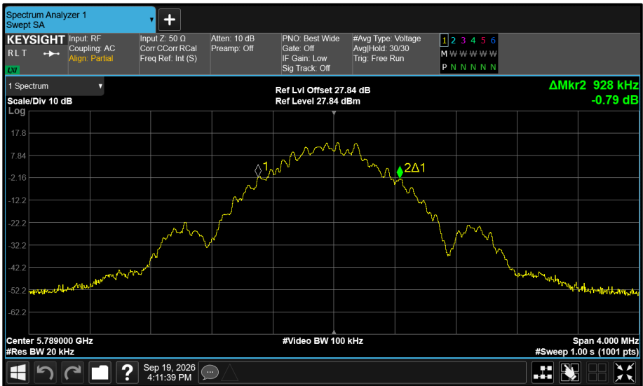
Figure 617 - Core 0 5789 MHz (CH64) 99% Bandwidth
