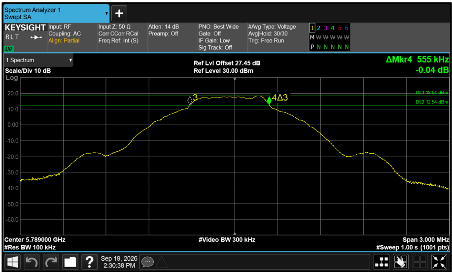
Figure 574 - Core 1 5789 MHz (CH64) 6 dB Bandwidth
