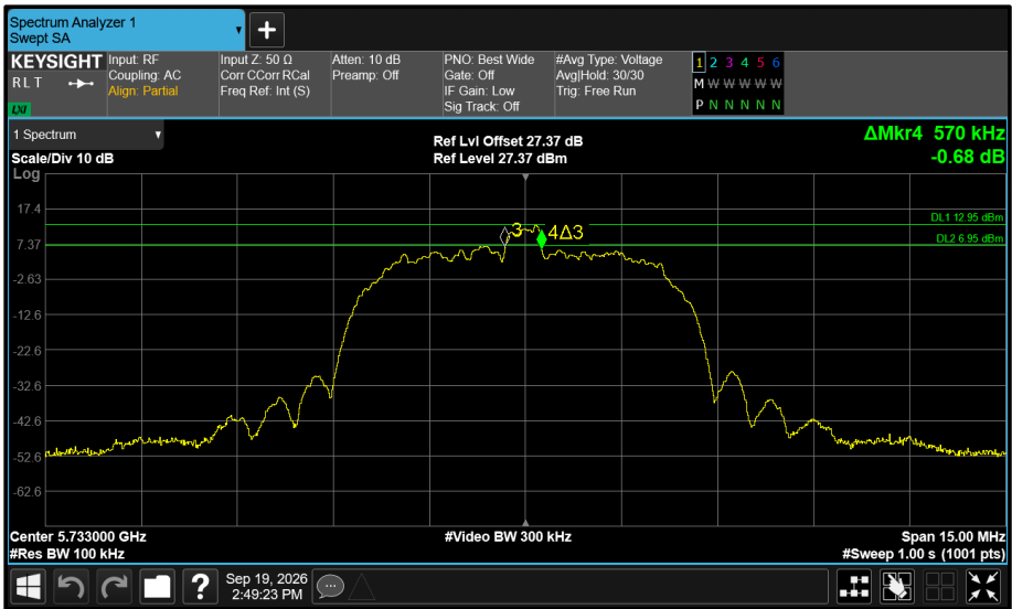
Figure 584 - Core 1 5733 MHz (CH8) 6 dB Bandwidth
