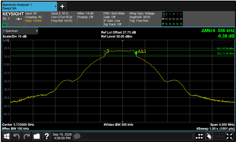
Figure 614 - Core 0 5733 MHz (CH8) 6 dB Bandwidth
