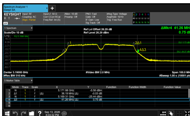
Figure 394 - 802.11a40 Minimum 99% OBW
