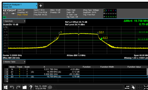
Figure 392 - 802.11a20 Minimum 99% OBW
