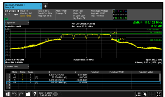
Figure 373 - 802.11a80 Maximum 99% OBW
