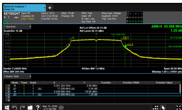
Figure 430 - 802.11n HT20 Minimum 26 dB EBW
