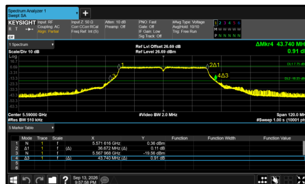
Figure 379 - 802.11n HT40 Maximum 99% OBW
