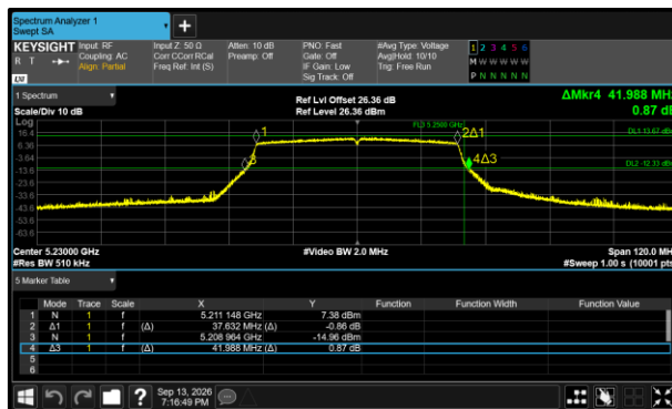
Figure 440 - 802.11ax HE40 SU Minimum 26 dB EBW
