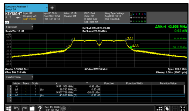
Figure 395 - 802.11a40 Maximum 99% OBW
