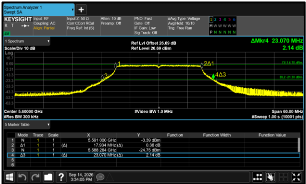
Figure 417 - 802.11ac VHT20 Maximum 99% OBW
