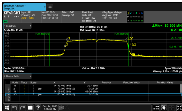
Figure 434 - 802.11ac VHT80 Minimum 26 dB EBW
