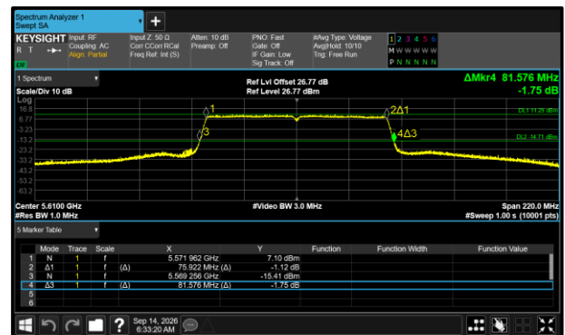
Figure 435 - 802.11ac VHT80 Maximum 26 dB EBW
