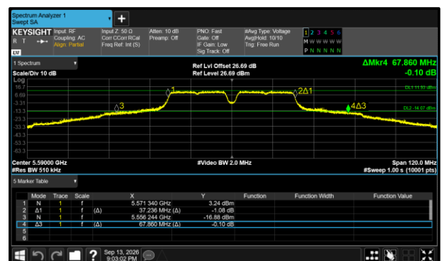
Figure 371 - 802.11a40 Maximum 99% OBW
