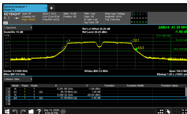
Figure 370 - 802.11a40 Minimum 99% OBW
