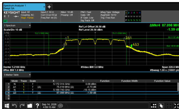
Figure 372 - 802.11a80 Minimum 99% OBW
