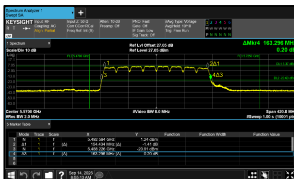
Figure 374 - 802.11a160 Minimum 99% OBW
