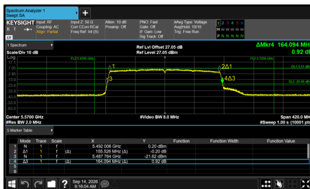
Figure 390 - 802.11ax HE160 SU Minimum 99% OBW
