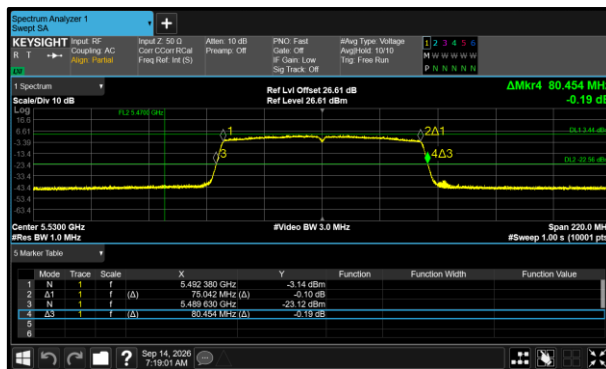
Figure 380 - 802.11ac VHT80 Minimum 99% OBW
