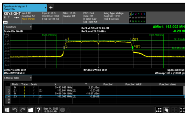
Figure 436 - 802.11ac VHT160 Minimum 26 dB EBW
