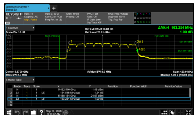
Figure 399 - 802.11a160 Maximum 99% OBW
