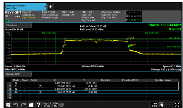
Figure 421 - 802.11ac VHT160 Maximum 99% OBW
