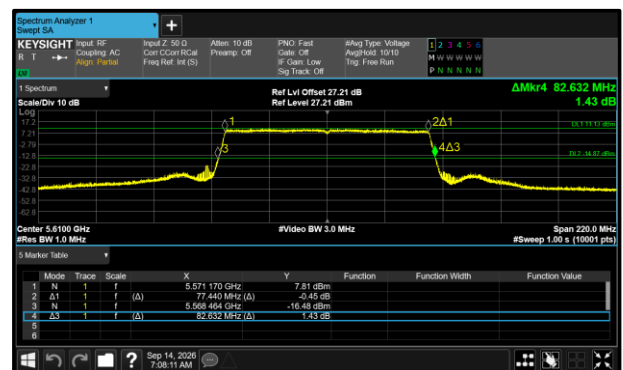
Figure 389 - 802.11ax HE80 SU Maximum 99% OBW
