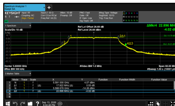
Figure 431 - 802.11n HT20 Maximum 26 dB EBW
