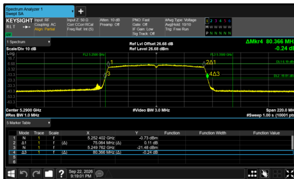
Figure 404 - 802.11ac VHT80 Minimum 99% OBW
