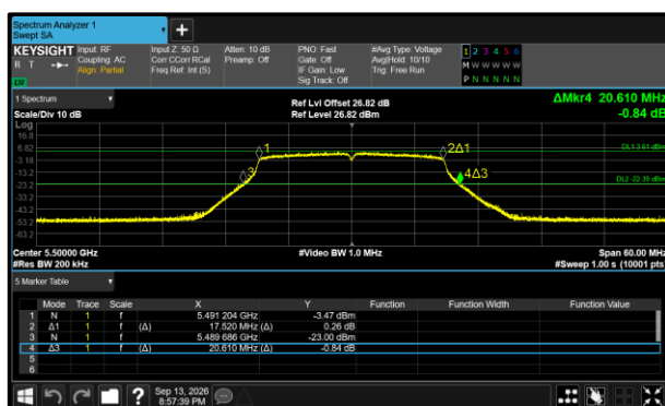
Figure 376 - 802.11n HT20 Minimum 99% OBW
