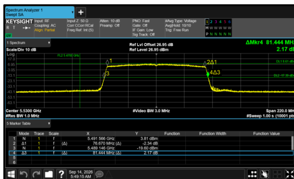
Figure 442 - 802.11ax HE80 SU Minimum 26 dB EBW
