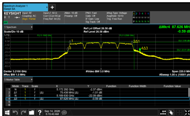
Figure 396 - 802.11a80 Minimum 99% OBW
