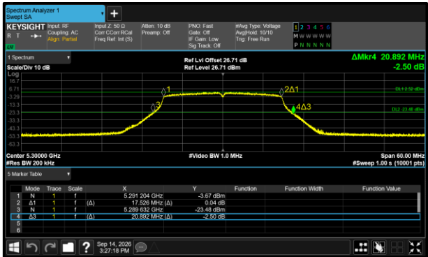
Figure 416 - 802.11ac VHT20 Minimum 99% OBW
