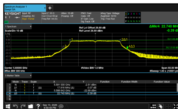
Figure 377 - 802.11n HT20 Maximum 99% OBW
