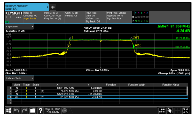
Figure 381 - 802.11ac VHT80 Maximum 99% OBW
