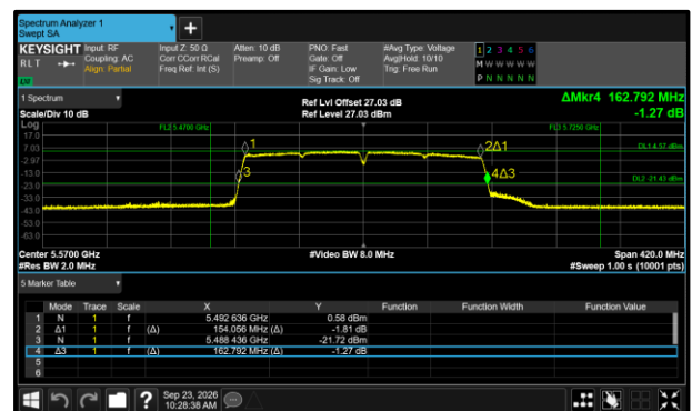
Figure 407 - 802.11ac VHT160 Maximum 99% OBW
