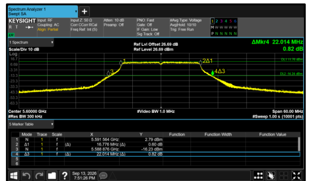
Figure 369 - 802.11a20 Maximum 99% OBW
