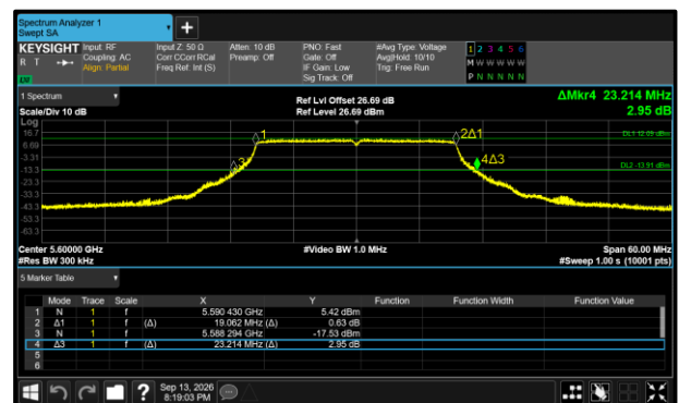
Figure 439 - 802.11ax HE20 SU Maximum 26 dB EBW
