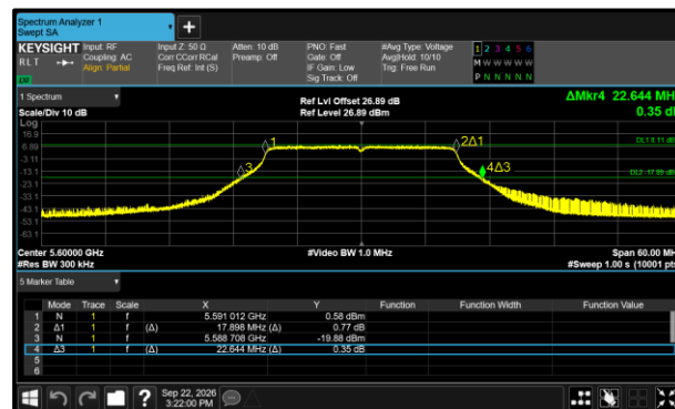
Figure 401 - 802.11n HT20 Maximum 99% OBW
