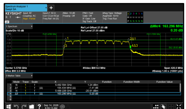
Figure 375 - 802.11a160 Maximum 99% OBW
