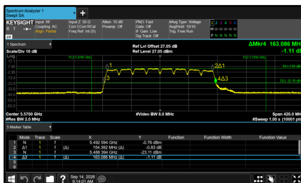
Figure 398 - 802.11a160 Minimum 99% OBW
