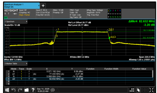
Figure 365 - 802.11ax HE80 SU Maximum 99% OBW
