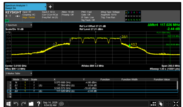
Figure 397 - 802.11a80 Maximum 99% OBW
