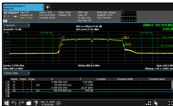
Figure 382 - 802.11ac VHT160 Minimum 99% OBW
