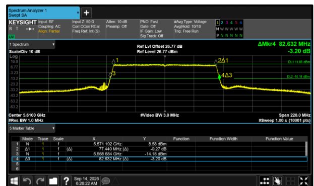
Figure 443 - 802.11ax HE80 SU Maximum 26 dB EBW
