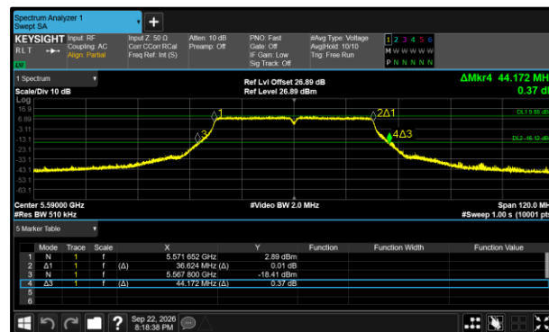
Figure 403 - 802.11n HT40 Maximum 99% OBW
