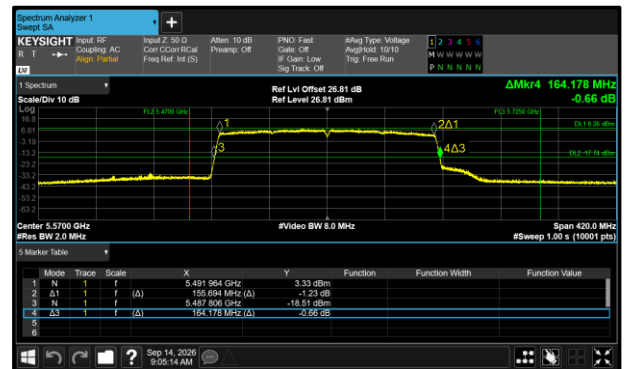
Figure 367 - 802.11ax HE160 SU Maximum 99% OBW
