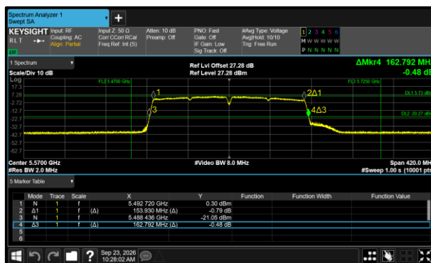
Figure 406 - 802.11ac VHT160 Minimum 99% OBW
