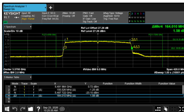
Figure 414 - 802.11ax HE160 SU Minimum 99% OBW
