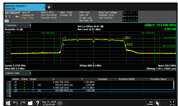
Figure 383 - 802.11ac VHT160 Maximum 99% OBW
