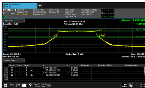
Figure 368 - 802.11a20 Minimum 99% OBW
