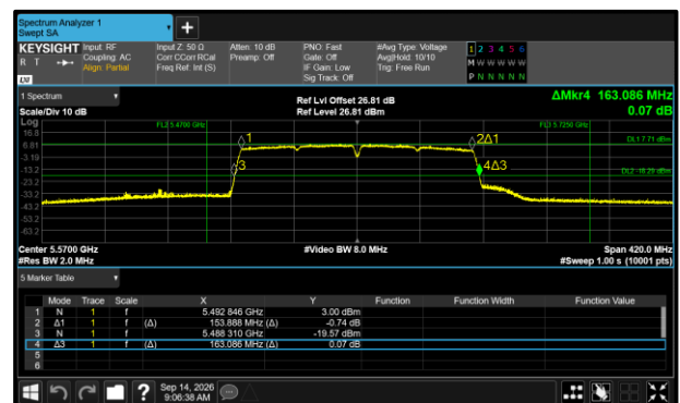
Figure 437 - 802.11ac VHT160 Maximum 26 dB EBW
