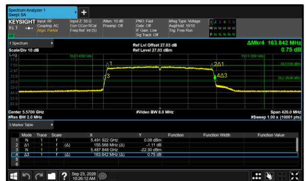
Figure 415 - 802.11ax HE160 SU Maximum 99% OBW
