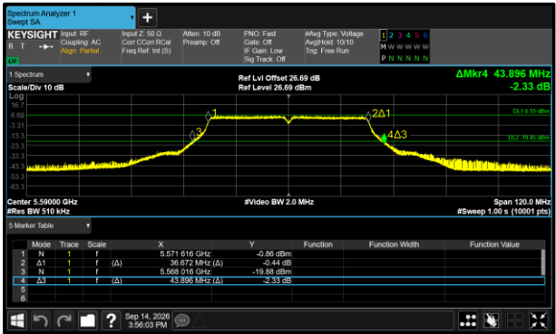
Figure 419 - 802.11ac VHT40 Maximum 99% OBW
