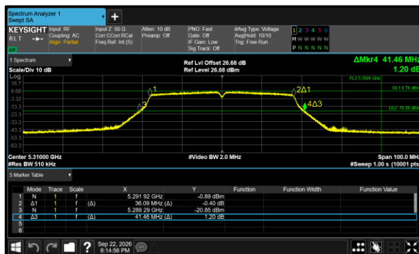
Figure 402 - 802.11n HT40 Minimum 99% OBW
