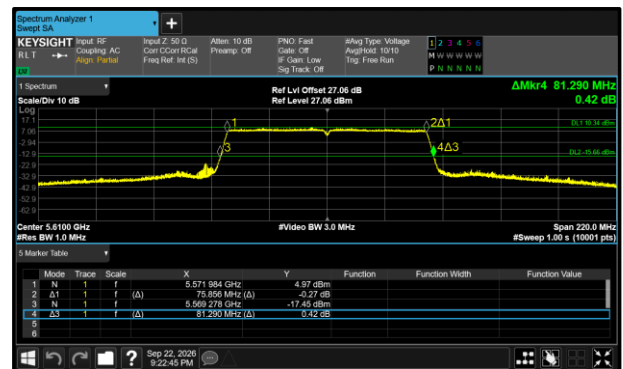
Figure 405 - 802.11ac VHT80 Maximum 99% OBW
