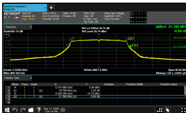
Figure 438 - 802.11ax HE20 SU Minimum 26 dB EBW
