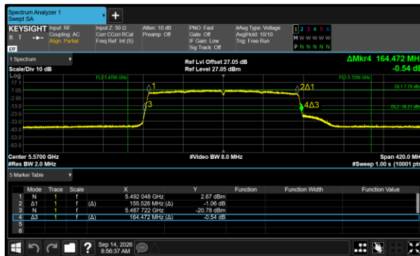
Figure 366 - 802.11ax HE160 SU Minimum 99% OBW
