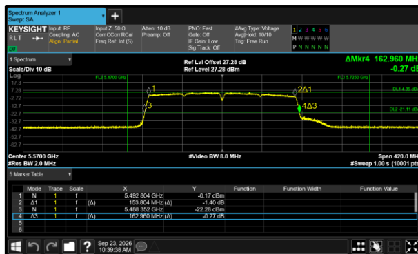
Figure 420 - 802.11ac VHT160 Minimum 99% OBW
