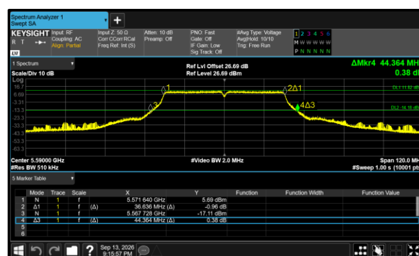
Figure 433 - 802.11n HT40 Maximum 26 dB EBW
