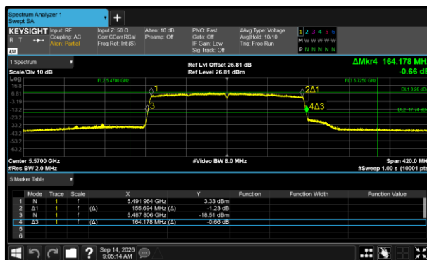
Figure 444 - 802.11ax HE160 SU Minimum 26 dB EBW
