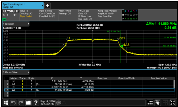
Figure 418 - 802.11ac VHT40 Minimum 99% OBW
