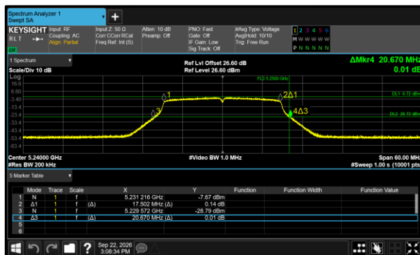
Figure 400 - 802.11n HT20 Minimum 99% OBW
