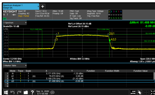
Figure 388 - 802.11ax HE80 SU Minimum 99% OBW
