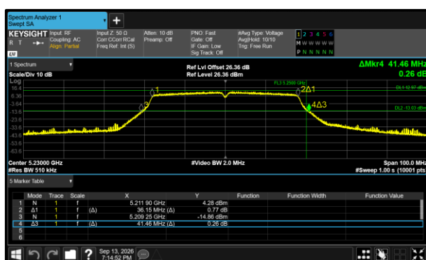
Figure 432 - 802.11n HT40 Minimum 26 dB EBW
