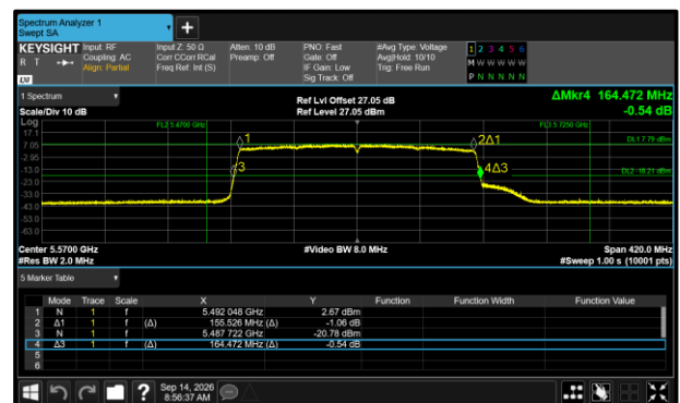
Figure 445 - 802.11ax HE160 SU Maximum 26 dB EBW
