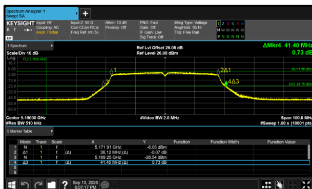
Figure 378 - 802.11n HT40 Minimum 99% OBW
