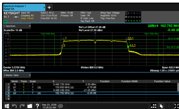
Figure 484 - 802.11ac VHT160 Minimum 26 dB EBW
