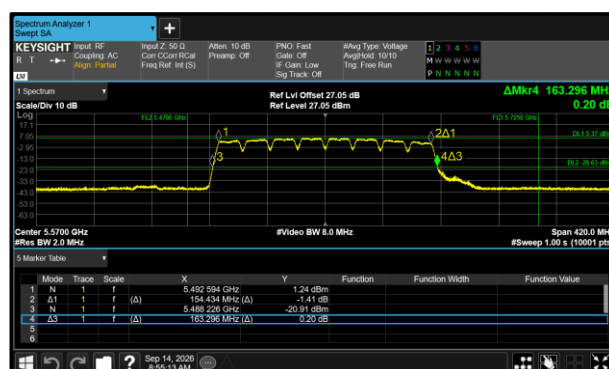
Figure 453 - 802.11a160 Maximum 26 dB EBW
