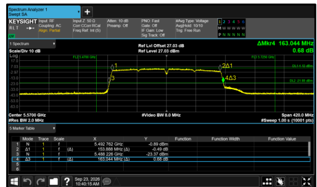
Figure 499 - 802.11ac VHT160 Maximum 26 dB EBW
