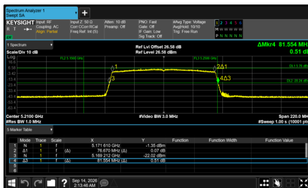
Figure 466 - 802.11ax HE80 SU Minimum 26 dB EBW
