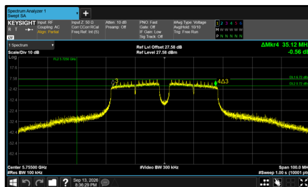
Figure 523 - 802.11a40 Maximum 6 dB EBW
