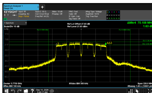
Figure 525 - 802.11a80 Maximum 6 dB EBW
