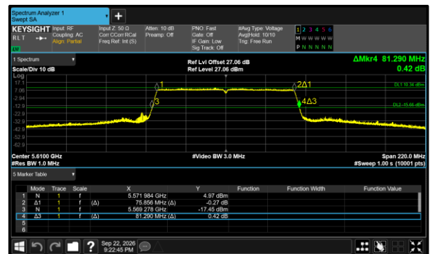
Figure 483 - 802.11ac VHT80 Maximum 26 dB EBW
