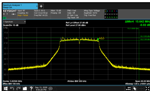
Figure 538 - 802.11a20 Minimum 6 dB EBW
