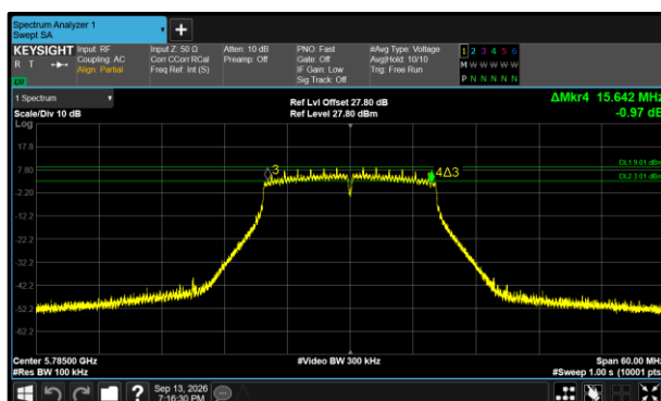
Figure 520 - 802.11a20 Minimum 6 dB EBW
