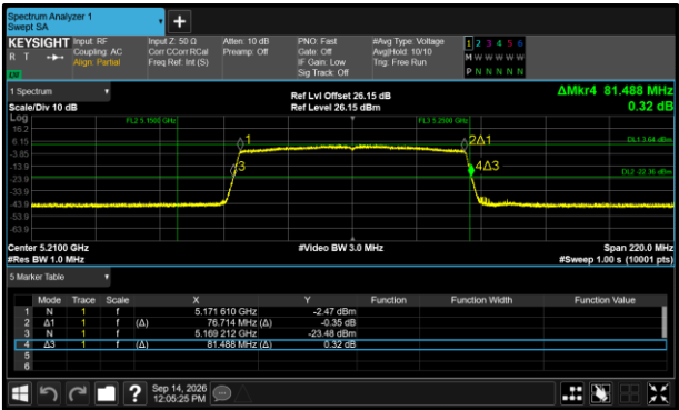
Figure 504 - 802.11ax HE80 SU Minimum 26 dB EBW
