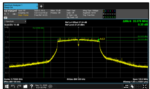
Figure 511 - 802.11n HT40 Maximum 6 dB EBW
