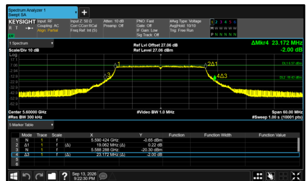
Figure 463 - 802.11ax HE20 SU Maximum 26 dB EBW
