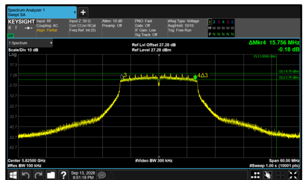
Figure 539 - 802.11a20 Maximum 6 dB EBW
