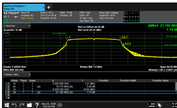
Figure 486 - 802.11ax HE20 SU Minimum 26 dB EBW
