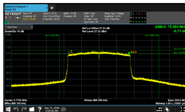
Figure 519 - 802.11ax HE80 SU Maximum 6 dB EBW
