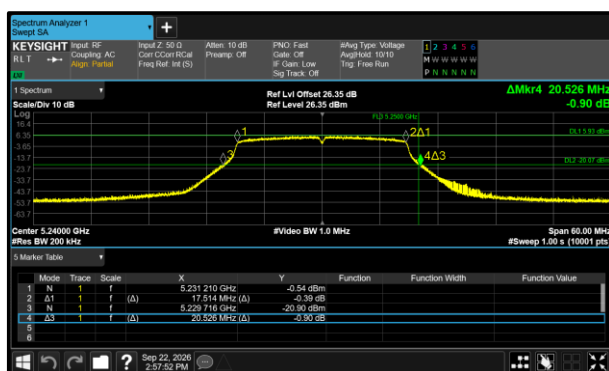
Figure 478 - 802.11n HT20 Minimum 26 dB EBW
