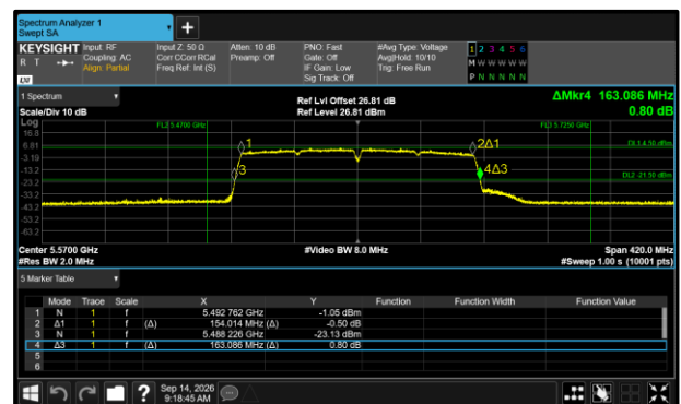
Figure 461 - 802.11ac VHT160 Maximum 26 dB EBW
