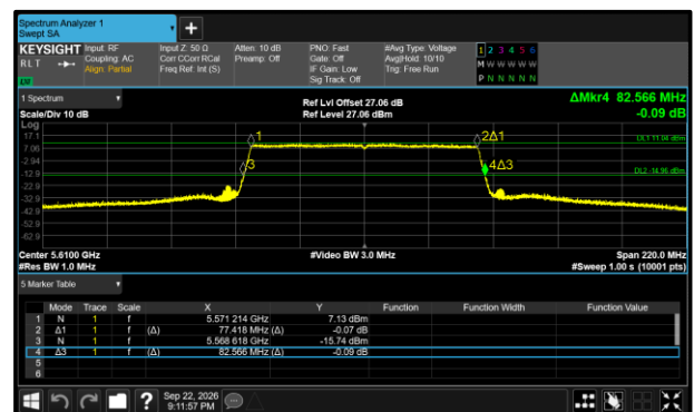
Figure 491 - 802.11ax HE80 SU Maximum 26 dB EBW
