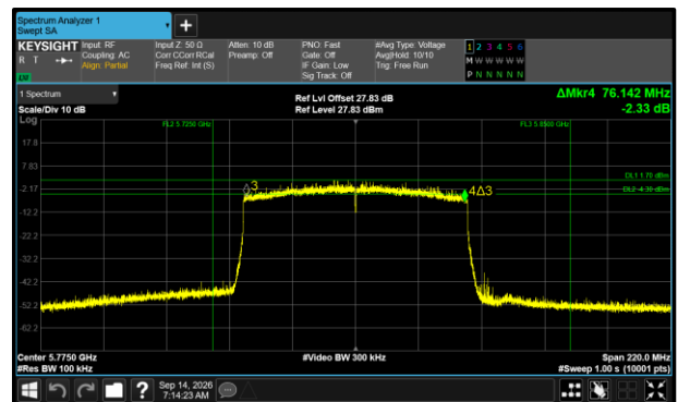
Figure 537 - 802.11ax HE80 SU Maximum 6 dB EBW
