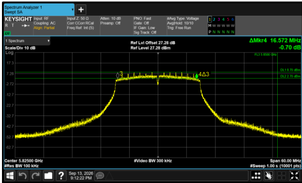
Figure 527 - 802.11n HT20 Maximum 6 dB EBW
