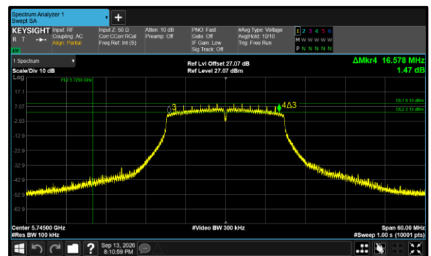
Figure 509 - 802.11n HT20 Maximum 6 dB EBW
