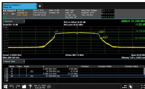
Figure 462 - 802.11ax HE20 SU Minimum 26 dB EBW
