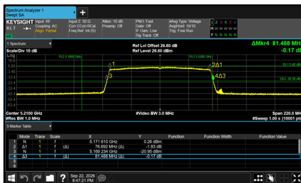
Figure 490 - 802.11ax HE80 SU Minimum 26 dB EBW
