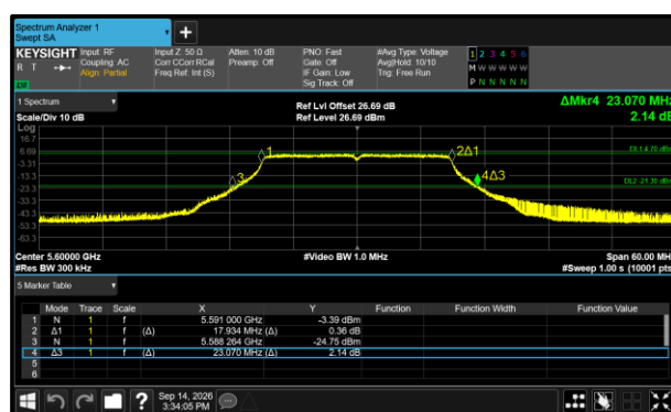
Figure 495 - 802.11ac VHT20 Maximum 26 dB EBW
