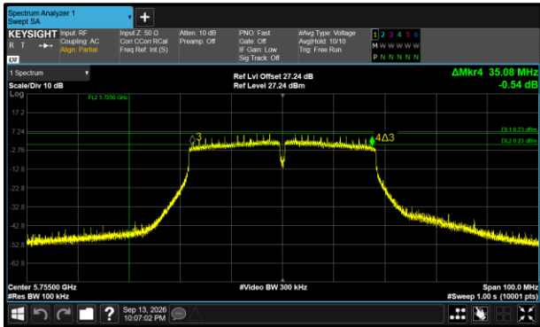
Figure 529 - 802.11n HT40 Maximum 6 dB EBW
