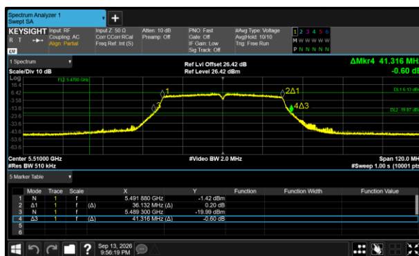
Figure 456 - 802.11n HT40 Minimum 26 dB EBW
