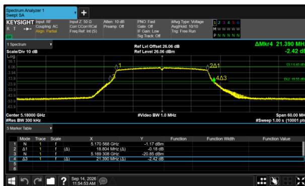
Figure 500 - 802.11ax HE20 SU Minimum 26 dB EBW
