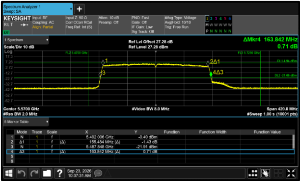
Figure 506 - 802.11ax HE160 SU Minimum 26 dB EBW
