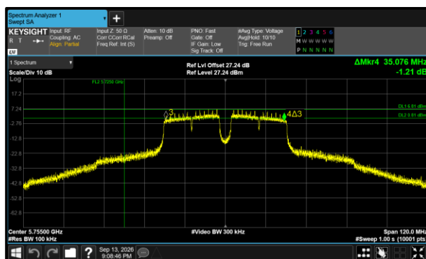
Figure 522 - 802.11a40 Minimum 6 dB EBW
