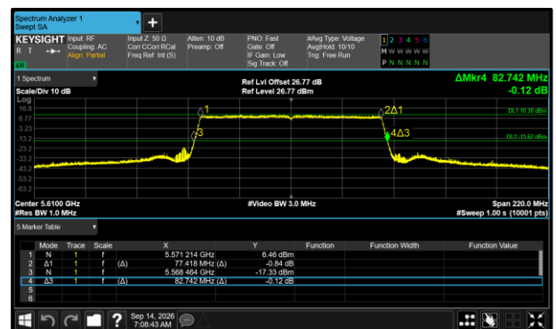
Figure 467 - 802.11ax HE80 SU Maximum 26 dB EBW
