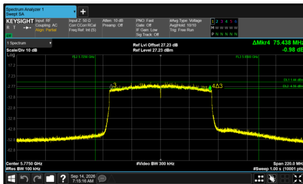
Figure 536 - 802.11ax HE80 SU Minimum 6 dB EBW
