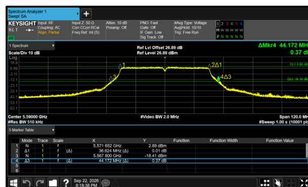
Figure 481 - 802.11n HT40 Maximum 26 dB EBW
