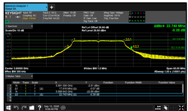
Figure 455 - 802.11n HT20 Maximum 26 dB EBW
