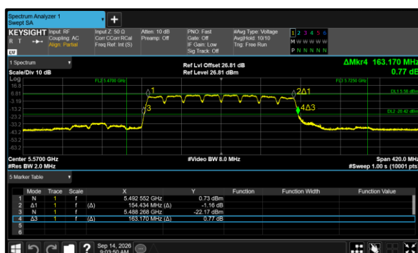
Figure 452 - 802.11a160 Minimum 26 dB EBW
