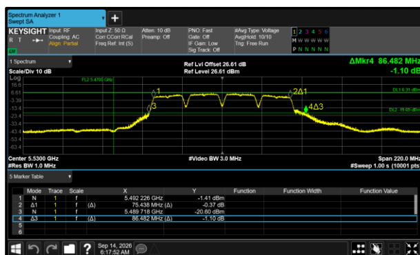
Figure 450 - 802.11a80 Minimum 26 dB EBW
