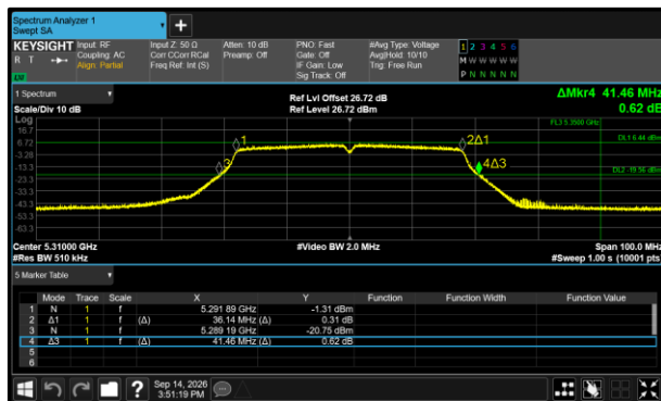
Figure 496 - 802.11ac VHT40 Minimum 26 dB EBW
