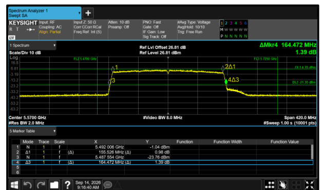
Figure 469 - 802.11ax HE160 SU Maximum 26 dB EBW
