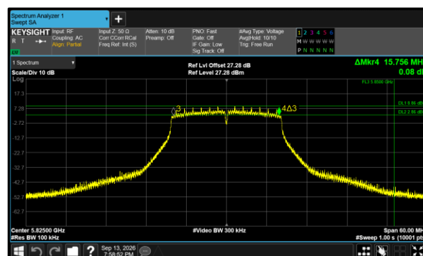
Figure 521 - 802.11a20 Maximum 6 dB EBW
