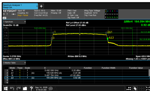
Figure 468 - 802.11ax HE160 SU Minimum 26 dB EBW
