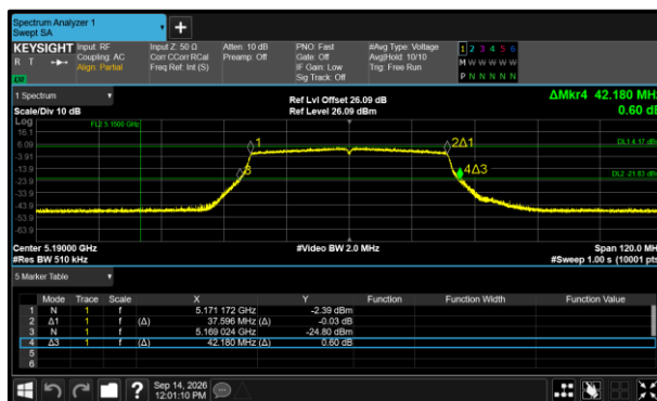
Figure 502 - 802.11ax HE40 SU Minimum 26 dB EBW
