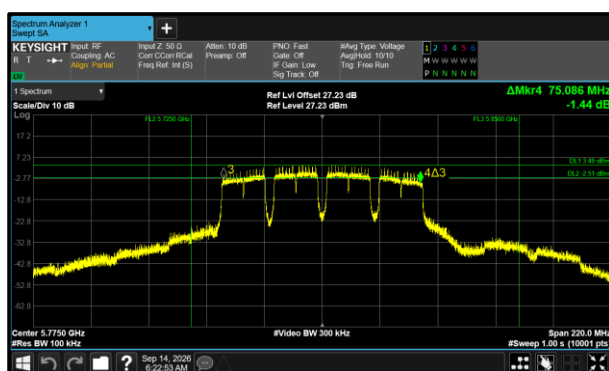
Figure 524 - 802.11a80 Minimum 6 dB EBW
