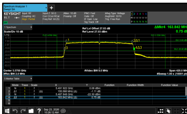
Figure 492 - 802.11ax HE160 SU Minimum 26 dB EBW
