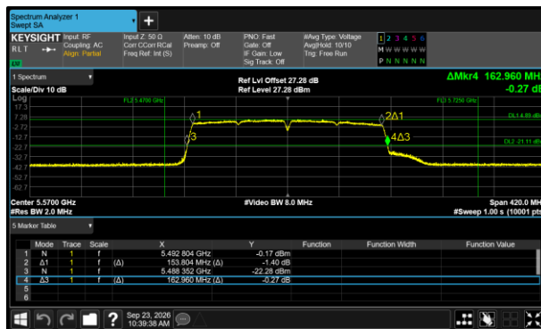
Figure 498 - 802.11ac VHT160 Minimum 26 dB EBW
