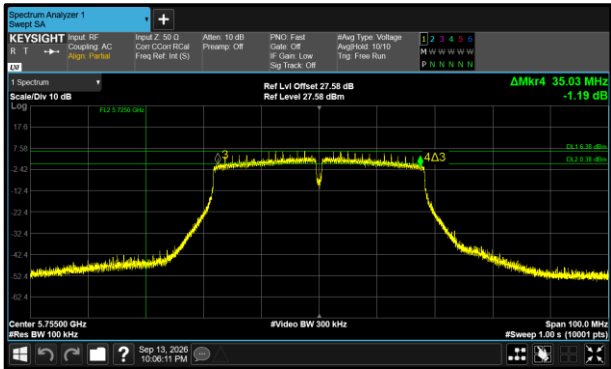
Figure 528 - 802.11n HT40 Minimum 6 dB EBW
