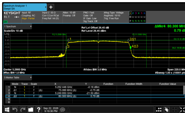
Figure 482 - 802.11ac VHT80 Minimum 26 dB EBW
