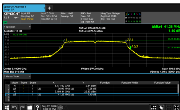
Figure 480 - 802.11n HT40 Minimum 26 dB EBW
