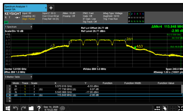
Figure 451 - 802.11a80 Maximum 26 dB EBW
