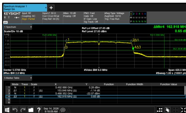
Figure 460 - 802.11ac VHT160 Minimum 26 dB EBW
