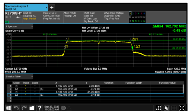
Figure 485 - 802.11ac VHT160 Maximum 26 dB EBW
