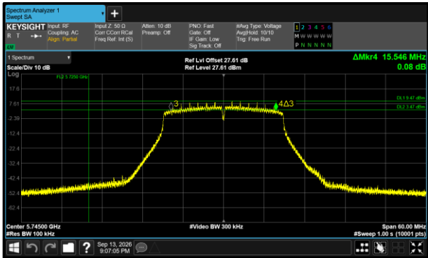
Figure 526 - 802.11n HT20 Minimum 6 dB EBW
