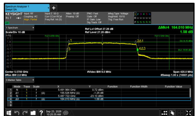
Figure 493 - 802.11ax HE160 SU Maximum 26 dB EBW
