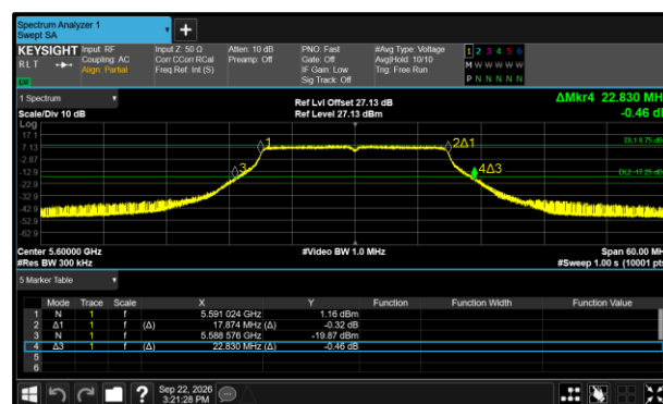
Figure 479 - 802.11n HT20 Maximum 26 dB EBW
