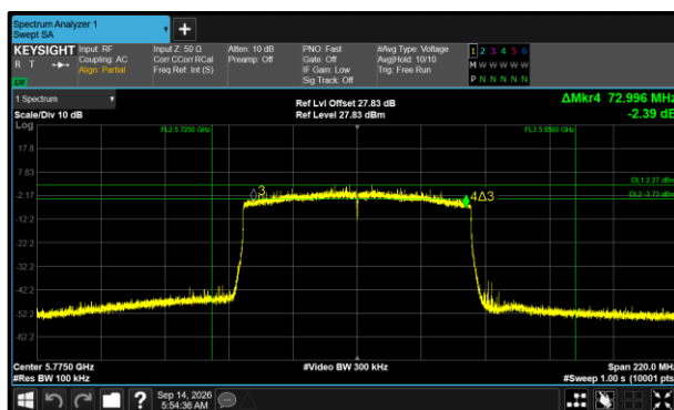
Figure 518 - 802.11ax HE80 SU Minimum 6 dB EBW
