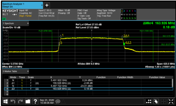
Figure 507 - 802.11ax HE160 SU Maximum 26 dB EBW
