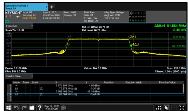
Figure 459 - 802.11ac VHT80 Maximum 26 dB EBW
