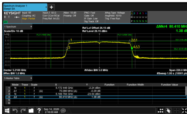
Figure 458 - 802.11ac VHT80 Minimum 26 dB EBW
