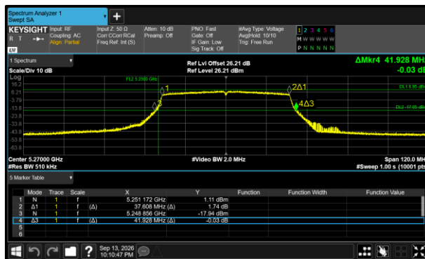
Figure 464 - 802.11ax HE40 SU Minimum 26 dB EBW
