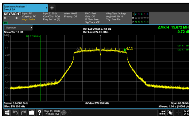
Figure 508 - 802.11n HT20 Minimum 6 dB EBW
