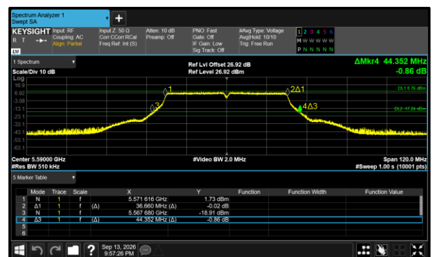
Figure 457 - 802.11n HT40 Maximum 26 dB EBW
