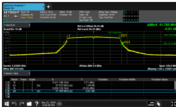
Figure 488 - 802.11ax HE40 SU Minimum 26 dB EBW
