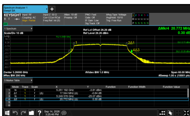
Figure 494 - 802.11ac VHT20 Minimum 26 dB EBW
