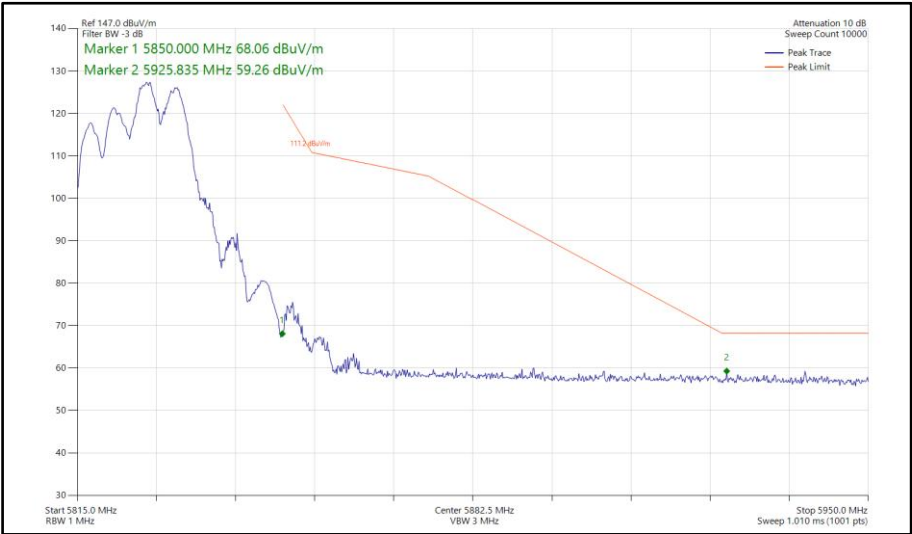
Figure 658 - 802.11be EHT20, RU106+26-83, CDD, Core 0-1 - 5825 MHz Band Edge Frequency 5850 MHz
