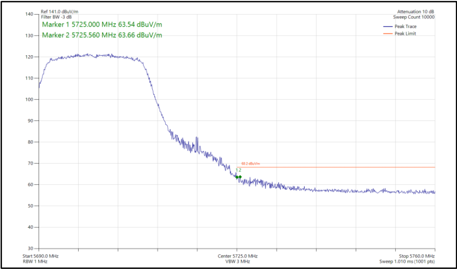
Figure 690 - 802.11ac VHT20, TxBF, Core 0-1 - 5700 MHz Band Edge Frequency 5725 MHz
