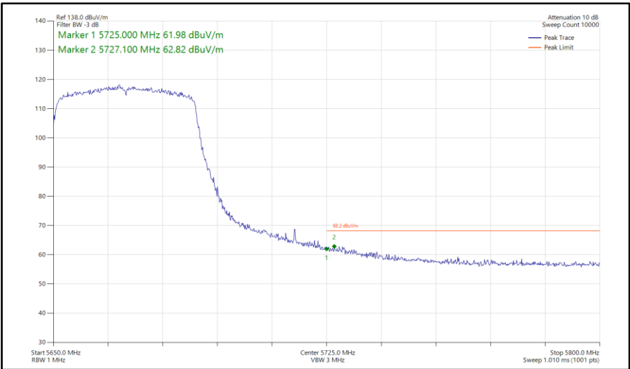
Figure 720 - 802.11ax HE40, SU, SISO, Core 0 - 5670 MHz Band Edge Frequency 5725 MHz
