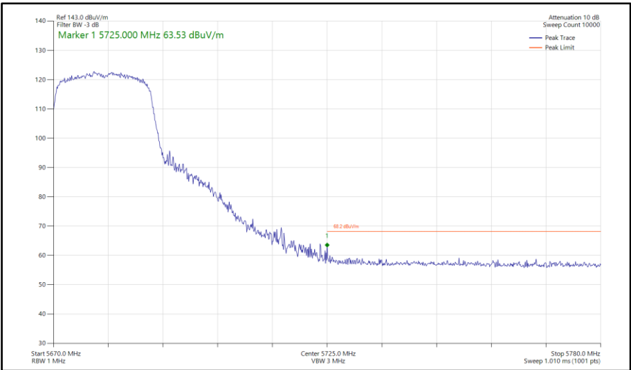
Figure 691 - 802.11ax HE20, SU, TxBF, Core 0-1 - 5680 MHz Band Edge Frequency 5725 MHz
