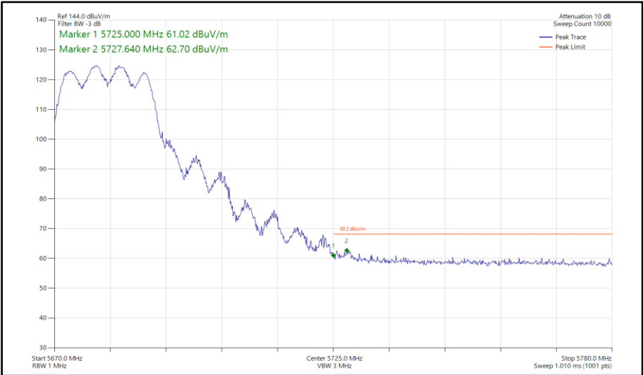
Figure 643 - 802.11n HT20, CDD, Core 0-1 - 5680 MHz Band Edge Frequency 5725 MHz
