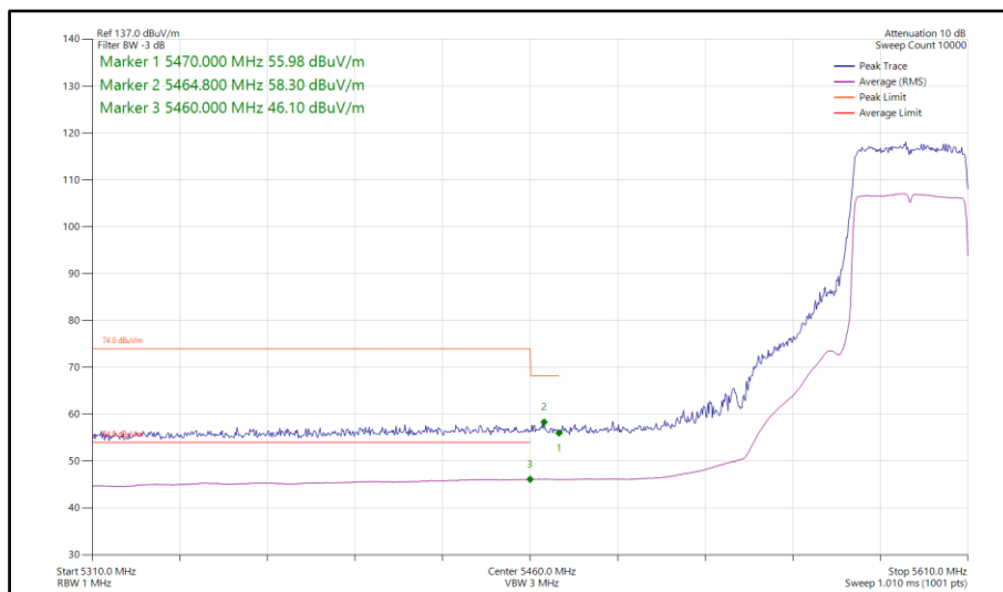
Figure 706 - 802.11ax HE40, SU, SISO, Core 0 - 5590 MHz Band Edge Frequency 5470 MHz
