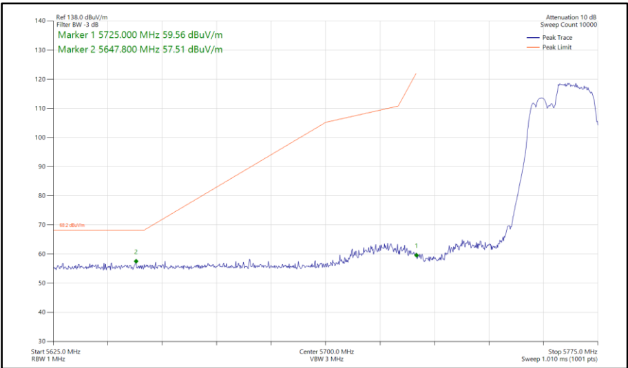
Figure 714 - 802.11be EHT40, RU106+26-85, SISO, Core 0 - 5755 MHz Band Edge Frequency 5725 MHz
