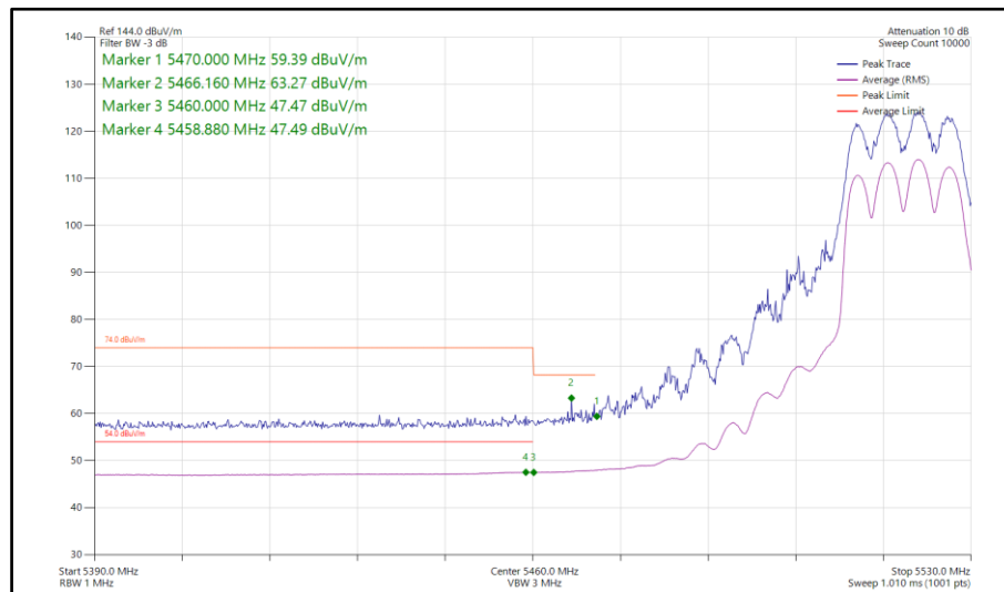
Figure 634 - 802.11ax HE20, SU, CDD, Core 0-1 - 5520 MHz Band Edge Frequency 5470 MHz
