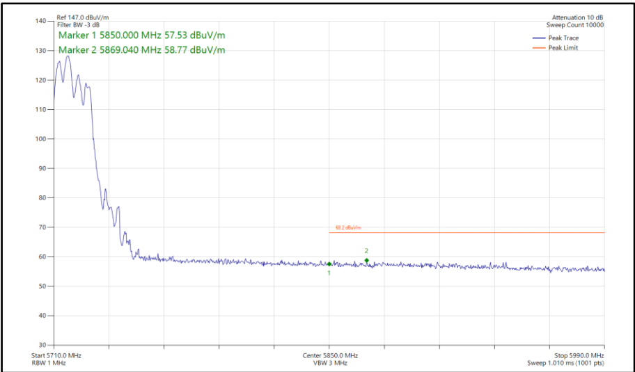
Figure 678 - 802.11ax HE20, RU106-53, SDM, Core 0-1 - 5720 MHz Band Edge Frequency 5850 MHz
