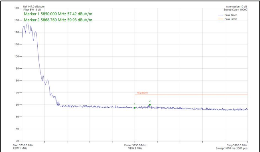
Figure 681 - 802.11be EHT20, RU106+26-82, SDM, Core 0-1 - 5720 MHz Band Edge Frequency 5850 MHz
