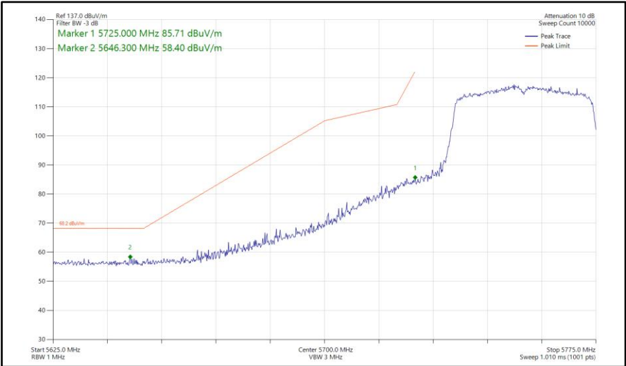
Figure 712 - 802.11ax HE40, SU, SISO, Core 0 - 5755 MHz Band Edge Frequency 5725 MHz
