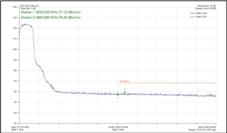
Figure 677 - 802.11ax HE20, SU, SDM, Core 0-1 - 5720 MHz Band Edge Frequency 5850 MHz
