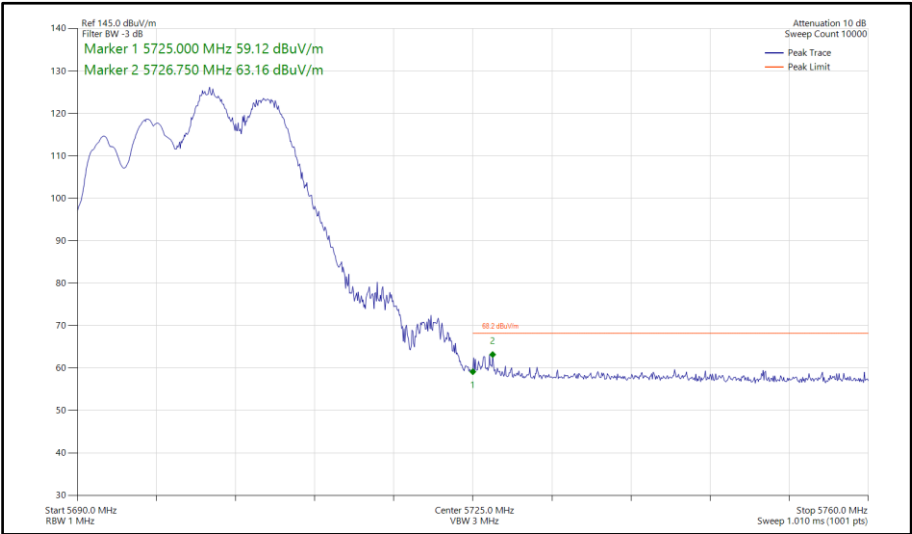
Figure 648 - 802.11be EHT20, RU106+26-83, CDD, Core 0-1 - 5700 MHz Band Edge Frequency 5725 MHz
