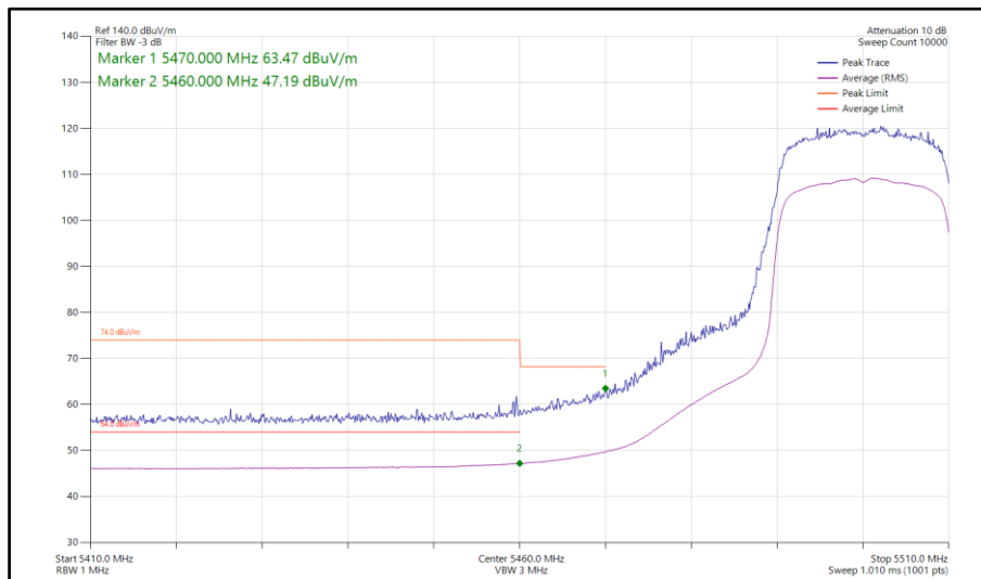
Figure 661 - 802.11ax HE20, SU, SDM, Core 0-1 - 5500 MHz Band Edge Frequency 5470 MHz
