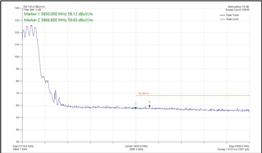
Figure 653 - 802.11ax HE20, SU, CDD, Core 0-1 - 5720 MHz Band Edge Frequency 5850 MHz
