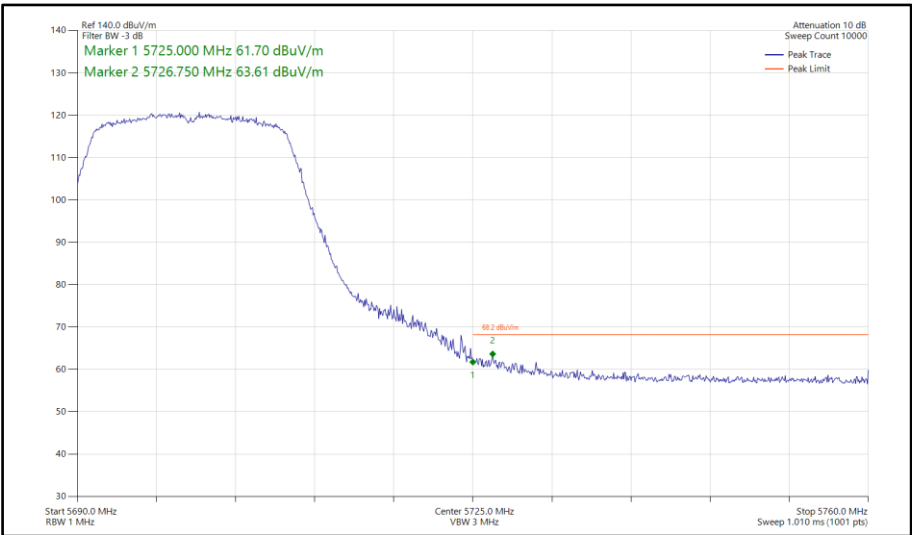
Figure 670 - 802.11n HT20, SDM, Core 0-1 - 5700 MHz Band Edge Frequency 5725 MHz
