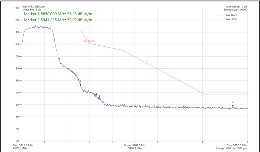
Figure 694 - 802.11ac VHT20, TxBF, Core 0-1 - 5825 MHz Band Edge Frequency 5850 MHz
