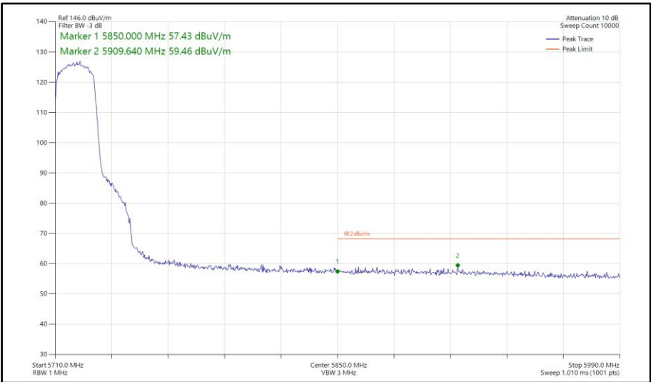
Figure 695 - 802.11ax HE20, SU, TxBF, Core 0-1 - 5720 MHz Band Edge Frequency 5850 MHz
