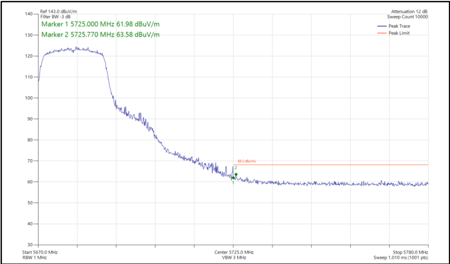
Figure 669 - 802.11n HT20, SDM, Core 0-1 - 5680 MHz Band Edge Frequency 5725 MHz
