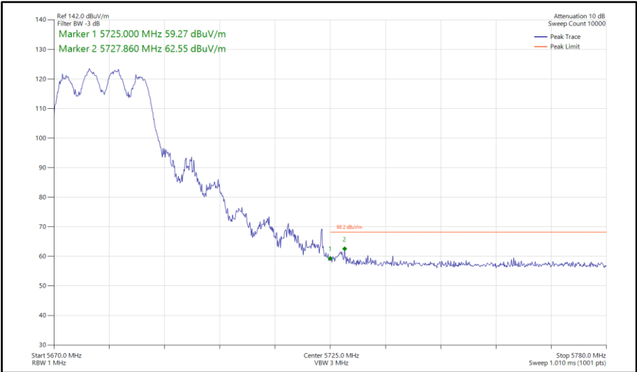
Figure 645 - 802.11ax HE20, SU, CDD, Core 0-1 - 5680 MHz Band Edge Frequency 5725 MHz
