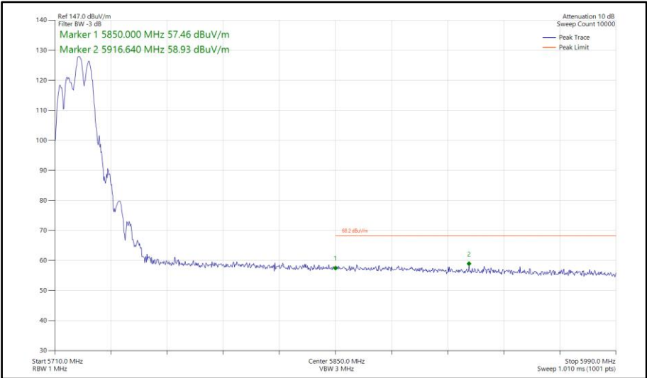
Figure 657 - 802.11be EHT20, RU106+26-83, CDD, Core 0-1 - 5720 MHz Band Edge Frequency 5850 MHz
