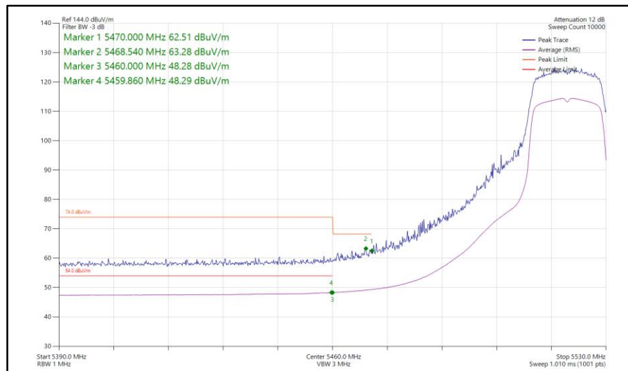
Figure 684 - 802.11ac VHT20, TxBF, Core 0-1 - 5520 MHz Band Edge Frequency 5470 MHz
