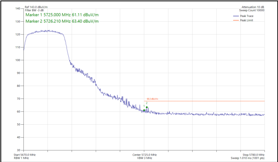
Figure 689 - 802.11ac VHT20, TxBF, Core 0-1 - 5680 MHz Band Edge Frequency 5725 MHz
