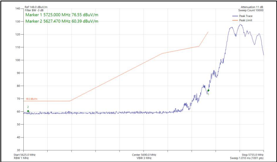
Figure 640 - 802.11be EHT20, RU106+26-82, CDD, Core 0-1 - 5745 MHz Band Edge Frequency 5725 MHz
