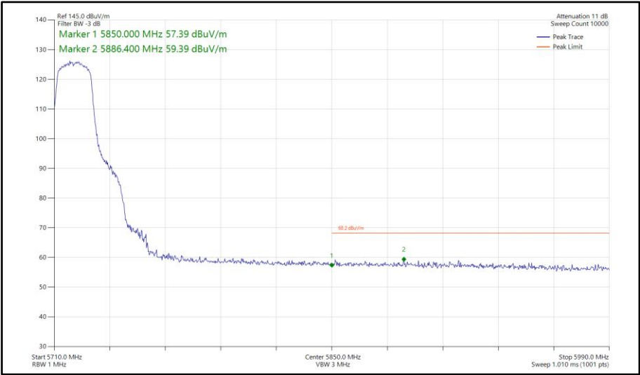
Figure 693 - 802.11ac VHT20, TxBF, Core 0-1 - 5720 MHz Band Edge Frequency 5850 MHz
