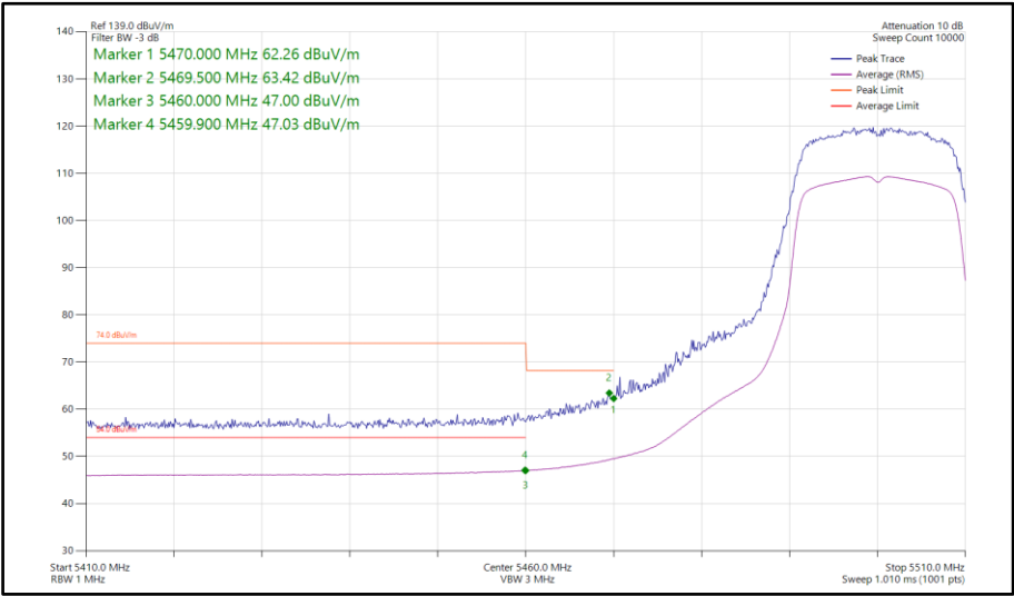
Figure 659 - 802.11n HT20, SDM, Core 0-1 - 5500 MHz Band Edge Frequency 5470 MHz
