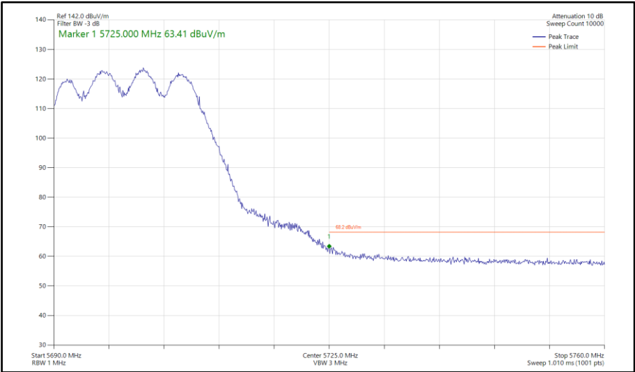
Figure 646 - 802.11ax HE20, SU, CDD, Core 0-1 - 5700 MHz Band Edge Frequency 5725 MHz
