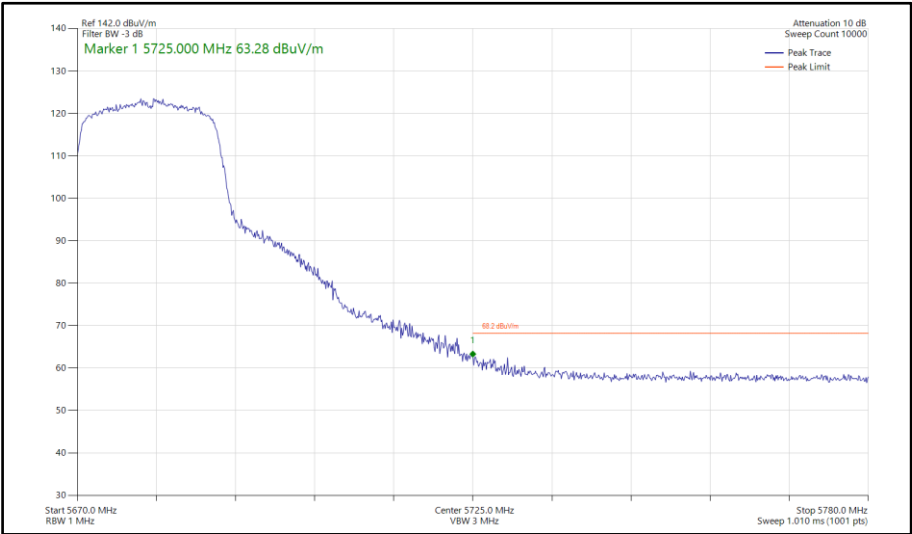
Figure 671 - 802.11ax HE20, SU, SDM, Core 0-1 - 5680 MHz Band Edge Frequency 5725 MHz
