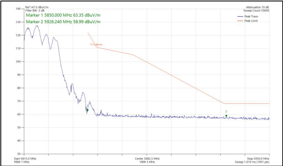
Figure 656 - 802.11ax HE20, RU106-53, CDD, Core 0-1 - 5825 MHz Band Edge Frequency 5850 MHz
