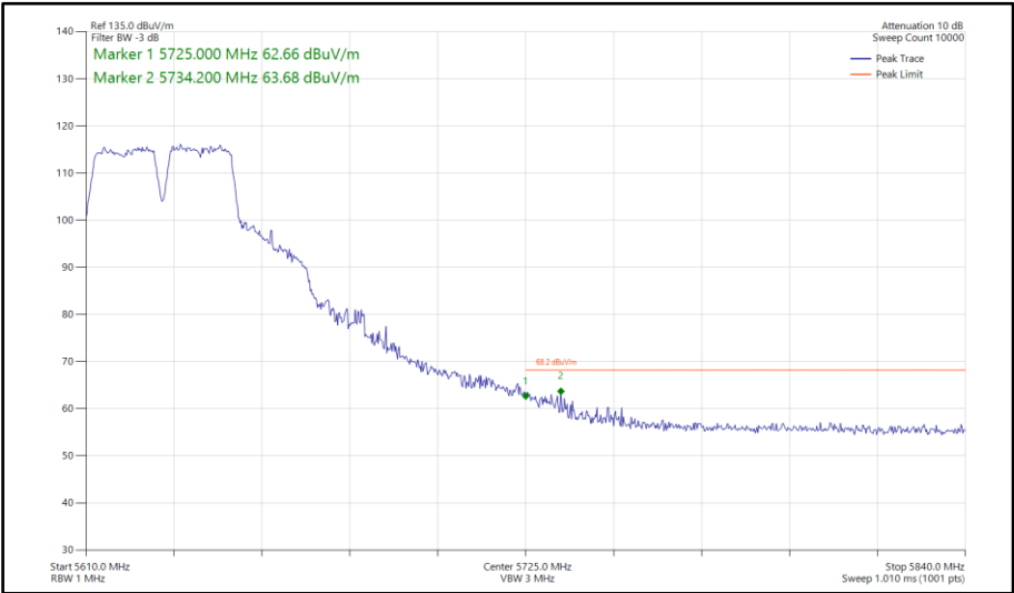
Figure 715 - 802.11a a40, SISO, Core 0 - 5630 MHz Band Edge Frequency 5725 MHz
