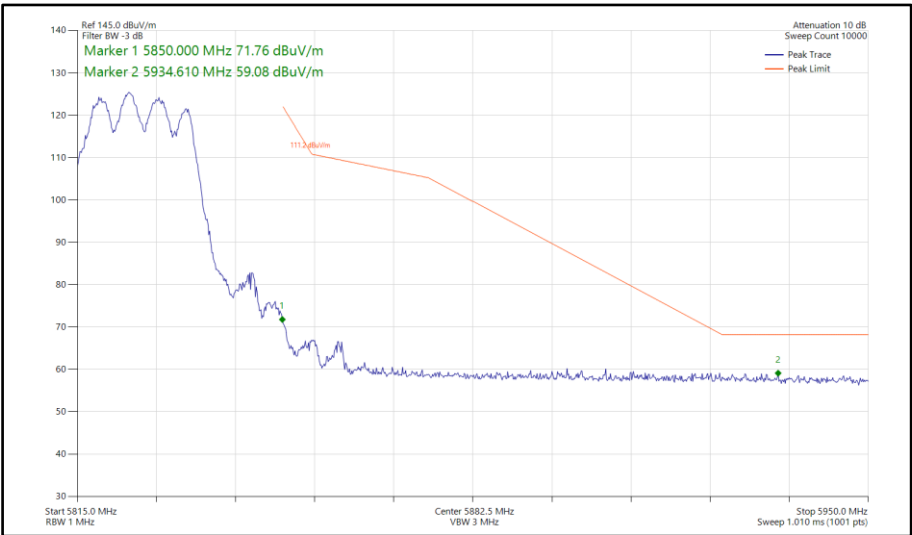
Figure 655 - 802.11ax HE20, SU, CDD, Core 0-1 - 5825 MHz Band Edge Frequency 5850 MHz
