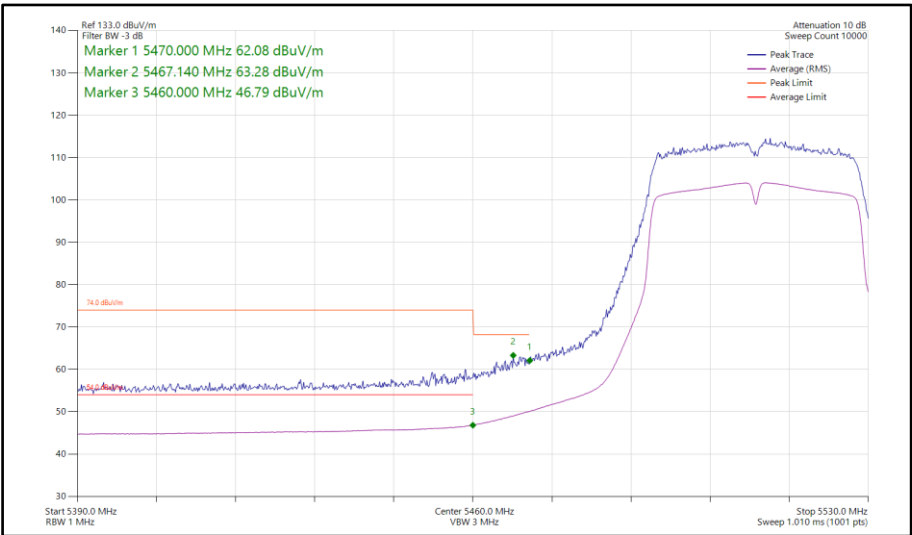
Figure 700 - 802.11n HT40, SISO, Core 0 - 5510 MHz Band Edge Frequency 5470 MHz
