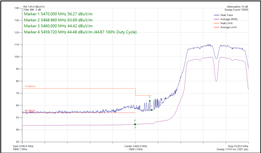
Figure 697 - 802.11a a40, SISO, Core 0 - 5510 MHz Band Edge Frequency 5470 MHz
