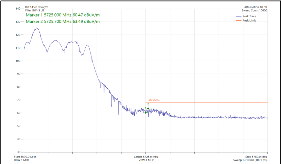
Figure 647 - 802.11ax HE20, RU52-37, CDD, Core 0-1 - 5700 MHz Band Edge Frequency 5725 MHz
