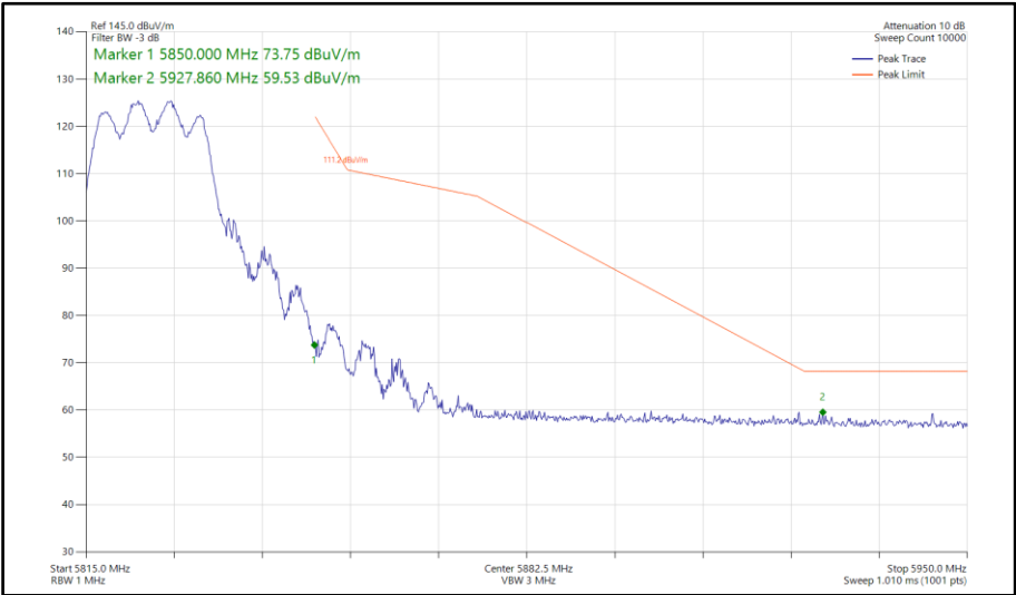
Figure 650 - 802.11a, CDD, Core 0-1 - 5825 MHz Band Edge Frequency 5850 MHz
