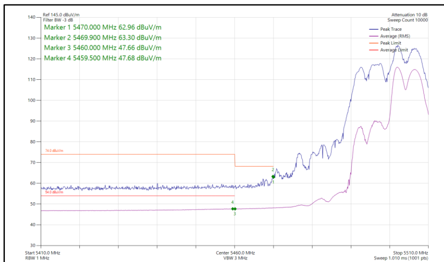
Figure 633 - 802.11ax HE20, RU106-54, CDD, Core 0-1 - 5500 MHz Band Edge Frequency 5470 MHz
