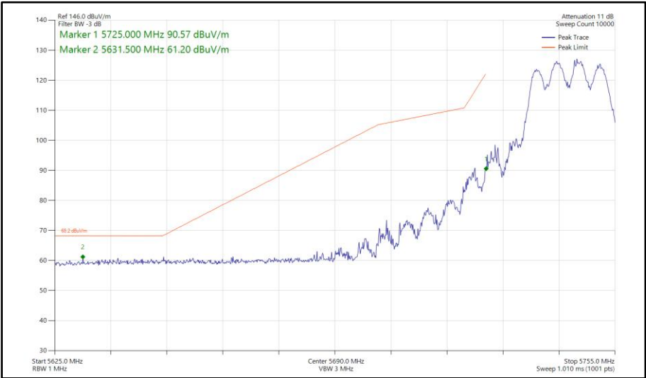
Figure 638 - 802.11ax HE20, SU, CDD, Core 0-1 - 5745 MHz Band Edge Frequency 5725 MHz
