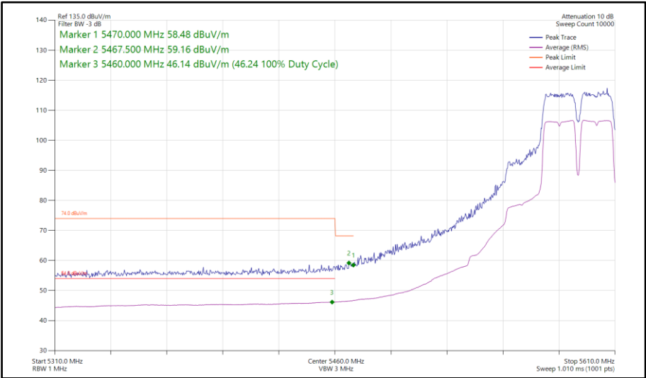
Figure 699 - 802.11a a40, SISO, Core 0 - 5590 MHz Band Edge Frequency 5470 MHz
