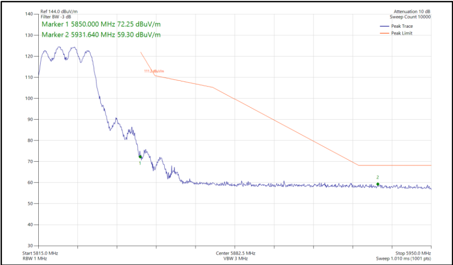
Figure 652 - 802.11n HT20, CDD, Core 0-1 - 5825 MHz Band Edge Frequency 5850 MHz
