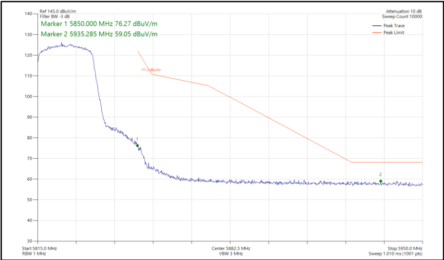
Figure 696 - 802.11ax HE20, SU, TxBF, Core 0-1 - 5825 MHz Band Edge Frequency 5850 MHz
