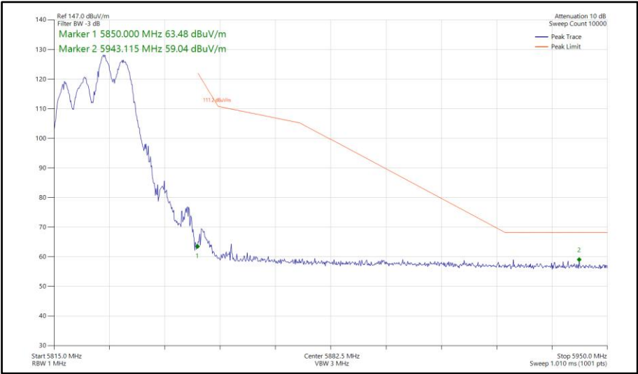
Figure 680 - 802.11ax HE20, RU106-54, SDM, Core 0-1 - 5825 MHz Band Edge Frequency 5850 MHz
