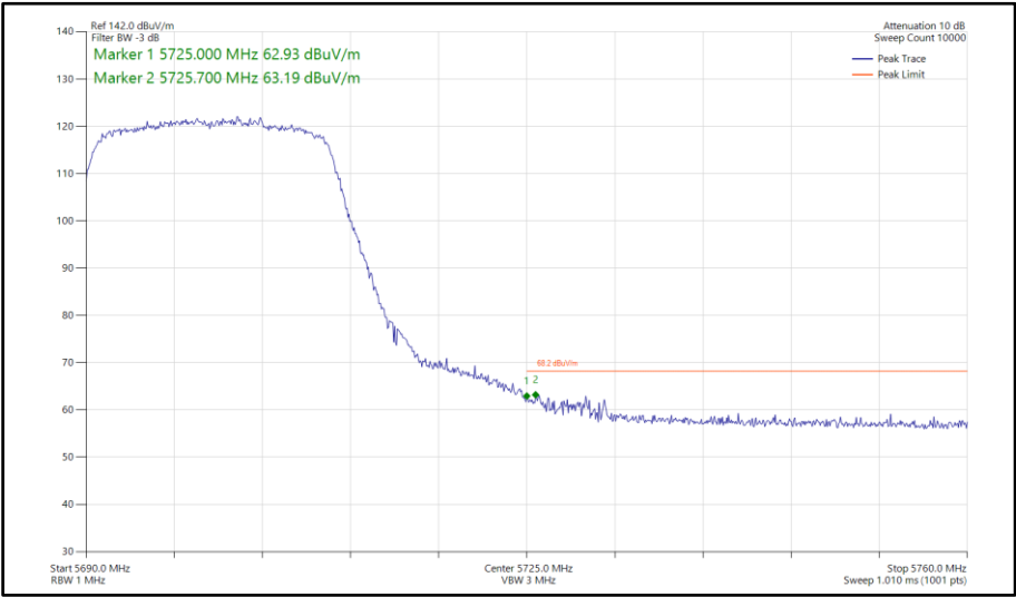
Figure 692 - 802.11ax HE20, SU, TxBF, Core 0-1 - 5700 MHz Band Edge Frequency 5725 MHz
