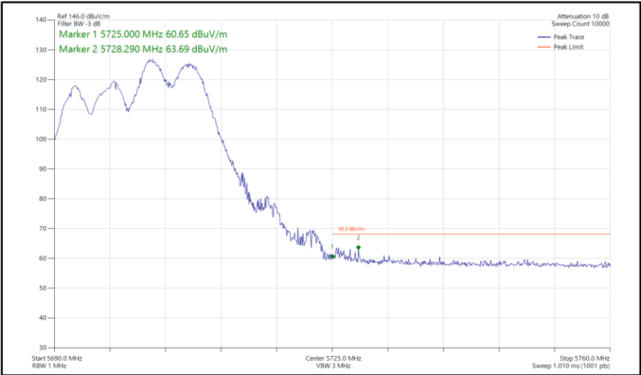
Figure 673 - 802.11ax HE20, RU106-54, SDM, Core 0-1 - 5700 MHz Band Edge Frequency 5725 MHz
