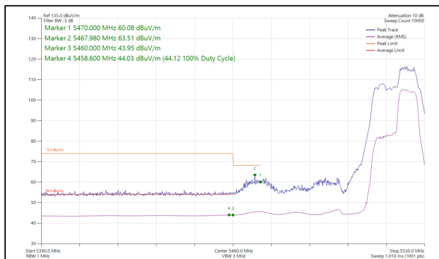
Figure 708 - 802.11be EHT40, RU52+26-75, SISO, Core 0 - 5510 MHz Band Edge Frequency 5470 MHz
