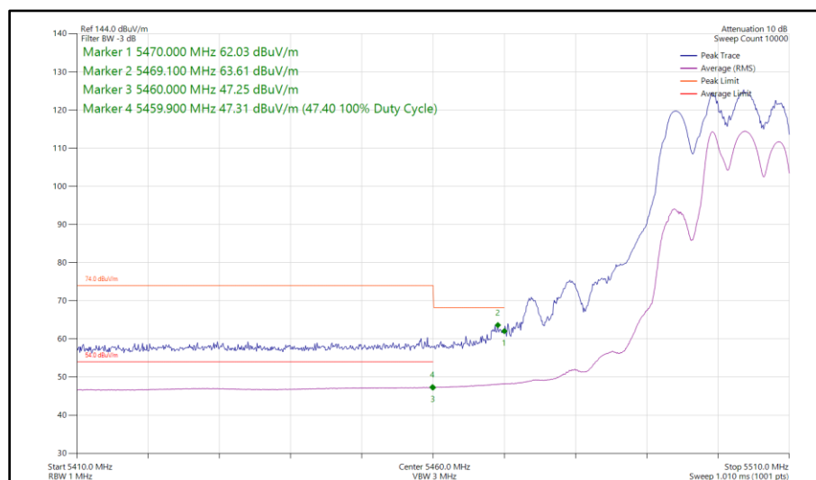
Figure 635 - 802.11be EHT20, RU106+26-83, CDD, Core 0-1 - 5500 MHz Band Edge Frequency 5470 MHz
