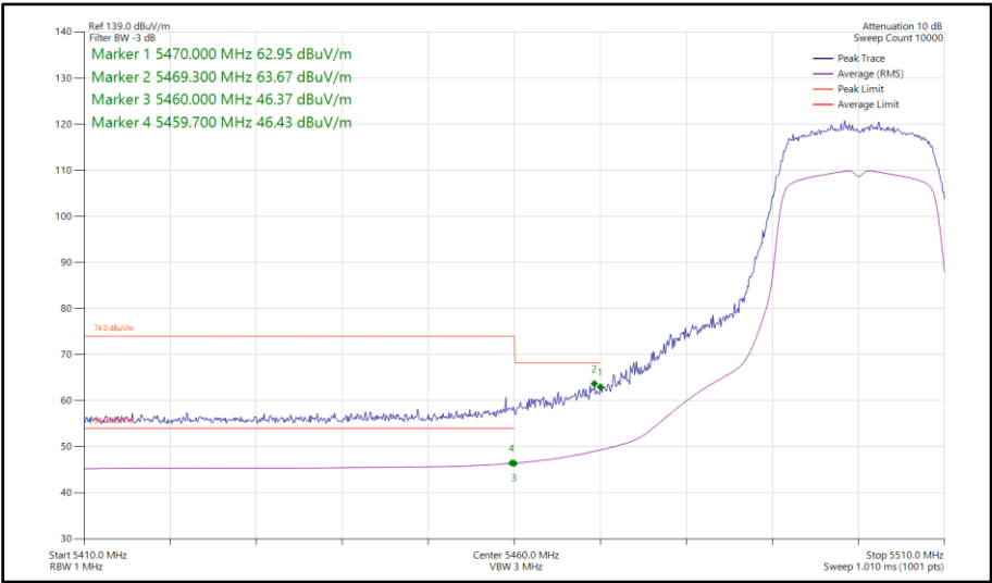
Figure 683 - 802.11ac VHT20, TxBF, Core 0-1 - 5500 MHz Band Edge Frequency 5470 MHz
