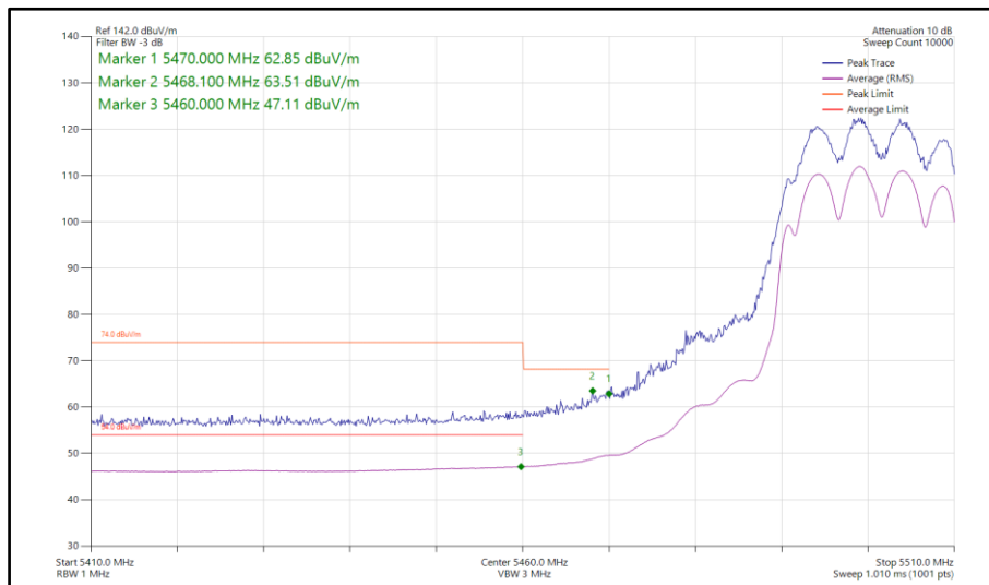
Figure 632 - 802.11ax HE20, SU, CDD, Core 0-1 - 5500 MHz Band Edge Frequency 5470 MHz
