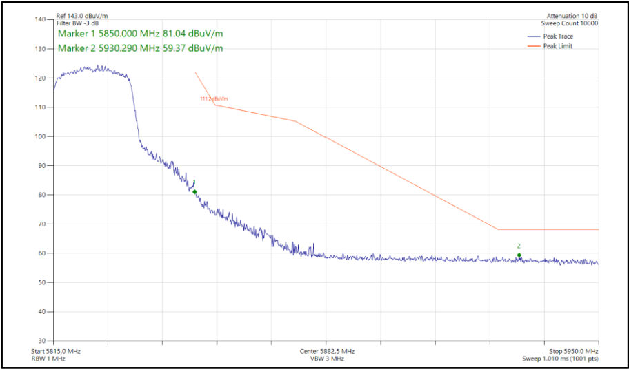
Figure 679 - 802.11ax HE20, SU, SDM, Core 0-1 - 5825 MHz Band Edge Frequency 5850 MHz
