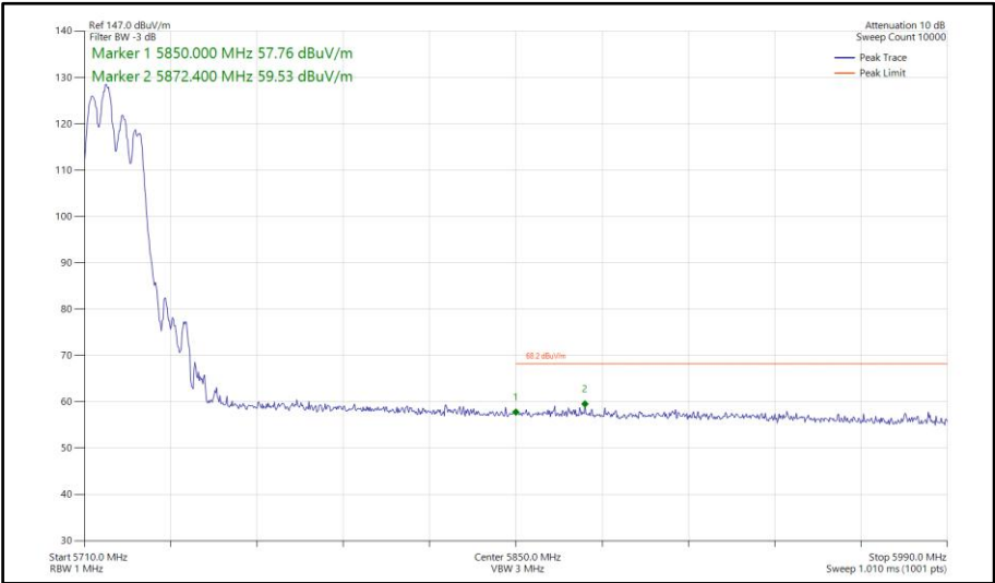
Figure 654 - 802.11ax HE20, RU106-53, CDD, Core 0-1 - 5720 MHz Band Edge Frequency 5850 MHz
