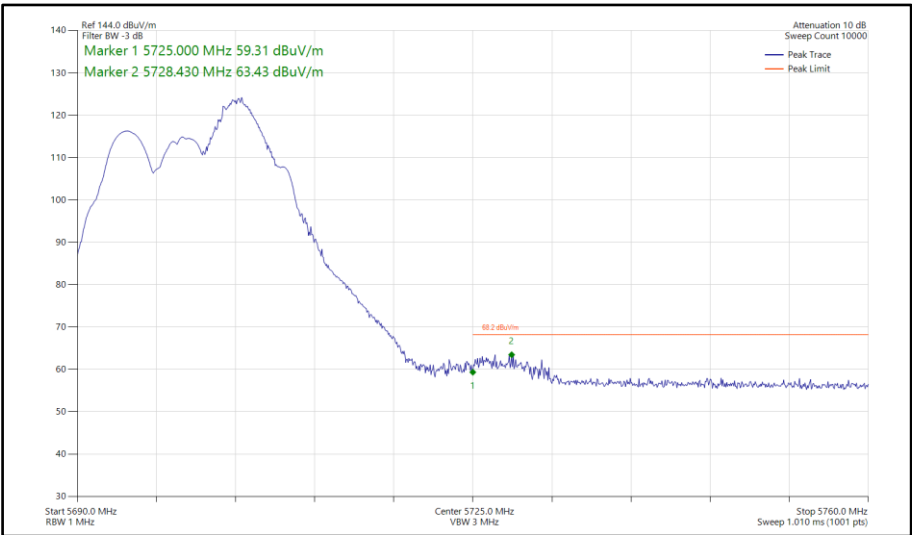
Figure 674 - 802.11be EHT20, RU52+26-72, SDM, Core 0-1 - 5700 MHz Band Edge Frequency 5725 MHz
