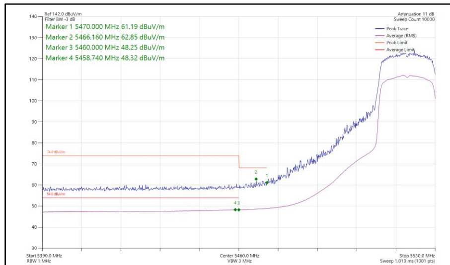
Figure 663 - 802.11ax HE20, SU, SDM, Core 0-1 - 5520 MHz Band Edge Frequency 5470 MHz
