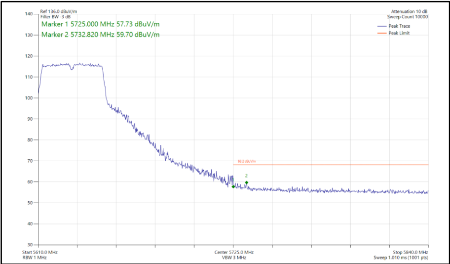
Figure 717 - 802.11n HT40, SISO, Core 0 - 5630 MHz Band Edge Frequency 5725 MHz
