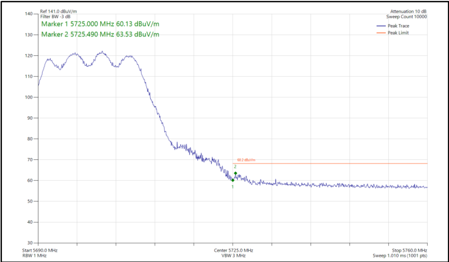
Figure 644 - 802.11n HT20, CDD, Core 0-1 - 5700 MHz Band Edge Frequency 5725 MHz
