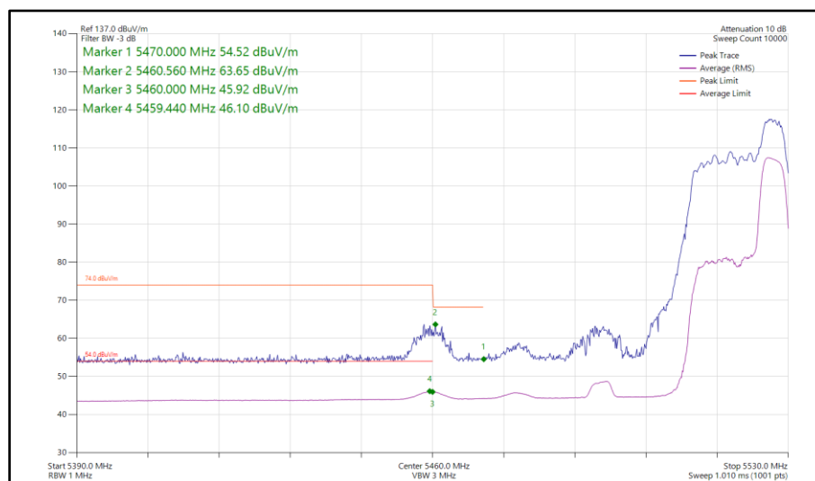
Figure 704 - 802.11ax HE40, RU52-44, SISO, Core 0 - 5510 MHz Band Edge Frequency 5470 MHz
