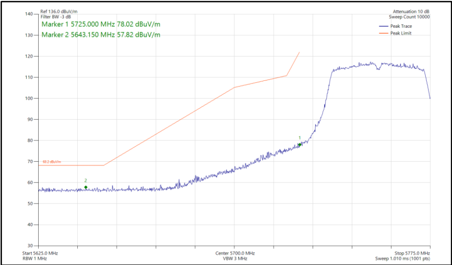
Figure 711 - 802.11n HT40, SISO, Core 0 - 5755 MHz Band Edge Frequency 5725 MHz
