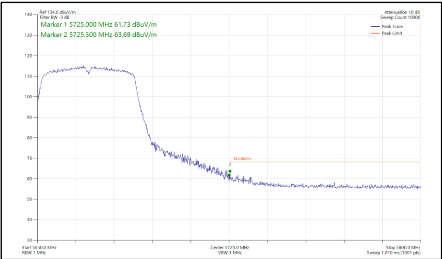
Figure 718 - 802.11n HT40, SISO, Core 0 - 5670 MHz Band Edge Frequency 5725 MHz
