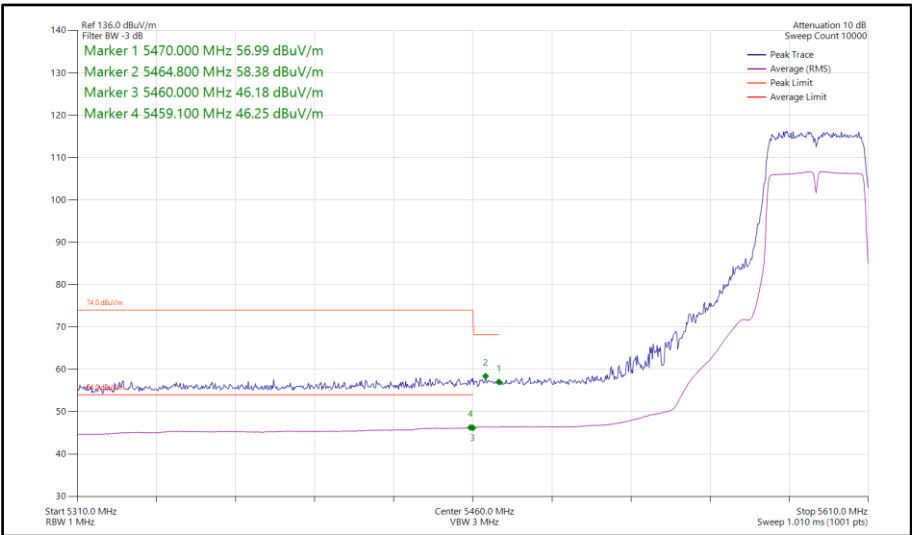
Figure 702 - 802.11n HT40, SISO, Core 0 - 5590 MHz Band Edge Frequency 5470 MHz
