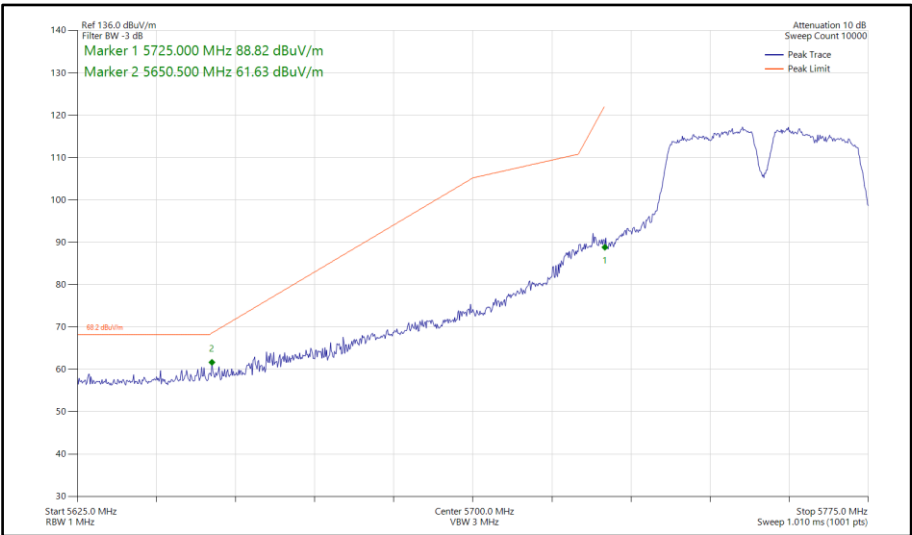
Figure 710 - 802.11a a40, SISO, Core 0 - 5755 MHz Band Edge Frequency 5725 MHz
