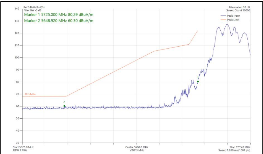
Figure 668 - 802.11be EHT20, RU106+26-82, SDM, Core 0-1 - 5745 MHz Band Edge Frequency 5725 MHz
