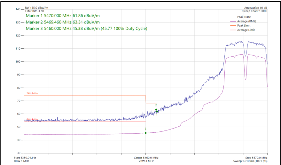
Figure 698 - 802.11a a40, SISO, Core 0 - 5550 MHz Band Edge Frequency 5470 MHz
