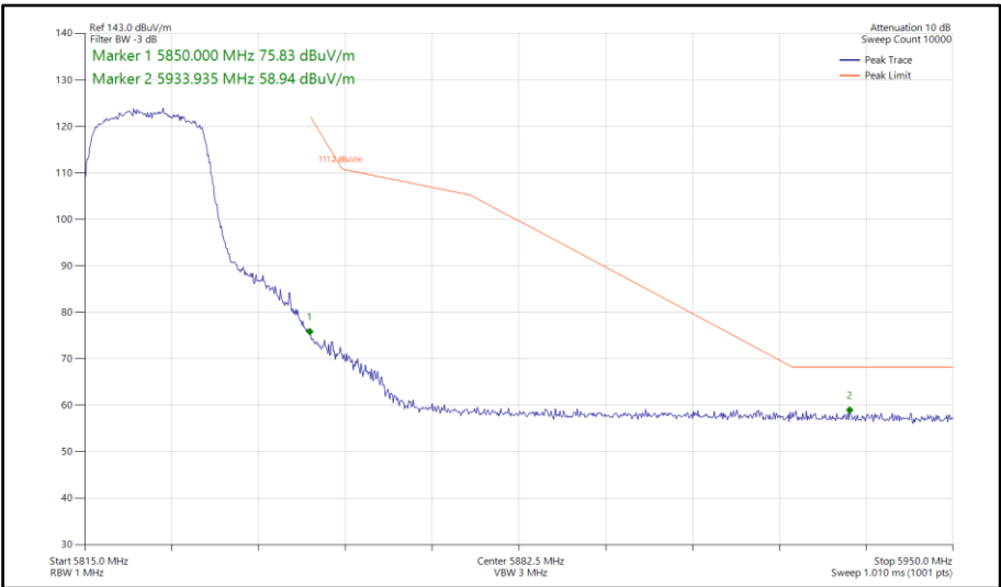
Figure 676 - 802.11n HT20, SDM, Core 0-1 - 5825 MHz Band Edge Frequency 5850 MHz
