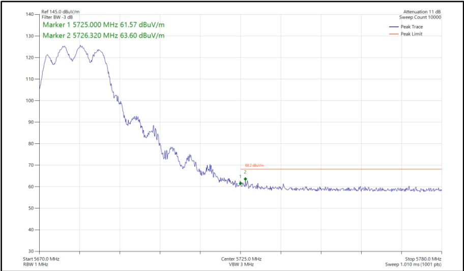
Figure 641 - 802.11a, CDD, Core 0-1 - 5680 MHz Band Edge Frequency 5725 MHz
