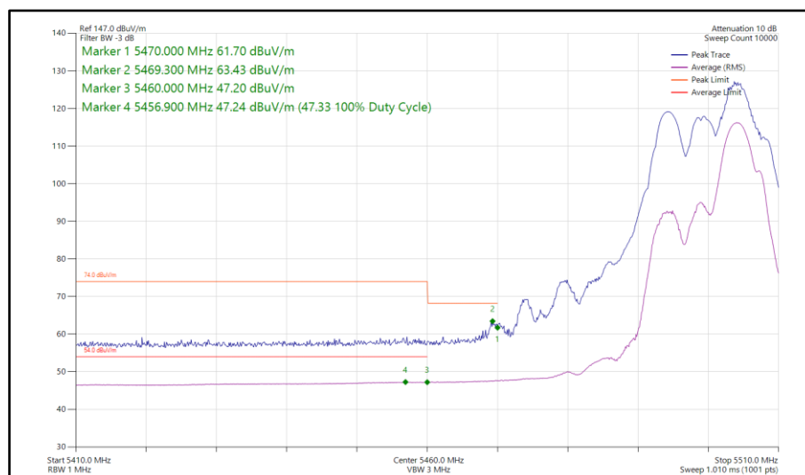
Figure 664 - 802.11be EHT20, RU52+26-72, SDM, Core 0-1 - 5500 MHz Band Edge Frequency 5470 MHz
