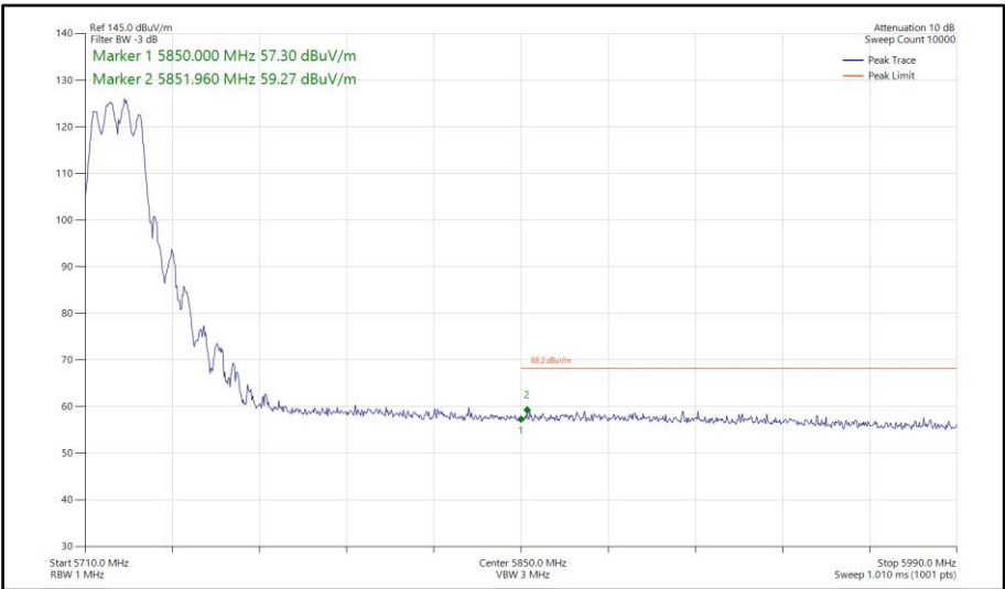
Figure 649 - 802.11a, CDD, Core 0-1 - 5720 MHz Band Edge Frequency 5850 MHz
