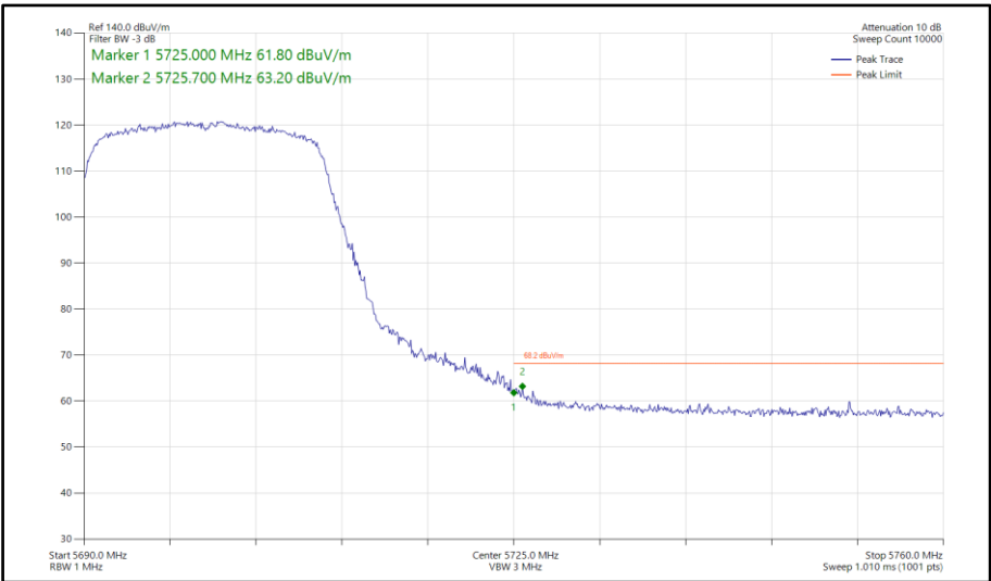
Figure 672 - 802.11ax HE20, SU, SDM, Core 0-1 - 5700 MHz Band Edge Frequency 5725 MHz
