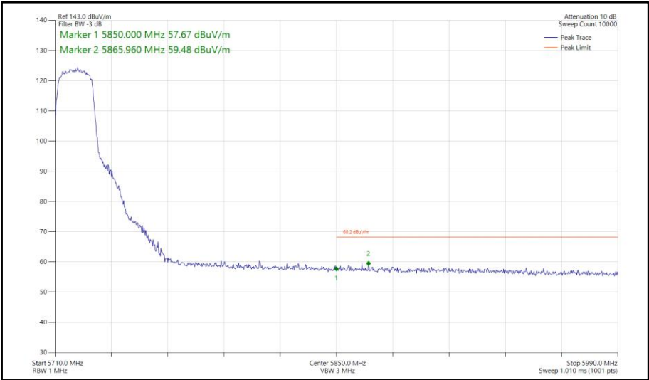
Figure 675 - 802.11n HT20, SDM, Core 0-1 - 5720 MHz Band Edge Frequency 5850 MHz
