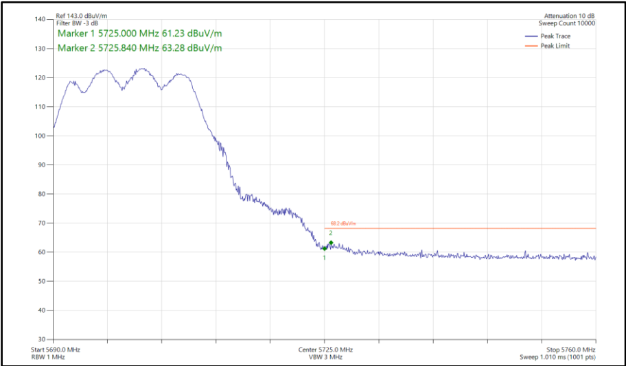
Figure 642 - 802.11a, CDD, Core 0-1 - 5700 MHz Band Edge Frequency 5725 MHz
