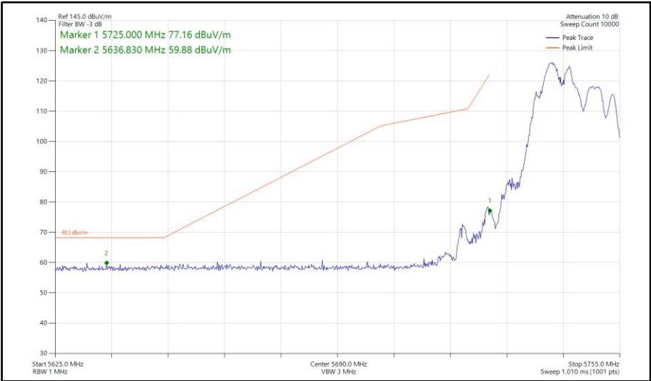
Figure 667 - 802.11ax HE20, RU106-53, SDM, Core 0-1 - 5745 MHz Band Edge Frequency 5725 MHz
