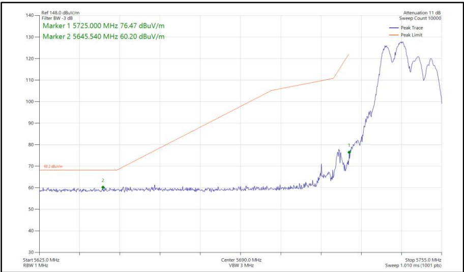
Figure 639 - 802.11ax HE20, RU106-53, CDD, Core 0-1 - 5745 MHz Band Edge Frequency 5725 MHz
