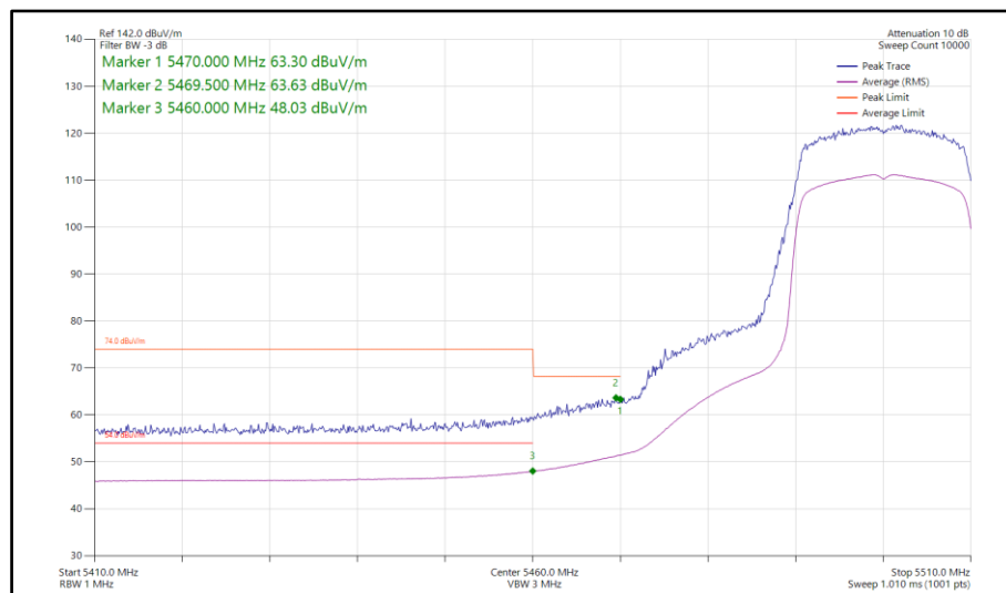
Figure 685 - 802.11ax HE20, SU, TxBF, Core 0-1 - 5500 MHz Band Edge Frequency 5470 MHz
