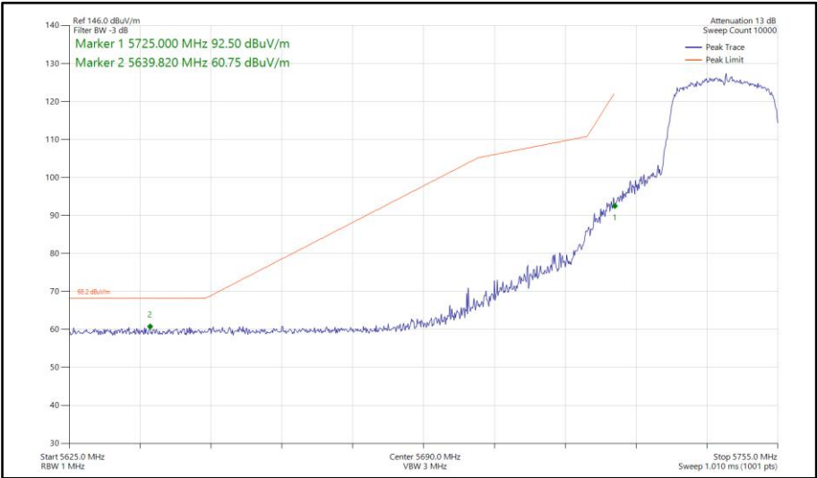
Figure 688 - 802.11ax HE20, SU, TxBF, Core 0-1 - 5745 MHz Band Edge Frequency 5725 MHz
