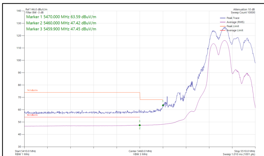
Figure 662 - 802.11ax HE20, RU106-53, SDM, Core 0-1 - 5500 MHz Band Edge Frequency 5470 MHz
