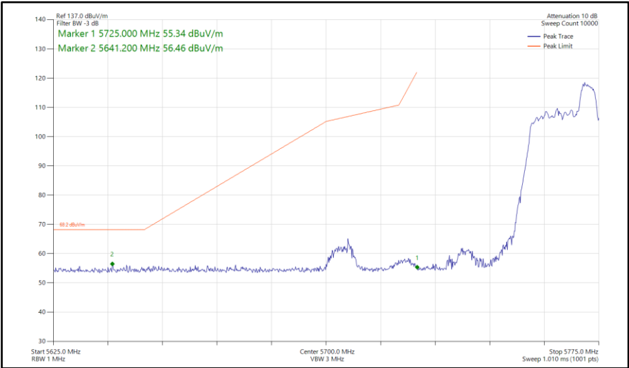
Figure 713 - 802.11ax HE40, RU52-44, SISO, Core 0 - 5755 MHz Band Edge Frequency 5725 MHz
