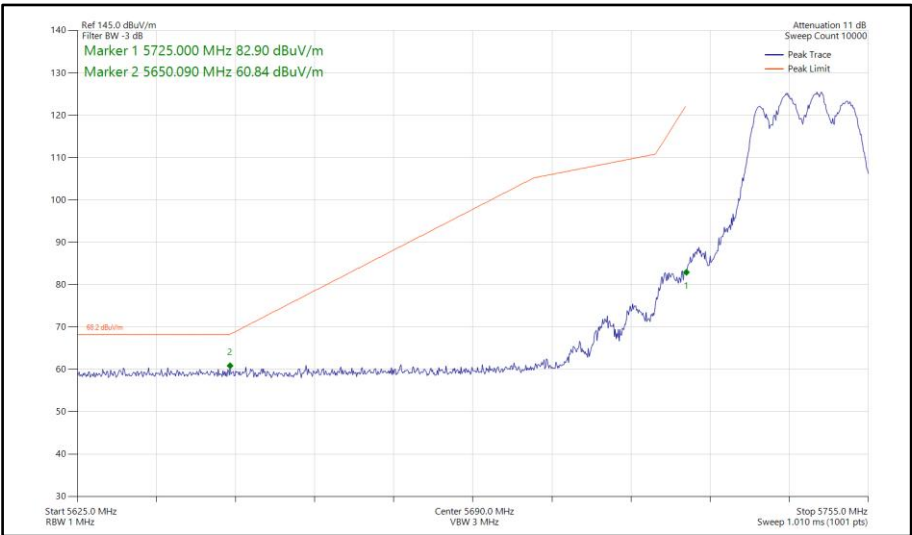
Figure 637 - 802.11n HT20, CDD, Core 0-1 - 5745 MHz Band Edge Frequency 5725 MHz
