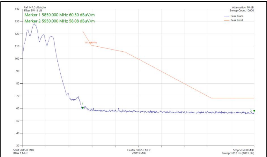
Figure 682 - 802.11be EHT20, RU52+26-70, SDM, Core 0-1 - 5825 MHz Band Edge Frequency 5850 MHz
