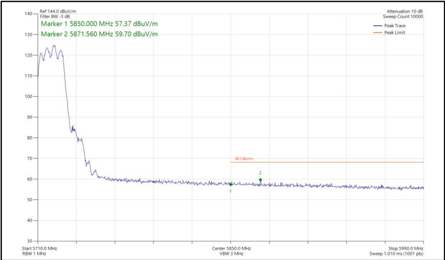
Figure 651 - 802.11n HT20, CDD, Core 0-1 - 5720 MHz Band Edge Frequency 5850 MHz
