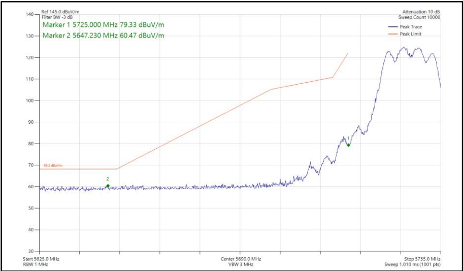
Figure 636 - 802.11a, CDD, Core 0-1 - 5745 MHz Band Edge Frequency 5725 MHz
