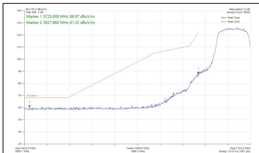
Figure 687 - 802.11ac VHT20, TxBF, Core 0-1 - 5745 MHz Band Edge Frequency 5725 MHz
