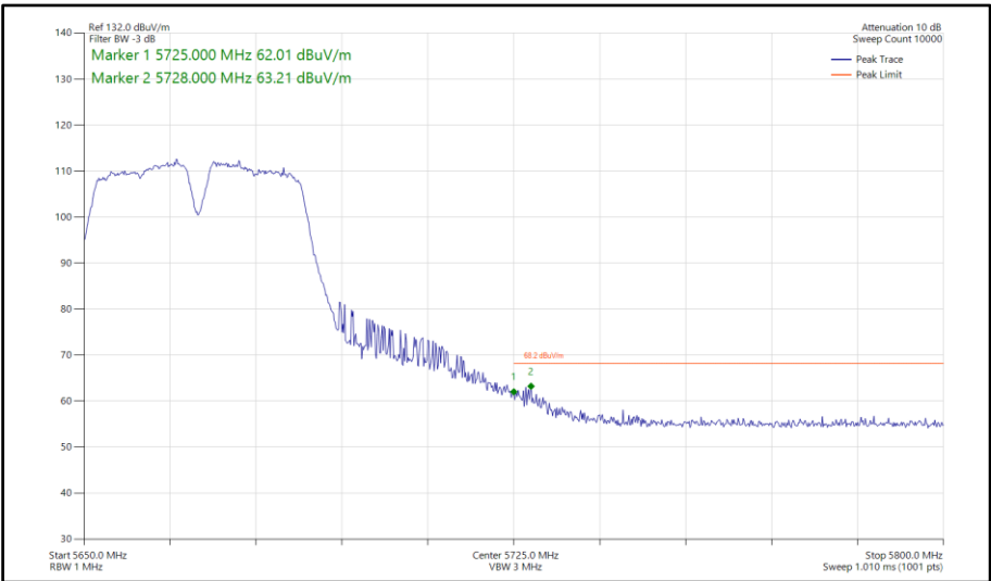
Figure 716 - 802.11a a40, SISO, Core 0 - 5670 MHz Band Edge Frequency 5725 MHz
