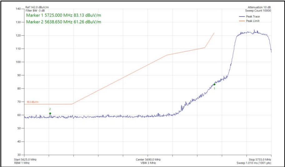
Figure 665 - 802.11n HT20, SDM, Core 0-1 - 5745 MHz Band Edge Frequency 5725 MHz
