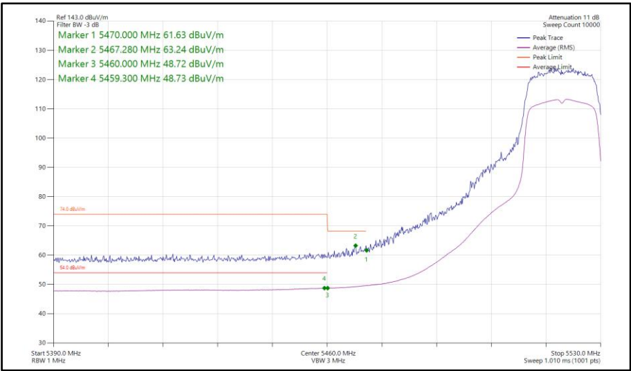
Figure 660 - 802.11n HT20, SDM, Core 0-1 - 5520 MHz Band Edge Frequency 5470 MHz
