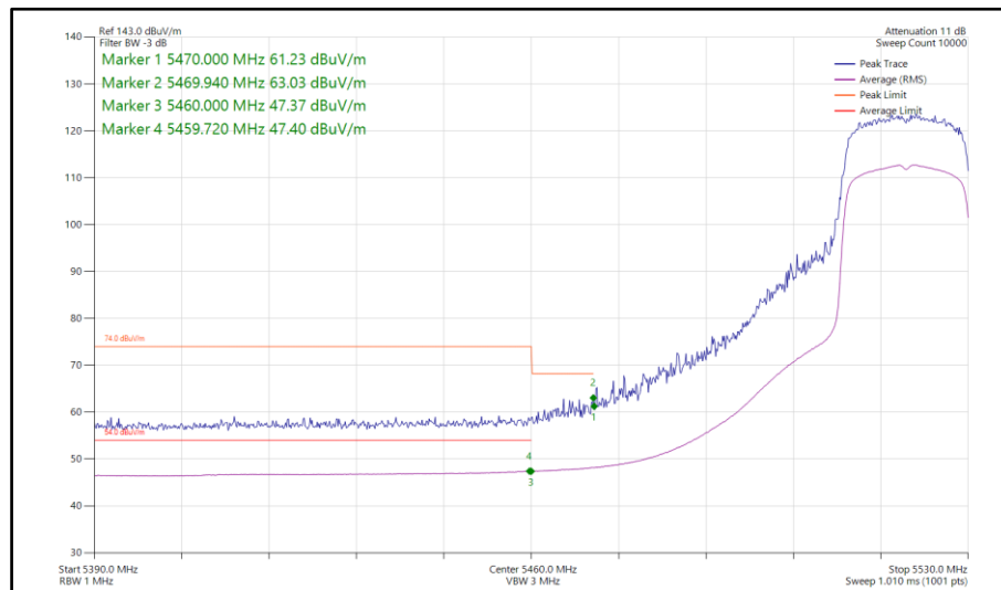
Figure 686 - 802.11ax HE20, SU, TxBF, Core 0-1 - 5520 MHz Band Edge Frequency 5470 MHz
