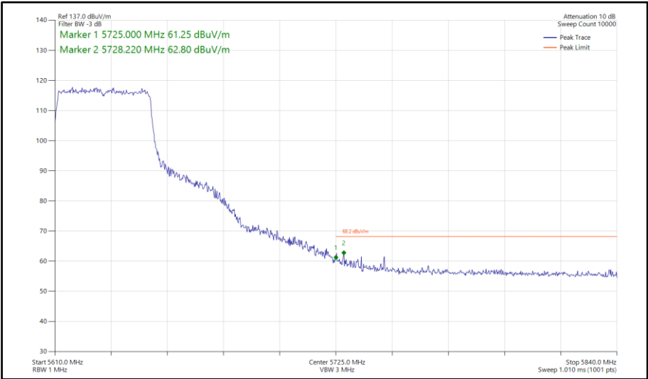
Figure 719 - 802.11ax HE40, SU, SISO, Core 0 - 5630 MHz Band Edge Frequency 5725 MHz
