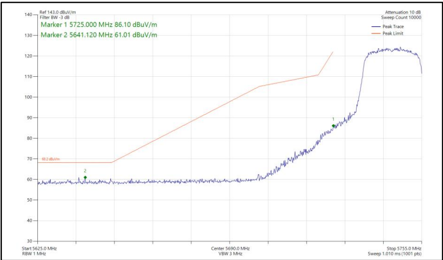
Figure 666 - 802.11ax HE20, SU, SDM, Core 0-1 - 5745 MHz Band Edge Frequency 5725 MHz
