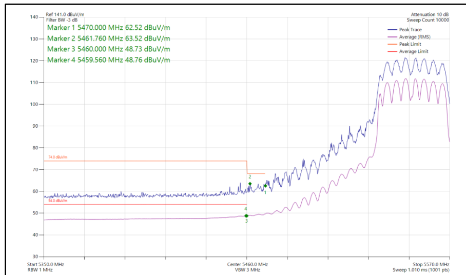
Figure 773 - 802.11n HT40, CDD, Core 0-1 - 5550 MHz Band Edge Frequency 5470 MHz
