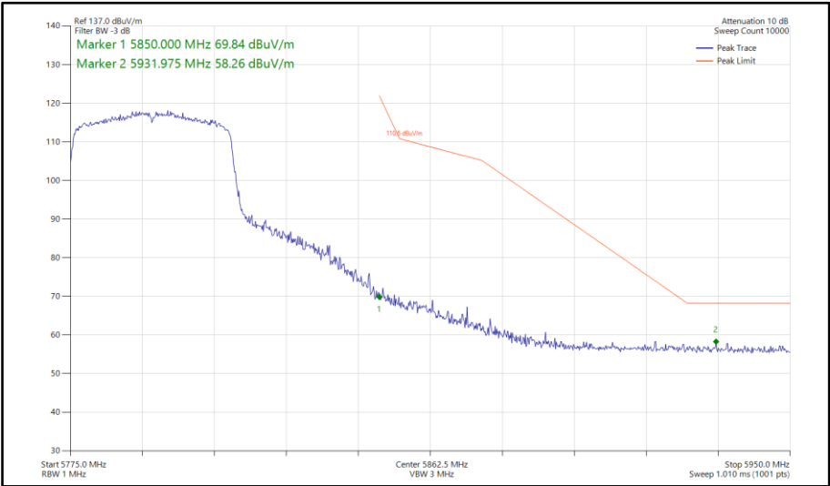
Figure 729 - 802.11ax HE40, SU, SISO, Core 0 - 5795 MHz Band Edge Frequency 5850 MHz
