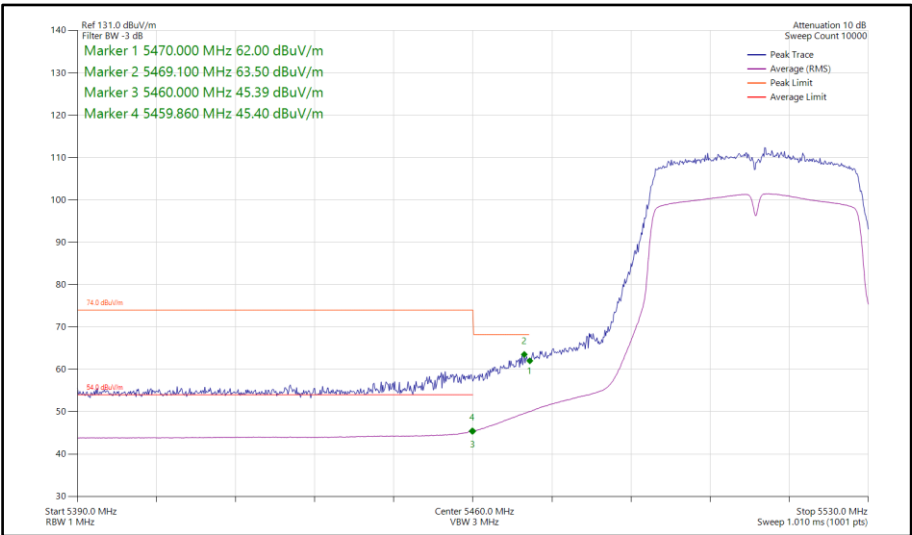
Figure 736 - 802.11n HT40, SISO, Core 1 - 5510 MHz Band Edge Frequency 5470 MHz
