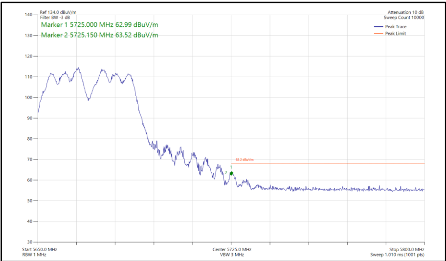
Figure 788 - 802.11a a40, CDD, Core 0-1 - 5670 MHz Band Edge Frequency 5725 MHz
