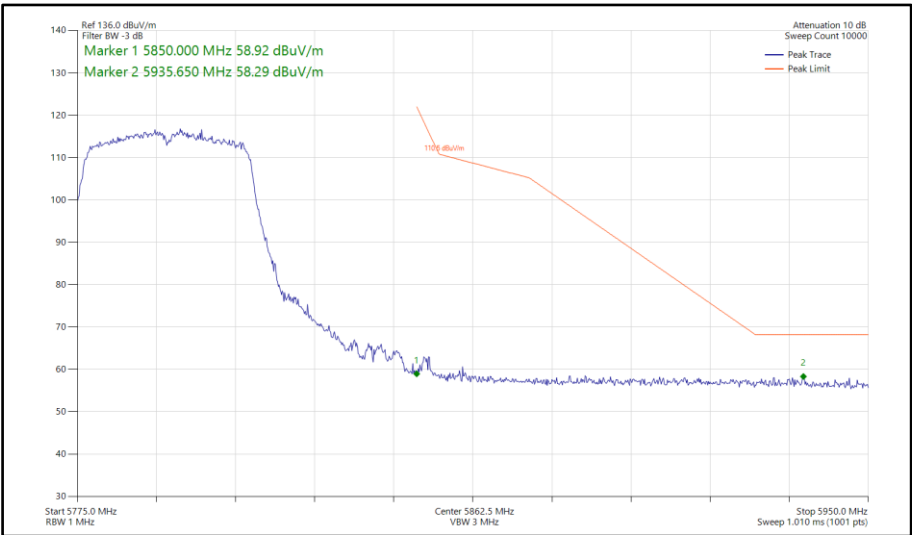
Figure 726 - 802.11n HT40, SISO, Core 0 - 5795 MHz Band Edge Frequency 5850 MHz
