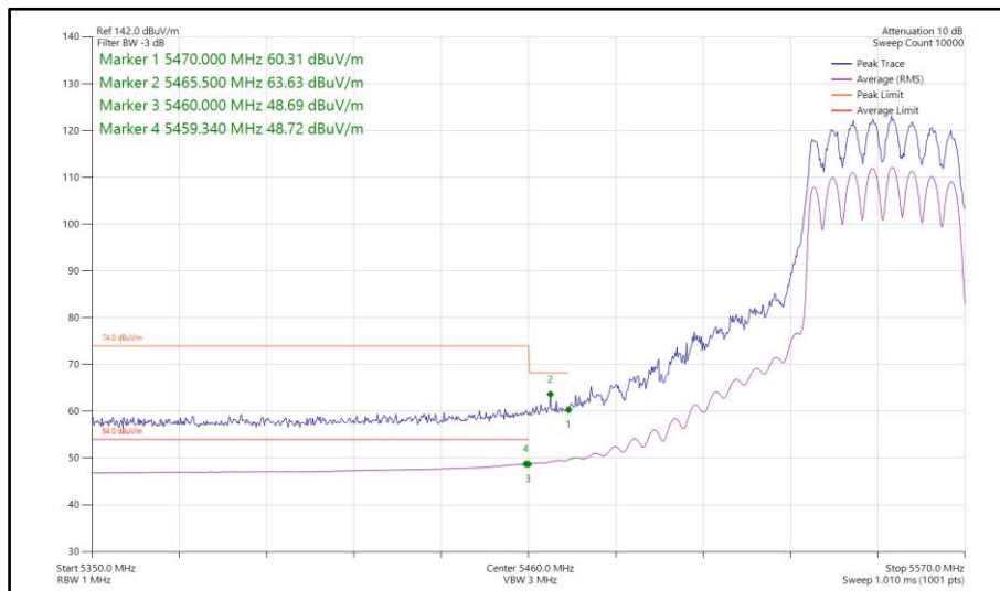
Figure 777 - 802.11ax HE40, SU, CDD, Core 0-1 - 5550 MHz Band Edge Frequency 5470 MHz
