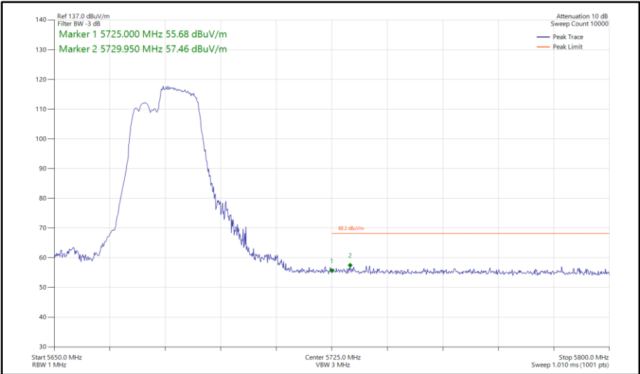
Figure 758 - 802.11be EHT40, RU106+26-85, SISO, Core 1 - 5670 MHz Band Edge Frequency 5725 MHz
