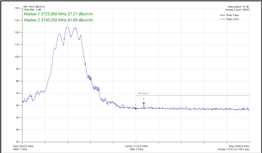
Figure 794 - 802.11be EHT40, RU106+26-85, CDD, Core 0-1 - 5670 MHz Band Edge Frequency 5725 MHz
