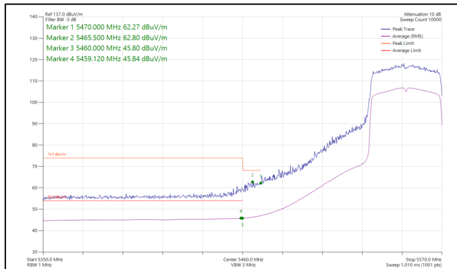
Figure 741 - 802.11ax HE40, SU, SISO, Core 1 - 5550 MHz Band Edge Frequency 5470 MHz
