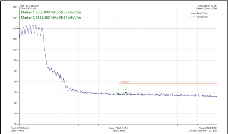
Figure 799 - 802.11ax HE40, SU, CDD, Core 0-1 - 5710 MHz Band Edge Frequency 5850 MHz
