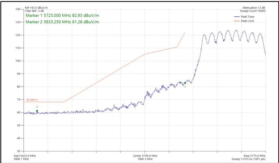
Figure 784 - 802.11ax HE40, SU, CDD, Core 0-1 - 5755 MHz Band Edge Frequency 5725 MHz
