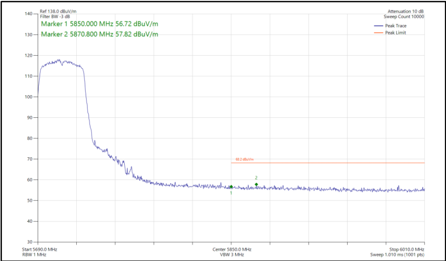
Figure 761 - 802.11n HT40, SISO, Core 1 - 5710 MHz Band Edge Frequency 5850 MHz
