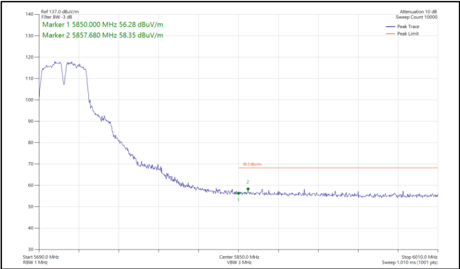
Figure 759 - 802.11a a40, SISO, Core 1 - 5710 MHz Band Edge Frequency 5850 MHz
