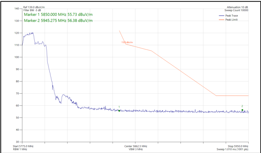
Figure 766 - 802.11ax HE40, RU106-53, SISO, Core 1 - 5795 MHz Band Edge Frequency 5850 MHz
