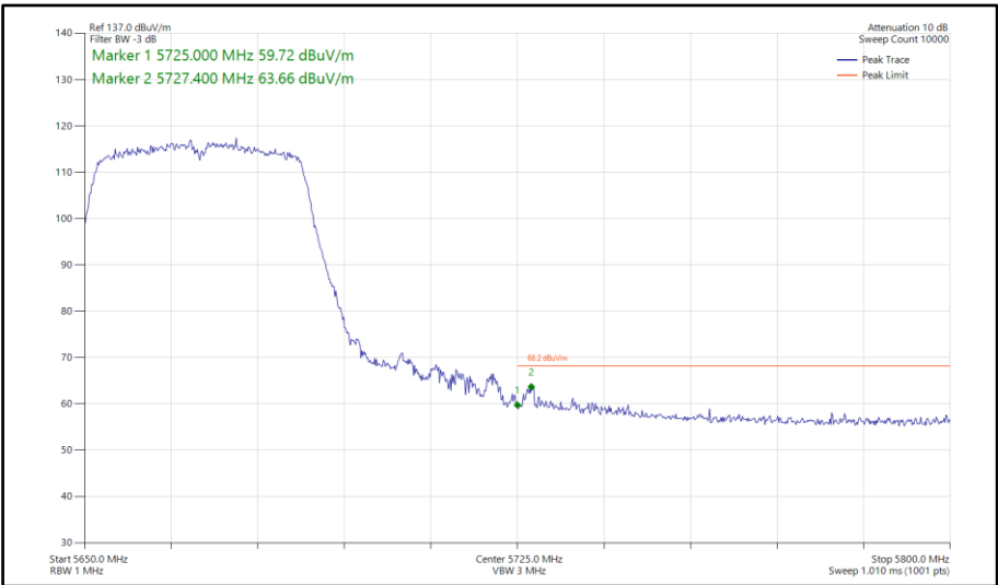
Figure 754 - 802.11n HT40, SISO, Core 1 - 5670 MHz Band Edge Frequency 5725 MHz
