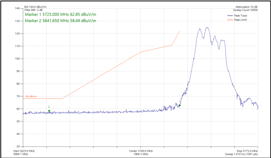
Figure 785 - 802.11ax HE40, RU106-53, CDD, Core 0-1 - 5755 MHz Band Edge Frequency 5725 MHz
