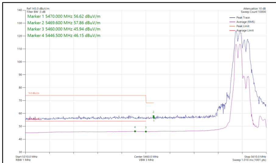
Figure 779 - 802.11ax HE40, RU106-53, CDD, Core 0-1 - 5590 MHz Band Edge Frequency 5470 MHz
