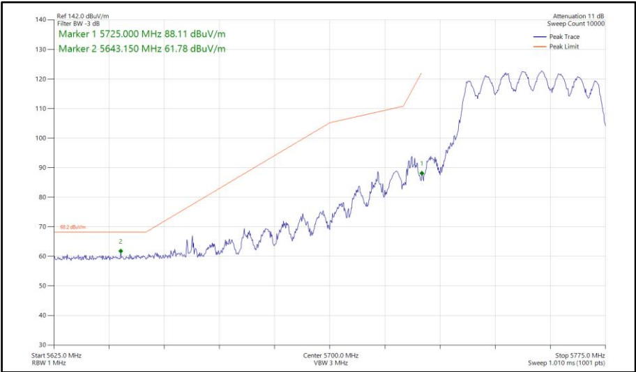
Figure 783 - 802.11n HT40, CDD, Core 0-1 - 5755 MHz Band Edge Frequency 5725 MHz
