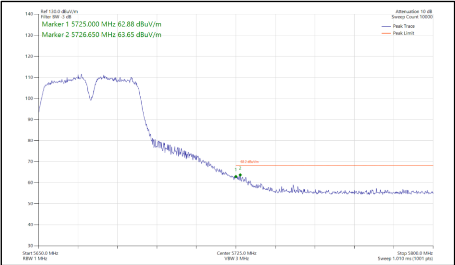
Figure 752 - 802.11a a40, SISO, Core 1 - 5670 MHz Band Edge Frequency 5725 MHz
