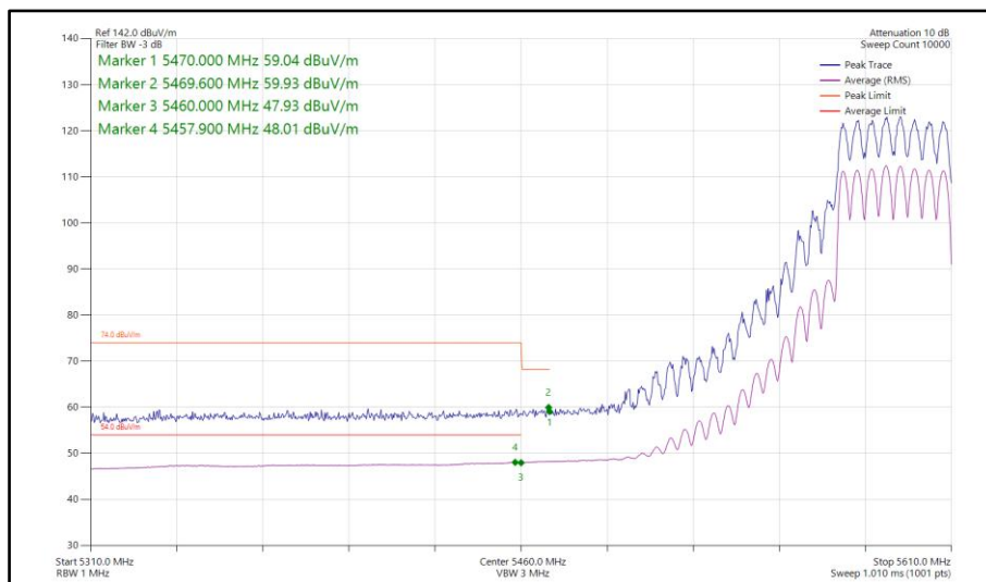
Figure 778 - 802.11ax HE40, SU, CDD, Core 0-1 - 5590 MHz Band Edge Frequency 5470 MHz
