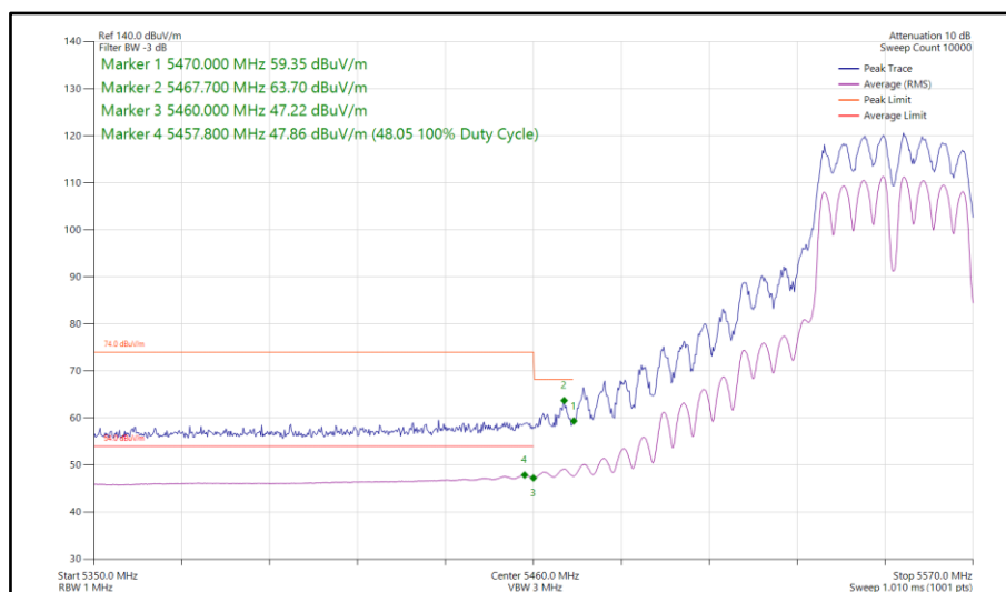
Figure 770 - 802.11a a40, CDD, Core 0-1 - 5550 MHz Band Edge Frequency 5470 MHz
