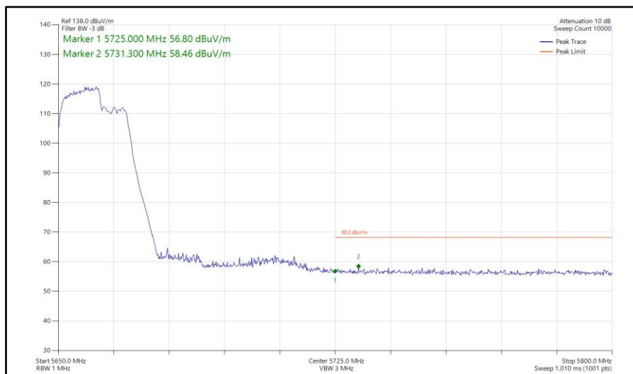
Figure 722 - 802.11be EHT40, RU106+26-82, SISO, Core 0 - 5670 MHz Band Edge Frequency 5725 MHz
