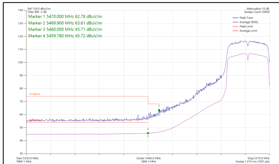
Figure 737 - 802.11n HT40, SISO, Core 1 - 5550 MHz Band Edge Frequency 5470 MHz
