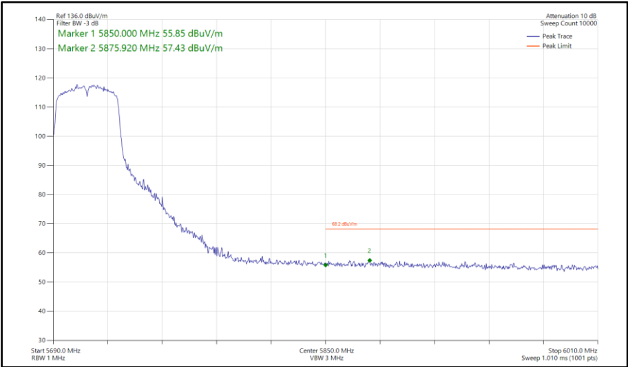
Figure 725 - 802.11n HT40, SISO, Core 0 - 5710 MHz Band Edge Frequency 5850 MHz
