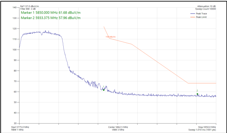
Figure 762 - 802.11n HT40, SISO, Core 1 - 5795 MHz Band Edge Frequency 5850 MHz
