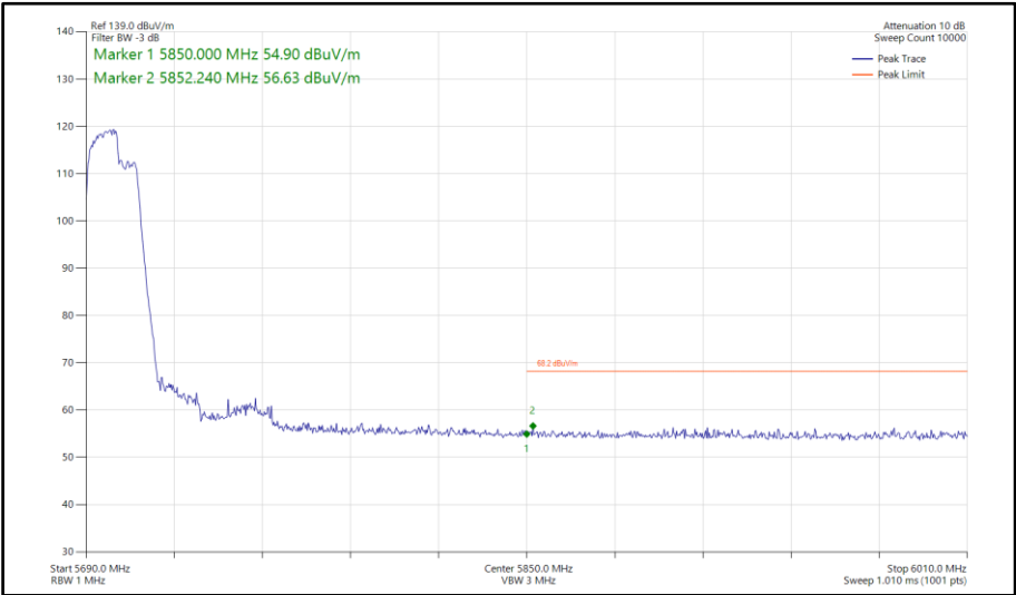
Figure 731 - 802.11be EHT40, RU106+26-82, SISO, Core 0 - 5710 MHz Band Edge Frequency 5850 MHz
