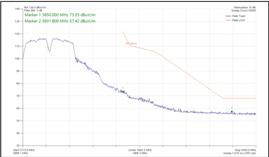
Figure 724 - 802.11a a40, SISO, Core 0 - 5795 MHz Band Edge Frequency 5850 MHz
