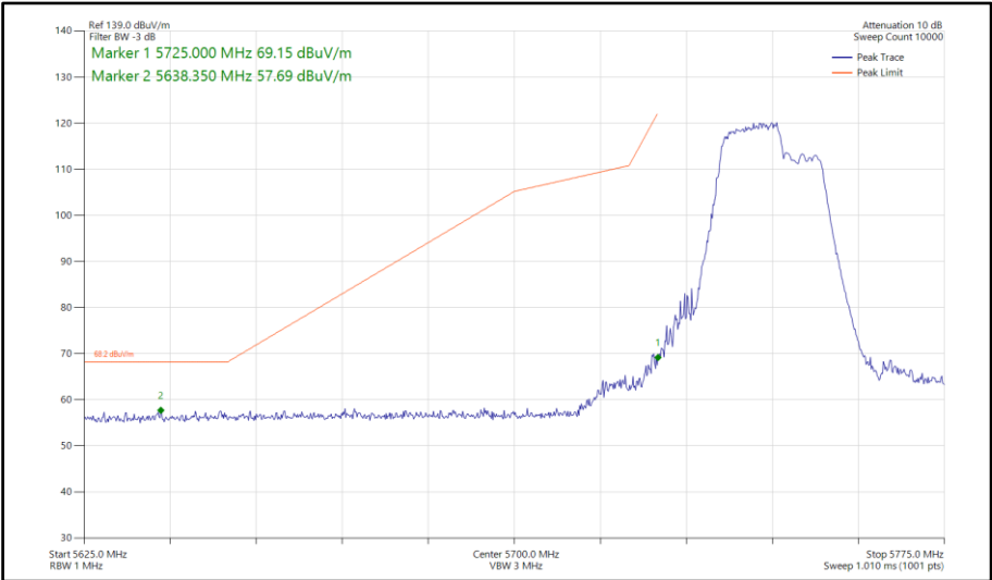
Figure 750 - 802.11be EHT40, RU106+26-82, SISO, Core 1 - 5755 MHz Band Edge Frequency 5725 MHz
