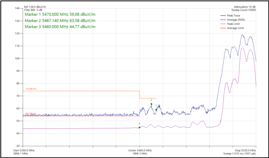
Figure 776 - 802.11ax HE40, RU106-56, CDD, Core 0-1 - 5510 MHz Band Edge Frequency 5470 MHz
