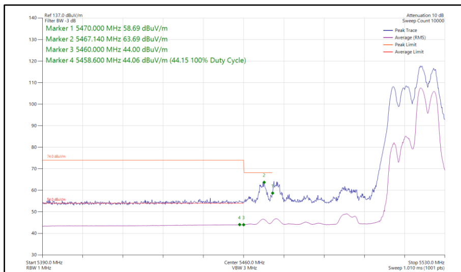
Figure 780 - 802.11be EHT40, RU52+26-75, CDD, Core 0-1 - 5510 MHz Band Edge Frequency 5470 MHz
