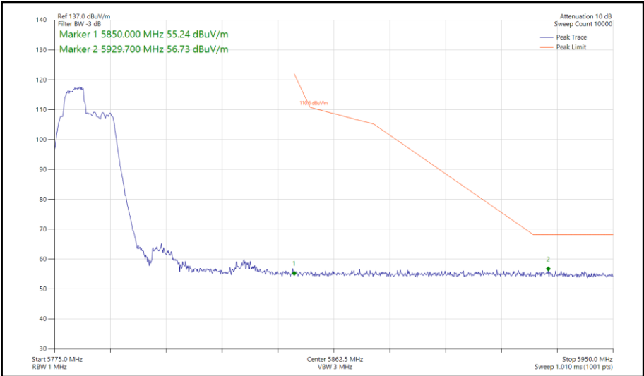
Figure 732 - 802.11be EHT40, RU52+26-70, SISO, Core 0 - 5795 MHz Band Edge Frequency 5850 MHz
