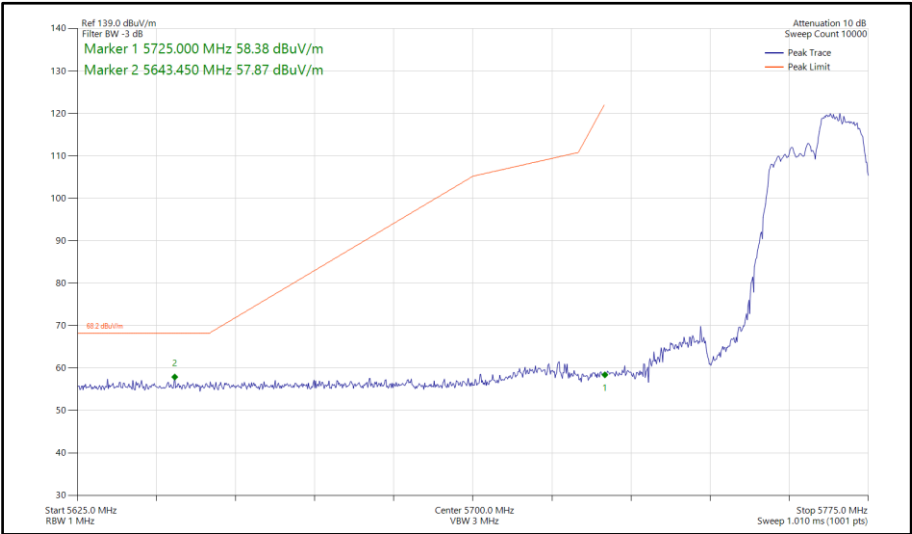
Figure 749 - 802.11ax HE40, RU106-56, SISO, Core 1 - 5755 MHz Band Edge Frequency 5725 MHz
