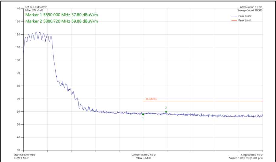
Figure 797 - 802.11n HT40, CDD, Core 0-1 - 5710 MHz Band Edge Frequency 5850 MHz
