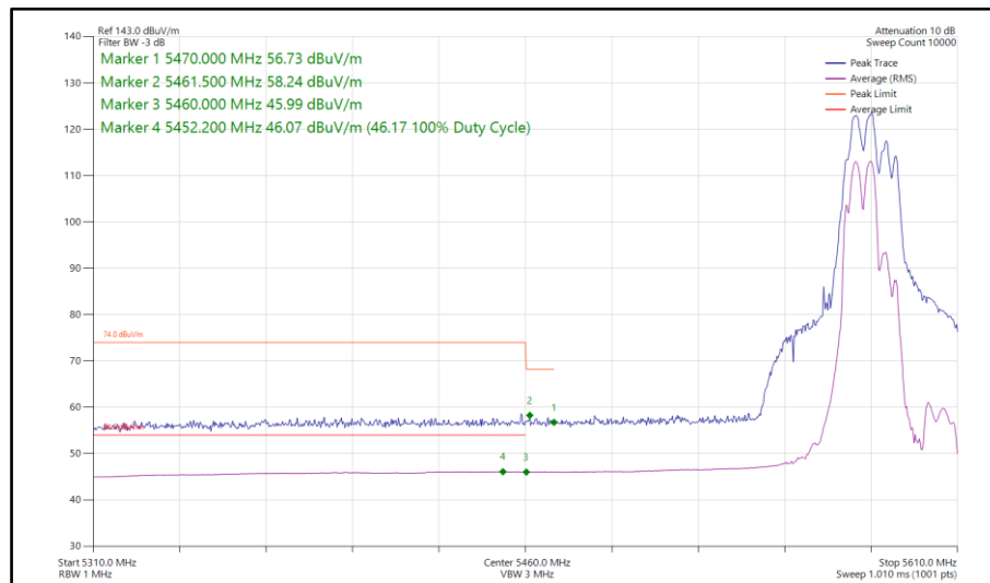
Figure 781 - 802.11be EHT40, RU106+26-82, CDD, Core 0-1 - 5590 MHz Band Edge Frequency 5470 MHz
