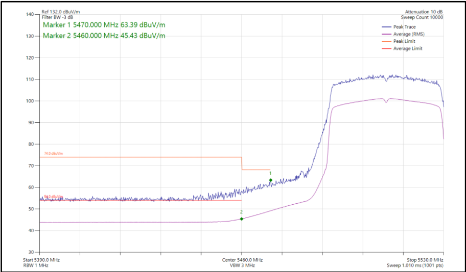
Figure 739 - 802.11ax HE40, SU, SISO, Core 1 - 5510 MHz Band Edge Frequency 5470 MHz
