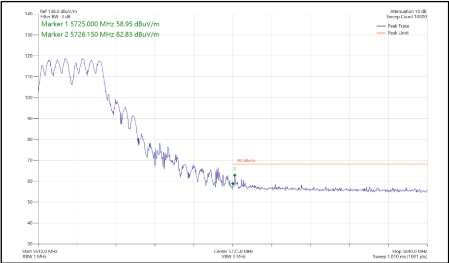
Figure 787 - 802.11a a40, CDD, Core 0-1 - 5630 MHz Band Edge Frequency 5725 MHz
