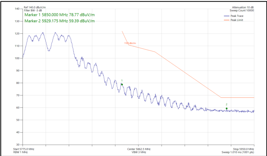
Figure 796 - 802.11a a40, CDD, Core 0-1 - 5795 MHz Band Edge Frequency 5850 MHz
