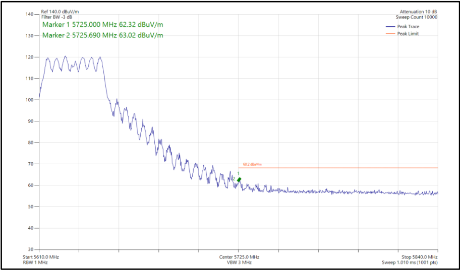
Figure 789 - 802.11n HT40, CDD, Core 0-1 - 5630 MHz Band Edge Frequency 5725 MHz
