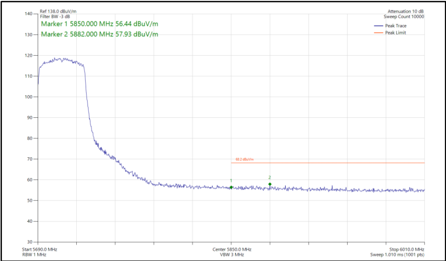
Figure 727 - 802.11ax HE40, SU, SISO, Core 0 - 5710 MHz Band Edge Frequency 5850 MHz
