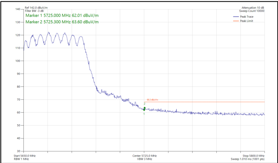
Figure 792 - 802.11ax HE40, SU, CDD, Core 0-1 - 5670 MHz Band Edge Frequency 5725 MHz
