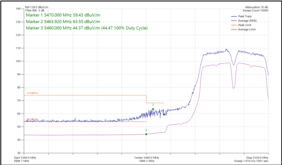
Figure 733 - 802.11a a40, SISO, Core 1 - 5510 MHz Band Edge Frequency 5470 MHz
