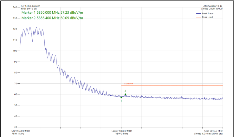
Figure 795 - 802.11a a40, CDD, Core 0-1 - 5710 MHz Band Edge Frequency 5850 MHz
