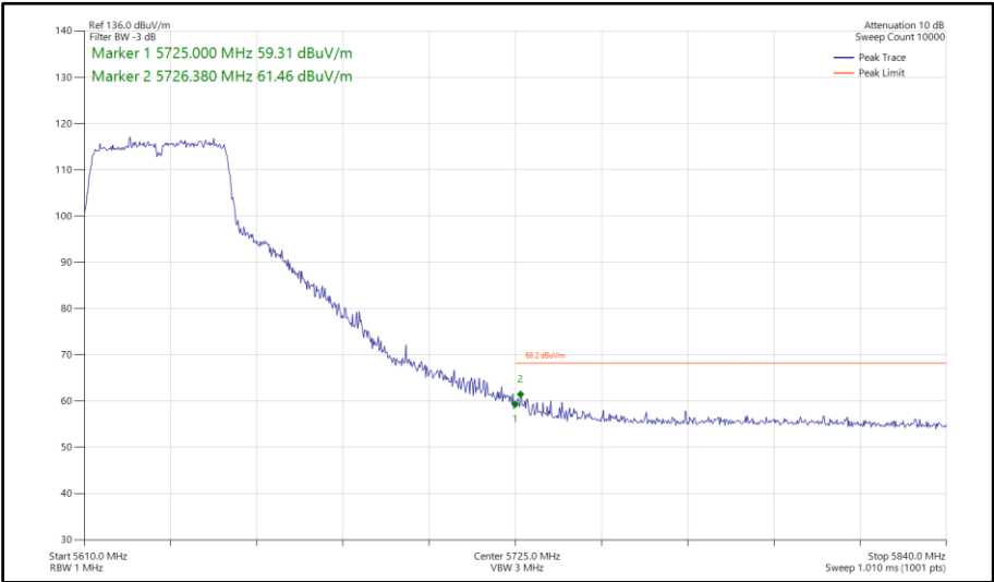
Figure 753 - 802.11n HT40, SISO, Core 1 - 5630 MHz Band Edge Frequency 5725 MHz
