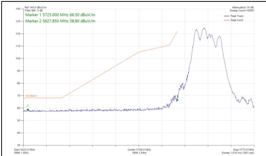
Figure 786 - 802.11be EHT40, RU106+26-82, CDD, Core 0-1 - 5755 MHz Band Edge Frequency 5725 MHz
