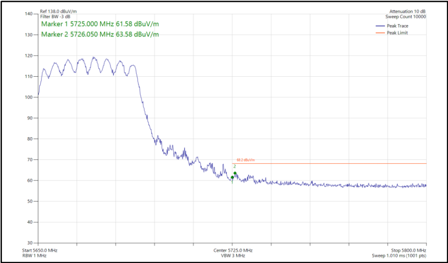
Figure 790 - 802.11n HT40, CDD, Core 0-1 - 5670 MHz Band Edge Frequency 5725 MHz
