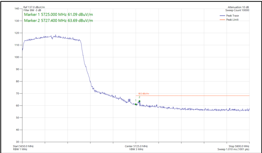
Figure 756 - 802.11ax HE40, SU, SISO, Core 1 - 5670 MHz Band Edge Frequency 5725 MHz
