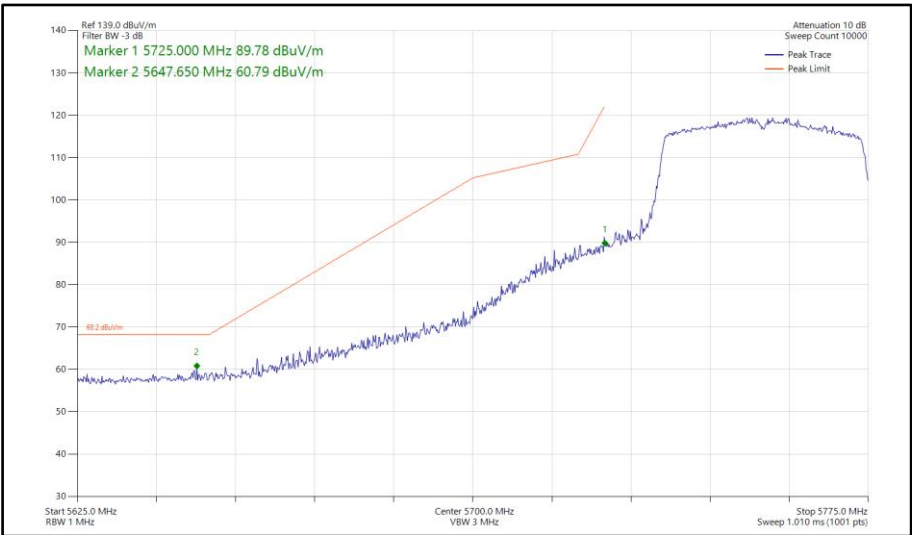
Figure 748 - 802.11ax HE40, SU, SISO, Core 1 - 5755 MHz Band Edge Frequency 5725 MHz
