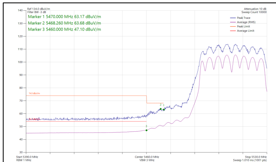
Figure 772 - 802.11n HT40, CDD, Core 0-1 - 5510 MHz Band Edge Frequency 5470 MHz
