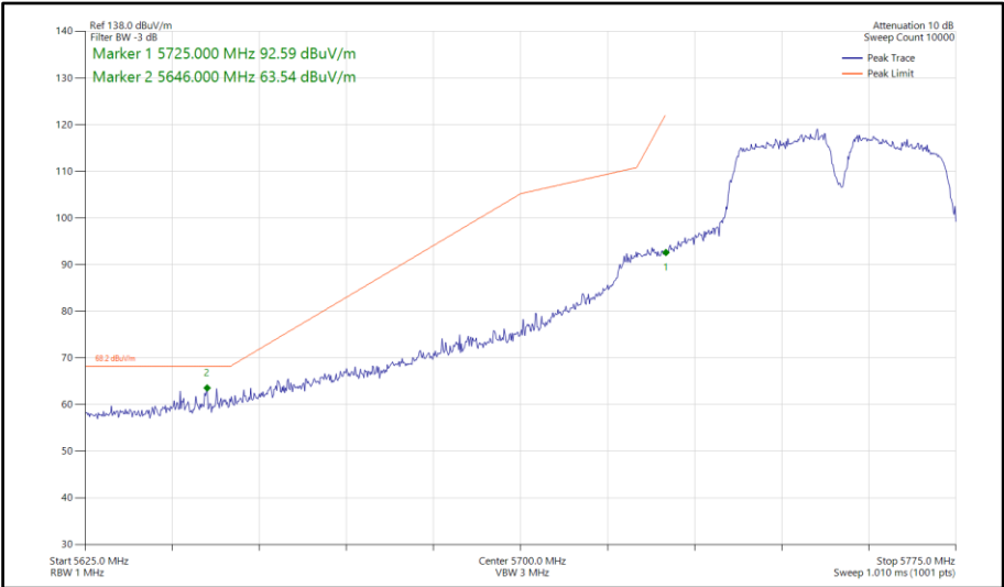
Figure 746 - 802.11a a40, SISO, Core 1 - 5755 MHz Band Edge Frequency 5725 MHz
