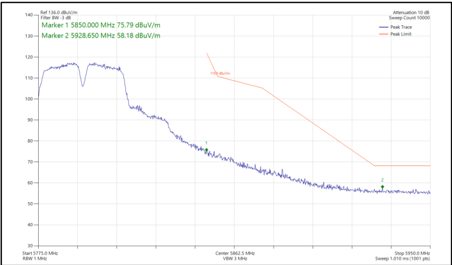
Figure 760 - 802.11a a40, SISO, Core 1 - 5795 MHz Band Edge Frequency 5850 MHz
