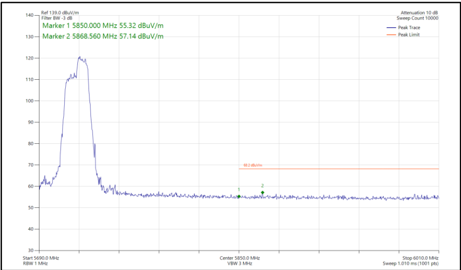
Figure 728 - 802.11ax HE40, RU106-56, SISO, Core 0 - 5710 MHz Band Edge Frequency 5850 MHz
