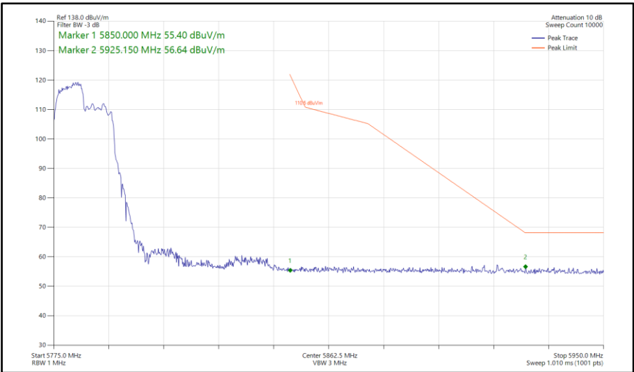
Figure 730 - 802.11ax HE40, RU106-53, SISO, Core 0 - 5795 MHz Band Edge Frequency 5850 MHz
