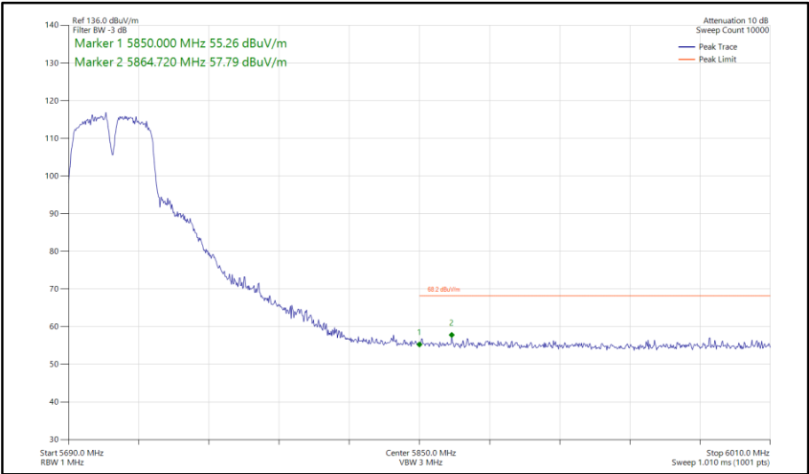
Figure 723 - 802.11a a40, SISO, Core 0 - 5710 MHz Band Edge Frequency 5850 MHz
