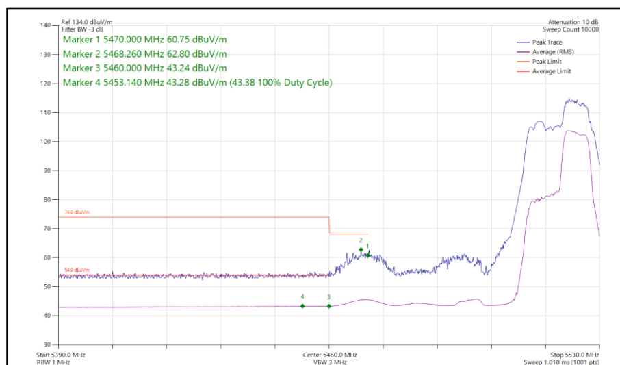
Figure 744 - 802.11be EHT40, RU52+26-75, SISO, Core 1 - 5510 MHz Band Edge Frequency 5470 MHz
