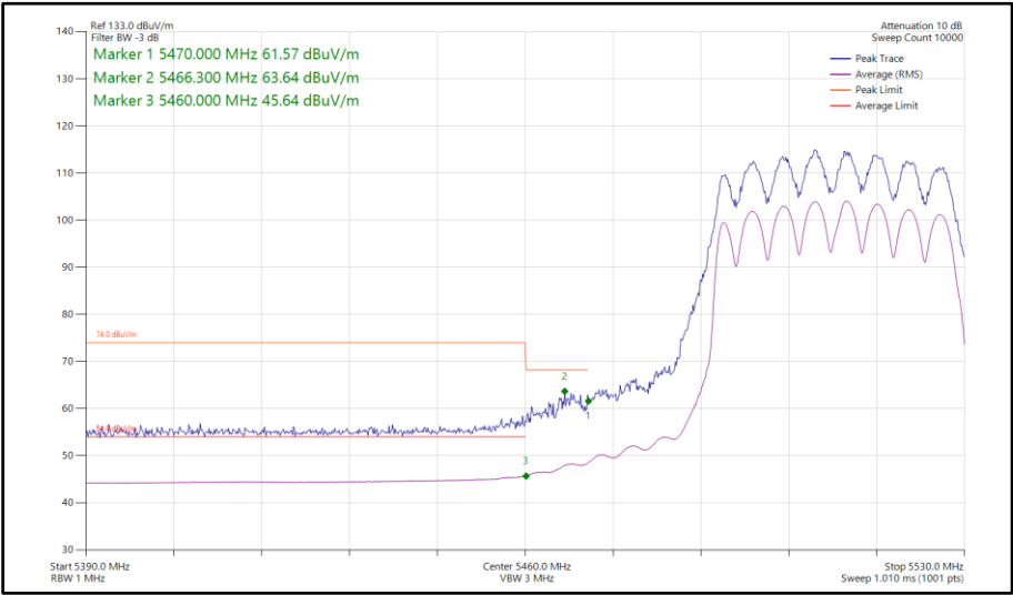
Figure 775 - 802.11ax HE40, SU, CDD, Core 0-1 - 5510 MHz Band Edge Frequency 5470 MHz
