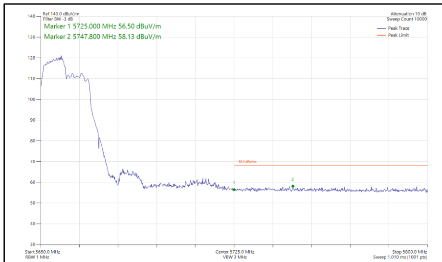
Figure 721 - 802.11ax HE40, RU106-53, SISO, Core 0 - 5670 MHz Band Edge Frequency 5725 MHz
