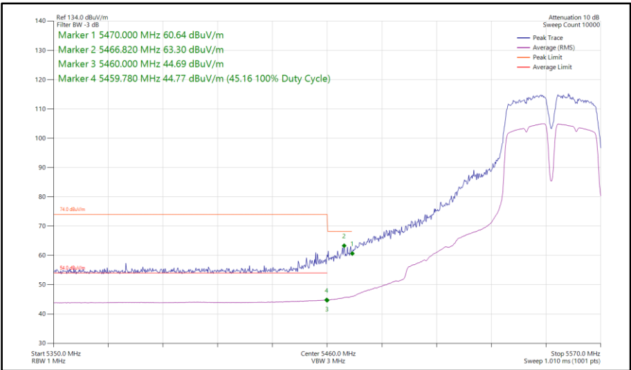
Figure 734 - 802.11a a40, SISO, Core 1 - 5550 MHz Band Edge Frequency 5470 MHz
