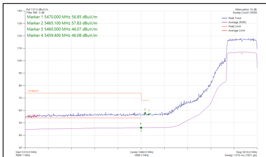
Figure 742 - 802.11ax HE40, SU, SISO, Core 1 - 5590 MHz Band Edge Frequency 5470 MHz
