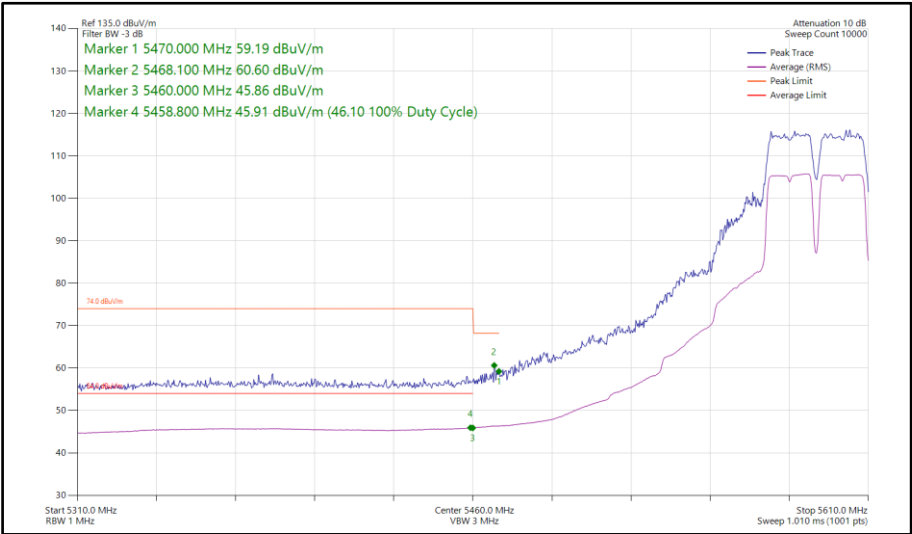
Figure 735 - 802.11a a40, SISO, Core 1 - 5590 MHz Band Edge Frequency 5470 MHz
