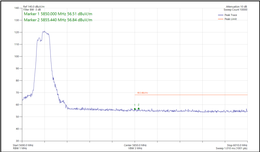
Figure 767 - 802.11be EHT40, RU106+26-85, SISO, Core 1 - 5710 MHz Band Edge Frequency 5850 MHz
