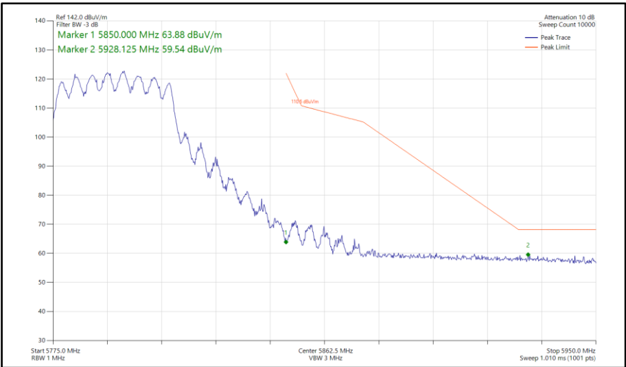
Figure 798 - 802.11n HT40, CDD, Core 0-1 - 5795 MHz Band Edge Frequency 5850 MHz
