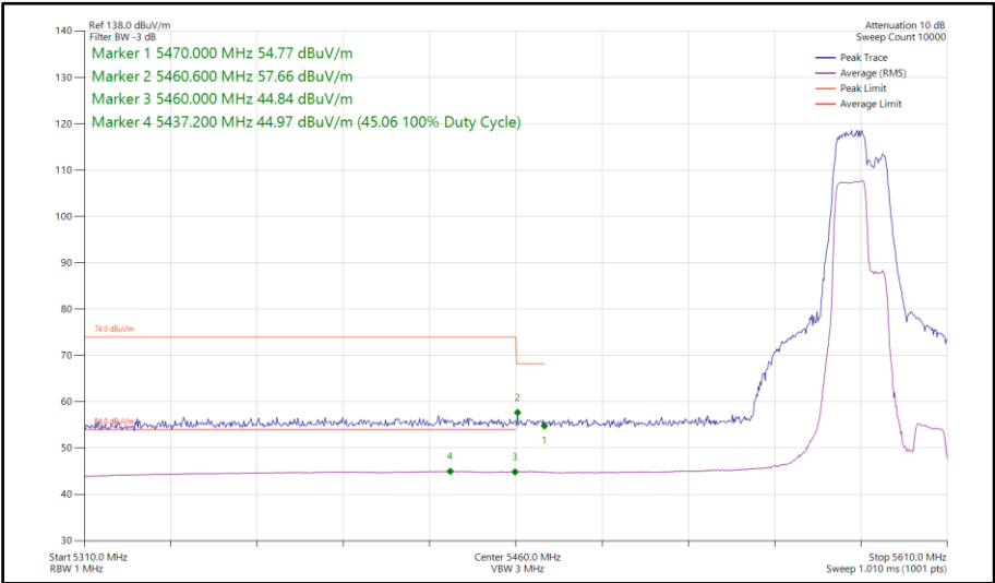
Figure 745 - 802.11be EHT40, RU106+26-82, SISO, Core 1 - 5590 MHz Band Edge Frequency 5470 MHz
