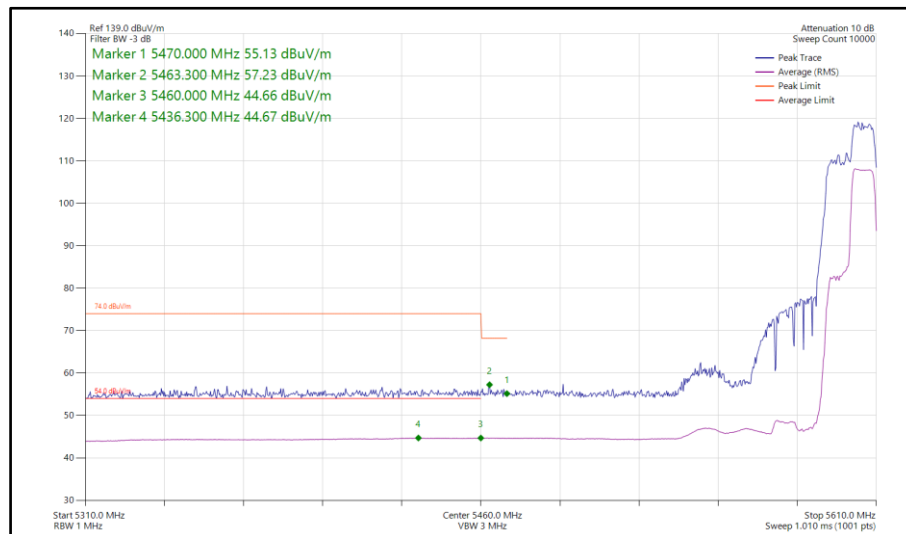
Figure 743 - 802.11ax HE40, RU106-56, SISO, Core 1 - 5590 MHz Band Edge Frequency 5470 MHz
