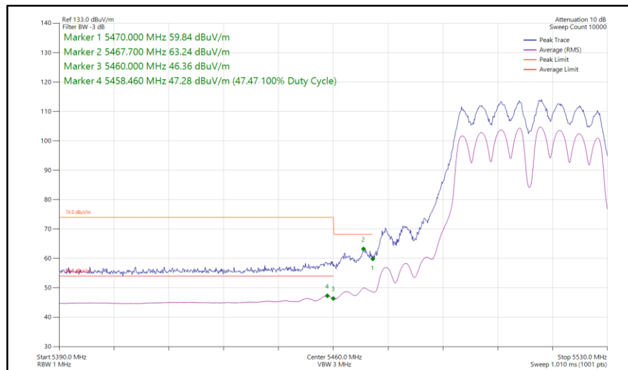
Figure 769 - 802.11a a40, CDD, Core 0-1 - 5510 MHz Band Edge Frequency 5470 MHz
