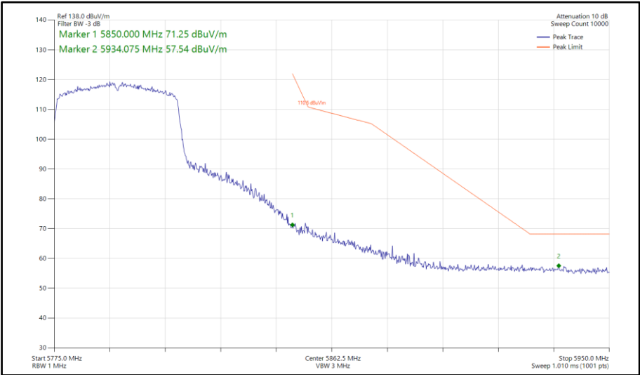
Figure 765 - 802.11ax HE40, SU, SISO, Core 1 - 5795 MHz Band Edge Frequency 5850 MHz
