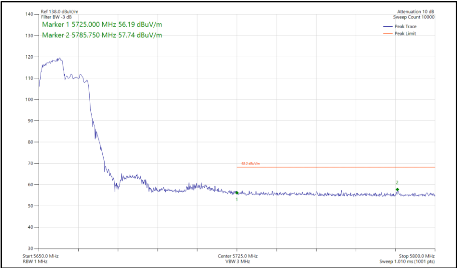
Figure 757 - 802.11ax HE40, RU106-53, SISO, Core 1 - 5670 MHz Band Edge Frequency 5725 MHz
