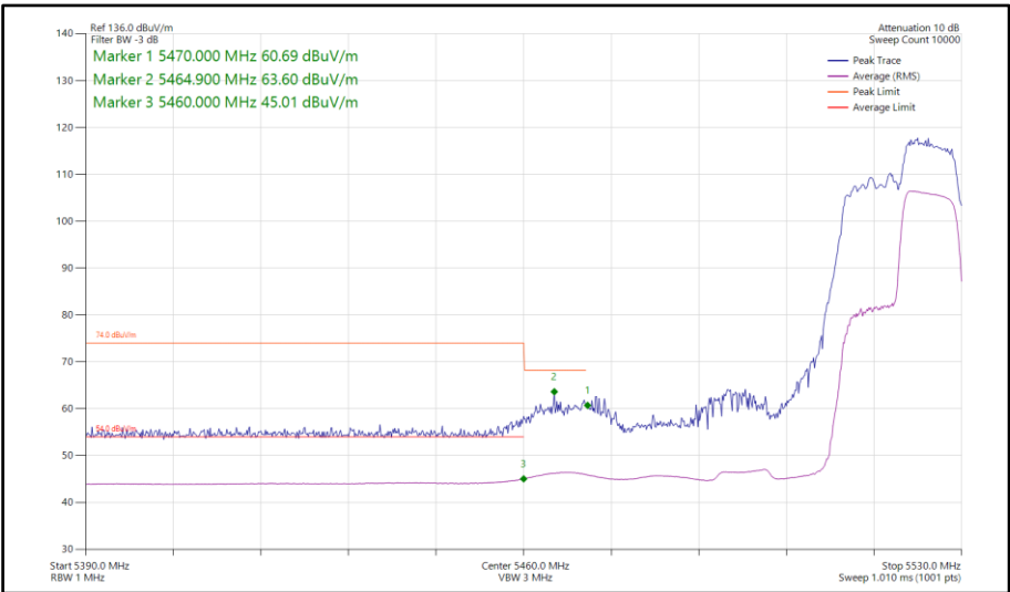
Figure 740 - 802.11ax HE40, RU106-56, SISO, Core 1 - 5510 MHz Band Edge Frequency 5470 MHz
