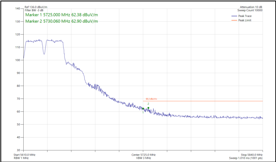
Figure 751 - 802.11a a40, SISO, Core 1 - 5630 MHz Band Edge Frequency 5725 MHz
