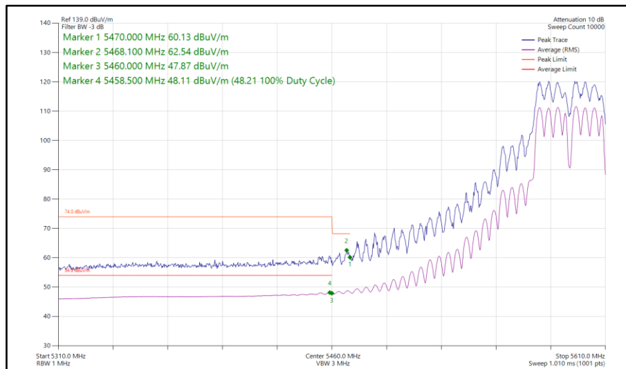
Figure 771 - 802.11a a40, CDD, Core 0-1 - 5590 MHz Band Edge Frequency 5470 MHz
