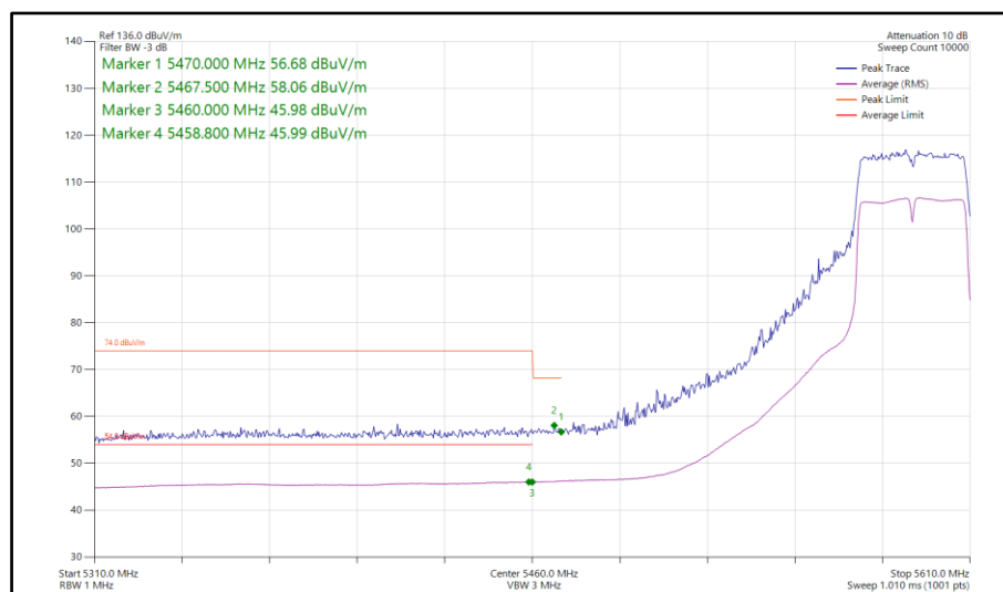
Figure 738 - 802.11n HT40, SISO, Core 1 - 5590 MHz Band Edge Frequency 5470 MHz
