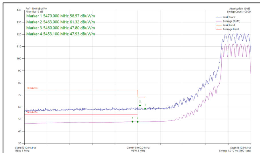
Figure 774 - 802.11n HT40, CDD, Core 0-1 - 5590 MHz Band Edge Frequency 5470 MHz
