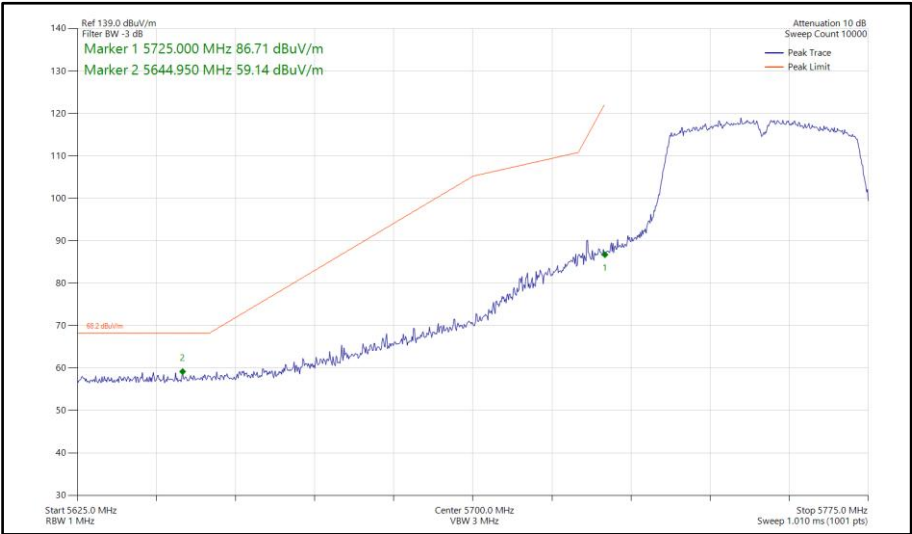
Figure 747 - 802.11n HT40, SISO, Core 1 - 5755 MHz Band Edge Frequency 5725 MHz
