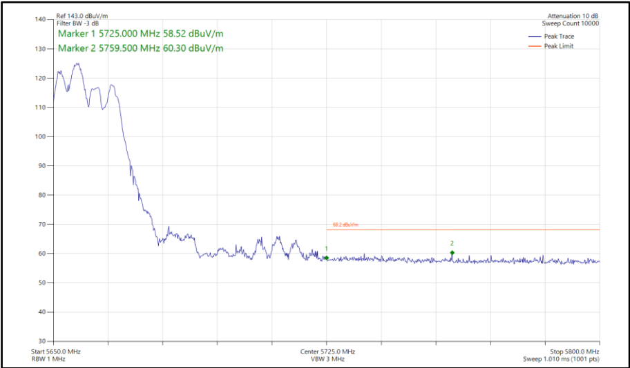
Figure 793 - 802.11ax HE40, RU106-53, CDD, Core 0-1 - 5670 MHz Band Edge Frequency 5725 MHz
