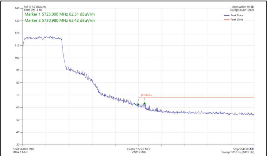
Figure 755 - 802.11ax HE40, SU, SISO, Core 1 - 5630 MHz Band Edge Frequency 5725 MHz
