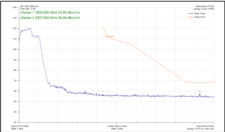
Figure 768 - 802.11be EHT40, RU106+26-82, SISO, Core 1 - 5795 MHz Band Edge Frequency 5850 MHz
