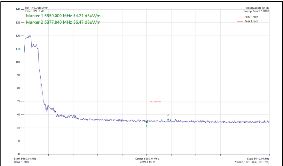
Figure 764 - 802.11ax HE40, RU106-53, SISO, Core 1 - 5710 MHz Band Edge Frequency 5850 MHz
