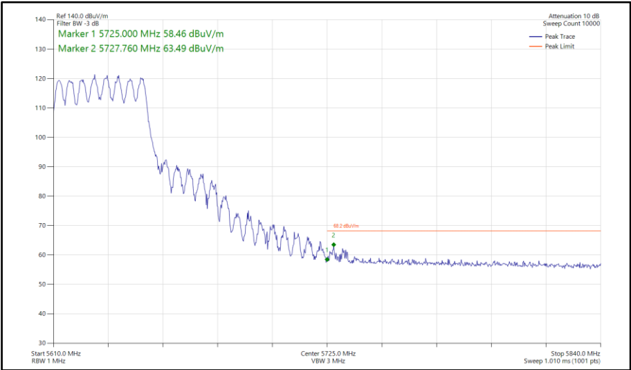
Figure 791 - 802.11ax HE40, SU, CDD, Core 0-1 - 5630 MHz Band Edge Frequency 5725 MHz
