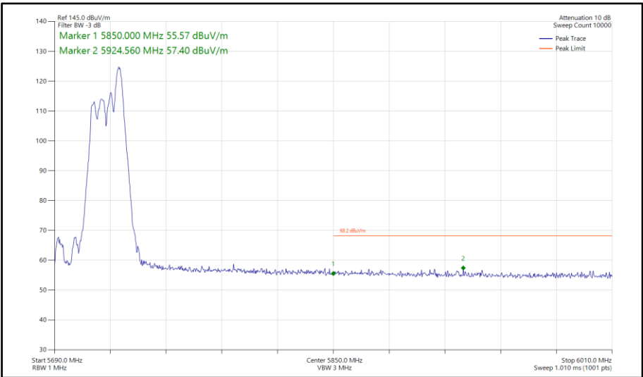
Figure 800 - 802.11ax HE40, RU52-44, CDD, Core 0-1 - 5710 MHz Band Edge Frequency 5850 MHz
