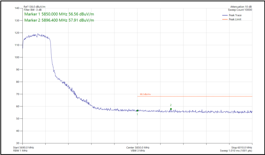
Figure 763 - 802.11ax HE40, SU, SISO, Core 1 - 5710 MHz Band Edge Frequency 5850 MHz
