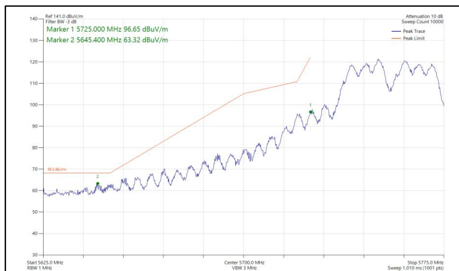
Figure 782 - 802.11a a40, CDD, Core 0-1 - 5755 MHz Band Edge Frequency 5725 MHz
