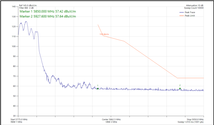
Figure 830 - 802.11ax HE40, RU106-53, SDM, Core 0-1 - 5795 MHz Band Edge Frequency 5850 MHz
