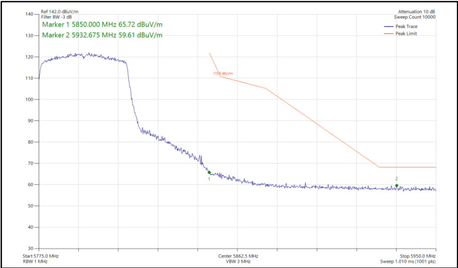
Figure 829 - 802.11ax HE40, SU, SDM, Core 0-1 - 5795 MHz Band Edge Frequency 5850 MHz
