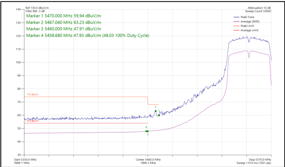
Figure 806 - 802.11n HT40, SDM, Core 0-1 - 5550 MHz Band Edge Frequency 5470 MHz
