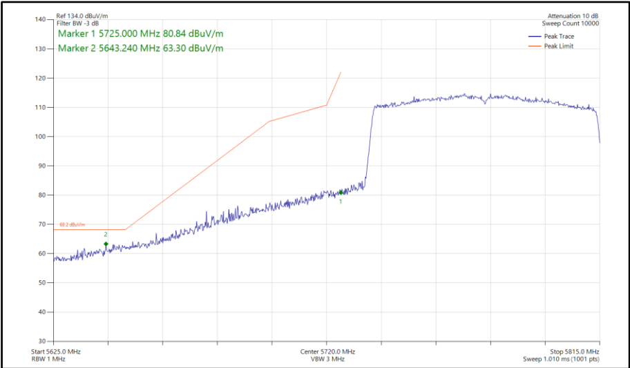
Figure 881 - 802.11ax HE80, SU, SISO, Core 1 - 5775 MHz Band Edge Frequency 5725 MHz
