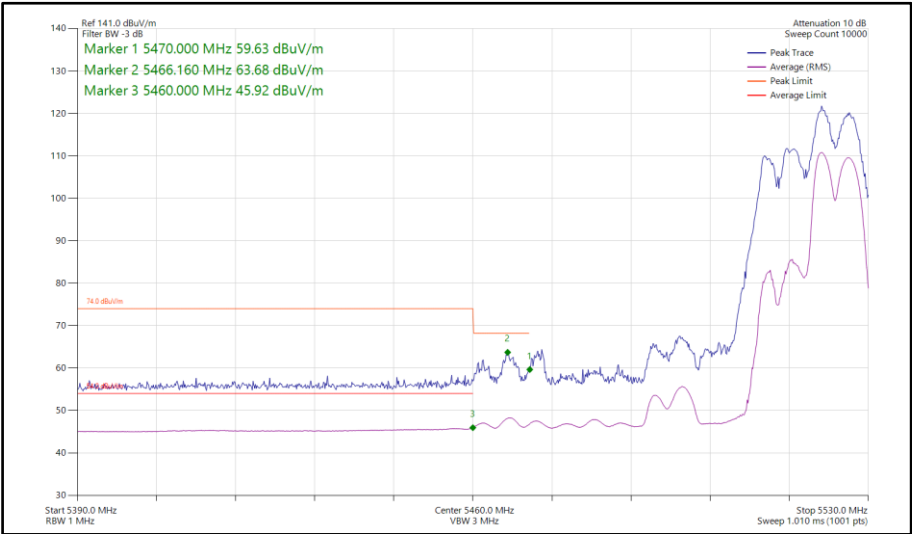
Figure 809 - 802.11ax HE40, RU106-56, SDM, Core 0-1 - 5510 MHz Band Edge Frequency 5470 MHz
