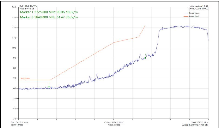
Figure 816 - 802.11ax HE40, SU, SDM, Core 0-1 - 5755 MHz Band Edge Frequency 5725 MHz
