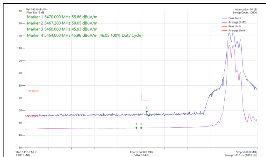
Figure 814 - 802.11be EHT40, RU106+26-82, SDM, Core 0-1 - 5590 MHz Band Edge Frequency 5470 MHz
