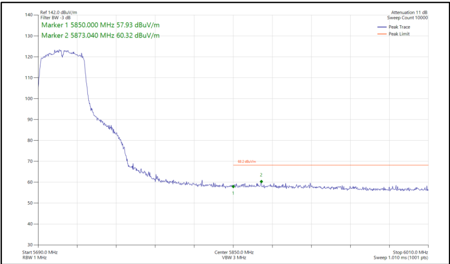
Figure 845 - 802.11ac VHT40, TxBF, Core 0-1 - 5710 MHz Band Edge Frequency 5850 MHz
