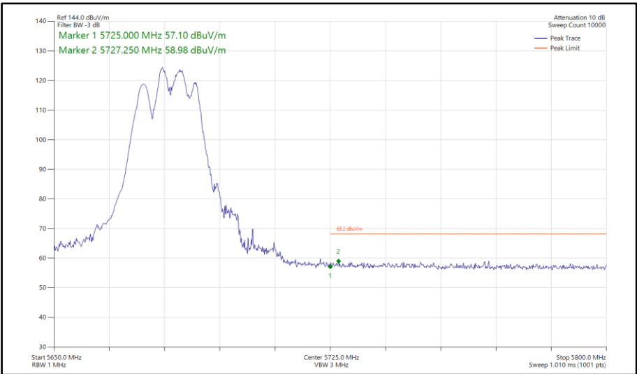
Figure 824 - 802.11be EHT40, RU106+26-85, SDM, Core 0-1 - 5670 MHz Band Edge Frequency 5725 MHz
