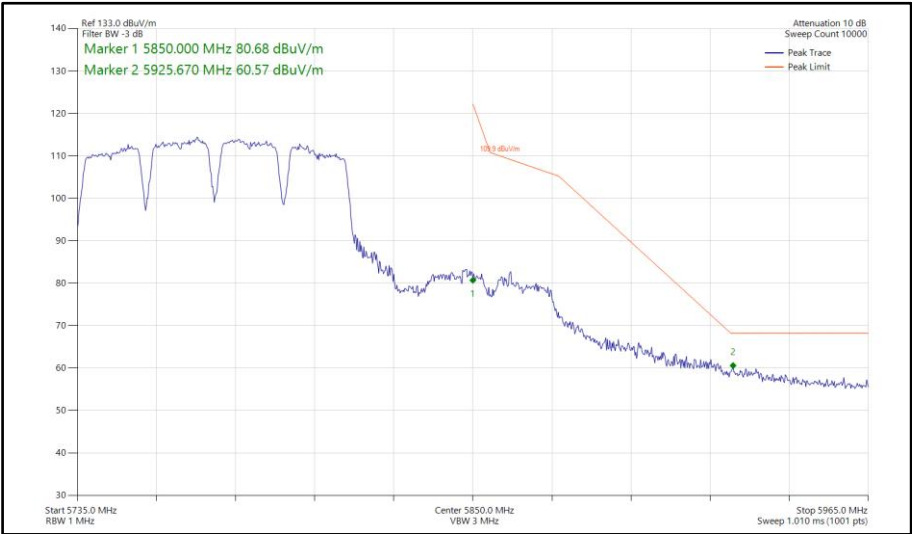
Figure 865 - 802.11a a80, SISO, Core 0 - 5775 MHz Band Edge Frequency 5850 MHz
