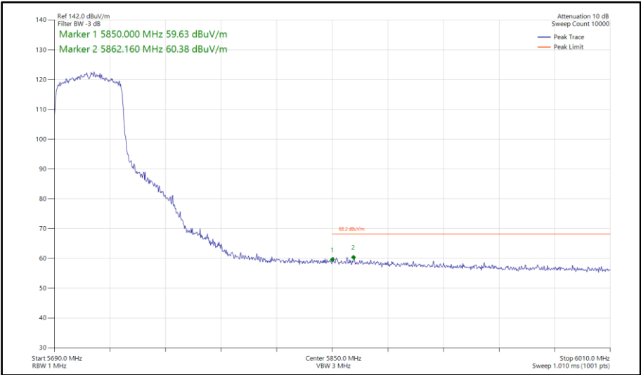
Figure 827 - 802.11ax HE40, SU, SDM, Core 0-1 - 5710 MHz Band Edge Frequency 5850 MHz
