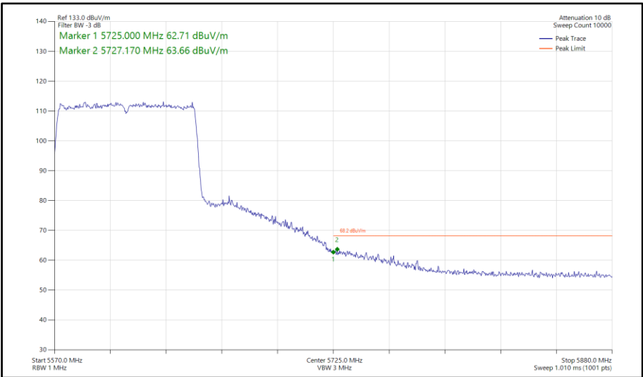
Figure 860 - 802.11ac VHT80, SISO, Core 0 - 5610 MHz Band Edge Frequency 5725 MHz
