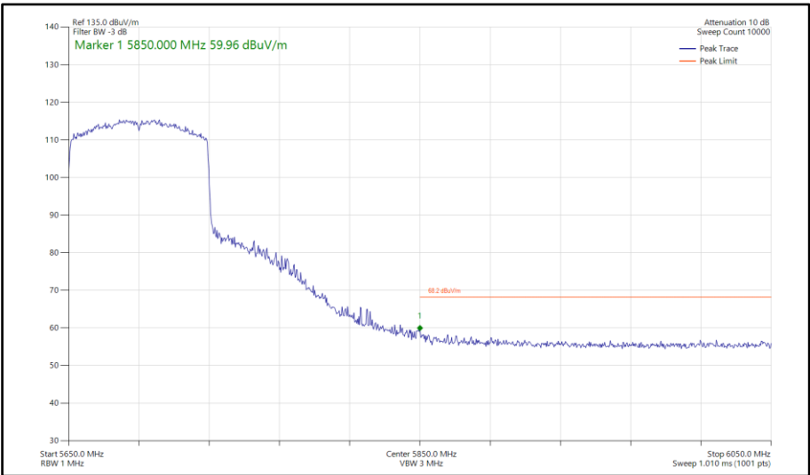
Figure 868 - 802.11ax HE80, SU, SISO, Core 0 - 5690 MHz Band Edge Frequency 5850 MHz
