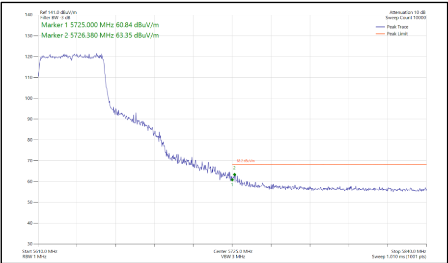
Figure 843 - 802.11ax HE40, SU, TxBF, Core 0-1 - 5630 MHz Band Edge Frequency 5725 MHz
