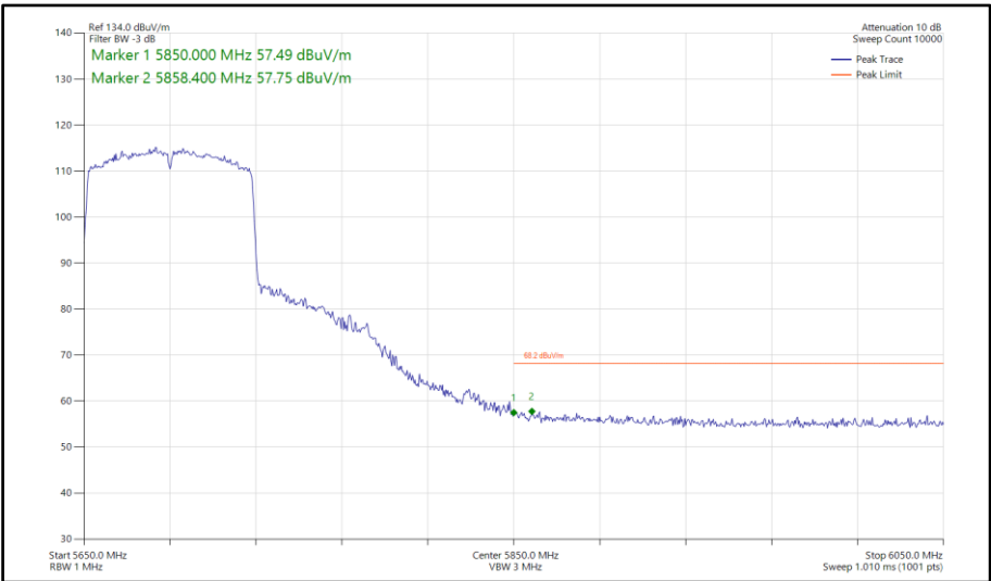
Figure 866 - 802.11ac VHT80, SISO, Core 0 - 5690 MHz Band Edge Frequency 5850 MHz
