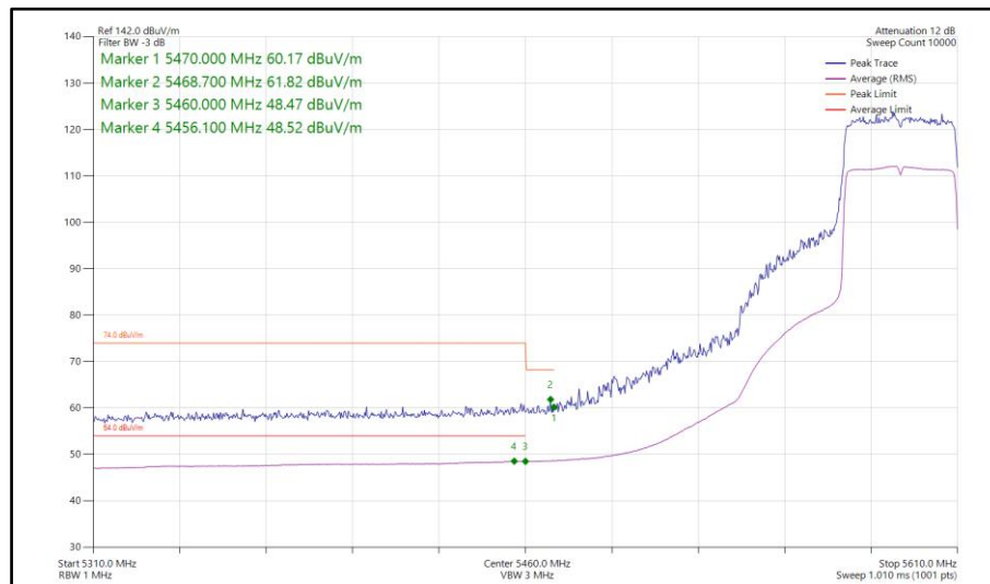
Figure 838 - 802.11ax HE40, SU, TxBF, Core 0-1 - 5590 MHz Band Edge Frequency 5470 MHz
