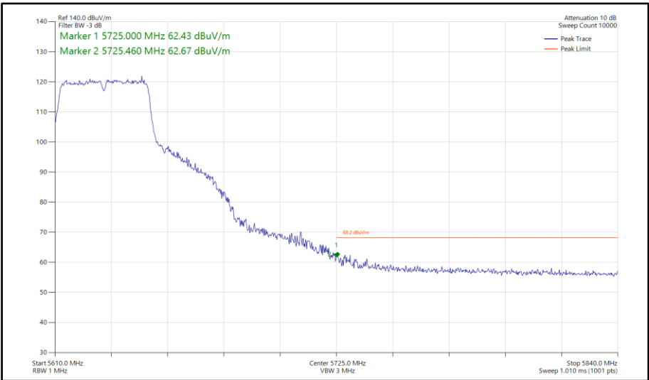
Figure 841 - 802.11ac VHT40, TxBF, Core 0-1 - 5630 MHz Band Edge Frequency 5725 MHz
