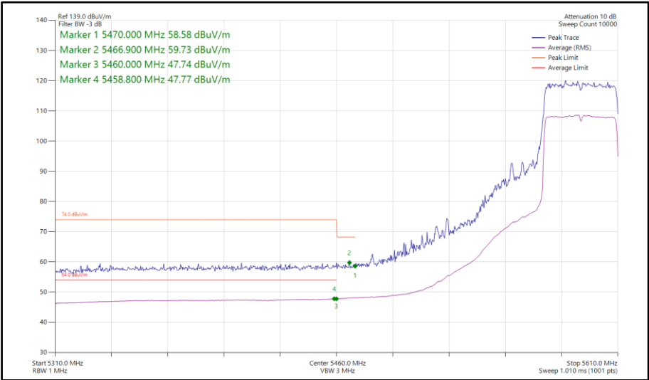
Figure 811 - 802.11ax HE40, SU, SDM, Core 0-1 - 5590 MHz Band Edge Frequency 5470 MHz
