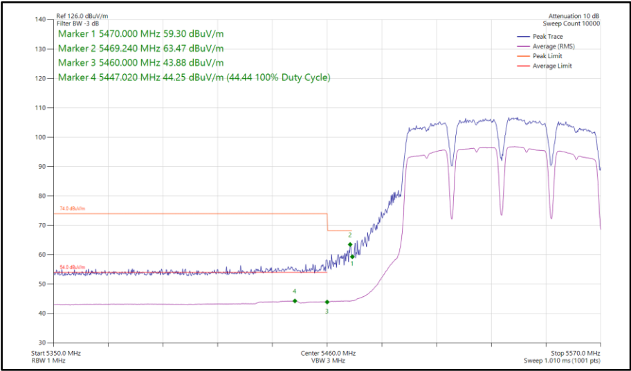
Figure 849 - 802.11a a80, SISO, Core 0 - 5530 MHz Band Edge Frequency 5470 MHz
