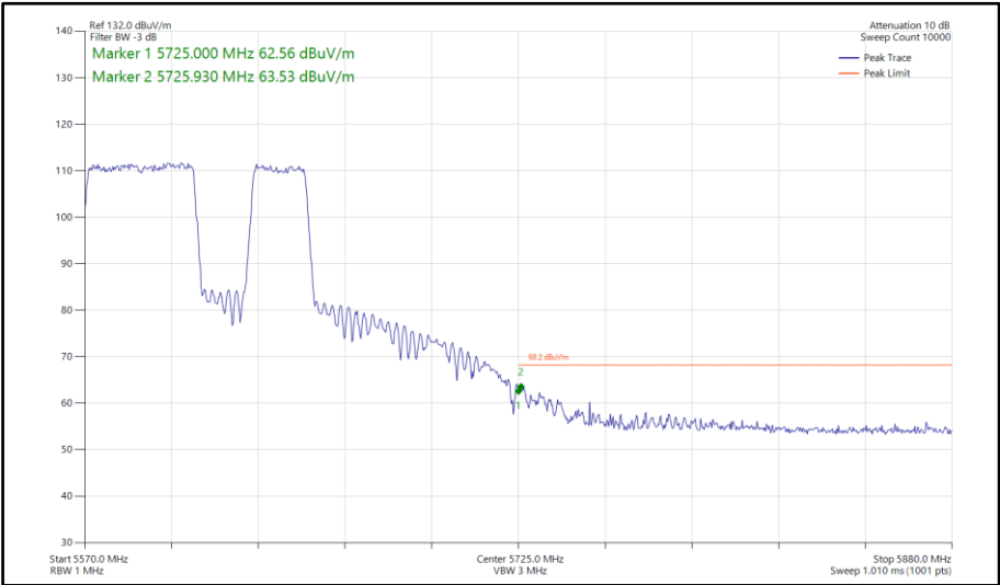
Figure 863 - 802.11be EHT80, RU484+242-92, SISO, Core 0 - 5610 MHz Band Edge Frequency 5725 MHz
