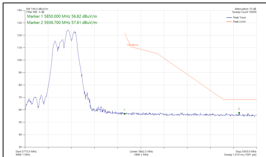
Figure 802 - 802.11ax HE40, RU106-56, CDD, Core 0-1 - 5795 MHz Band Edge Frequency 5850 MHz
