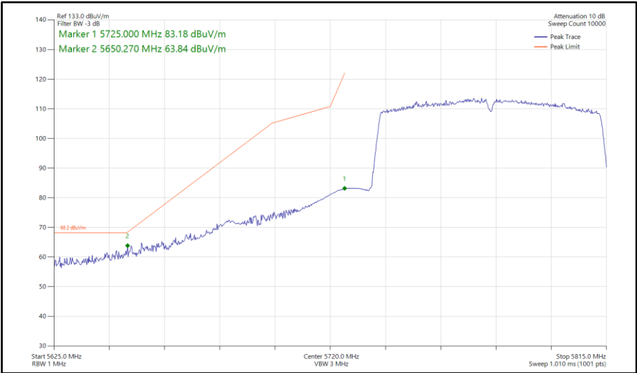
Figure 855 - 802.11ac VHT80, SISO, Core 0 - 5775 MHz Band Edge Frequency 5725 MHz
