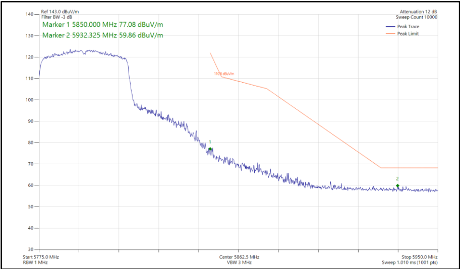
Figure 848 - 802.11ax HE40, SU, TxBF, Core 0-1 - 5795 MHz Band Edge Frequency 5850 MHz
