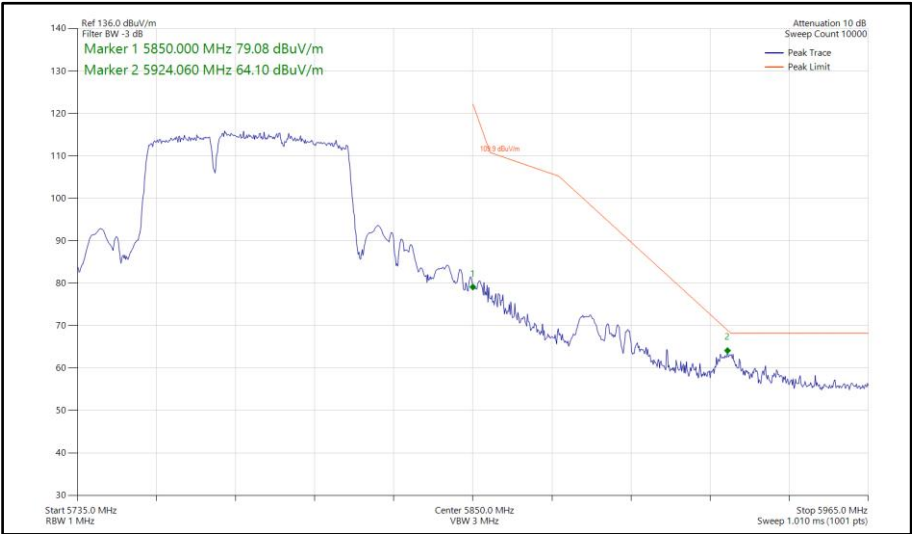
Figure 873 - 802.11be EHT80, RU484+242-90, SISO, Core 0 - 5775 MHz Band Edge Frequency 5850 MHz
