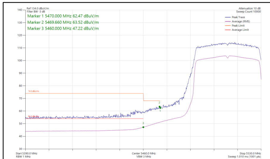
Figure 836 - 802.11ax HE40, SU, TxBF, Core 0-1 - 5510 MHz Band Edge Frequency 5470 MHz
