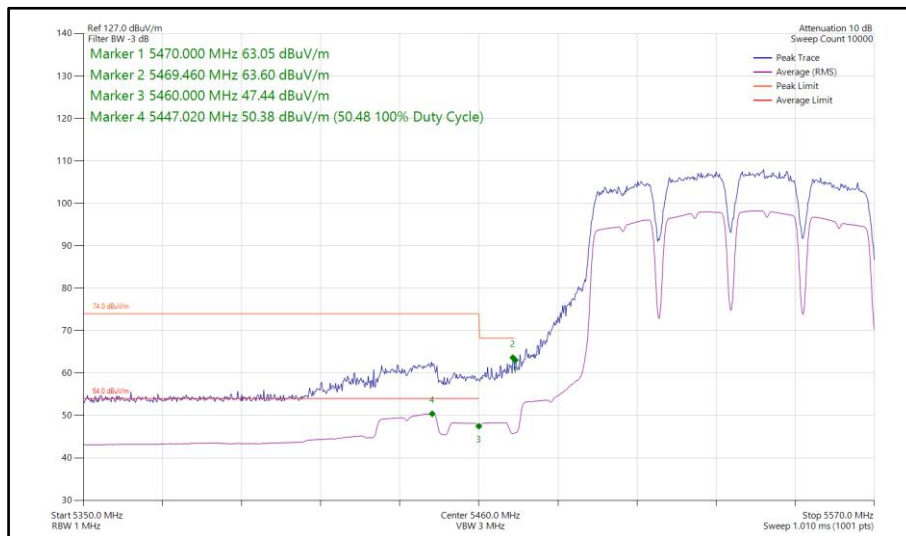
Figure 874 - 802.11a a80, SISO, Core 1 - 5530 MHz Band Edge Frequency 5470 MHz
