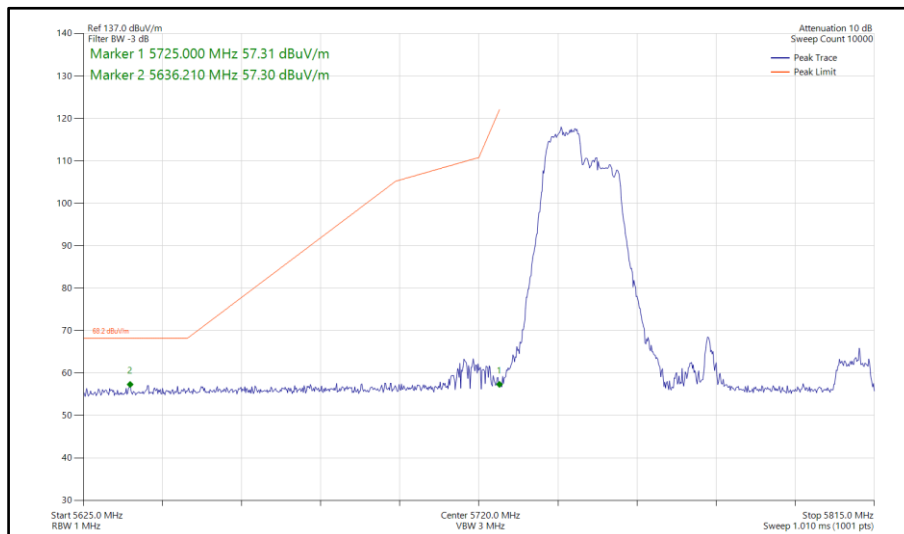
Figure 882 - 802.11ax HE80, RU106-53, SISO, Core 1 - 5775 MHz Band Edge Frequency 5725 MHz
