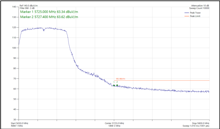
Figure 842 - 802.11ac VHT40, TxBF, Core 0-1 - 5670 MHz Band Edge Frequency 5725 MHz
