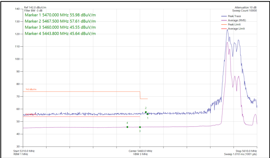
Figure 812 - 802.11ax HE40, RU52-37, SDM, Core 0-1 - 5590 MHz Band Edge Frequency 5470 MHz
