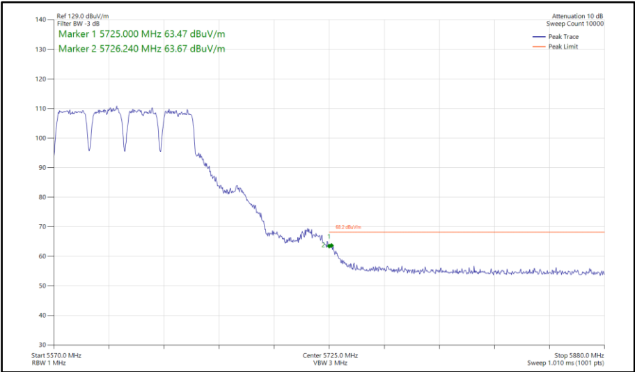
Figure 859 - 802.11a a80, SISO, Core 0 - 5610 MHz Band Edge Frequency 5725 MHz
