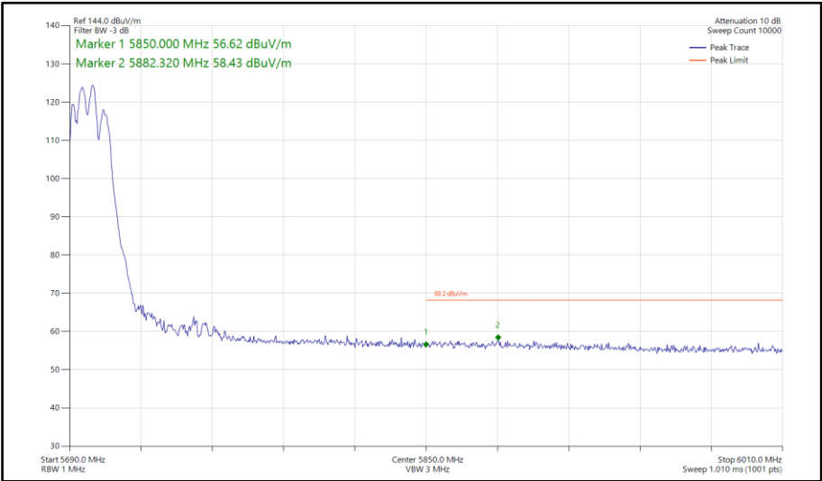
Figure 831 - 802.11be EHT40, RU106+26-82, SDM, Core 0-1 - 5710 MHz Band Edge Frequency 5850 MHz
