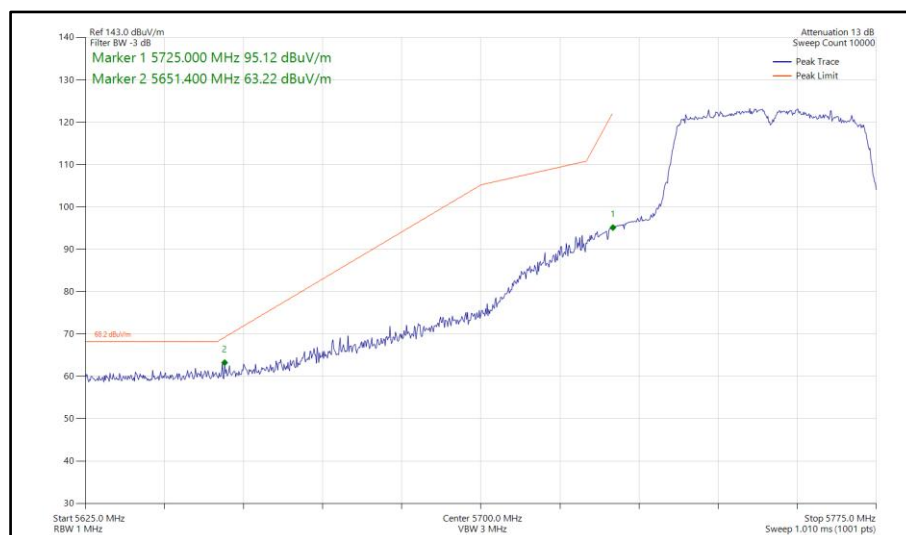
Figure 839 - 802.11ac VHT40, TxBF, Core 0-1 - 5755 MHz Band Edge Frequency 5725 MHz
