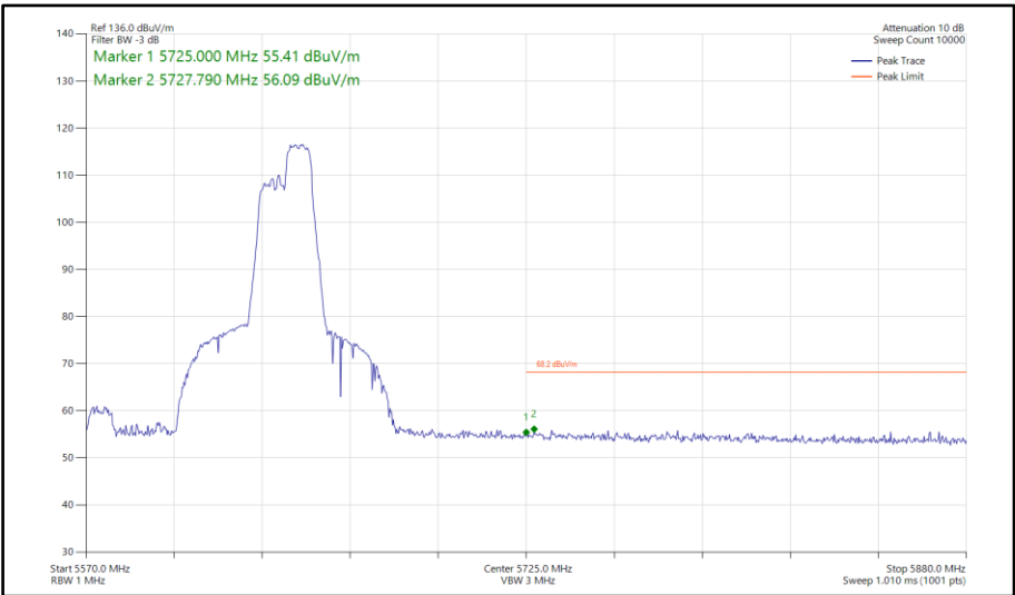
Figure 862 - 802.11ax HE80, RU106-60, SISO, Core 0 - 5610 MHz Band Edge Frequency 5725 MHz
