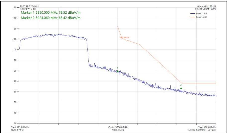
Figure 870 - 802.11ax HE80, SU, SISO, Core 0 - 5775 MHz Band Edge Frequency 5850 MHz
