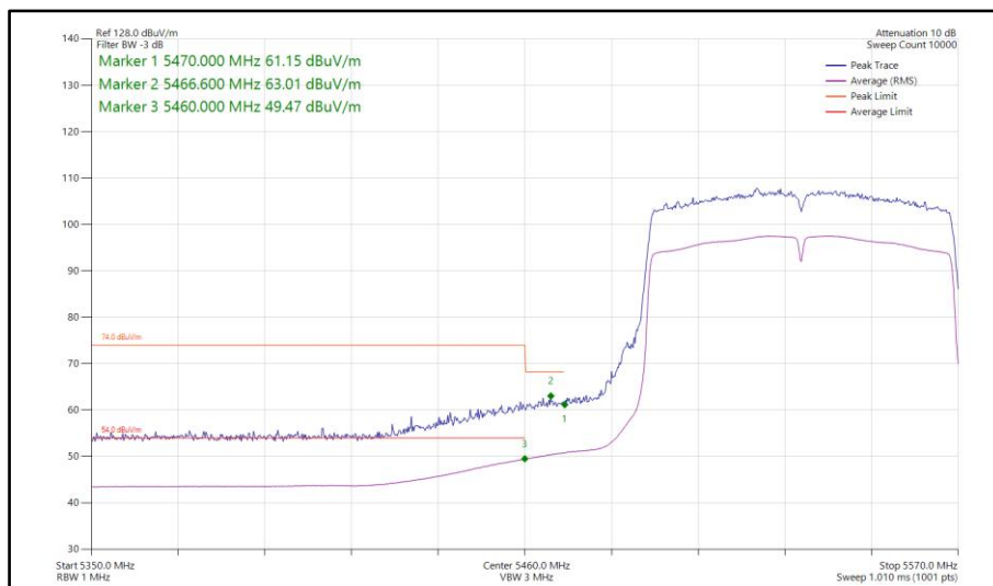
Figure 875 - 802.11ac VHT80, SISO, Core 1 - 5530 MHz Band Edge Frequency 5470 MHz
