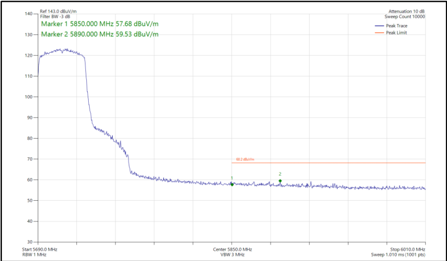
Figure 847 - 802.11ax HE40, SU, TxBF, Core 0-1 - 5710 MHz Band Edge Frequency 5850 MHz
