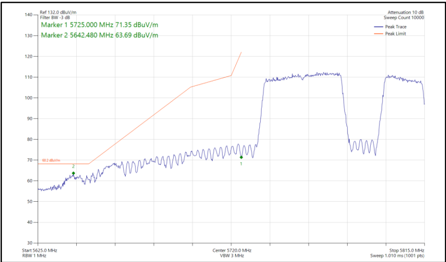
Figure 858 - 802.11be EHT80, RU484+242-92, SISO, Core 0 - 5775 MHz Band Edge Frequency 5725 MHz
