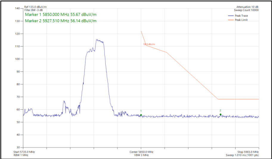
Figure 871 - 802.11ax HE80, RU106-60, SISO, Core 0 - 5775 MHz Band Edge Frequency 5850 MHz
