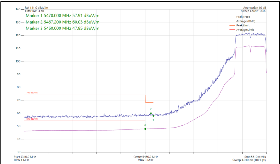
Figure 835 - 802.11ac VHT40, TxBF, Core 0-1 - 5590 MHz Band Edge Frequency 5470 MHz
