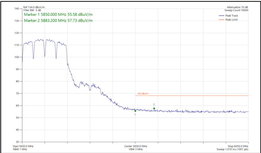
Figure 864 - 802.11a a80, SISO, Core 0 - 5690 MHz Band Edge Frequency 5850 MHz
