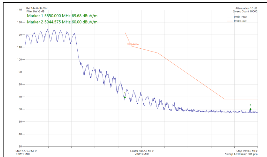
Figure 801 - 802.11ax HE40, SU, CDD, Core 0-1 - 5795 MHz Band Edge Frequency 5850 MHz
