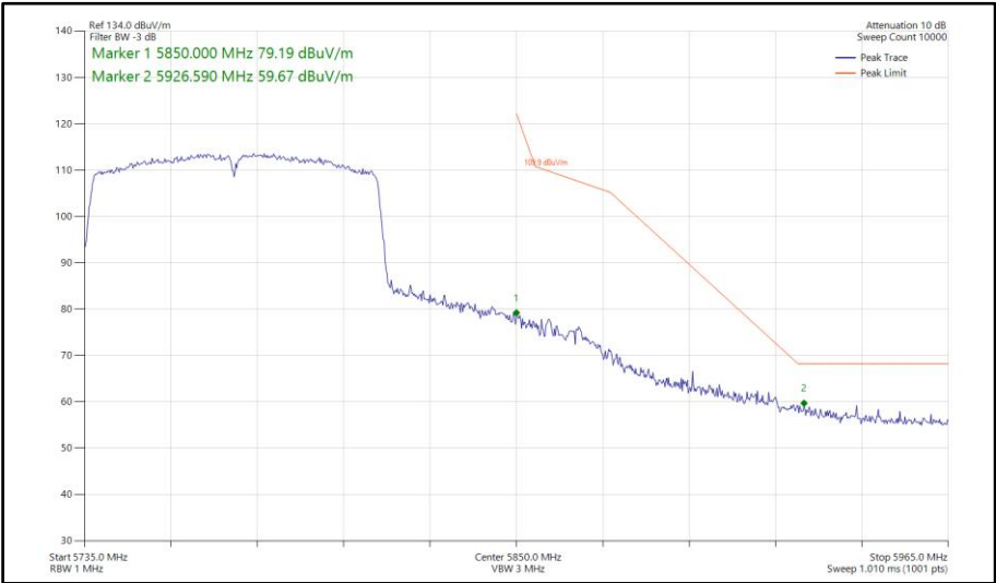
Figure 867 - 802.11ac VHT80, SISO, Core 0 - 5775 MHz Band Edge Frequency 5850 MHz
