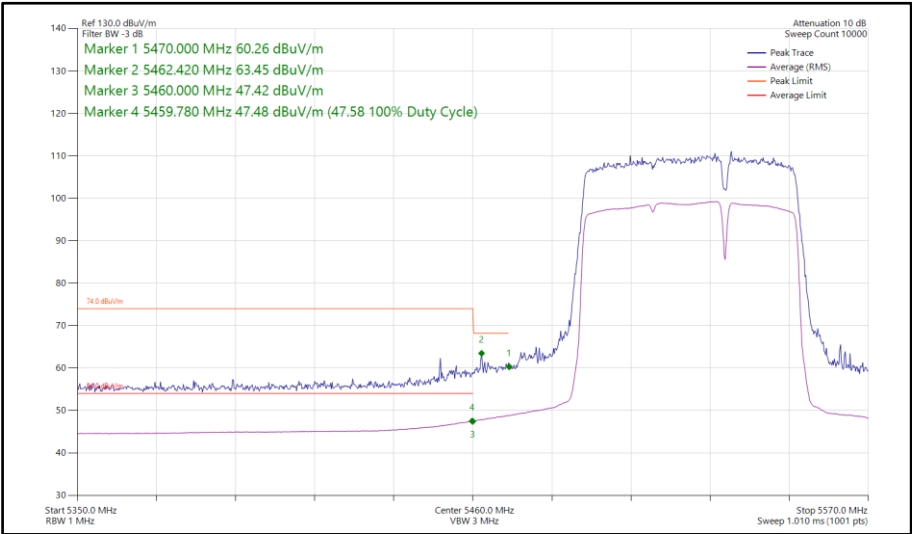
Figure 853 - 802.11be EHT80, RU484+242-93, SISO, Core 0 - 5530 MHz Band Edge Frequency 5470 MHz
