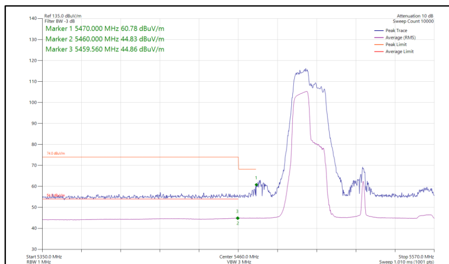
Figure 877 - 802.11ax HE80, RU106-53, SISO, Core 1 - 5530 MHz Band Edge Frequency 5470 MHz
