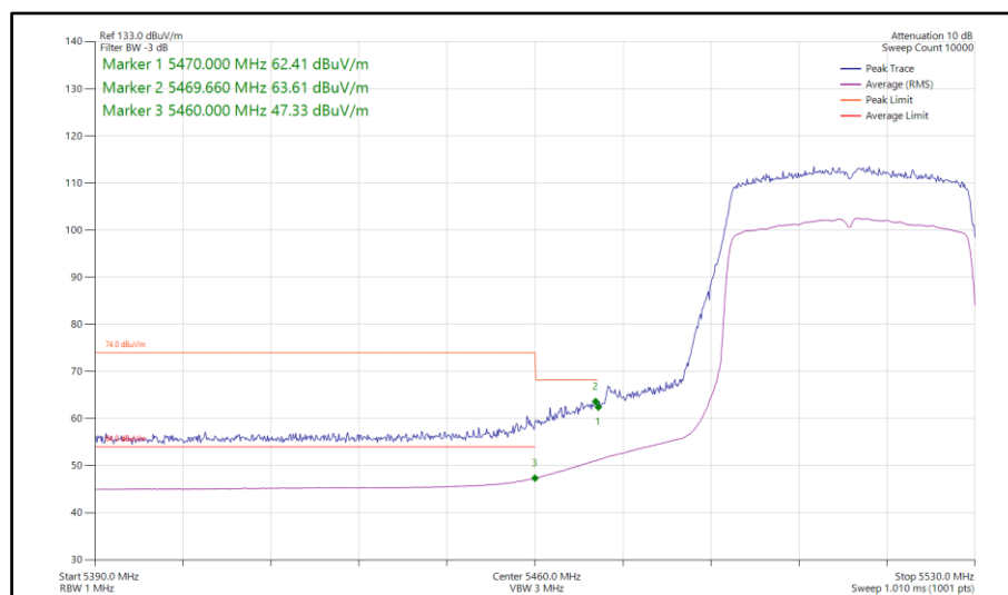
Figure 808 - 802.11ax HE40, SU, SDM, Core 0-1 - 5510 MHz Band Edge Frequency 5470 MHz
