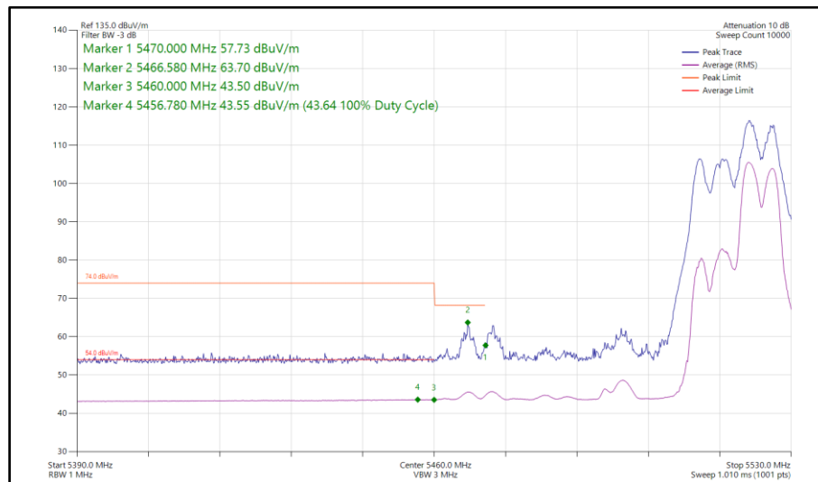
Figure 813 - 802.11be EHT40, RU52+26-75, SDM, Core 0-1 - 5510 MHz Band Edge Frequency 5470 MHz
