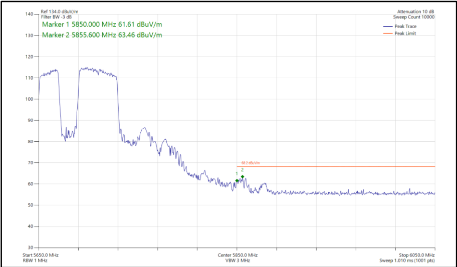
Figure 872 - 802.11be EHT80, RU484+242-91, SISO, Core 0 - 5690 MHz Band Edge Frequency 5850 MHz
