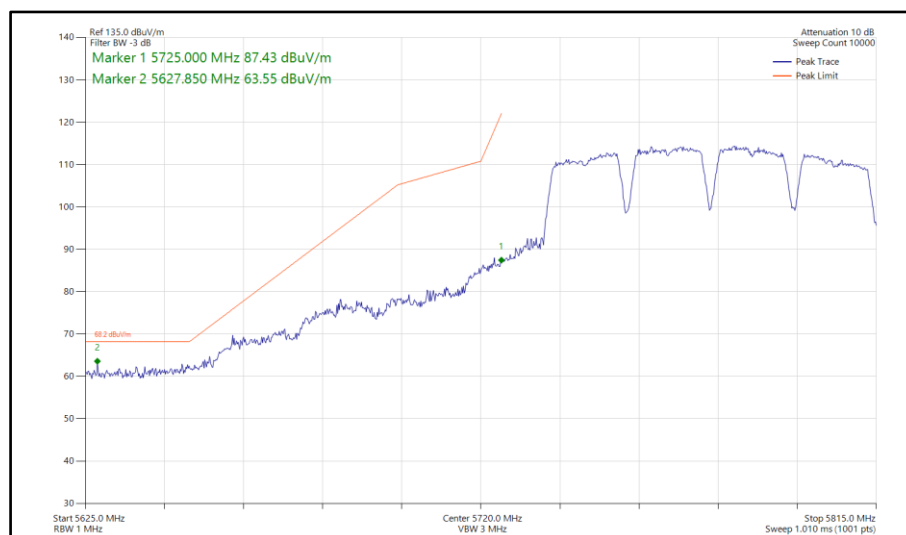
Figure 879 - 802.11a a80, SISO, Core 1 - 5775 MHz Band Edge Frequency 5725 MHz
