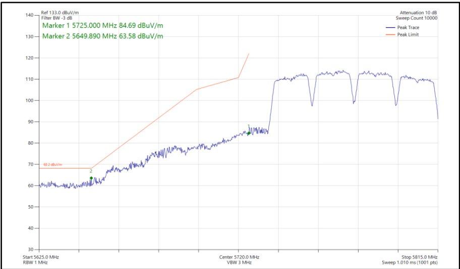
Figure 854 - 802.11a a80, SISO, Core 0 - 5775 MHz Band Edge Frequency 5725 MHz
