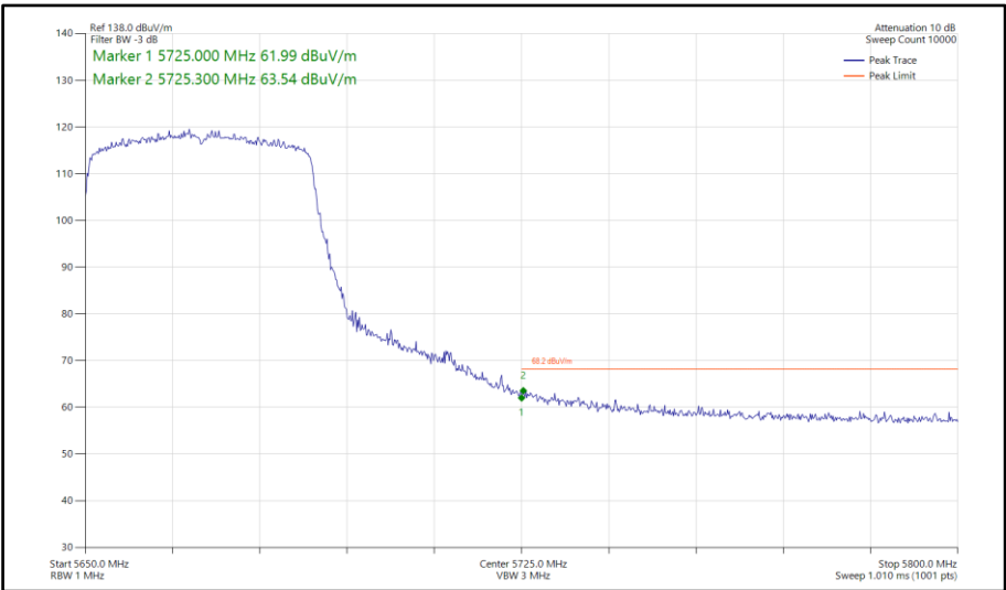
Figure 822 - 802.11ax HE40, SU, SDM, Core 0-1 - 5670 MHz Band Edge Frequency 5725 MHz
