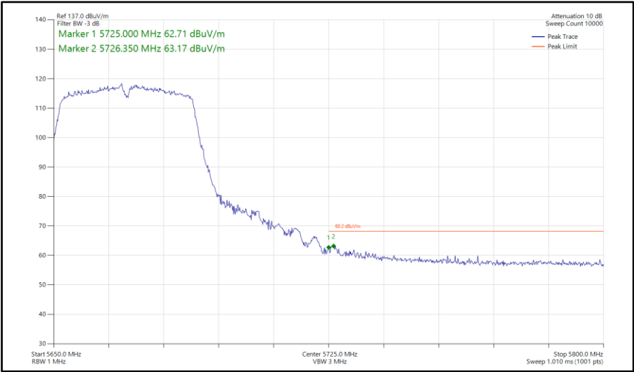
Figure 820 - 802.11n HT40, SDM, Core 0-1 - 5670 MHz Band Edge Frequency 5725 MHz
