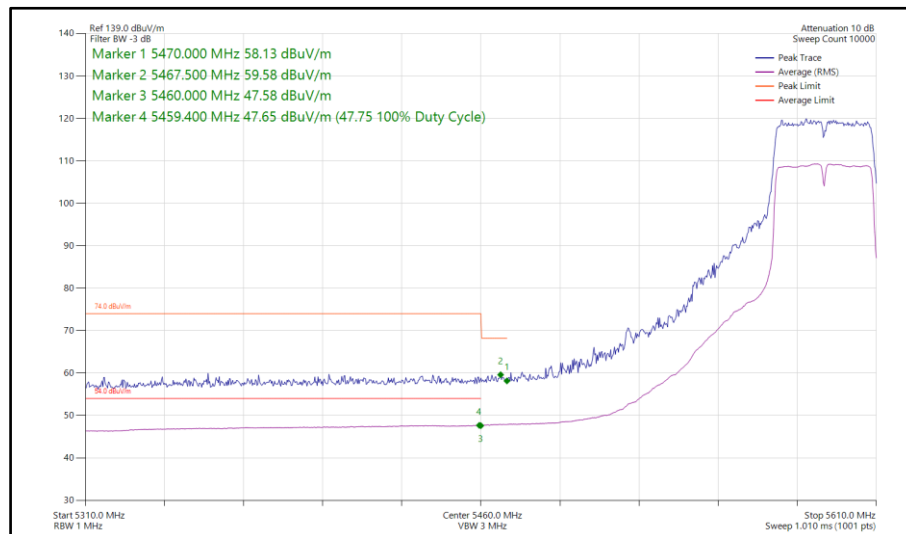
Figure 807 - 802.11n HT40, SDM, Core 0-1 - 5590 MHz Band Edge Frequency 5470 MHz
