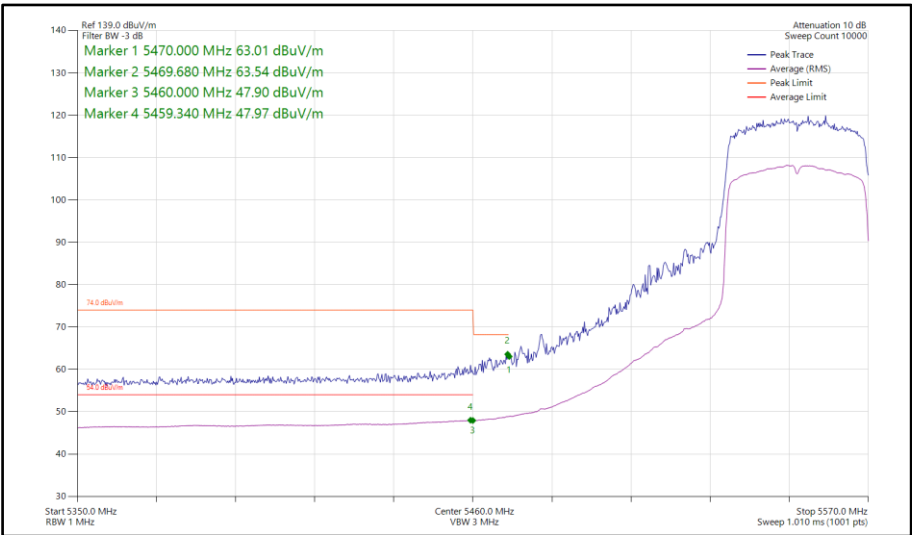
Figure 810 - 802.11ax HE40, SU, SDM, Core 0-1 - 5550 MHz Band Edge Frequency 5470 MHz
