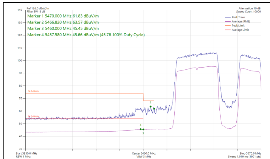
Figure 878 - 802.11be EHT80, RU484+242-92, SISO, Core 1 - 5530 MHz Band Edge Frequency 5470 MHz
