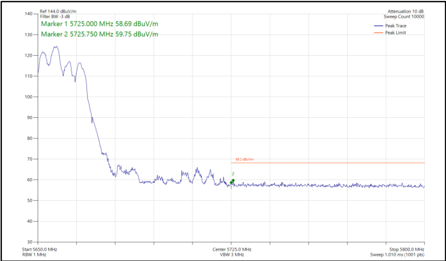
Figure 823 - 802.11ax HE40, RU106-53, SDM, Core 0-1 - 5670 MHz Band Edge Frequency 5725 MHz
