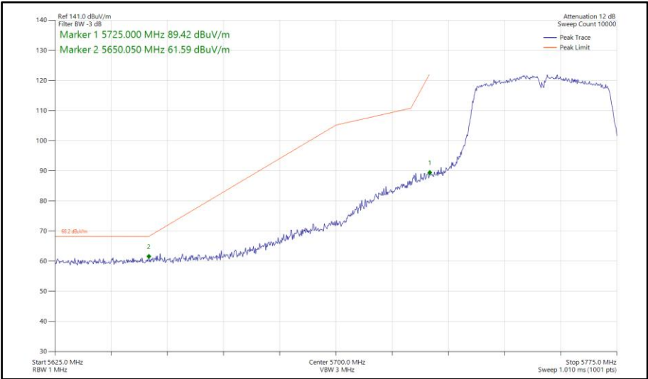
Figure 815 - 802.11n HT40, SDM, Core 0-1 - 5755 MHz Band Edge Frequency 5725 MHz
