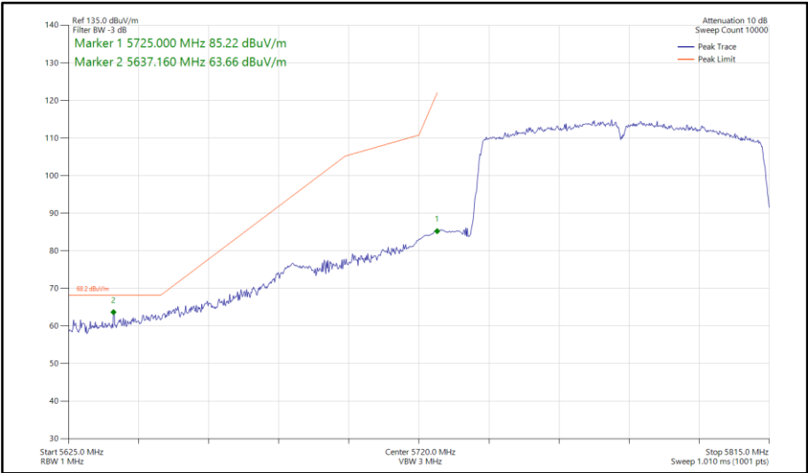
Figure 880 - 802.11ac VHT80, SISO, Core 1 - 5775 MHz Band Edge Frequency 5725 MHz
