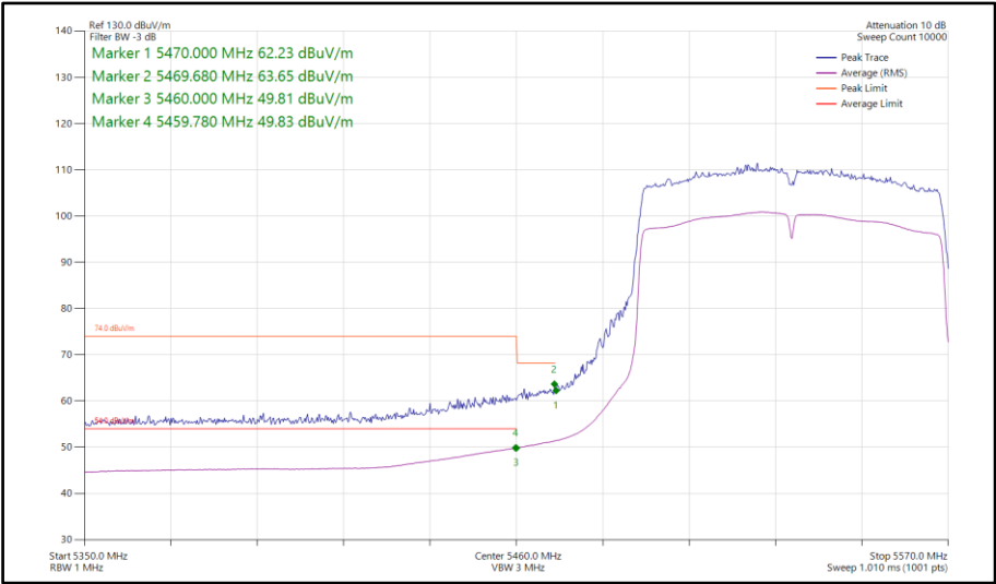
Figure 850 - 802.11ac VHT80, SISO, Core 0 - 5530 MHz Band Edge Frequency 5470 MHz
