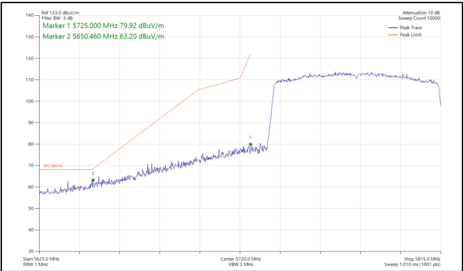
Figure 856 - 802.11ax HE80, SU, SISO, Core 0 - 5775 MHz Band Edge Frequency 5725 MHz
