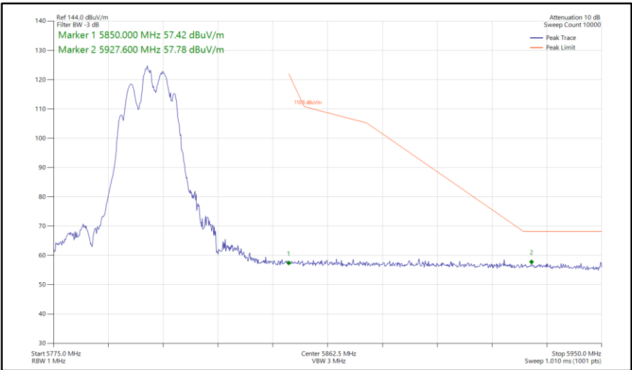
Figure 832 - 802.11be EHT40, RU106+26-85, SDM, Core 0-1 - 5795 MHz Band Edge Frequency 5850 MHz
