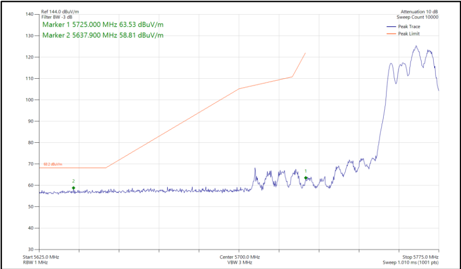
Figure 818 - 802.11be EHT40, RU106+26-85, SDM, Core 0-1 - 5755 MHz Band Edge Frequency 5725 MHz
