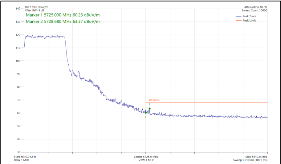
Figure 821 - 802.11ax HE40, SU, SDM, Core 0-1 - 5630 MHz Band Edge Frequency 5725 MHz
