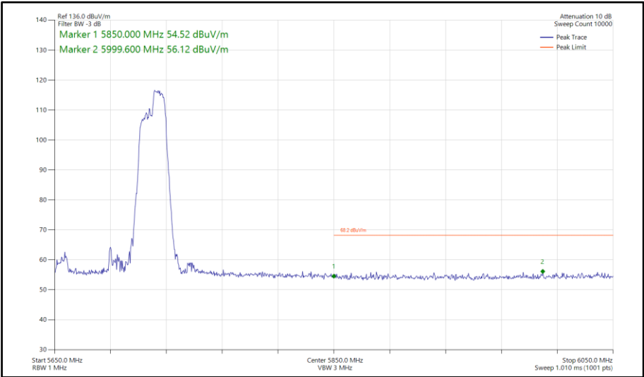
Figure 869 - 802.11ax HE80, RU106-60, SISO, Core 0 - 5690 MHz Band Edge Frequency 5850 MHz
