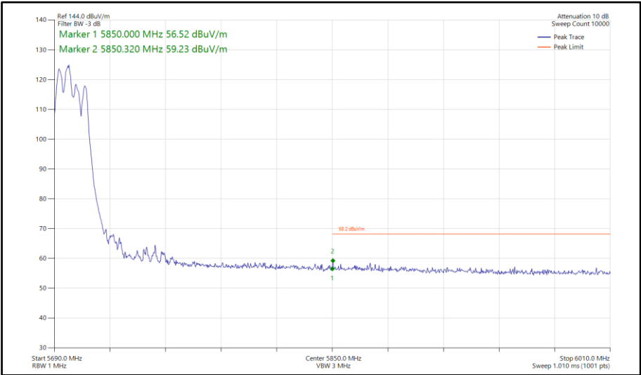
Figure 803 - 802.11be EHT40, RU106+26-82, CDD, Core 0-1 - 5710 MHz Band Edge Frequency 5850 MHz
