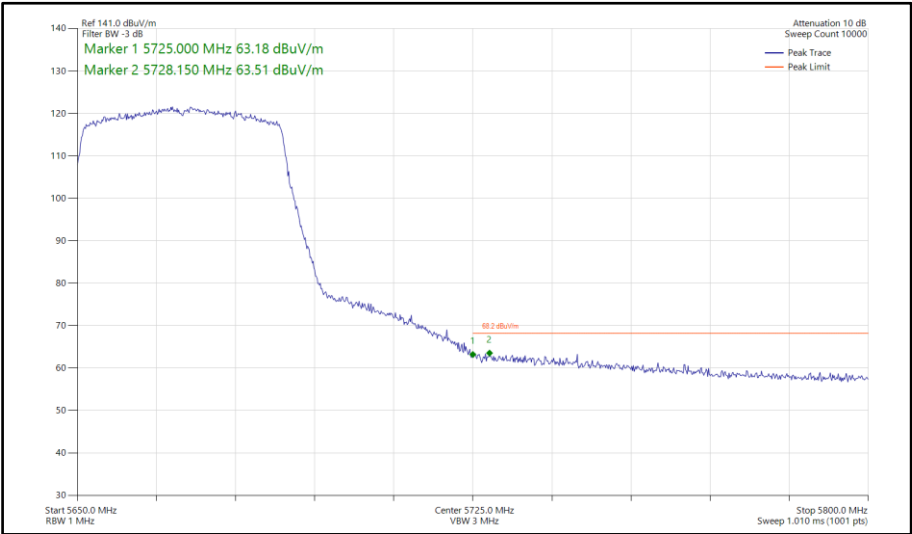
Figure 844 - 802.11ax HE40, SU, TxBF, Core 0-1 - 5670 MHz Band Edge Frequency 5725 MHz
