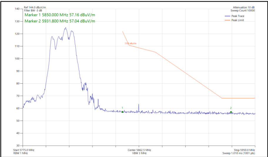
Figure 804 - 802.11be EHT40, RU106+26-85, CDD, Core 0-1 - 5795 MHz Band Edge Frequency 5850 MHz
