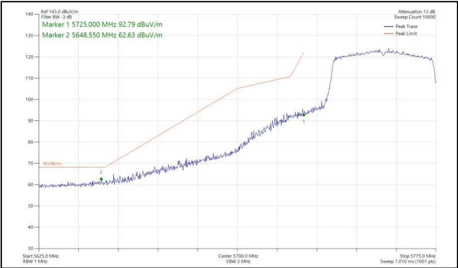
Figure 840 - 802.11ax HE40, SU, TxBF, Core 0-1 - 5755 MHz Band Edge Frequency 5725 MHz
