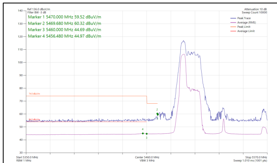
Figure 852 - 802.11ax HE80, RU52-37, SISO, Core 0 - 5530 MHz Band Edge Frequency 5470 MHz
