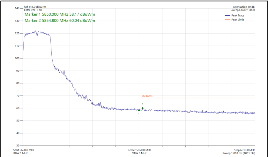
Figure 825 - 802.11n HT40, SDM, Core 0-1 - 5710 MHz Band Edge Frequency 5850 MHz
