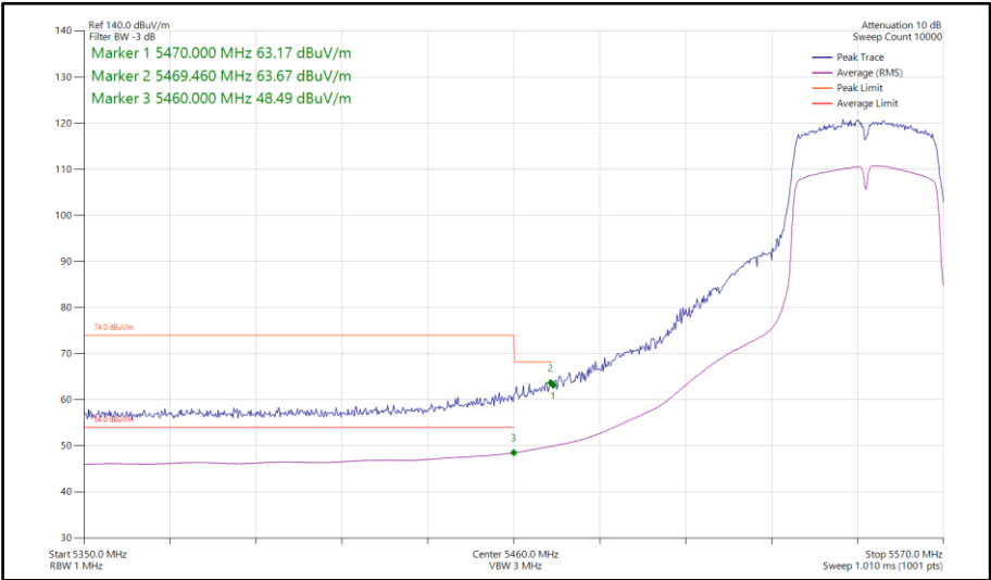
Figure 834 - 802.11ac VHT40, TxBF, Core 0-1 - 5550 MHz Band Edge Frequency 5470 MHz
