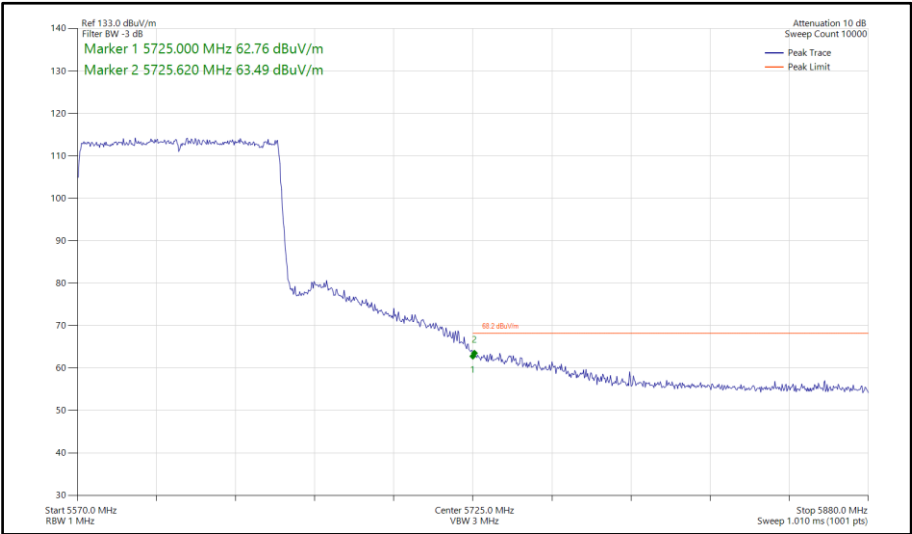
Figure 861 - 802.11ax HE80, SU, SISO, Core 0 - 5610 MHz Band Edge Frequency 5725 MHz
