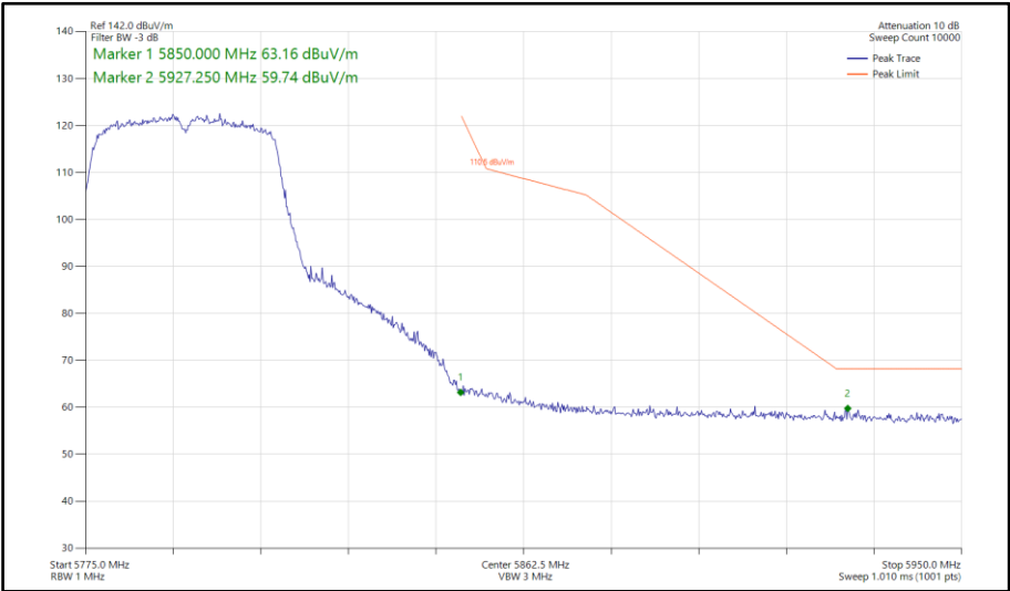
Figure 846 - 802.11ac VHT40, TxBF, Core 0-1 - 5795 MHz Band Edge Frequency 5850 MHz
