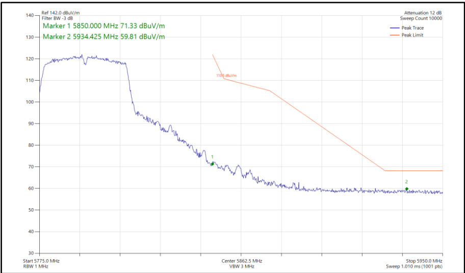
Figure 826 - 802.11n HT40, SDM, Core 0-1 - 5795 MHz Band Edge Frequency 5850 MHz
