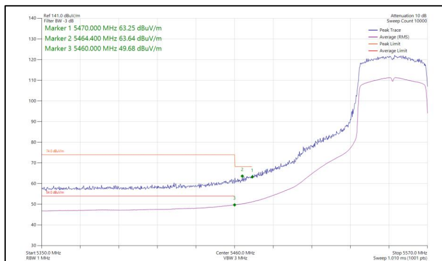
Figure 837 - 802.11ax HE40, SU, TxBF, Core 0-1 - 5550 MHz Band Edge Frequency 5470 MHz
