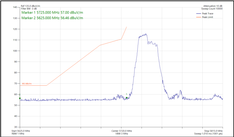
Figure 857 - 802.11ax HE80, RU106-53, SISO, Core 0 - 5775 MHz Band Edge Frequency 5725 MHz
