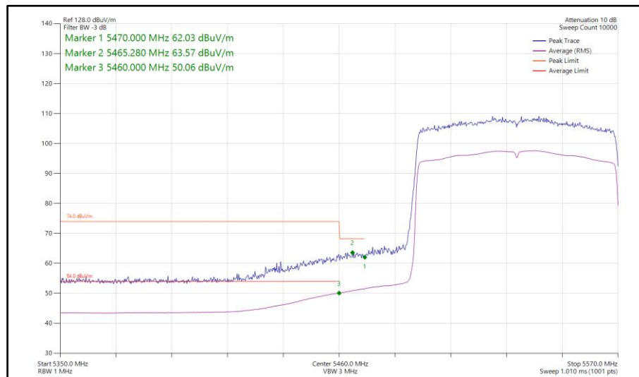
Figure 876 - 802.11ax HE80, SU, SISO, Core 1 - 5530 MHz Band Edge Frequency 5470 MHz
