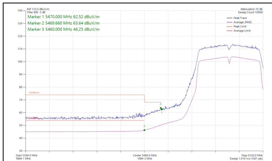
Figure 833 - 802.11ac VHT40, TxBF, Core 0-1 - 5510 MHz Band Edge Frequency 5470 MHz
