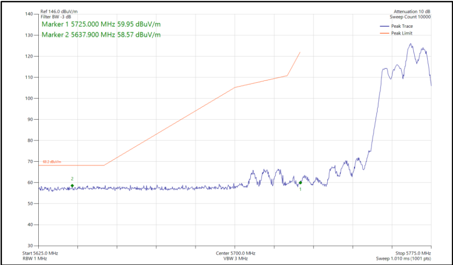
Figure 817 - 802.11ax HE40, RU106-56, SDM, Core 0-1 - 5755 MHz Band Edge Frequency 5725 MHz
