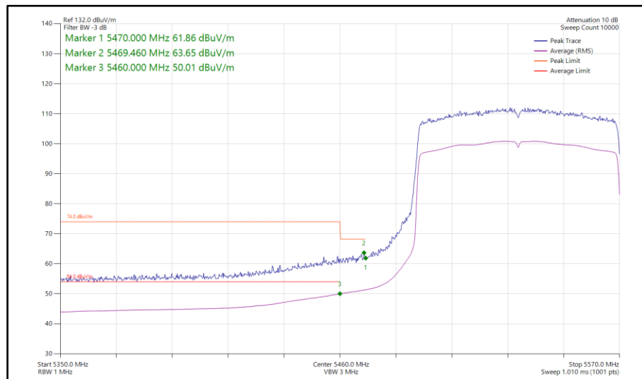
Figure 851 - 802.11ax HE80, SU, SISO, Core 0 - 5530 MHz Band Edge Frequency 5470 MHz
