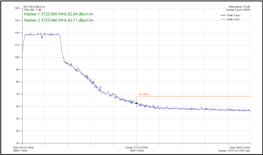
Figure 819 - 802.11n HT40, SDM, Core 0-1 - 5630 MHz Band Edge Frequency 5725 MHz
