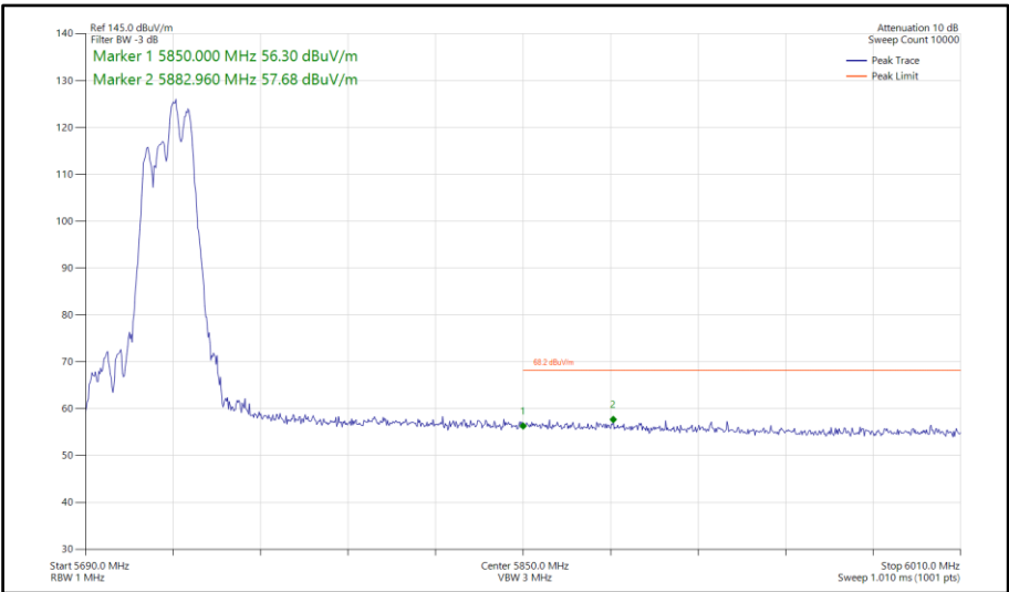
Figure 828 - 802.11ax HE40, RU106-56, SDM, Core 0-1 - 5710 MHz Band Edge Frequency 5850 MHz
