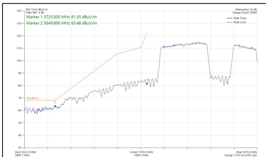
Figure 883 - 802.11be EHT80, RU484+242-92, SISO, Core 1 - 5775 MHz Band Edge Frequency 5725 MHz
