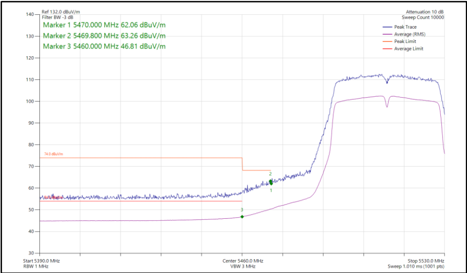
Figure 805 - 802.11n HT40, SDM, Core 0-1 - 5510 MHz Band Edge Frequency 5470 MHz
