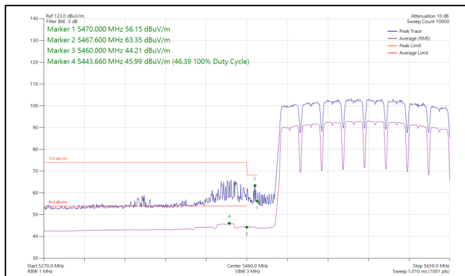
Figure 954 - 802.11a a160, SISO, Core 0 - 5570 MHz Band Edge Frequency 5470 MHz
