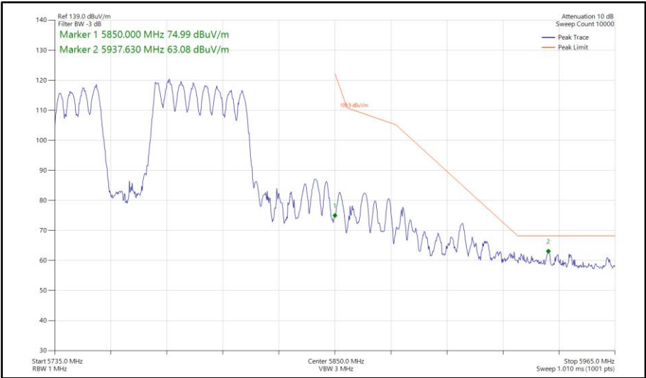
Figure 923 - 802.11be EHT80, RU484+242-91, CDD, Core 0-1 - 5775 MHz Band Edge Frequency 5850 MHz
