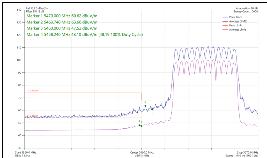
Figure 927 - 802.11be EHT80, RU484+242-93, SDM, Core 0-1 - 5530 MHz Band Edge Frequency 5470 MHz
