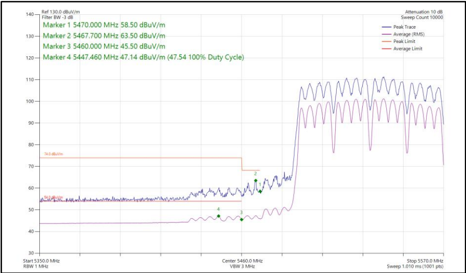
Figure 899 - 802.11a a80, CDD, Core 0-1 - 5530 MHz Band Edge Frequency 5470 MHz
