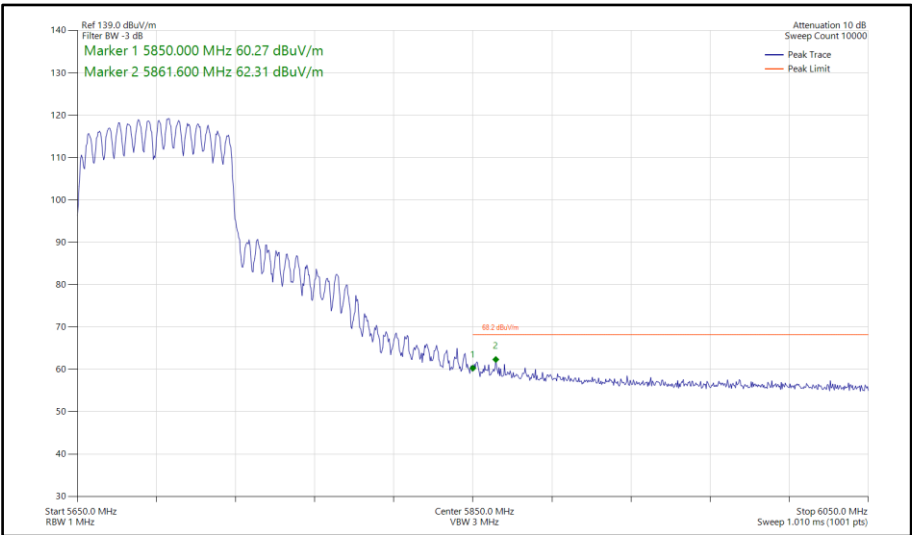
Figure 916 - 802.11ac VHT80, CDD, Core 0-1 - 5690 MHz Band Edge Frequency 5850 MHz
