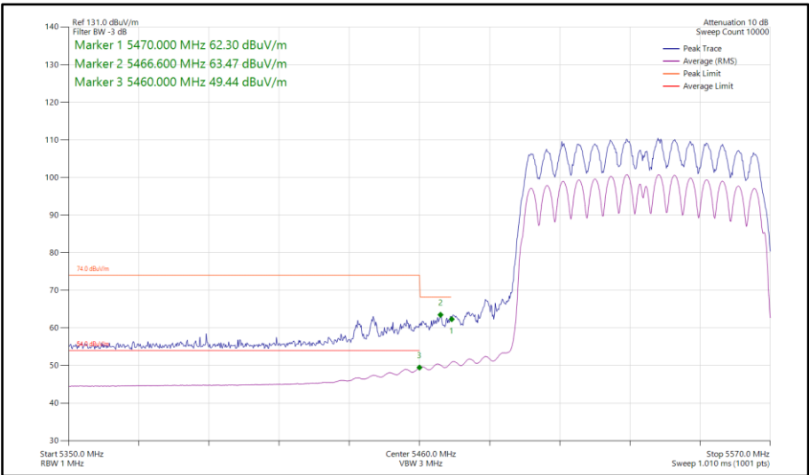
Figure 900 - 802.11ac VHT80, CDD, Core 0-1 - 5530 MHz Band Edge Frequency 5470 MHz
