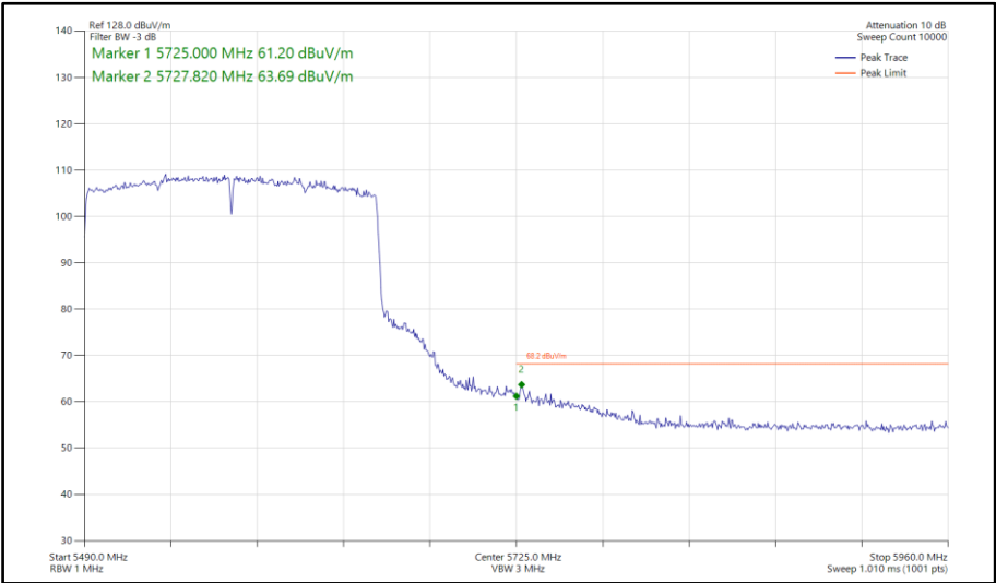
Figure 961 - 802.11ax HE160, SU, SISO, Core 0 - 5570 MHz Band Edge Frequency 5725 MHz
