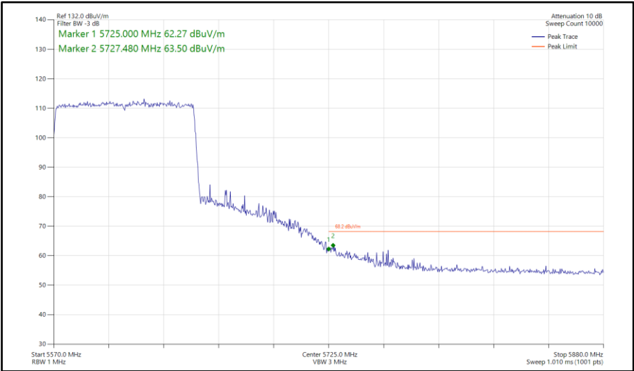
Figure 886 - 802.11ax HE80, SU, SISO, Core 1 - 5610 MHz Band Edge Frequency 5725 MHz
