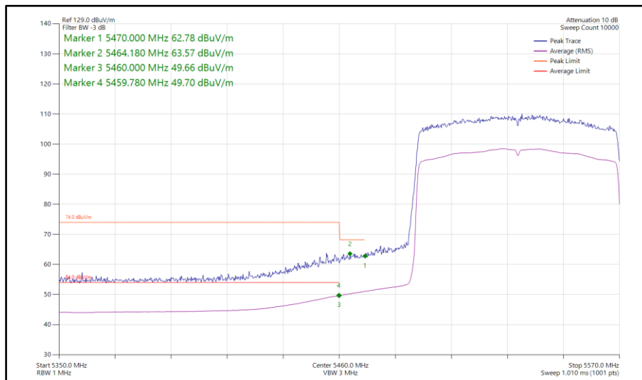
Figure 945 - 802.11ax HE80, SU, TxBF, Core 0-1 - 5530 MHz Band Edge Frequency 5470 MHz
