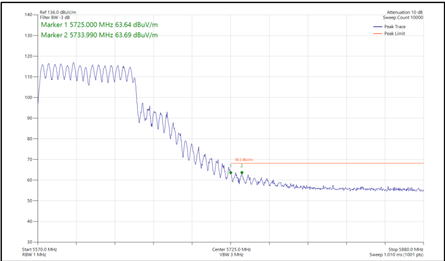
Figure 910 - 802.11ac VHT80, CDD, Core 0-1 - 5610 MHz Band Edge Frequency 5725 MHz
