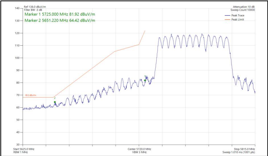
Figure 908 - 802.11be EHT80, RU484+242-93, CDD, Core 0-1 - 5775 MHz Band Edge Frequency 5725 MHz
