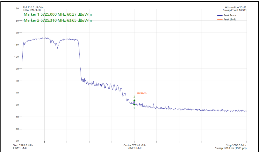
Figure 948 - 802.11ac VHT80, TxBF, Core 0-1 - 5610 MHz Band Edge Frequency 5725 MHz
