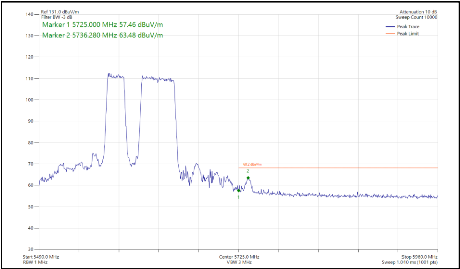
Figure 963 - 802.11be EHT160, RU484+242-91S, SISO, Core 0 - 5570 MHz Band Edge Frequency 5725 MHz
