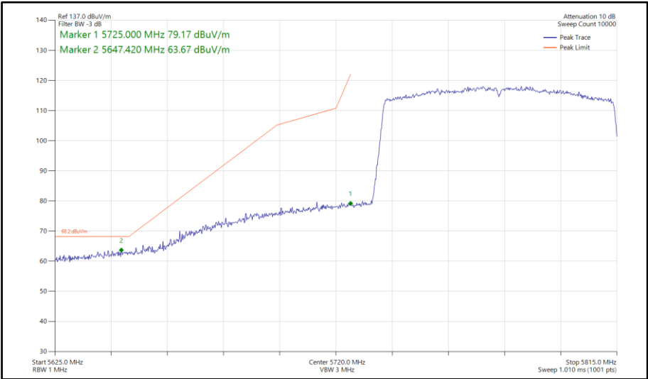
Figure 947 - 802.11ax HE80, SU, TxBF, Core 0-1 - 5775 MHz Band Edge Frequency 5725 MHz
