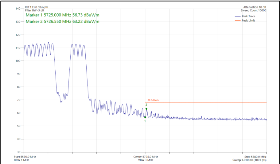
Figure 935 - 802.11be EHT80, RU484+242-92, SDM, Core 0-1 - 5610 MHz Band Edge Frequency 5725 MHz
