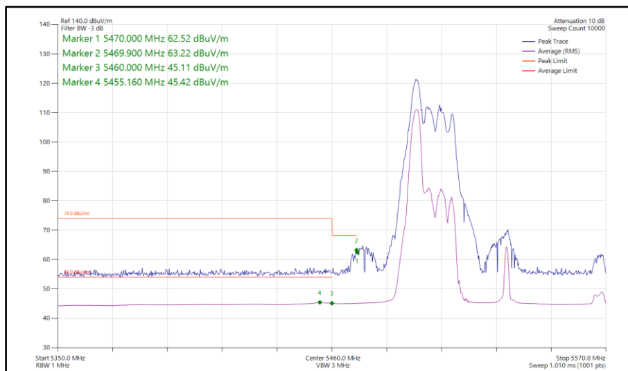
Figure 902 - 802.11ax HE80, RU52-37, CDD, Core 0-1 - 5530 MHz Band Edge Frequency 5470 MHz
