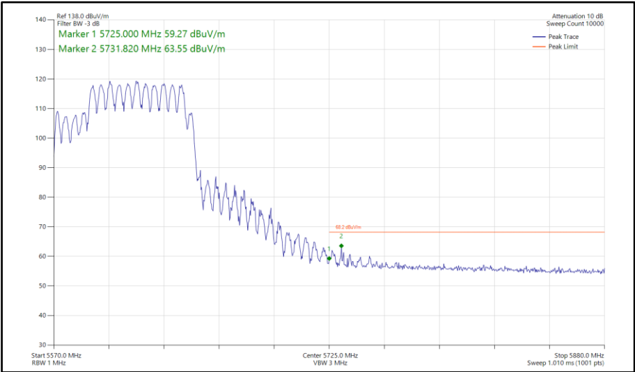
Figure 913 - 802.11be EHT80, RU484+242-90, CDD, Core 0-1 - 5610 MHz Band Edge Frequency 5725 MHz
