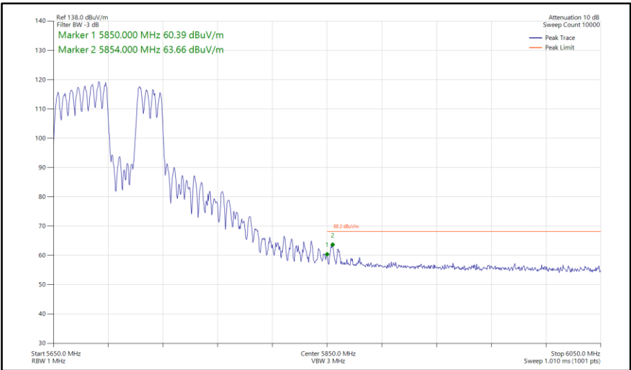
Figure 922 - 802.11be EHT80, RU484+242-92, CDD, Core 0-1 - 5690 MHz Band Edge Frequency 5850 MHz
