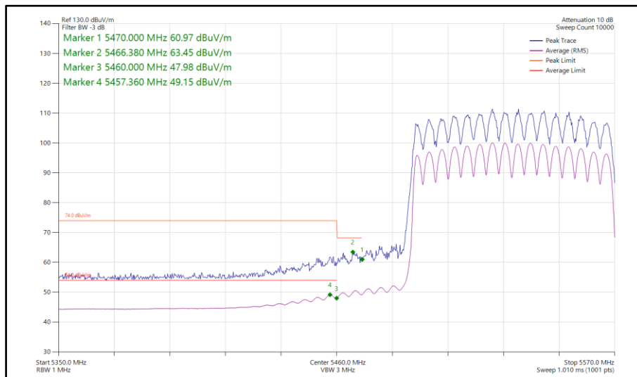
Figure 901 - 802.11ax HE80, SU, CDD, Core 0-1 - 5530 MHz Band Edge Frequency 5470 MHz
