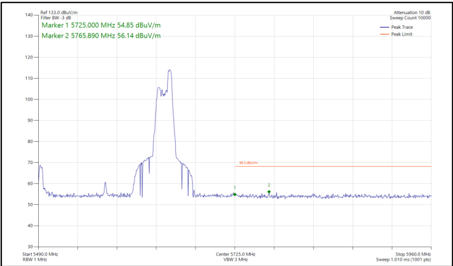
Figure 962 - 802.11ax HE160, RU52-52S, SISO, Core 0 - 5570 MHz Band Edge Frequency 5725 MHz
