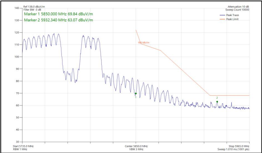
Figure 943 - 802.11be EHT80, RU484+242-92, SDM, Core 0-1 - 5775 MHz Band Edge Frequency 5850 MHz
