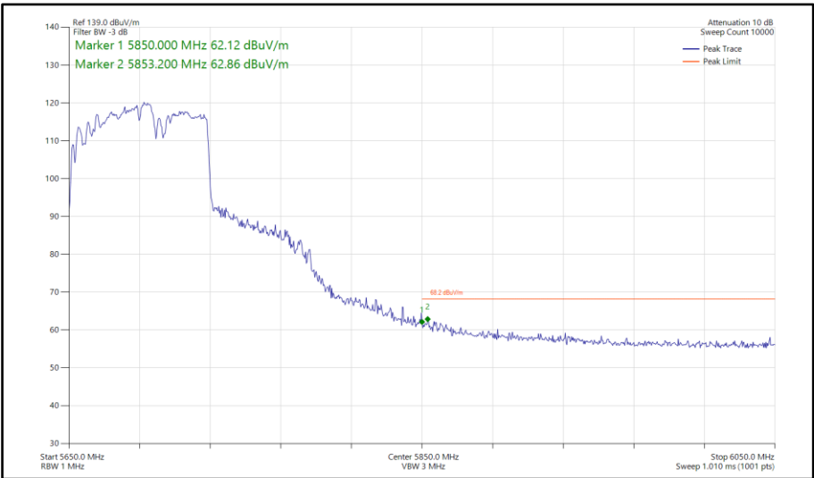
Figure 950 - 802.11ac VHT80, TxBF, Core 0-1 - 5690 MHz Band Edge Frequency 5850 MHz
