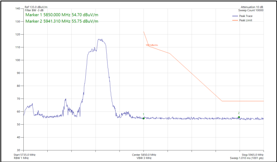
Figure 896 - 802.11ax HE80, RU106-60, SISO, Core 1 - 5775 MHz Band Edge Frequency 5850 MHz
