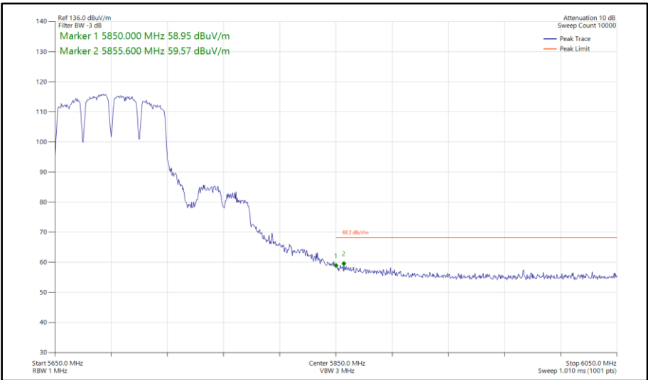
Figure 889 - 802.11a a80, SISO, Core 1 - 5690 MHz Band Edge Frequency 5850 MHz
