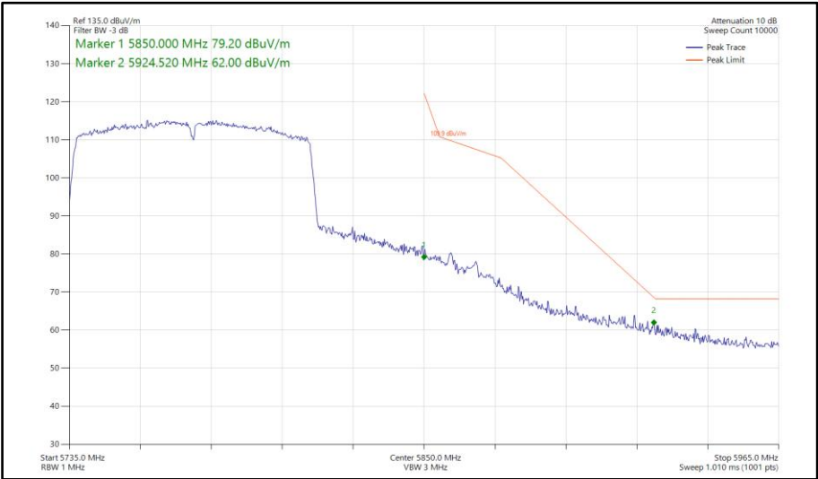
Figure 892 - 802.11ac VHT80, SISO, Core 1 - 5775 MHz Band Edge Frequency 5850 MHz
