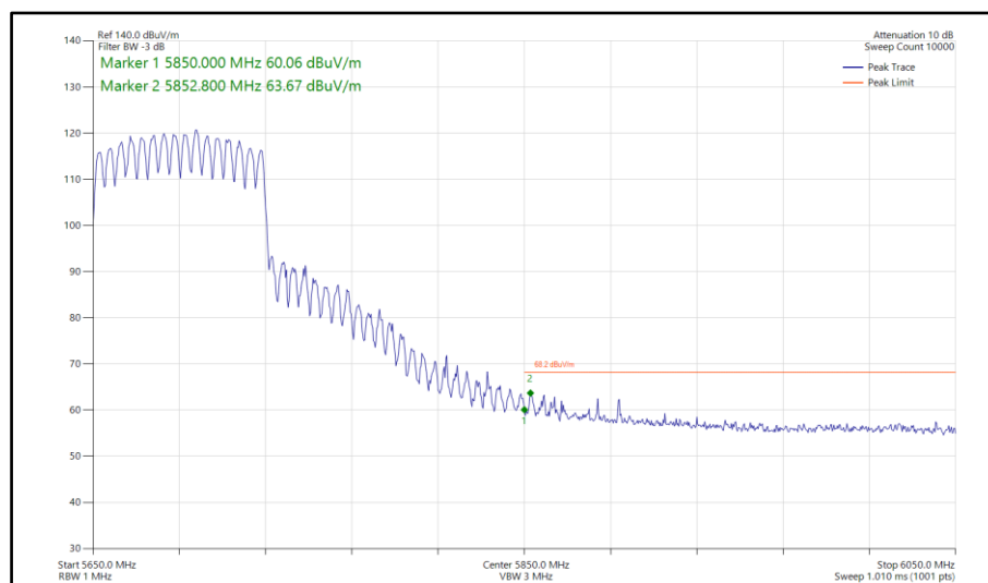
Figure 918 - 802.11ax HE80, SU, CDD, Core 0-1 - 5690 MHz Band Edge Frequency 5850 MHz
