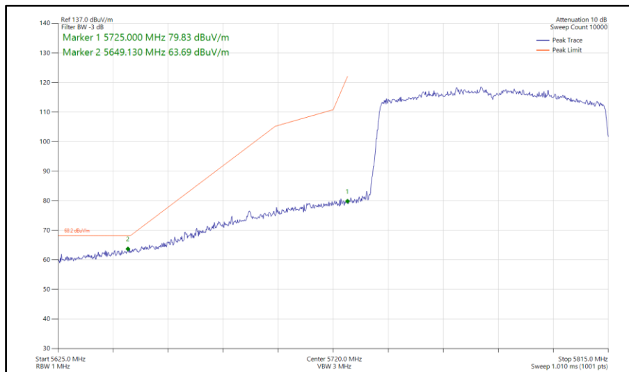
Figure 929 - 802.11ax HE80, SU, SDM, Core 0-1 - 5775 MHz Band Edge Frequency 5725 MHz
