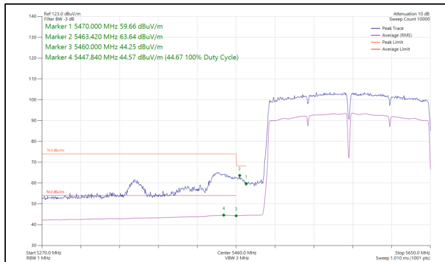
Figure 955 - 802.11ac VHT160, SISO, Core 0 - 5570 MHz Band Edge Frequency 5470 MHz
