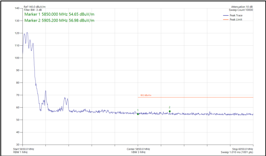
Figure 919 - 802.11ax HE80, RU106-53, CDD, Core 0-1 - 5690 MHz Band Edge Frequency 5850 MHz
