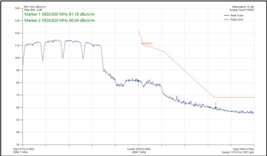
Figure 890 - 802.11a a80, SISO, Core 1 - 5775 MHz Band Edge Frequency 5850 MHz
