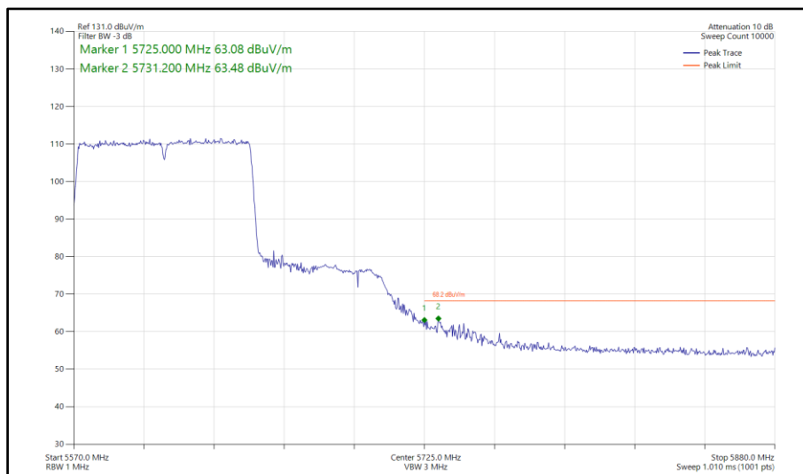
Figure 885 - 802.11ac VHT80, SISO, Core 1 - 5610 MHz Band Edge Frequency 5725 MHz
