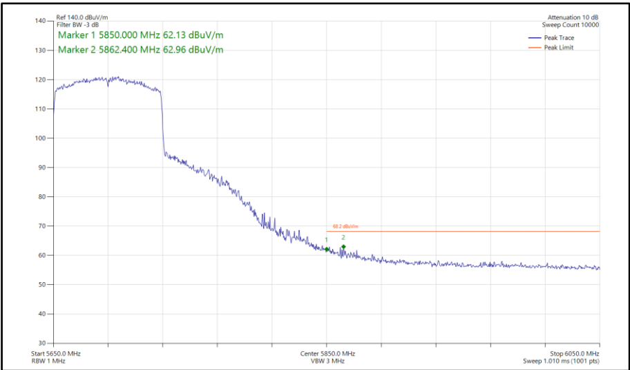
Figure 952 - 802.11ax HE80, SU, TxBF, Core 0-1 - 5690 MHz Band Edge Frequency 5850 MHz
