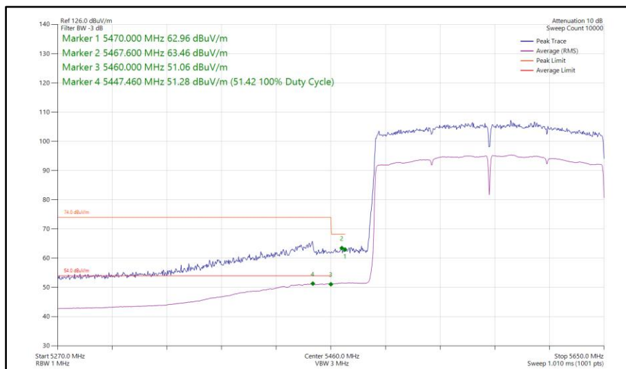
Figure 966 - 802.11ax HE160, SU, SISO, Core 1 - 5570 MHz Band Edge Frequency 5470 MHz
