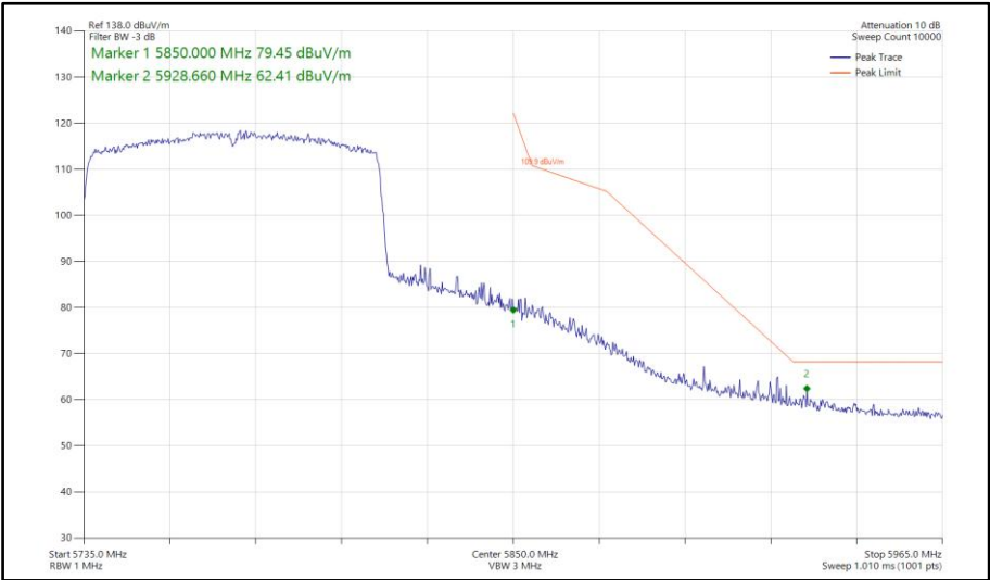
Figure 953 - 802.11ax HE80, SU, TxBF, Core 0-1 - 5775 MHz Band Edge Frequency 5850 MHz
