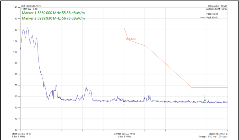
Figure 941 - 802.11ax HE80, RU106-53, SDM, Core 0-1 - 5775 MHz Band Edge Frequency 5850 MHz
