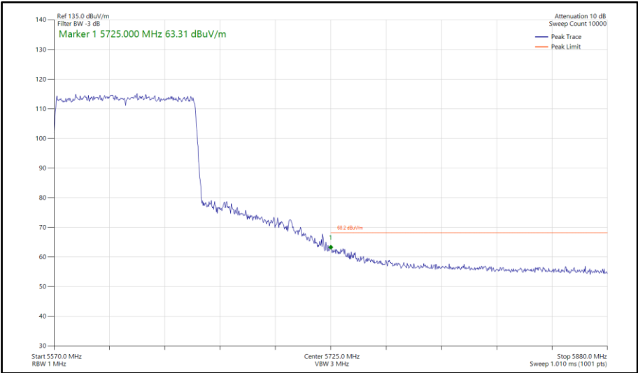
Figure 933 - 802.11ax HE80, SU, SDM, Core 0-1 - 5610 MHz Band Edge Frequency 5725 MHz
