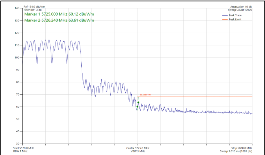
Figure 909 - 802.11a a80, CDD, Core 0-1 - 5610 MHz Band Edge Frequency 5725 MHz
