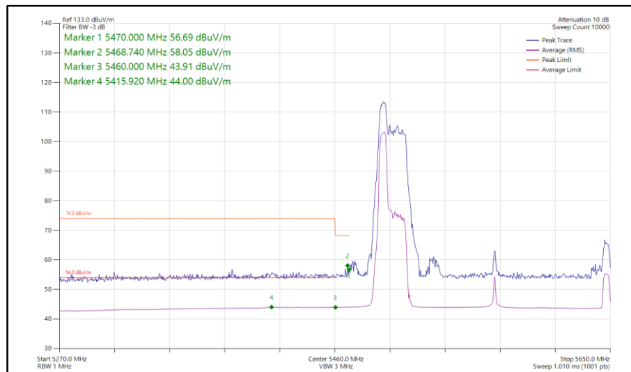
Figure 957 - 802.11ax HE160, RU52-37P, SISO, Core 0 - 5570 MHz Band Edge Frequency 5470 MHz
