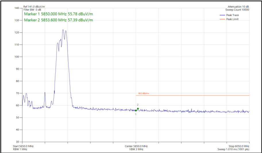
Figure 939 - 802.11ax HE80, RU106-60, SDM, Core 0-1 - 5690 MHz Band Edge Frequency 5850 MHz
