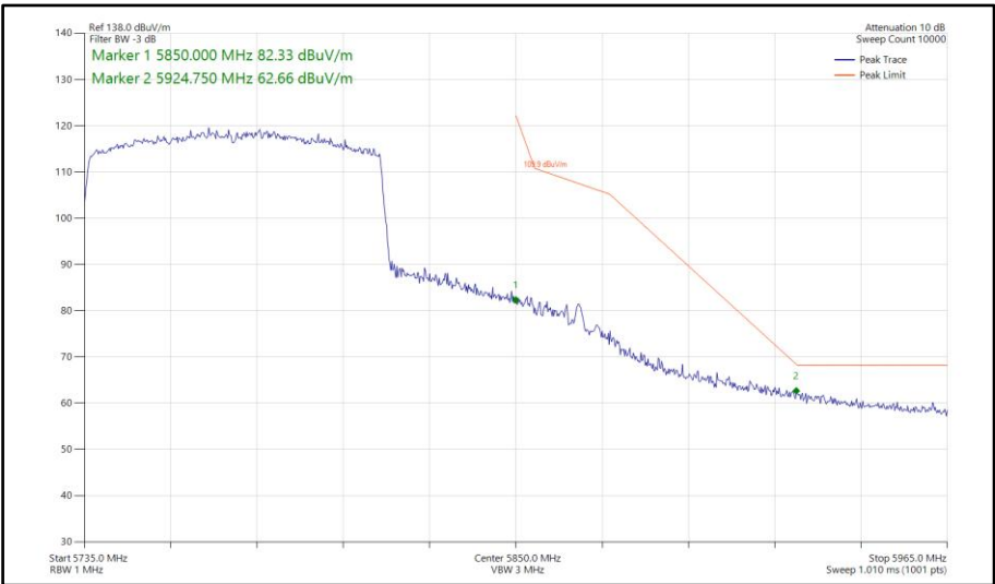
Figure 940 - 802.11ax HE80, SU, SDM, Core 0-1 - 5775 MHz Band Edge Frequency 5850 MHz
