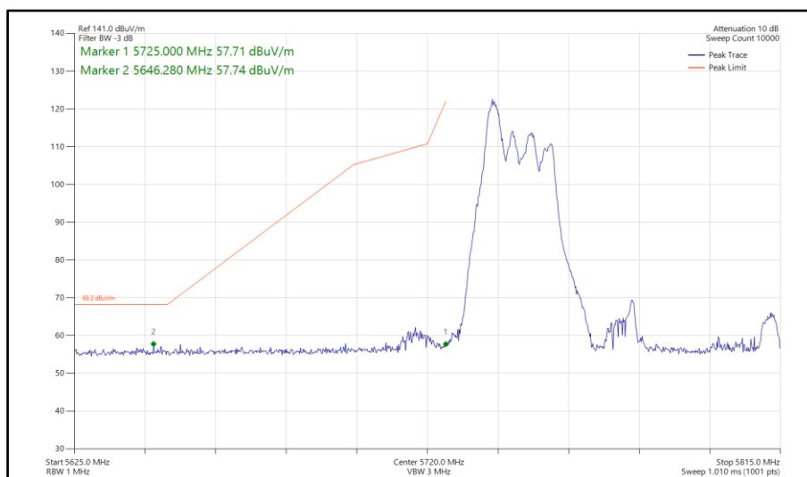
Figure 930 - 802.11ax HE80, RU52-37, SDM, Core 0-1 - 5775 MHz Band Edge Frequency 5725 MHz
