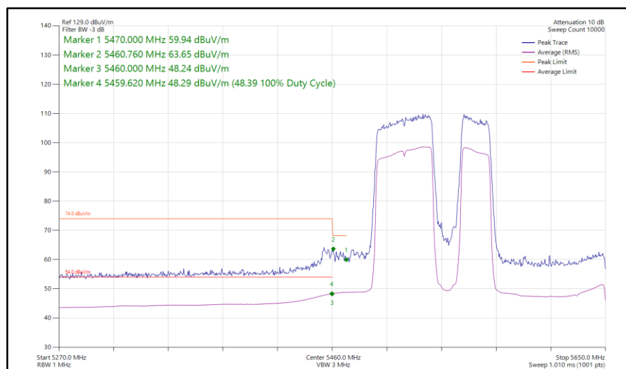
Figure 958 - 802.11be EHT160, RU484+242-92P, SISO, Core 0 - 5570 MHz Band Edge Frequency 5470 MHz
