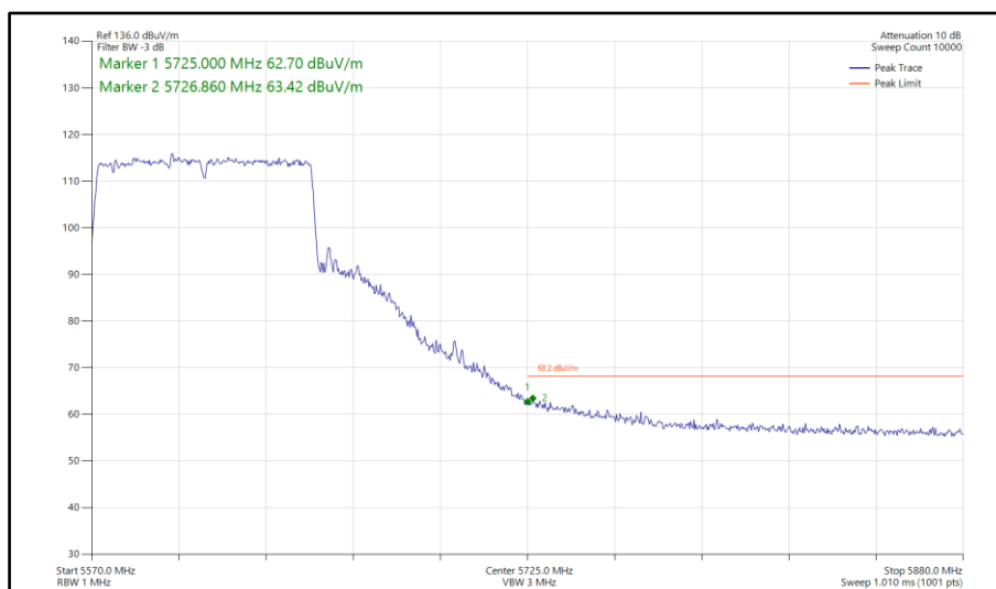
Figure 932 - 802.11ac VHT80, SDM, Core 0-1 - 5610 MHz Band Edge Frequency 5725 MHz
