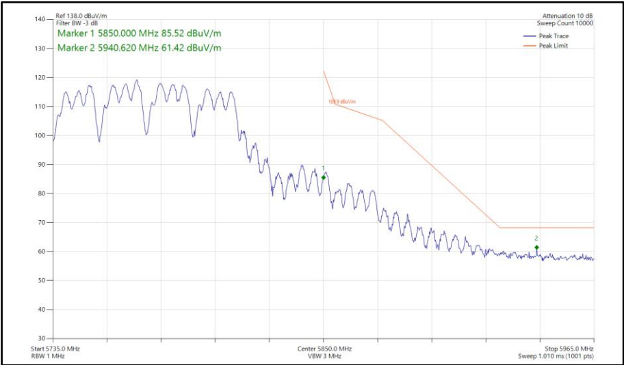
Figure 915 - 802.11a a80, CDD, Core 0-1 - 5775 MHz Band Edge Frequency 5850 MHz
