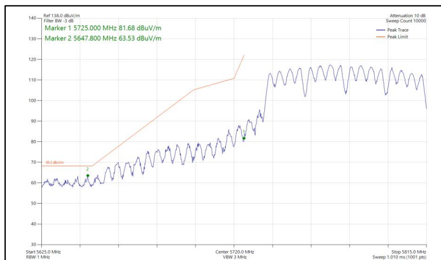
Figure 904 - 802.11a a80, CDD, Core 0-1 - 5775 MHz Band Edge Frequency 5725 MHz
