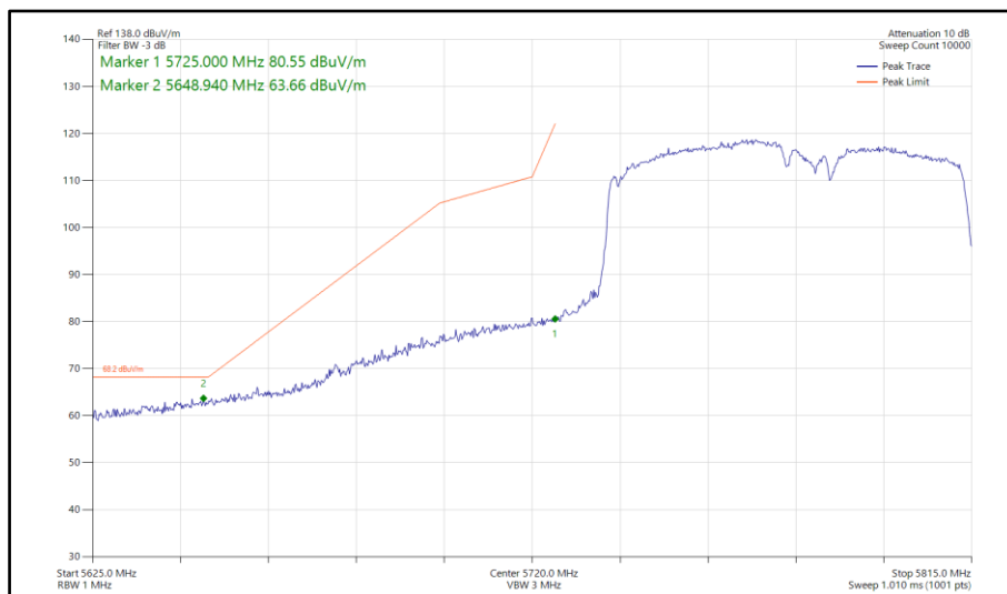
Figure 946 - 802.11ac VHT80, TxBF, Core 0-1 - 5775 MHz Band Edge Frequency 5725 MHz
