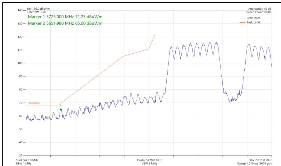
Figure 931 - 802.11be EHT80, RU484+242-92, SDM, Core 0-1 - 5775 MHz Band Edge Frequency 5725 MHz
