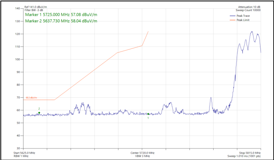
Figure 907 - 802.11ax HE80, RU106-60, CDD, Core 0-1 - 5775 MHz Band Edge Frequency 5725 MHz
