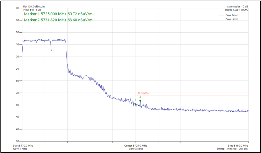
Figure 888 - 802.11be EHT80, RU484+242-93, SISO, Core 1 - 5610 MHz Band Edge Frequency 5725 MHz
