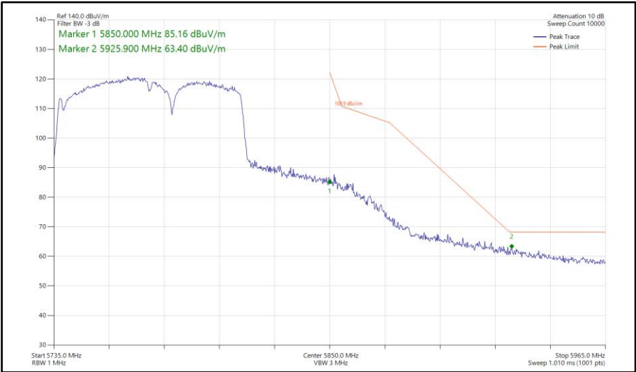
Figure 951 - 802.11ac VHT80, TxBF, Core 0-1 - 5775 MHz Band Edge Frequency 5850 MHz
