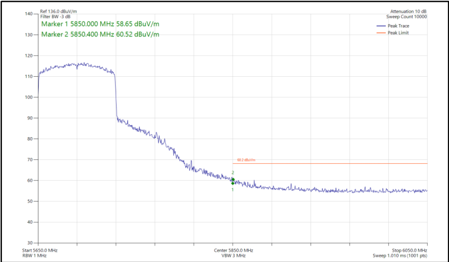
Figure 893 - 802.11ax HE80, SU, SISO, Core 1 - 5690 MHz Band Edge Frequency 5850 MHz
