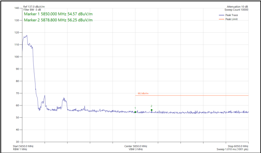
Figure 894 - 802.11ax HE80, RU106-53, SISO, Core 1 - 5690 MHz Band Edge Frequency 5850 MHz
