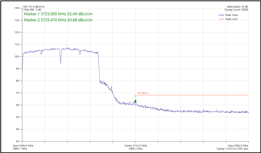
Figure 960 - 802.11ac VHT160, SISO, Core 0 - 5570 MHz Band Edge Frequency 5725 MHz
