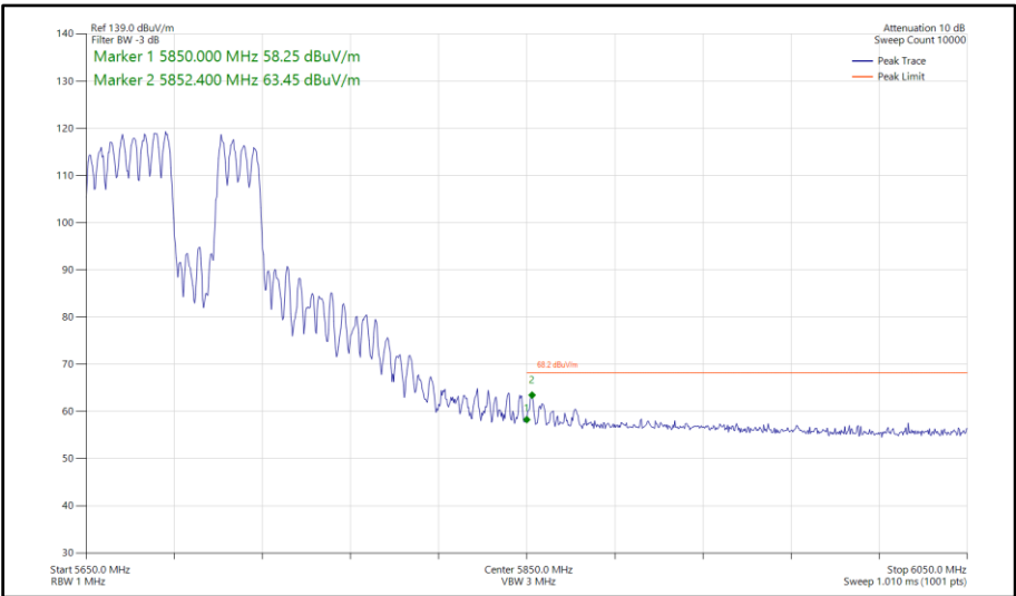
Figure 942 - 802.11be EHT80, RU484+242-92, SDM, Core 0-1 - 5690 MHz Band Edge Frequency 5850 MHz
