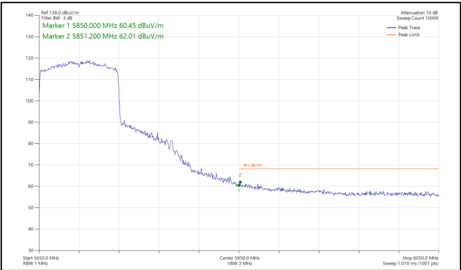
Figure 938 - 802.11ax HE80, SU, SDM, Core 0-1 - 5690 MHz Band Edge Frequency 5850 MHz
