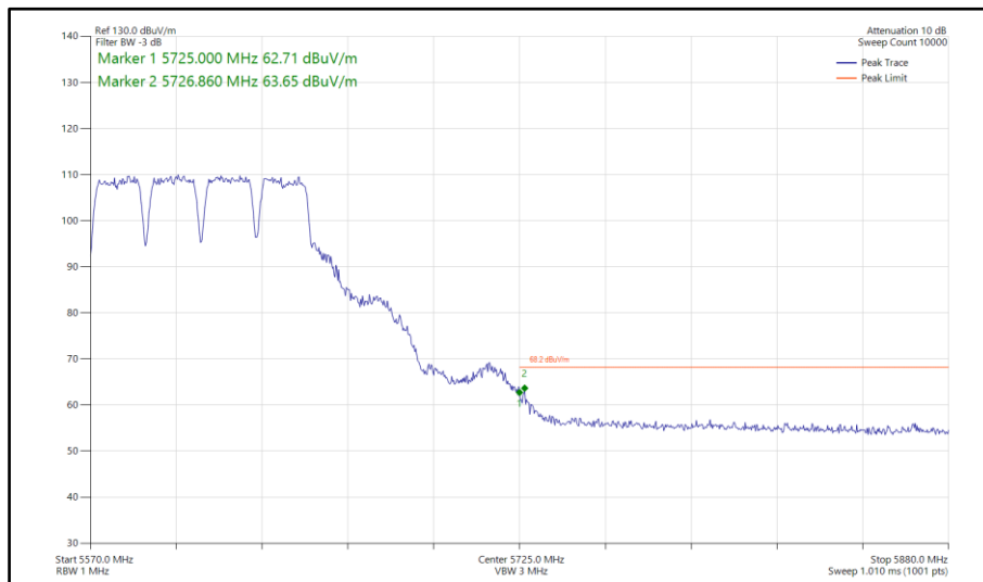
Figure 884 - 802.11a a80, SISO, Core 1 - 5610 MHz Band Edge Frequency 5725 MHz
