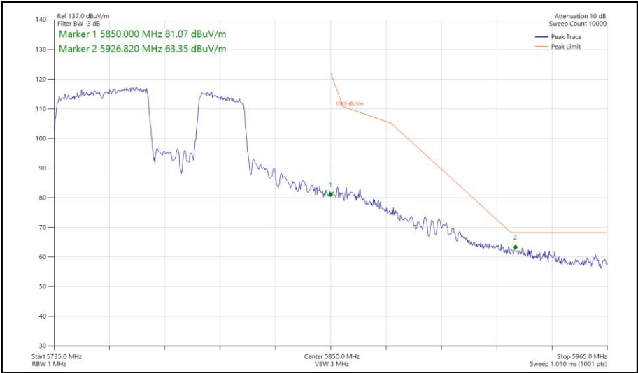
Figure 898 - 802.11be EHT80, RU484+242-92, SISO, Core 1 - 5775 MHz Band Edge Frequency 5850 MHz
