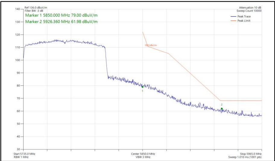
Figure 895 - 802.11ax HE80, SU, SISO, Core 1 - 5775 MHz Band Edge Frequency 5850 MHz
