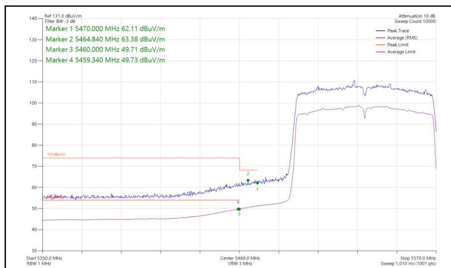
Figure 924 - 802.11ac VHT80, SDM, Core 0-1 - 5530 MHz Band Edge Frequency 5470 MHz
