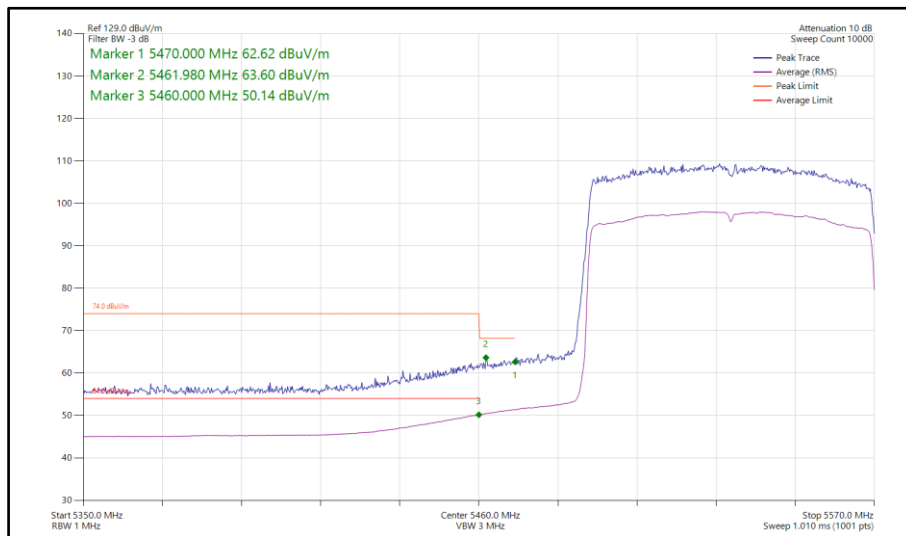
Figure 925 - 802.11ax HE80, SU, SDM, Core 0-1 - 5530 MHz Band Edge Frequency 5470 MHz
