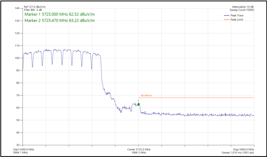
Figure 959 - 802.11a a160, SISO, Core 0 - 5570 MHz Band Edge Frequency 5725 MHz
