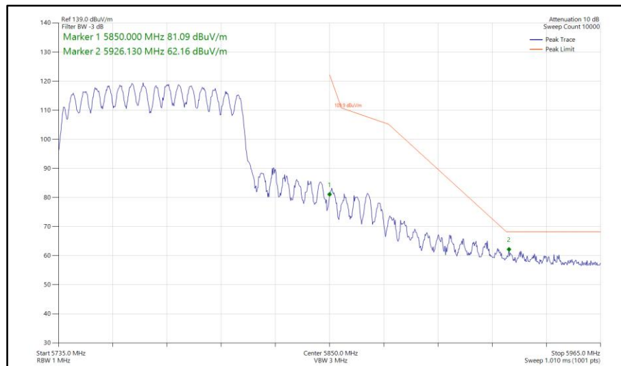
Figure 917 - 802.11ac VHT80, CDD, Core 0-1 - 5775 MHz Band Edge Frequency 5850 MHz
