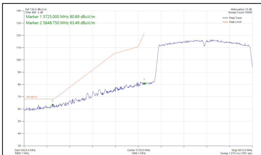
Figure 928 - 802.11ac VHT80, SDM, Core 0-1 - 5775 MHz Band Edge Frequency 5725 MHz
