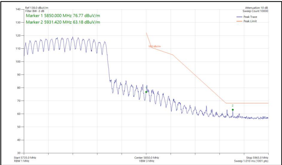
Figure 920 - 802.11ax HE80, SU, CDD, Core 0-1 - 5775 MHz Band Edge Frequency 5850 MHz
