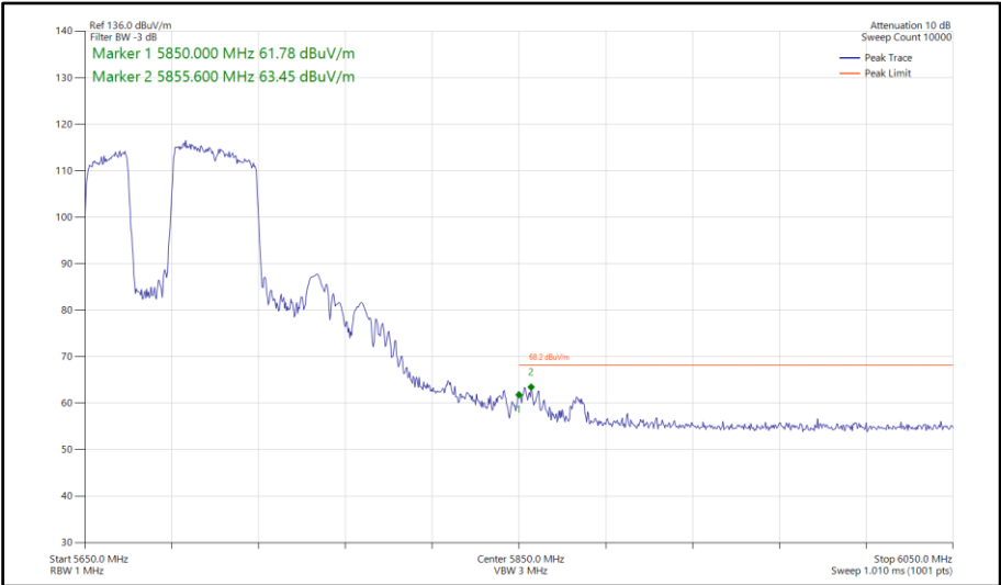
Figure 897 - 802.11be EHT80, RU484+242-91, SISO, Core 1 - 5690 MHz Band Edge Frequency 5850 MHz
