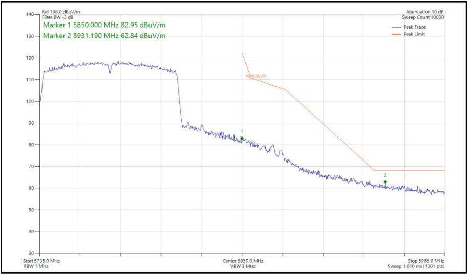
Figure 937 - 802.11ac VHT80, SDM, Core 0-1 - 5775 MHz Band Edge Frequency 5850 MHz
