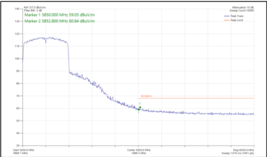
Figure 936 - 802.11ac VHT80, SDM, Core 0-1 - 5690 MHz Band Edge Frequency 5850 MHz
