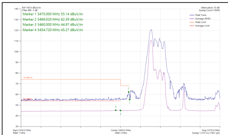
Figure 926 - 802.11ax HE80, RU52-37, SDM, Core 0-1 - 5530 MHz Band Edge Frequency 5470 MHz
