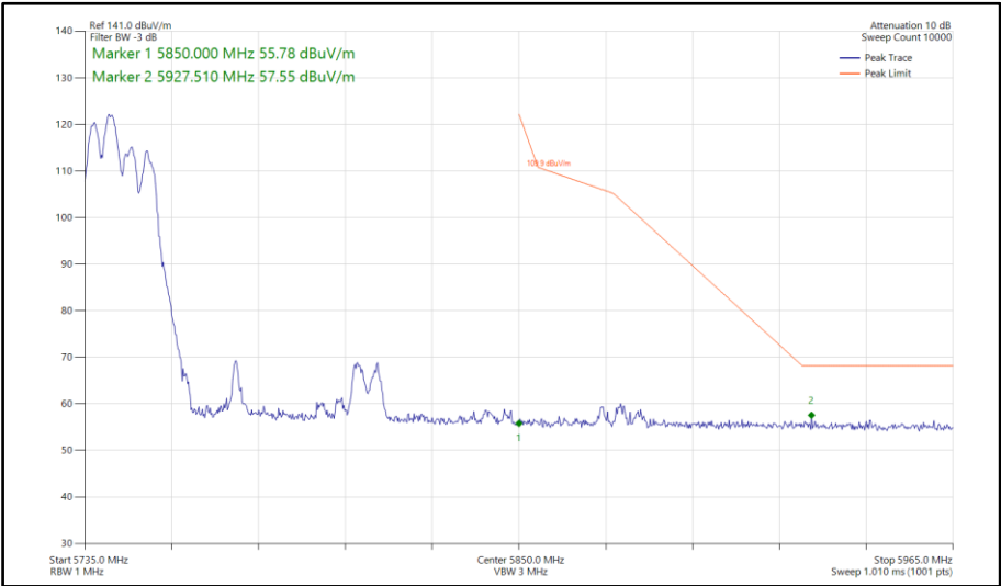
Figure 921 - 802.11ax HE80, RU106-53, CDD, Core 0-1 - 5775 MHz Band Edge Frequency 5850 MHz
