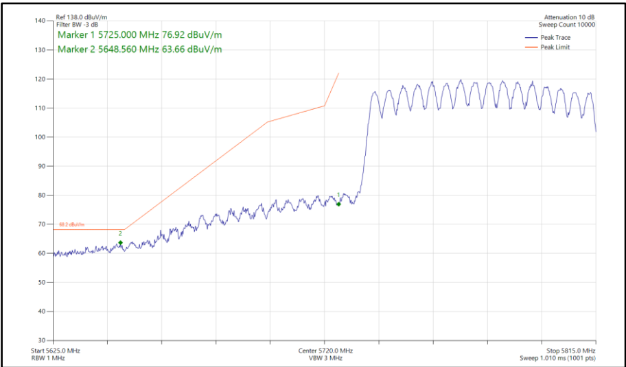
Figure 906 - 802.11ax HE80, SU, CDD, Core 0-1 - 5775 MHz Band Edge Frequency 5725 MHz
