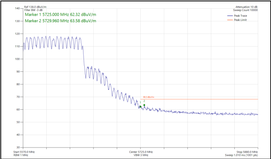
Figure 911 - 802.11ax HE80, SU, CDD, Core 0-1 - 5610 MHz Band Edge Frequency 5725 MHz
