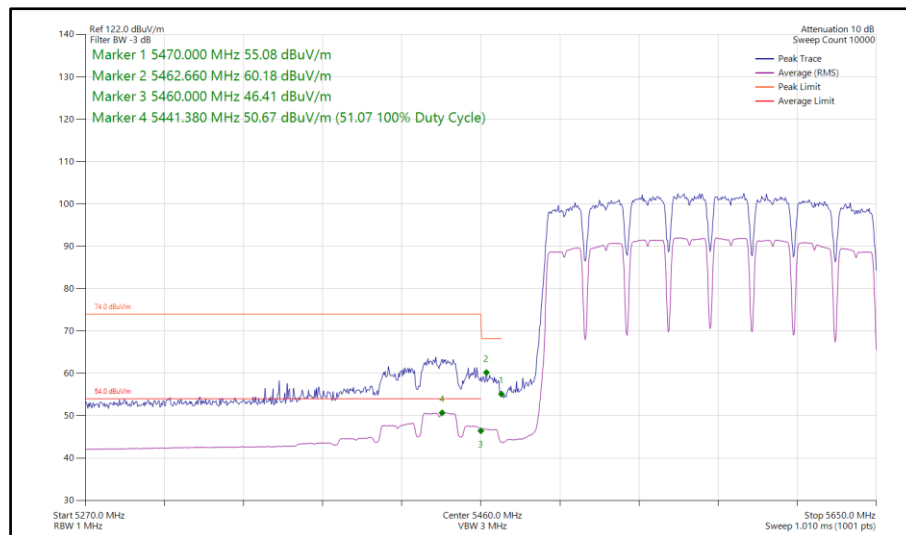
Figure 964 - 802.11a a160, SISO, Core 1 - 5570 MHz Band Edge Frequency 5470 MHz
