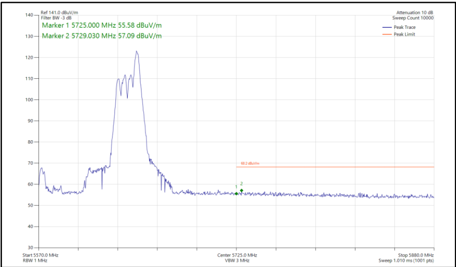
Figure 934 - 802.11ax HE80, RU52-52, SDM, Core 0-1 - 5610 MHz Band Edge Frequency 5725 MHz
