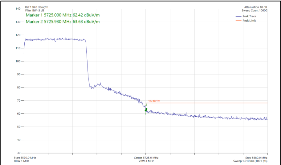
Figure 949 - 802.11ax HE80, SU, TxBF, Core 0-1 - 5610 MHz Band Edge Frequency 5725 MHz
