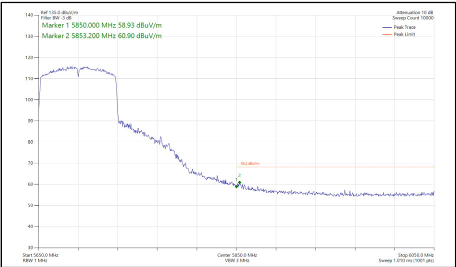
Figure 891 - 802.11ac VHT80, SISO, Core 1 - 5690 MHz Band Edge Frequency 5850 MHz
