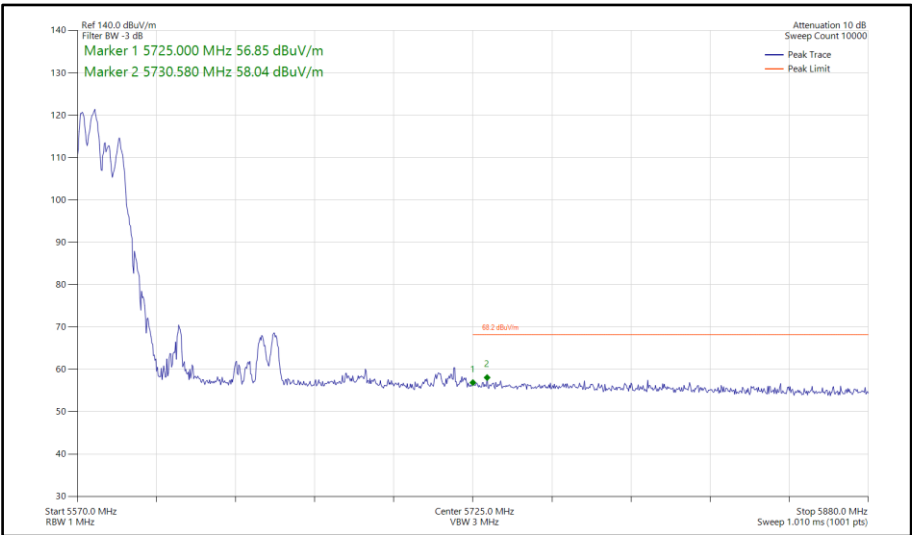
Figure 912 - 802.11ax HE80, RU106-53, CDD, Core 0-1 - 5610 MHz Band Edge Frequency 5725 MHz
