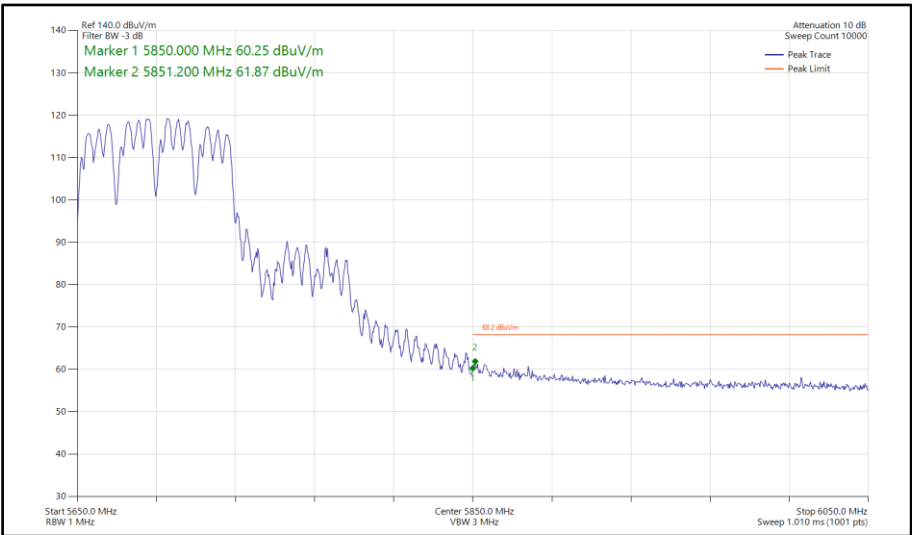
Figure 914 - 802.11a a80, CDD, Core 0-1 - 5690 MHz Band Edge Frequency 5850 MHz
