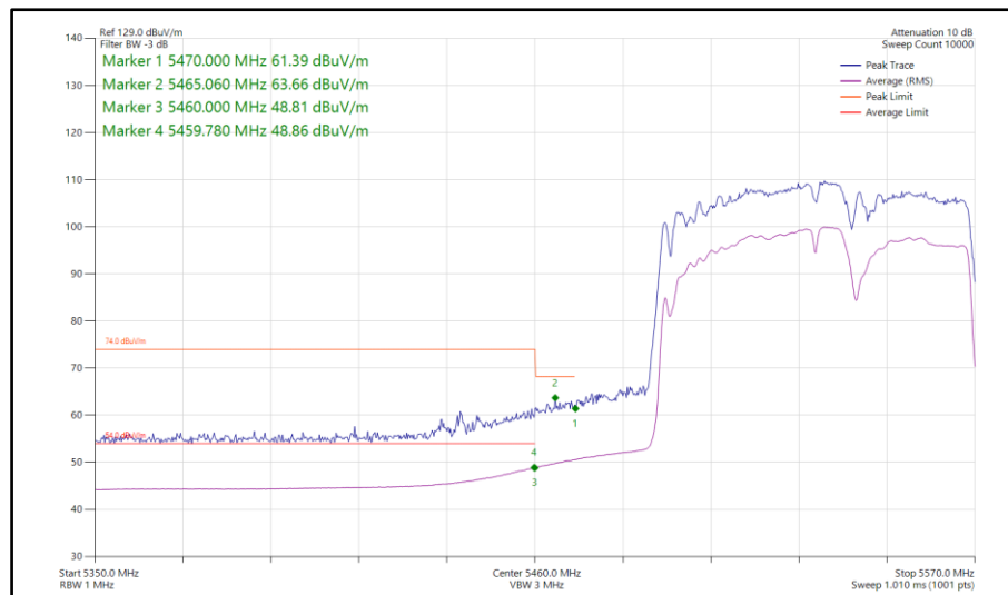
Figure 944 - 802.11ac VHT80, TxBF, Core 0-1 - 5530 MHz Band Edge Frequency 5470 MHz
