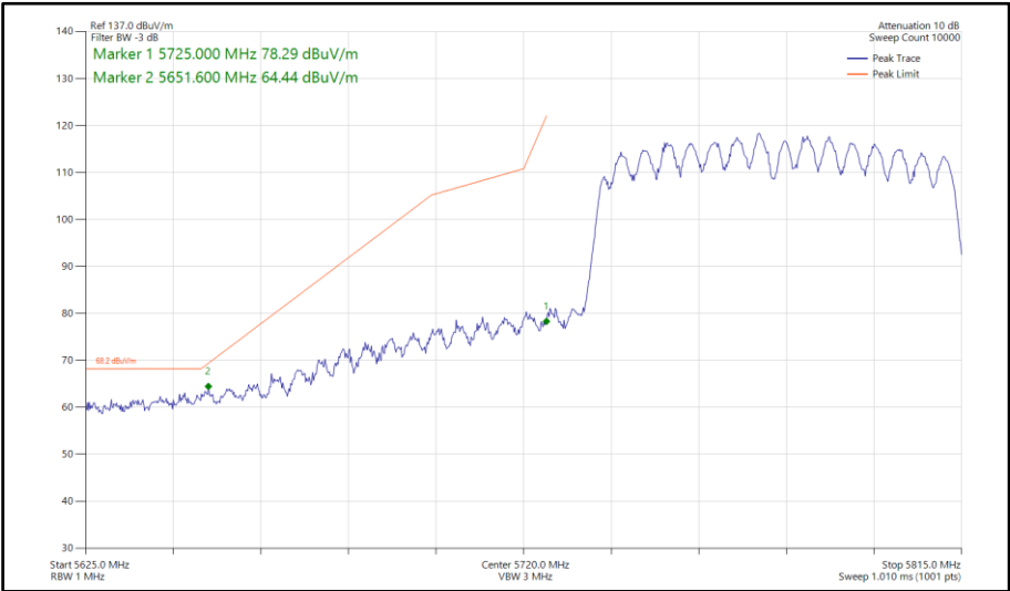
Figure 905 - 802.11ac VHT80, CDD, Core 0-1 - 5775 MHz Band Edge Frequency 5725 MHz
