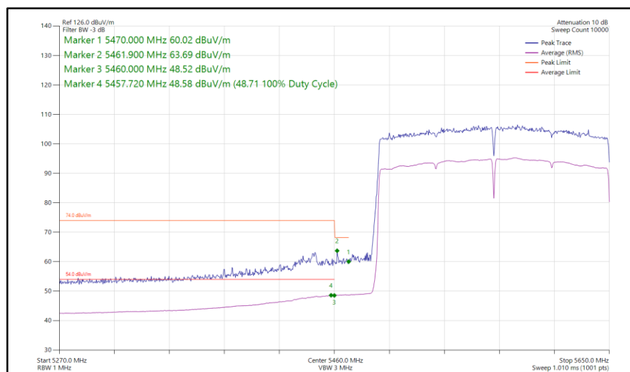
Figure 956 - 802.11ax HE160, SU, SISO, Core 0 - 5570 MHz Band Edge Frequency 5470 MHz
