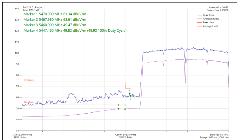
Figure 965 - 802.11ac VHT160, SISO, Core 1 - 5570 MHz Band Edge Frequency 5470 MHz
