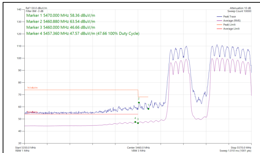
Figure 903 - 802.11be EHT80, RU484+242-91, CDD, Core 0-1 - 5530 MHz Band Edge Frequency 5470 MHz
