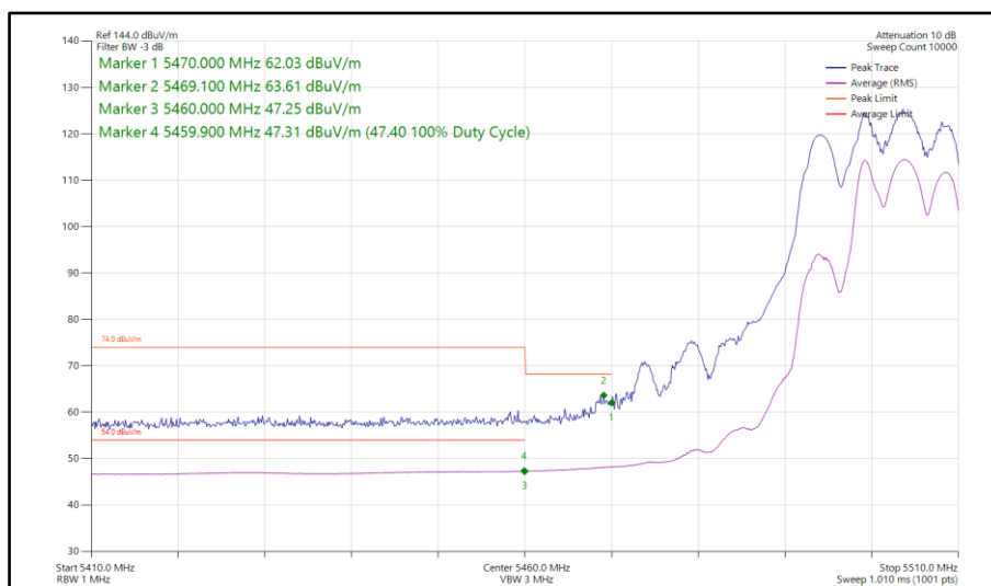
Figure 72 - 802.11be EHT20, RU106+26-83, CDD, Core 0-1 - 5500 MHz Band Edge Frequency 5460 MHz
