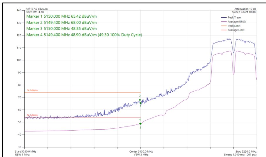
Figure 104 - 802.11a a40, SISO, Core 0 - 5230 MHz Band Edge Frequency 5150 MHz
