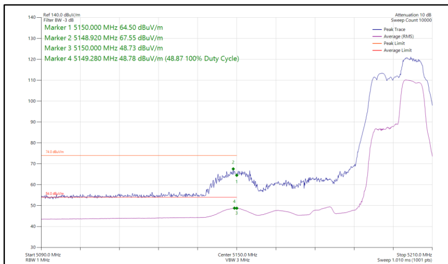
Figure 110 - 802.11be EHT40, RU52+26-75, SISO, Core 0 - 5190 MHz Band Edge Frequency 5150 MHz
