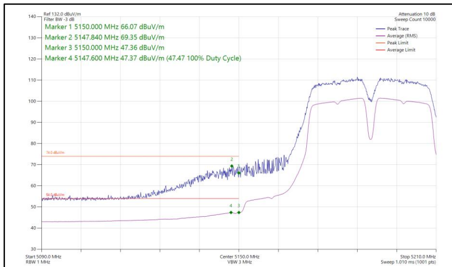
Figure 103 - 802.11a a40, SISO, Core 0 - 5190 MHz Band Edge Frequency 5150 MHz
