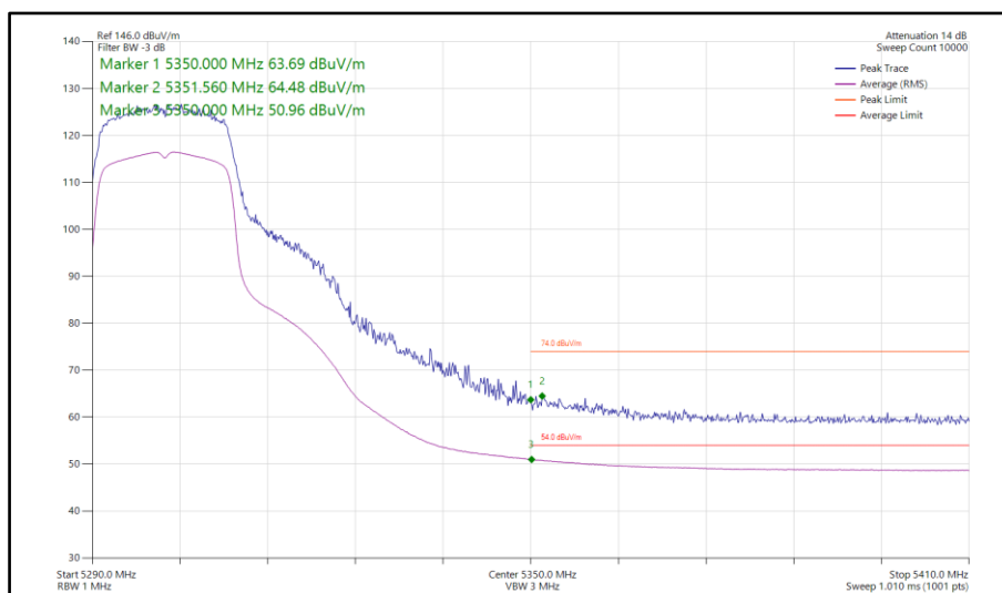
Figure 95 - 802.11ac VHT20, TxBF, Core 0-1 - 5300 MHz Band Edge Frequency 5350 MHz
