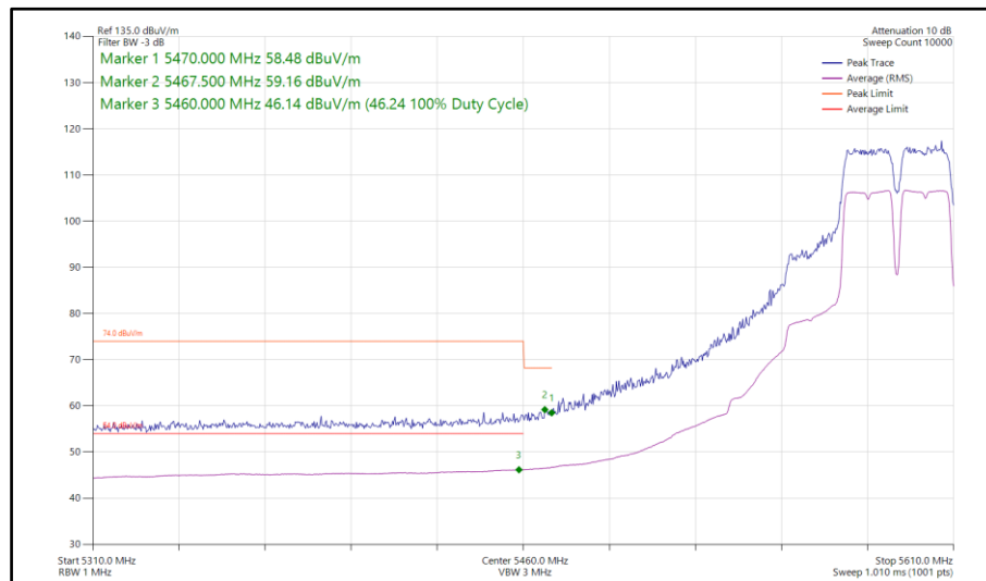
Figure 121 - 802.11a a40, SISO, Core 0 - 5590 MHz Band Edge Frequency 5460 MHz
