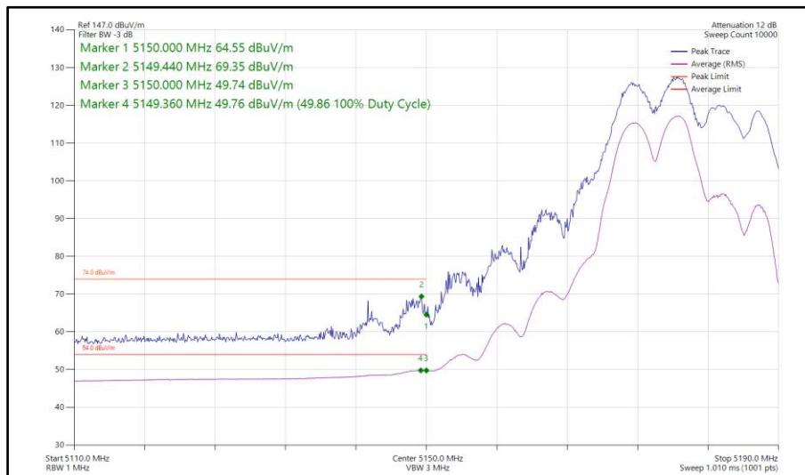
Figure 78 - 802.11be EHT20, RU106+26-82, SDM, Core 0-1 - 5180 MHz Band Edge Frequency 5150 MHz
