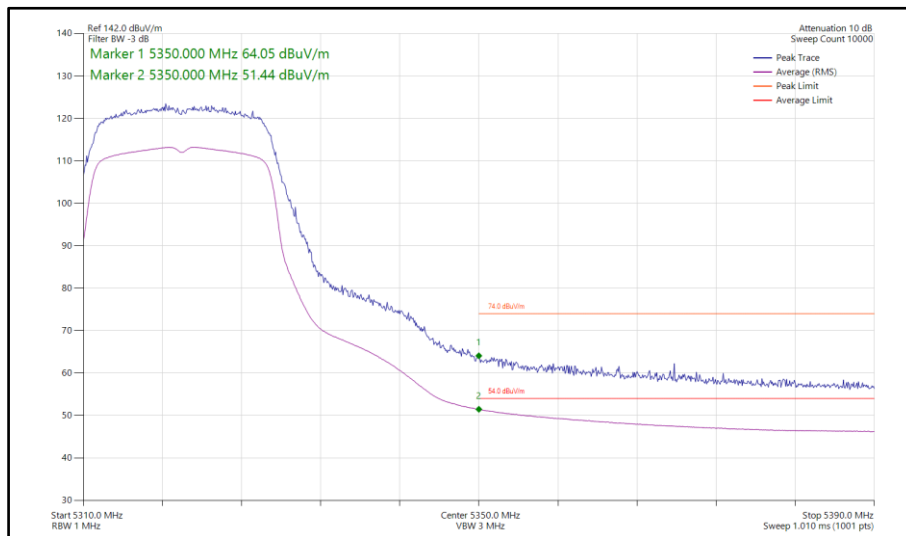
Figure 96 - 802.11ac VHT20, TxBF, Core 0-1 - 5320 MHz Band Edge Frequency 5350 MHz
