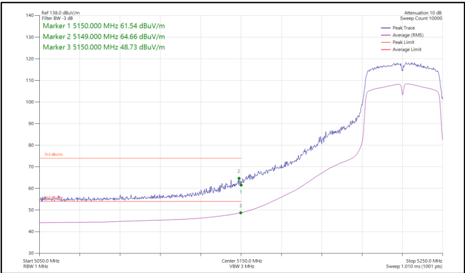
Figure 106 - 802.11n HT40, SISO, Core 0 - 5230 MHz Band Edge Frequency 5150 MHz
