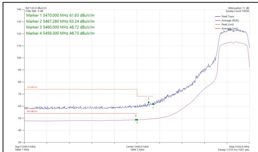
Figure 86 - 802.11n HT20, SDM, Core 0-1 - 5520 MHz Band Edge Frequency 5460 MHz
