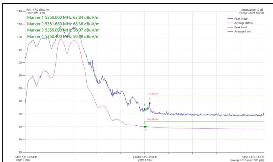
Figure 83 - 802.11ax HE20, RU106-54, SDM, Core 0-1 - 5320 MHz Band Edge Frequency 5350 MHz
