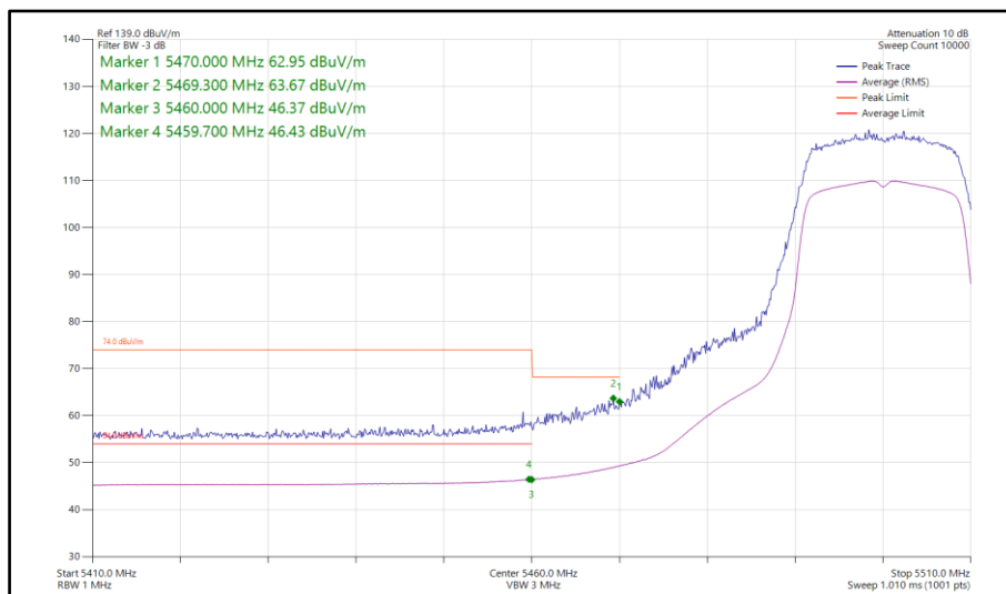
Figure 99 - 802.11ac VHT20, TxBF, Core 0-1 - 5500 MHz Band Edge Frequency 5460 MHz
