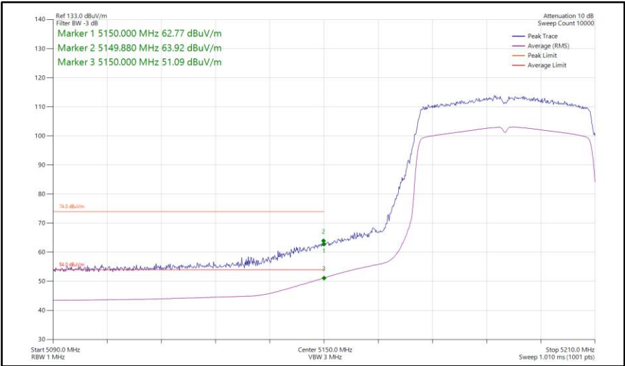
Figure 107 - 802.11ax HE40, SU, SISO, Core 0 - 5190 MHz Band Edge Frequency 5150 MHz
