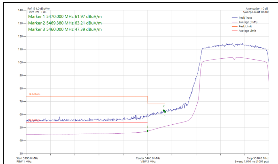
Figure 125 - 802.11ax HE40, SU, SISO, Core 0 - 5510 MHz Band Edge Frequency 5460 MHz
