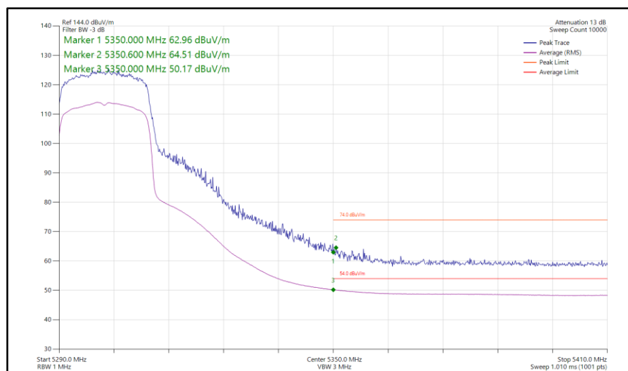
Figure 81 - 802.11ax HE20, SU, SDM, Core 0-1 - 5300 MHz Band Edge Frequency 5350 MHz
