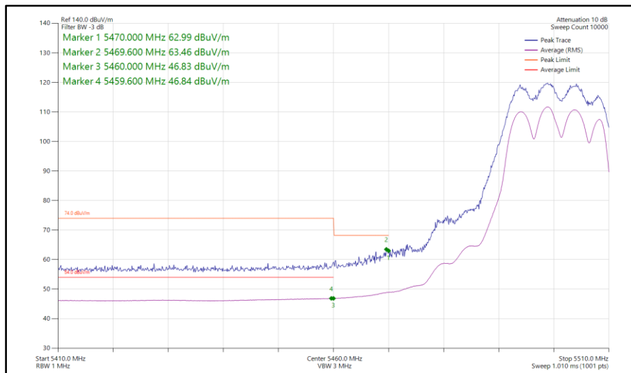
Figure 67 - 802.11n HT20, CDD, Core 0-1 - 5500 MHz Band Edge Frequency 5460 MHz
