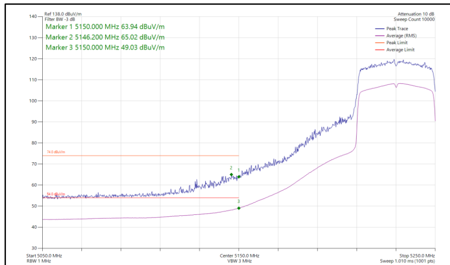
Figure 138 - 802.11ax HE40, SU, SISO, Core 1 - 5230 MHz Band Edge Frequency 5150 MHz
