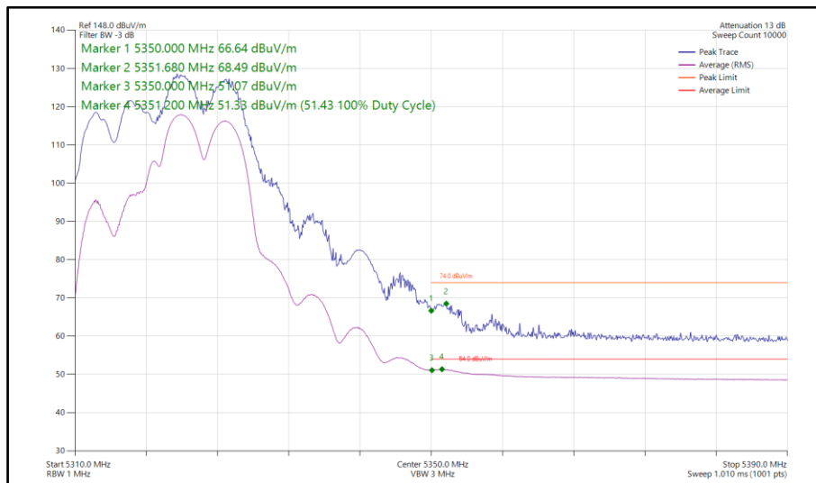
Figure 84 - 802.11be EHT20, RU106+26-83, SDM, Core 0-1 - 5320 MHz Band Edge Frequency 5350 MHz
