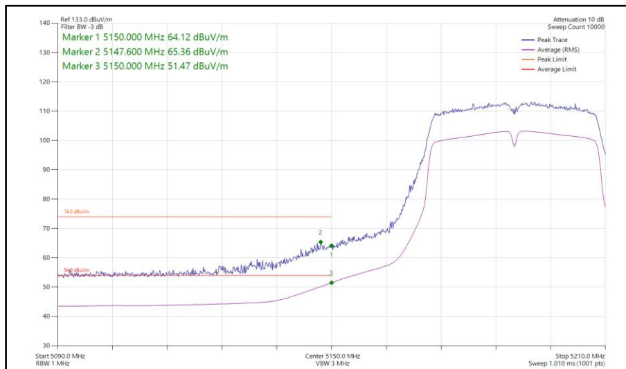
Figure 134 - 802.11n HT40, SISO, Core 1 - 5190 MHz Band Edge Frequency 5150 MHz
