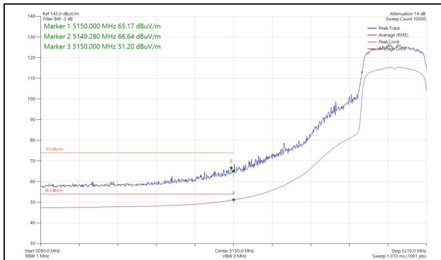
Figure 94 - 802.11ax HE20, SU, TxBF, Core 0-1 - 5200 MHz Band Edge Frequency 5150 MHz
