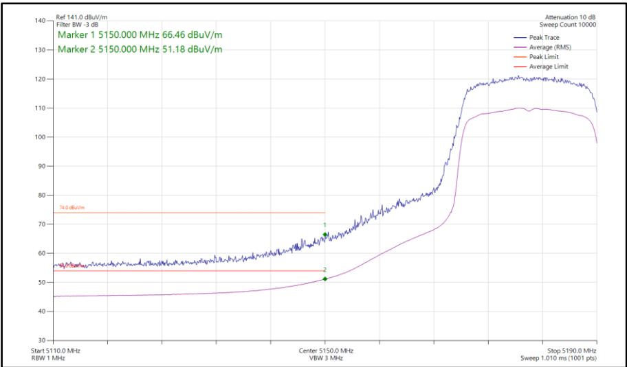
Figure 75 - 802.11ax HE20, SU, SDM, Core 0-1 - 5180 MHz Band Edge Frequency 5150 MHz
