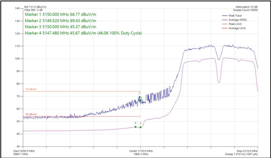
Figure 132 - 802.11a a40, SISO, Core 1 - 5190 MHz Band Edge Frequency 5150 MHz
