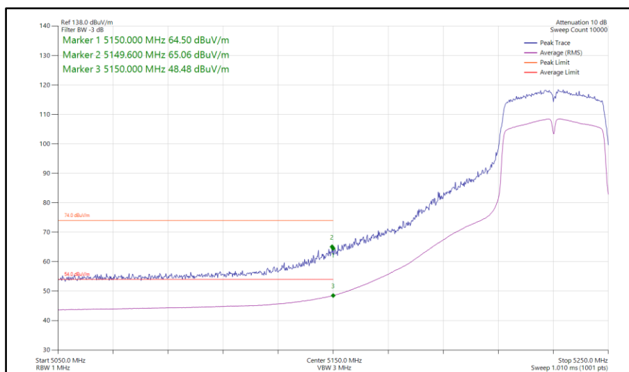
Figure 135 - 802.11n HT40, SISO, Core 1 - 5230 MHz Band Edge Frequency 5150 MHz
