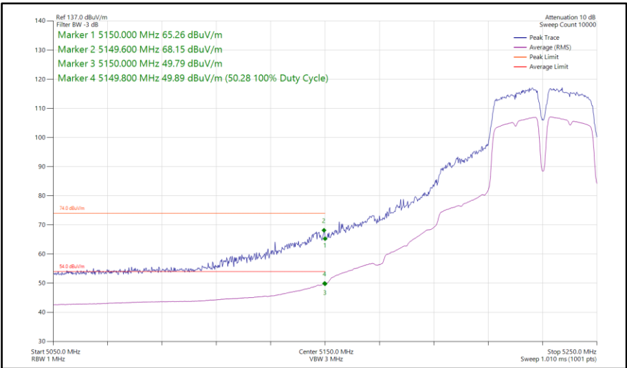
Figure 133 - 802.11a a40, SISO, Core 1 - 5230 MHz Band Edge Frequency 5150 MHz
