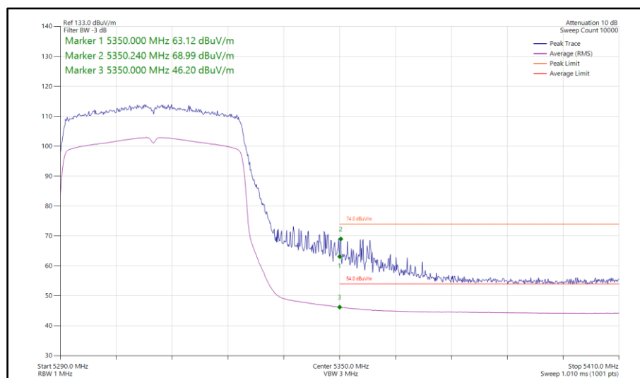
Figure 116 - 802.11ax HE40, SU, SISO, Core 0 - 5310 MHz Band Edge Frequency 5350 MHz
