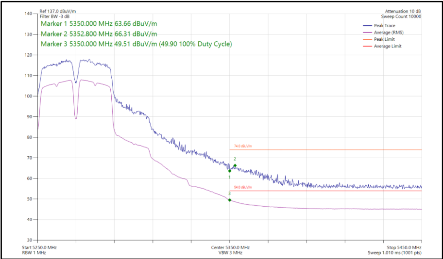
Figure 111 - 802.11a a40, SISO, Core 0 - 5270 MHz Band Edge Frequency 5350 MHz
