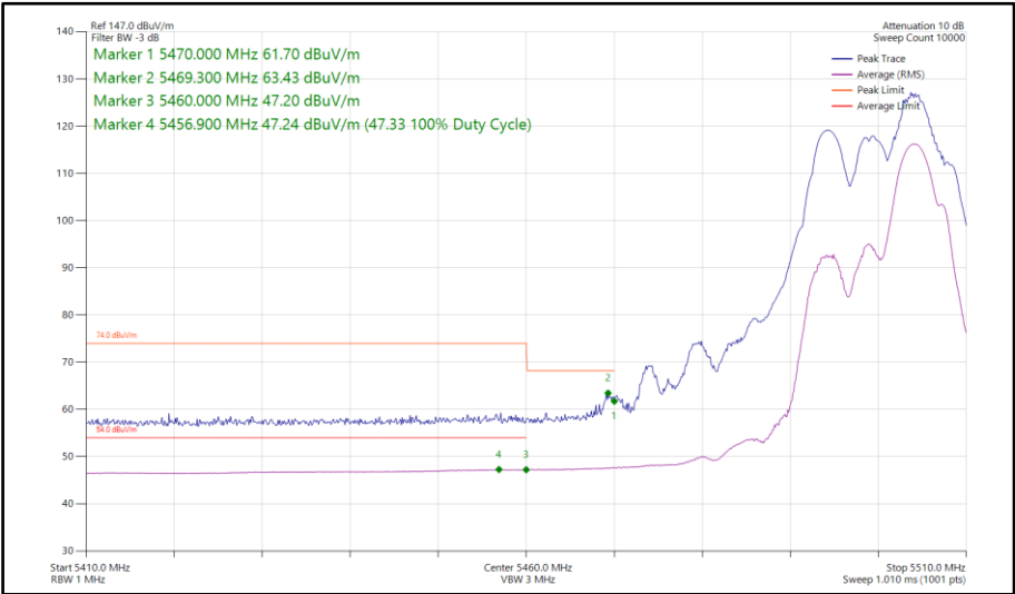
Figure 90 - 802.11be EHT20, RU52+26-72, SDM, Core 0-1 - 5500 MHz Band Edge Frequency 5460 MHz
