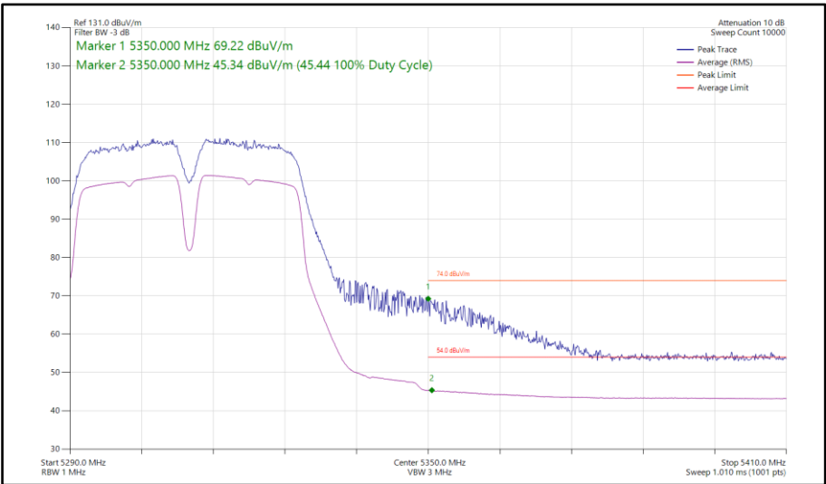
Figure 112 - 802.11a a40, SISO, Core 0 - 5310 MHz Band Edge Frequency 5350 MHz
