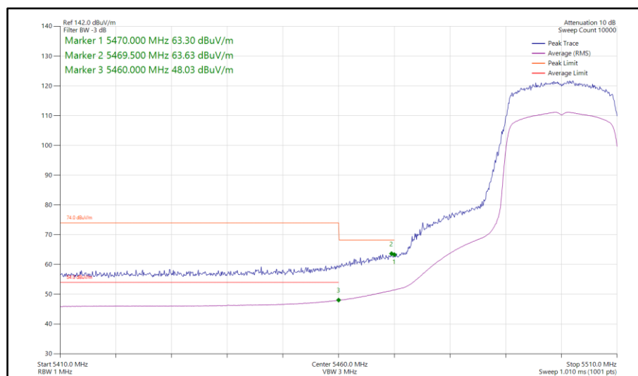
Figure 101 - 802.11ax HE20, SU, TxBF, Core 0-1 - 5500 MHz Band Edge Frequency 5460 MHz
