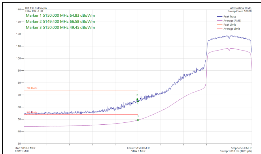
Figure 109 - 802.11ax HE40, SU, SISO, Core 0 - 5230 MHz Band Edge Frequency 5150 MHz
