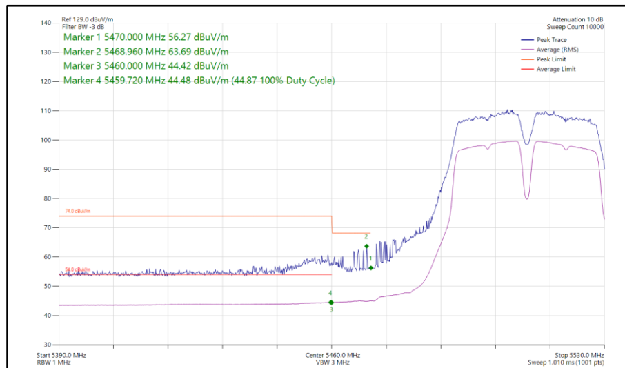
Figure 119 - 802.11a a40, SISO, Core 0 - 5510 MHz Band Edge Frequency 5460 MHz
