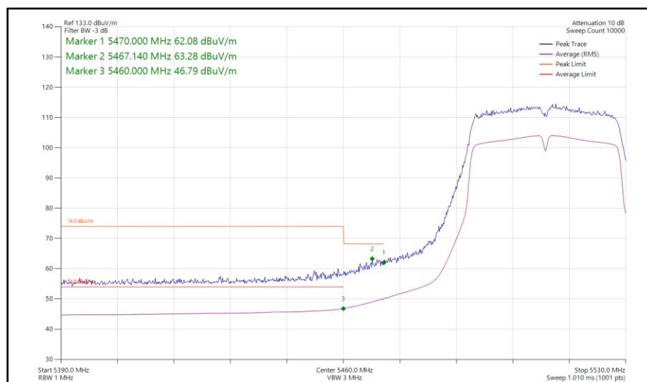
Figure 122 - 802.11n HT40, SISO, Core 0 - 5510 MHz Band Edge Frequency 5460 MHz
