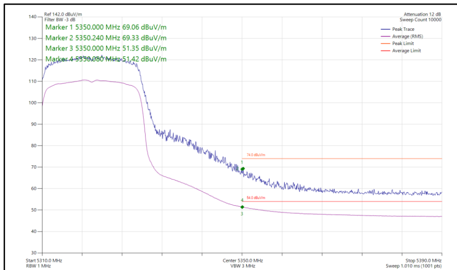
Figure 82 - 802.11ax HE20, SU, SDM, Core 0-1 - 5320 MHz Band Edge Frequency 5350 MHz
