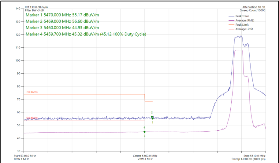
Figure 131 - 802.11be EHT40, RU106+26-82, SISO, Core 0 - 5590 MHz Band Edge Frequency 5460 MHz
