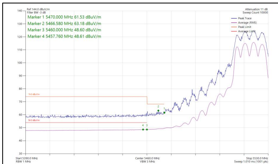
Figure 68 - 802.11n HT20, CDD, Core 0-1 - 5520 MHz Band Edge Frequency 5460 MHz
