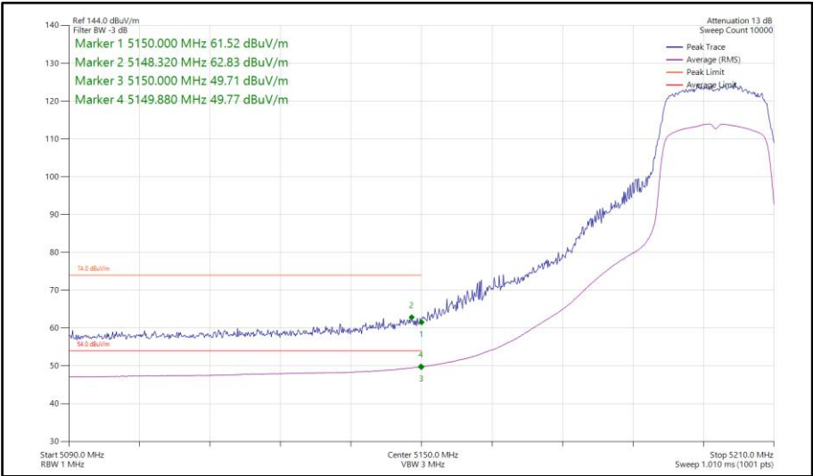
Figure 74 - 802.11n HT20, SDM, Core 0-1 - 5200 MHz Band Edge Frequency 5150 MHz
