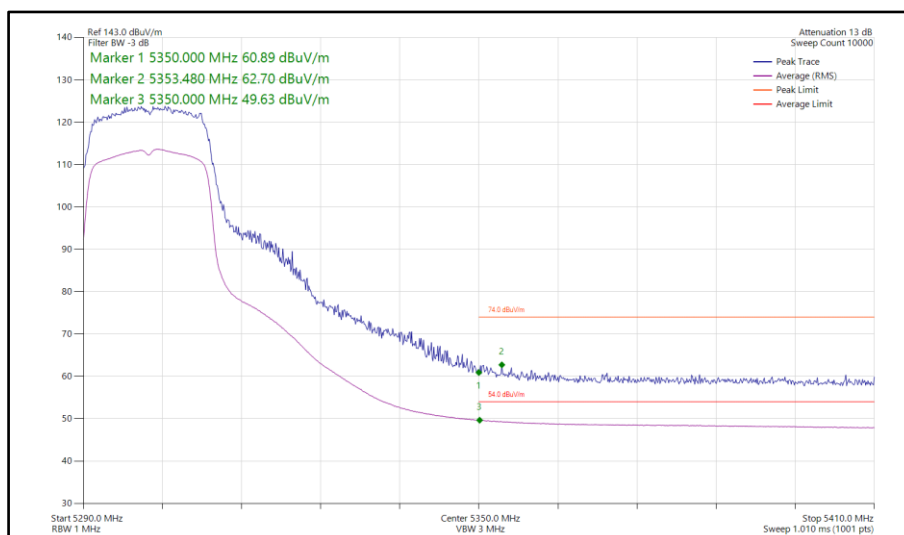
Figure 79 - 802.11n HT20, SDM, Core 0-1 - 5300 MHz Band Edge Frequency 5350 MHz
