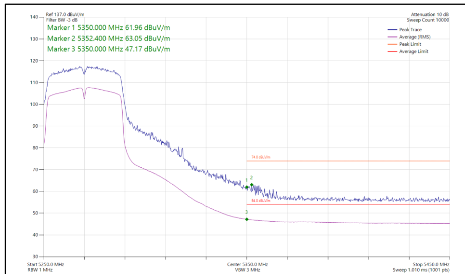
Figure 113 - 802.11n HT40, SISO, Core 0 - 5270 MHz Band Edge Frequency 5350 MHz
