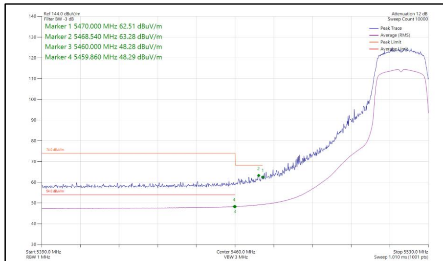
Figure 100 - 802.11ac VHT20, TxBF, Core 0-1 - 5520 MHz Band Edge Frequency 5460 MHz
