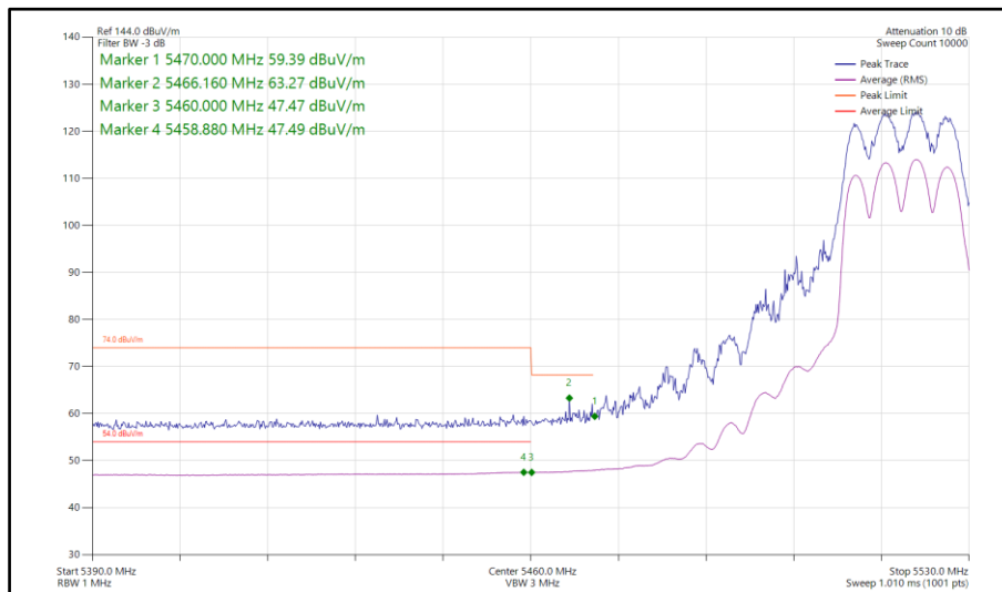
Figure 71 - 802.11ax HE20, SU, CDD, Core 0-1 - 5520 MHz Band Edge Frequency 5460 MHz
