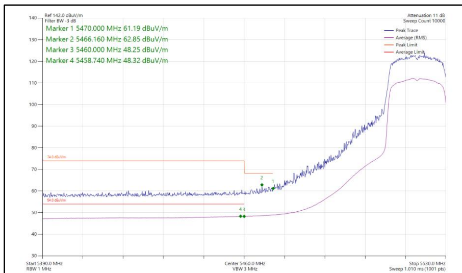
Figure 89 - 802.11ax HE20, SU, SDM, Core 0-1 - 5520 MHz Band Edge Frequency 5460 MHz
