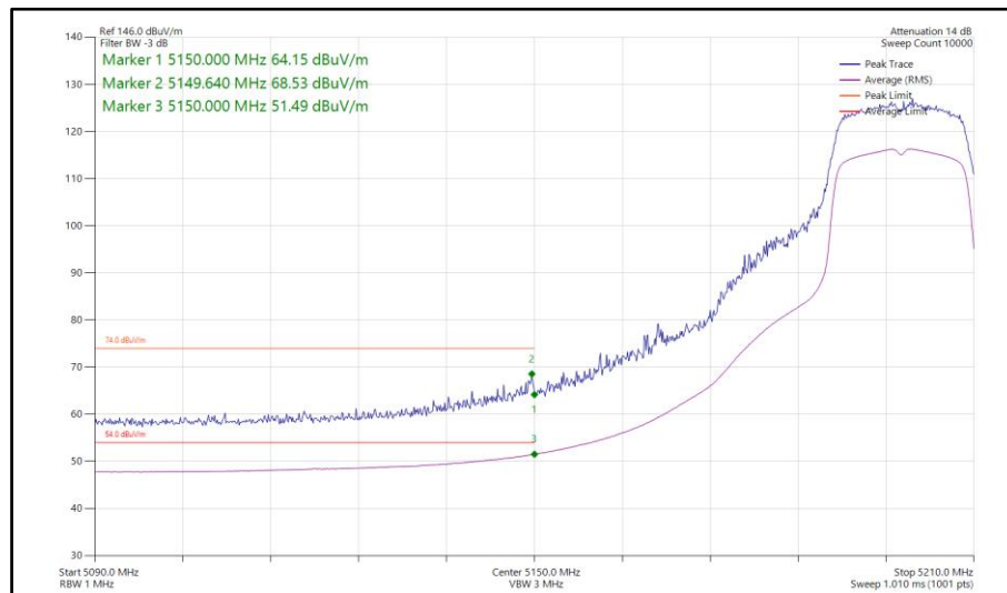
Figure 92 - 802.11ac VHT20, TxBF, Core 0-1 - 5200 MHz Band Edge Frequency 5150 MHz
