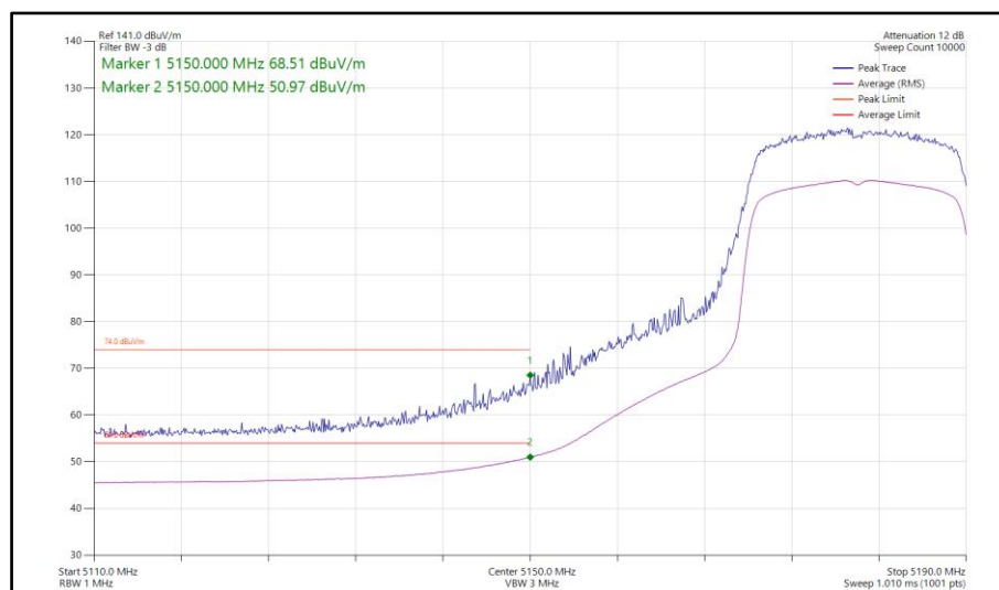
Figure 93 - 802.11ax HE20, SU, TxBF, Core 0-1 - 5180 MHz Band Edge Frequency 5150 MHz
