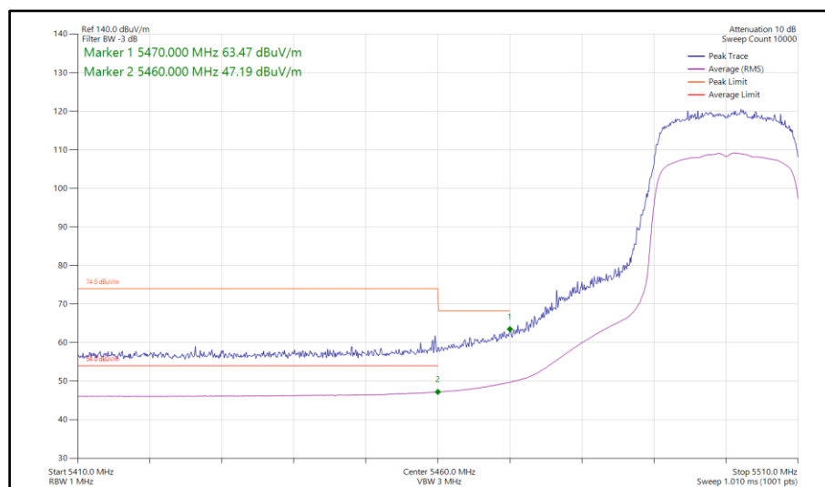
Figure 87 - 802.11ax HE20, SU, SDM, Core 0-1 - 5500 MHz Band Edge Frequency 5460 MHz
