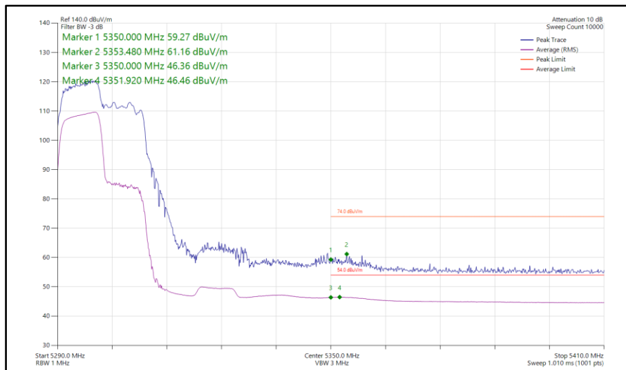
Figure 117 - 802.11ax HE40, RU106-53, SISO, Core 0 - 5310 MHz Band Edge Frequency 5350 MHz
