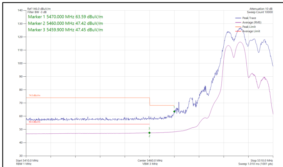
Figure 88 - 802.11ax HE20, RU106-53, SDM, Core 0-1 - 5500 MHz Band Edge Frequency 5460 MHz
