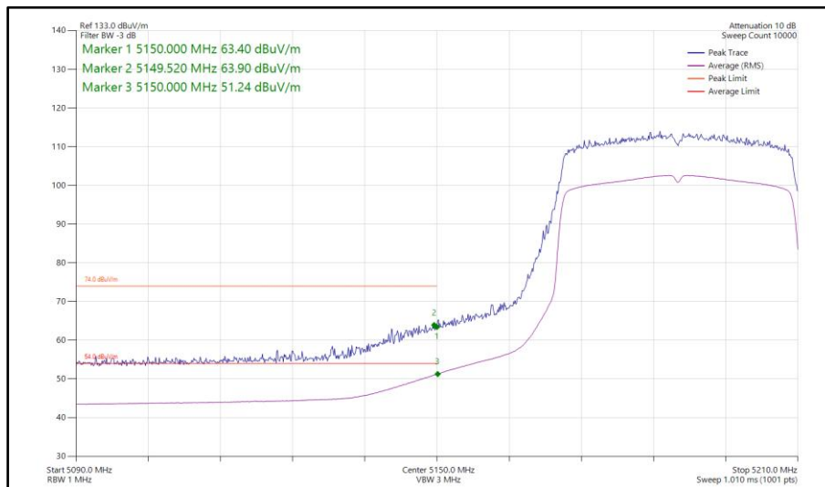
Figure 136 - 802.11ax HE40, SU, SISO, Core 1 - 5190 MHz Band Edge Frequency 5150 MHz
