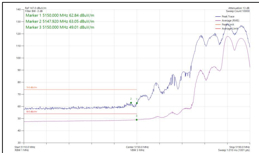
Figure 76 - 802.11ax HE20, RU106-54, SDM, Core 0-1 - 5180 MHz Band Edge Frequency 5150 MHz
