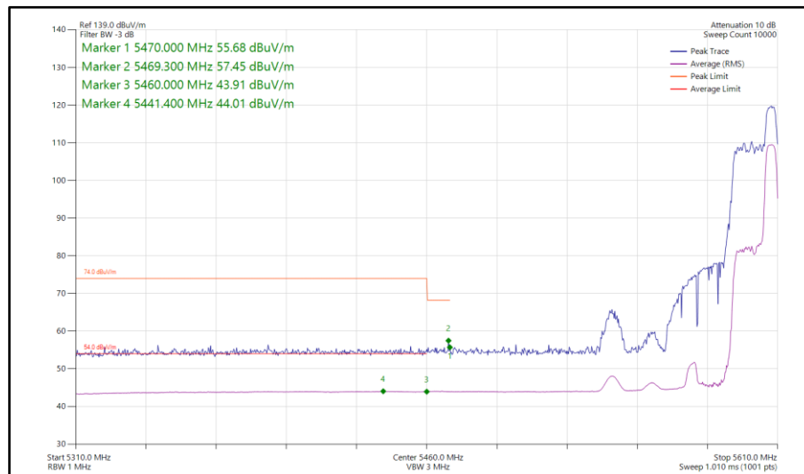
Figure 129 - 802.11ax HE40, RU52-44, SISO, Core 0 - 5590 MHz Band Edge Frequency 5460 MHz
