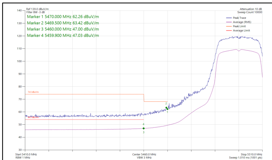
Figure 85 - 802.11n HT20, SDM, Core 0-1 - 5500 MHz Band Edge Frequency 5460 MHz
