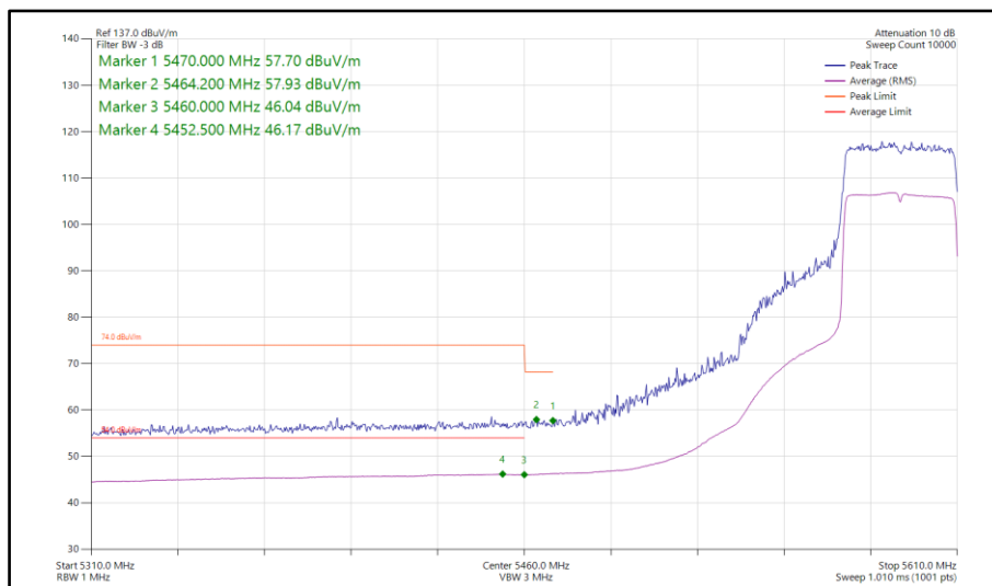
Figure 128 - 802.11ax HE40, SU, SISO, Core 0 - 5590 MHz Band Edge Frequency 5460 MHz
