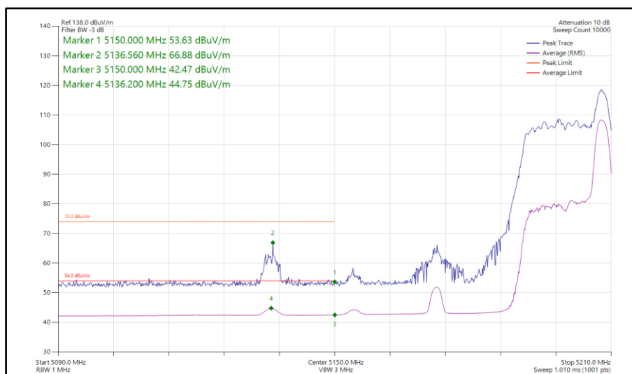
Figure 137 - 802.11ax HE40, RU26-17, SISO, Core 1 - 5190 MHz Band Edge Frequency 5150 MHz
