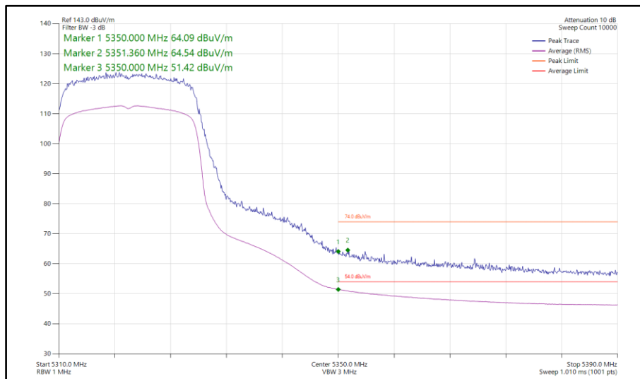
Figure 98 - 802.11ax HE20, SU, TxBF, Core 0-1 - 5320 MHz Band Edge Frequency 5350 MHz
