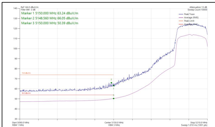
Figure 77 - 802.11ax HE20, SU, SDM, Core 0-1 - 5200 MHz Band Edge Frequency 5150 MHz
