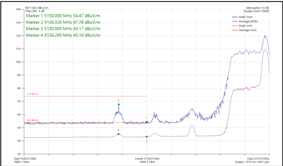
Figure 108 - 802.11ax HE40, RU26-17, SISO, Core 0 - 5190 MHz Band Edge Frequency 5150 MHz
