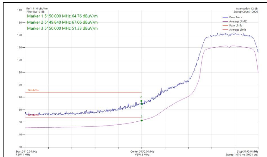
Figure 91 - 802.11ac VHT20, TxBF, Core 0-1 - 5180 MHz Band Edge Frequency 5150 MHz
