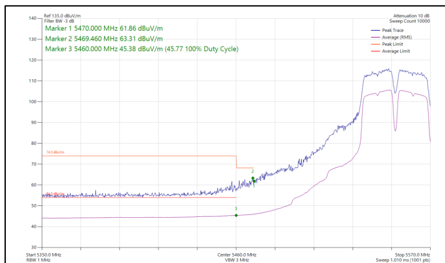
Figure 120 - 802.11a a40, SISO, Core 0 - 5550 MHz Band Edge Frequency 5460 MHz
