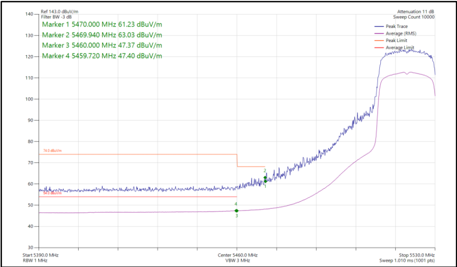
Figure 102 - 802.11ax HE20, SU, TxBF, Core 0-1 - 5520 MHz Band Edge Frequency 5460 MHz
