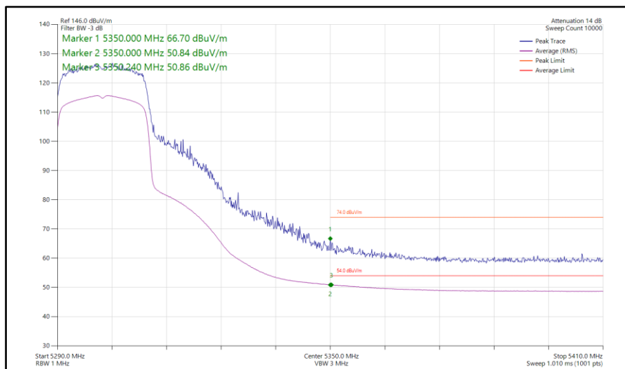
Figure 97 - 802.11ax HE20, SU, TxBF, Core 0-1 - 5300 MHz Band Edge Frequency 5350 MHz
