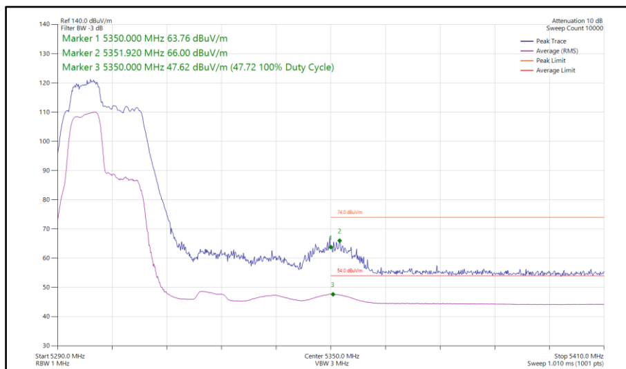
Figure 118 - 802.11be EHT40, RU52+26-70, SISO, Core 0 - 5310 MHz Band Edge Frequency 5350 MHz
