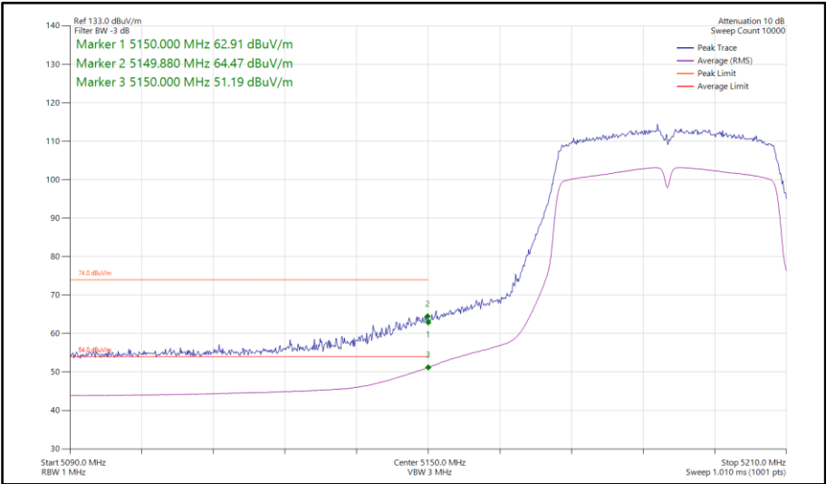
Figure 105 - 802.11n HT40, SISO, Core 0 - 5190 MHz Band Edge Frequency 5150 MHz
