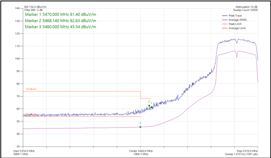
Figure 123 - 802.11n HT40, SISO, Core 0 - 5550 MHz Band Edge Frequency 5460 MHz
