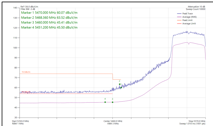
Figure 127 - 802.11ax HE40, SU, SISO, Core 0 - 5550 MHz Band Edge Frequency 5460 MHz
