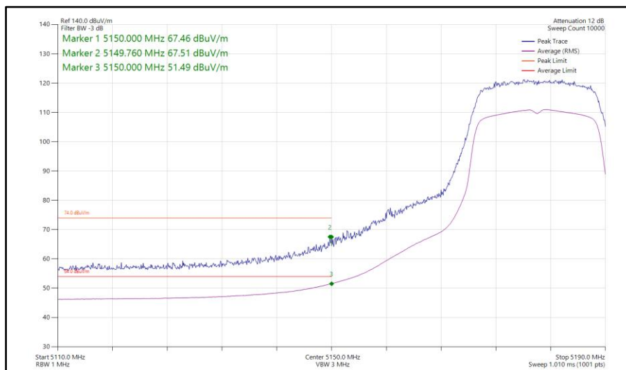
Figure 73 - 802.11n HT20, SDM, Core 0-1 - 5180 MHz Band Edge Frequency 5150 MHz
