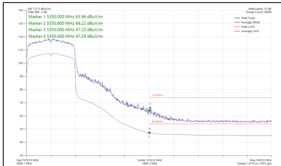
Figure 115 - 802.11ax HE40, SU, SISO, Core 0 - 5270 MHz Band Edge Frequency 5350 MHz
