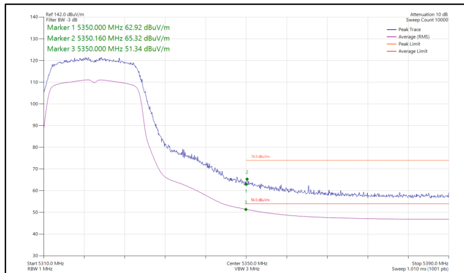
Figure 80 - 802.11n HT20, SDM, Core 0-1 - 5320 MHz Band Edge Frequency 5350 MHz
