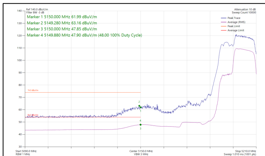
Figure 139 - 802.11be EHT40, RU106+26-85, SISO, Core 1 - 5190 MHz Band Edge Frequency 5150 MHz
