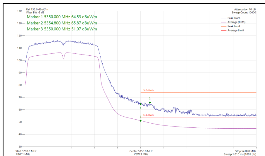
Figure 114 - 802.11n HT40, SISO, Core 0 - 5310 MHz Band Edge Frequency 5350 MHz
