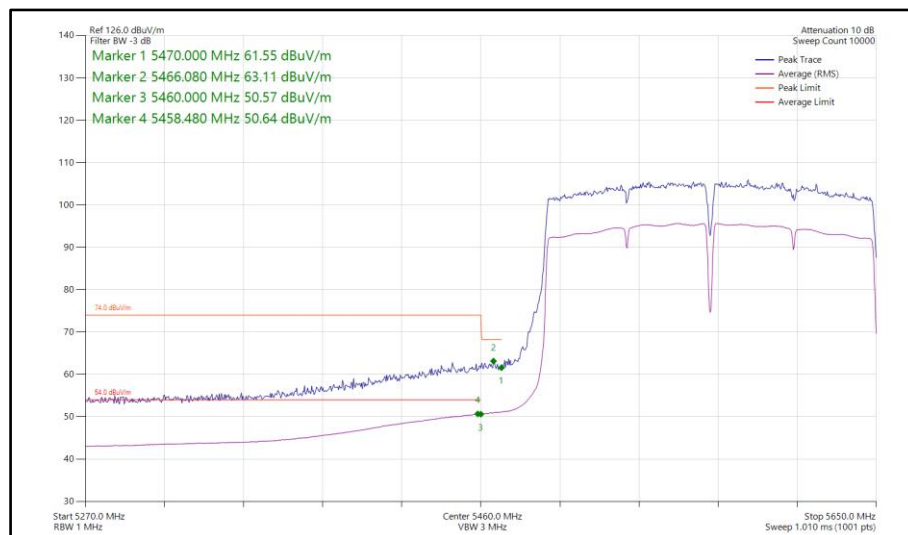
Figure 350 - 802.11ac VHT160, TxBF, Core 0-1 - 5570 MHz Band Edge Frequency 5460 MHz
