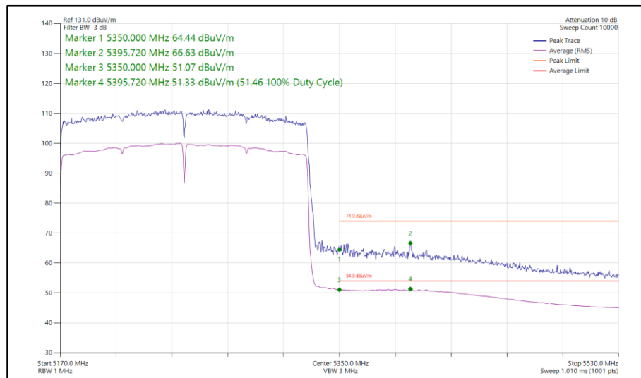
Figure 349 - 802.11ax HE160, SU, TxBF, Core 0-1 - 5250 MHz Band Edge Frequency 5350 MHz
