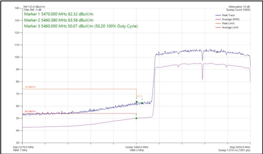
Figure 351 - 802.11ax HE160, SU, TxBF, Core 0-1 - 5570 MHz Band Edge Frequency 5460 MHz
