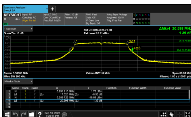
Figure 352 - 802.11n HT20 Minimum 99% OBW
