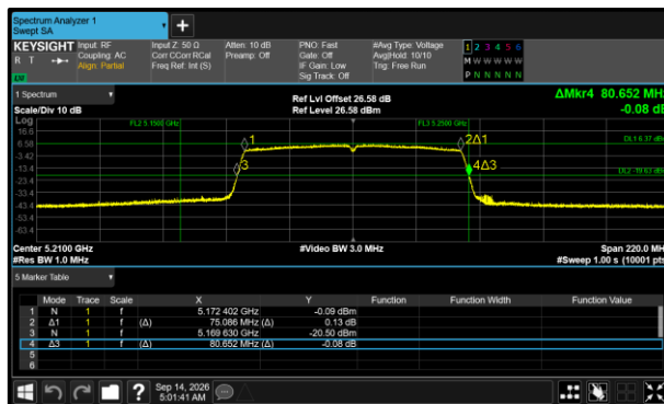
Figure 356 - 802.11ac VHT80 Minimum 99% OBW
