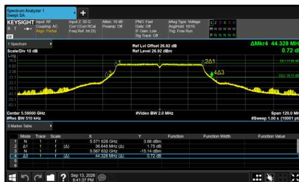
Figure 355 - 802.11n HT40 Maximum 99% OBW
