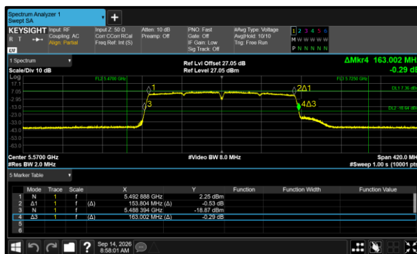
Figure 358 - 802.11ac VHT160 Minimum 99% OBW
