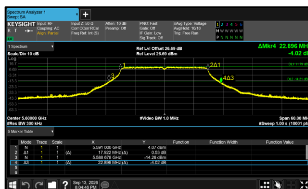
Figure 353 - 802.11n HT20 Maximum 99% OBW
