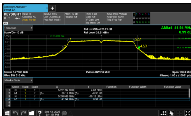
Figure 354 - 802.11n HT40 Minimum 99% OBW
