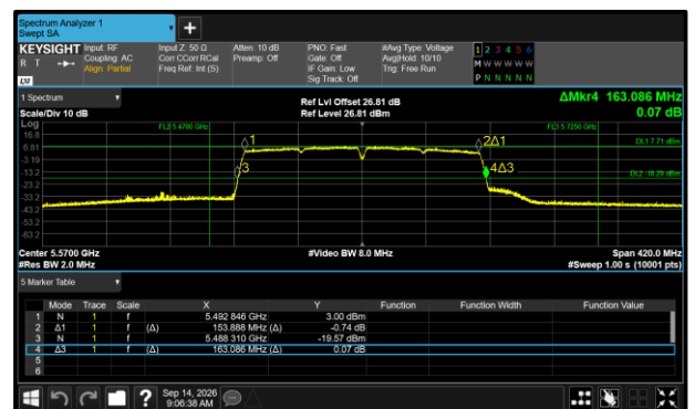
Figure 359 - 802.11ac VHT160 Maximum 99% OBW
