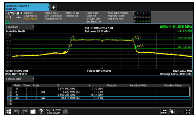
Figure 357 - 802.11ac VHT80 Maximum 99% OBW
