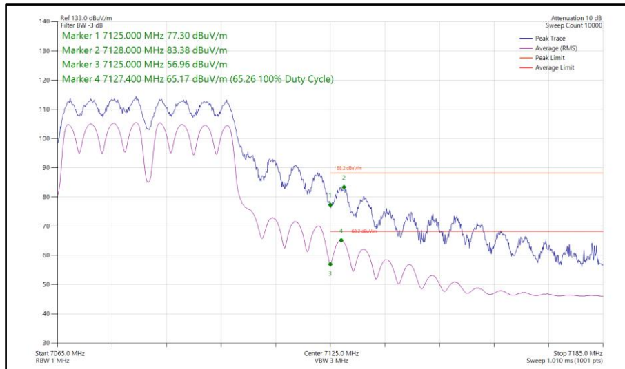
Figure 362 - 802.11a a40, CDD, Core 0-1 - 7085 MHz Band Edge Frequency 7125 MHz
