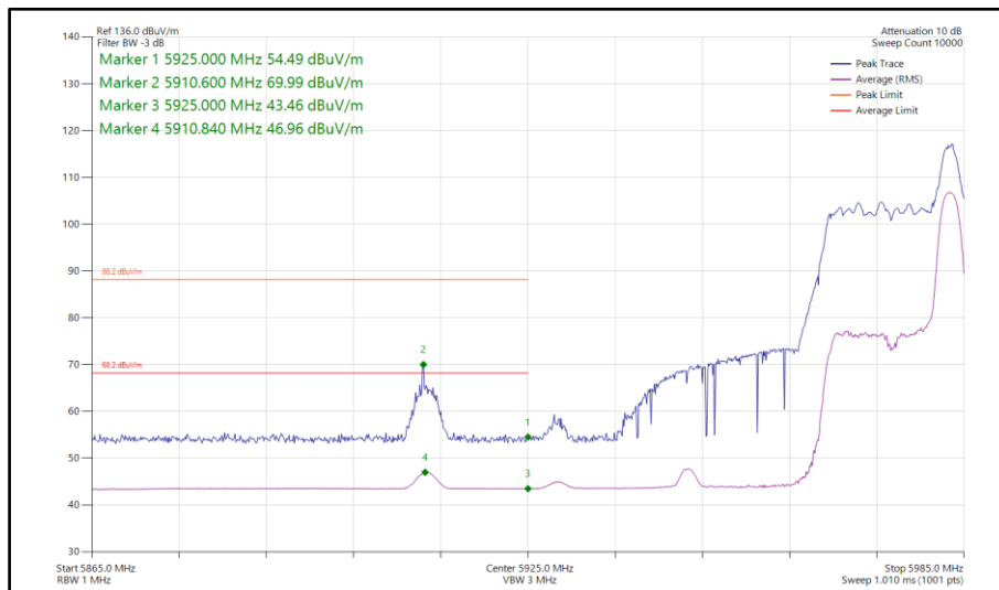
Figure 349 - 802.11ax HE40, RU26-17, SISO, Core 1 - 5965 MHz Band Edge Frequency 5925 MHz
