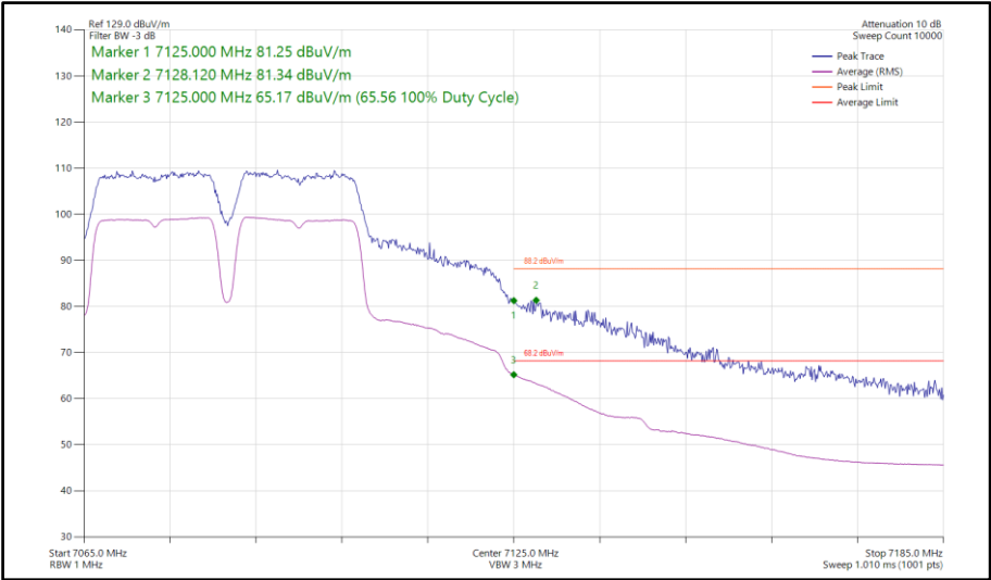
Figure 342 - 802.11a a40, SISO, Core 0 - 7085 MHz Band Edge Frequency 7125 MHz
