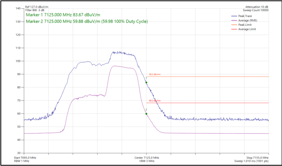
Figure 312 - 802.11be EHT20, RU52+26-72, SISO, Core 1 - 7115 MHz Band Edge Frequency 7125 MHz
