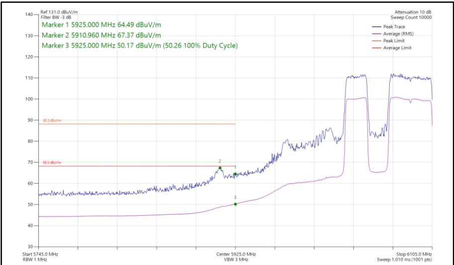
Figure 381 - 802.11be EHT80, RU484+242-91, SISO, Core 0 - 6065 MHz Band Edge Frequency 5925 MHz
