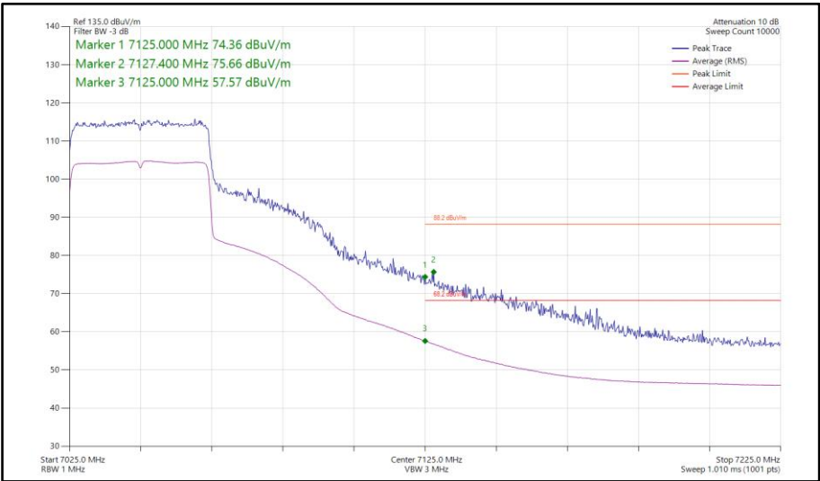
Figure 353 - 802.11ax HE40, SU, SISO, Core 1 - 7045 MHz Band Edge Frequency 7125 MHz
