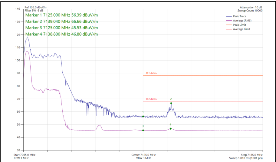
Figure 355 - 802.11ax HE40, RU26-0, SISO, Core 1 - 7085 MHz Band Edge Frequency 7125 MHz
