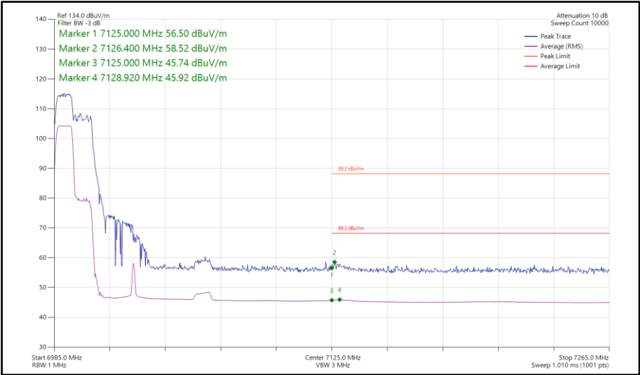
Figure 384 - 802.11ax HE80, RU106-53, SISO, Core 0 - 7025 MHz Band Edge Frequency 7125 MHz
