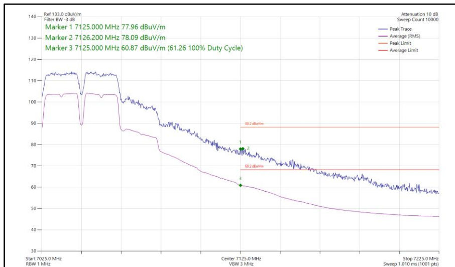
Figure 351 - 802.11a a40, SISO, Core 1 - 7045 MHz Band Edge Frequency 7125 MHz
