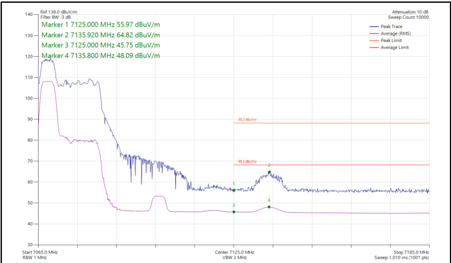
Figure 345 - 802.11ax HE40, RU52-37, SISO, Core 0 - 7085 MHz Band Edge Frequency 7125 MHz
