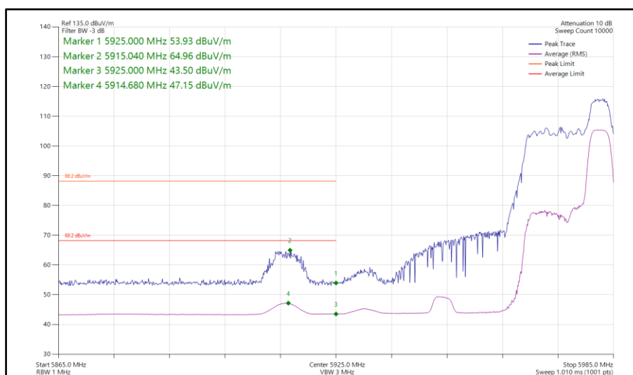
Figure 339 - 802.11ax HE40, RU52-44, SISO, Core 0 - 5965 MHz Band Edge Frequency 5925 MHz
