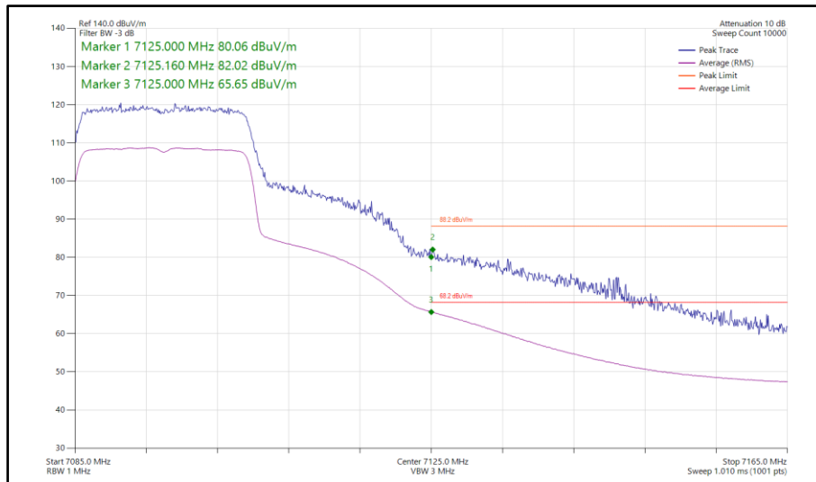
Figure 328 - 802.11ax HE20, SU, SDM, Core 0-1 - 7095 MHz Band Edge Frequency 7125 MHz
