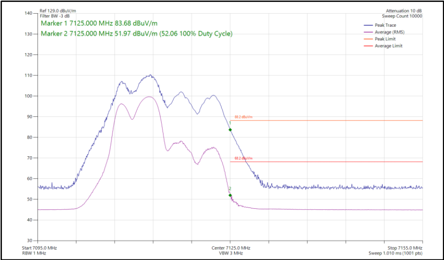
Figure 324 - 802.11be EHT20, RU52+26-70, CDD, Core 0-1 - 7115 MHz Band Edge Frequency 7125 MHz
