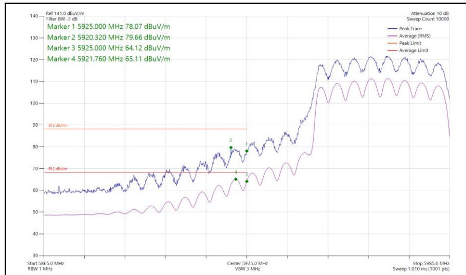
Figure 358 - 802.11ax HE40, SU, CDD, Core 0-1 - 5965 MHz Band Edge Frequency 5925 MHz
