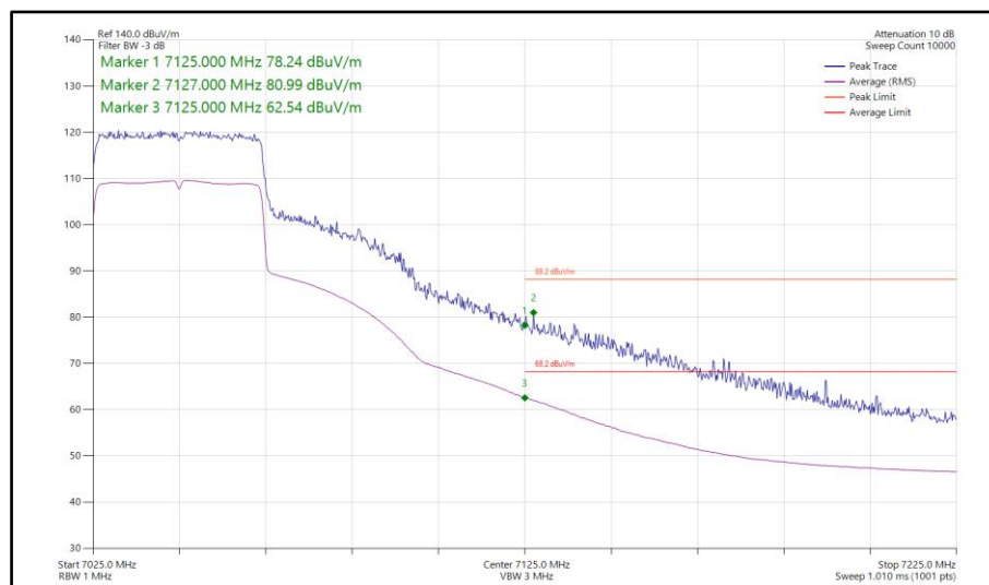
Figure 375 - 802.11ax HE40, SU, TxBF, Core 0-1 - 7045 MHz Band Edge Frequency 7125 MHz
