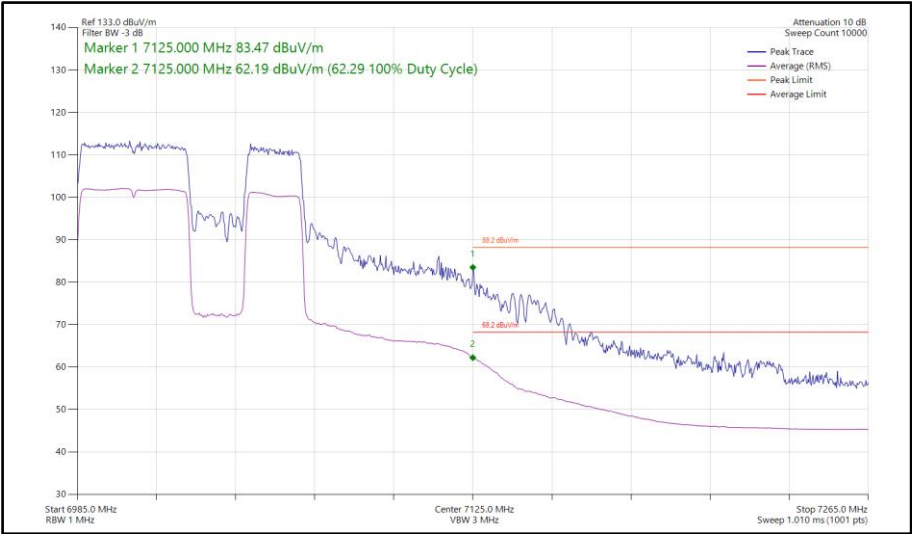
Figure 386 - 802.11be EHT80, RU484+242-92, SISO, Core 0 - 7025 MHz Band Edge Frequency 7125 MHz
