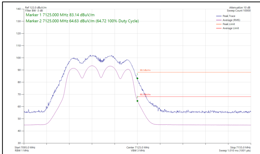
Figure 318 - 802.11a, CDD, Core 0-1 - 7115 MHz Band Edge Frequency 7125 MHz
