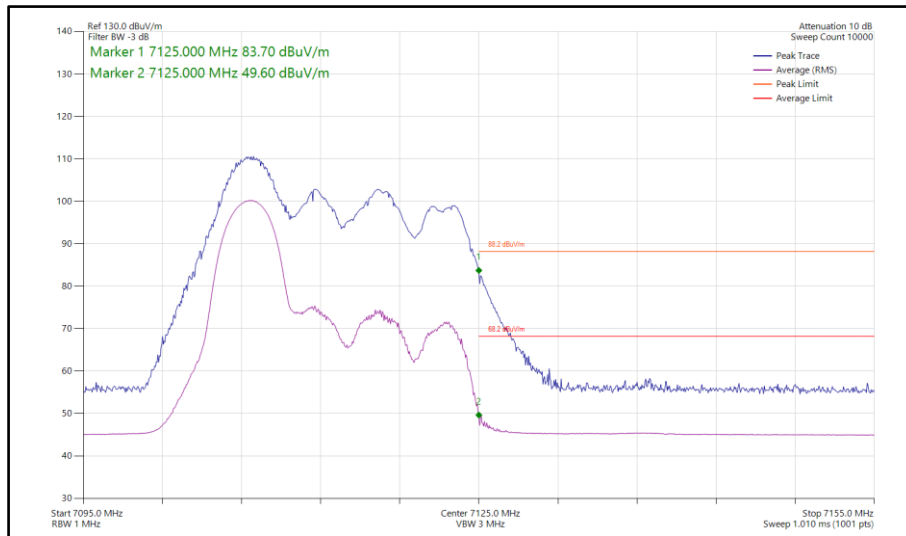
Figure 322 - 802.11ax HE20, RU52-37, CDD, Core 0-1 - 7115 MHz Band Edge Frequency 7125 MHz
