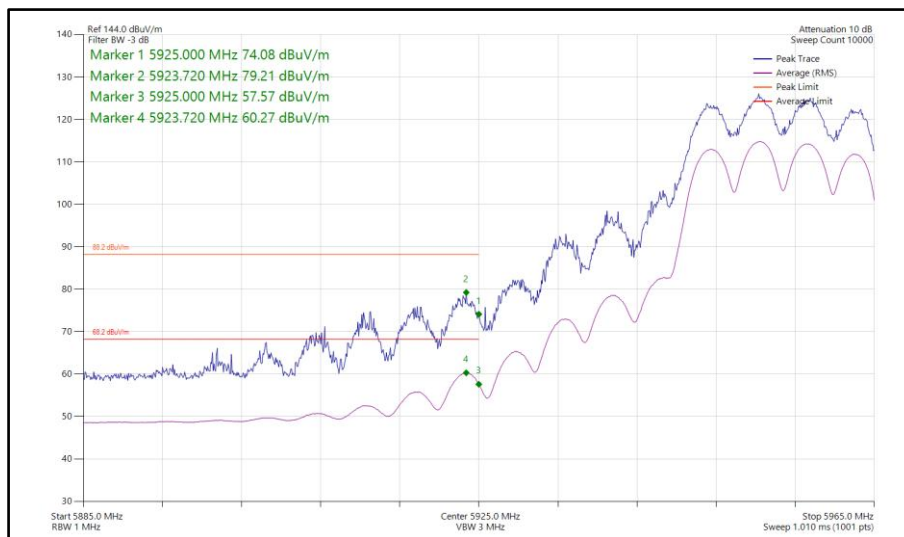
Figure 314 - 802.11ax HE20, SU, CDD, Core 0-1 - 5955 MHz Band Edge Frequency 5925 MHz
