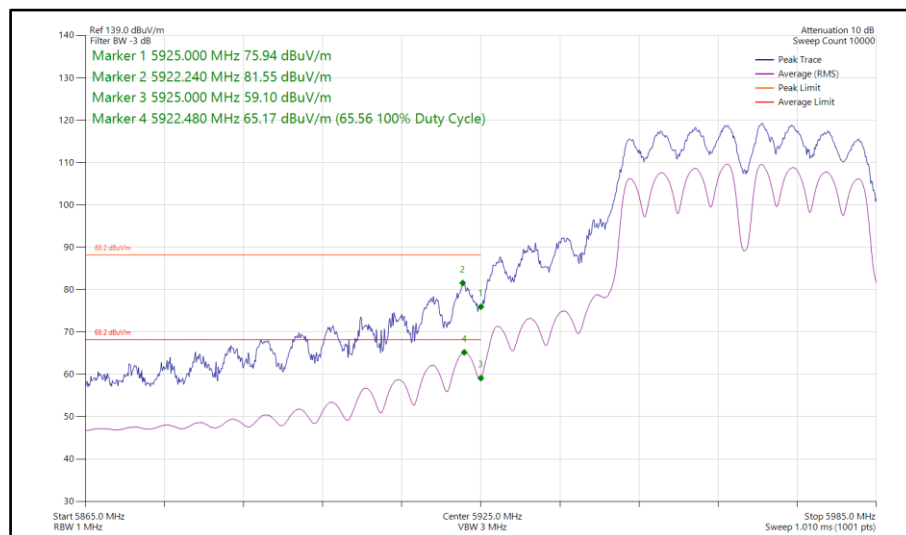
Figure 357 - 802.11a a40, CDD, Core 0-1 - 5965 MHz Band Edge Frequency 5925 MHz
