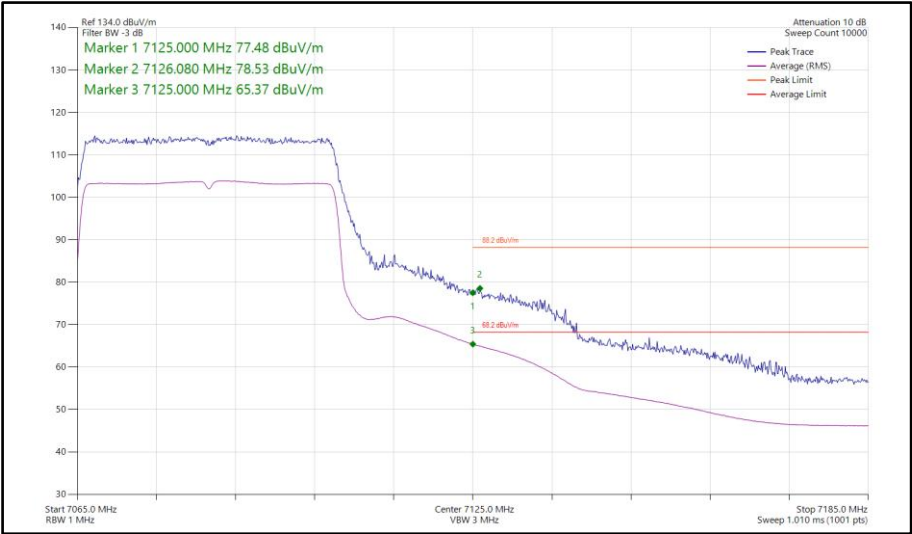
Figure 344 - 802.11ax HE40, SU, SISO, Core 0 - 7085 MHz Band Edge Frequency 7125 MHz
