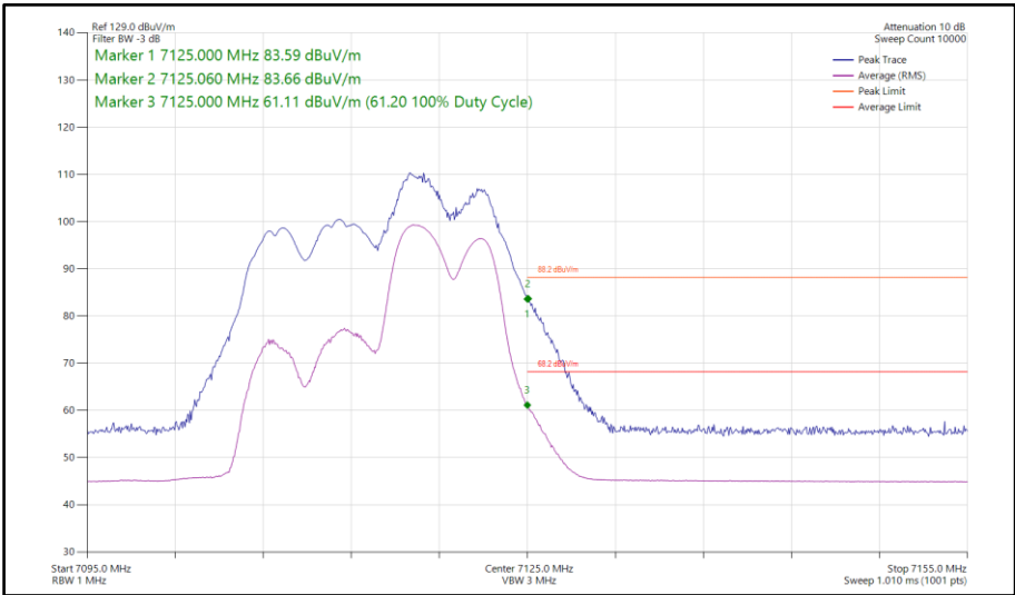
Figure 333 - 802.11be EHT20, RU52+26-72, SDM, Core 0-1 - 7115 MHz Band Edge Frequency 7125 MHz
