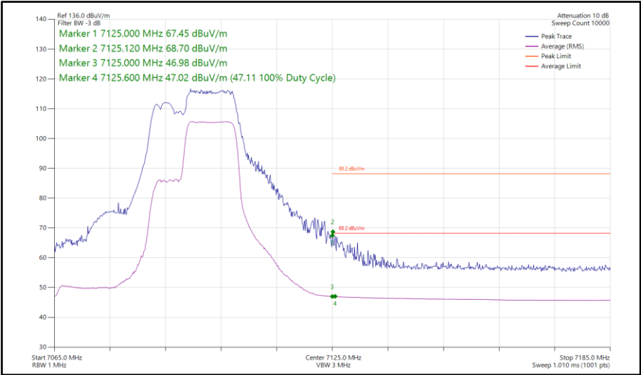
Figure 356 - 802.11be EHT40, RU106+26-85, SISO, Core 1 - 7085 MHz Band Edge Frequency 7125 MHz
