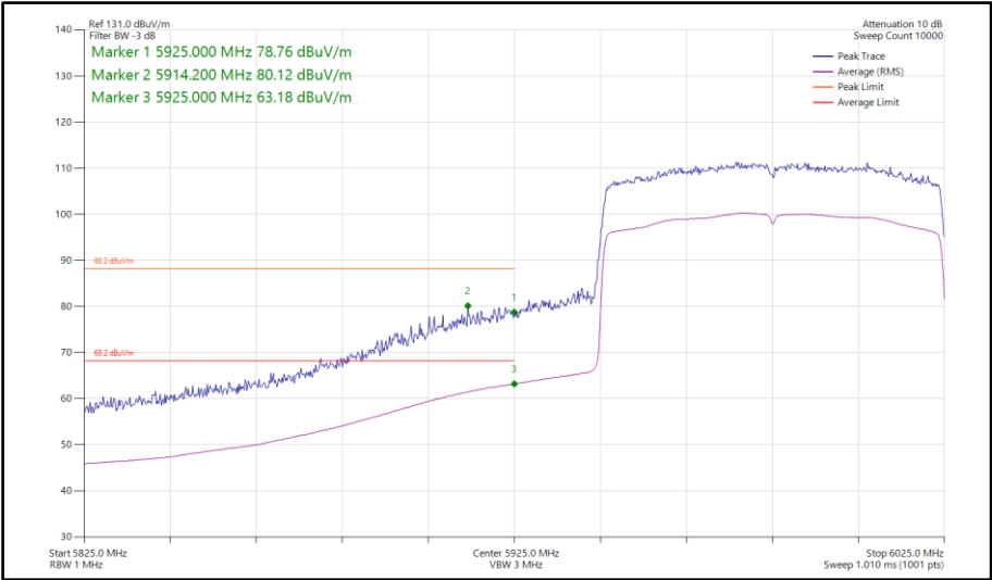
Figure 378 - 802.11ax HE80, SU, SISO, Core 0 - 5985 MHz Band Edge Frequency 5925 MHz
