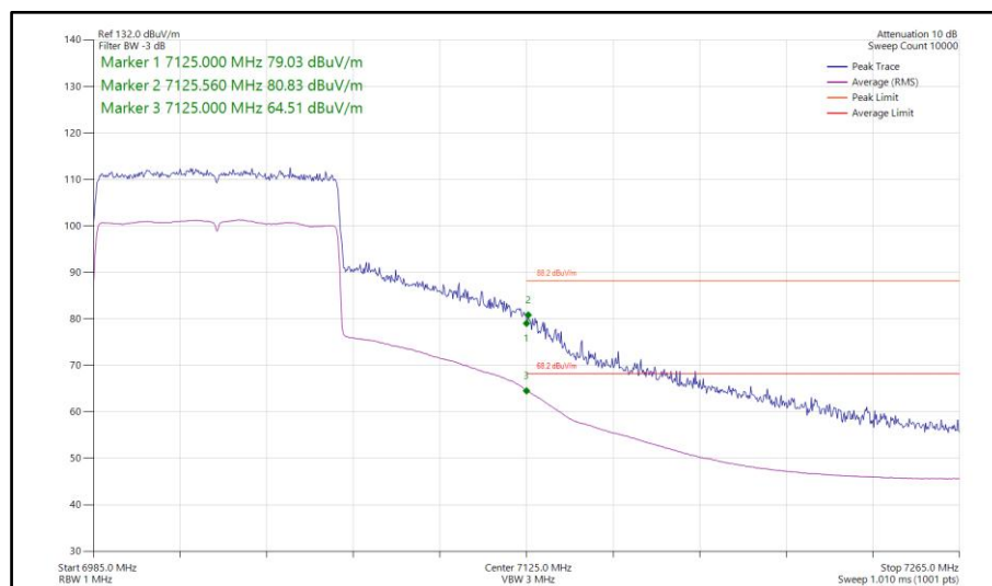
Figure 383 - 802.11ax HE80, SU, SISO, Core 0 - 7025 MHz Band Edge Frequency 7125 MHz
