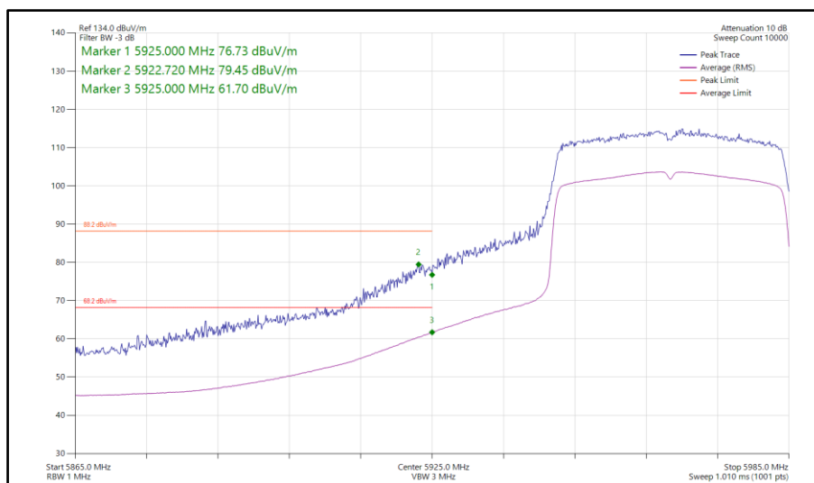
Figure 338 - 802.11ax HE40, SU, SISO, Core 0 - 5965 MHz Band Edge Frequency 5925 MHz
