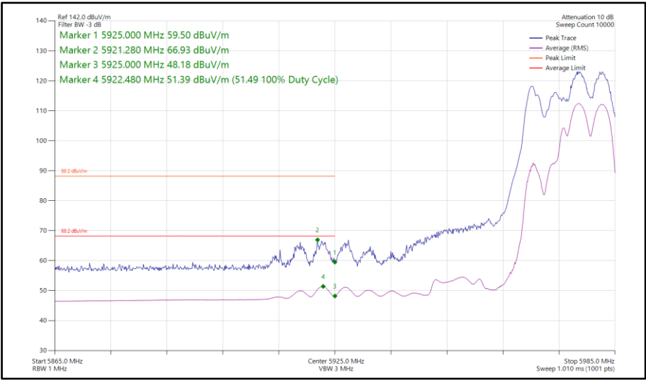
Figure 369 - 802.11be EHT40, RU106+26-85, SDM, Core 0-1 - 5965 MHz Band Edge Frequency 5925 MHz
