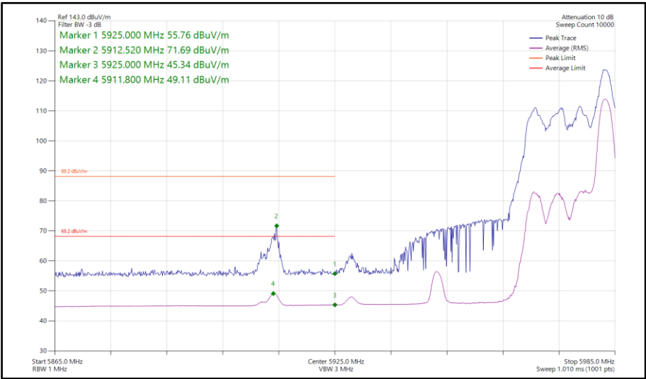
Figure 368 - 802.11ax HE40, RU26-17, SDM, Core 0-1 - 5965 MHz Band Edge Frequency 5925 MHz
