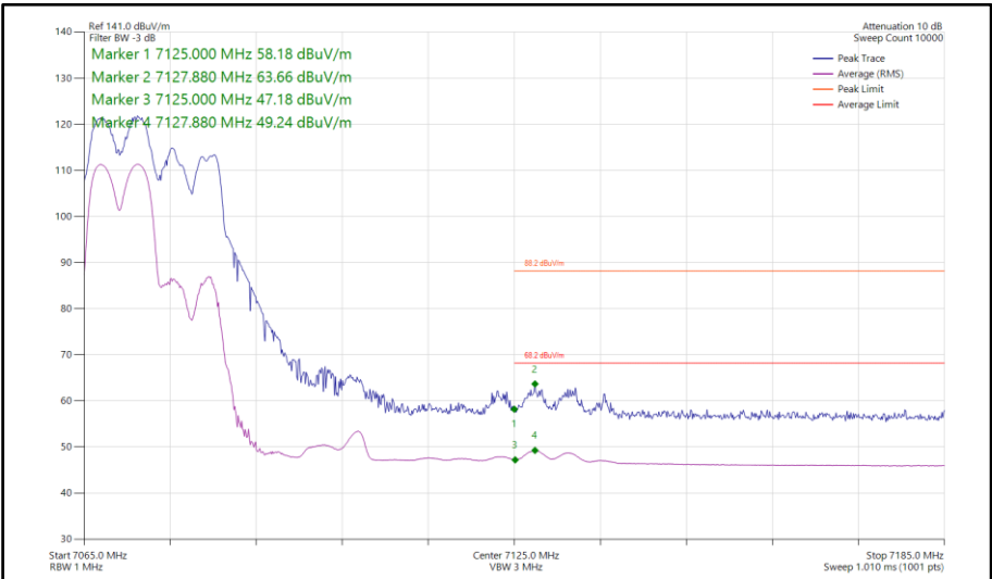
Figure 365 - 802.11ax HE40, RU106-53, CDD, Core 0-1 - 7085 MHz Band Edge Frequency 7125 MHz
