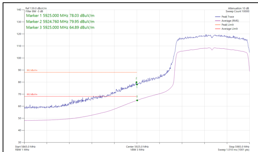
Figure 367 - 802.11ax HE40, SU, SDM, Core 0-1 - 5965 MHz Band Edge Frequency 5925 MHz
