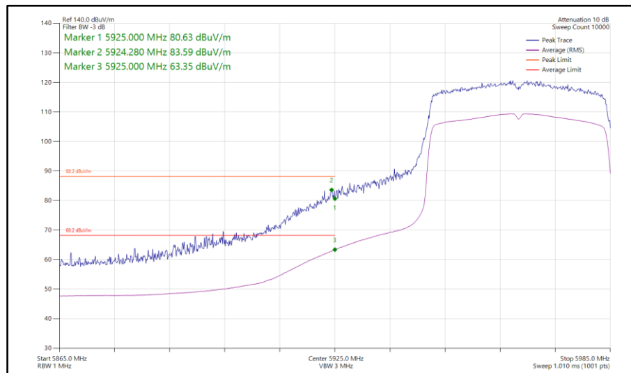
Figure 374 - 802.11ax HE40, SU, TxBF, Core 0-1 - 5965 MHz Band Edge Frequency 5925 MHz
