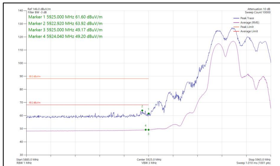
Figure 326 - 802.11ax HE20, RU106-53, SDM, Core 0-1 - 5955 MHz Band Edge Frequency 5925 MHz
