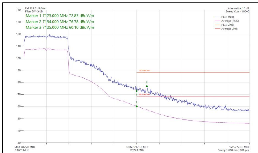
Figure 370 - 802.11ax HE40, SU, SDM, Core 0-1 - 7045 MHz Band Edge Frequency 7125 MHz
