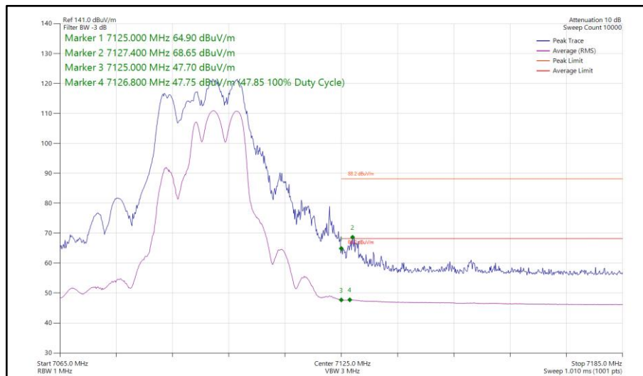
Figure 373 - 802.11be EHT40, RU106+26-85, SDM, Core 0-1 - 7085 MHz Band Edge Frequency 7125 MHz
