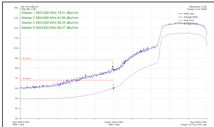
Figure 334 - 802.11ax HE20, SU, TxBF, Core 0-1 - 5955 MHz Band Edge Frequency 5925 MHz
