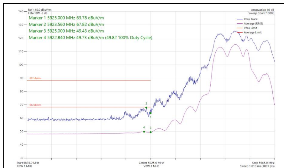
Figure 327 - 802.11be EHT20, RU106+26-82, SDM, Core 0-1 - 5955 MHz Band Edge Frequency 5925 MHz
