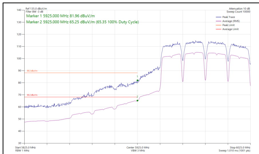
Figure 377 - 802.11a a80, SISO, Core 0 - 5985 MHz Band Edge Frequency 5925 MHz
