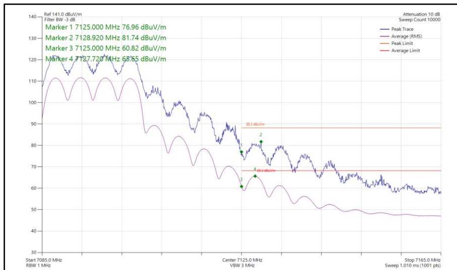
Figure 319 - 802.11ax HE20, SU, CDD, Core 0-1 - 7095 MHz Band Edge Frequency 7125 MHz
