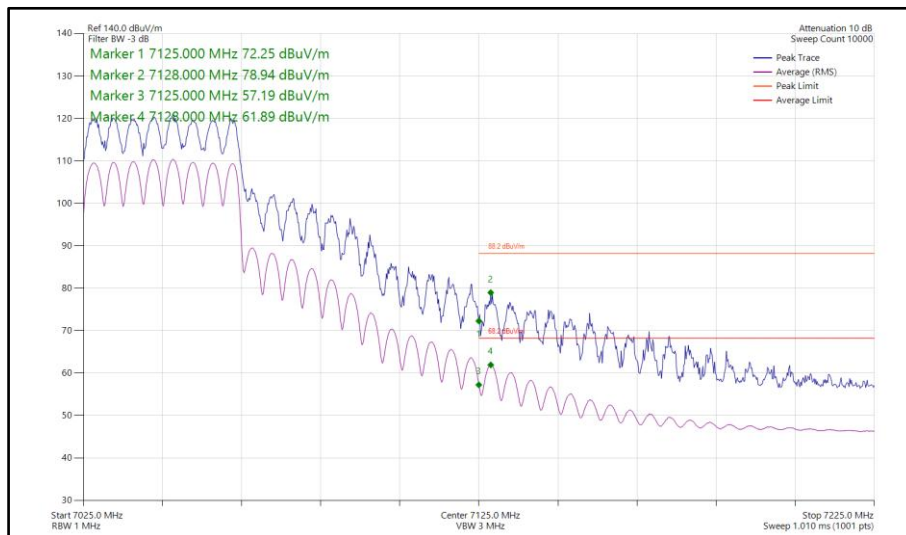
Figure 363 - 802.11ax HE40, SU, CDD, Core 0-1 - 7045 MHz Band Edge Frequency 7125 MHz
