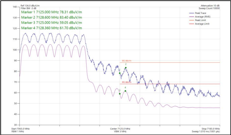
Figure 364 - 802.11ax HE40, SU, CDD, Core 0-1 - 7085 MHz Band Edge Frequency 7125 MHz
