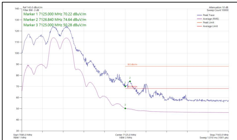
Figure 329 - 802.11ax HE20, RU106-54, SDM, Core 0-1 - 7095 MHz Band Edge Frequency 7125 MHz
