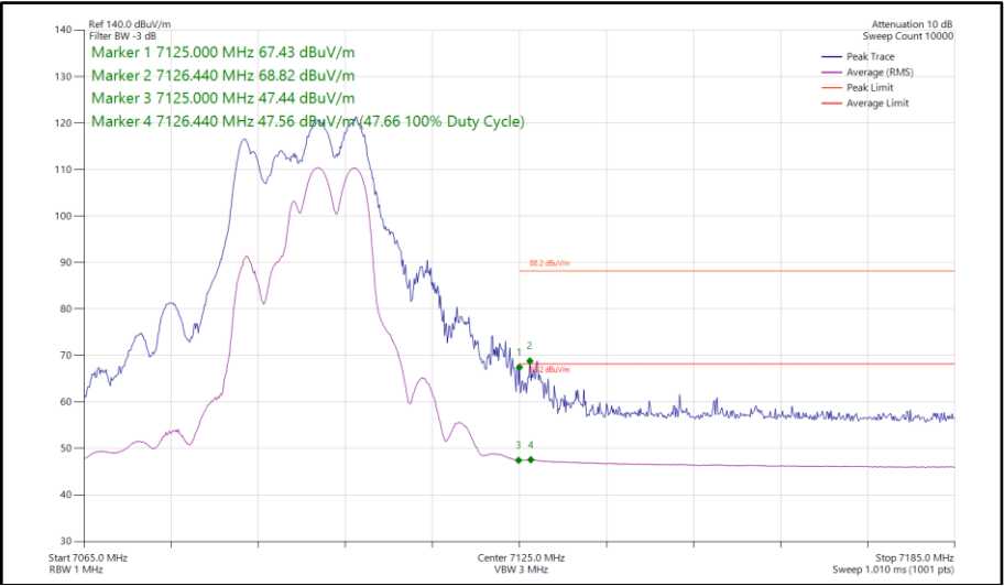
Figure 366 - 802.11be EHT40, RU106+26-85, CDD, Core 0-1 - 7085 MHz Band Edge Frequency 7125 MHz
