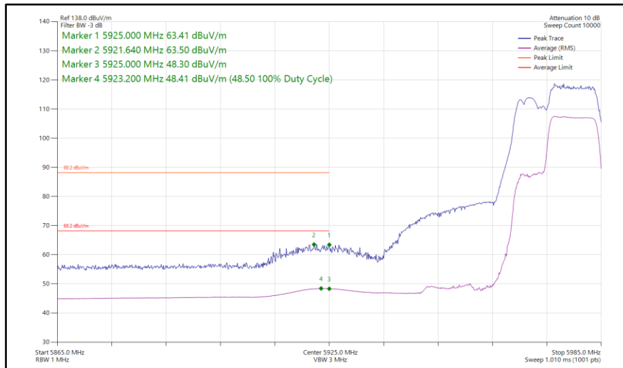
Figure 350 - 802.11be EHT40, RU106+26-85, SISO, Core 1 - 5965 MHz Band Edge Frequency 5925 MHz
