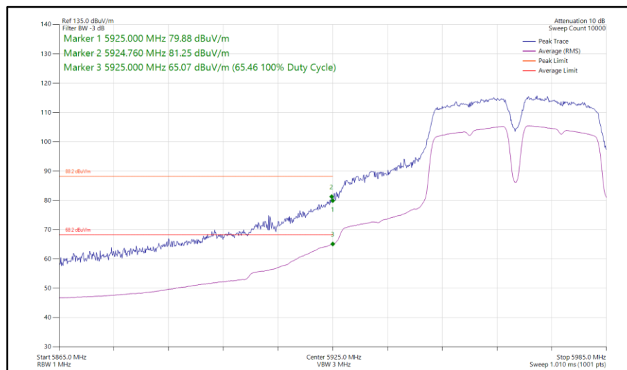
Figure 347 - 802.11a a40, SISO, Core 1 - 5965 MHz Band Edge Frequency 5925 MHz
