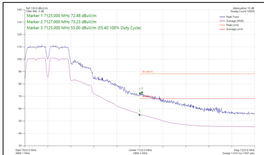
Figure 341 - 802.11a a40, SISO, Core 0 - 7045 MHz Band Edge Frequency 7125 MHz
