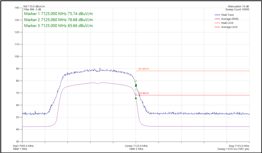
Figure 336 - 802.11ax HE20, SU, TxBF, Core 0-1 - 7115 MHz Band Edge Frequency 7125 MHz
