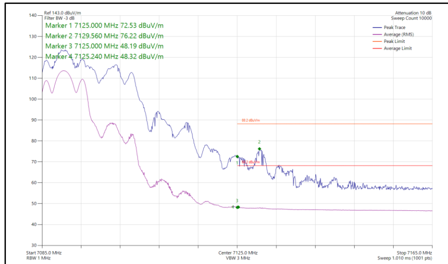
Figure 320 - 802.11ax HE20, RU106-53, CDD, Core 0-1 - 7095 MHz Band Edge Frequency 7125 MHz
