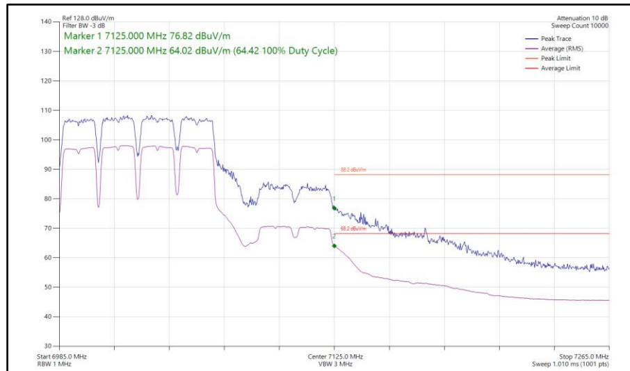
Figure 382 - 802.11a a80, SISO, Core 0 - 7025 MHz Band Edge Frequency 7125 MHz
