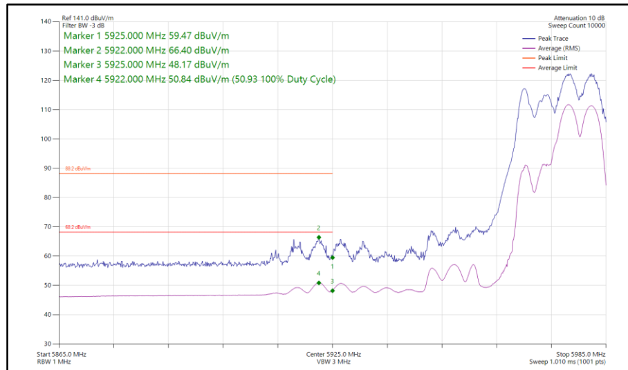
Figure 360 - 802.11be EHT40, RU106+26-85, CDD, Core 0-1 - 5965 MHz Band Edge Frequency 5925 MHz
