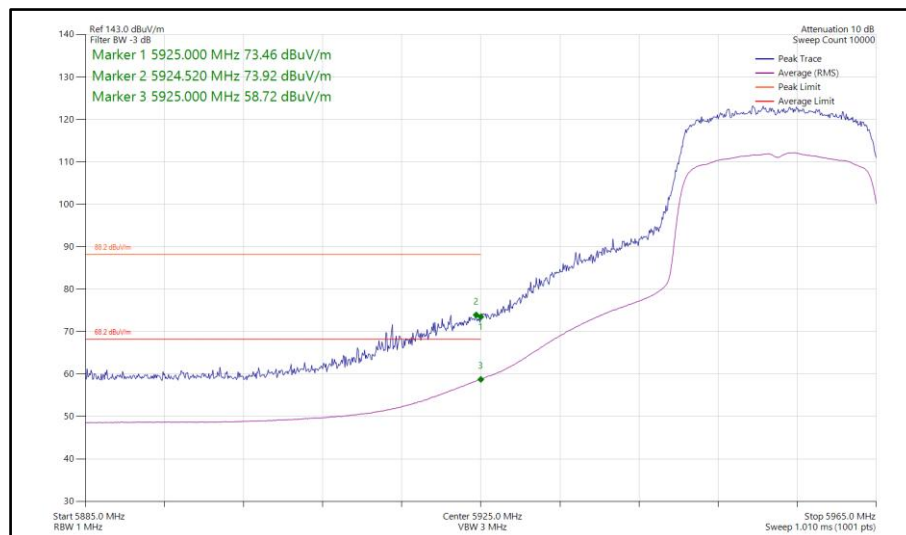
Figure 325 - 802.11ax HE20, SU, SDM, Core 0-1 - 5955 MHz Band Edge Frequency 5925 MHz
