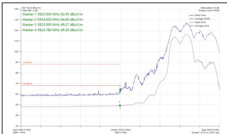
Figure 315 - 802.11ax HE20, RU106-53, CDD, Core 0-1 - 5955 MHz Band Edge Frequency 5925 MHz
