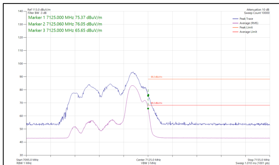
Figure 331 - 802.11ax HE20, RU52-40, SDM, Core 0-1 - 7115 MHz Band Edge Frequency 7125 MHz
