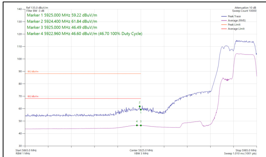
Figure 340 - 802.11be EHT40, RU106+26-85, SISO, Core 0 - 5965 MHz Band Edge Frequency 5925 MHz
