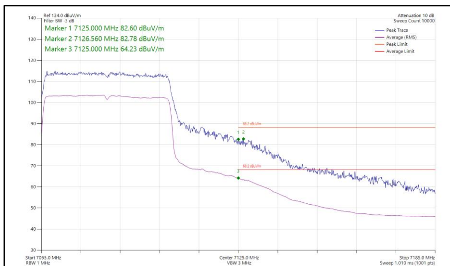
Figure 371 - 802.11ax HE40, SU, SDM, Core 0-1 - 7085 MHz Band Edge Frequency 7125 MHz
