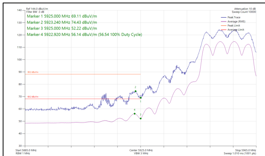
Figure 313 - 802.11a, CDD, Core 0-1 - 5955 MHz Band Edge Frequency 5925 MHz
