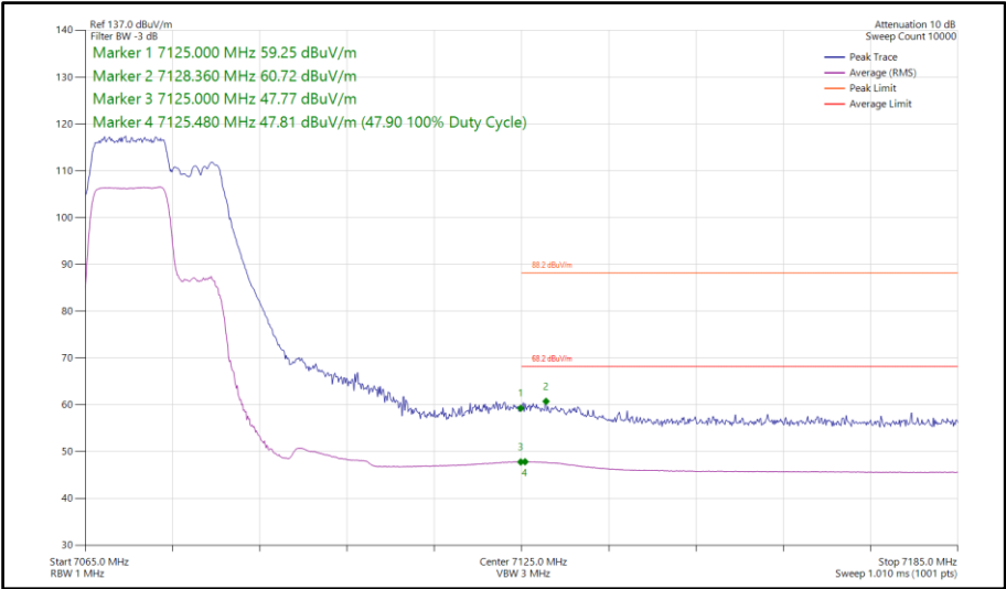
Figure 346 - 802.11be EHT40, RU106+26-82, SISO, Core 0 - 7085 MHz Band Edge Frequency 7125 MHz
