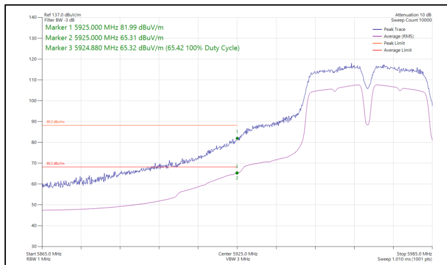
Figure 337 - 802.11a a40, SISO, Core 0 - 5965 MHz Band Edge Frequency 5925 MHz
