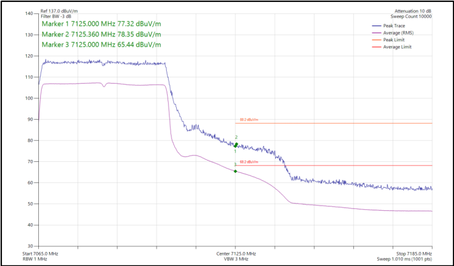
Figure 376 - 802.11ax HE40, SU, TxBF, Core 0-1 - 7085 MHz Band Edge Frequency 7125 MHz
