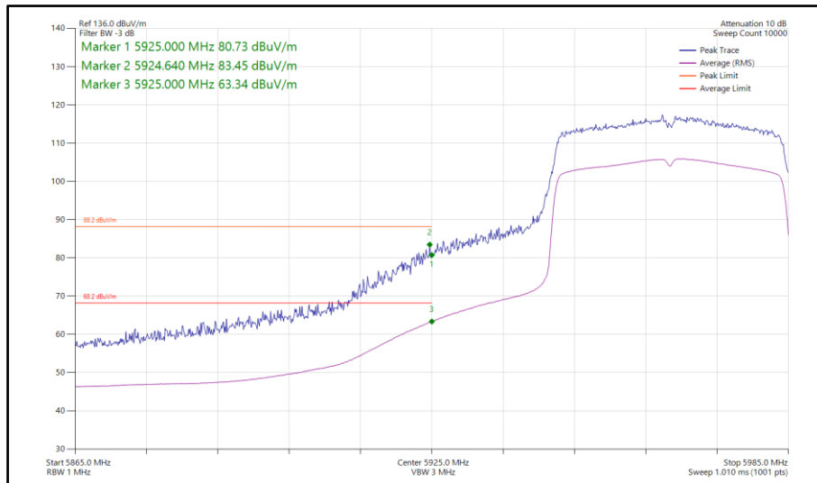
Figure 348 - 802.11ax HE40, SU, SISO, Core 1 - 5965 MHz Band Edge Frequency 5925 MHz
