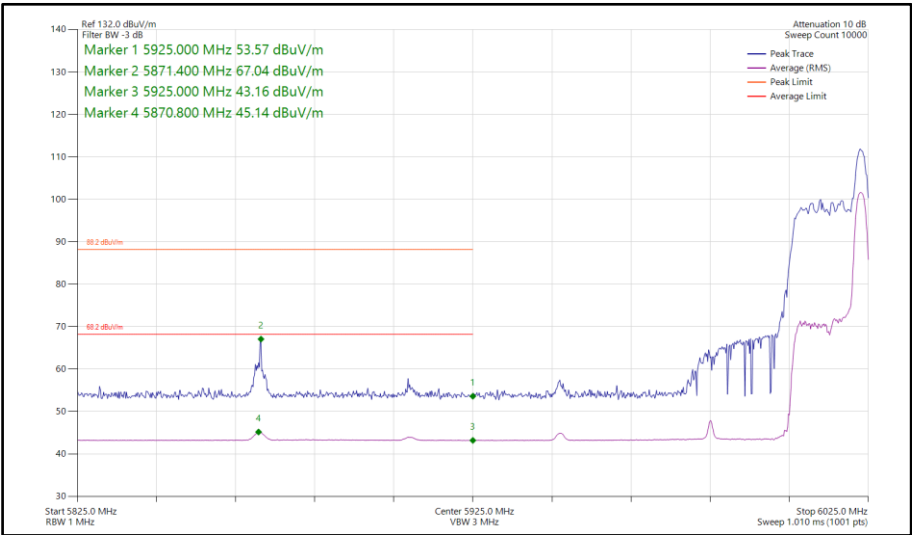
Figure 379 - 802.11ax HE80, RU26-36, SISO, Core 0 - 5985 MHz Band Edge Frequency 5925 MHz
