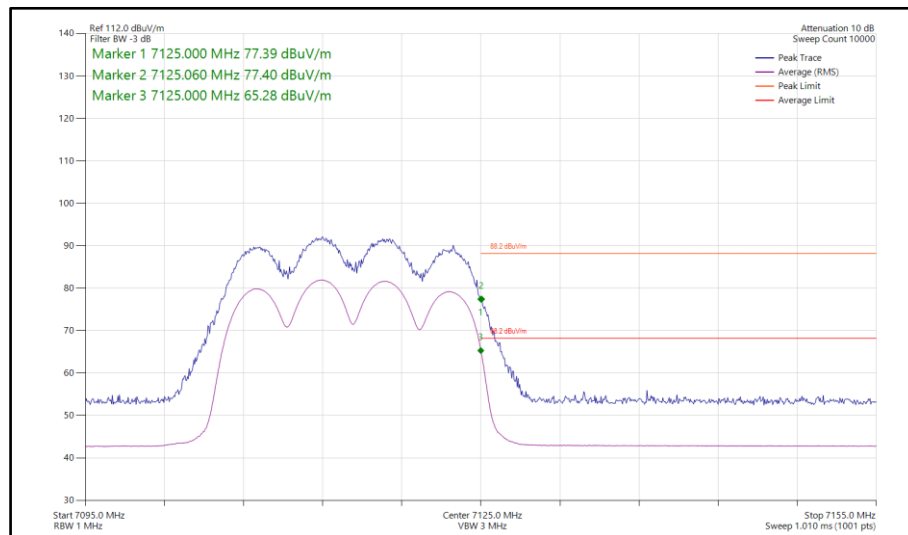
Figure 321 - 802.11ax HE20, SU, CDD, Core 0-1 - 7115 MHz Band Edge Frequency 7125 MHz
