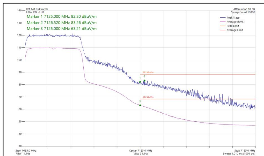
Figure 335 - 802.11ax HE20, SU, TxBF, Core 0-1 - 7095 MHz Band Edge Frequency 7125 MHz
