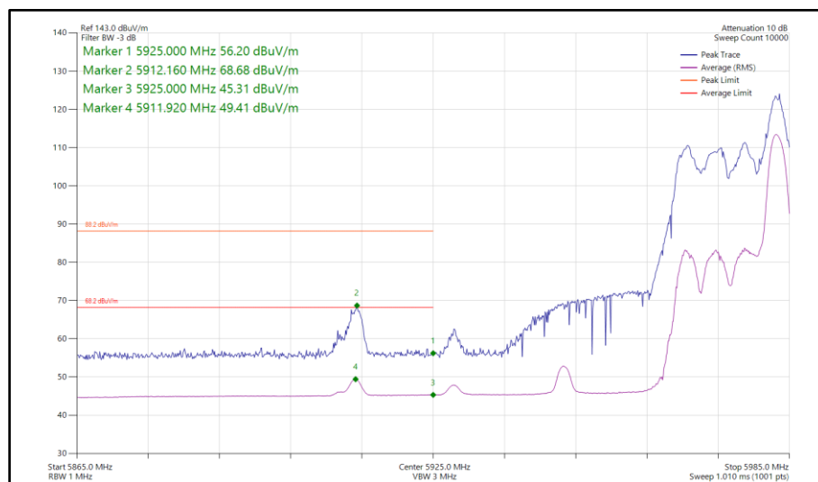
Figure 359 - 802.11ax HE40, RU26-17, CDD, Core 0-1 - 5965 MHz Band Edge Frequency 5925 MHz
