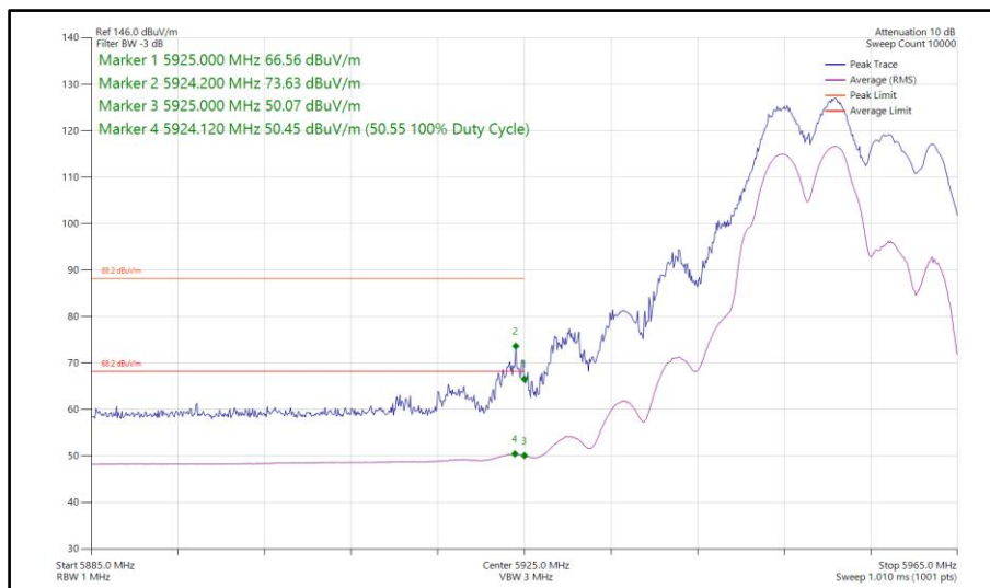
Figure 316 - 802.11be EHT20, RU106+26-82, CDD, Core 0-1 - 5955 MHz Band Edge Frequency 5925 MHz
