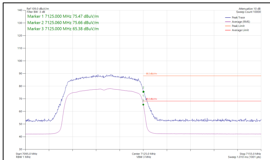
Figure 330 - 802.11ax HE20, SU, SDM, Core 0-1 - 7115 MHz Band Edge Frequency 7125 MHz
