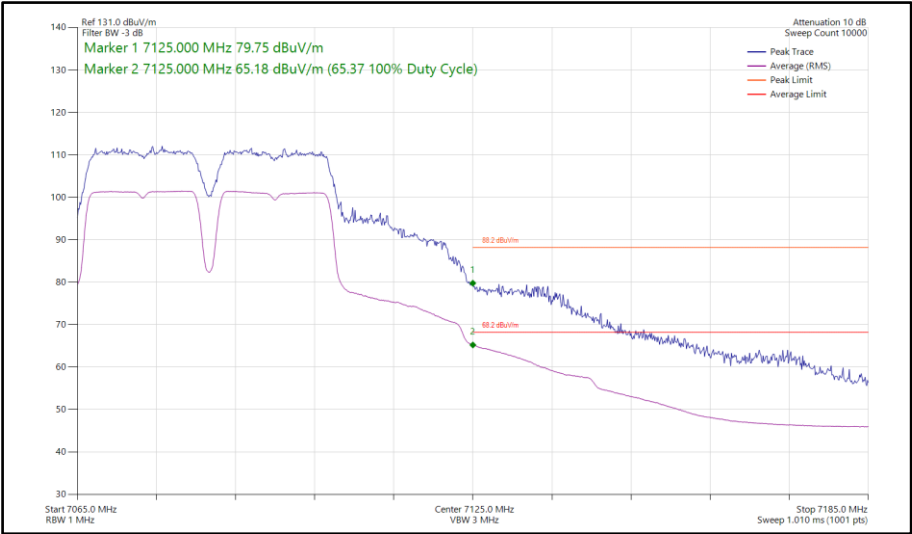
Figure 352 - 802.11a a40, SISO, Core 1 - 7085 MHz Band Edge Frequency 7125 MHz
