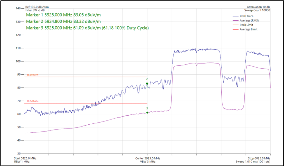
Figure 380 - 802.11be EHT80, RU484+242-92, SISO, Core 0 - 5985 MHz Band Edge Frequency 5925 MHz
