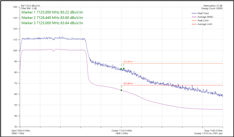
Figure 354 - 802.11ax HE40, SU, SISO, Core 1 - 7085 MHz Band Edge Frequency 7125 MHz
