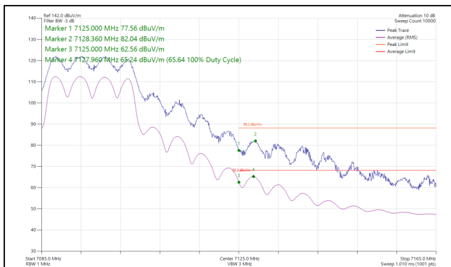
Figure 317 - 802.11a, CDD, Core 0-1 - 7095 MHz Band Edge Frequency 7125 MHz
