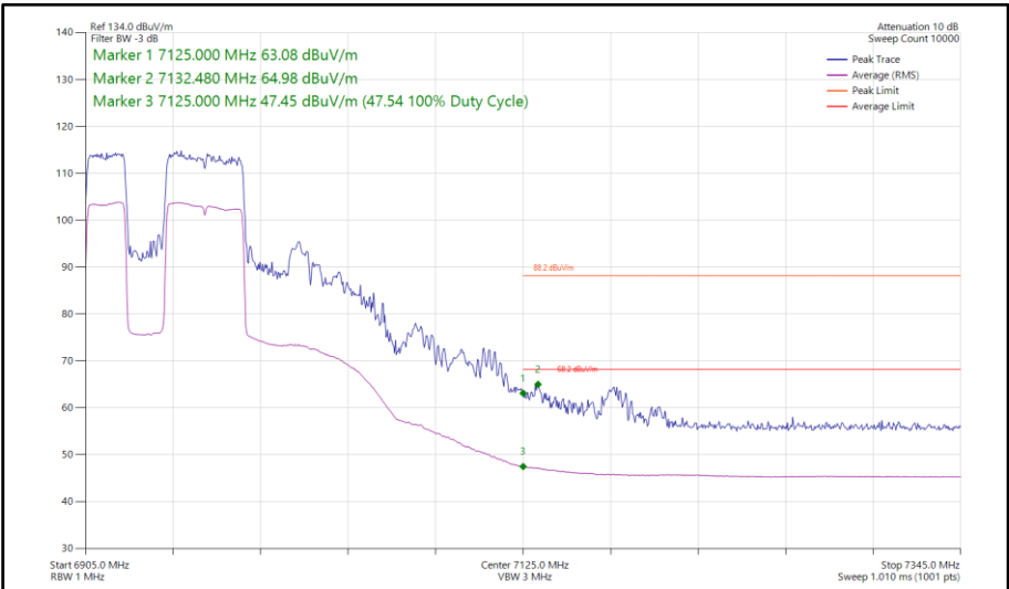
Figure 385 - 802.11be EHT80, RU484+242-91, SISO, Core 0 - 6945 MHz Band Edge Frequency 7125 MHz
