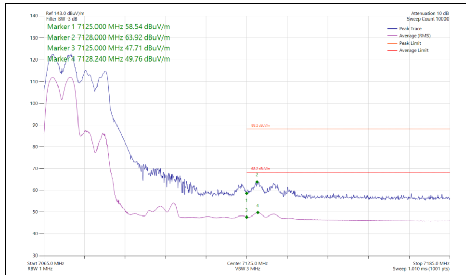
Figure 372 - 802.11ax HE40, RU106-53, SDM, Core 0-1 - 7085 MHz Band Edge Frequency 7125 MHz
