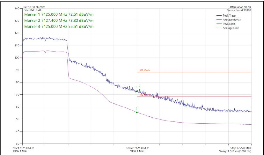
Figure 343 - 802.11ax HE40, SU, SISO, Core 0 - 7045 MHz Band Edge Frequency 7125 MHz
