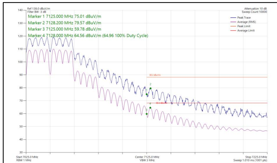
Figure 361 - 802.11a a40, CDD, Core 0-1 - 7045 MHz Band Edge Frequency 7125 MHz
