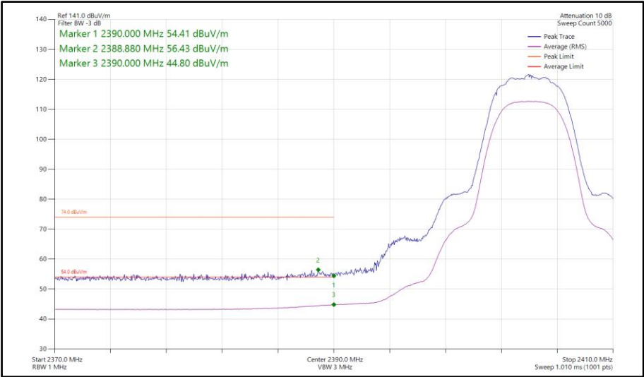
Figure 151 - Bluetooth HDRPM12, SISO, Core 1 - 2404 MHz Band Edge Frequency 2390 MHz
