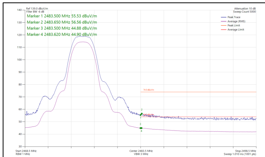
Figure 133 - Bluetooth HDT3, SISO, Core 0 - 2476 MHz Band Edge Frequency 2483.5 MHz
