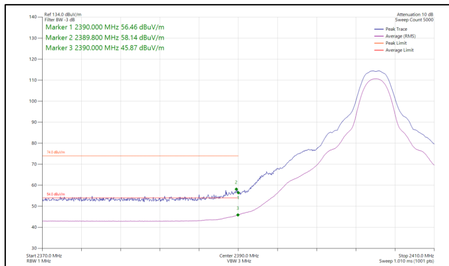
Figure 91 - Bluetooth HDT3, MIMO, Core 0-1 - 2404 MHz Band Edge Frequency 2390 MHz
