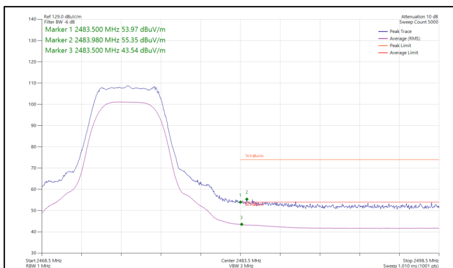
Figure 110 - Bluetooth XHDRPM8, MIMO, Core 0-1 - 2475 MHz Band Edge Frequency 2483.5 MHz
