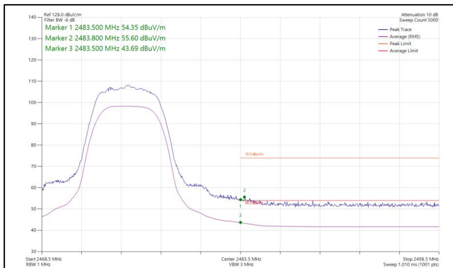
Figure 109 - Bluetooth HDRPM12, MIMO, Core 0-1 - 2475 MHz Band Edge Frequency 2483.5 MHz
