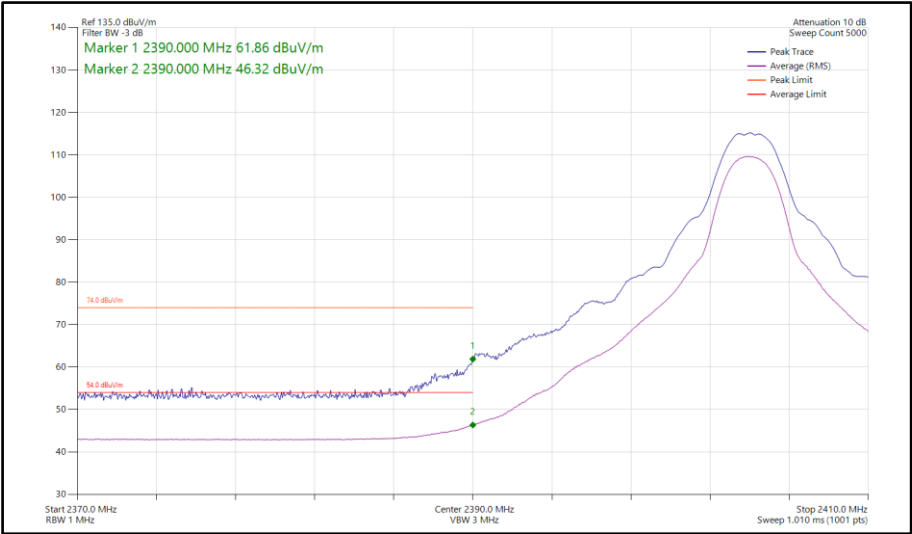
Figure 93 - Bluetooth HDT6, MIMO, Core 0-1 - 2404 MHz Band Edge Frequency 2390 MHz
