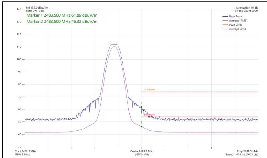
Figure 75 - Bluetooth LE1M, SISO, Core 2 - 2480 MHz Band Edge Frequency 2483.5 MHz
