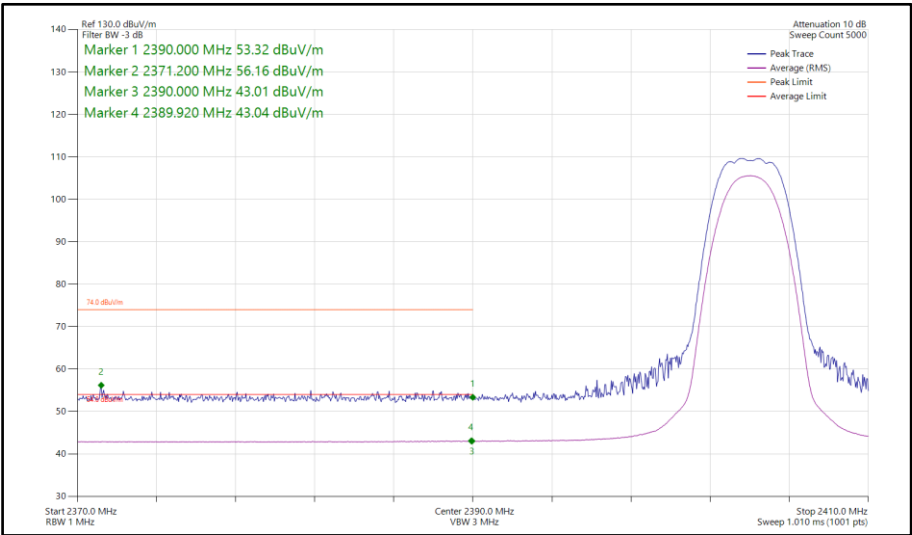
Figure 94 - Bluetooth HDRPS2, MIMO, Core 0-1 - 2404 MHz Band Edge Frequency 2390 MHz
