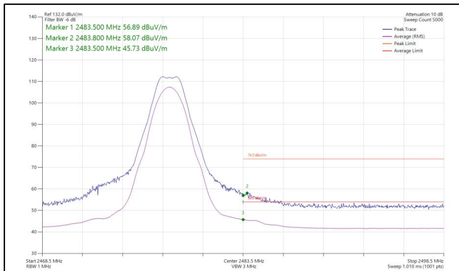
Figure 76 - Bluetooth LE2M, SISO, Core 2 - 2478 MHz Band Edge Frequency 2483.5 MHz
