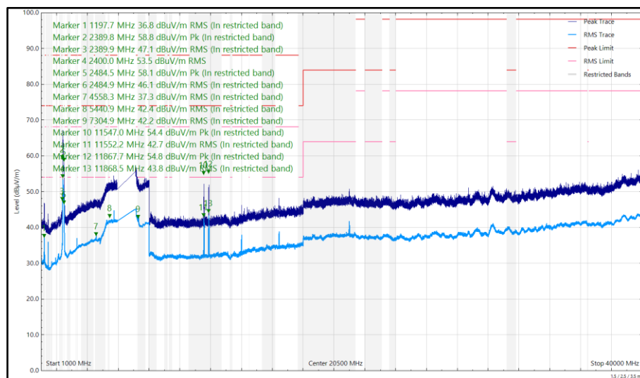
Figure 49 - 2437 MHz (CH6), HT20, Core 0 + Core 1 and 6995 MHz (CH209), HE20, SU, CDD, Core 0 + Core 1 and 2450 MHz (CH20), Thread, iPA, Core 2, 1 GHz to 40 GHz, Vertical
