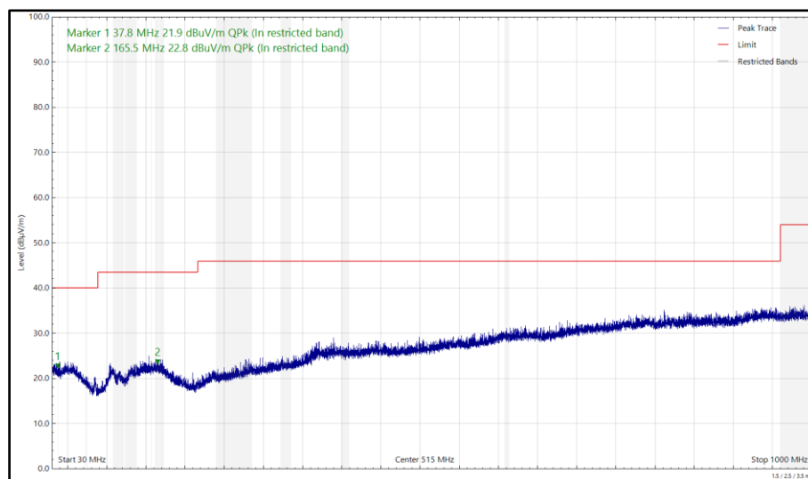
Figure 22 - 6995 MHz (CH209), HE20, SU, CDD, Core 0 + Core 1 and 2440 MHz (CH18), Thread, ePA, Core 1, 30 MHz to 1 GHz, Horizontal (Peak)
