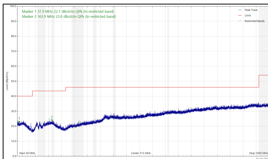
Figure 26 - 2437 MHz (CH6), HT20, CDD, Core 0 + Core 1 and 2450 MHz, DH5, iPA, Core 2 and 5788 MHz, DH5, ePA, Core 0 + Core 1, 30 MHz to 1 GHz, Horizontal (Peak)
