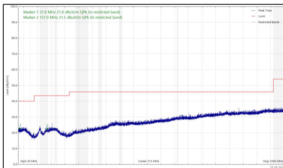
Figure 6 - 6995 MHz (CH209), HE20, SU, CDD, Core 0 + Core 1 and 2441 MHz, DH5, ePA, Core 0 + Core 1, 30 MHz to 1 GHz, Horizontal (Peak)
