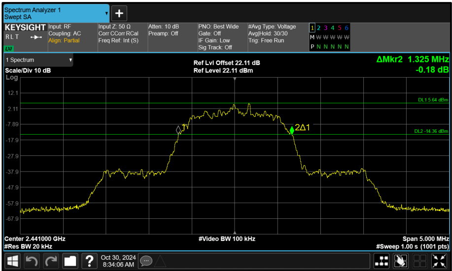
Figure 105 - Core 2 (C) 2441 MHz (CH39) 20 dB Bandwidth
