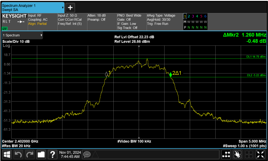
Figure 127 - Core 1 (B) 2402 MHz (CH0) 20 dB Bandwidth
