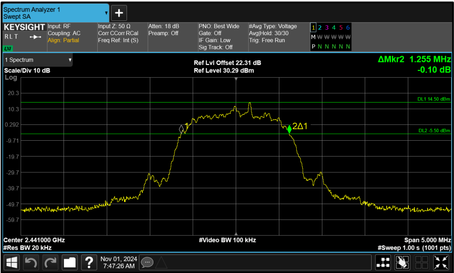
Figure 128 - Core 1 (B) 2441 MHz (CH39) 20 dB Bandwidth
