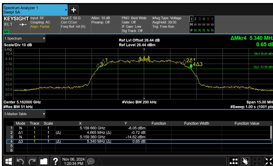
Figure 43 - Core 1 (B) 5162 MHz (CH12) 26 dB and 99% Bandwidth
