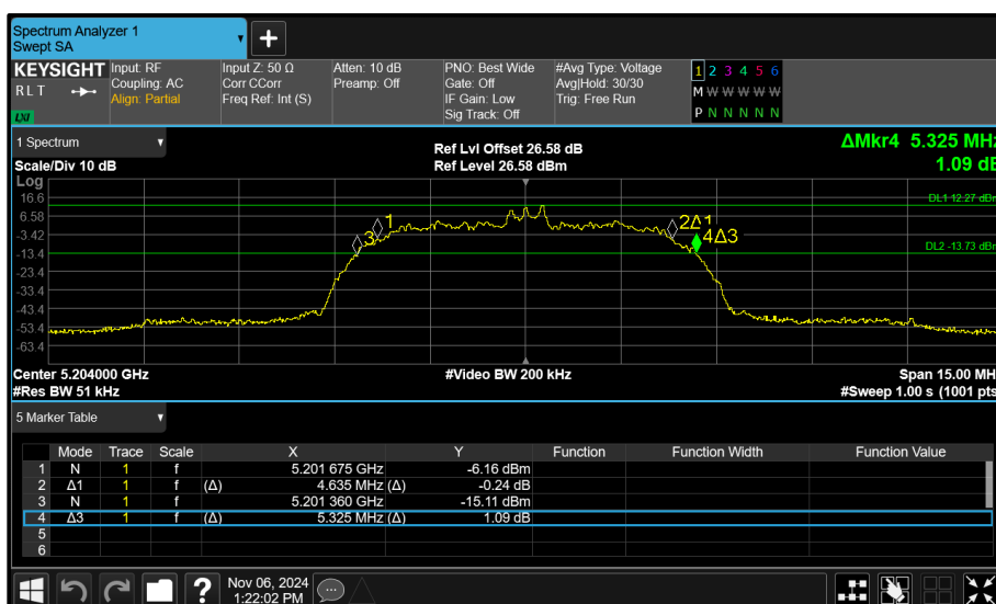
Figure 44 - Core 1 (B) 5204 MHz (CH54) 26 dB and 99% Bandwidth
