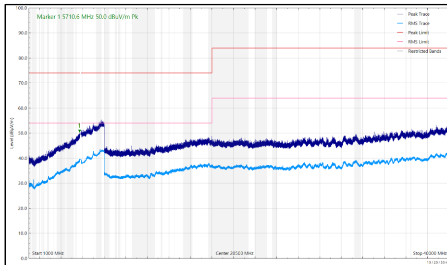
Figure 211 - 5733 MHz, DH5, ePA, Core 0 + Core 1, 1 GHz to 40 GHz, Horizontal
