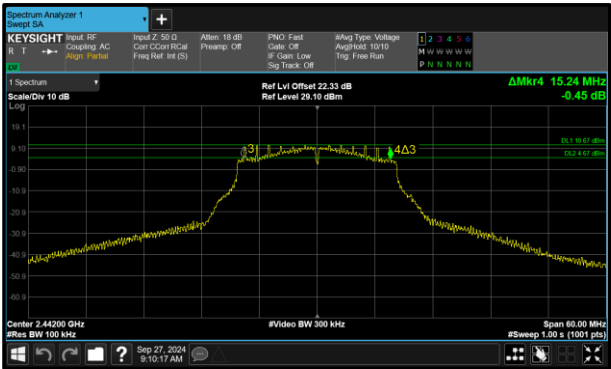
Figure 54 - 802.11g Minimum 6 dB EBW
