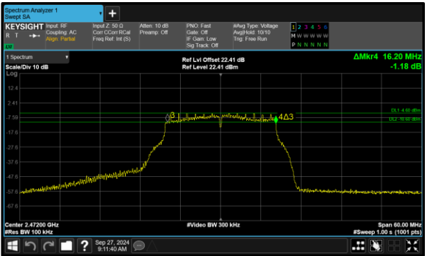
Figure 55 - 802.11g Maximum 6 dB EBW
