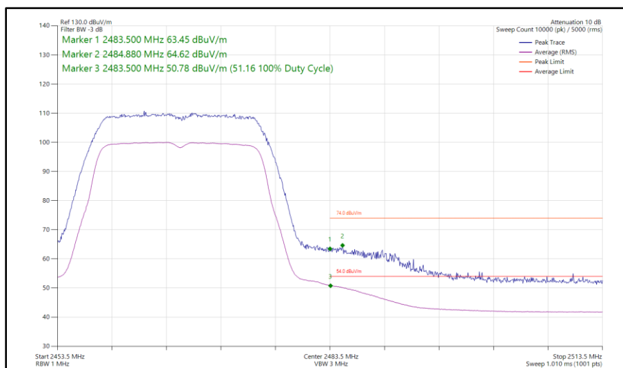
Figure 12 - 802.11n HT20, SISO, Core 0 - 2467 MHz Band Edge Frequency 2483.5 MHz
