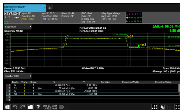
Figure 18 - 802.11ax HE80 SU SP Maximum 26 dB EBW
