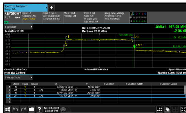
Figure 20 - 802.11ax HE160 SU SP Maximum 26 dB EBW
