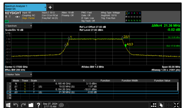
Figure 114 - 802.11ax HE20 SU SP Maximum 26 dB EBW
