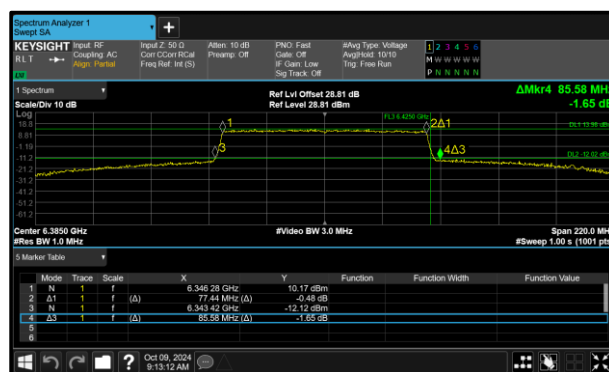
Figure 118 - 802.11ax HE80 SU SP Maximum 26 dB EBW
