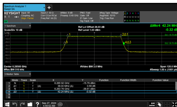
Figure 78 - 802.11ax HE40 SU VLP Maximum 26 dB EBW
