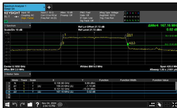
Figure 120 - 802.11ax HE160 SU SP Maximum 26 dB EBW
