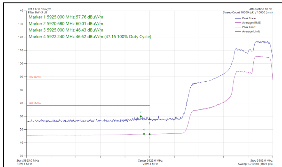
Figure 199 - 802.11ax HE40, RU 106-56, SISO, Core 0 - 5965 MHz Band Edge Frequency 5925 MHz
