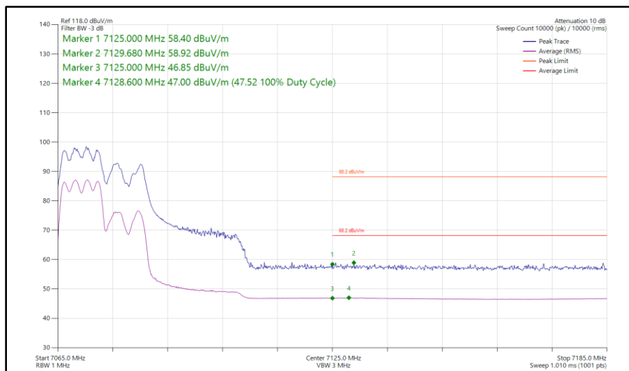
Figure 209 - 802.11ax HE40, RU 106-53, CDD, Core 0 - Core 1 - 7085 MHz Band Edge Frequency 7125 MHz
