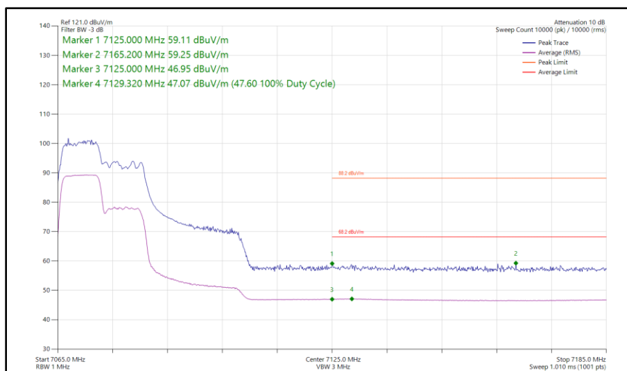
Figure 205 - 802.11ax HE40, RU 106-53, SISO, Core 1 - 7085 MHz Band Edge Frequency 7125 MHz
