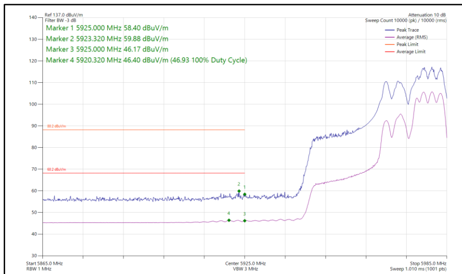
Figure 207 - 802.11ax HE40, RU 106-56, CDD, Core 0 - Core 1 - 5965 MHz Band Edge Frequency 5925 MHz
