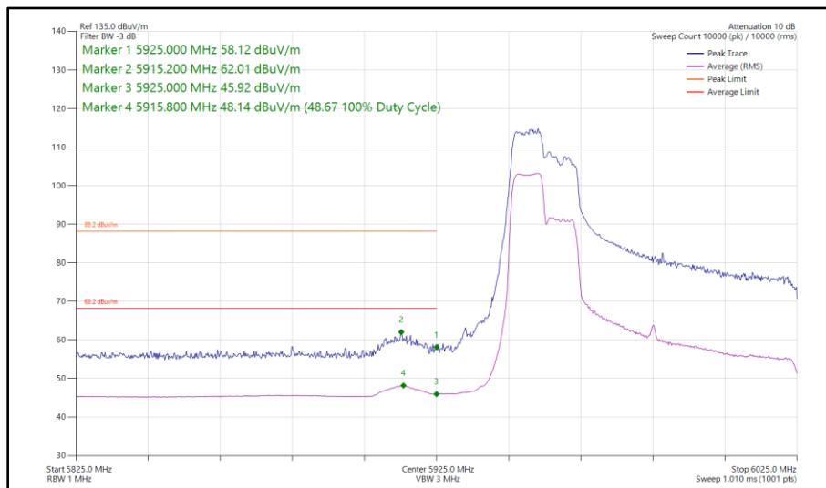
Figure 217 - 802.11ax HE80, RU 106-53, SISO, Core 0 - 5985 MHz Band Edge Frequency 5925 MHz
