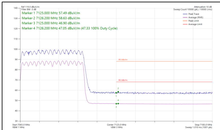
Figure 208 - 802.11ax HE40, SU, CDD, Core 0 - Core 1 - 7085 MHz Band Edge Frequency 7125 MHz
