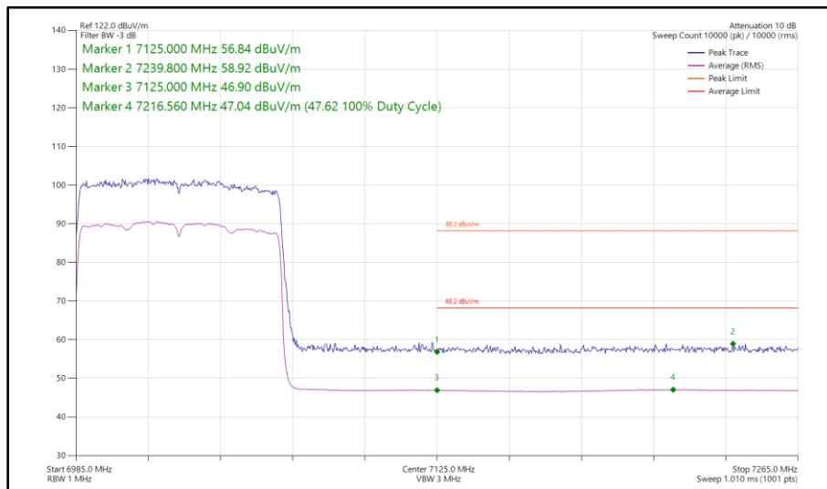
Figure 218 - 802.11ax HE80, SU, SISO, Core 0 - 7025 MHz Band Edge Frequency 7125 MHz
