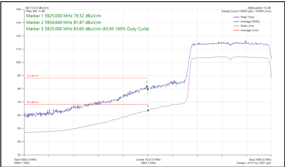
Figure 202 - 802.11ax HE40, SU, SISO, Core 1 - 5965 MHz Band Edge Frequency 5925 MHz
