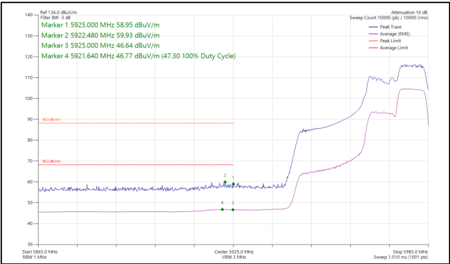
Figure 203 - 802.11ax HE40, RU 106-56, SISO, Core 1 - 5965 MHz Band Edge Frequency 5925 MHz
