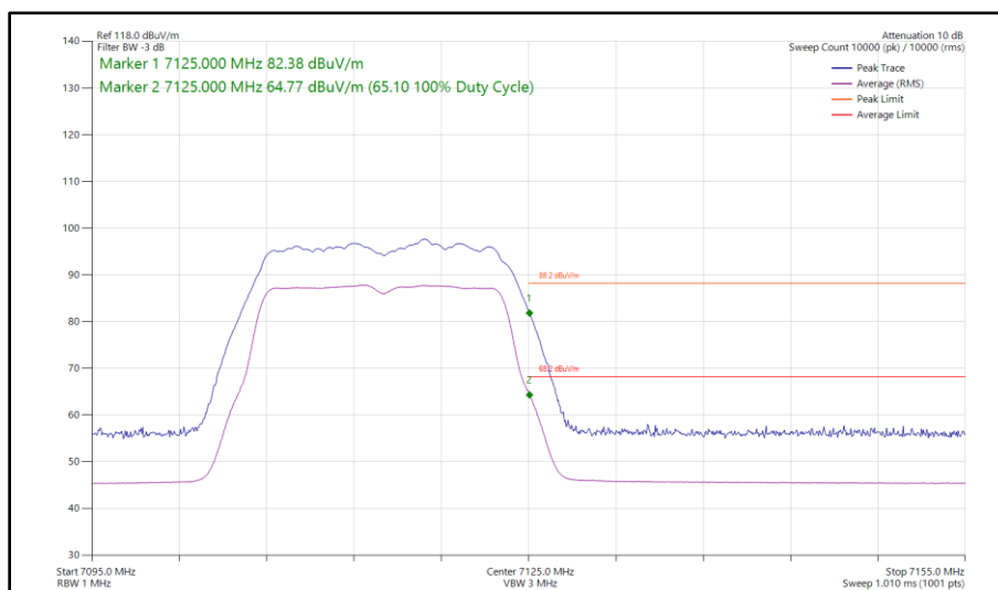
Figure 185 - 802.11a, SISO, Core 1 - 7115 MHz Band Edge Frequency 7125 MHz
