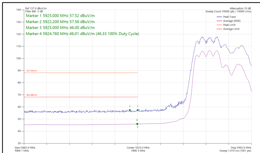
Figure 189 - 802.11ax HE20, RU 106-53, CDD, Core 0 - Core 1 - 5955 MHz Band Edge Frequency 5925 MHz
