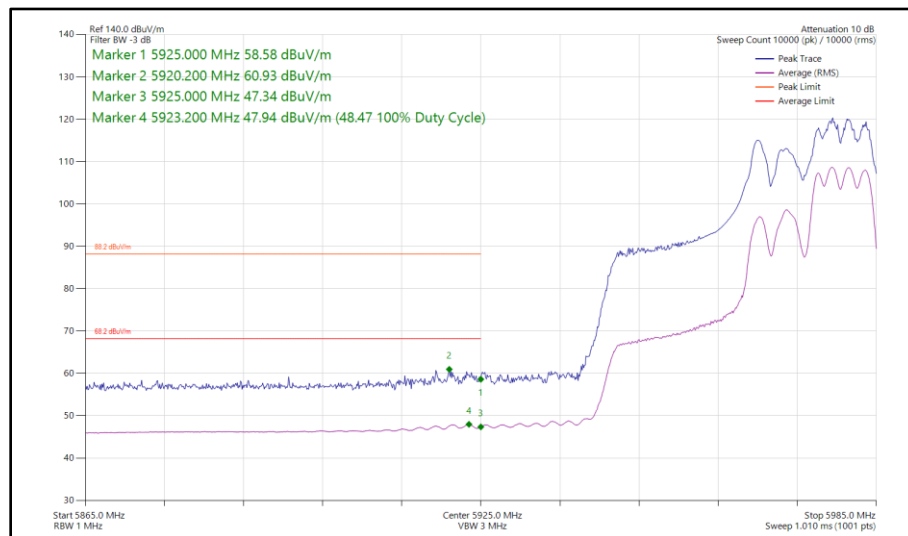
Figure 211 - 802.11ax HE40, RU 106-56, SDM, Core 0 - Core 1 - 5965 MHz Band Edge Frequency 5925 MHz
