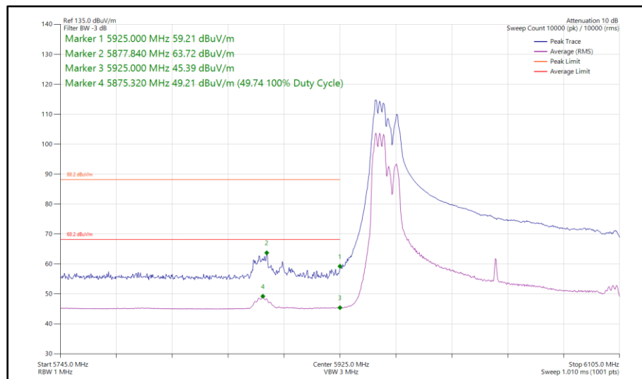
Figure 247 - 802.11ax HE160, RU 106-53P, SDM, Core 0 - Core 1 - 6025 MHz Band Edge Frequency 5925 MHz
