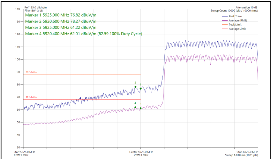
Figure 224 - 802.11ax HE80, SU, CDD, Core 0 - Core 1 - 5985 MHz Band Edge Frequency 5925 MHz
