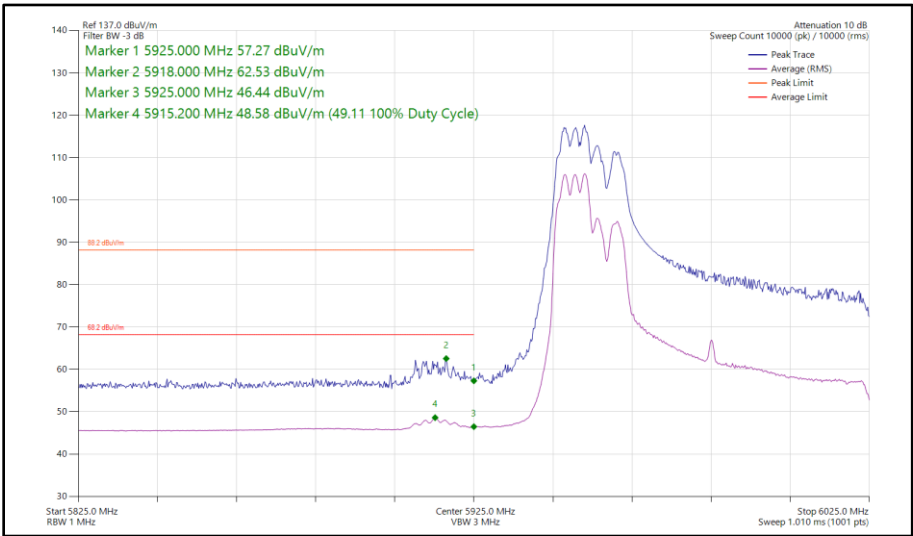
Figure 225 - 802.11ax HE80, RU 106-53, CDD, Core 0 - Core 1 - 5985 MHz Band Edge Frequency 5925 MHz
