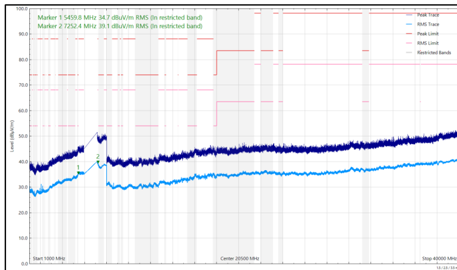
Figure 275 - U-NII-8 - 6895 MHz (CH189), HE20, SU, CDD, Core 0 + Core 1, 1 GHz to 40 GHz, Horizontal
