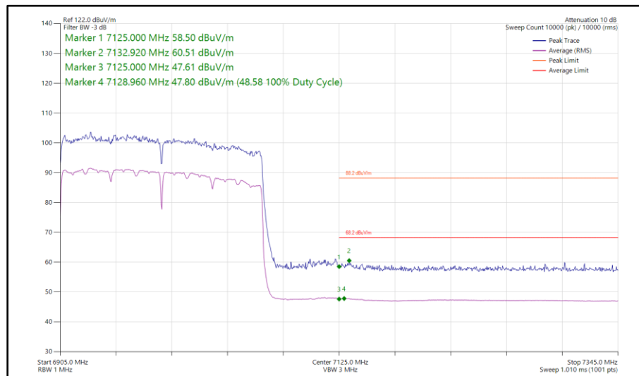
Figure 236 - 802.11ax HE160, SU, SISO, Core 0 - 6985 MHz Band Edge Frequency 7125 MHz
