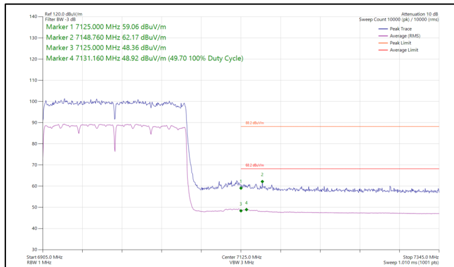
Figure 240 - 802.11ax HE160, SU, SISO, Core 1 - 6985 MHz Band Edge Frequency 7125 MHz
