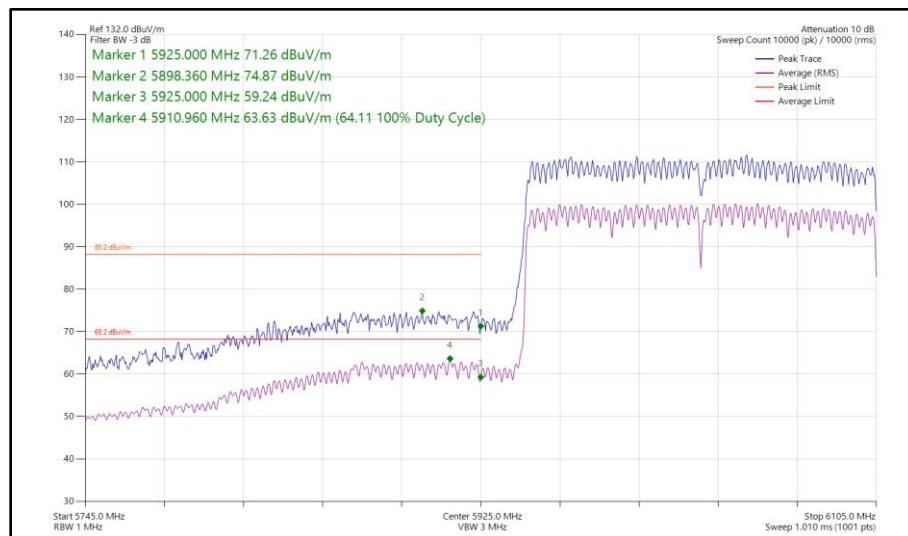
Figure 242 - 802.11ax HE160, SU, CDD, Core 0 - Core 1 - 6025 MHz Band Edge Frequency 5925 MHz
