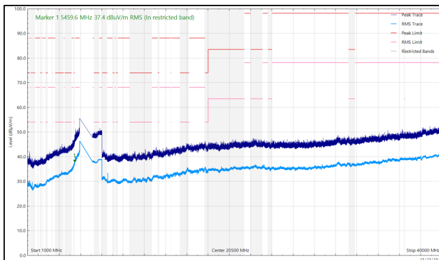
Figure 258 - U-NII-5 - 6415 MHz (CH93), HE20, SU, CDD, Core 0 + Core 1, 1 GHz to 40 GHz, Vertical
