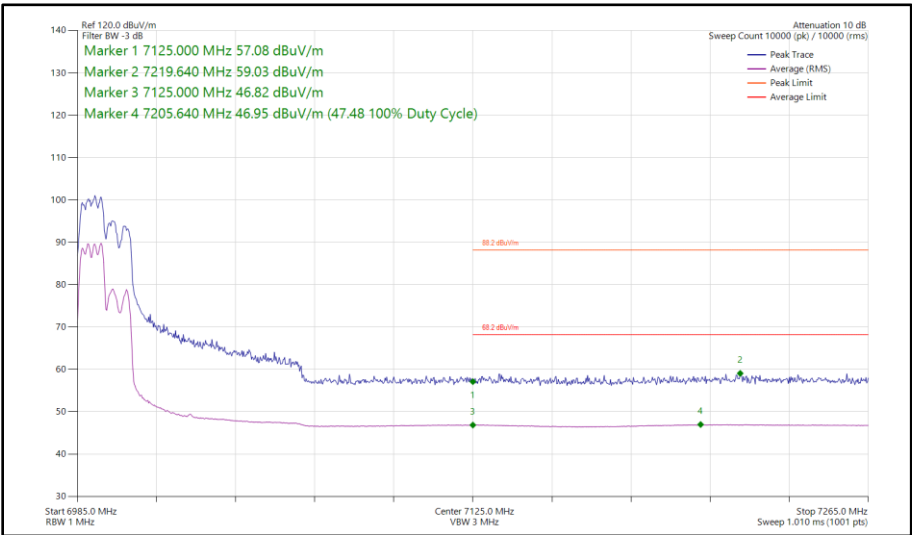
Figure 231 - 802.11ax HE80, RU 106-53, SDM, Core 0 - Core 1 - 7025 MHz Band Edge Frequency 7125 MHz
