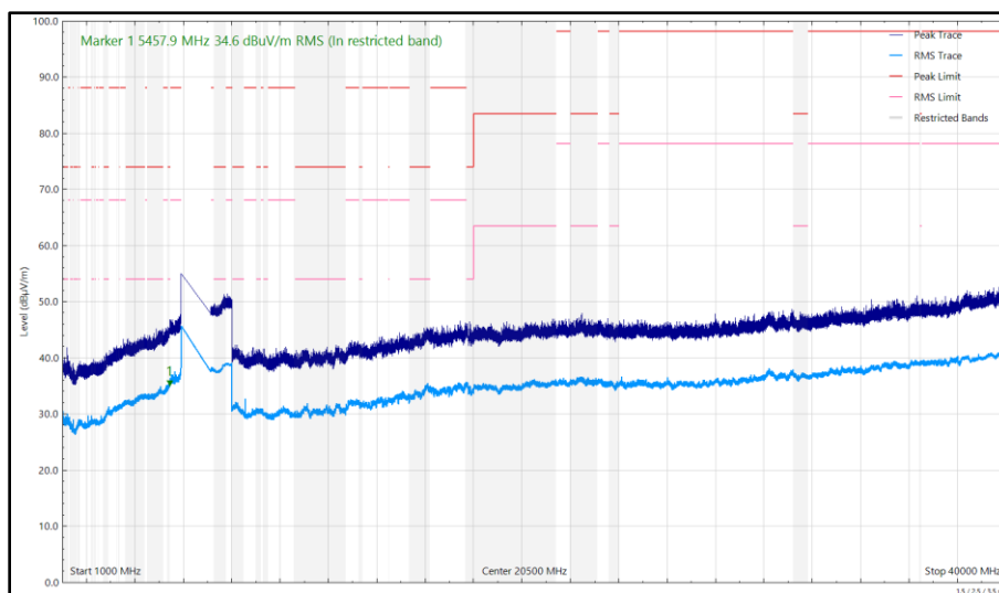
Figure 257 - U-NII-5 - 6415 MHz (CH93), HE20, SU, CDD, Core 0 + Core 1, 1 GHz to 40 GHz, Horizontal
