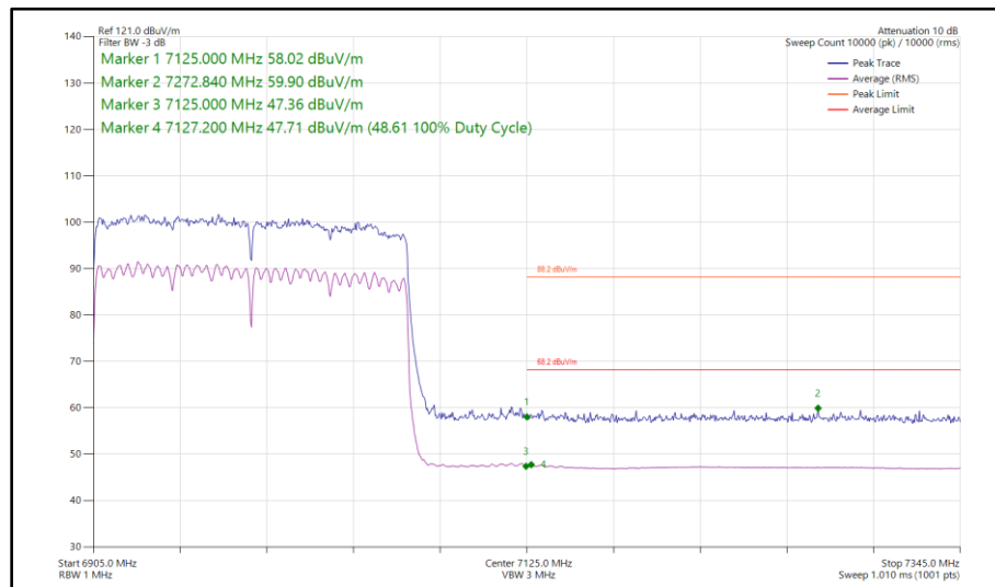
Figure 248 - 802.11ax HE160, SU, SDM, Core 0 - Core 1 - 6985 MHz Band Edge Frequency 7125 MHz
