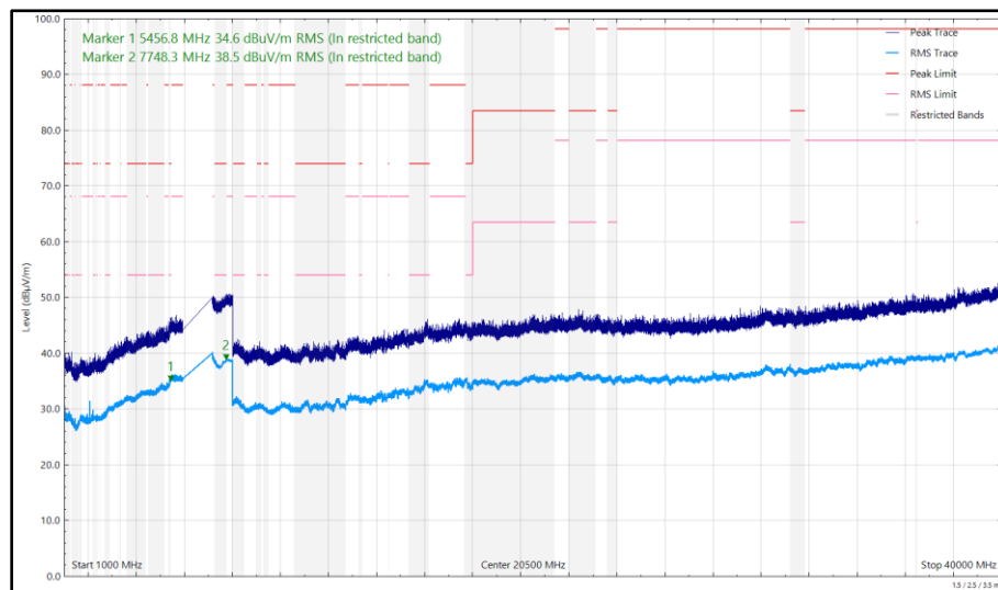
Figure 273 - U-NII-7 - 6855 MHz (CH181), HE20, SU, CDD, Core 0 + Core 1, 1 GHz to 40 GHz, Horizontal
