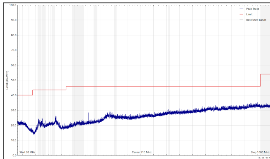
Figure 253 - U-NII-5 - 6175 MHz (CH45), HE20, SU, CDD, Core 0 + Core 1, 30 MHz to 1 GHz, Horizontal (Peak)
