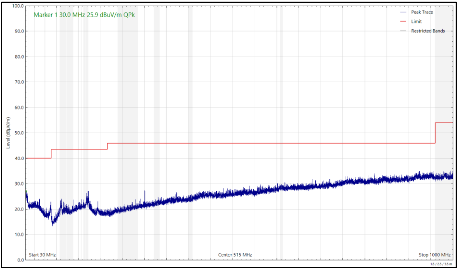
Figure 271 - U-NII-7 - 6695 MHz (CH149), HE20, SU, CDD, Core 0 + Core 1, 30 MHz to 1 GHz, Vertical (Peak)
