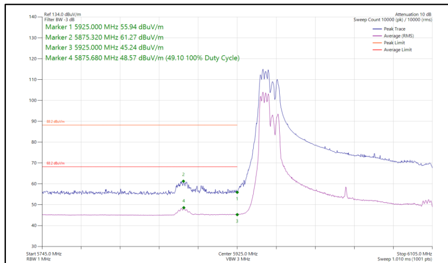
Figure 243 - 802.11ax HE160, RU 106-53P, CDD, Core 0 - Core 1 - 6025 MHz Band Edge Frequency 5925 MHz
