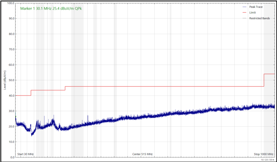
Figure 263 - U-NII-6 - 6475 MHz (CH105), HE20, SU, CDD, Core 0 + Core 1, 30 MHz to 1 GHz, Vertical (Peak)
