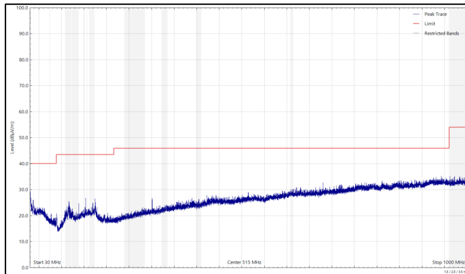
Figure 255 - U-NII-5 - 6175 MHz (CH45), HE20, SU, CDD, Core 0 + Core 1, 30 MHz to 1 GHz, Vertical (Peak)
