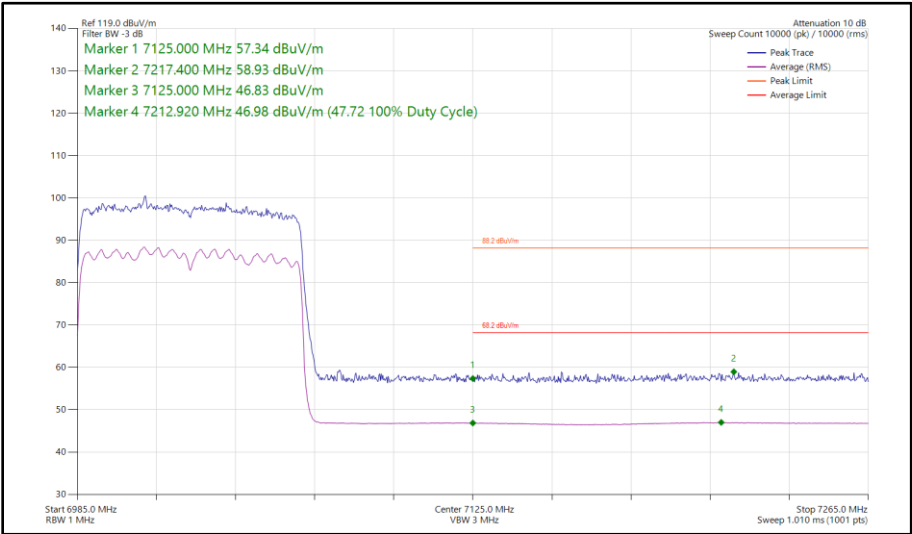
Figure 230 - 802.11ax HE80, SU, SDM, Core 0 - Core 1 - 7025 MHz Band Edge Frequency 7125 MHz
