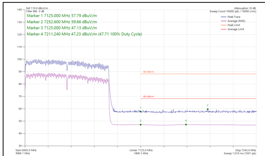
Figure 244 - 802.11ax HE160, SU, CDD, Core 0 - Core 1 - 6985 MHz Band Edge Frequency 7125 MHz
