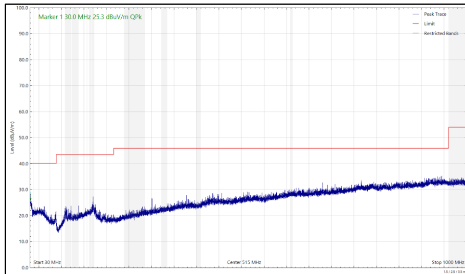
Figure 279 - U-NII-8 - 6995 MHz (CH209), HE20, SU, CDD, Core 0 + Core 1, 30 MHz to 1 GHz, Vertical (Peak)
