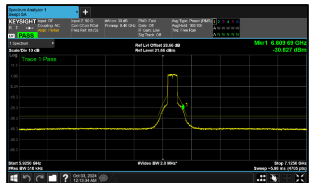
Figure 329 - B (Core 1) 802.11ax HE40 SU SP 6565 MHz (CH123)
