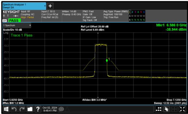
Figure 323 - B (Core 1) 802.11ax HE80 SU LPI 6545 MHz (CH19)
