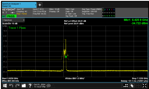
Figure 297 - A (Core 0) 802.11ax HE20 RU26 SP 6415 MHz (CH93)
