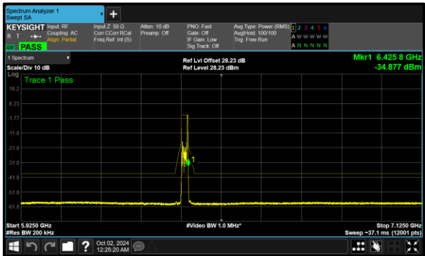
Figure 333 - B (Core 1) 802.11ax HE20 RU26 SP 6415 MHz (CH93)
