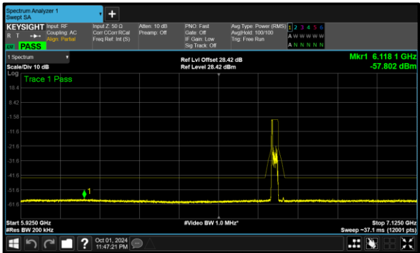
Figure 316 - A (Core 0) 802.11ax HE20 RU26 SP 6695 MHz (CH149)
