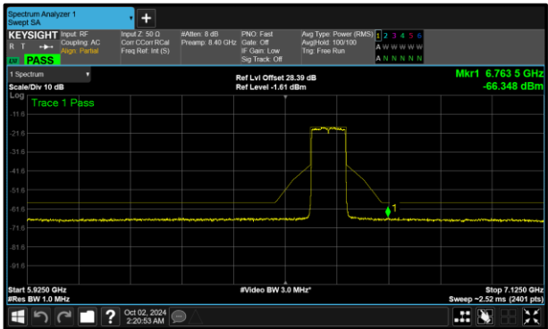
Figure 319 - B (Core 1) 802.11ax HE80 SU VLP 6625 MHz (CH135)
