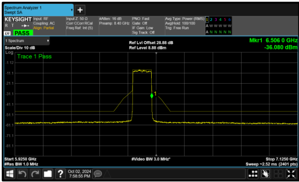
Figure 286 - A (Core 0) 802.11ax HE80 SU LPI 6465 MHz (CH103)
