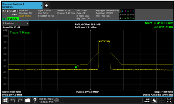
Figure 340 - A (Core 0) 802.11ax HE80 SU LPI 6625 MHz (CH135)
