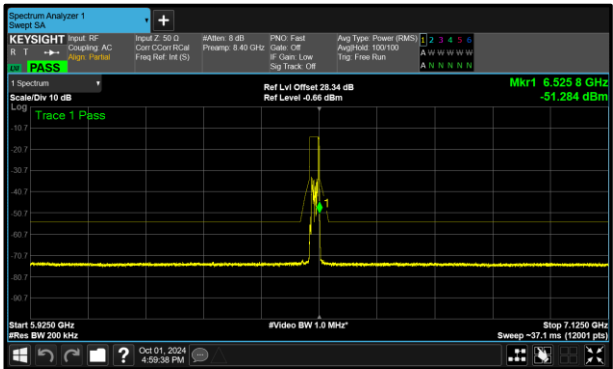
Figure 289 - A (Core 0) 802.11ax HE20 RU26 LPI 6515 MHz (CH113)
