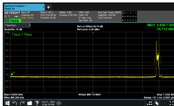
Figure 309 - A (Core 0) 802.11ax HE20 RU26 LPI 6995 MHz (CH209)
