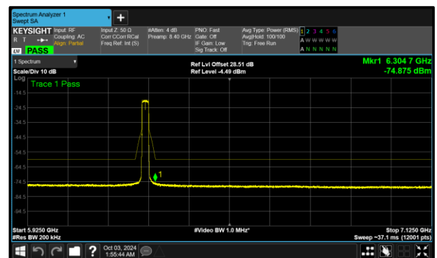
Figure 300 - A (Core 0) 802.11ax HE20 SU VLP 6275 MHz (CH65)
