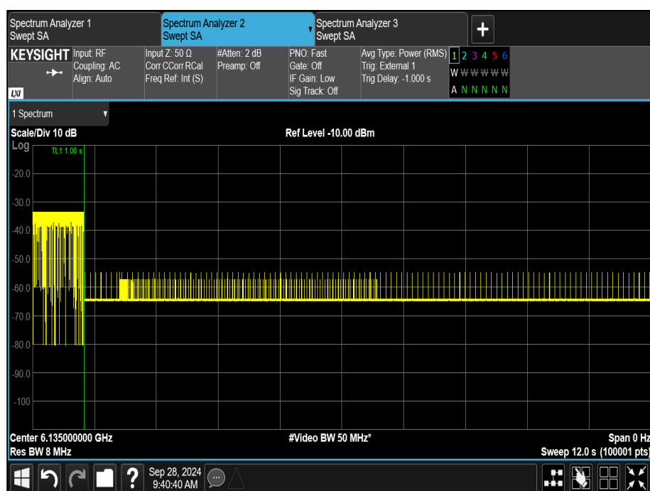
Figure 346 - U-NII-5, Minimum Bandwidth
