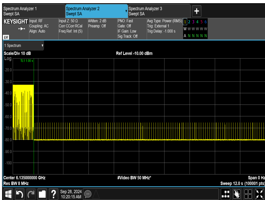
Figure 348 - U-NII-5, Minimum Bandwidth (AWGN Mid)
