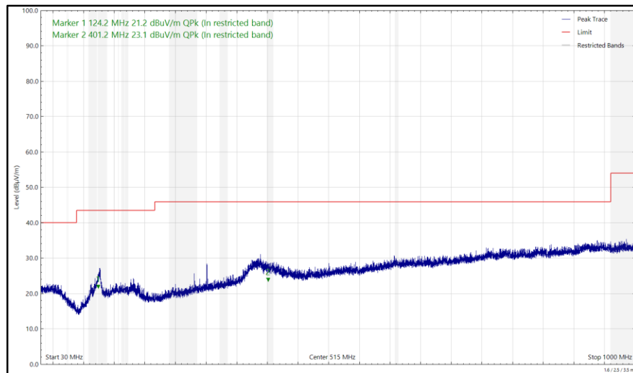
Figure 102 - 6995 MHz (CH209), HE20, SU, CDD, Core 0 + Core 1 and 2440 MHz (CH18), ePA, Core 1, 30 MHz to 1 GHz, Horizontal (Peak)
