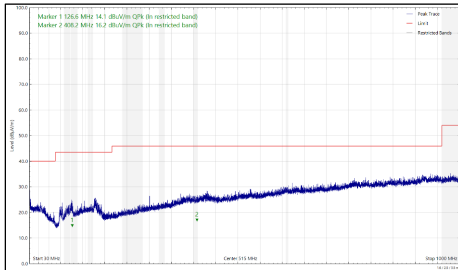
Figure 96 - 6175 MHz (CH45), HE20, SU, CDD, Core 0 + Core 1 and 2440 MHz (CH18), ePA, Core 1, 30 MHz to 1 GHz, Vertical (Peak)
