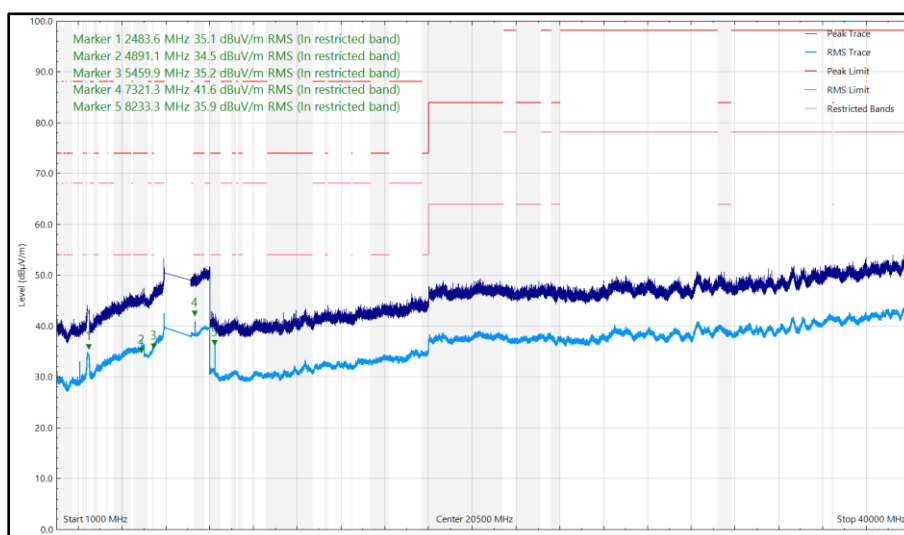
Figure 95 - 6175 MHz (CH45), HE20, SU, CDD, Core 0 + Core 1 and 2440 MHz (CH18), ePA, Core 1, 1 GHz to 40 GHz, Horizontal
