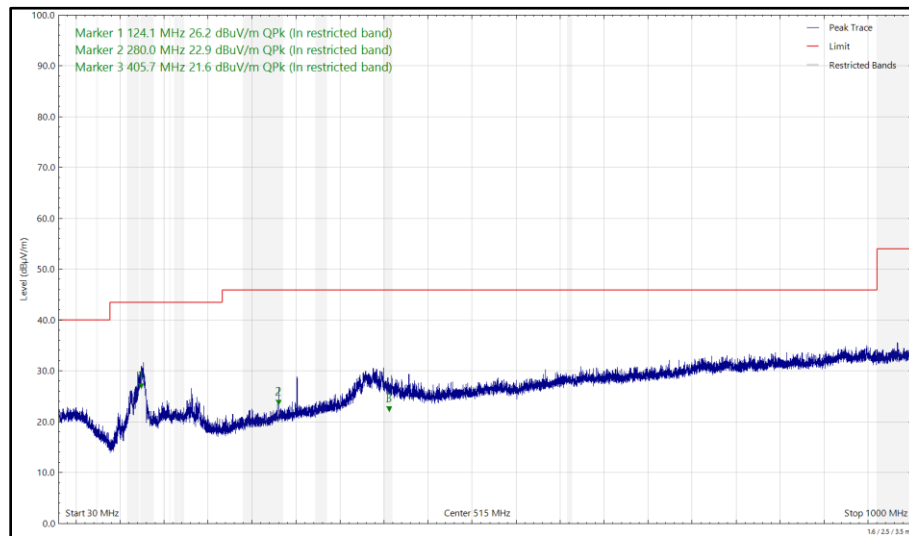
Figure 106 - 6995 MHz (CH209), HE20, SU, CDD, Core 0 + Core 1 and 2440 MHz (CH18), iPA, Core 2, 30 MHz to 1 GHz, Horizontal (Peak)
