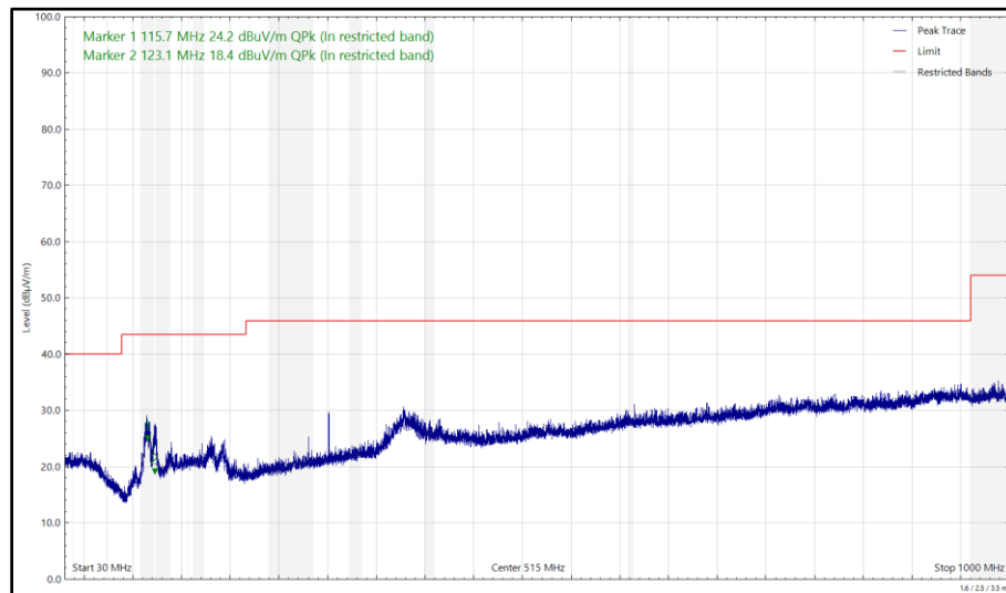
Figure 58 - 5240 MHz (CH48), HT20, CDD, Core 0 + Core 1 and 2440 MHz (CH18), ePA, Core 0, 30 MHz to 1 GHz, Horizontal (Peak)
