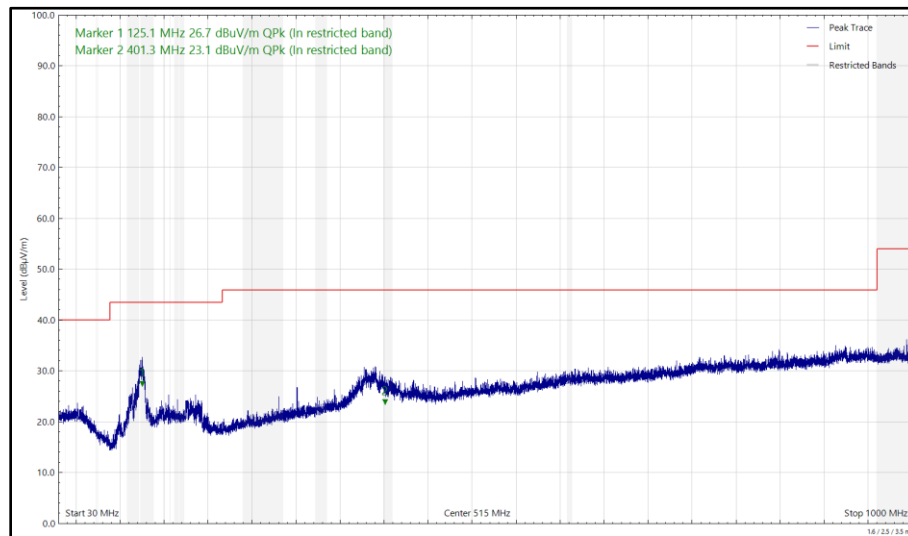
Figure 98 - 6175 MHz (CH45), HE20, SU, CDD, Core 0 + Core 1 and 2440 MHz (CH18), iPA, Core 2, 30 MHz to 1 GHz, Horizontal (Peak)
