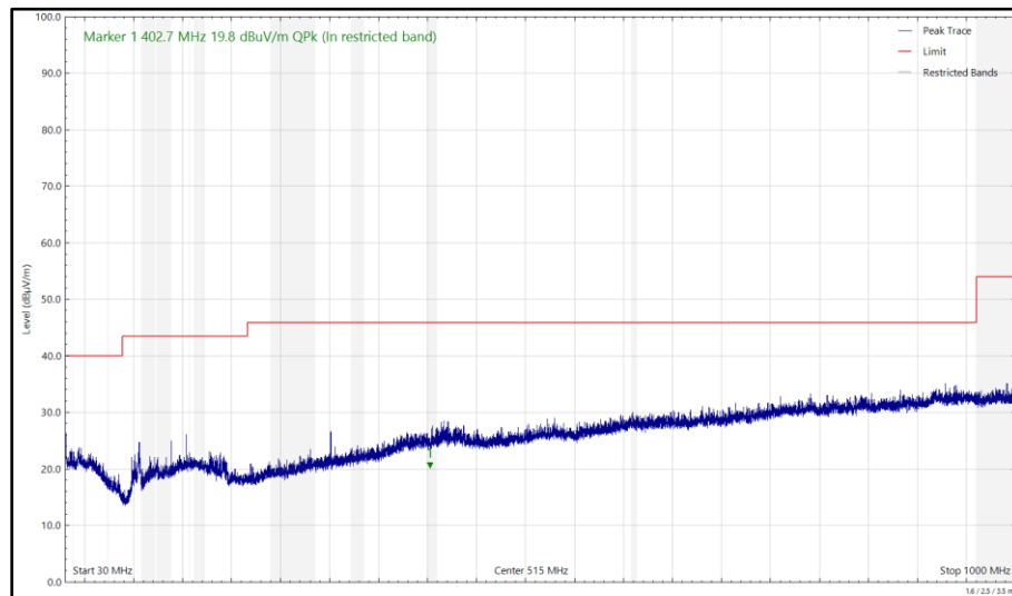
Figure 72 - 5785 MHz (CH157), HT20, CDD, Core 0 + Core 1 and 2440 MHz (CH18), iPA, Core 2, 30 MHz to 1 GHz, Vertical (Peak)
