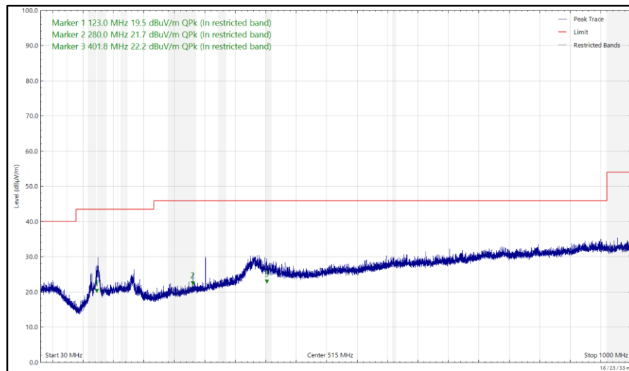
Figure 78 - 5640 MHz (CH128), HT20, CDD, Core 0 + Core 1 and 2440 MHz (CH18), ePA, Core 0, 30 MHz to 1 GHz, Horizontal (Peak)
