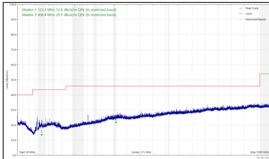
Figure 84 - 5640 MHz (CH128), HT20, CDD, Core 0 + Core 1 and 2440 MHz (CH18), ePA, Core 1, 30 MHz to 1 GHz, Vertical (Peak)
