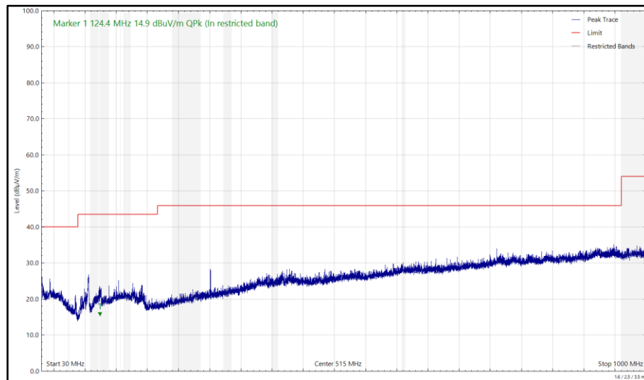
Figure 64 - 5240 MHz (CH48), HT20, CDD, Core 0 + Core 1 and 2440 MHz (CH18), iPA, Core 2, 30 MHz to 1 GHz, Vertical (Peak)
