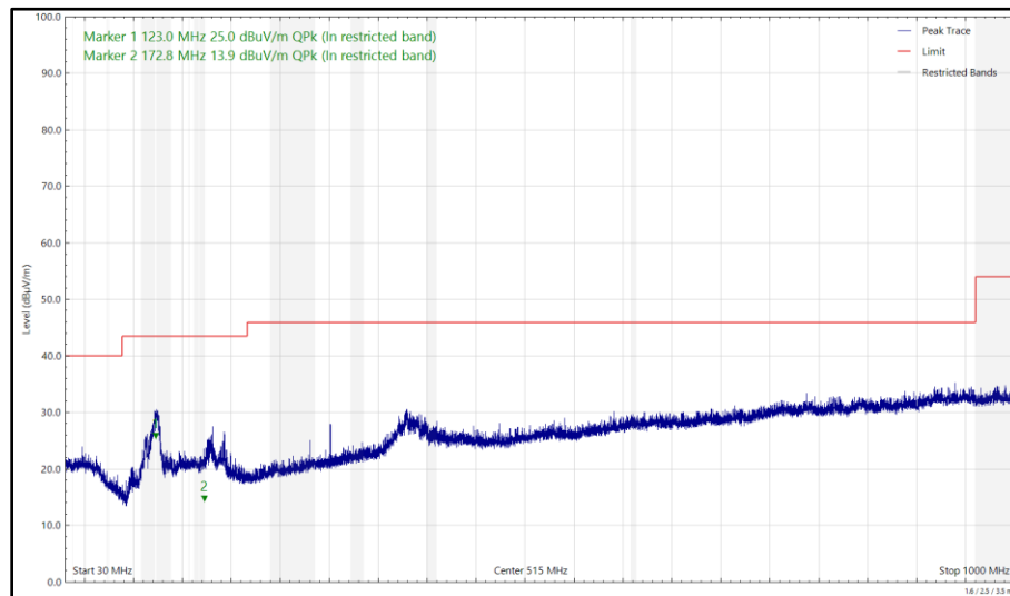
Figure 66 - 5640 MHz (CH128), HT20, CDD, Core 0 + Core 1 and 2440 MHz (CH18), iPA, Core 2, 30 MHz to 1 GHz, Horizontal (Peak)
