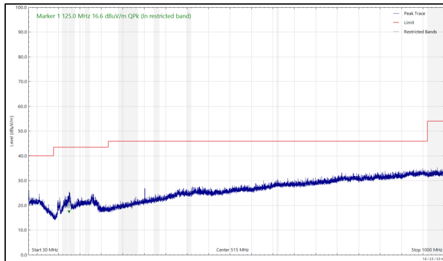
Figure 100 - 6175 MHz (CH45), HE20, SU, CDD, Core 0 + Core 1 and 2440 MHz (CH18), iPA, Core 2, 30 MHz to 1 GHz, Vertical (Peak)
