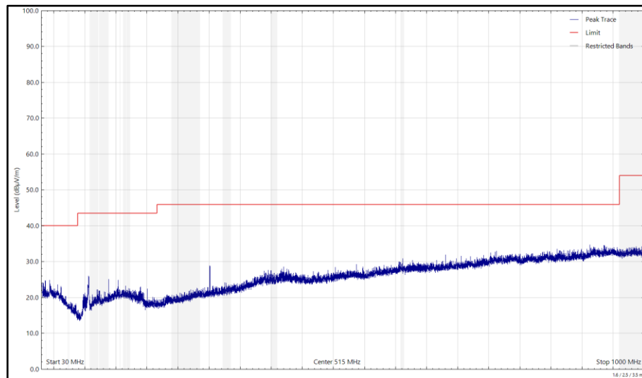
Figure 88 - 5785 MHz (CH157), HT20, CDD, Core 0 + Core 1 and 2440 MHz (CH18), ePA, Core 0, 30 MHz to 1 GHz, Vertical (Peak)
