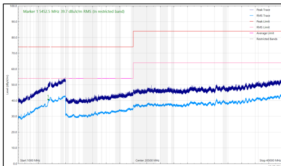
Figure 91 - 5785 MHz (CH157), HT20, CDD, Core 0 + Core 1 and 2440 MHz (CH18), ePA, Core 1, 1 GHz to 40 GHz, Horizontal
