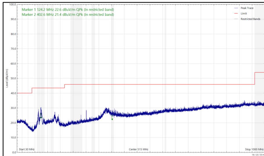
Figure 74 - 5240 MHz (CH48), HT20, CDD, Core 0 + Core 1 and 2440 MHz (CH18), ePA, Core 1, 30 MHz to 1 GHz, Horizontal (Peak)
