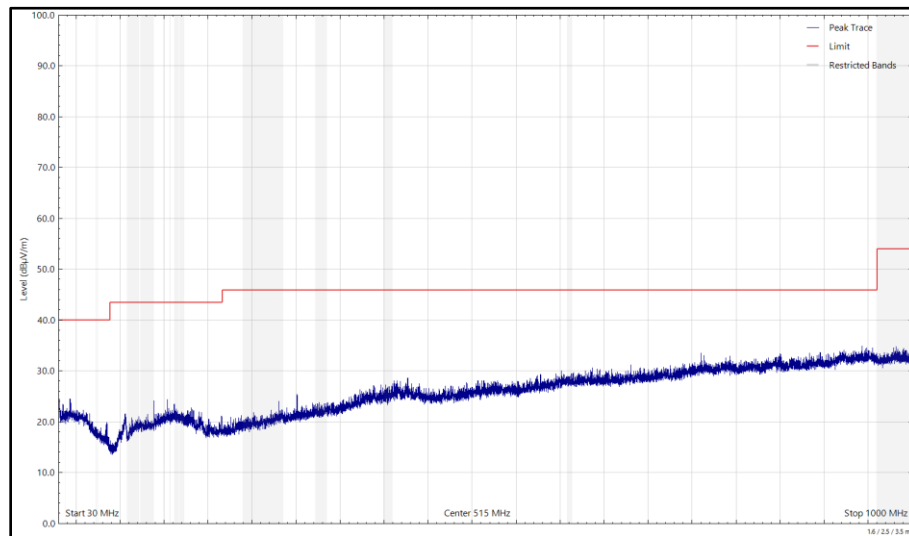
Figure 92 - 5785 MHz (CH157), HT20, CDD, Core 0 + Core 1 and 2440 MHz (CH18), ePA, Core 1, 30 MHz to 1 GHz, Vertical (Peak)
