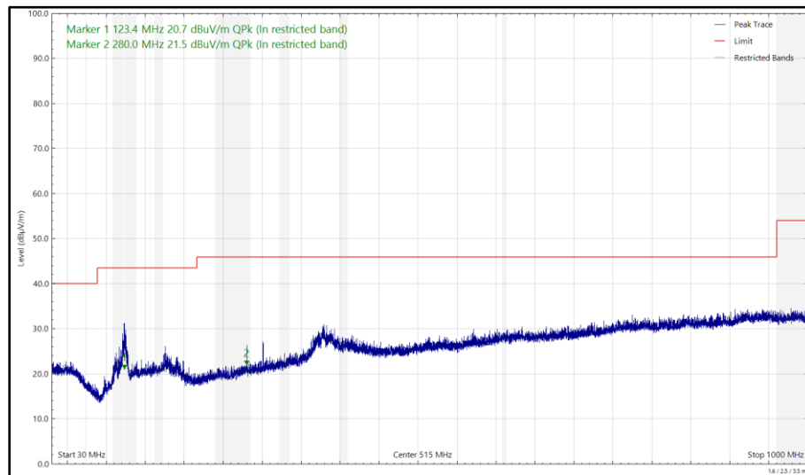
Figure 82 - 5640 MHz (CH128), HT20, CDD, Core 0 + Core 1 and 2440 MHz (CH18), ePA, Core 1, 30 MHz to 1 GHz, Horizontal (Peak)
