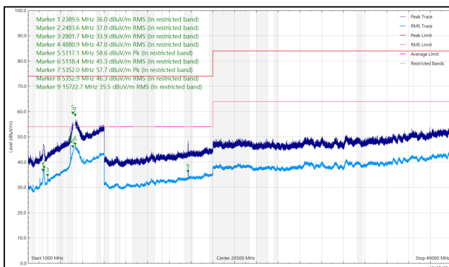
Figure 61 - 5240 MHz (CH48), HT20, CDD, Core 0 + Core 1 and 2440 MHz (CH18), ePA, Core 0, 1 GHz to 40 GHz, Vertical
