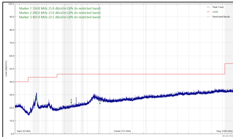
Figure 110 - 6175 MHz (CH45), HE20, SU, CDD, Core 0 + Core 1 and 2440 MHz (CH18), ePA, Core 0, 30 MHz to 1 GHz, Horizontal (Peak)
