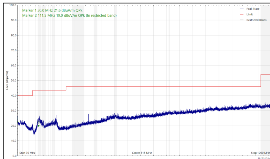
Figure 56 - 2442MHz (CH7), HT20, Core 1 and 5788MHz (CH5788), DH5, ePA, Core 0, 30 MHz to 1 GHz, Vertical (Peak)
