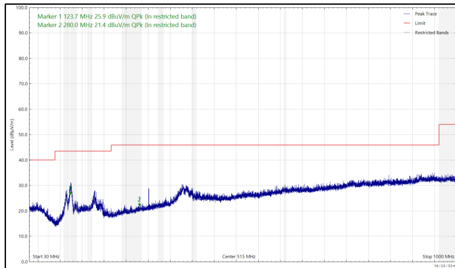
Figure 62 - 5240 MHz (CH48), HT20, CDD, Core 0 + Core 1 and 2440 MHz (CH18), iPA, Core 2, 30 MHz to 1 GHz, Horizontal (Peak)
