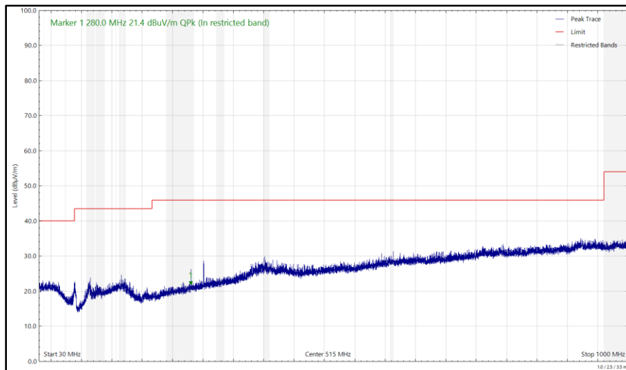
Figure 54 - 2442MHz (CH7), HT20, Core 1 and 5788MHz (CH5788), DH5, ePA, Core 0, 30 MHz to 1 GHz, Horizontal (Peak)
