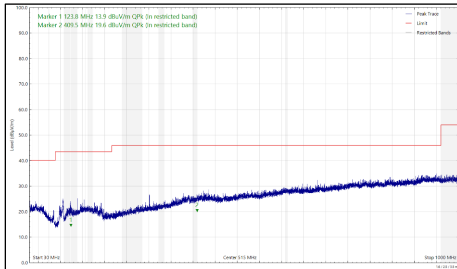
Figure 68 - 5640 MHz (CH128), HT20, CDD, Core 0 + Core 1 and 2440 MHz (CH18), iPA, Core 2, 30 MHz to 1 GHz, Vertical (Peak)
