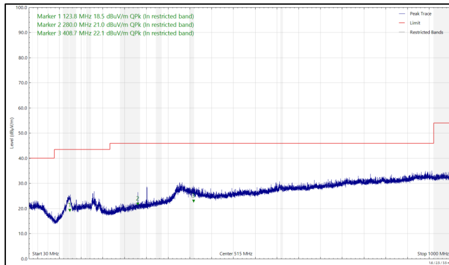
Figure 86 - 5785 MHz (CH157), HT20, CDD, Core 0 + Core 1 and 2440 MHz (CH18), ePA, Core 0, 30 MHz to 1 GHz, Horizontal (Peak)
