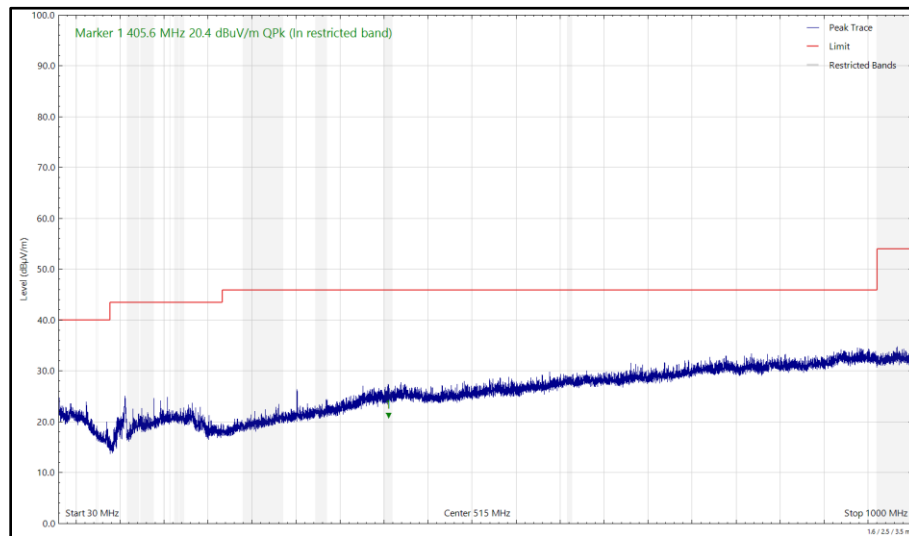
Figure 80 - 5640 MHz (CH128), HT20, CDD, Core 0 + Core 1 and 2440 MHz (CH18), ePA, Core 0, 30 MHz to 1 GHz, Vertical (Peak)
