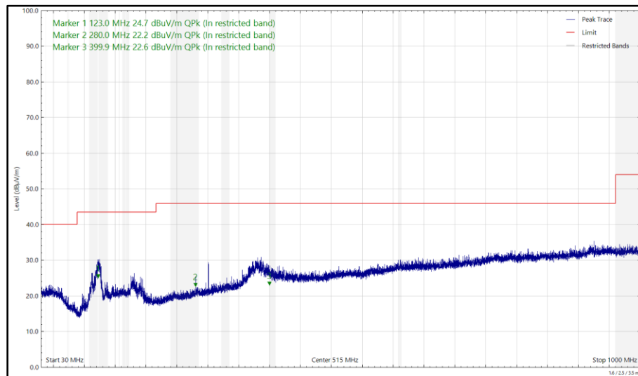
Figure 70 - 5785 MHz (CH157), HT20, CDD, Core 0 + Core 1 and 2440 MHz (CH18), iPA, Core 2, 30 MHz to 1 GHz, Horizontal (Peak)
