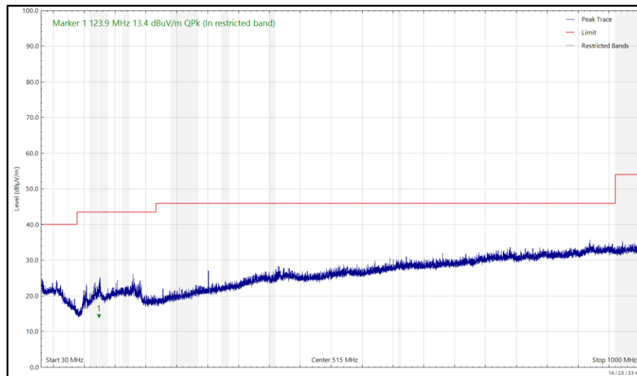
Figure 104 - 6995 MHz (CH209), HE20, SU, CDD, Core 0 + Core 1 and 2440 MHz (CH18), ePA, Core 1, 30 MHz to 1 GHz, Vertical (Peak)
