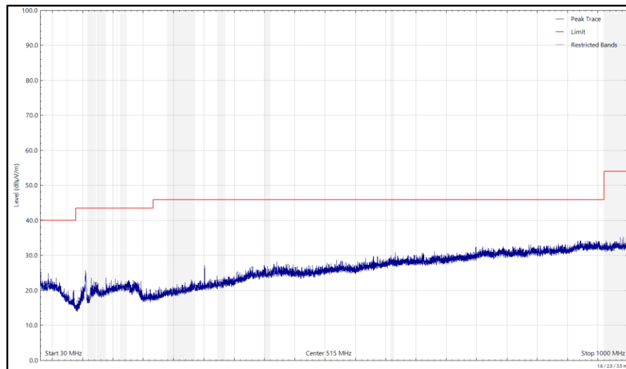
Figure 76 - 5240 MHz (CH48), HT20, CDD, Core 0 + Core 1 and 2440 MHz (CH18), ePA, Core 1, 30 MHz to 1 GHz, Vertical (Peak)
