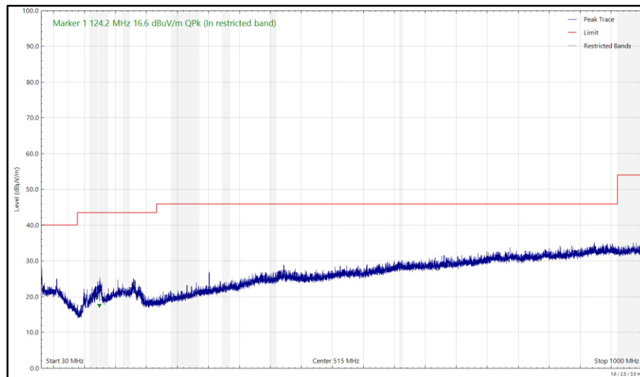
Figure 108 - 6995 MHz (CH209), HE20, SU, CDD, Core 0 + Core 1 and 2440 MHz (CH18), iPA, Core 2, 30 MHz to 1 GHz, Vertical (Peak)
