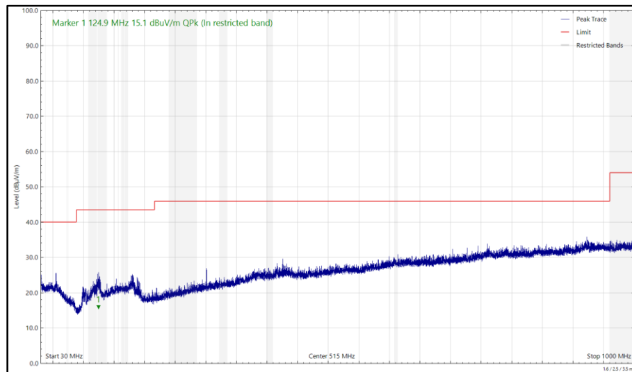
Figure 116 - 6995 MHz (CH209), HE20, SU, CDD, Core 0 + Core 1 and 2440 MHz (CH18), ePA, Core 0, 30 MHz to 1 GHz, Vertical (Peak)
