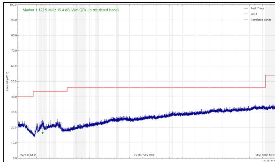
Figure 112 - 6175 MHz (CH45), HE20, SU, CDD, Core 0 + Core 1 and 2440 MHz (CH18), ePA, Core 0, 30 MHz to 1 GHz, Vertical (Peak)
