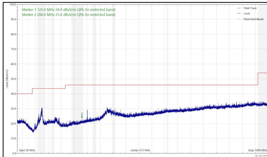
Figure 114 - 6995 MHz (CH209), HE20, SU, CDD, Core 0 + Core 1 and 2440 MHz (CH18), ePA, Core 0, 30 MHz to 1 GHz, Horizontal (Peak)
