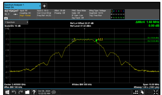
Figure 30 - Core 0 (A) 2405 MHz (CH11) 6 dB Bandwidth
