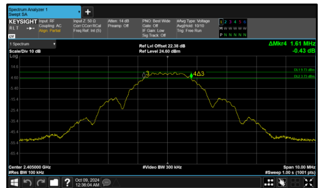
Figure 18 - Core 1 (B) 2405 MHz (CH11) 6 dB Bandwidth
