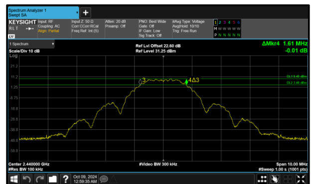
Figure 26 - Core 2 (C) 2440 MHz (CH18) 6 dB Bandwidth
