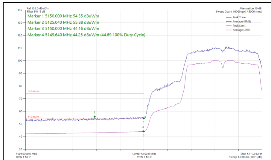
Figure 46 - 802.11n HT40, SISO, Core 0 - 5190 MHz Band Edge Frequency 5150 MHz
