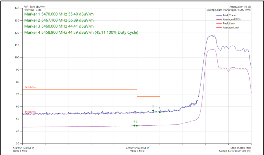
Figure 24 - 802.11ax HE20, RU 52-37, SISO, Core 1 - 5500 MHz Band Edge Frequency 5460 MHz
