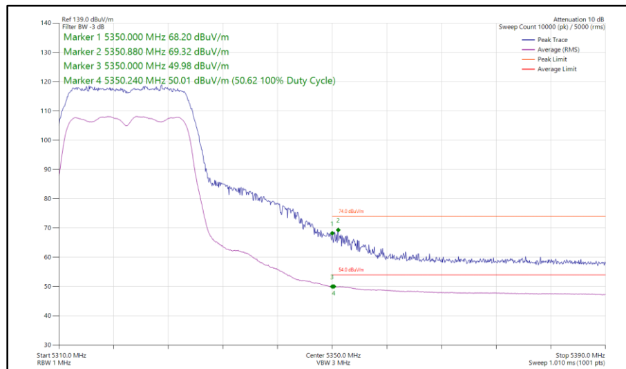
Figure 37 - 802.11n HT20, SDM, Core 0 - Core 1 - 5320 MHz Band Edge Frequency 5350 MHz
