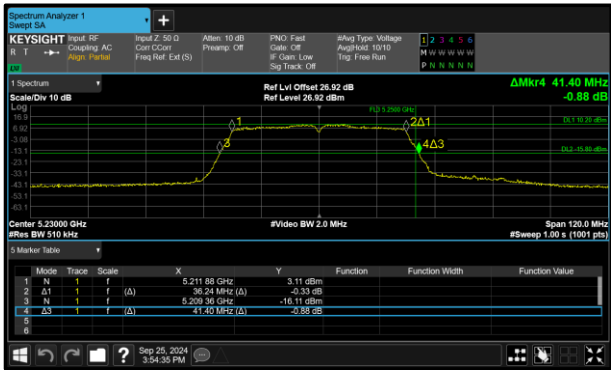
Figure 206 - 802.11n HT40 Minimum 99% OBW
