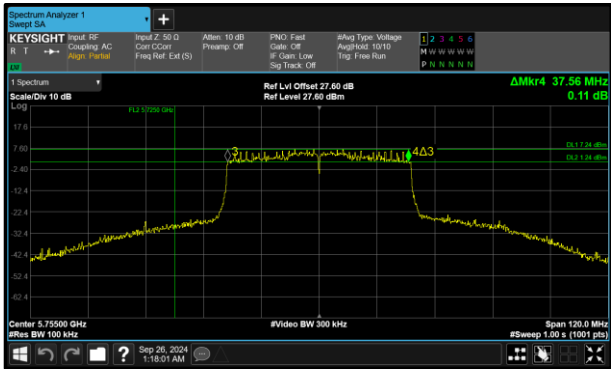
Figure 228 - 802.11ax HE40 SU Minimum 6 dB EBW
