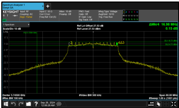
Figure 220 - 802.11n HT20 Minimum 6 dB EBW
