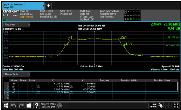
Figure 204 - 802.11n HT20 Minimum 99% OBW
