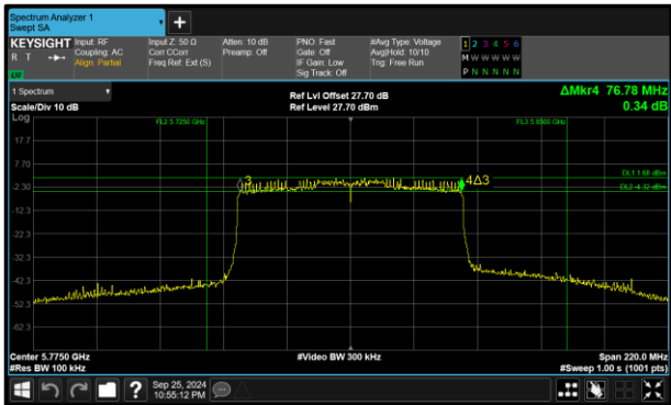
Figure 202 - 802.11ax HE80 SU Minimum 6 dB EBW
