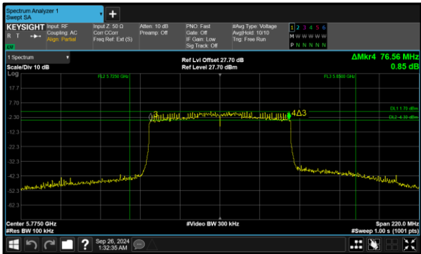
Figure 230 - 802.11ax HE80 SU Minimum 6 dB EBW
