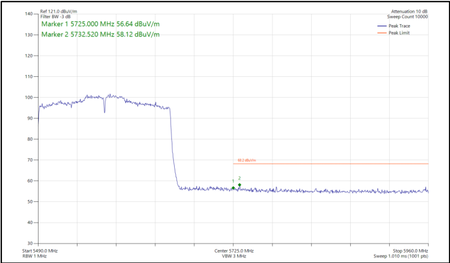
Figure 442 - 802.11ax HE160, SU, SISO, Core 1 - 5570 MHz Band Edge Frequency 5725 MHz
