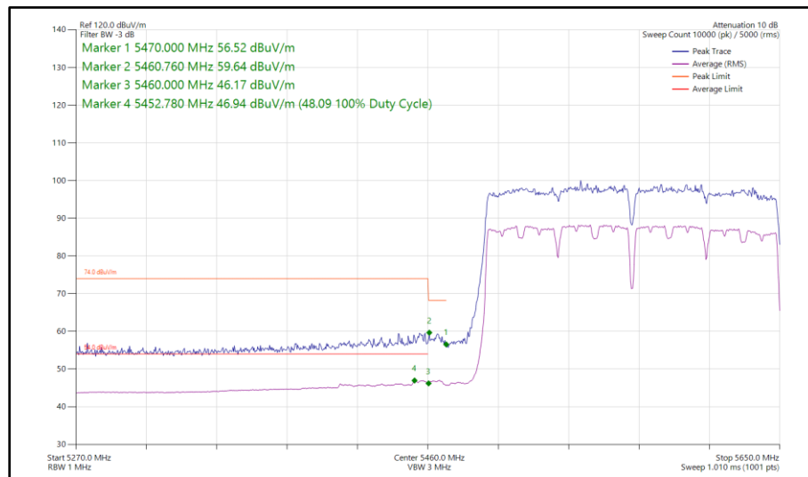
Figure 438 - 802.11ac VHT160, SISO, Core 1 - 5570 MHz Band Edge Frequency 5470 MHz
