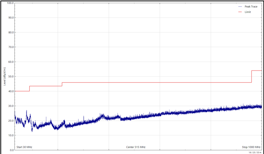
Figure 459 - U-NII-1 - 5180 MHz (CH36), 802.11a, Core 0, 30 MHz to 1 GHz, Vertical (Peak)
