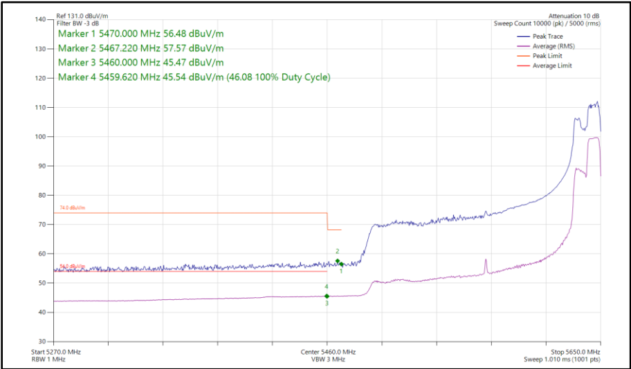
Figure 434 - 802.11ax HE160, RU 106-60S, SISO, Core 0 - 5570 MHz Band Edge Frequency 5470 MHz
