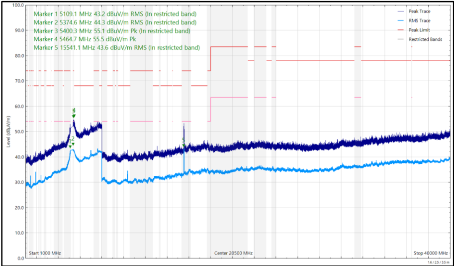
Figure 460 - U-NII-1 - 5180 MHz (CH36), 802.11a, Core 0, 1 GHz to 40 GHz, Vertical
