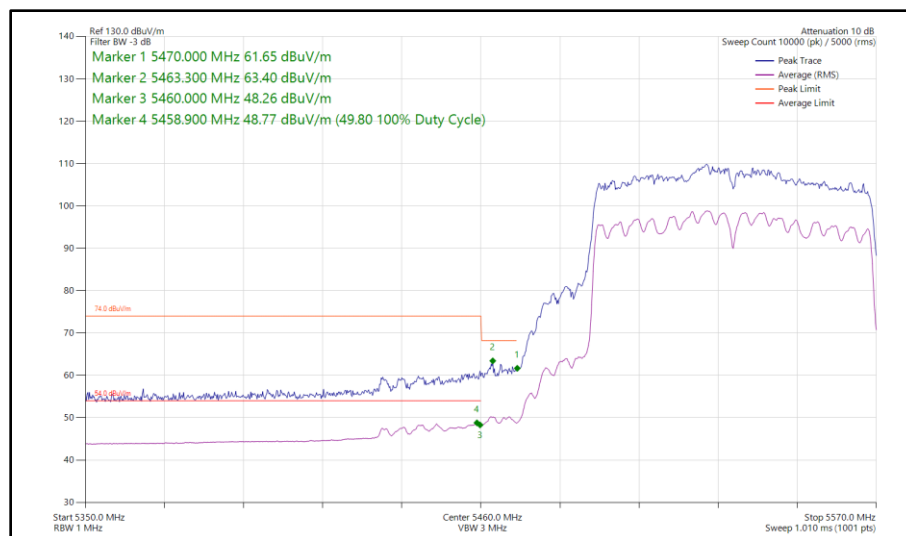
Figure 412 - 802.11ac VHT80, SDM, Core 0 - Core 1 - 5530 MHz Band Edge Frequency 5470 MHz
