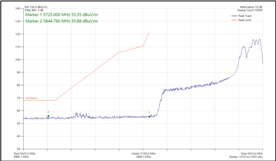
Figure 405 - 802.11ax HE80, RU 106-60, CDD, Core 0 - Core 1 - 5775 MHz Band Edge Frequency 5725 MHz
