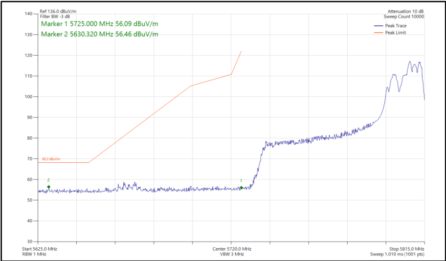
Figure 417 - 802.11ax HE80, RU 106-60, SDM, Core 0 - Core 1 - 5775 MHz Band Edge Frequency 5725 MHz
