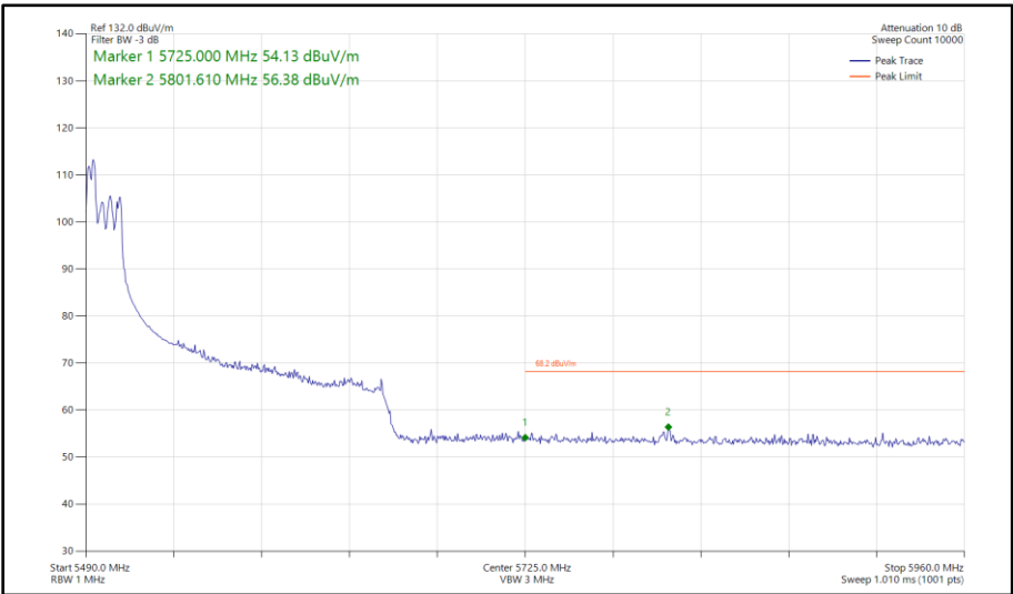
Figure 449 - 802.11ax HE160, RU 52-37P, CDD, Core 0 - Core 1 - 5570 MHz Band Edge Frequency 5725 MHz
