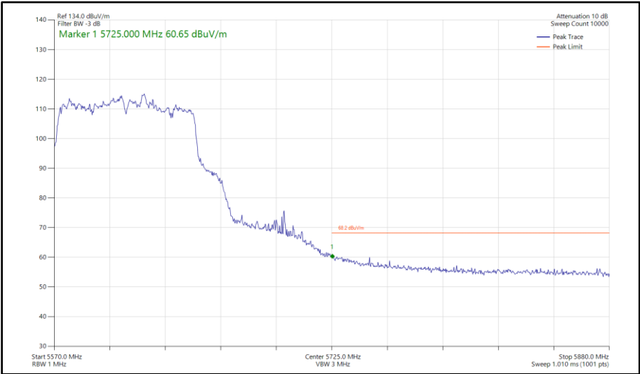
Figure 428 - 802.11ac VHT80, TxBF, Core 0 - Core 1 - 5610 MHz Band Edge Frequency 5725 MHz
