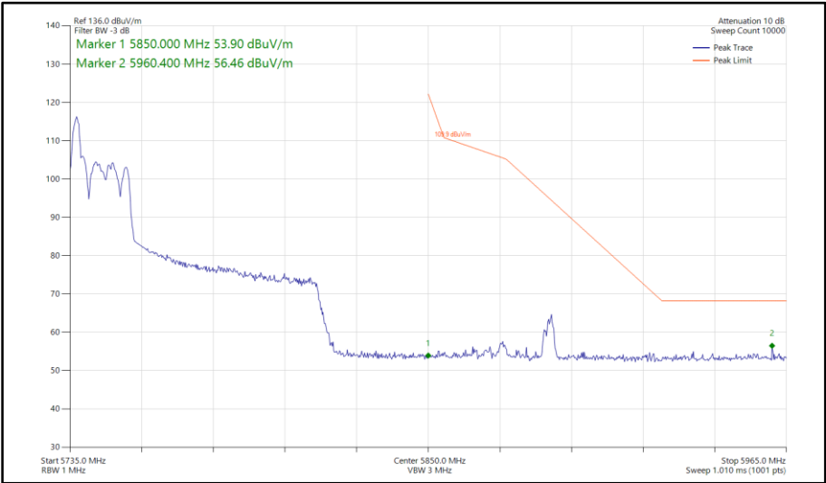
Figure 411 - 802.11ax HE80, RU 26-0, CDD, Core 0 - Core 1 - 5775 MHz Band Edge Frequency 5850 MHz
