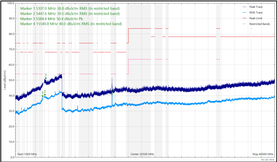
Figure 458 - U-NII-1 - 5180 MHz (CH36), 802.11a, Core 0, 1 GHz to 40 GHz, Horizontal
