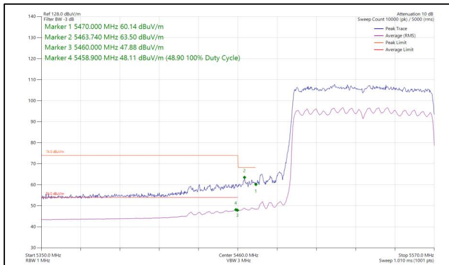
Figure 413 - 802.11ax HE80, SU, SDM, Core 0 - Core 1 - 5530 MHz Band Edge Frequency 5470 MHz
