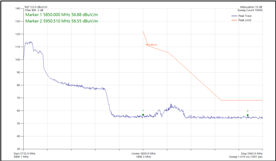
Figure 399 - 802.11ax HE80, RU 106-53, SISO, Core 1 - 5775 MHz Band Edge Frequency 5850 MHz
