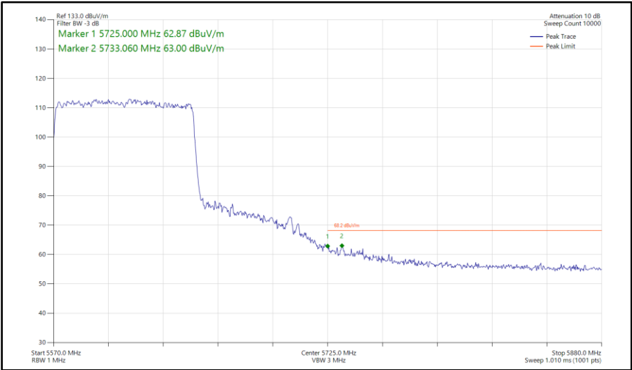
Figure 419 - 802.11ax HE80, SU, SDM, Core 0 - Core 1 - 5610 MHz Band Edge Frequency 5725 MHz
