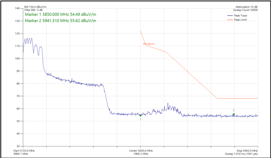
Figure 423 - 802.11ax HE80, RU 106-53, SDM, Core 0 - Core 1 - 5775 MHz Band Edge Frequency 5850 MHz
