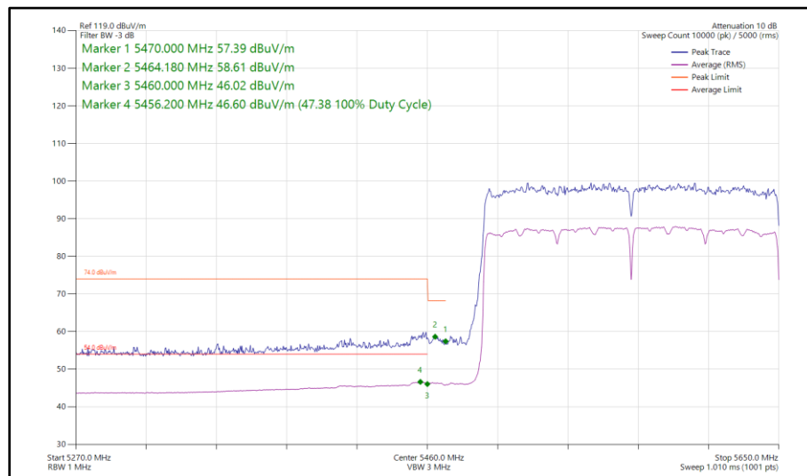
Figure 439 - 802.11ax HE160, SU, SISO, Core 1 - 5570 MHz Band Edge Frequency 5470 MHz
