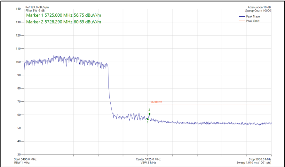
Figure 448 - 802.11ax HE160, SU, CDD, Core 0 - Core 1 - 5570 MHz Band Edge Frequency 5725 MHz
