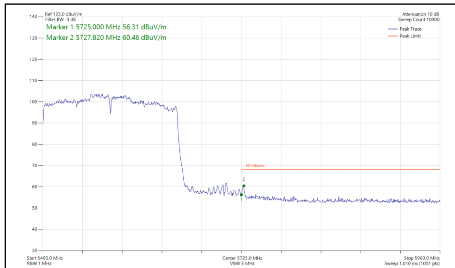
Figure 454 - 802.11ax HE160, SU, SDM, Core 0 - Core 1 - 5570 MHz Band Edge Frequency 5725 MHz
