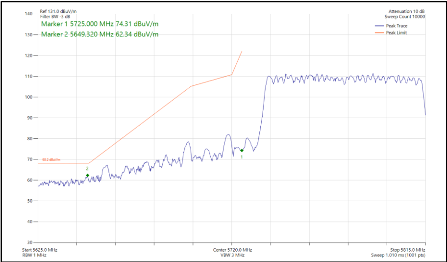
Figure 403 - 802.11ac VHT80, CDD, Core 0 - Core 1 - 5775 MHz Band Edge Frequency 5725 MHz
