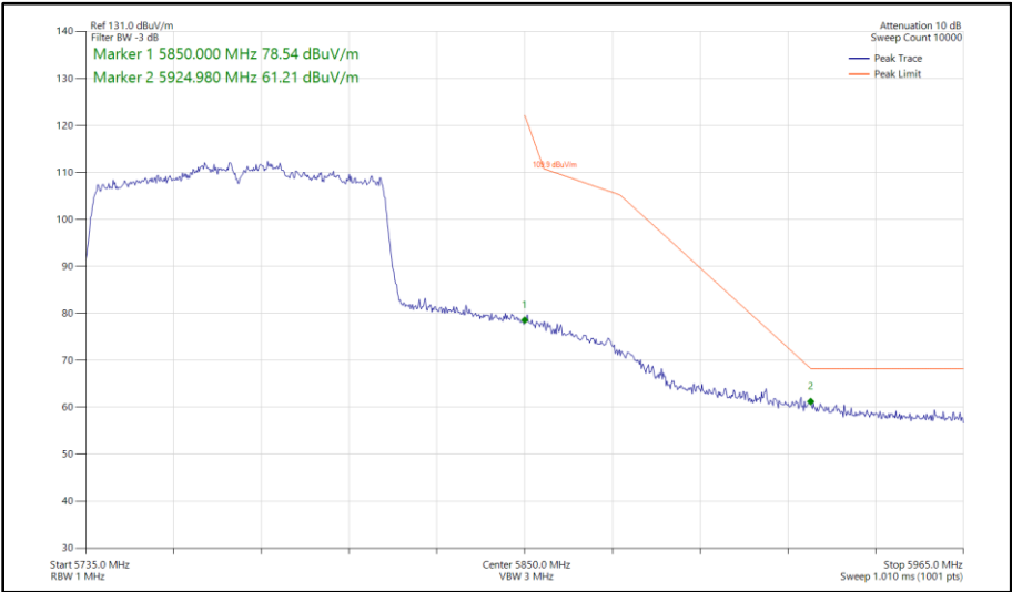
Figure 397 - 802.11ac VHT80, SISO, Core 1 - 5775 MHz Band Edge Frequency 5850 MHz
