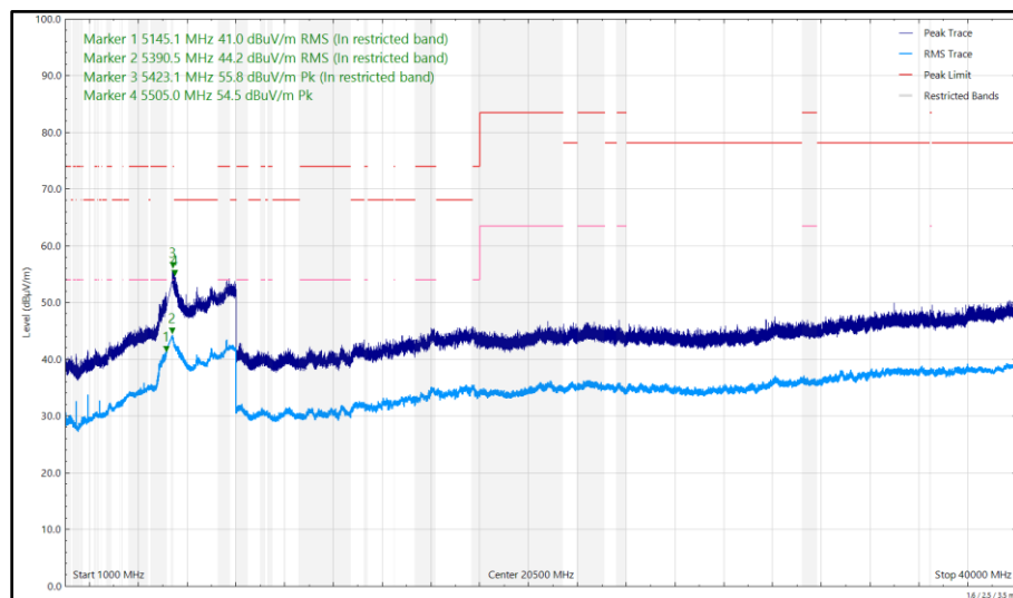
Figure 498 - U-NII-2A - 5320 MHz (CH64), 802.11a, Core 1, 1 GHz to 40 GHz, Vertical
