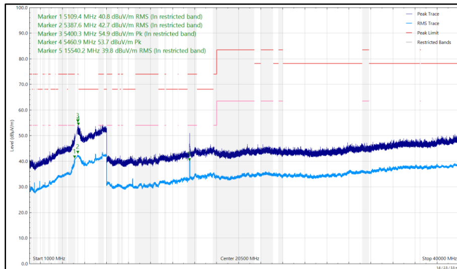
Figure 474 - U-NII-1 - 5180 MHz (CH36), HT20, CDD, Core 0 + Core 1, 1 GHz to 40 GHz, Horizontal
