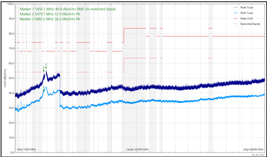
Figure 504 - U-NII-3 - 5745 MHz (CH149), 802.11a, Core 1, 1 GHz to 40 GHz, Vertical
