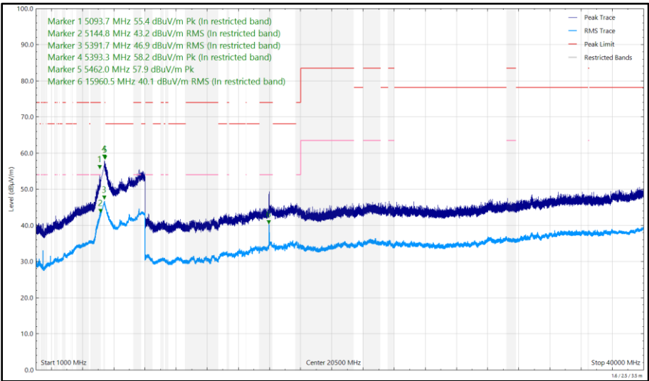
Figure 520 - U-NII-2A - 5320 MHz (CH64), HT20, CDD, Core 0 + Core 1, 1 GHz to 40 GHz, Vertical
