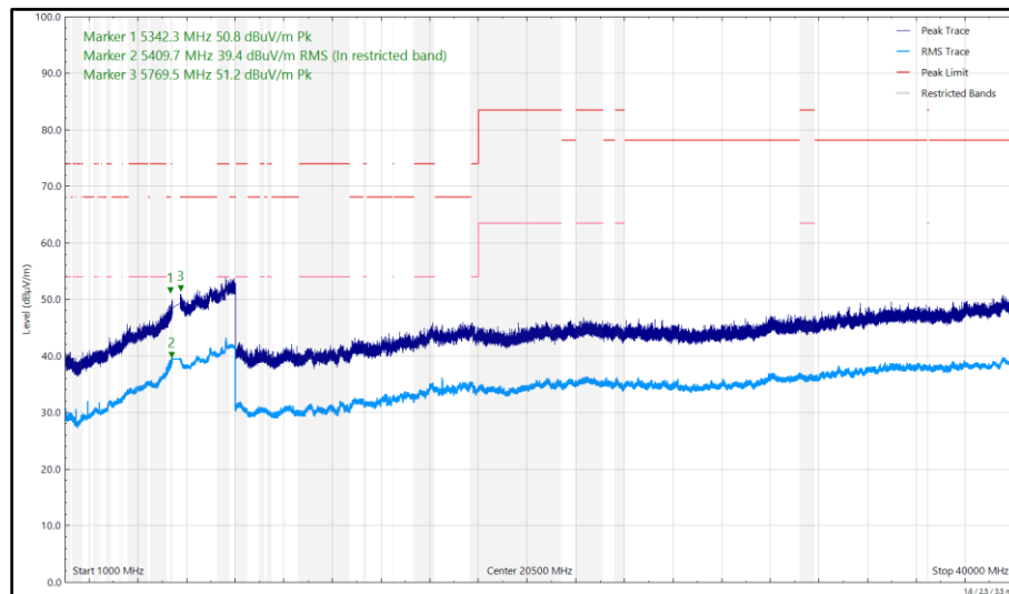
Figure 491 - U-NII-2C - 5500 MHz (CH100), 802.11a, Core 0, 1 GHz to 40 GHz, Horizontal
