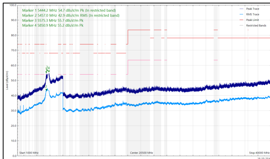
Figure 496 - U-NII-3 - 5745 MHz (CH149), 802.11a, Core 0, 1 GHz to 40 GHz, Vertical
