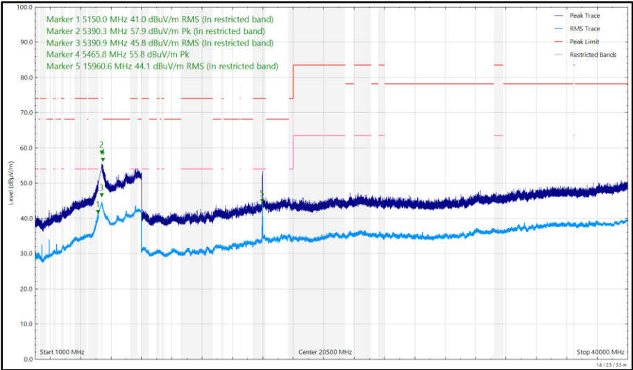
Figure 490 - U-NII-2A - 5320 MHz (CH64), 802.11a, Core 0, 1 GHz to 40 GHz, Vertical
