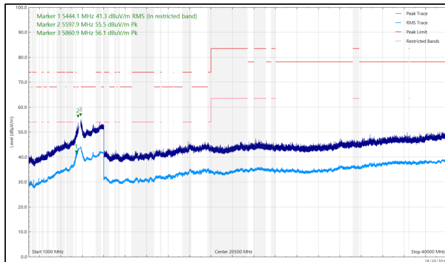
Figure 509 - U-NII-3 - 5745 MHz (CH149), HT20, CDD, Core 0 + Core 1, 1 GHz to 40 GHz, Horizontal
