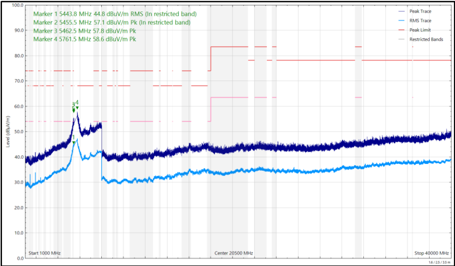
Figure 508 - U-NII-2C - 5700 MHz (CH140), HT20, CDD, Core 0 + Core 1, 1 GHz to 40 GHz, Vertical
