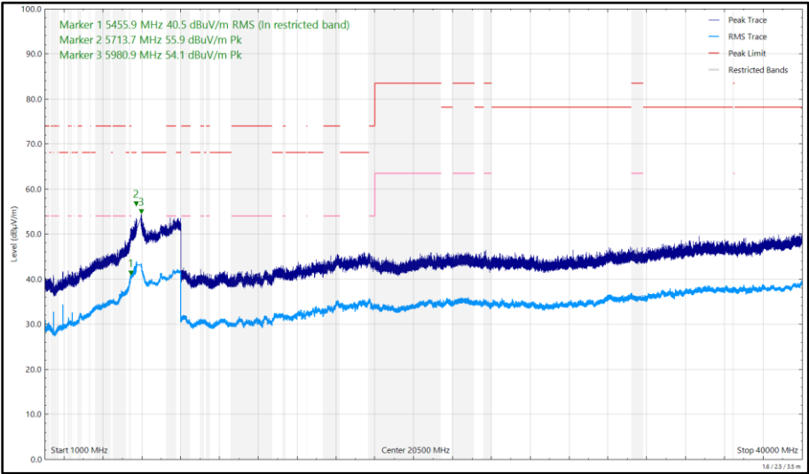
Figure 472 - U-NII-3 - 5825 MHz (CH165), 802.11a, Core 1, 1 GHz to 40 GHz, Vertical
