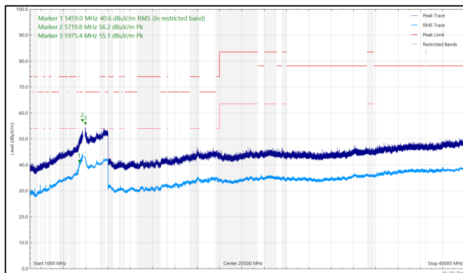
Figure 478 - U-NII-3 - 5825 MHz (CH165), HT20, CDD, Core 0 + Core 1, 1 GHz to 40 GHz, Horizontal
