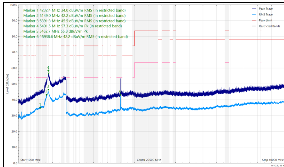
Figure 518 - U-NII-2A - 5320 MHz (CH64), HE20, RU52-37, CDD, Core 0 + Core 1, 1 GHz to 40 GHz, Vertical
