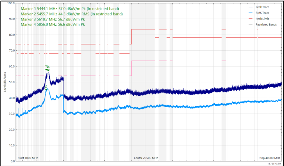
Figure 510 - U-NII-3 - 5745 MHz (CH149), HT20, CDD, Core 0 + Core 1, 1 GHz to 40 GHz, Vertical
