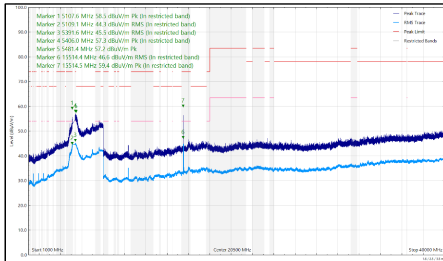
Figure 484 - U-NII-1 - 5180 MHz (CH36), HE20, RU26-0, CDD, Core 0 + Core 1, 1 GHz to 40 GHz, Vertical
