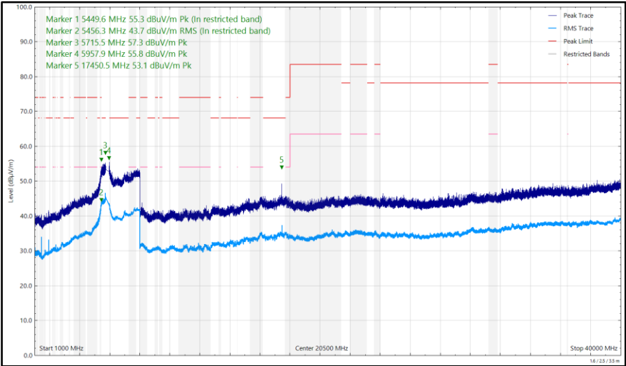
Figure 488 - U-NII-3 - 5825 MHz (CH165), HE20, RU26-0, CDD, Core 0 + Core 1, 1 GHz to 40 GHz, Vertical
