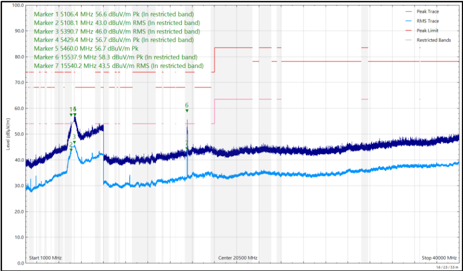
Figure 476 - U-NII-1 - 5180 MHz (CH36), HT20, CDD, Core 0 + Core 1, 1 GHz to 40 GHz, Vertical
