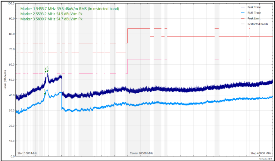
Figure 503 - U-NII-3 - 5745 MHz (CH149), 802.11a, Core 1, 1 GHz to 40 GHz, Horizontal
