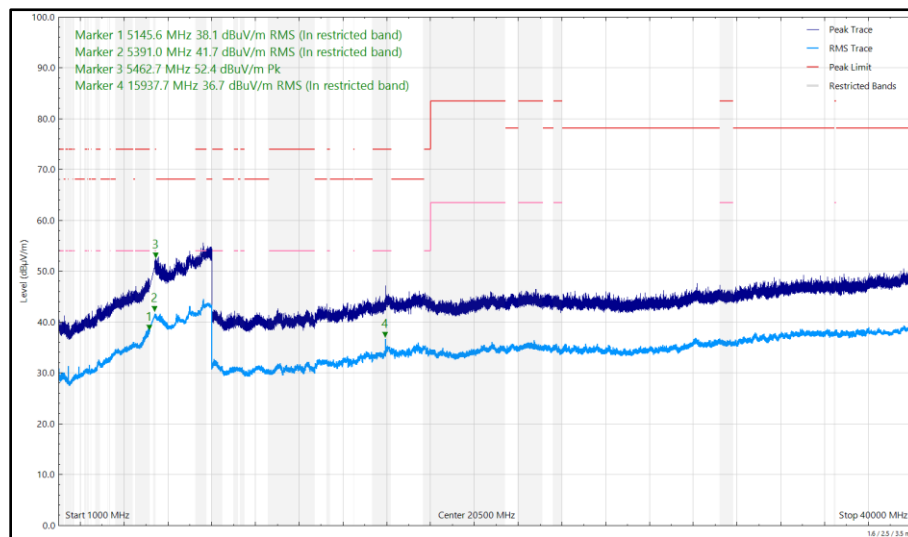
Figure 517 - U-NII-2A - 5320 MHz (CH64), HE20, RU52-37, CDD, Core 0 + Core 1, 1 GHz to 40 GHz, Horizontal
