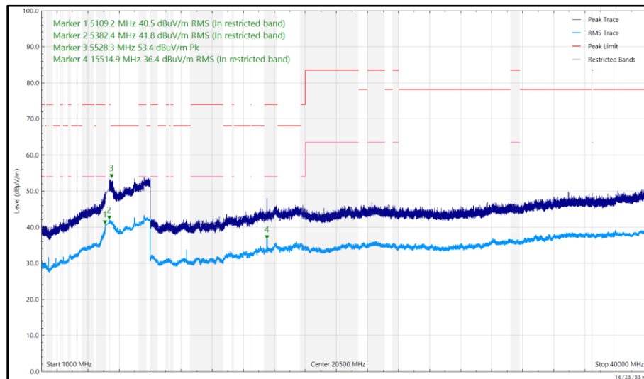
Figure 482 - U-NII-1 - 5180 MHz (CH36), HE20, RU26-0, CDD, Core 0 + Core 1, 1 GHz to 40 GHz, Horizontal
