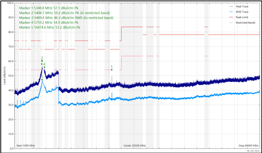
Figure 512 - U-NII-2C - 5500 MHz (CH100), HE20, RU52-37, CDD, Core 0 + Core 1, 1 GHz to 40 GHz, Vertical
