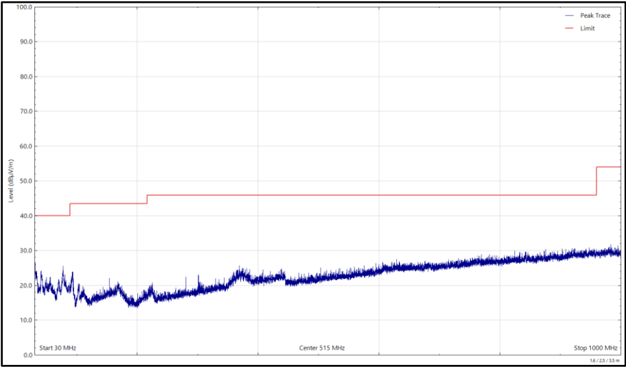
Figure 471 - U-NII-3 - 5825 MHz (CH165), 802.11a, Core 1, 30 MHz to 1 GHz, Vertical (Peak)
