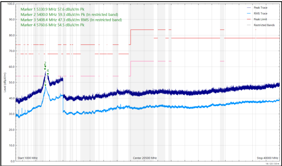
Figure 506 - U-NII-2C - 5500 MHz (CH100), HT20, CDD, Core 0 + Core 1, 1 GHz to 40 GHz, Vertical
