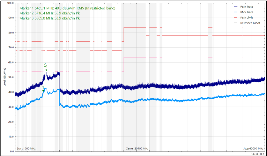
Figure 486 - U-NII-3 - 5825 MHz (CH165), HE20, RU26-0, CDD, Core 0 + Core 1, 1 GHz to 40 GHz, Horizontal
