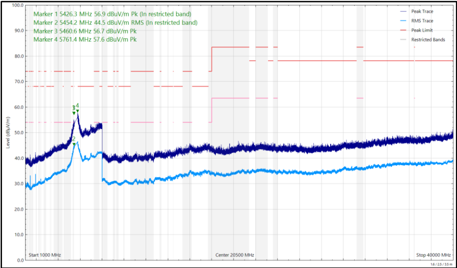
Figure 514 - U-NII-2C - 5700 MHz (CH140), HE20, RU52-37, CDD, Core 0 + Core 1, 1 GHz to 40 GHz, Vertical
