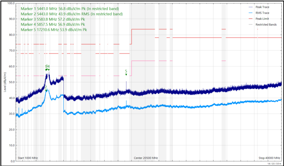
Figure 516 - U-NII-3 - 5745 MHz (CH149), HE20, RU26-0, CDD, Core 0 + Core 1, 1 GHz to 40 GHz, Vertical
