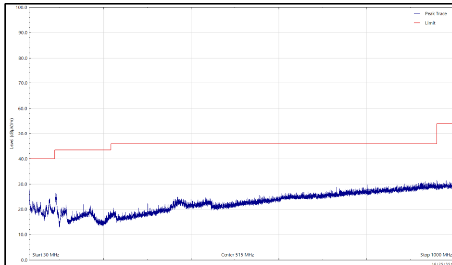
Figure 479 - U-NII-3 - 5825 MHz (CH165), HT20, CDD, Core 0 + Core 1, 30 MHz to 1 GHz, Vertical (Peak)
