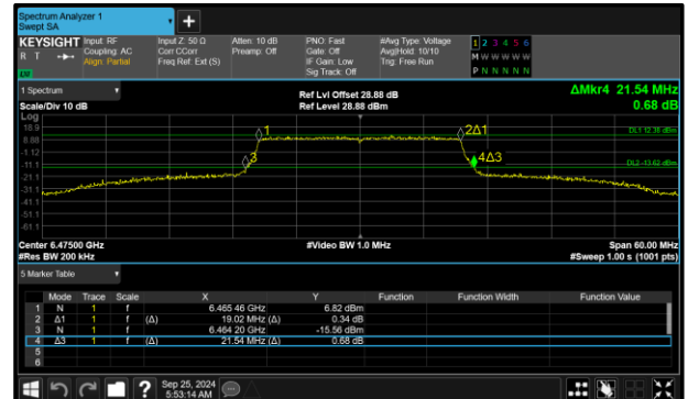
Figure 24 - 802.11ax HE20 SU SP Maximum 26 dB EBW
