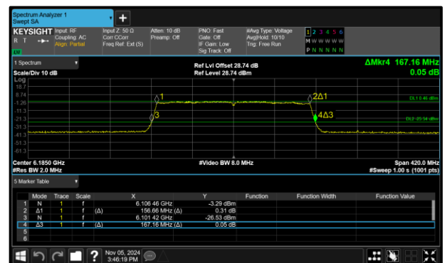
Figure 50 - 802.11ax HE160 SU VLP Maximum 99% OBW
