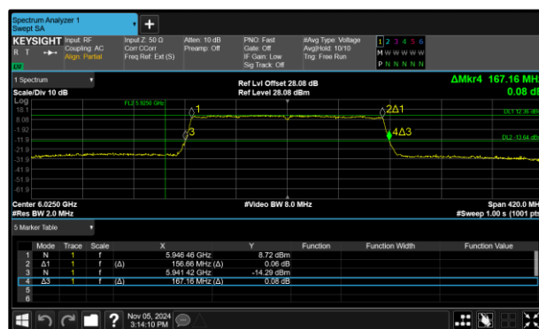
Figure 60 - 802.11ax HE160 SU SP Maximum 99% OBW
