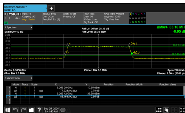
Figure 72 - 802.11ax HE80 SU VLP Maximum 26 dB EBW
