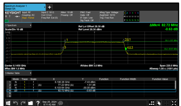
Figure 18 - 802.11ax HE80 SU VLP Maximum 26 dB EBW
