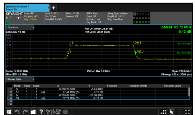
Figure 48 - 802.11ax HE80 SU VLP Maximum 99% OBW
