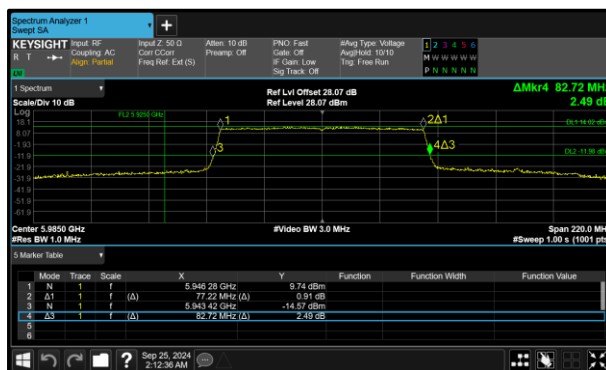
Figure 27 - 802.11ax HE80 SU SP Minimum 26 dB EBW
