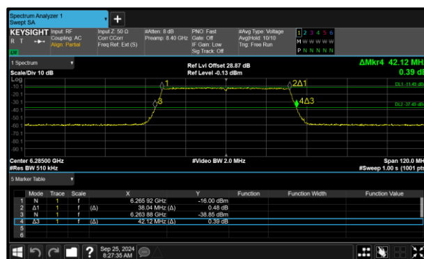
Figure 70 - 802.11ax HE40 SU VLP Maximum 26 dB EBW
