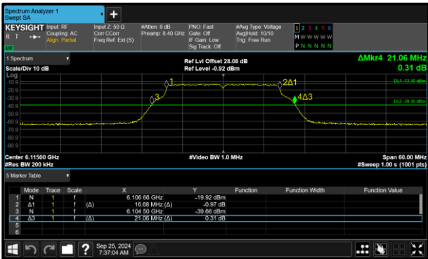
Figure 41 - 802.11a VLP Minimum 99% OBW
