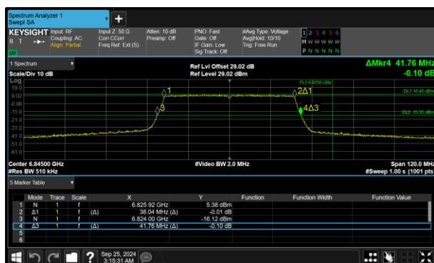
Figure 77 - 802.11ax HE40 SU SP Minimum 26 dB EBW
