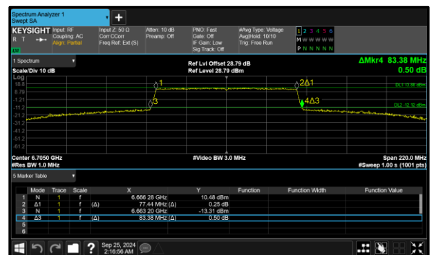
Figure 28 - 802.11ax HE80 SU SP Maximum 26 dB EBW
