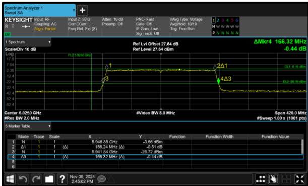
Figure 67 - 802.11ax HE160 SU LPI Minimum 26 dB EBW
