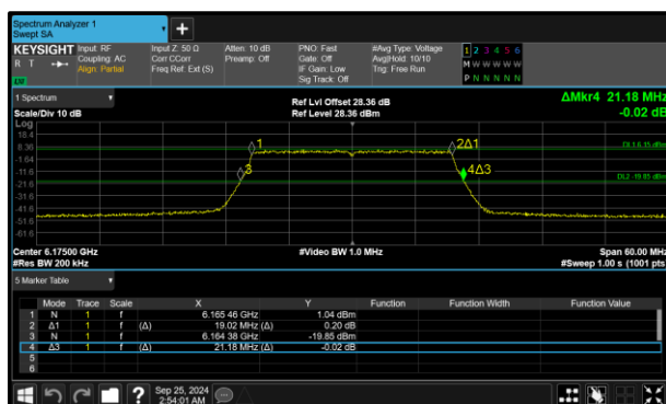
Figure 75 - 802.11ax HE20 SU SP Minimum 26 dB EBW
