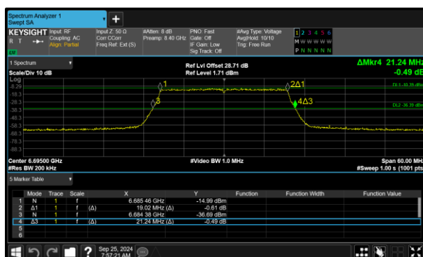
Figure 13 - 802.11ax HE20 SU VLP Minimum 26 dB EBW
