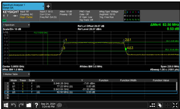
Figure 65 - 802.11ax HE80 SU LPI Minimum 26 dB EBW
