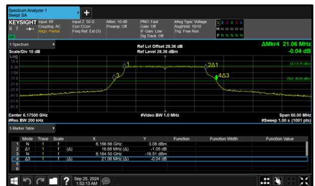
Figure 52 - 802.11a SP Maximum 99% OBW
