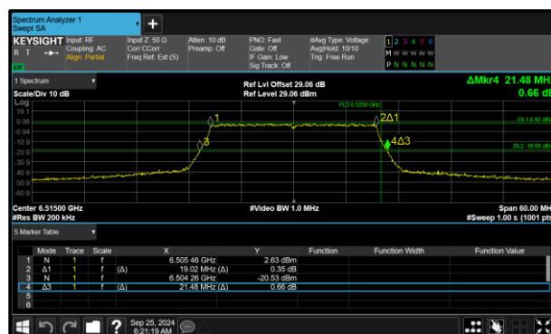
Figure 76 - 802.11ax HE20 SU SP Maximum 26 dB EBW
