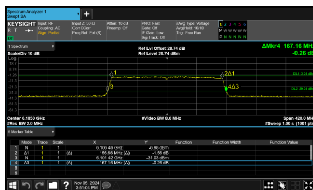
Figure 74 - 802.11ax HE160 SU VLP Maximum 26 dB EBW
