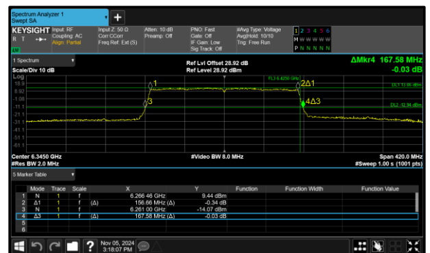
Figure 30 - 802.11ax HE160 SU SP Maximum 26 dB EBW
