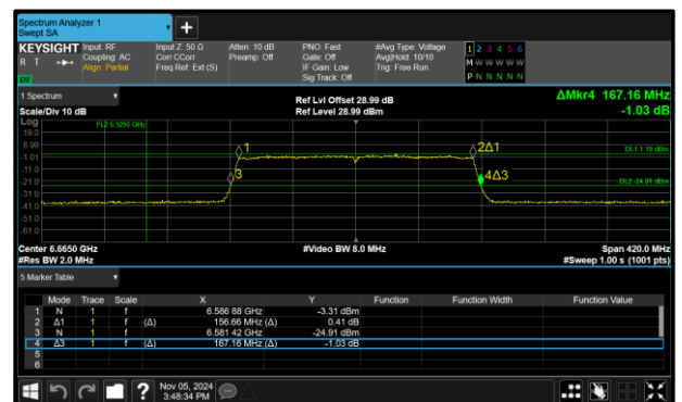
Figure 20 - 802.11ax HE160 SU VLP Maximum 26 dB EBW
