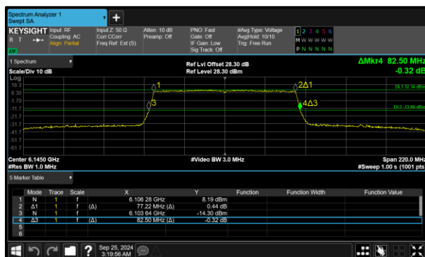
Figure 79 - 802.11ax HE80 SU SP Minimum 26 dB EBW
