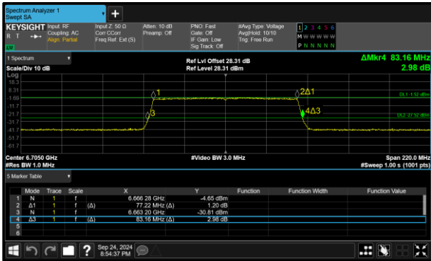
Figure 110 - 802.11ax HE80 SU LPI Maximum 26 dB EBW
