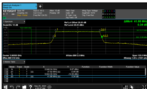
Figure 123 - 802.11ax HE40 SU SP Minimum 26 dB EBW
