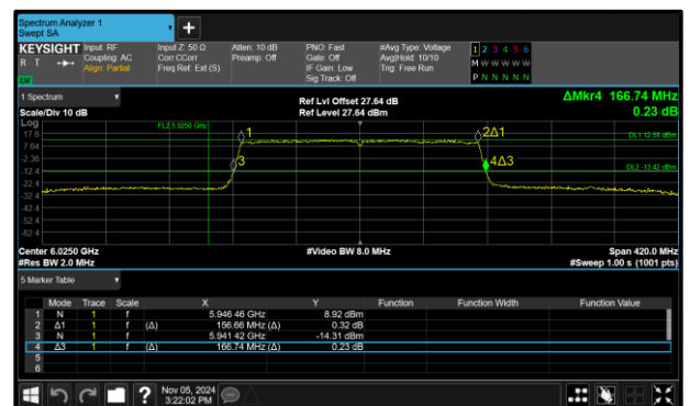
Figure 104 - 802.11ax HE160 SU SP Maximum 99% OBW
