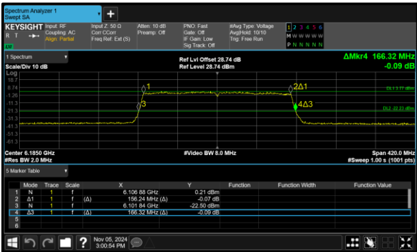
Figure 111 - 802.11ax HE160 SU LPI Minimum 26 dB EBW
