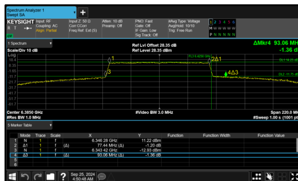
Figure 126 - 802.11ax HE80 SU SP Maximum 26 dB EBW
