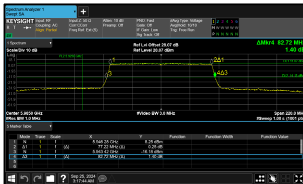
Figure 101 - 802.11ax HE80 SU SP Minimum 99% OBW
