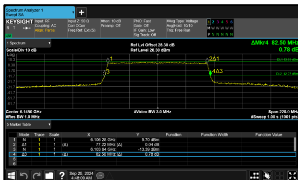
Figure 125 - 802.11ax HE80 SU SP Minimum 26 dB EBW
