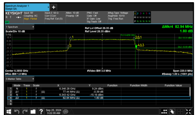
Figure 102 - 802.11ax HE80 SU SP Maximum 99% OBW
