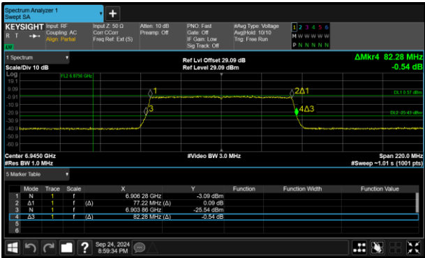
Figure 109 - 802.11ax HE80 SU LPI Minimum 26 dB EBW
