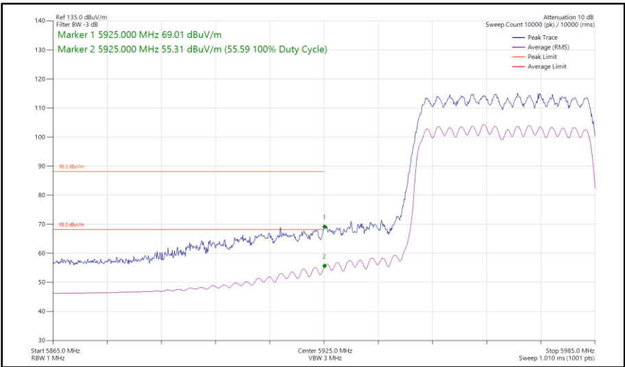
Figure 205 - 802.11ax HE40, SU, CDD, Core 0 - Core 1 - 5965 MHz Band Edge Frequency 5925 MHz
