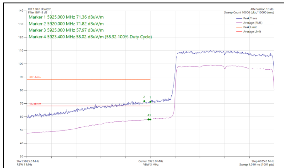
Figure 215 - 802.11ax HE80, SU, SISO, Core 0 - 5985 MHz Band Edge Frequency 5925 MHz
