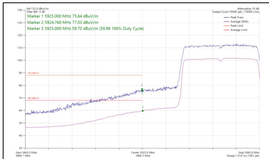
Figure 197 - 802.11ax HE40, SU, SISO, Core 0 - 5965 MHz Band Edge Frequency 5925 MHz
