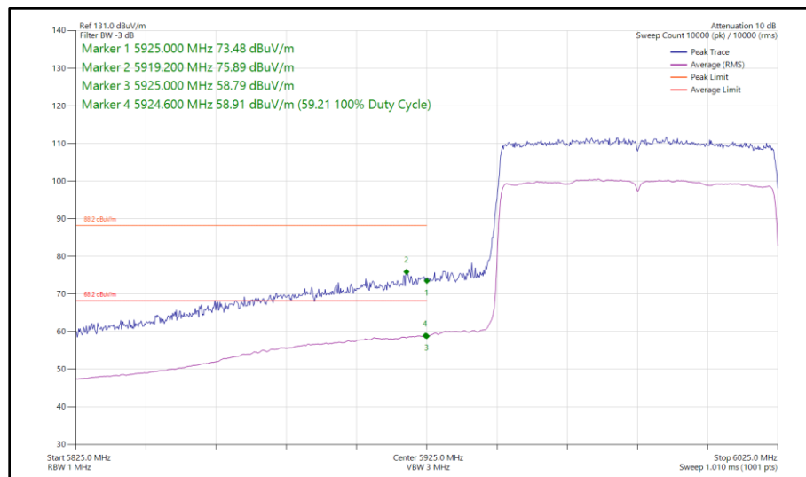
Figure 219 - 802.11ax HE80, SU, SISO, Core 1 - 5985 MHz Band Edge Frequency 5925 MHz
