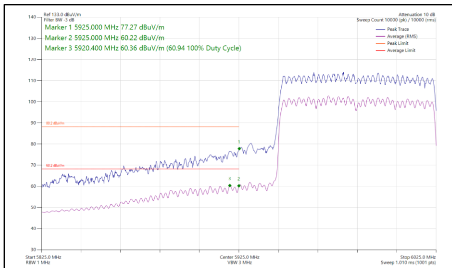
Figure 223 - 802.11ax HE80, SU, CDD, Core 0 - Core 1 - 5985 MHz Band Edge Frequency 5925 MHz
