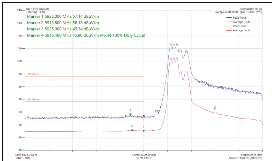
Figure 224 - 802.11ax HE80, RU 106-53, CDD, Core 0 - Core 1 - 5985 MHz Band Edge Frequency 5925 MHz
