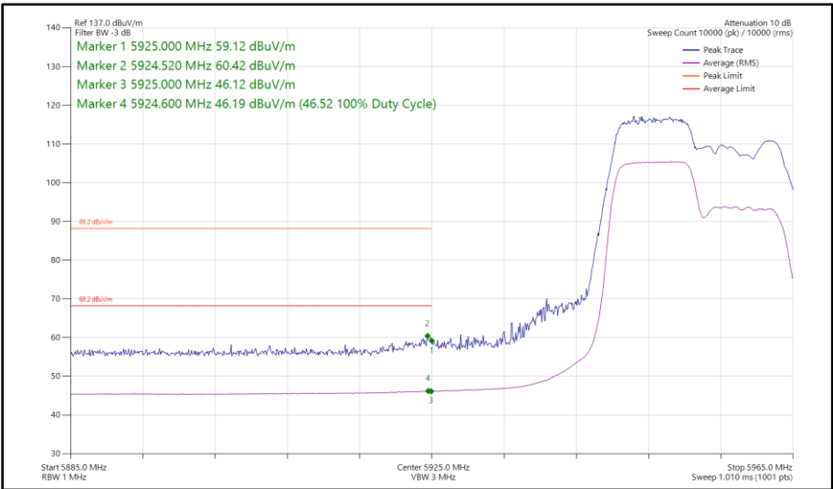
Figure 184 - 802.11ax HE20, RU 106-53, SISO, Core 1 - 5955 MHz Band Edge Frequency 5925 MHz
