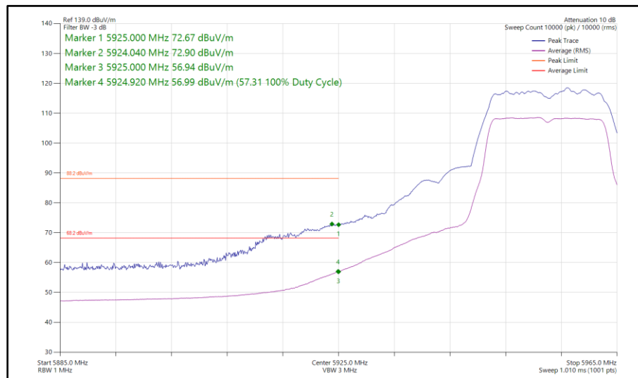
Figure 182 - 802.11a, SISO, Core 1 - 5955 MHz Band Edge Frequency 5925 MHz
