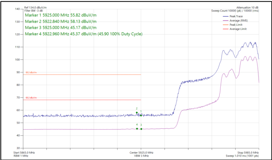
Figure 206 - 802.11ax HE40, RU 106-56, CDD, Core 0 - Core 1 - 5965 MHz Band Edge Frequency 5925 MHz
