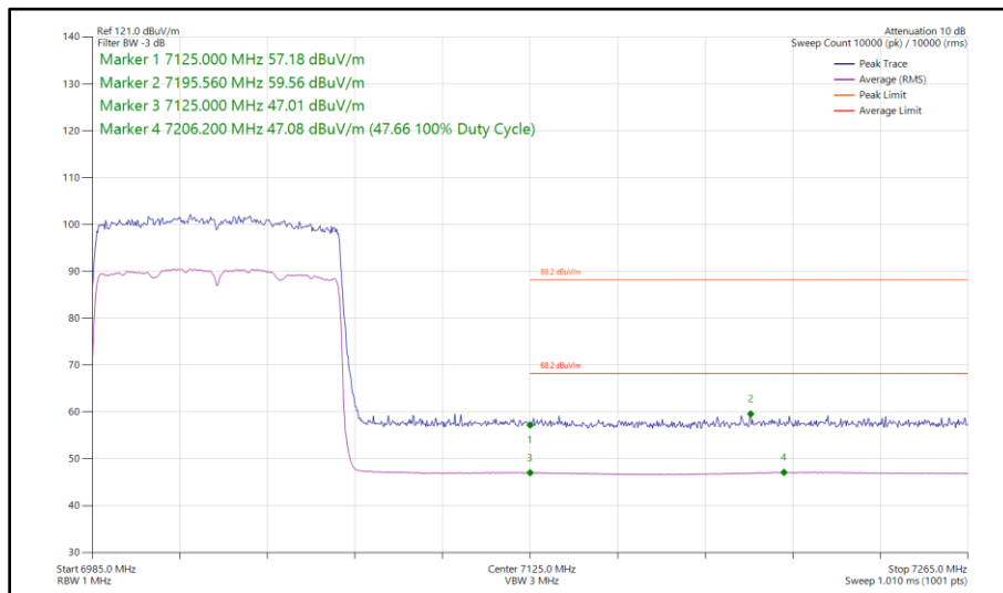
Figure 217 - 802.11ax HE80, SU, SISO, Core 0 - 7025 MHz Band Edge Frequency 7125 MHz
