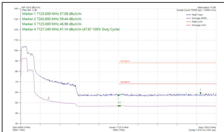
Figure 218 - 802.11ax HE80, RU 106-53, SISO, Core 0 - 7025 MHz Band Edge Frequency 7125 MHz
