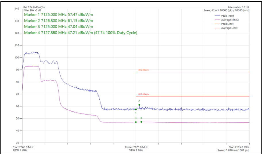
Figure 200 - 802.11ax HE40, RU 106-53, SISO, Core 0 - 7085 MHz Band Edge Frequency 7125 MHz
