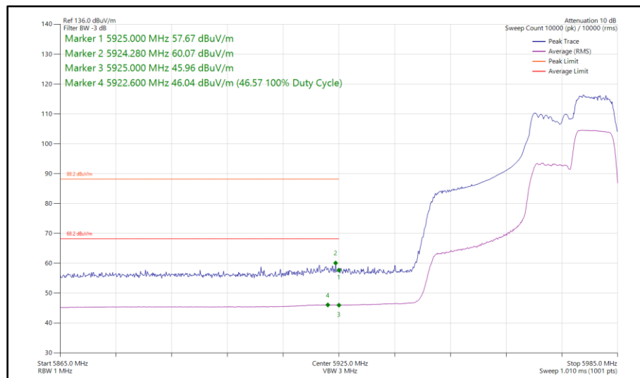
Figure 202 - 802.11ax HE40, RU 106-56, SISO, Core 1 - 5965 MHz Band Edge Frequency 5925 MHz
