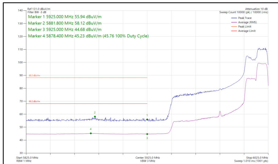
Figure 216 - 802.11ax HE80, RU 106-60, SISO, Core 0 - 5985 MHz Band Edge Frequency 5925 MHz
