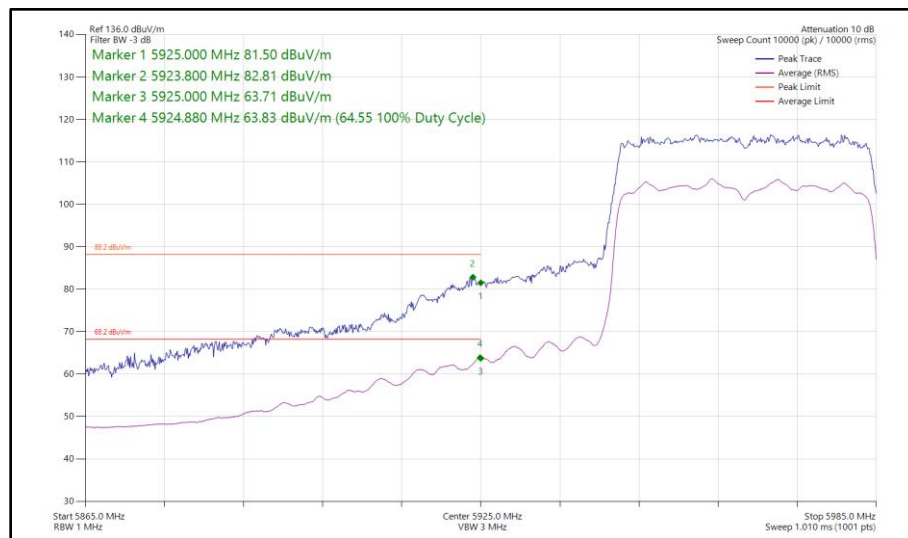
Figure 209 - 802.11ax HE40, SU, SDM, Core 0 - Core 1 - 5965 MHz Band Edge Frequency 5925 MHz
