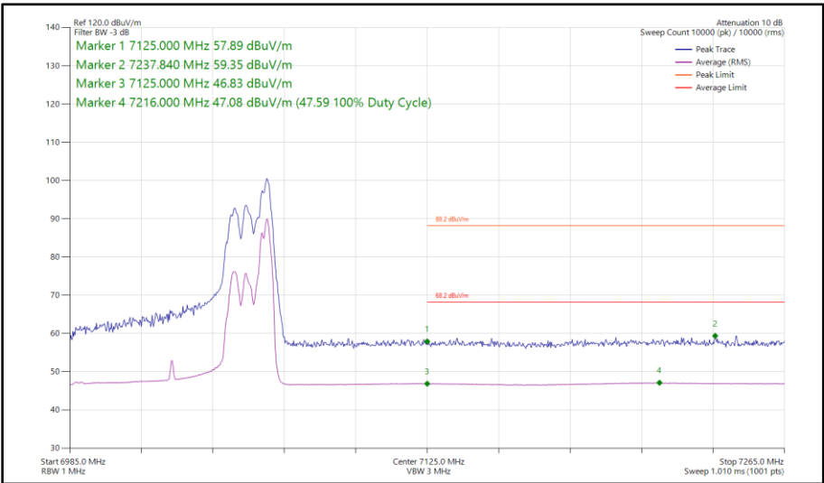
Figure 226 - 802.11ax HE80, RU 52-52, CDD, Core 0 - Core 1 - 7025 MHz Band Edge Frequency 7125 MHz
