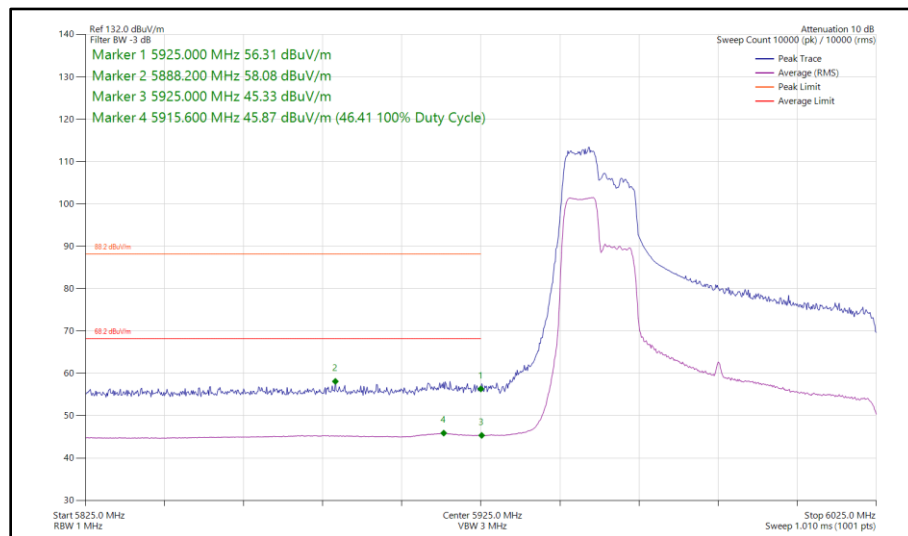
Figure 220 - 802.11ax HE80, RU 106-53, SISO, Core 1 - 5985 MHz Band Edge Frequency 5925 MHz
