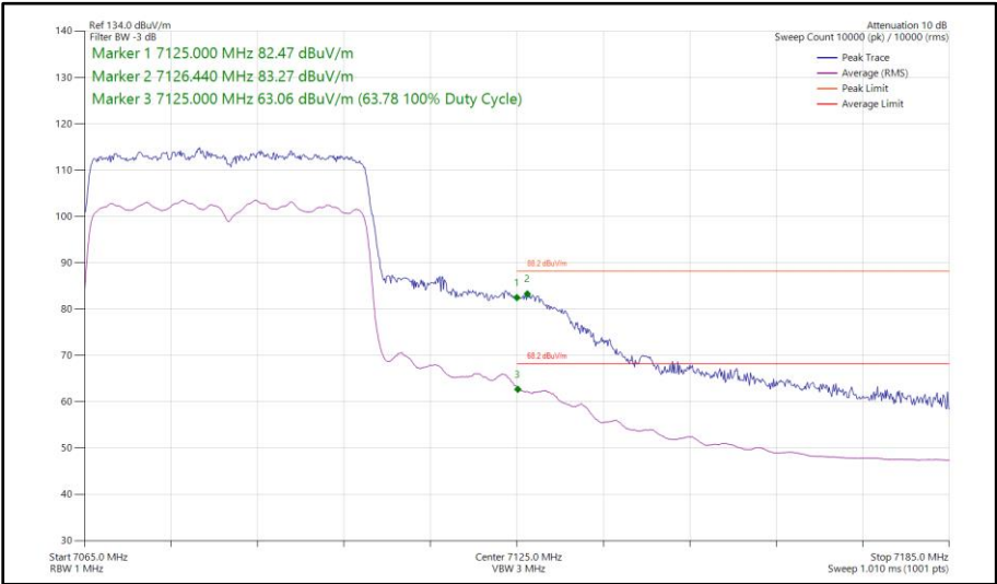
Figure 211 - 802.11ax HE40, SU, SDM, Core 0 - Core 1 - 7085 MHz Band Edge Frequency 7125 MHz
