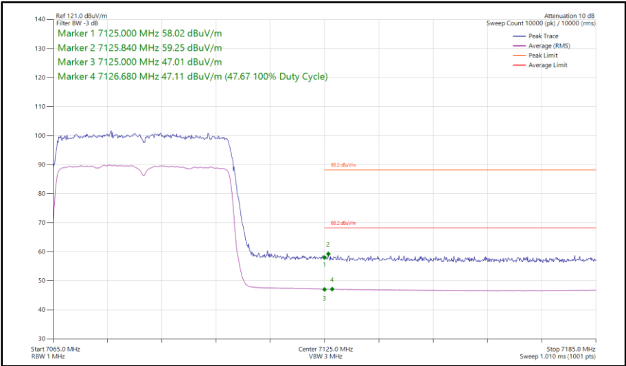
Figure 199 - 802.11ax HE40, SU, SISO, Core 0 - 7085 MHz Band Edge Frequency 7125 MHz
