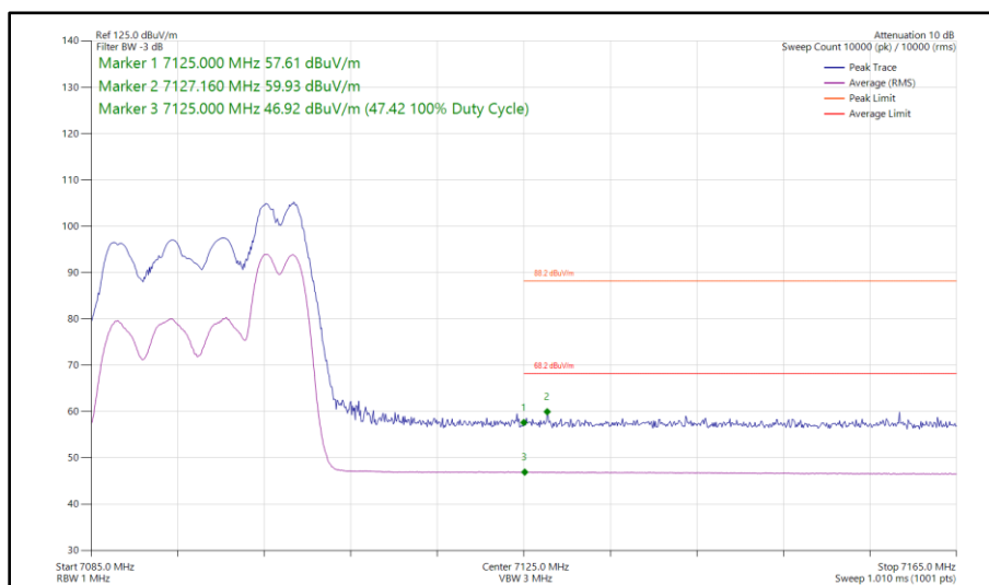
Figure 195 - 802.11ax HE20, RU 52-40, SDM, Core 0 - Core 1 - 7095 MHz Band Edge Frequency 7125 MHz
