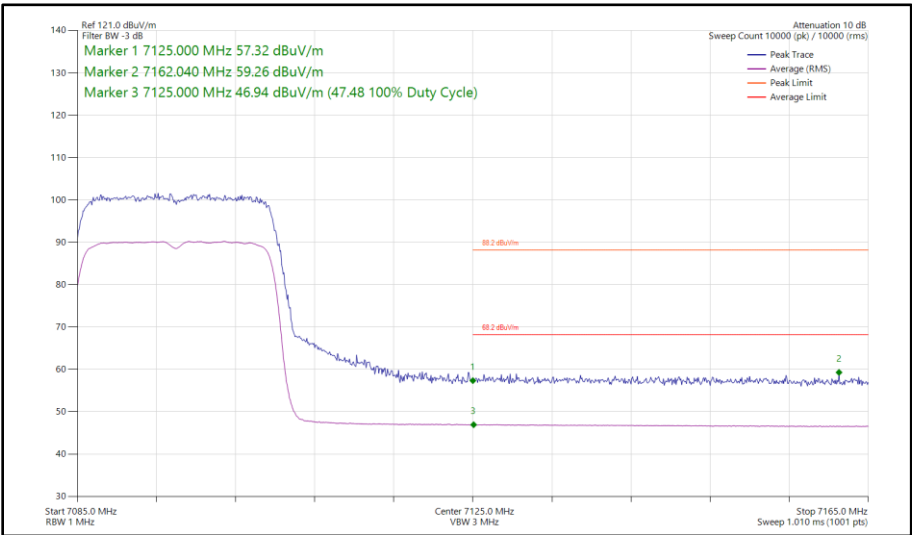
Figure 186 - 802.11ax HE20, SU, SISO, Core 1 - 7095 MHz Band Edge Frequency 7125 MHz
