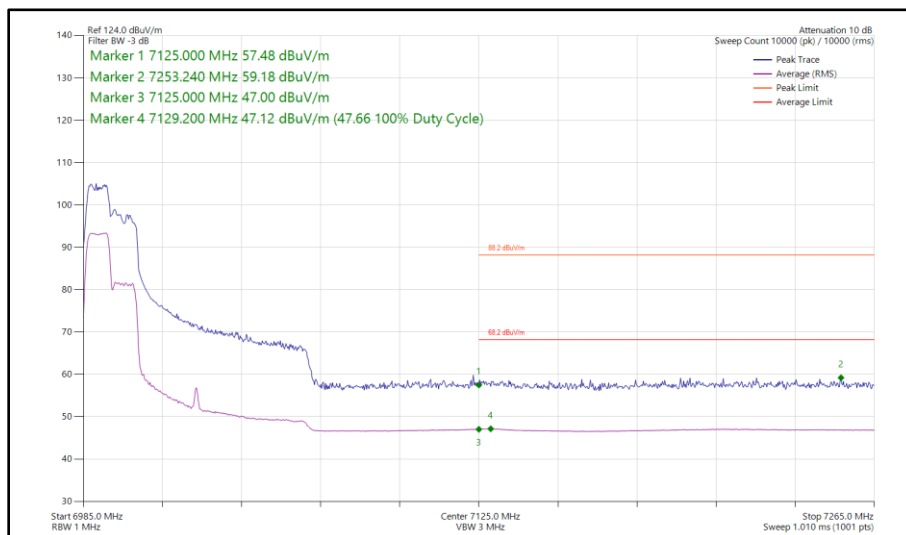
Figure 222 - 802.11ax HE80, RU 106-53, SISO, Core 1 - 7025 MHz Band Edge Frequency 7125 MHz
