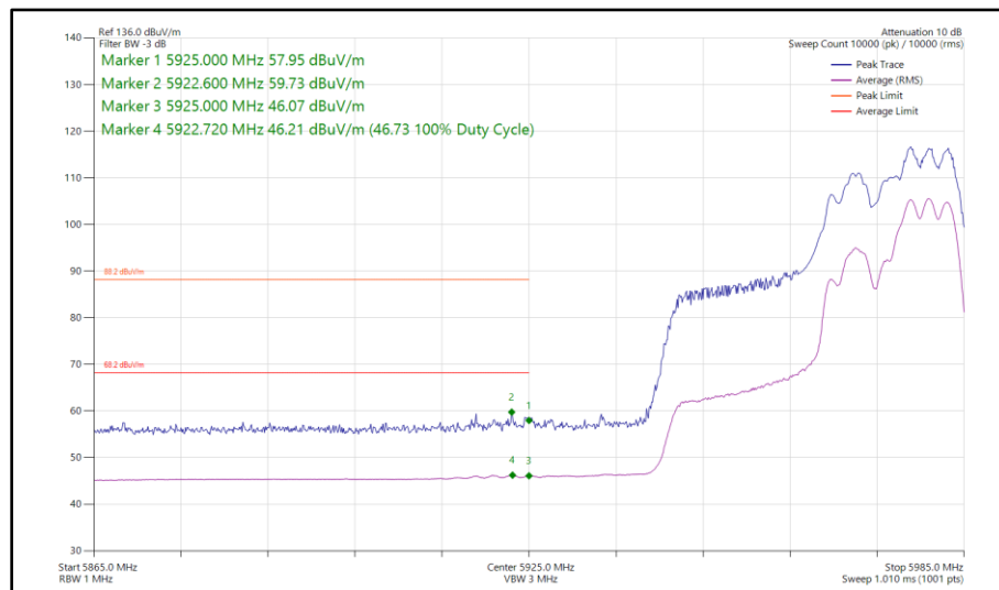
Figure 210 - 802.11ax HE40, RU 106-56, SDM, Core 0 - Core 1 - 5965 MHz Band Edge Frequency 5925 MHz
