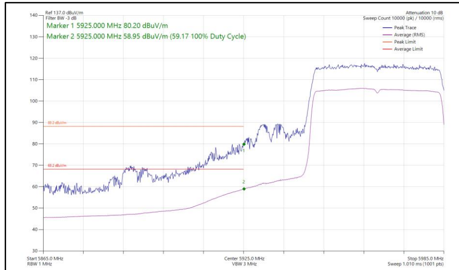
Figure 213 - 802.11ax HE40, SU, TxBF, Core 0 - Core 1 - 5965 MHz Band Edge Frequency 5925 MHz
