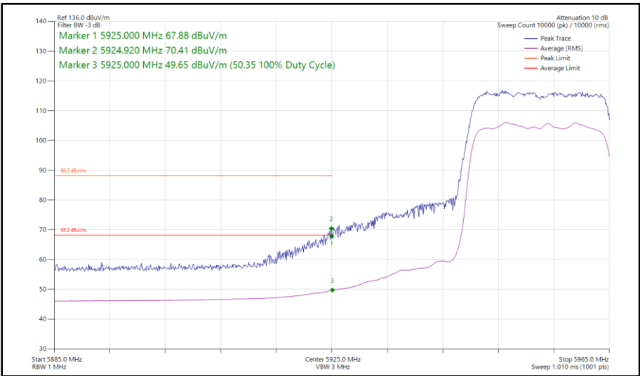
Figure 192 - 802.11ax HE20, SU, SDM, Core 0 - Core 1 - 5955 MHz Band Edge Frequency 5925 MHz
