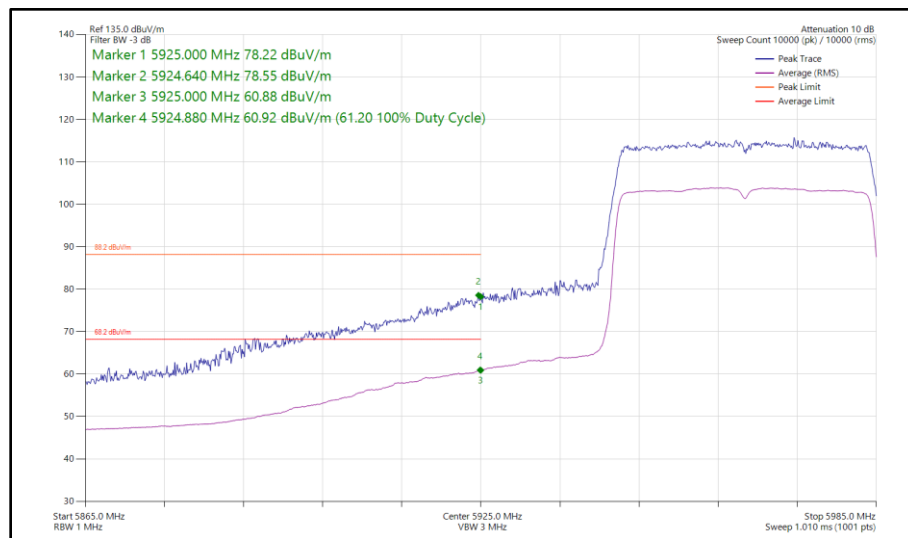
Figure 201 - 802.11ax HE40, SU, SISO, Core 1 - 5965 MHz Band Edge Frequency 5925 MHz
