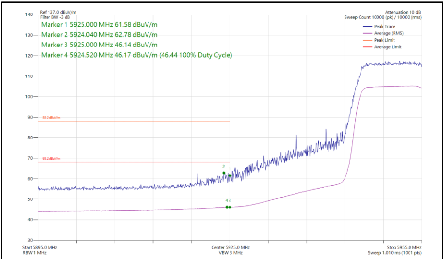
Figure 196 - 802.11ax HE20, SU, TxBF, Core 0 - Core 1 - 5935 MHz Band Edge Frequency 5925 MHz
