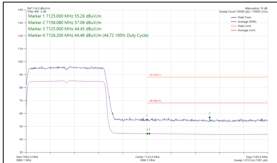
Figure 214 - 802.11ax HE40, SU, TxBF, Core 0 - Core 1 - 7085 MHz Band Edge Frequency 7125 MHz
