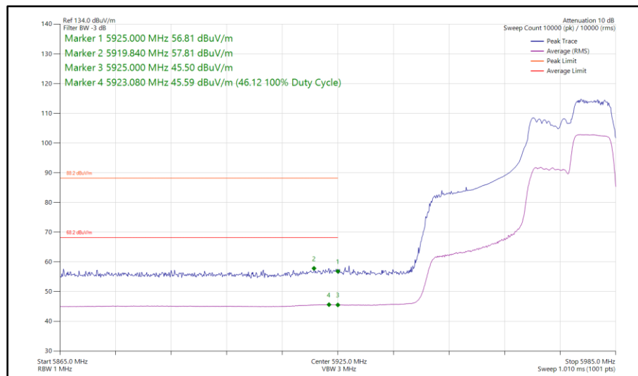
Figure 198 - 802.11ax HE40, RU 106-56, SISO, Core 0 - 5965 MHz Band Edge Frequency 5925 MHz
