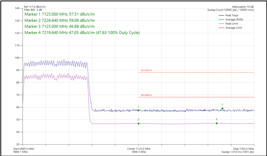
Figure 225 - 802.11ax HE80, SU, CDD, Core 0 - Core 1 - 7025 MHz Band Edge Frequency 7125 MHz
