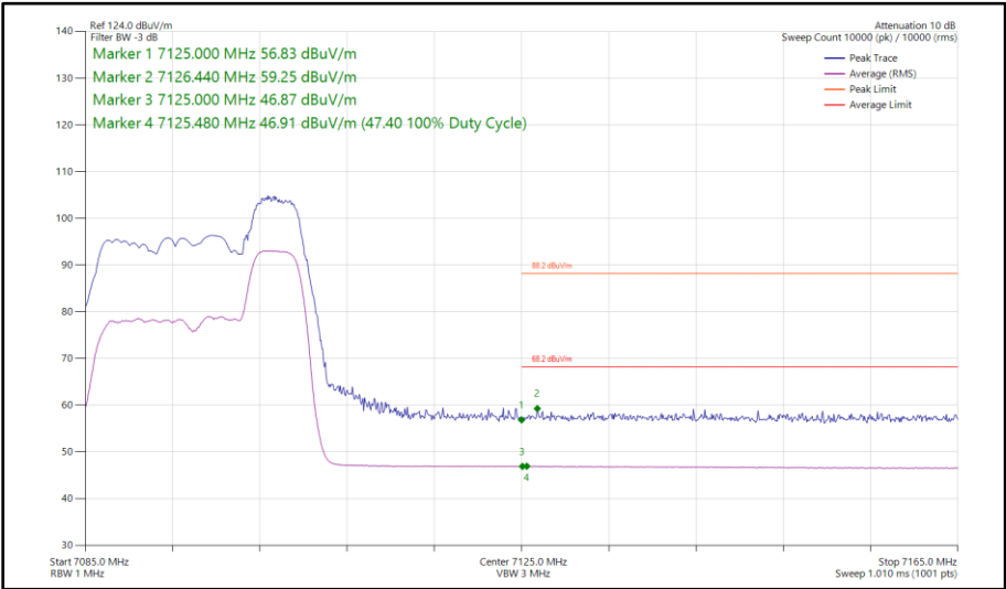
Figure 187 - 802.11ax HE20, RU 52-40, SISO, Core 1 - 7095 MHz Band Edge Frequency 7125 MHz
