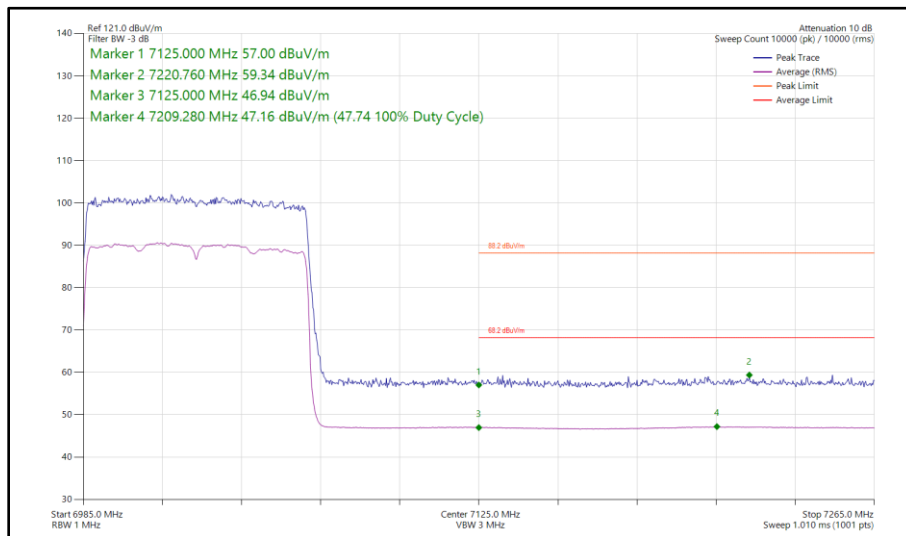
Figure 221 - 802.11ax HE80, SU, SISO, Core 1 - 7025 MHz Band Edge Frequency 7125 MHz
