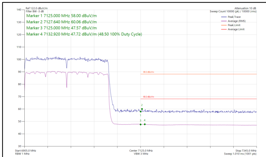
Figure 235 - 802.11ax HE160, SU, SISO, Core 0 - 6985 MHz Band Edge Frequency 7125 MHz
