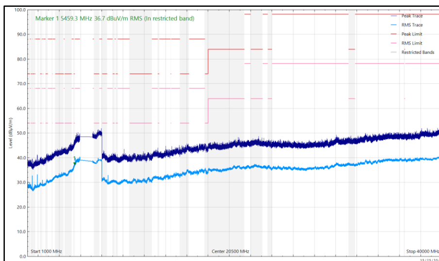
Figure 259 - 6435 MHz (CH97), HE20, SU, CDD, Core 0 + Core 1, 1 GHz to 40 GHz, Vertical
