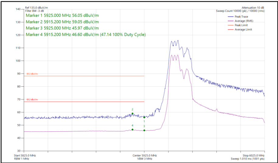
Figure 228 - 802.11ax HE80, RU 106-53, SDM, Core 0 - Core 1 - 5985 MHz Band Edge Frequency 5925 MHz
