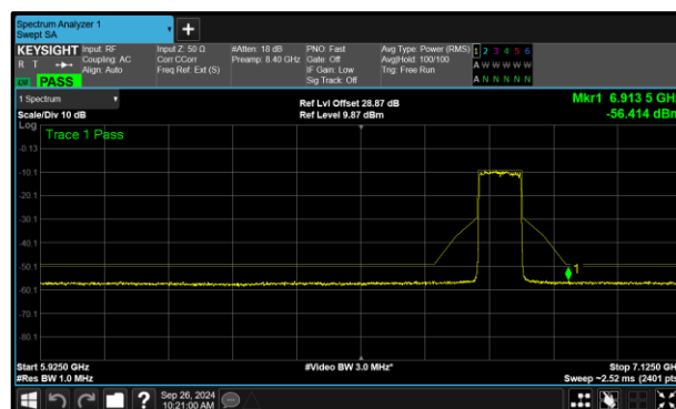
Figure 285 - A (Core 0) 802.11ax HE80 SU LPI 6785 MHz (CH167)
