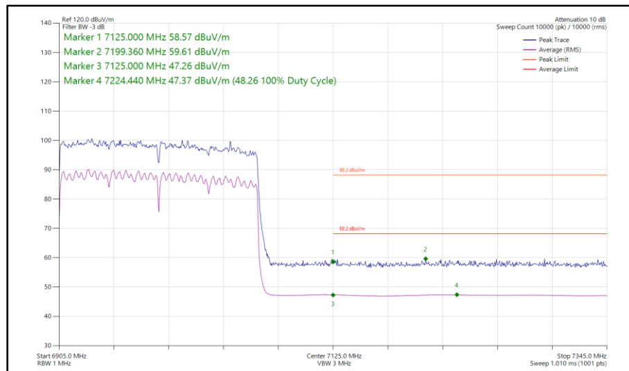
Figure 247 - 802.11ax HE160, SU, SDM, Core 0 - Core 1 - 6985 MHz Band Edge Frequency 7125 MHz
