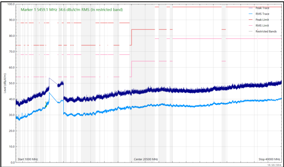
Figure 256 - 6415 MHz (CH93), HE20, SU, CDD, Core 0 + Core 1, 1 GHz to 40 GHz, Horizontal
