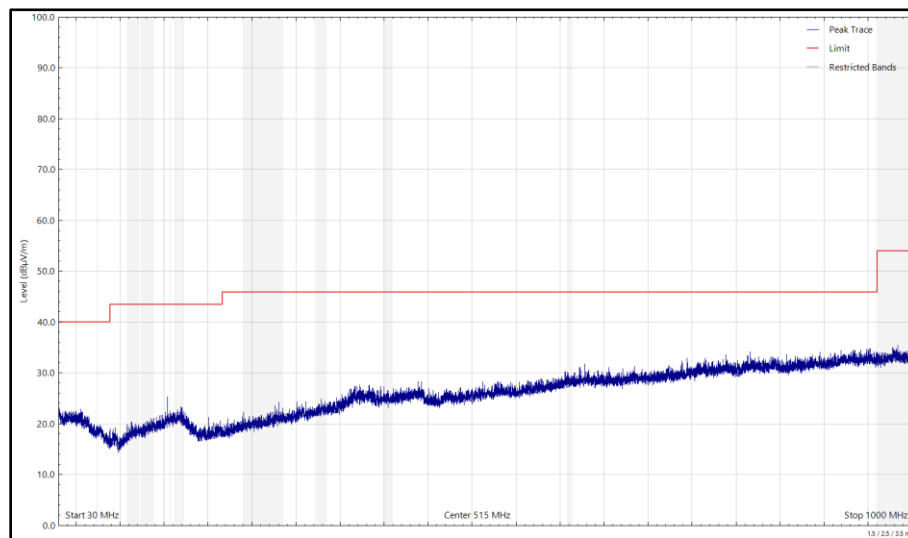
Figure 276 - 6995 MHz (CH209), HE20, SU, CDD, Core 0 + Core 1, 30 MHz to 1 GHz, Horizontal (Peak)
