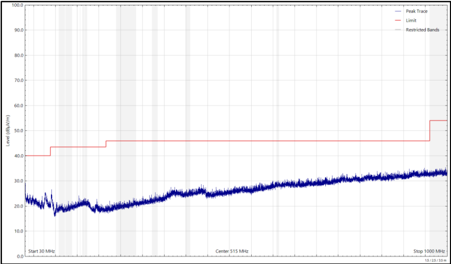
Figure 278 - 6995 MHz (CH209), HE20, SU, CDD, Core 0 + Core 1, 30 MHz to 1 GHz, Vertical (Peak)
