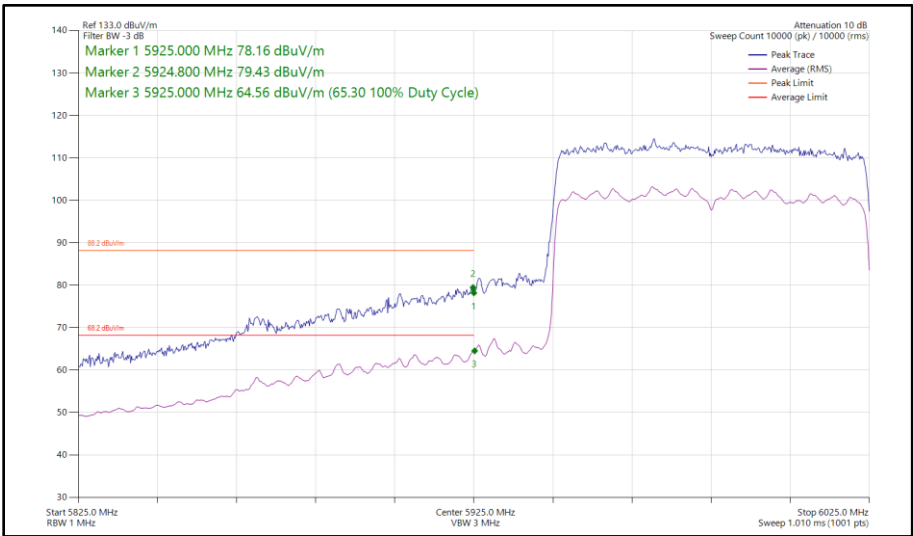
Figure 227 - 802.11ax HE80, SU, SDM, Core 0 - Core 1 - 5985 MHz Band Edge Frequency 5925 MHz
