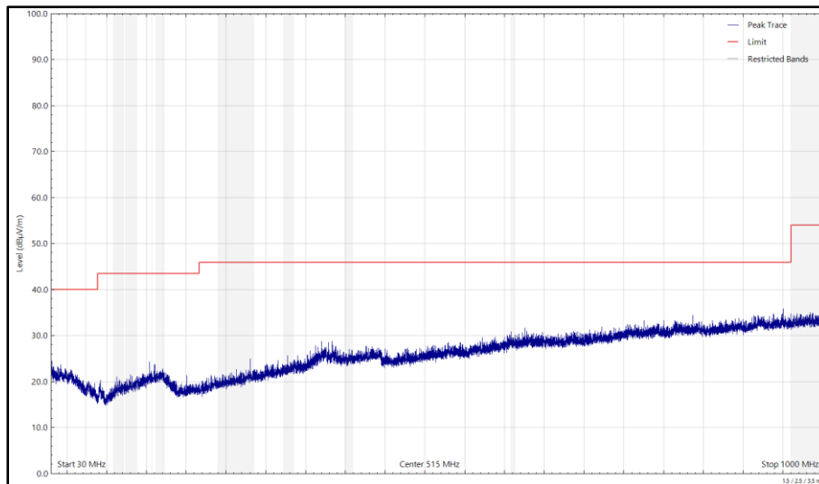
Figure 268 - 6695 MHz (CH149), HE20, SU, CDD, Core 0 + Core 1, 30 MHz to 1 GHz, Horizontal (Peak)
