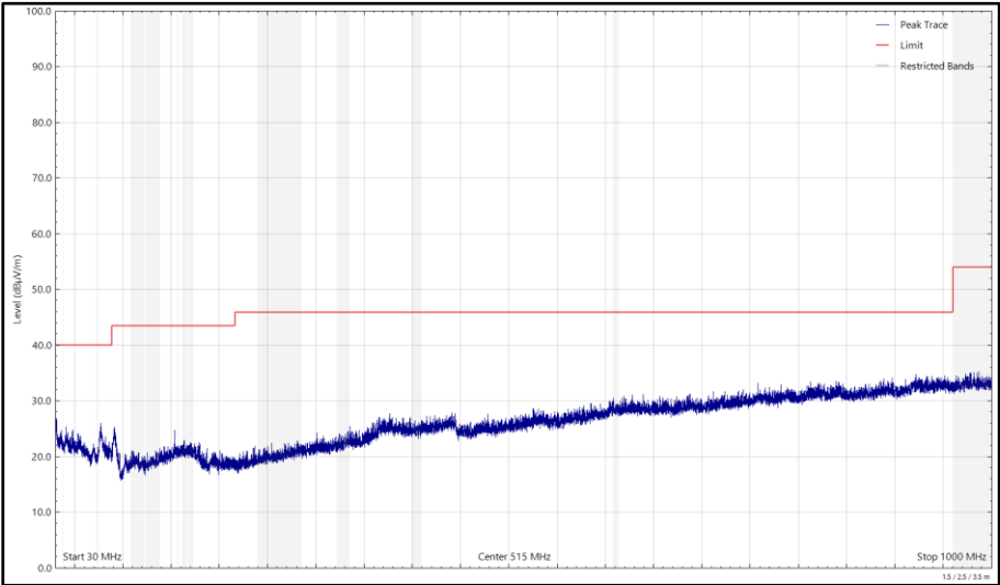
Figure 270 - 6695 MHz (CH149), HE20, SU, CDD, Core 0 + Core 1, 30 MHz to 1 GHz, Vertical (Peak)
