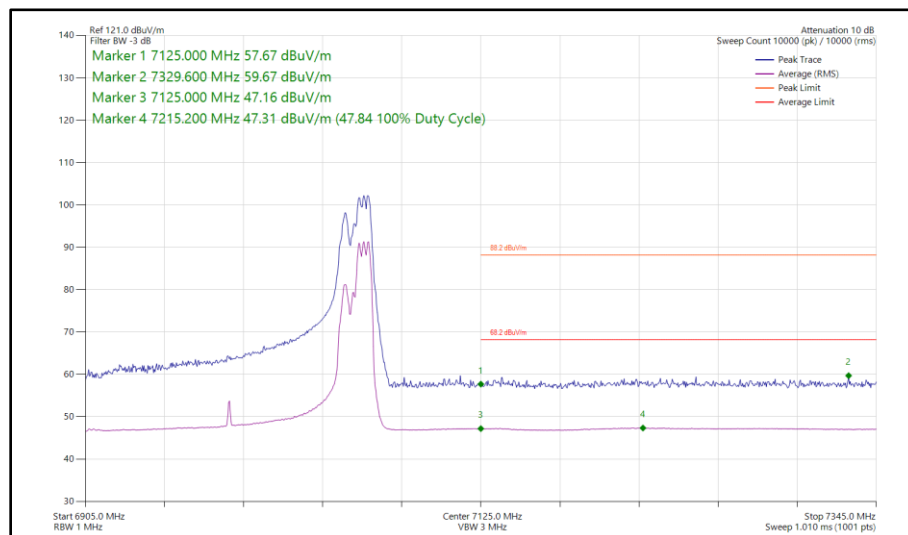
Figure 248 - 802.11ax HE160, RU 106-60S, SDM, Core 0 - Core 1 - 6985 MHz Band Edge Frequency 7125 MHz
