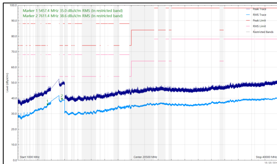
Figure 272 - 6855 MHz (CH181), HE20, SU, CDD, Core 0 + Core 1, 1 GHz to 40 GHz, Horizontal
