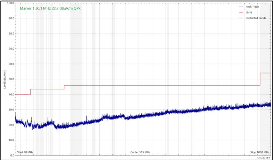
Figure 254 - 6175 MHz (CH45), HE20, SU, CDD, Core 0 + Core 1, 30 MHz to 1 GHz, Vertical (Peak)
