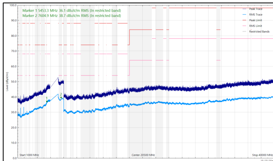
Figure 273 - 6855 MHz (CH181), HE20, SU, CDD, Core 0 + Core 1, 1 GHz to 40 GHz, Vertical
