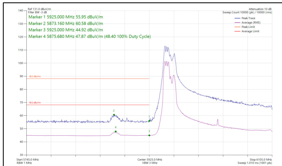
Figure 246 - 802.11ax HE160, RU 106-53P, SDM, Core 0 - Core 1 - 6025 MHz Band Edge Frequency 5925 MHz
