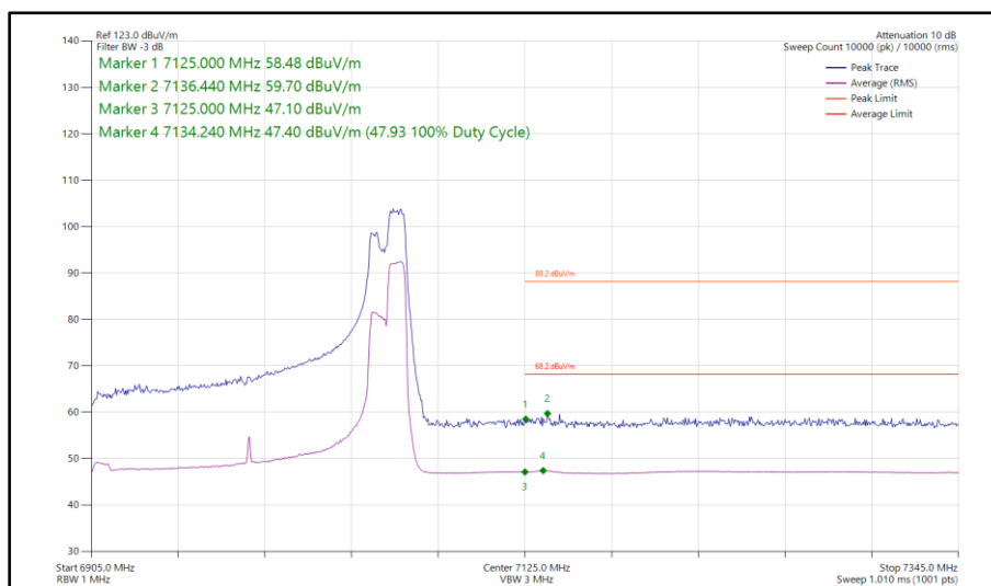
Figure 240 - 802.11ax HE160, RU 106-60S, SISO, Core 1 - 6985 MHz Band Edge Frequency 7125 MHz
