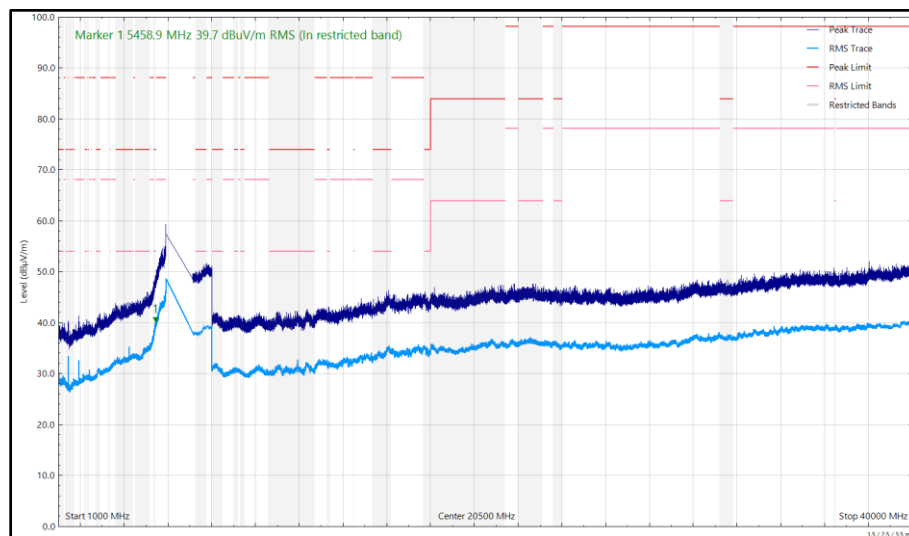
Figure 251 - 5955 MHz (CH1), HE20, SU, CDD, Core 0 + Core 1, 1 GHz to 40 GHz, Vertical
