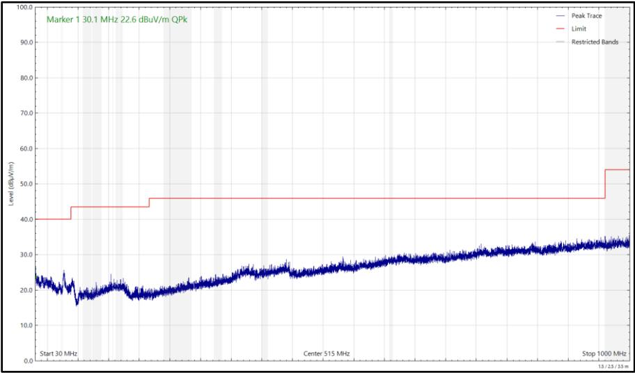
Figure 262 - 6475 MHz (CH105), HE20, SU, CDD, Core 0 + Core 1, 30 MHz to 1 GHz, Vertical (Peak)
