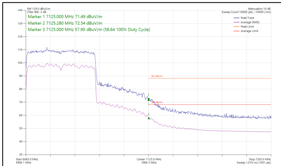
Figure 229 - 802.11ax HE80, SU, SDM, Core 0 - Core 1 - 7025 MHz Band Edge Frequency 7125 MHz
