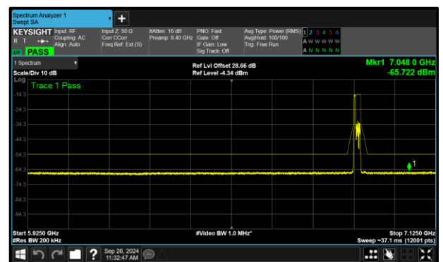
Figure 289 - B (Core 1) 802.11ax HE20 RU52 LPI 6895 MHz (CH189)
