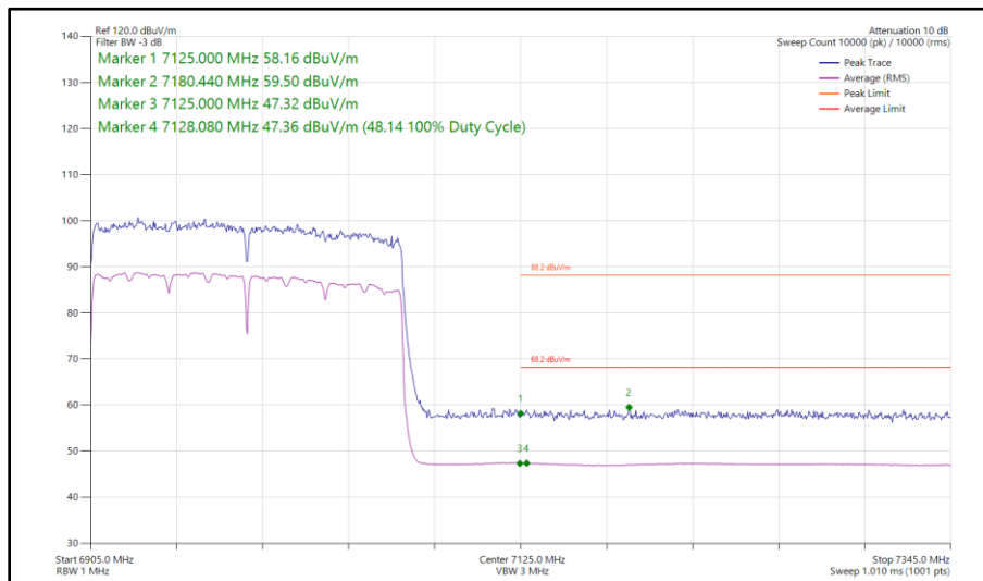
Figure 239 - 802.11ax HE160, SU, SISO, Core 1 - 6985 MHz Band Edge Frequency 7125 MHz
