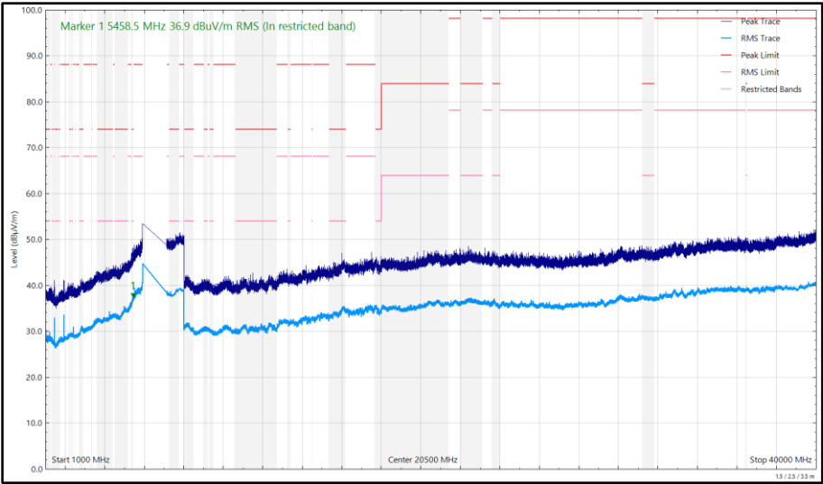
Figure 257 - 6415 MHz (CH93), HE20, SU, CDD, Core 0 + Core 1, 1 GHz to 40 GHz, Vertical
