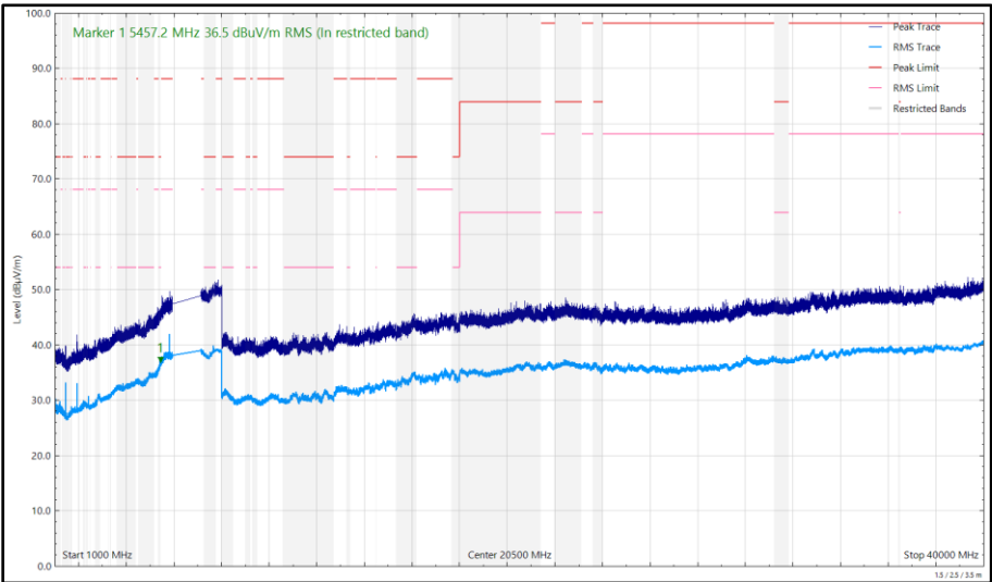
Figure 271 - 6695 MHz (CH149), HE20, SU, CDD, Core 0 + Core 1, 1 GHz to 40 GHz, Vertical
