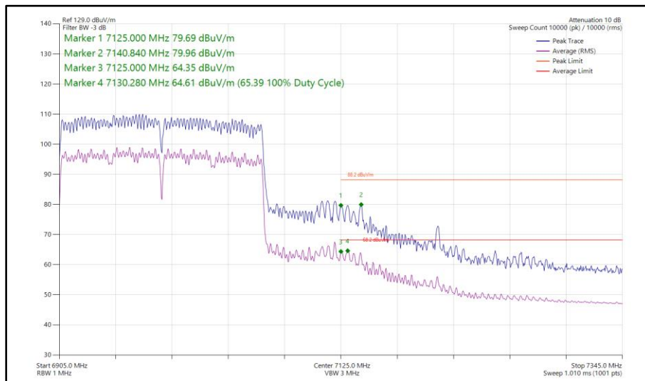
Figure 243 - 802.11ax HE160, SU, CDD, Core 0 - Core 1 - 6985 MHz Band Edge Frequency 7125 MHz
